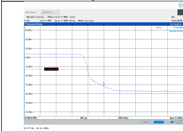
Band5-5MHz-QPSK-20625-25RB#0
