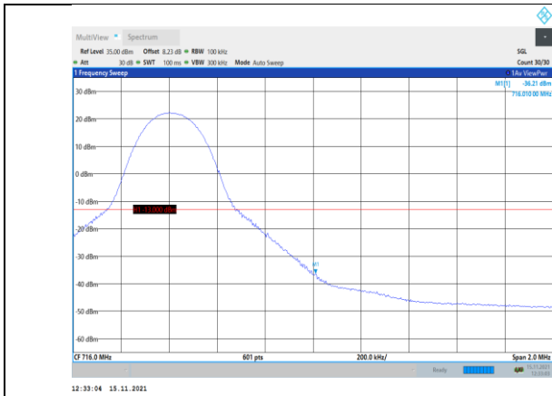
Band12-10MHz-QPSK-23130-1RB#49
