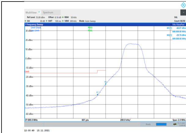
Band12-5MHz-16QAM-23035-1RB#0
