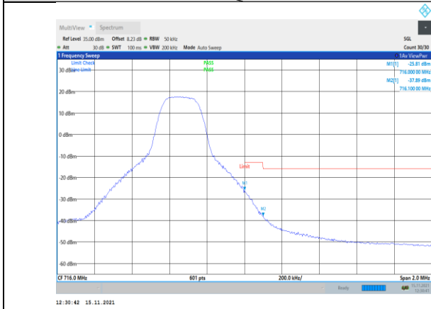
Band12-5MHz-16QAM-23155-1RB#24
