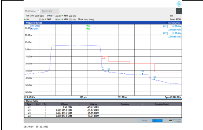
Band7-10MHz-QPSK-21400-50RB#0
