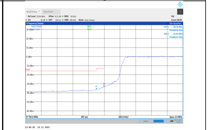
Band17-5MHz-16QAM-23755-25RB#0
