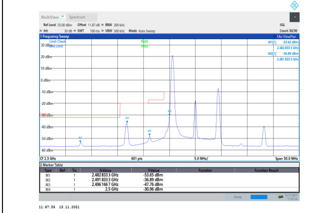
Band7-10MHz-16QAM-20800-1RB#0
