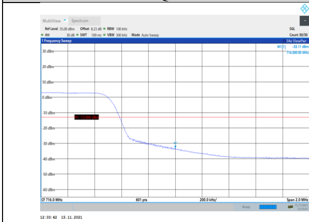
Band12-10MHz-QPSK-23130-50RB#0
