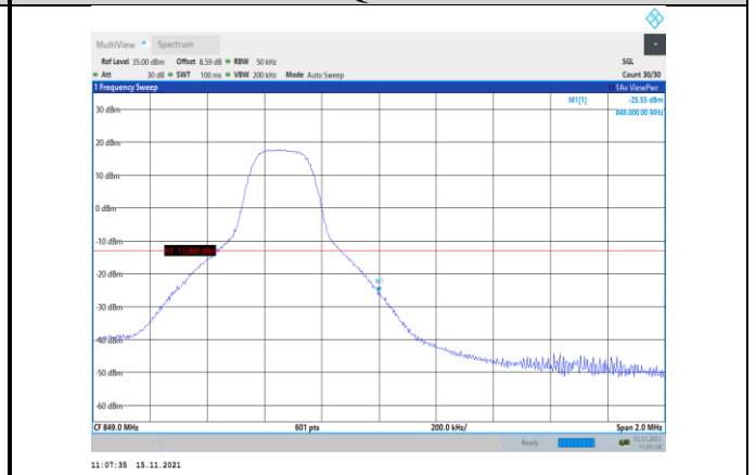
Band5-5MHz-16QAM-20625-1RB#24
