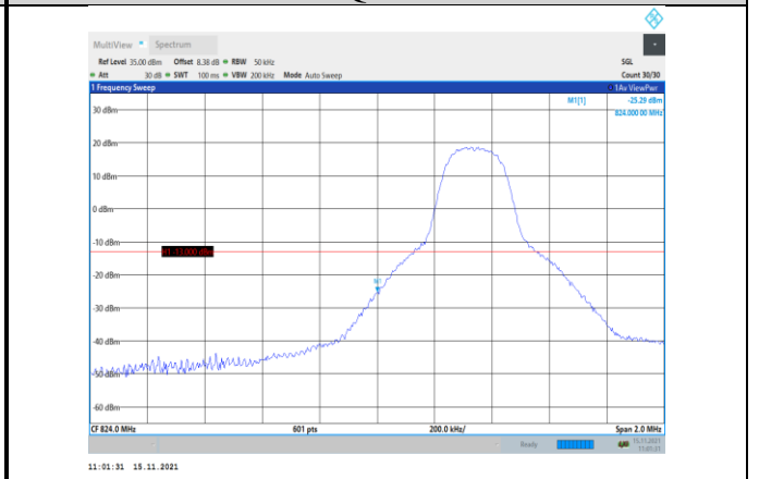
Band5-5MHz-QPSK-20425-1RB#0
