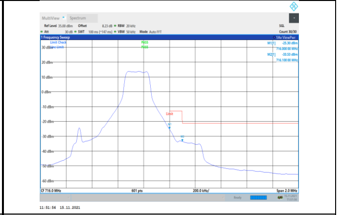
Band12-1.4MHz-16QAM-23173-1RB#5
