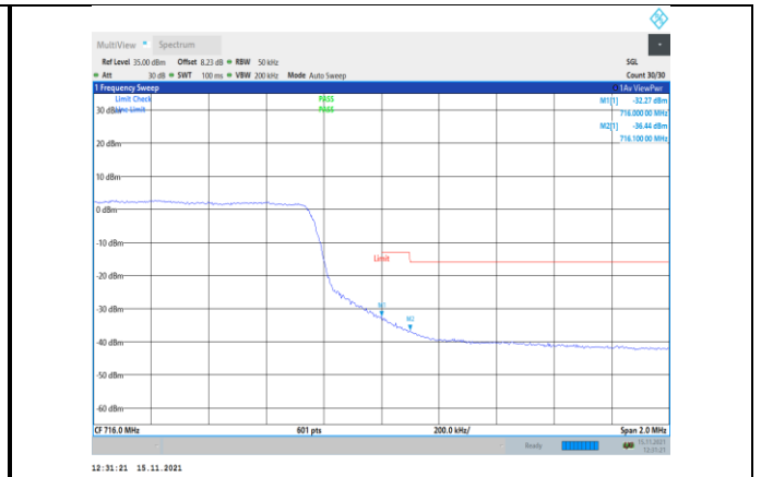
Band12-5MHz-16QAM-23155-25RB#0
