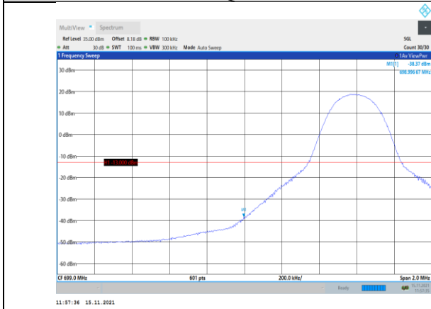
Band12-10MHz-16QAM-23060-1RB#0
