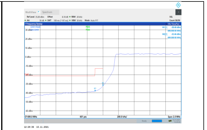
Band12-1.4MHz-16QAM-23017-6RB#0
