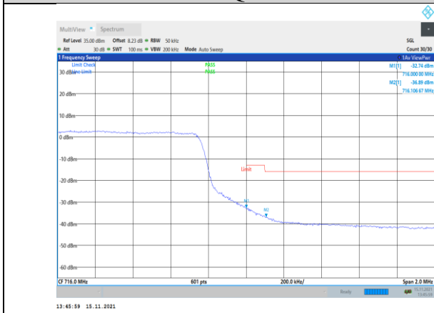
Band17-5MHz-16QAM-23825-25RB#0
