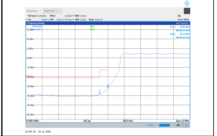
Band12-1.4MHz-QPSK-23017-6RB#0
