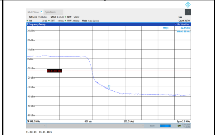
Band5-5MHz-16QAM-20625-25RB#0
