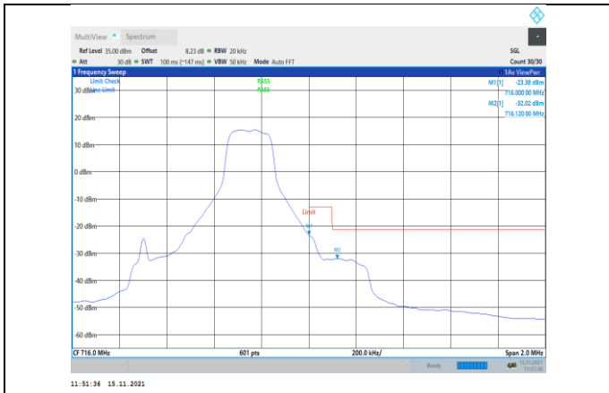
Band12-1.4MHz-QPSK-23173-1RB#5
