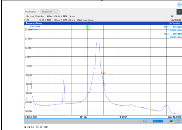
Band26-5MHz-16QAM-26765-1RB#24
