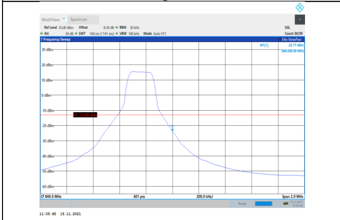
Band5-3MHz-16QAM-20635-1RB#14
