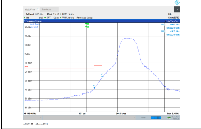
Band12-5MHz-QPSK-23035-1RB#0
