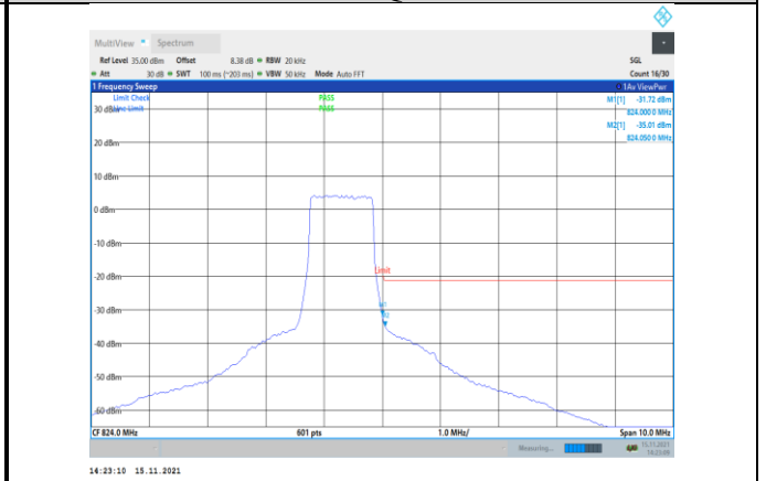
Band26-1.4MHz-16QAM-26783-6RB#0
