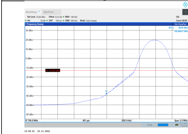
Band17-10MHz-QPSK-23780-1RB#0
