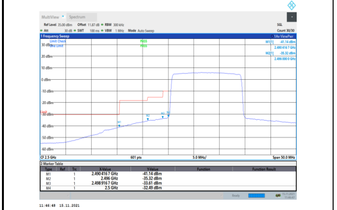
Band7-15MHz-16QAM-20825-75RB#0
