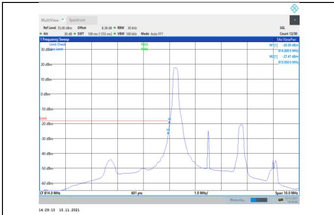
Band26-3MHz-QPSK-26705-1RB#0
