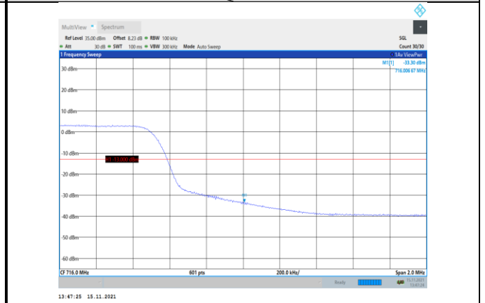
Band17-10MHz-QPSK-23800-50RB#0
