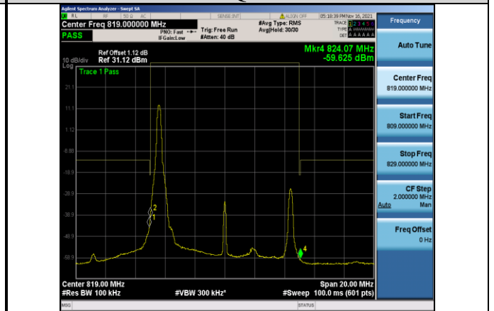
Band26-10MHz-QPSK-26740_Left-1RB#0
