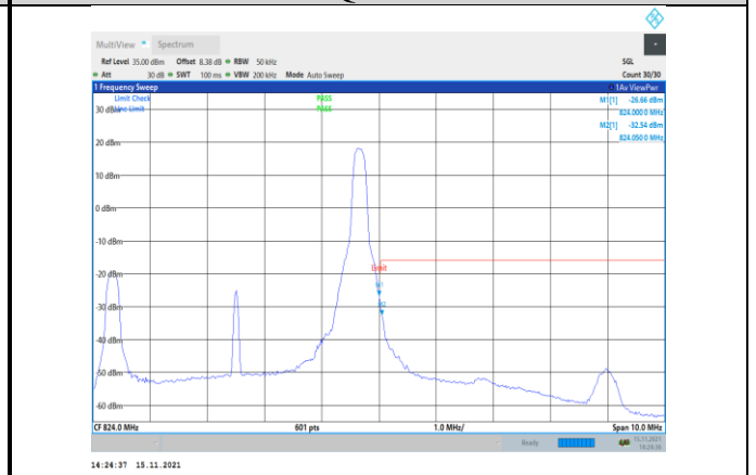
Band26-5MHz-QPSK-26765-1RB#24
