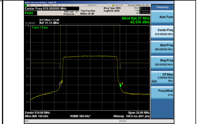
Band26-10MHz-QPSK-26740_Left-50RB#0
