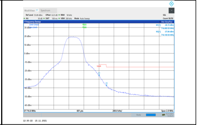
Band12-5MHz-QPSK-23155-1RB#24
