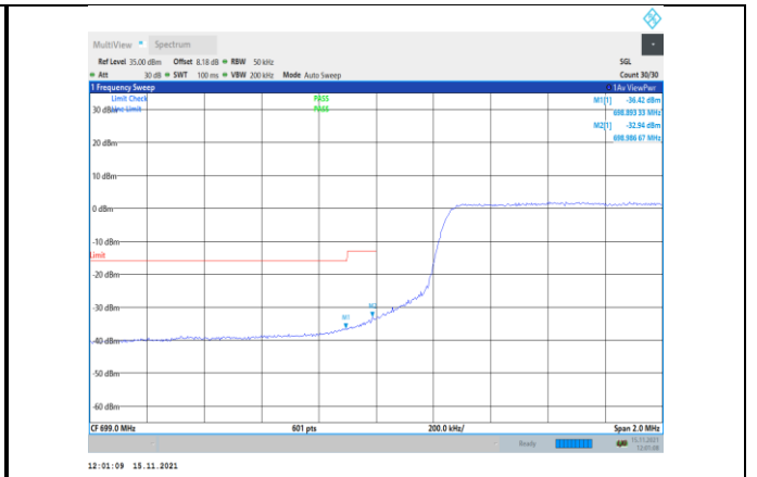
Band12-5MHz-QPSK-23035-25RB#0
