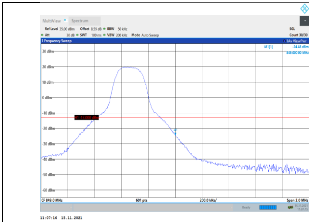
Band5-5MHz-QPSK-20625-1RB#24
