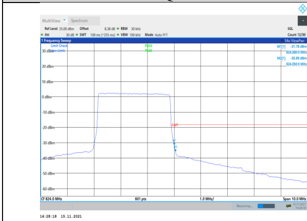
Band26-3MHz-16QAM-26775-15RB#0
