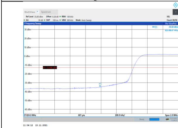
Band5-10MHz-QPSK-20450-50RB#0
