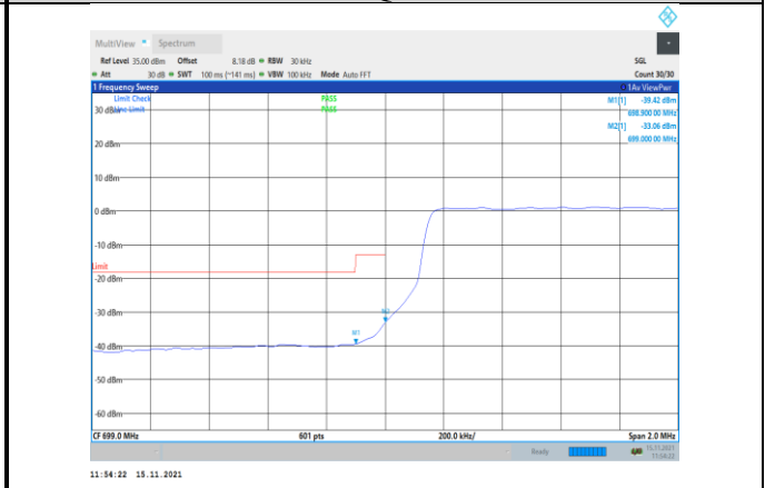
Band12-3MHz-16QAM-23025-15RB#0
