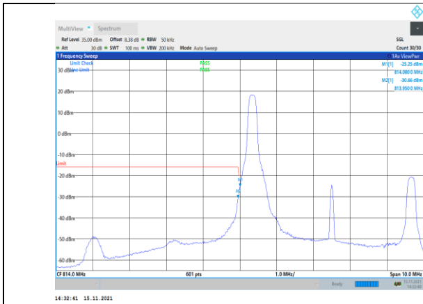
Band26-5MHz-16QAM-26715-1RB#0
