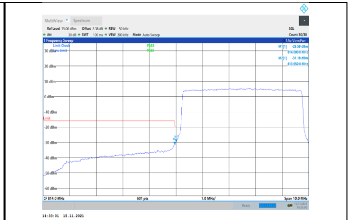
Band26-5MHz-QPSK-26715-25RB#0
