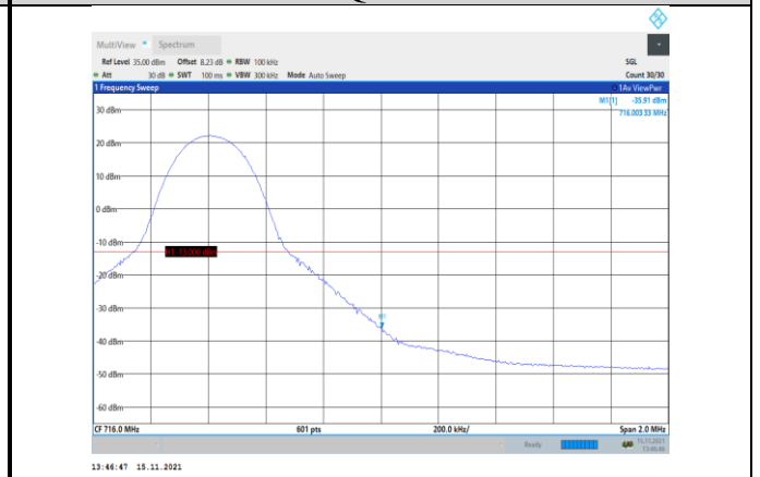
Band17-10MHz-QPSK-23800-1RB#49
