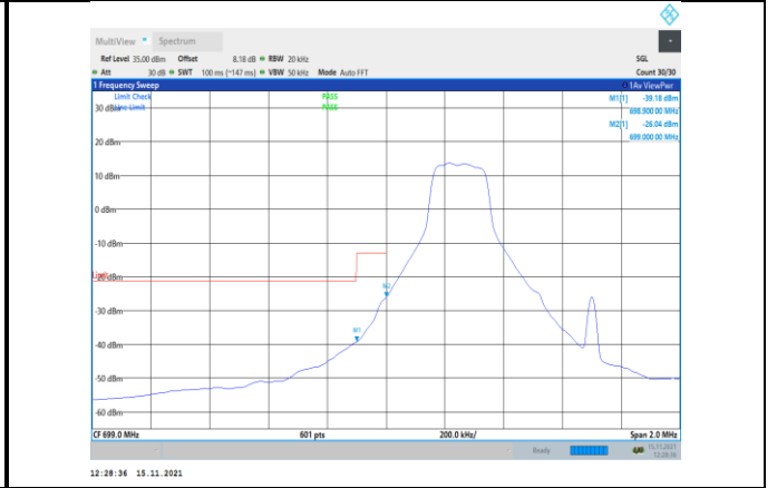
Band12-1.4MHz-QPSK-23017-1RB#0
