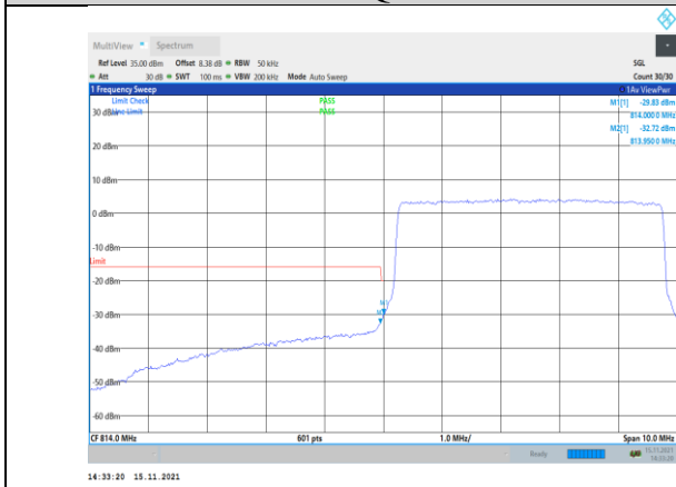
Band26-5MHz-16QAM-26715-25RB#0
