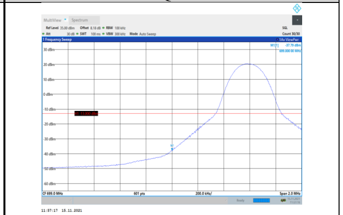
Band12-10MHz-QPSK-23060-1RB#0
