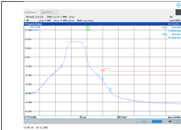
Band17-5MHz-16QAM-23825-1RB#24
