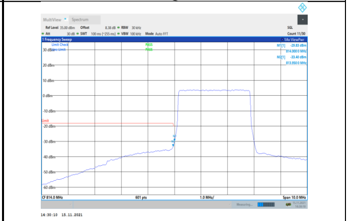
Band26-3MHz-16QAM-26705-15RB#0
