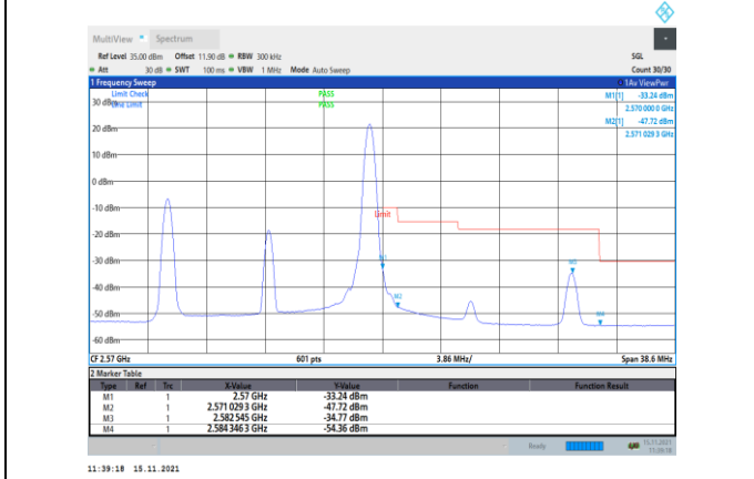
Band7-15MHz-QPSK-21375-1RB#74
