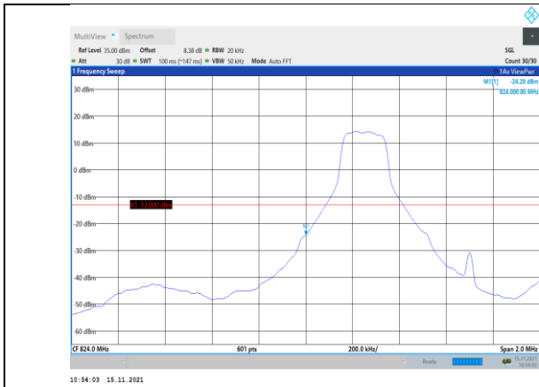
Band5-1.4MHz-QPSK-20407-1RB#0
