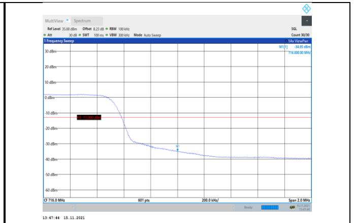
Band17-10MHz-16QAM-23800-50RB#0
