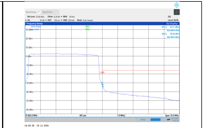
Band26-5MHz-16QAM-26765-25RB#0
