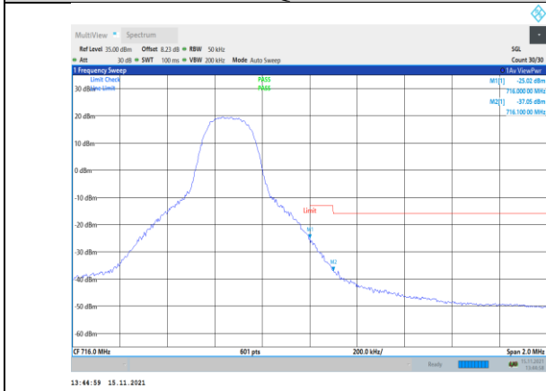
Band17-5MHz-QPSK-23825-1RB#24
