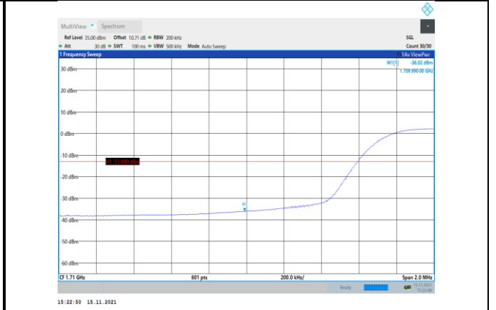
Band66-15MHz-16QAM-132047-75RB#0
