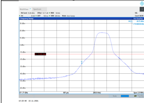
Band4-5MHz-16QAM-19975-1RB#0
