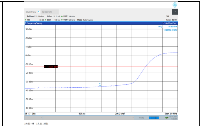
Band4-15MHz-QPSK-20025-75RB#0
