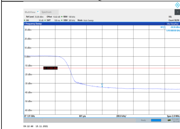
Band2-10MHz-16QAM-19150-50RB#0
