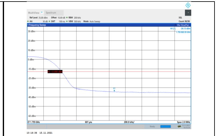
Band4-15MHz-16QAM-20325-75RB#0
