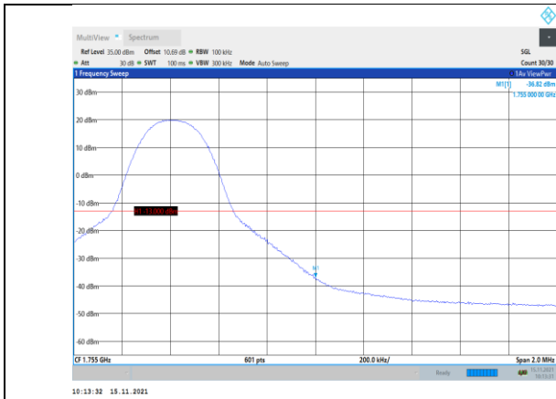
Band4-10MHz-16QAM-20350-1RB#49
