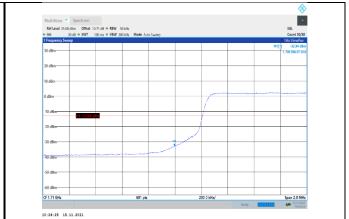
Band4-5MHz-16QAM-19975-25RB#0
