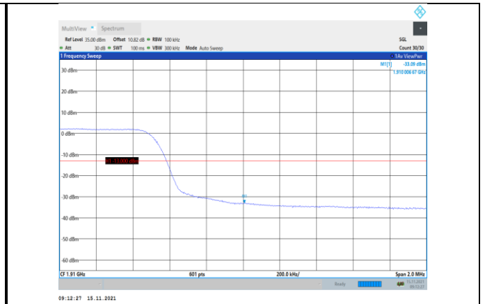
Band2-10MHz-QPSK-19150-50RB#0
