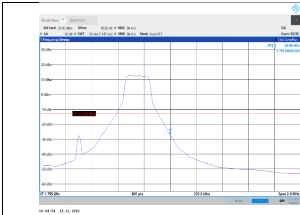
Band4-1.4MHz-16QAM-20393-1RB#5
