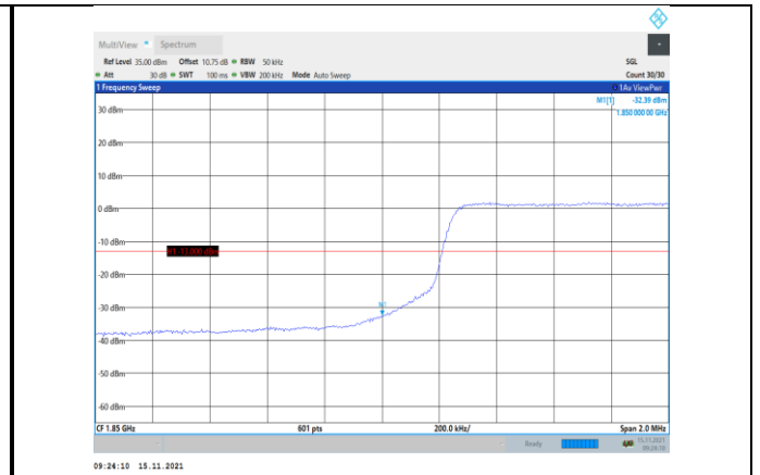
Band2-5MHz-16QAM-18625-25RB#0
