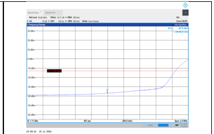
Band66-20MHz-QPSK-132072-100RB#0
