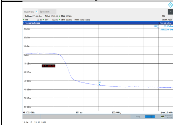
Band4-10MHz-16QAM-20350-50RB#0
