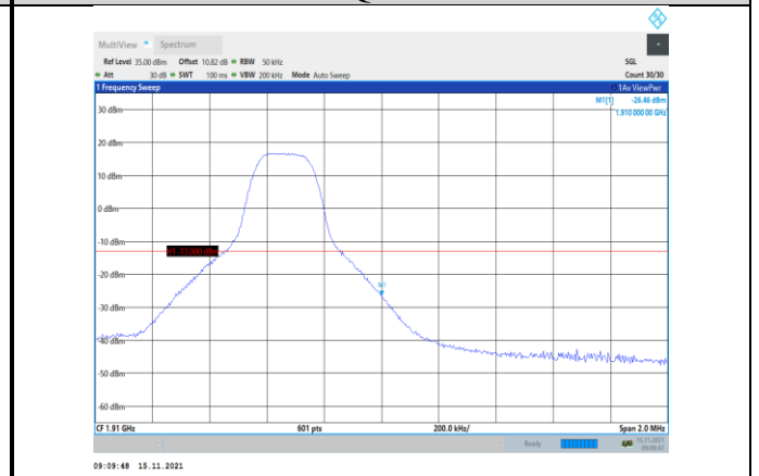
Band2-5MHz-16QAM-19175-1RB#24
