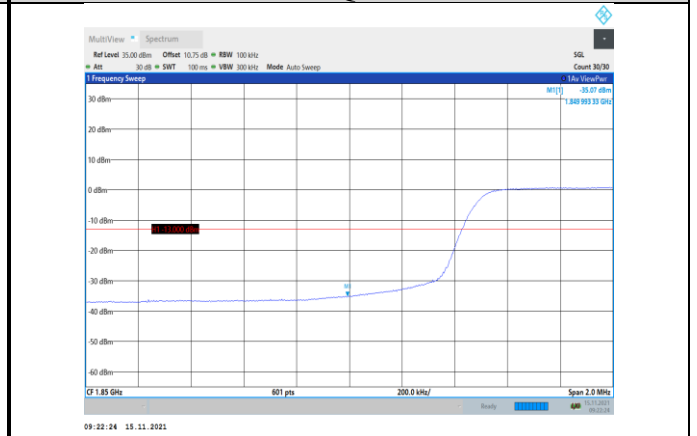
Band2-10MHz-16QAM-18650-50RB#0
