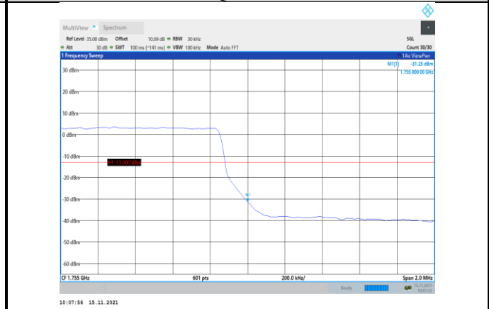
Band4-3MHz-QPSK-20385-15RB#0
