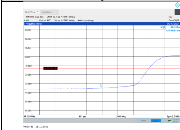
Band2-15MHz-16QAM-18675-75RB#0
