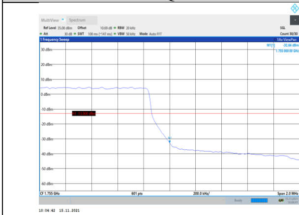
Band4-1.4MHz-16QAM-20393-6RB#0
