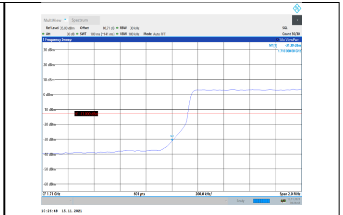
Band4-3MHz-QPSK-19965-15RB#0
