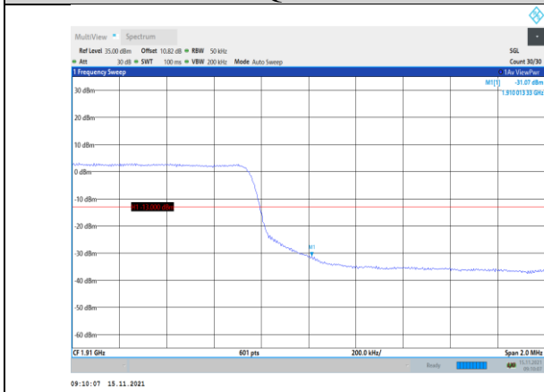
Band2-5MHz-QPSK-19175-25RB#0
