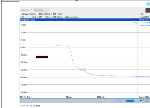
Band4-5MHz-QPSK-20375-25RB#0
