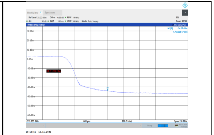
Band4-10MHz-QPSK-20350-50RB#0
