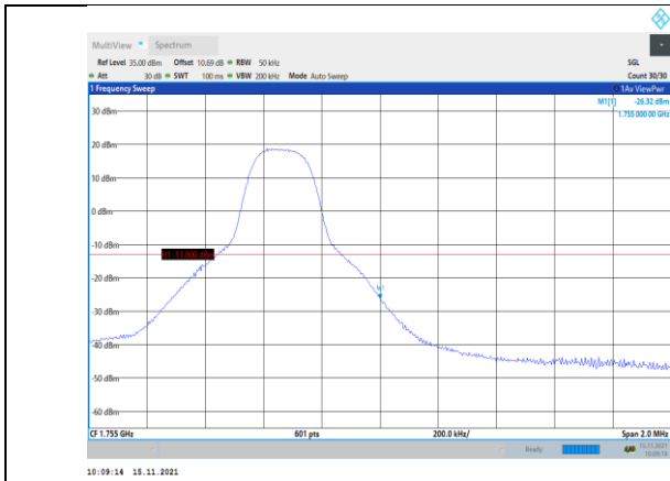
Band4-5MHz-QPSK-20375-1RB#24
