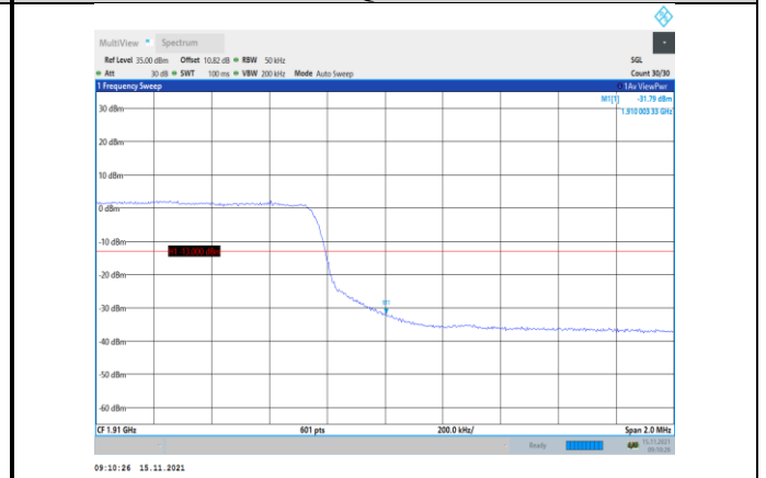
Band2-5MHz-16QAM-19175-25RB#0
