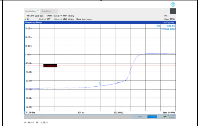
Band4-10MHz-16QAM-20000-50RB#0
