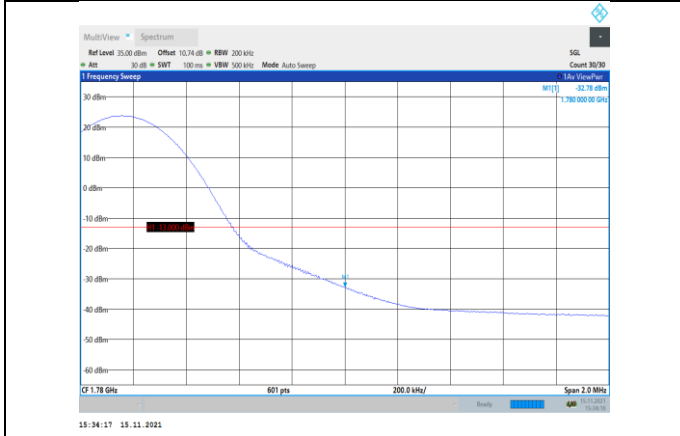
Band66-15MHz-QPSK-132597-1RB#74
