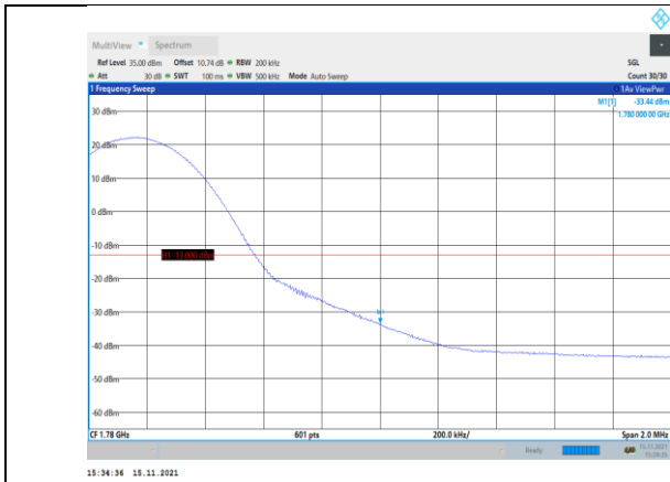
Band66-15MHz-16QAM-132597-1RB#74
