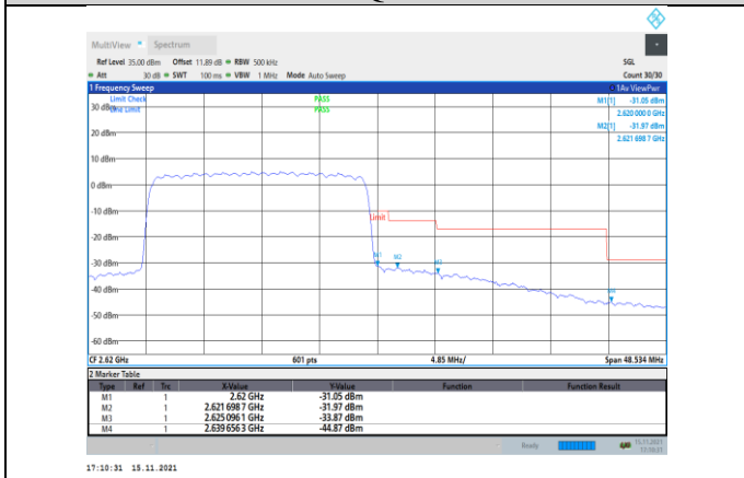
Band38-20MHz-16QAM-38150-100RB#0
