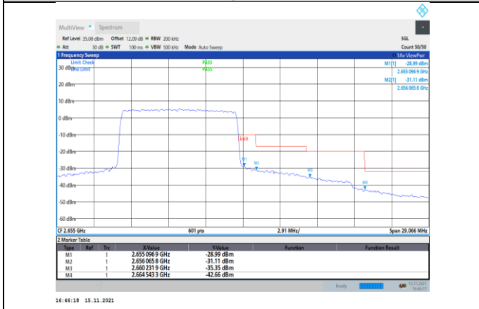
Band41-10MHz-QPSK-41190-50RB#0
