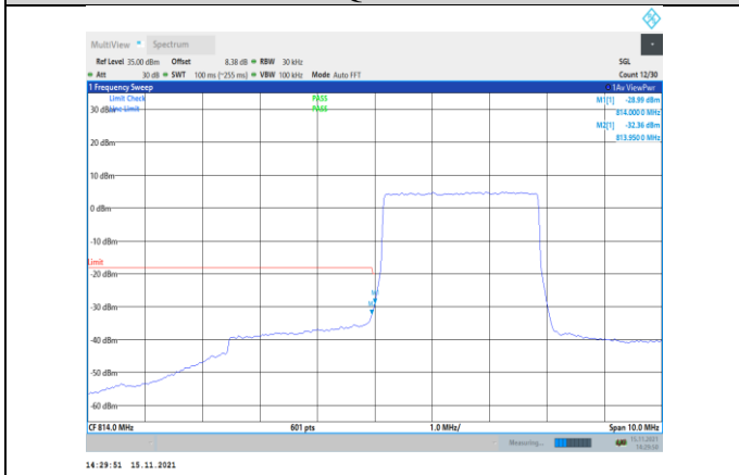
Band26-3MHz-QPSK-26705-15RB#0
