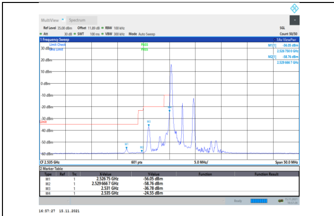
Band41-5MHz-16QAM-40065-1RB#0
