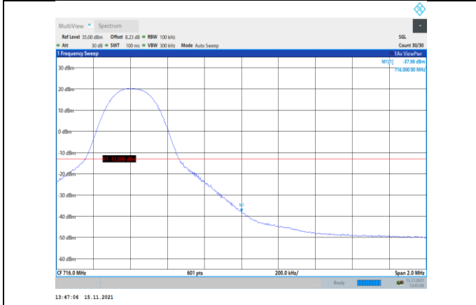
Band17-10MHz-16QAM-23800-1RB#49
