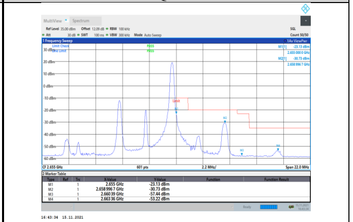
Band41-5MHz-QPSK-41215-1RB#24
