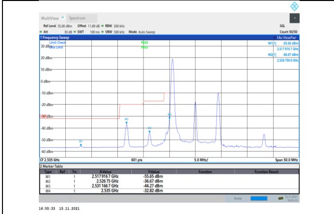
Band41-10MHz-16QAM-40090-1RB#0
