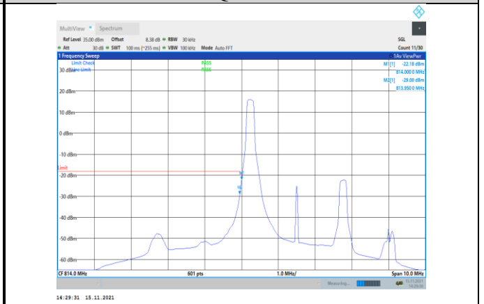
Band26-3MHz-16QAM-26705-1RB#0
