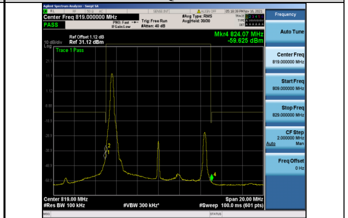
Band26-10MHz-QPSK-26740_Left-1RB#0
