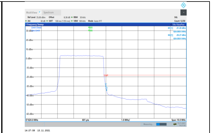
Band26-3MHz-QPSK-26775-15RB#0
