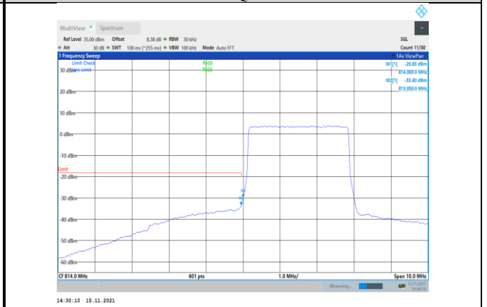
Band26-3MHz-16QAM-26705-15RB#0
