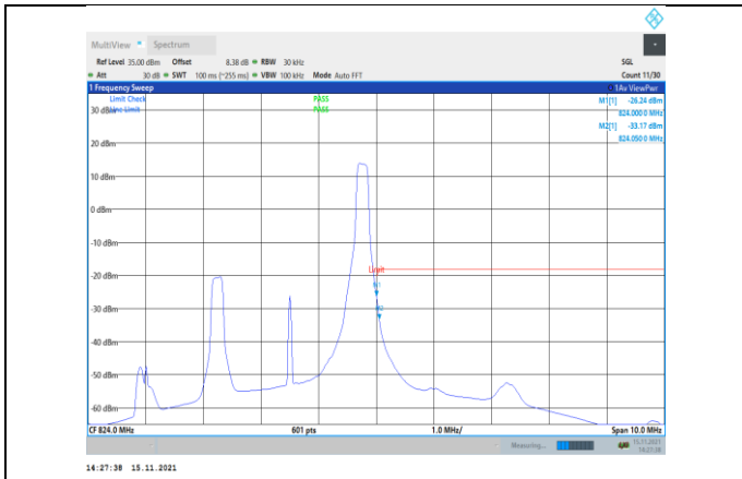
Band26-3MHz-16QAM-26775-1RB#14
