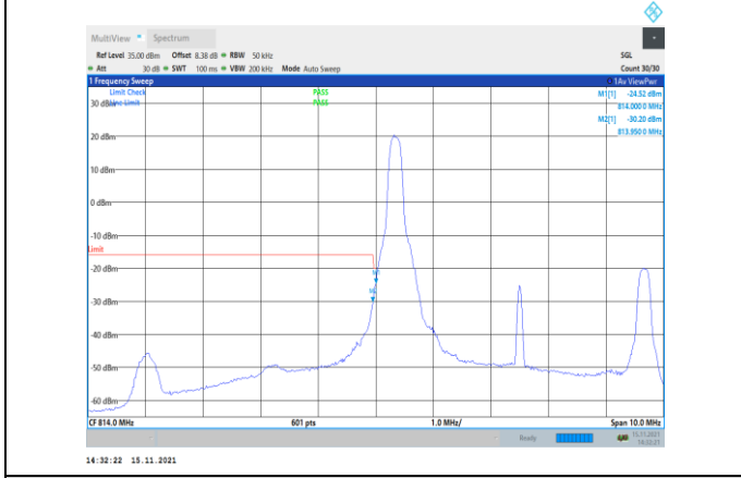
Band26-5MHz-QPSK-26715-1RB#0
