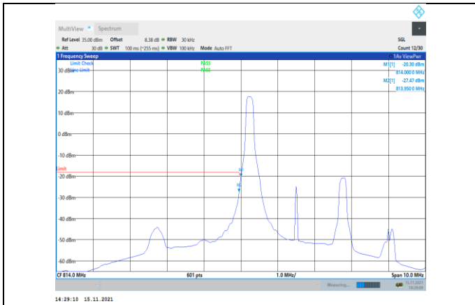
Band26-3MHz-QPSK-26705-1RB#0
