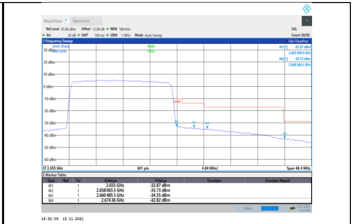
Band41-20MHz-16QAM-41140-100RB#0
