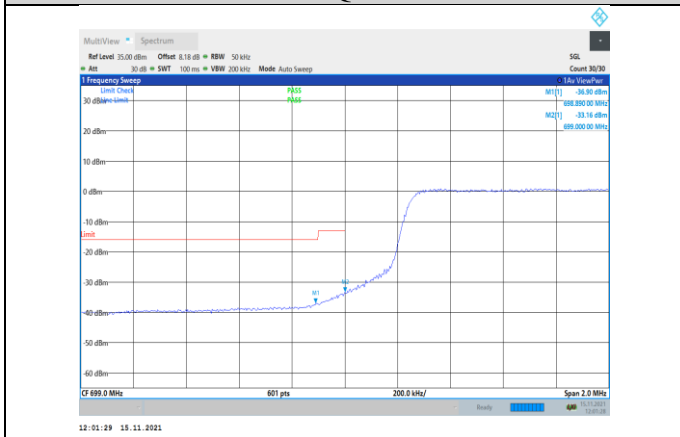
Band12-5MHz-16QAM-23035-25RB#0
