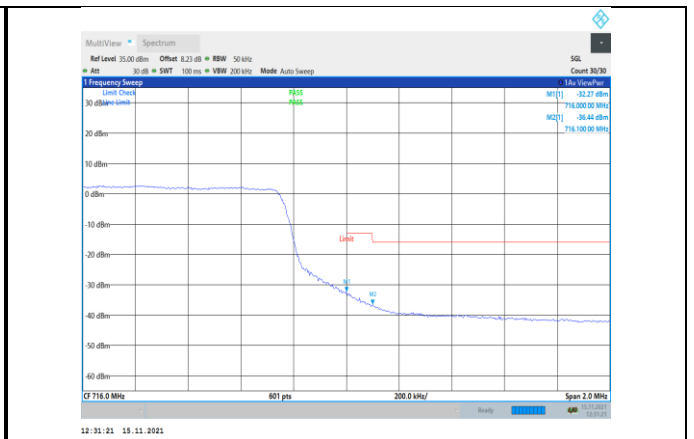
Band12-5MHz-16QAM-23155-25RB#0
