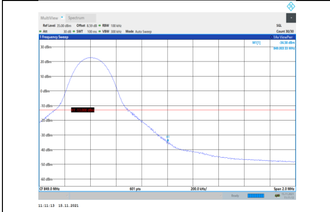
Band5-10MHz-QPSK-20600-1RB#49
