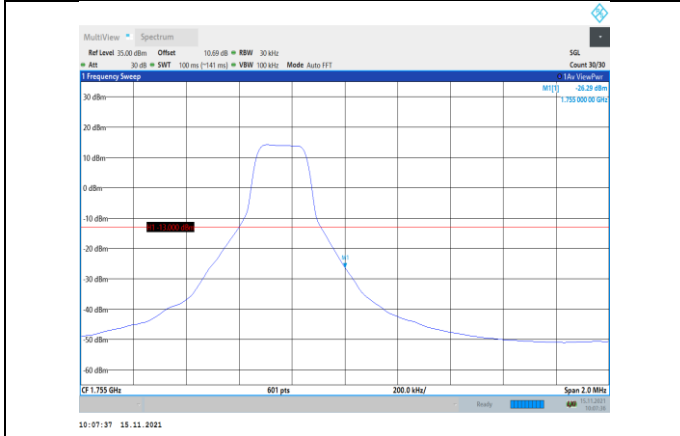
Band4-3MHz-16QAM-20385-1RB#14
