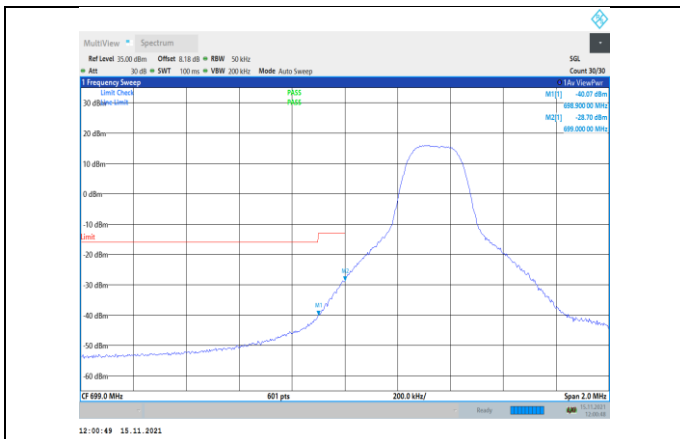
Band12-5MHz-16QAM-23035-1RB#0
