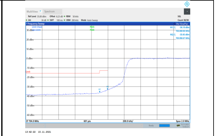
Band17-5MHz-16QAM-23755-25RB#0
