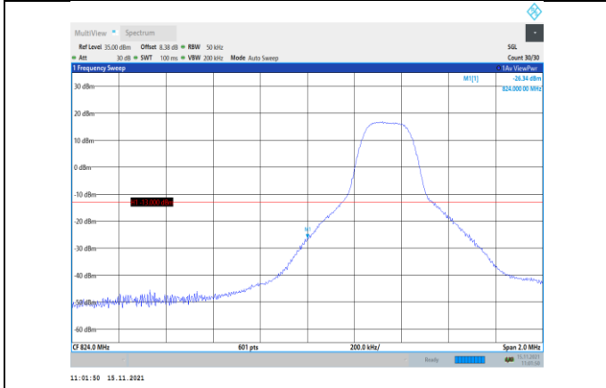
Band5-5MHz-16QAM-20425-1RB#0
