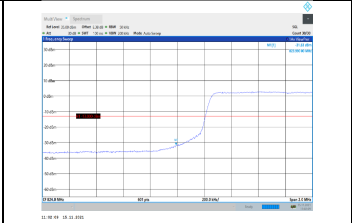
Band5-5MHz-QPSK-20425-25RB#0
