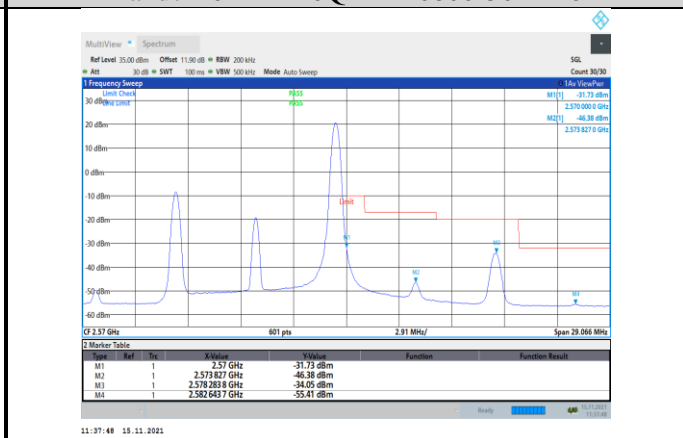
Band7-10MHz-16QAM-21400-1RB#49
