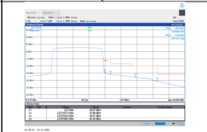
Band7-10MHz-16QAM-21400-50RB#0
