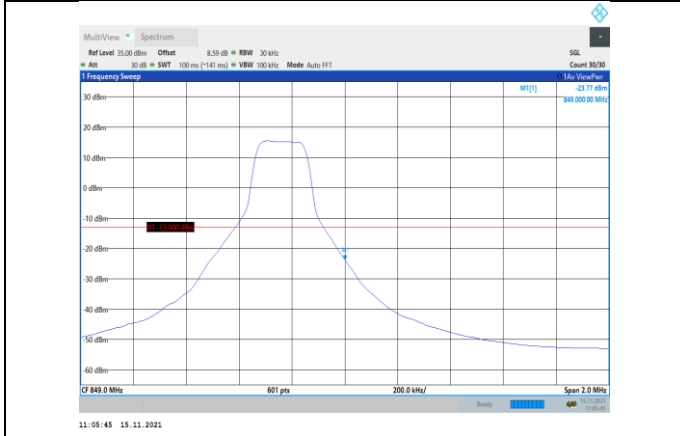
Band5-3MHz-16QAM-20635-1RB#14
