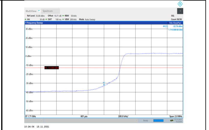
Band4-5MHz-QPSK-19975-25RB#0
