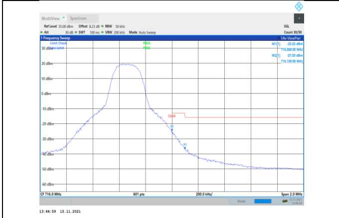
Band17-5MHz-QPSK-23825-1RB#24
