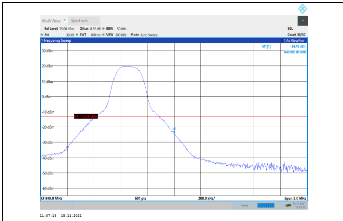
Band5-5MHz-QPSK-20625-1RB#24
