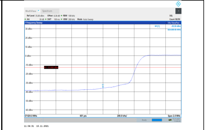
Band5-10MHz-16QAM-20450-50RB#0
