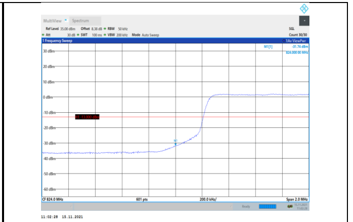
Band5-5MHz-16QAM-20425-25RB#0
