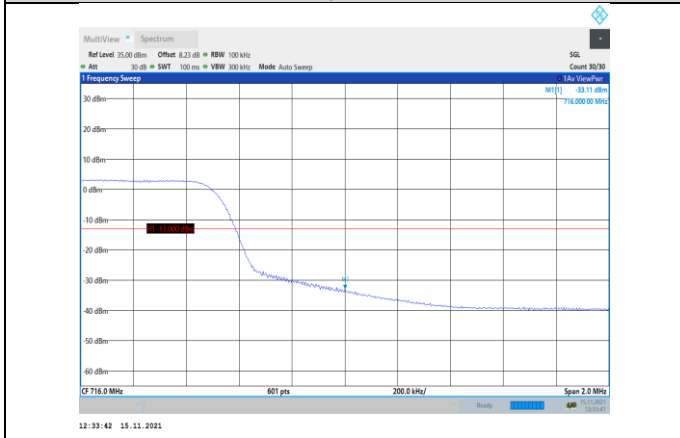
Band12-10MHz-QPSK-23130-50RB#0
