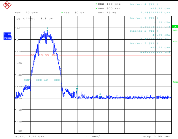
11B_Ant1_High_2462
