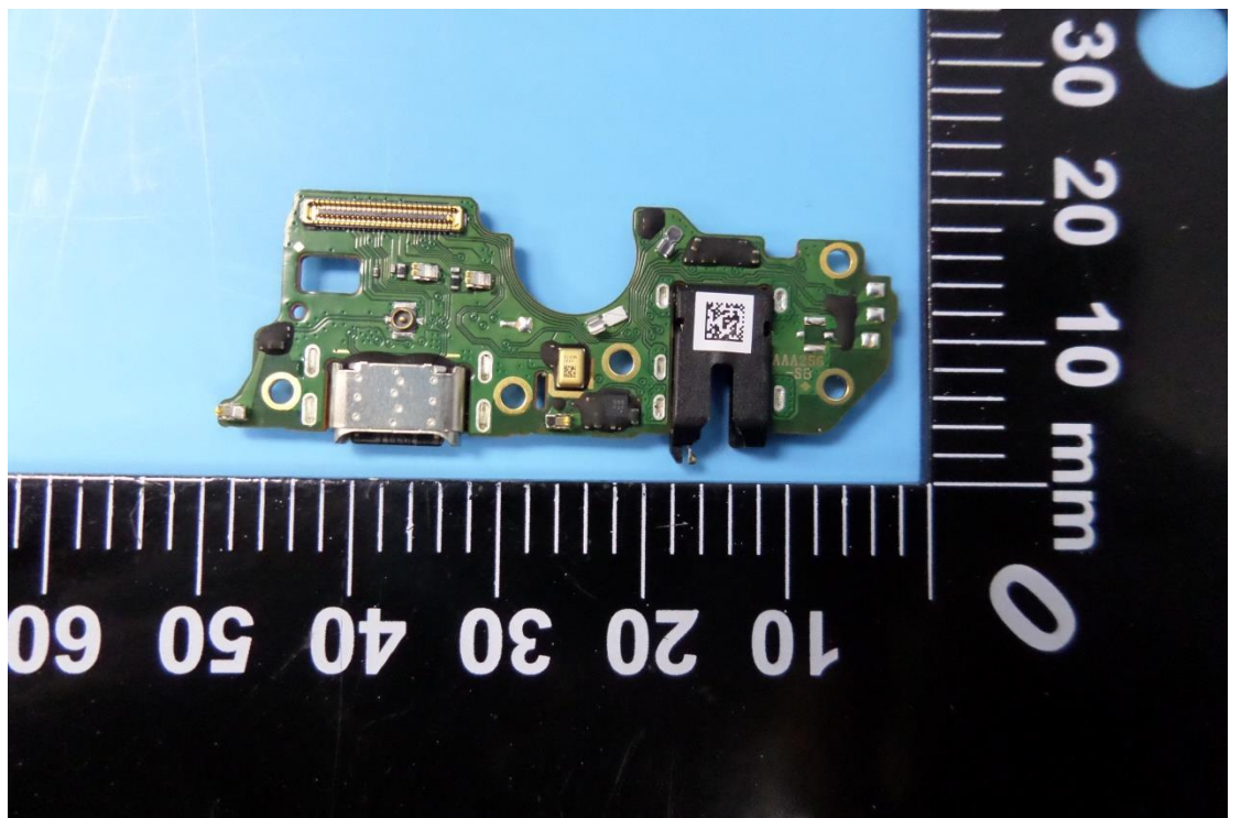
Photo 9 Inside of EUT
