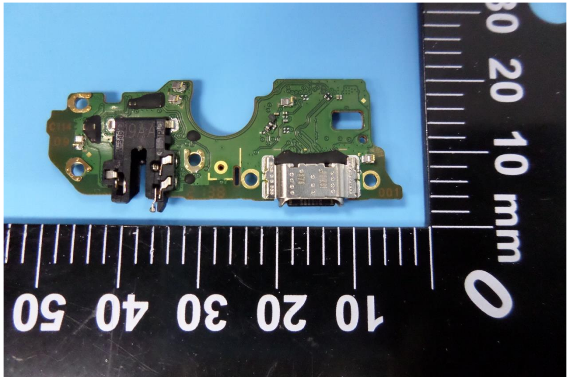
Photo 10 Inside of EUT
