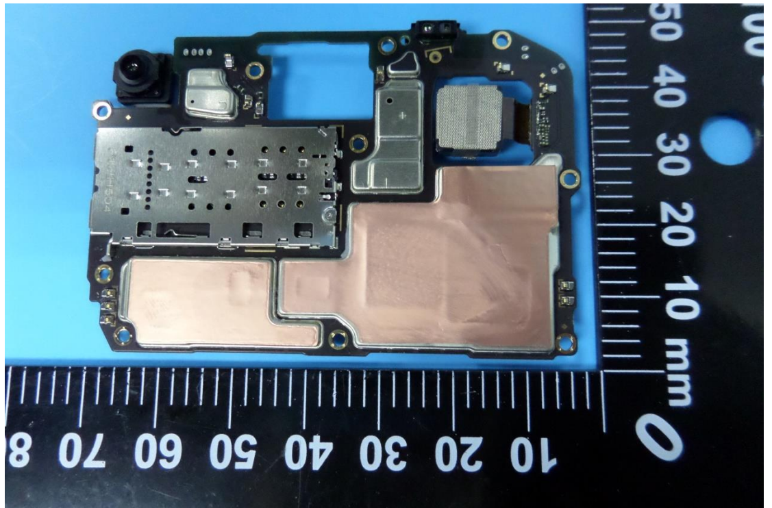
Photo 8 Inside of EUT
