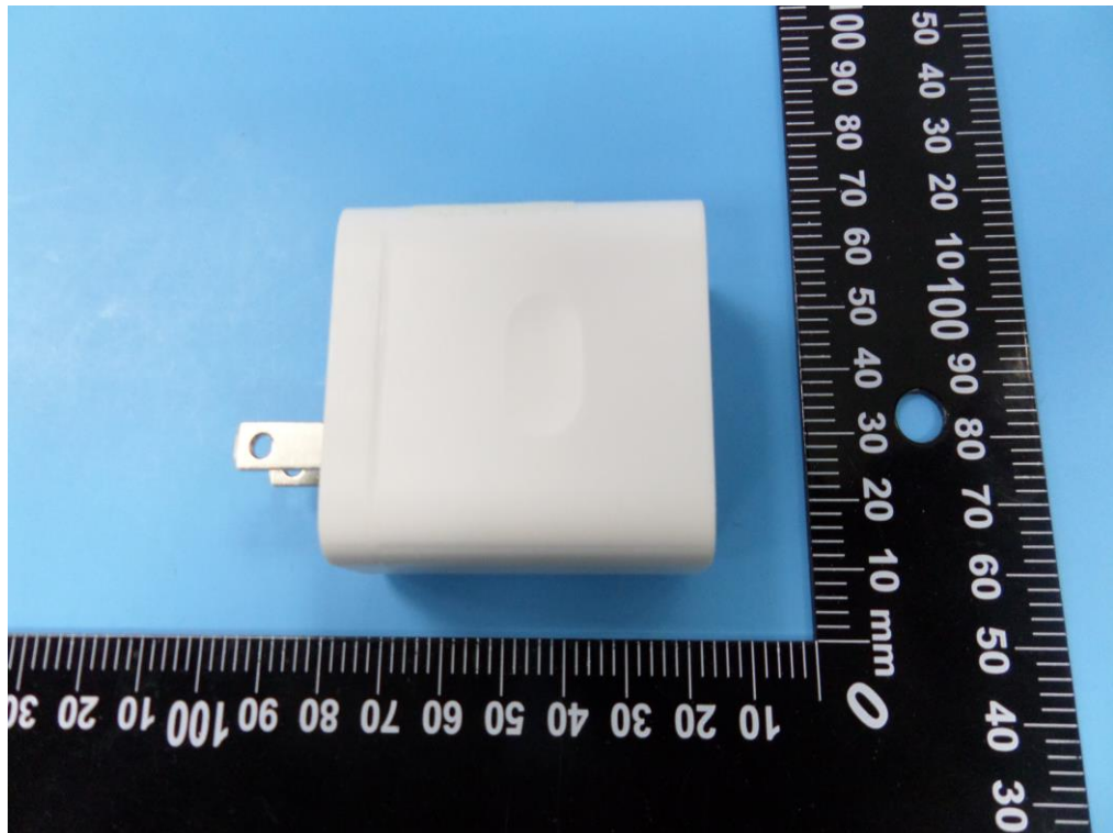
Photo 13 Appearance of AC adapter (VCB3HDUH)
