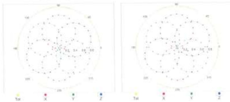
f=600 MHz,TEM
