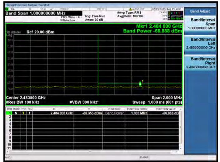
802.11b CHANNEL 9, Reference level
