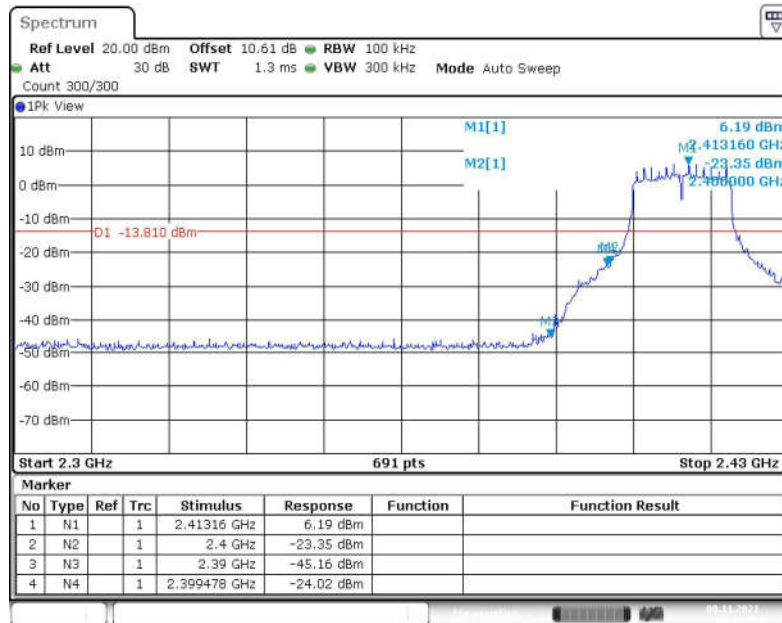
Fig.51 Band Edges (802.11g, CH 1)
