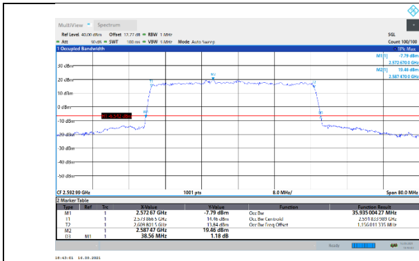
N41-30kHz-40MHz-DFT-16QAM-Mid-Outer_Full--- PASS
