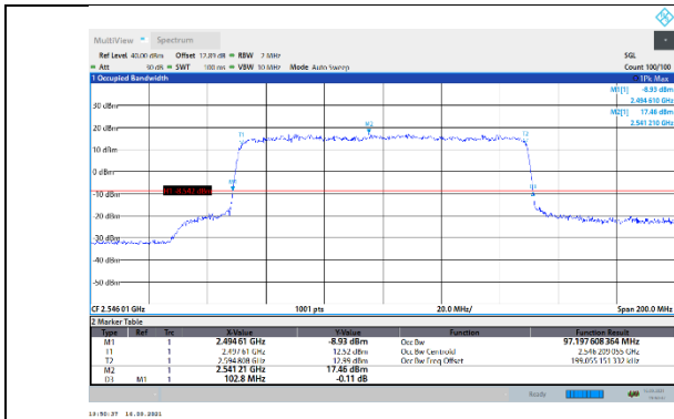
N41-30kHz-100MHz-CP-16QAM-Low-Outer_Full---PASS
