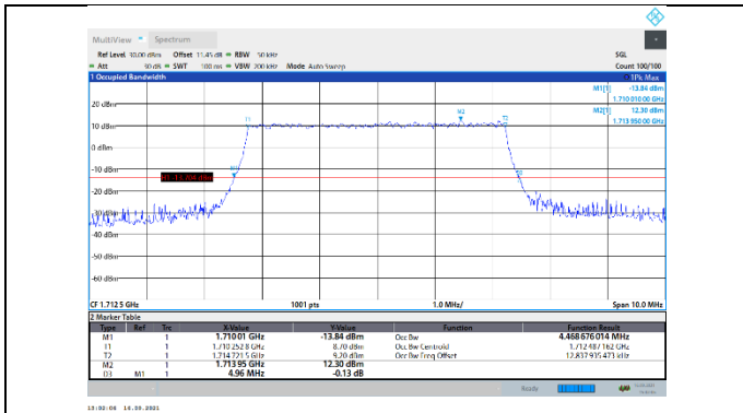
N66-15kHz-5MHz-CP-64QAM-Low-Outer_Full---PASS
