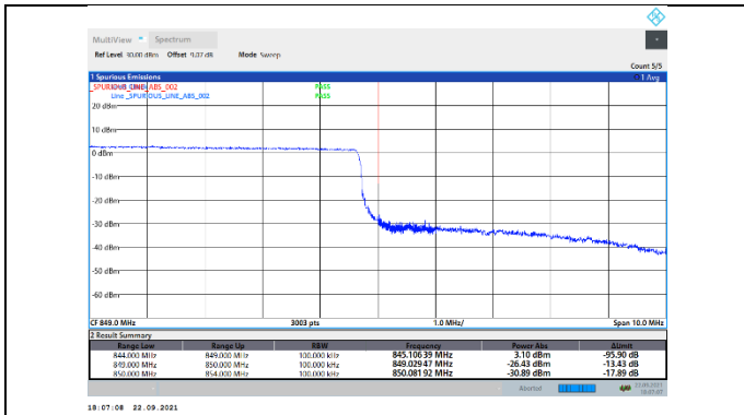
N5-15kHz-10MHz-CP-QPSK-High-Outer_Full---PASS
