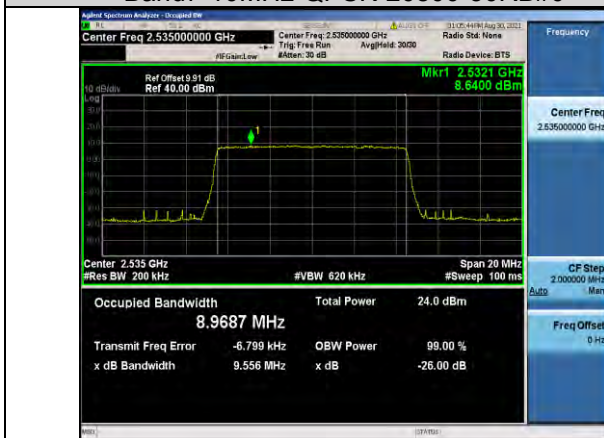
Band7-10MHz-QPSK-21100-50RB#0
