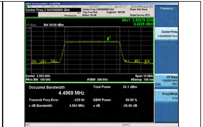
Band7-5MHz-16QAM-20775-25RB#0
