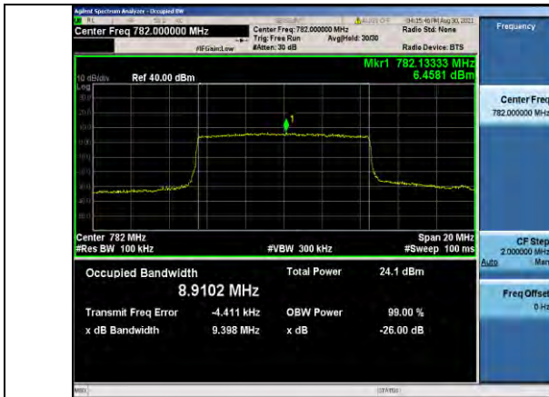
Band13-10MHz-QPSK-23230-50RB#0
