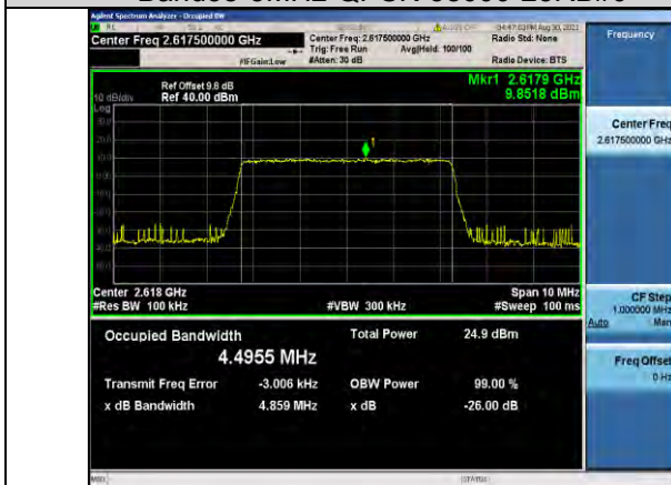
Band38-5MHz-QPSK-38225-25RB#0
