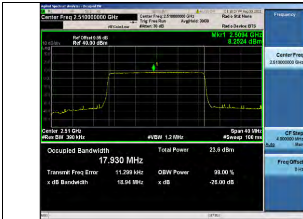
Band7-20MHz-QPSK-20850-100RB#0
