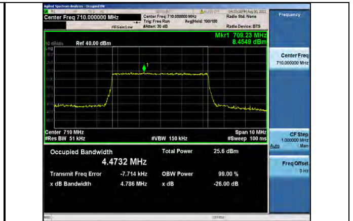
Band17-5MHz-QPSK-23790-25RB#0
