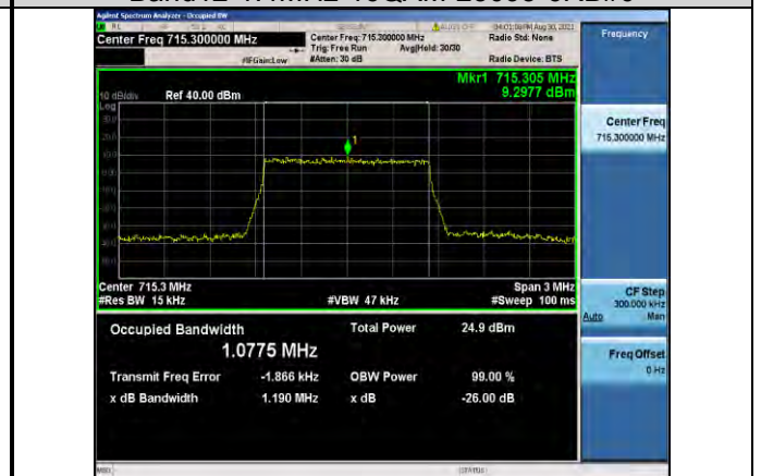
Band12-1.4MHz-16QAM-23173-6RB#0
