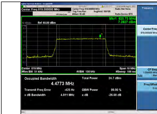
Band26-5MHz-16QAM-26740-25RB#0
