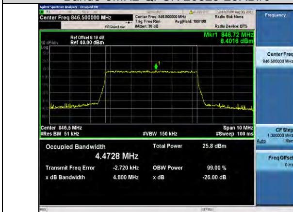
Band5-5MHz-QPSK-20625-25RB#0
