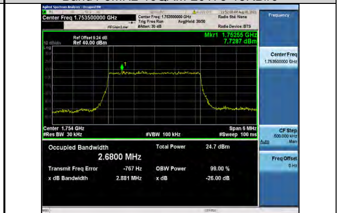
Band4-3MHz-16QAM-17535-15RB#0
