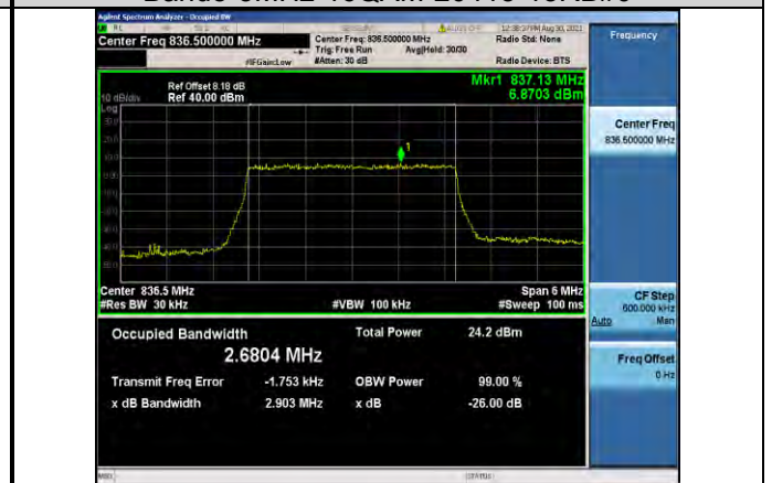
Band5-3MHz-16QAM-20525-15RB#0
