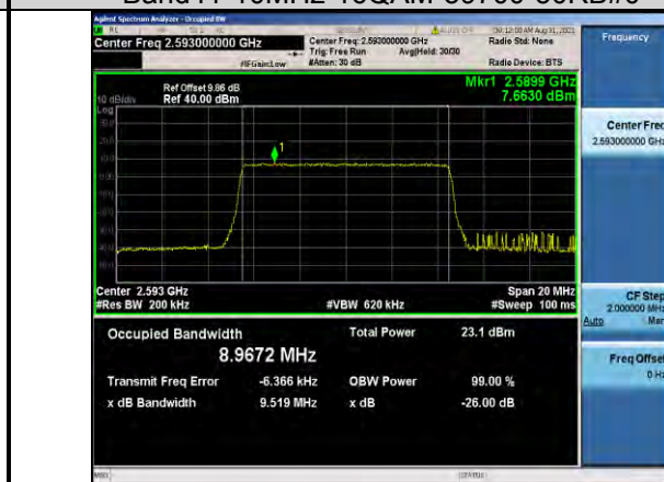
Band41-10MHz-16QAM-40620-50RB#0
