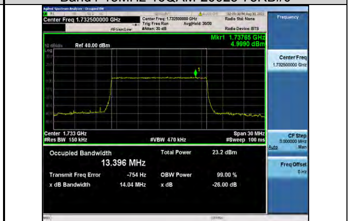
Band4-15MHz-16QAM-20175-75RB#0
