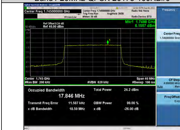
Band4-20MHz-QPSK-20300-100RB#0
