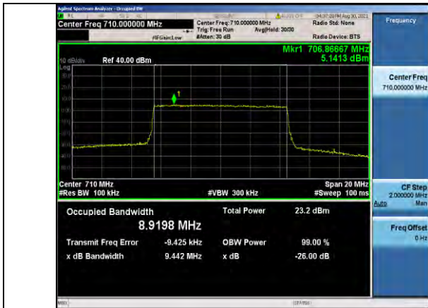
Band17-10MHz-16QAM-23790-50RB#0
