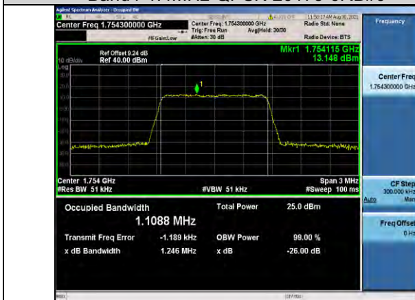
Band4-1.4MHz-QPSK-20393-6RB#0
