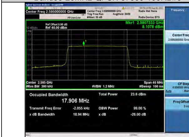
Band38-20MHz-QPSK-38000-100RB#0
