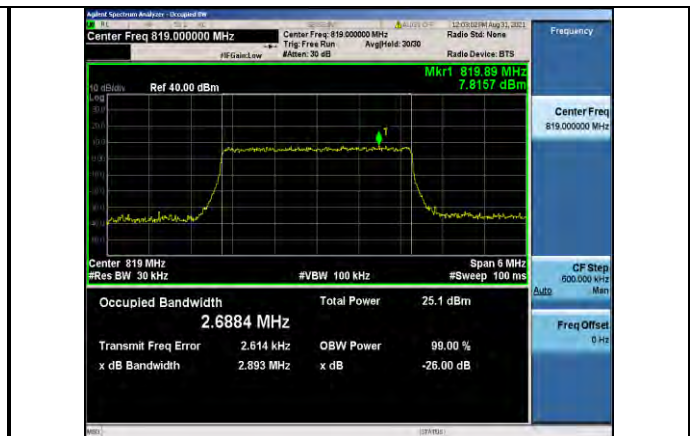
Band26-3MHz-QPSK-26740-15RB#0
