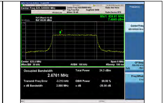
Band5-3MHz-16QAM-20415-15RB#0
