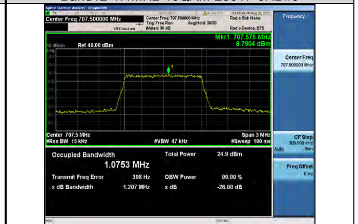
Band12-1.4MHz-16QAM-23095-6RB#0
