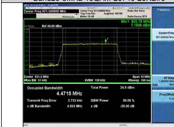
Band26-5MHz-16QAM-26765-25RB#0
