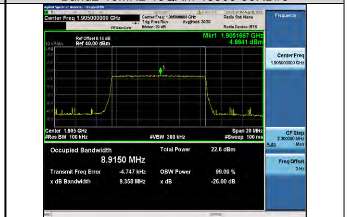
Band2-10MHz-16QAM-19050-50RB#0
