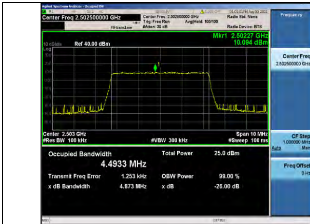
Band7-5MHz-QPSK-20775-25RB#0
