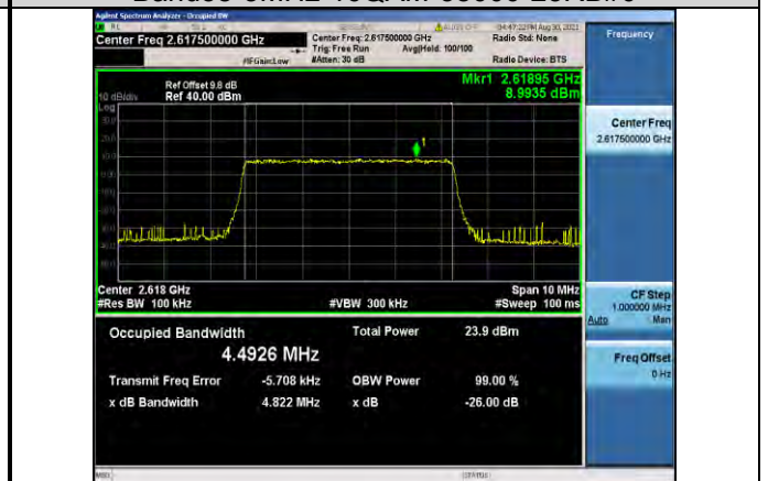
Band38-5MHz-16QAM-38225-25RB#0
