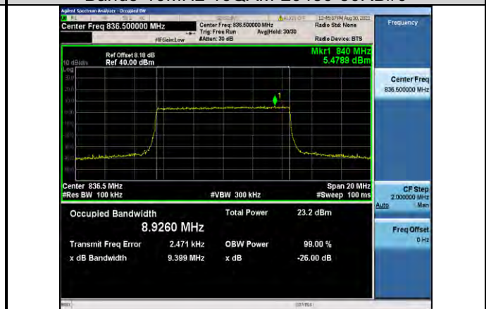
Band5-10MHz-16QAM-20525-50RB#0
