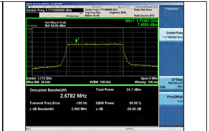
Band4-3MHz-16QAM-19965-15RB#0
