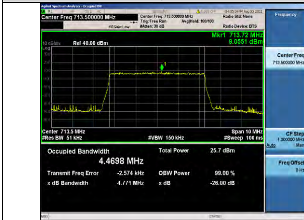
Band12-5MHz-QPSK-23155-25RB#0
