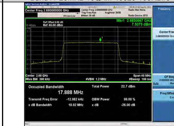
Band41-20MHz-16QAM-41490-100RB#0
