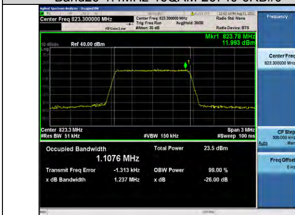
Band26-1.4MHz-16QAM-26783-6RB#0
