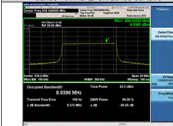
Band5-10MHz-QPSK-20525-50RB#0
