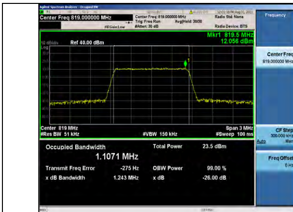
Band26-1.4MHz-16QAM-26740-6RB#0
