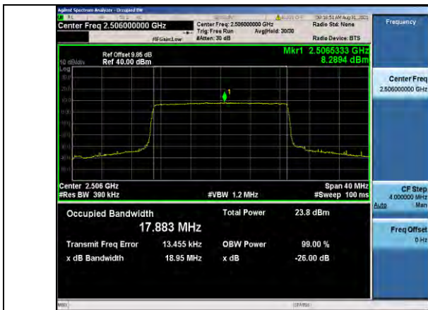
Band41-20MHz-QPSK-39750-100RB#0
