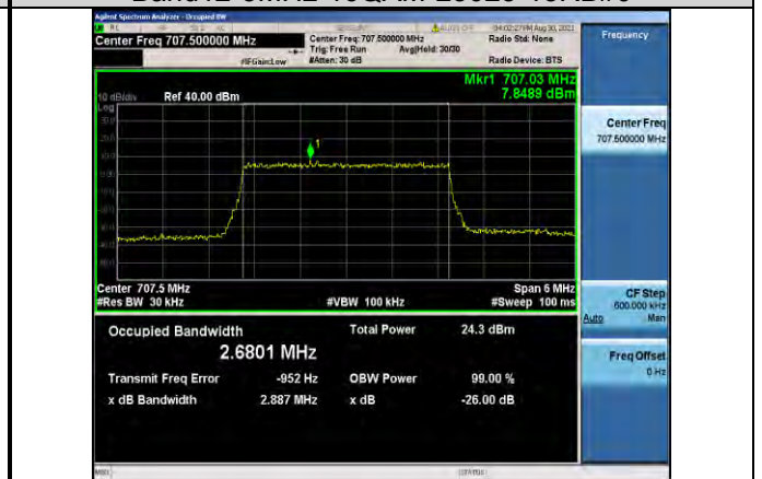
Band12-3MHz-16QAM-23095-15RB#0
