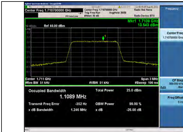
Band4-1.4MHz-QPSK-19957-6RB#0
