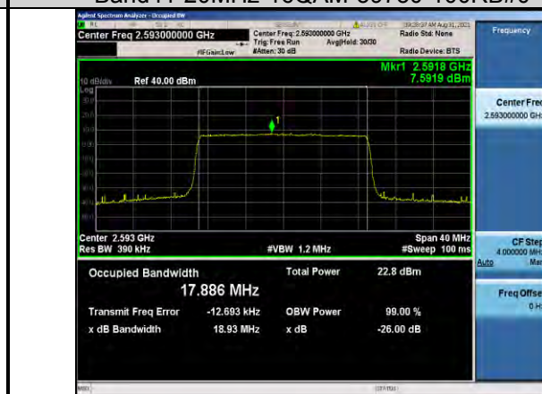
Band41-20MHz-16QAM-40620-100RB#0
