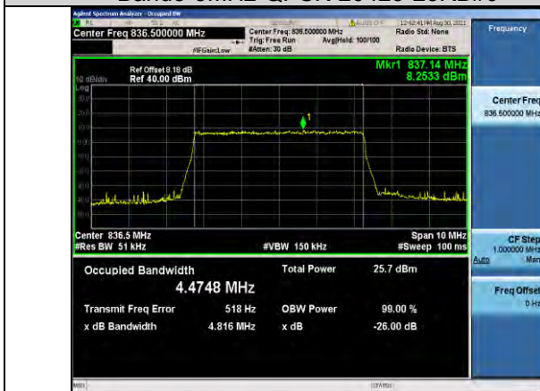
Band5-5MHz-QPSK-20525-25RB#0
