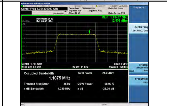
Band4-1.4MHz-16QAM-20393-6RB#0
