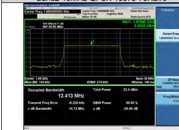
Band2-15MHz-QPSK-18800-75RB#0
