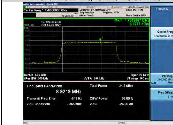
Band4-10MHz-QPSK-20350-50RB#0
