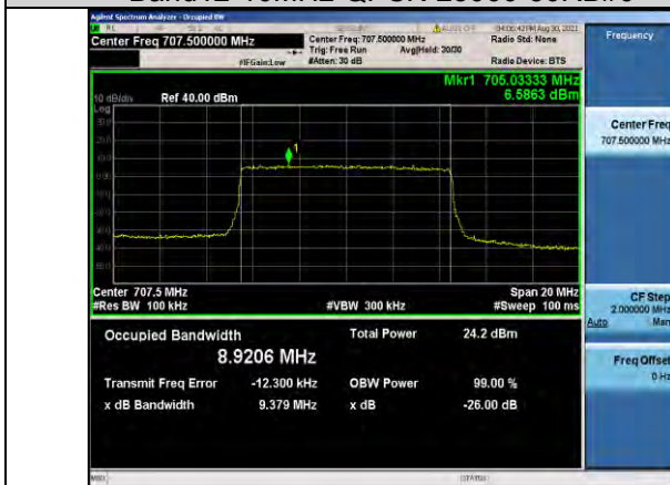
Band12-10MHz-QPSK-23095-50RB#0
