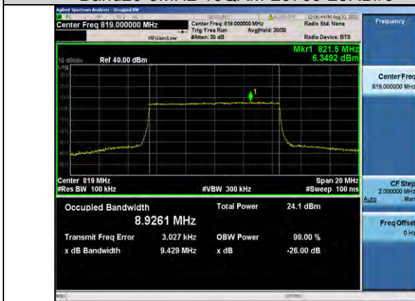
Band26-10MHz-QPSK-26740-50RB#0
