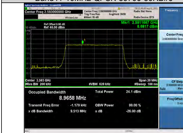
Band41-10MHz-QPSK-40620-50RB#0
