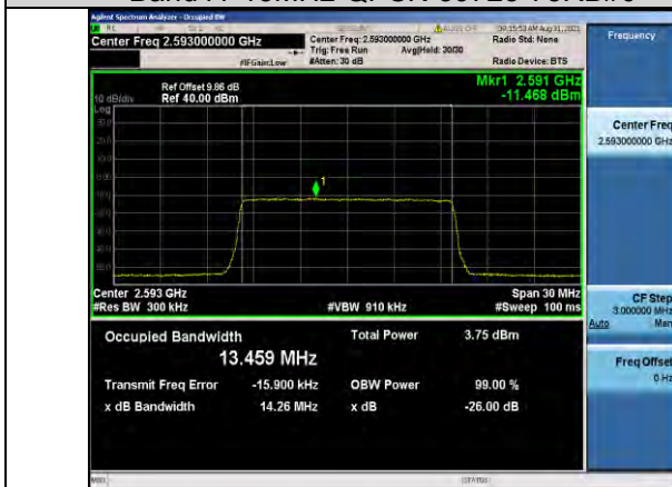
Band41-15MHz-QPSK-40620-75RB#0
