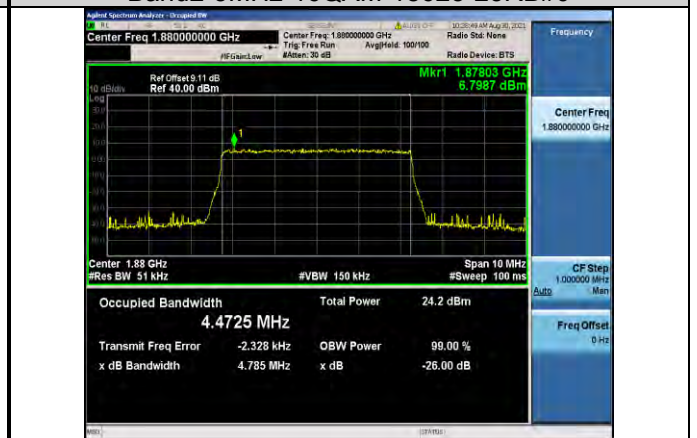
Band2-5MHz-16QAM-18900-25RB#0
