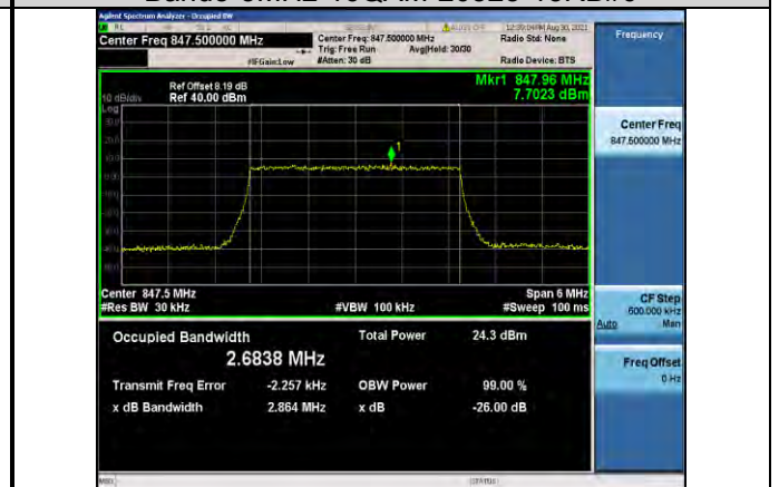
Band5-3MHz-16QAM-20635-15RB#0
