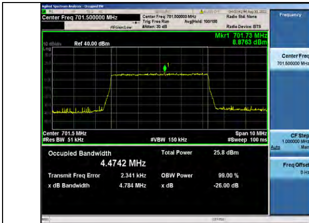
Band12-5MHz-QPSK-23035-25RB#0
