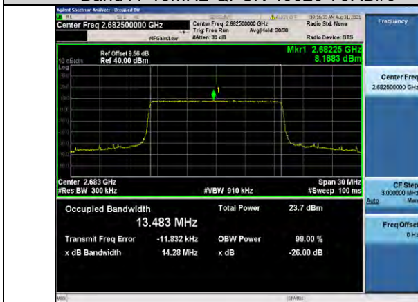
Band41-15MHz-QPSK-41515-75RB#0
