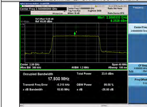
Band7-20MHz-QPSK-21350-100RB#0
