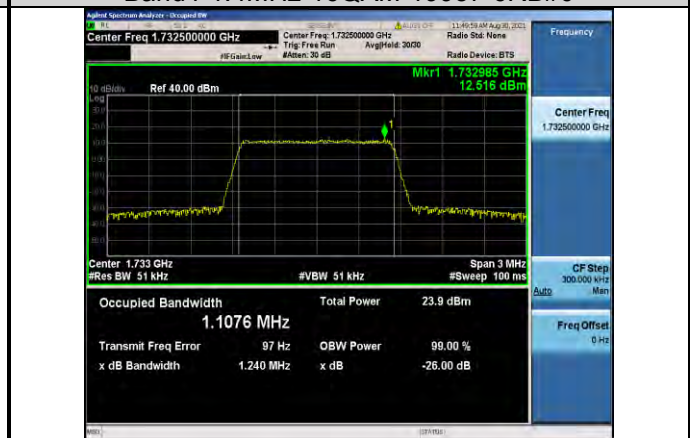
Band4-1.4MHz-16QAM-20175-6RB#0
