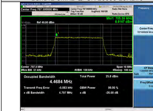
Band12-5MHz-QPSK-23095-25RB#0
