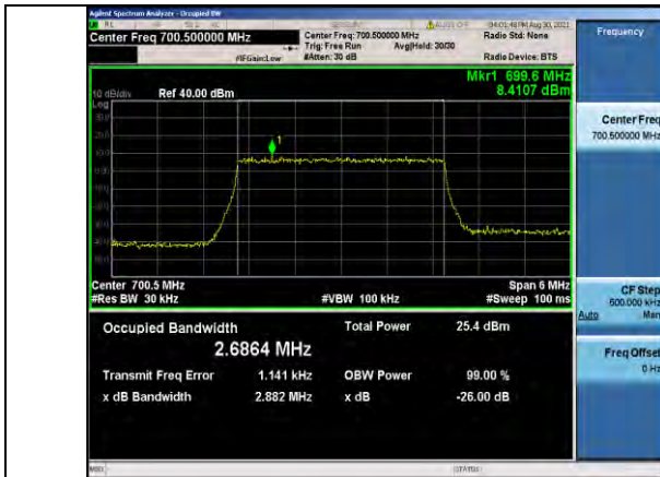
Band12-3MHz-QPSK-23025-15RB#0
