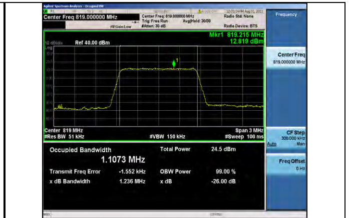
Band26-1.4MHz-QPSK-26740-6RB#0
