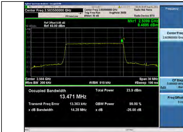
Band41-15MHz-QPSK-39725-75RB#0
