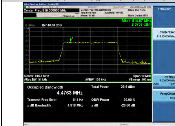
Band26-5MHz-QPSK-26715-25RB#0
