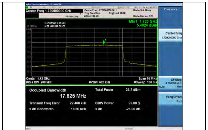
Band4-20MHz-16QAM-20050-100RB#0
