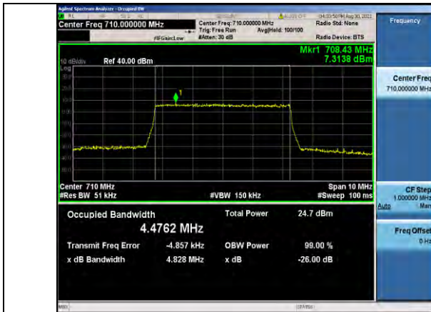
Band17-5MHz-16QAM-23790-25RB#0
