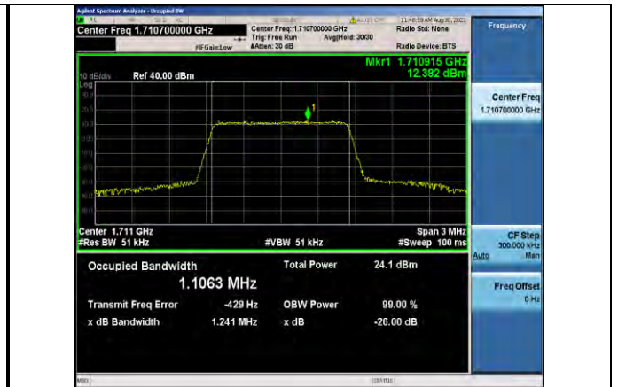
Band4-1.4MHz-16QAM-19957-6RB#0
