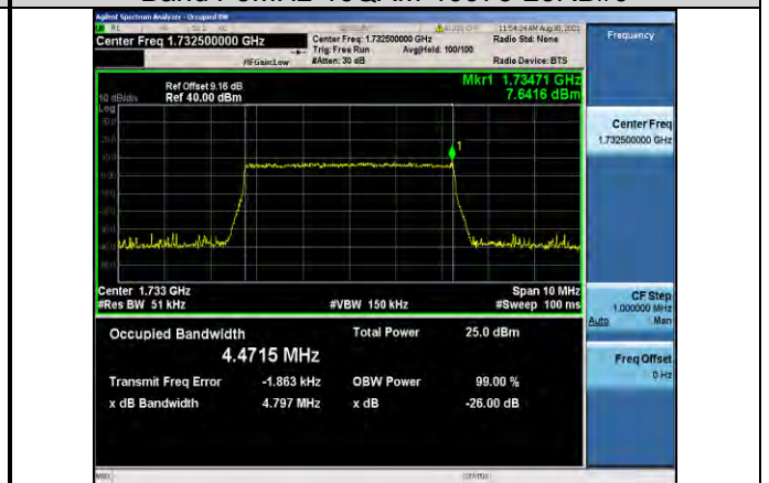
Band4-5MHz-16QAM-17325-25RB#0
