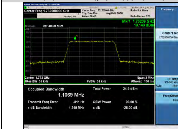
Band4-1.4MHz-QPSK-20175-6RB#0
