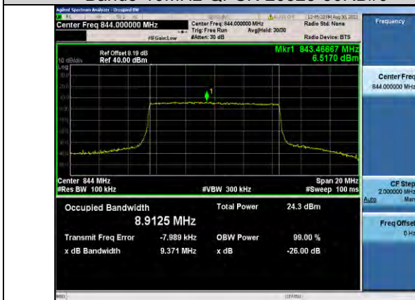
Band5-10MHz-QPSK-20600-50RB#0
