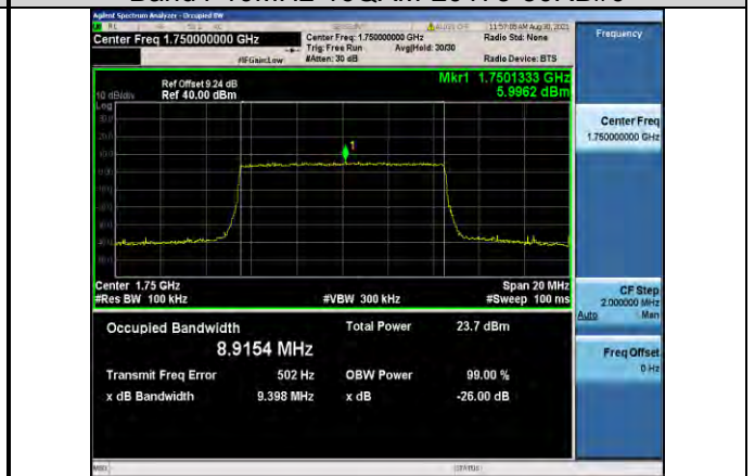
Band4-10MHz-16QAM-20350-50RB#0
