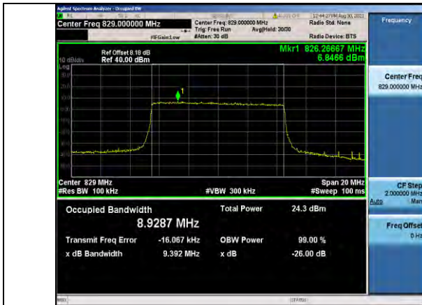
Band5-10MHz-QPSK-20450-50RB#0
