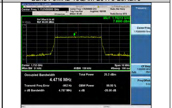
Band4-5MHz-16QAM-17525-25RB#0
