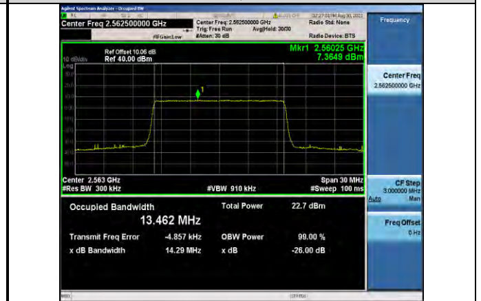
Band7-15MHz-16QAM-21375-75RB#0
