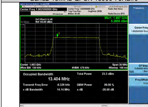
Band2-15MHz-QPSK-19125-75RB#0
