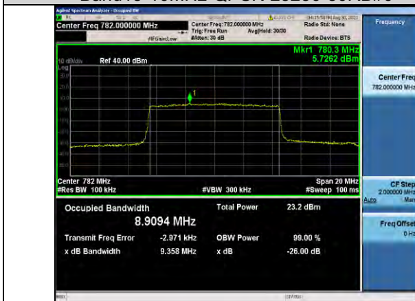
Band13-10MHz-16QAM-23230-50RB#0
