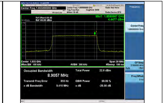
Band2-10MHz-16QAM-18650-50RB#0
