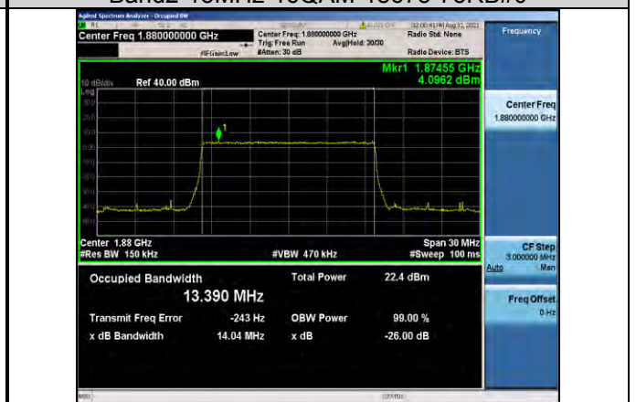
Band2-15MHz-16QAM-18800-75RB#0
