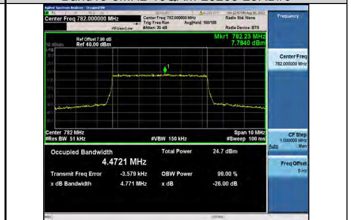
Band13-5MHz-16QAM-23230-25RB#0
