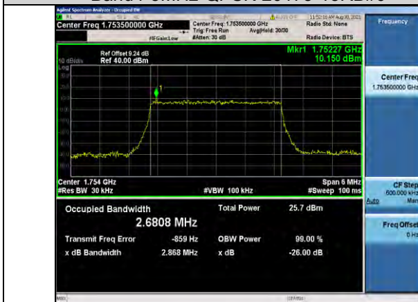
Band4-3MHz-QPSK-17535-15RB#0
