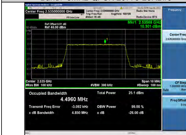
Band7-5MHz-QPSK-21100-25RB#0
