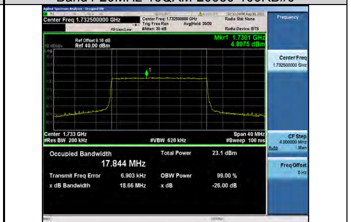
Band4-20MHz-16QAM-20175-100RB#0
