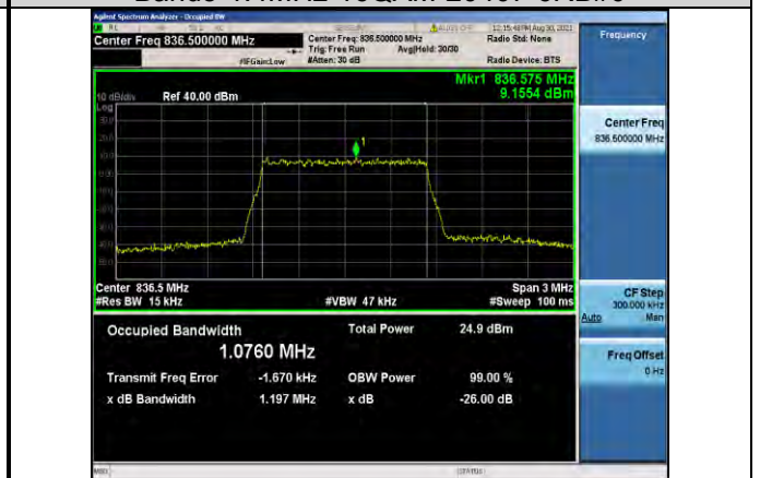
Band5-1.4MHz-16QAM-20525-6RB#0
