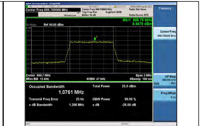
Band12-1.4MHz-16QAM-23017-6RB#0
