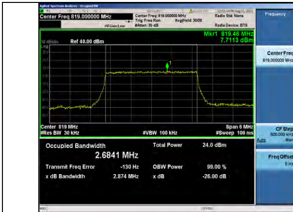
Band26-3MHz-16QAM-26740-15RB#0
