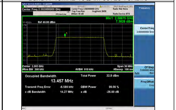
Band41-15MHz-16QAM-40620-75RB#0
