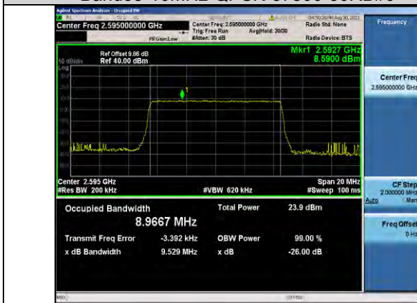
Band38-10MHz-QPSK-38000-50RB#0
