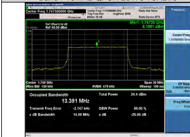
Band4-15MHz-QPSK-20325-75RB#0
