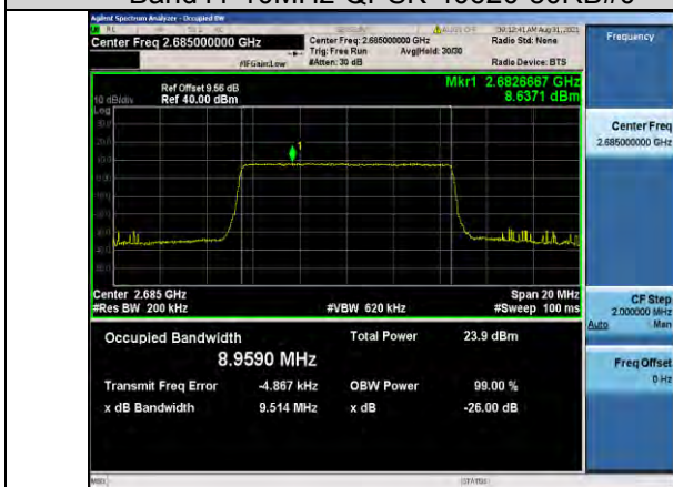
Band41-10MHz-QPSK-41540-50RB#0
