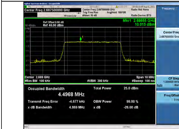
Band41-5MHz-QPSK-41565-25RB#0
