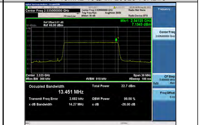
Band7-15MHz-16QAM-21100-75RB#0
