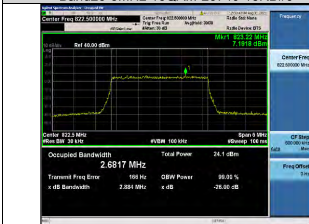
Band26-3MHz-16QAM-26775-15RB#0
