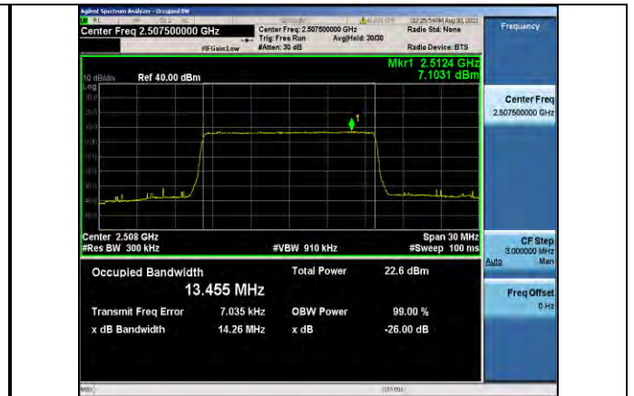
Band7-15MHz-16QAM-20825-75RB#0
