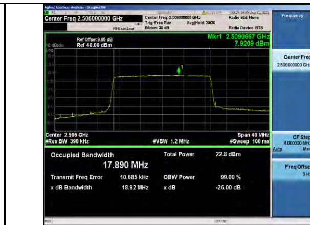
Band41-20MHz-16QAM-39750-100RB#0
