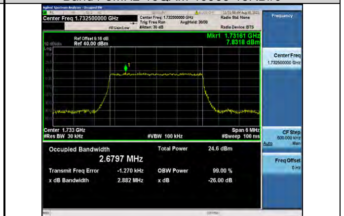
Band4-3MHz-16QAM-17325-15RB#0
