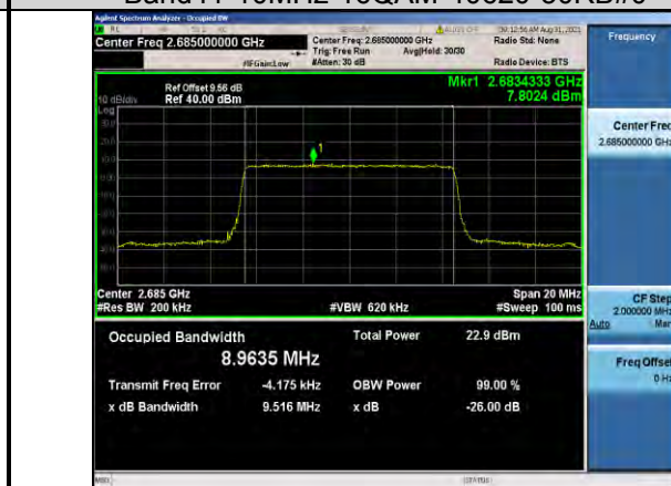
Band41-10MHz-16QAM-41540-50RB#0
