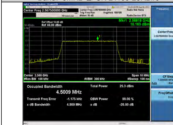
Band7-5MHz-QPSK-21425-25RB#0
