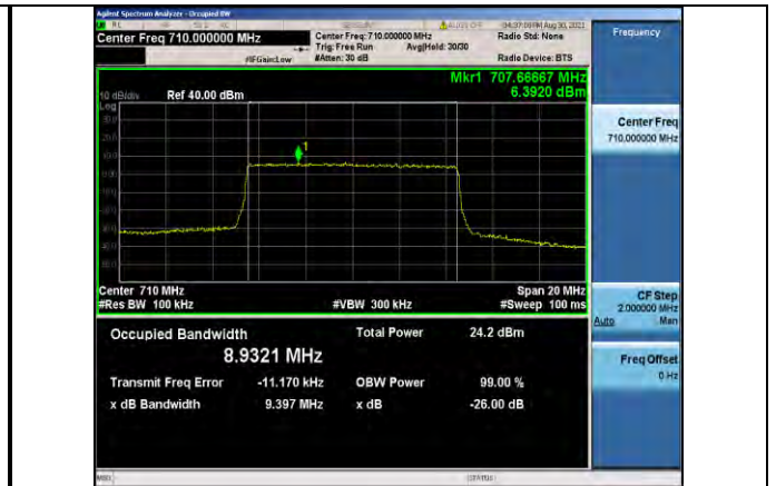
Band17-10MHz-QPSK-23790-50RB#0
