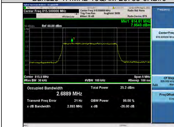
Band26-3MHz-QPSK-26705-15RB#0
