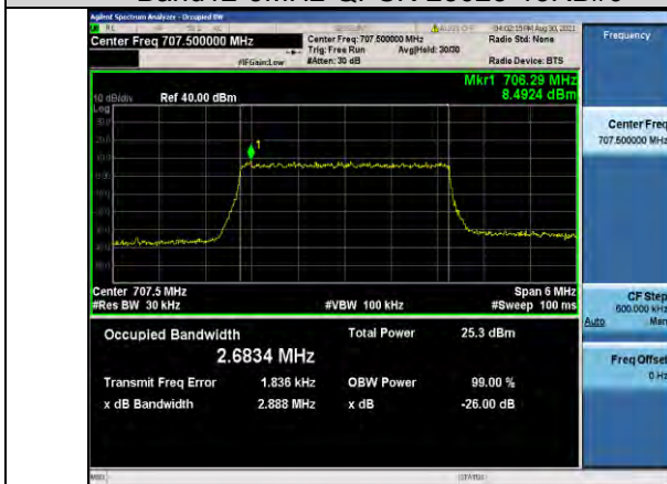
Band12-3MHz-QPSK-23095-15RB#0
