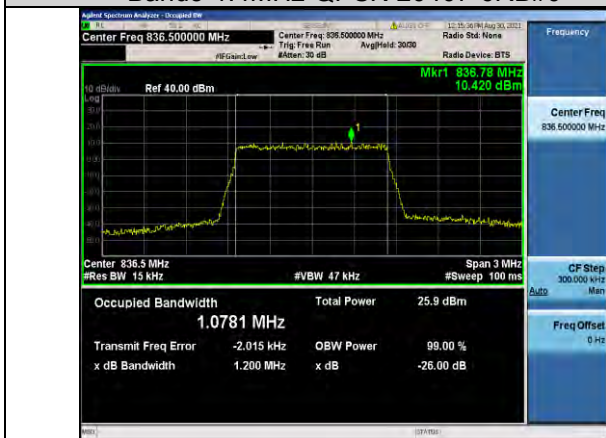
Band5-1.4MHz-QPSK-20525-6RB#0
