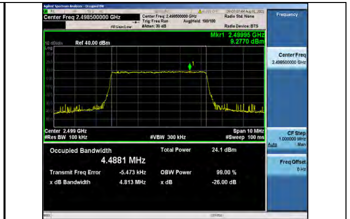
Band41-5MHz-16QAM-39675-25RB#0
