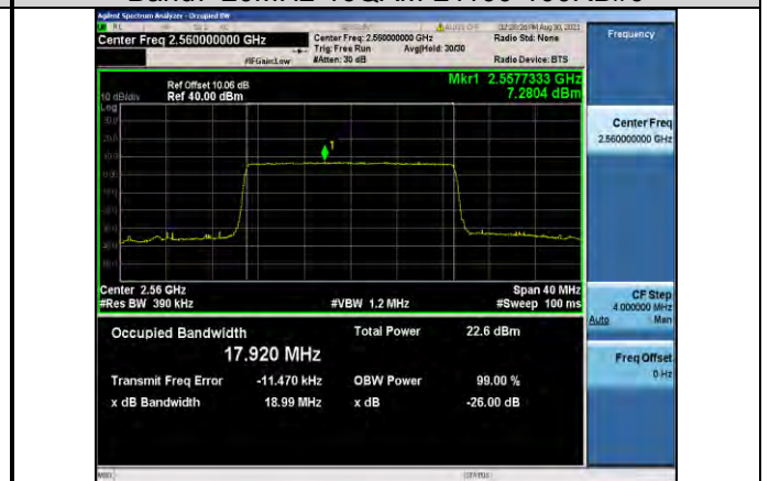
Band7-20MHz-16QAM-21350-100RB#0
