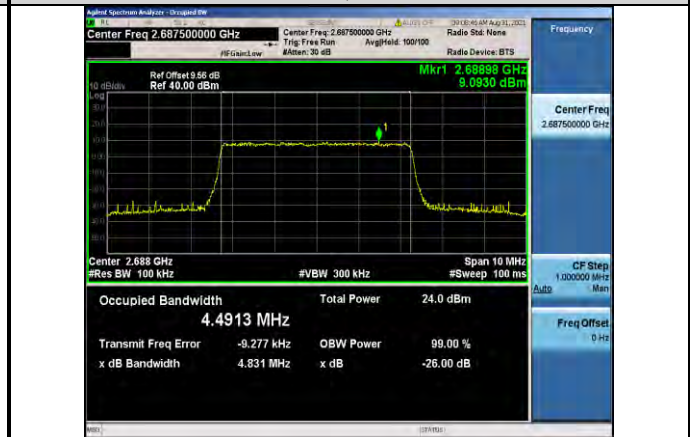
Band41-5MHz-16QAM-41565-25RB#0
