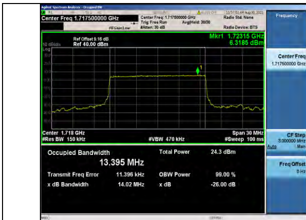
Band4-15MHz-QPSK-20025-75RB#0
