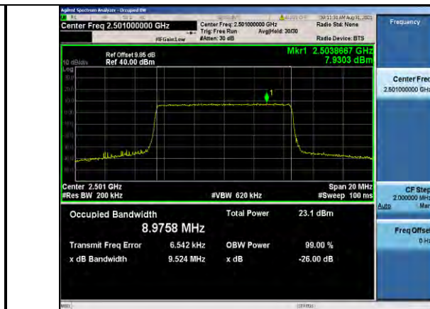
Band41-10MHz-16QAM-39700-50RB#0
