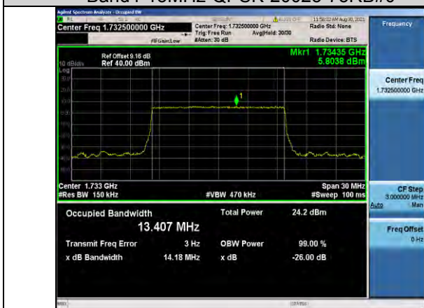
Band4-15MHz-QPSK-20175-75RB#0
