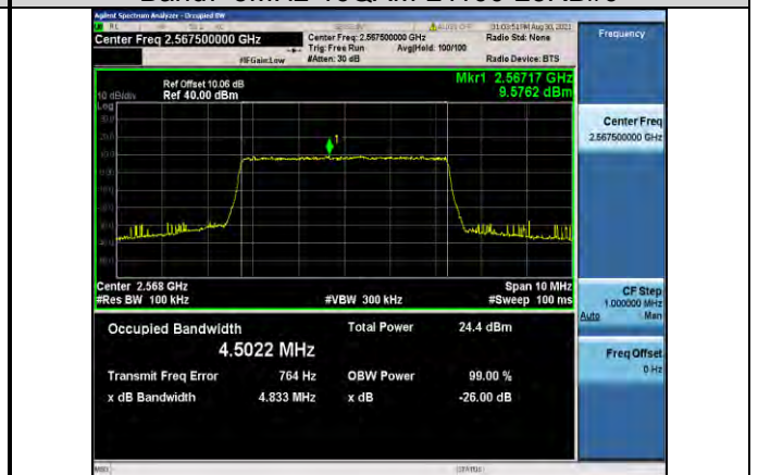
Band7-5MHz-16QAM-21425-25RB#0
