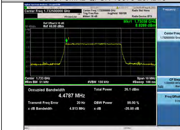
Band4-5MHz-QPSK-17325-25RB#0
