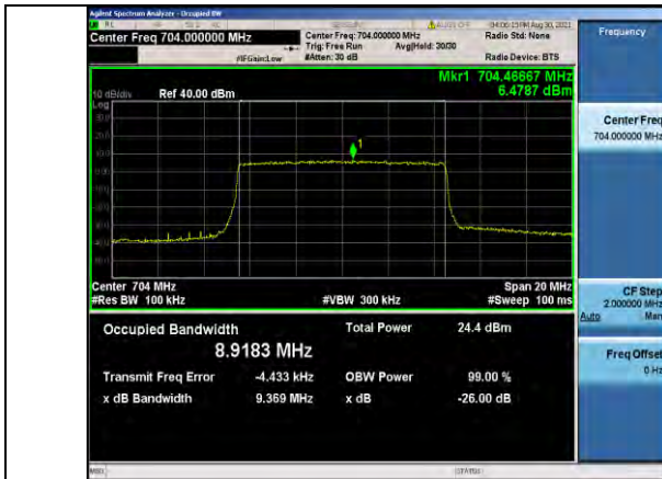
Band12-10MHz-QPSK-23060-50RB#0
