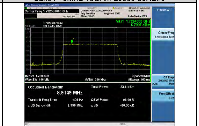
Band4-10MHz-16QAM-20175-50RB#0
