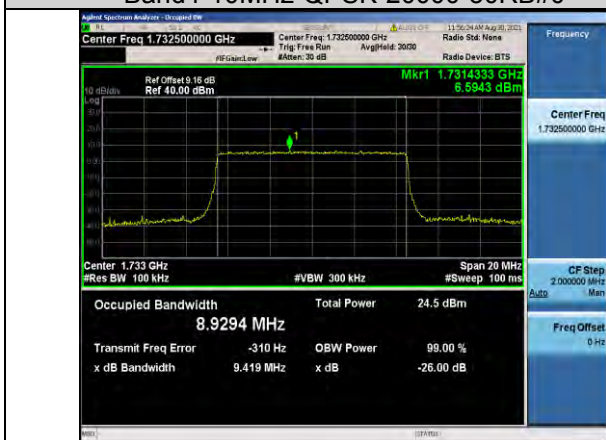
Band4-10MHz-QPSK-20175-50RB#0
