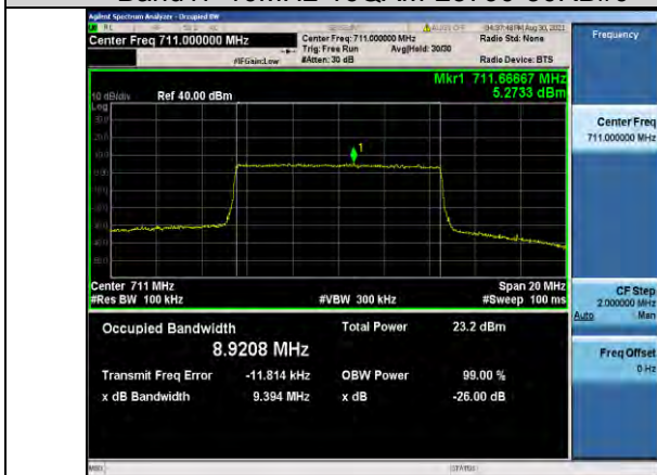
Band17-10MHz-16QAM-23800-50RB#0
