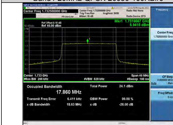
Band4-20MHz-QPSK-20175-100RB#0
