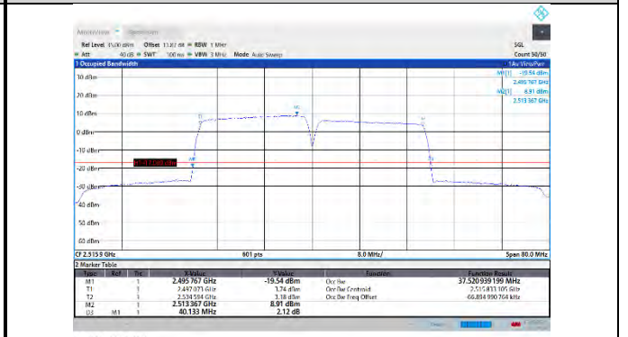
CA_41C-20MHz-20MHz-16QAM-16QAM-39750-39948-100RB#0-100RB#0
