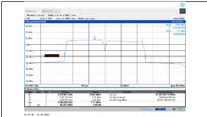
CA_38C-20MHz-20MHz-QPSK-QPSK-37952-38150-100#0-100#0
