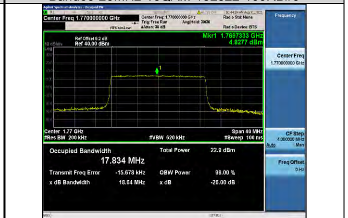
Band66-20MHz-16QAM-132572-100RB#0
