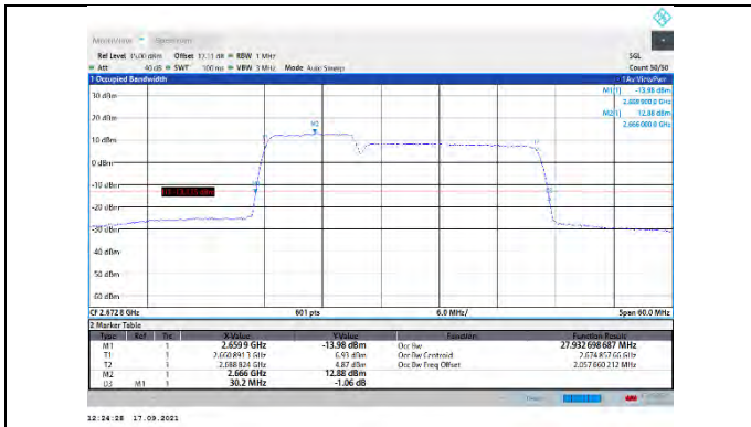
CA_41C-10MHz-20MHz-QPSK-QPSK-41346-41490-50RB#0-100RB#0
