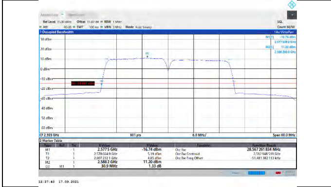
CA_41C-15MHz-15MHz-QPSK-QPSK-40545-40695-75RB#0-75RB#0
