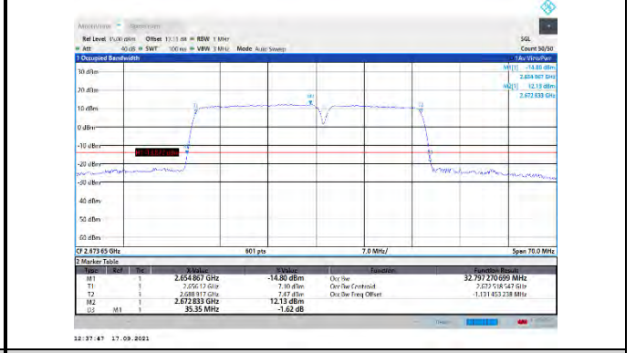
CA_41C-20MHz-15MHz-QPSK-QPSK-413CA_41C512-100RB#0-75RB#0
