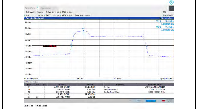
CA_41C-5MHz-20MHz-QPSK-QPSK-39683-39800-25RB#0-100RB#0
