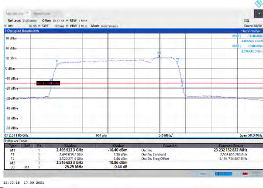
CA_41C-20MHz-5MHz-16QAM-16QAM-39750-39867-100RB#0-25RB#0
