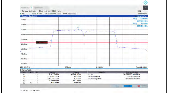
CA_41C-15MHz-15MHz-16QAM-16QAM-40545-40695-75RB#0-75RB#0
