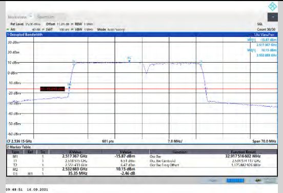
CA_7C-20MHz-15MHz-16QAM-16QAM-21026-21197-100RB#0-75RB#0
