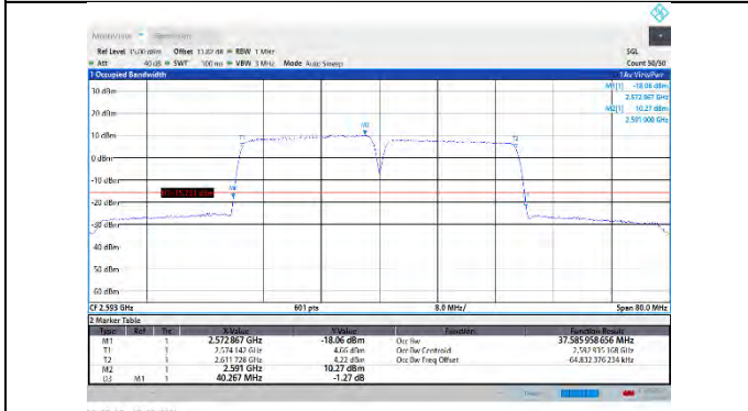
CA_41C-20MHz-20MHz-QPSK-QPSK-40521-40719-100RB#0-100RB#0
