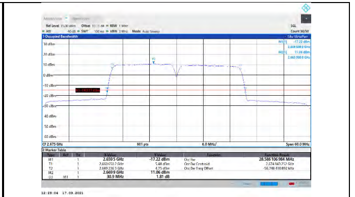
CA_41C-15MHz-15MHz-QPSK-QPSK-41365-41515-75RB#0-75RB#0
