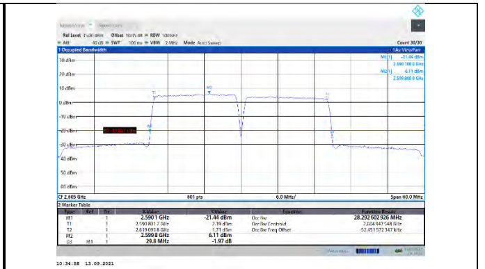
CA_38C-15MHz-15MHz-QPSK-38025-38175-75#0-75#0
