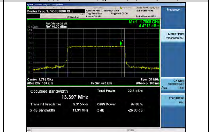
Band66-15MHz-16QAM-132322-75RB#0
