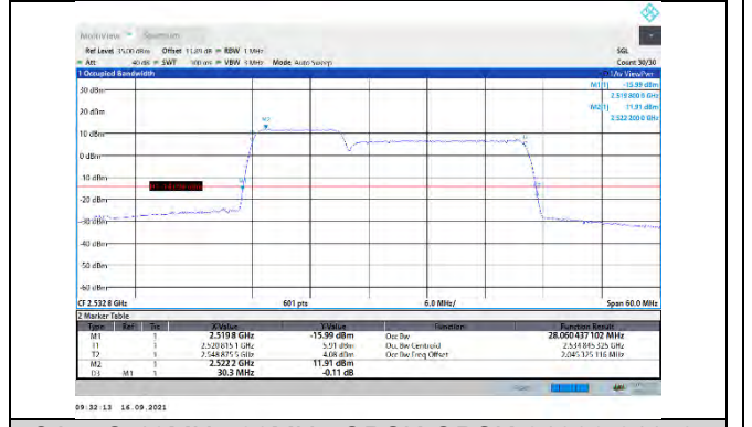
CA_7C-10MHz-20MHz-QPSK-QPSK-21006-21150-50RB#0-100RB#0
