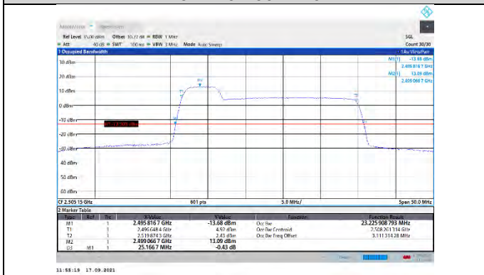
CA_41C-5MHz-20MHz-16QAM-16QAM-39683-39800-25RB#0-100RB#0
