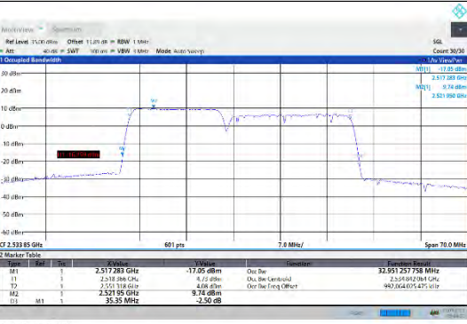
CA_7C-15MHz-20MHz-16QAM-16QAM-21003-21174-75RB#0-100RB#0
