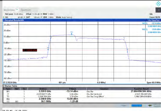
CA_7C-10MHz-20MHz-QPSK-QPSK-21206-21350-50RB#0-100RB#0
