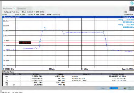
CA_7C-10MHz-20MHz-QPSK-QPSK-21006-21150-50RB#0-100RB#0
