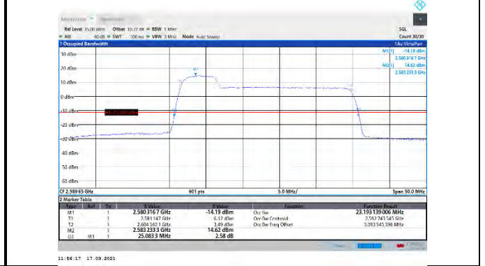
CA_41C-5MHz-20MHz-QPSK-QPSK-40528-40645-25RB#0-100RB#0
