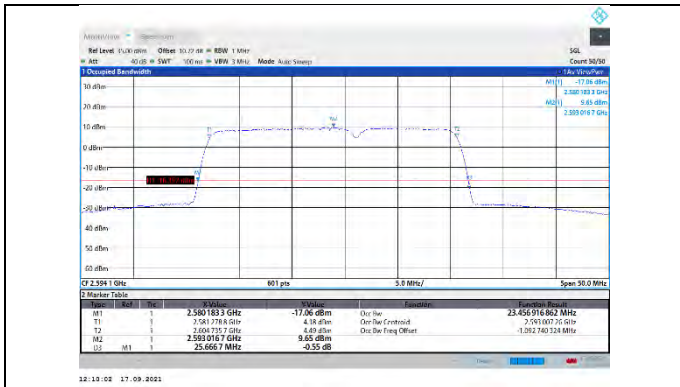
CA_41C-15MHz-10MHz-16QAM-16QAM-40571-40691-75RB#0-50RB#0
