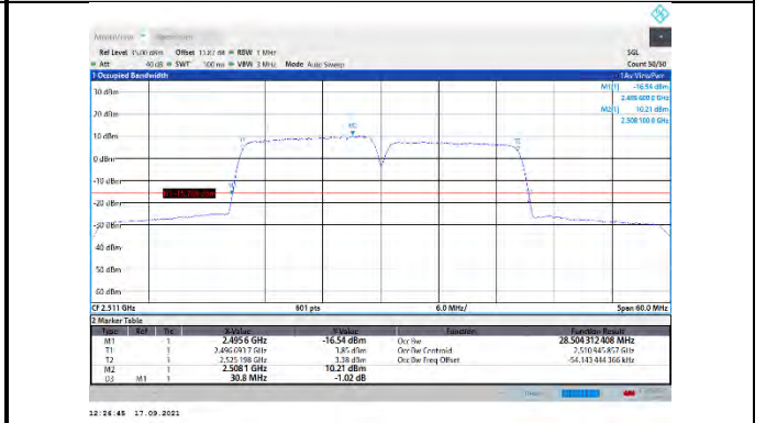
CA_41C-15MHz-15MHz-16QAM-16QAM-39725-39875-75RB#0-75RB#0
