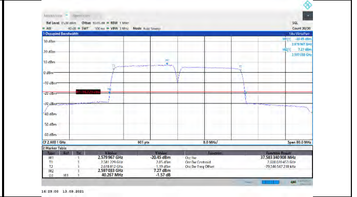
CA_38C-20MHz-20MHz-16QAM-16QAM-37952-38150-100RB#0-100RB#0
