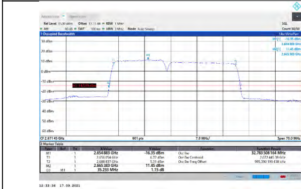
CA_41C-15MHz-20MHz-QPSK-QPSK-41319-41490-75RB#0-100RB#0
