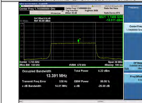
Band66-15MHz-QPSK-132322-75RB#0
