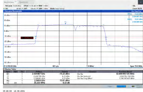
CA_7C-20MHz-15MHz-QPSK-QPSK-21201-21372-100RB#0-75RB#0
