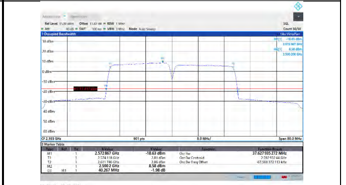
CA_41C-20MHz-20MHz-16QAM-16QAM-40521-40719-100RB#0-100RB#0
