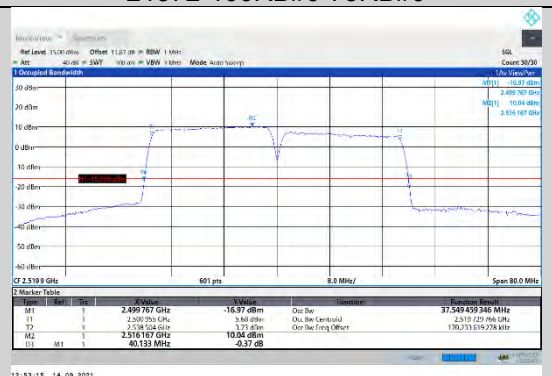
CA_7C-20MHz-20MHz-QPSK-QPSK-20850-21048-100RB#0-100RB#0
