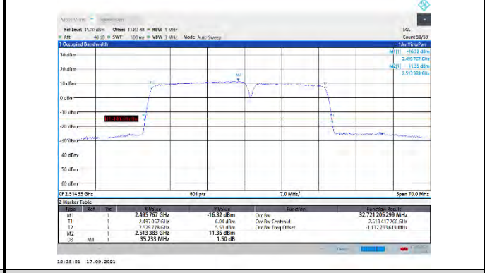
CA_41C-20MHz-15MHz-16QAM-16QAM-39750-39921-100RB#0-75RB#0
