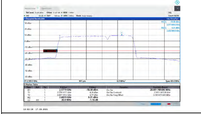
CA_41C-20MHz-10MHz-16QAM-16QAM-40571-40715-100RB#0-50RB#0
