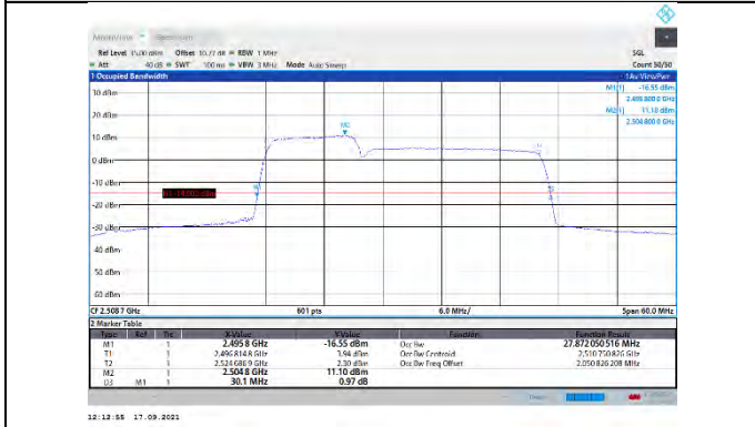
CA_41C-10MHz-20MHz-16QAM-16QAM-39705-39849-50RB#0-100RB#0
