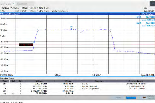
CA_7C-15MHz-10MHz-QPSK-QPSK-21051-21171-75RB#0-50RB#0
