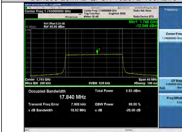
Band66-20MHz-QPSK-132322-100RB#0
