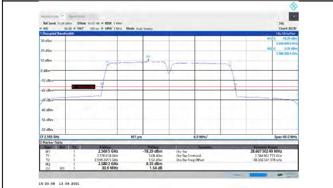
CA_38C-15MHz-15MHz-QPSK-QPSK-37825-37975-75RB#0-75RB#0
