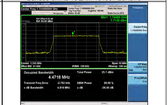
Band66-5MHz-16QAM-132322-25RB#0
