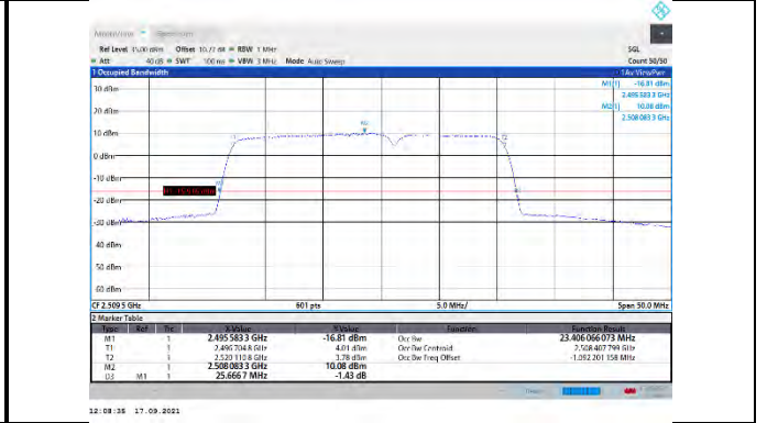
CA_41C-15MHz-10MHz-16QAM-16QAM-39725-39845-75RB#0-50RB#0
