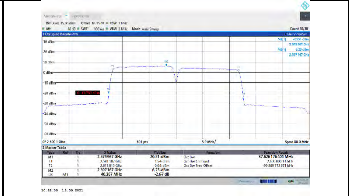
CA_38C-20MHz-20MHz-16QAM-16QAM-37952-38150-100#0-100#0
