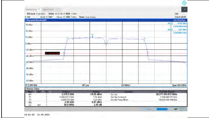
CA_38C-15MHz-15MHz-QPSK-QPSK-37925-38075-75RB#0-75RB#0
