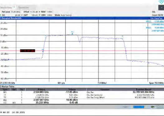
CA_7C-15MHz-20MHz-16QAM-16QAM-21179-21350-75RB#0-100RB#0
