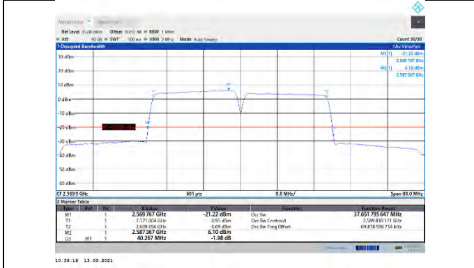
CA_38C-20MHz-20MHz-16QAM-16QAM-37850-38048-100#0-100#0
