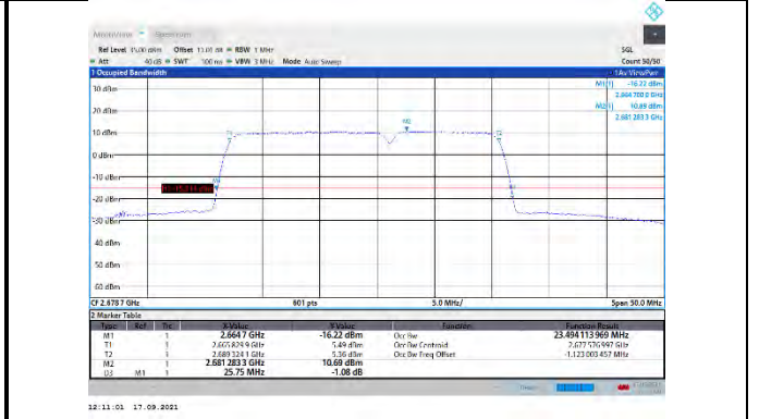
CA_41C-15MHz-10MHz-QPSK-QPSK-41417-4153CA_38C5RB#0-50RB#0
