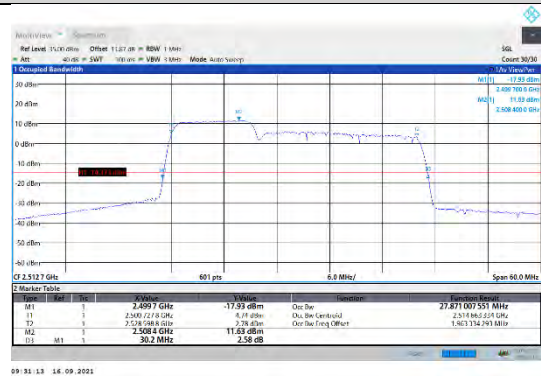
CA_7C-10MHz-20MHz-16QAM-16QAM-20805-20949-50RB#0-100RB#0
