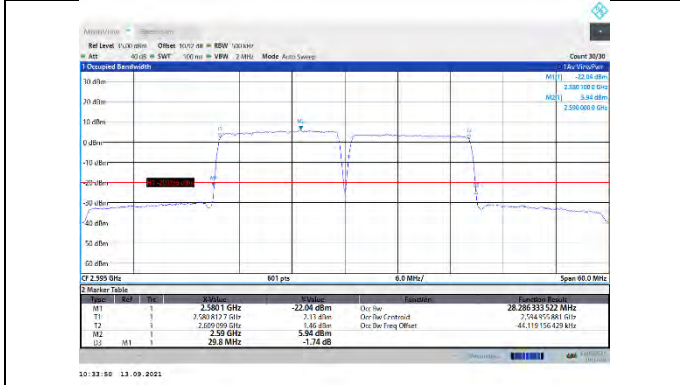
CA_38C-15MHz-15MHz-QPSK-QPSK-37925-38075-75#0-75#0
