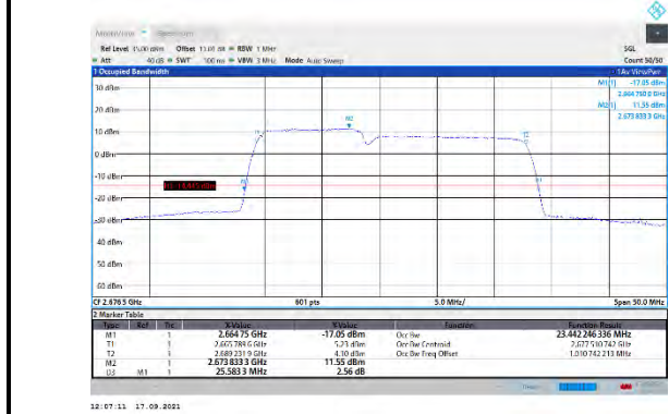
CA_41C-10MHz-15MHz-16QAM-16QAM-41395-41515-50RB#0-75RB#0
