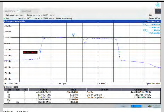
CA_7C-20MHz-15MHz-16QAM-16QAM-21201-21372-100RB#0-75RB#0
