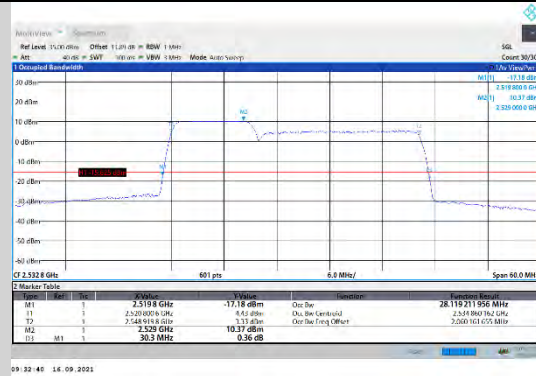
CA_7C-10MHz-20MHz-16QAM-16QAM-21150-50RB#0-100RB#0
