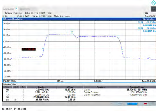
CA_41C-10MHz-15MHz-QPSK-QPSK-40549-40669-50RB#0-75RB#0
