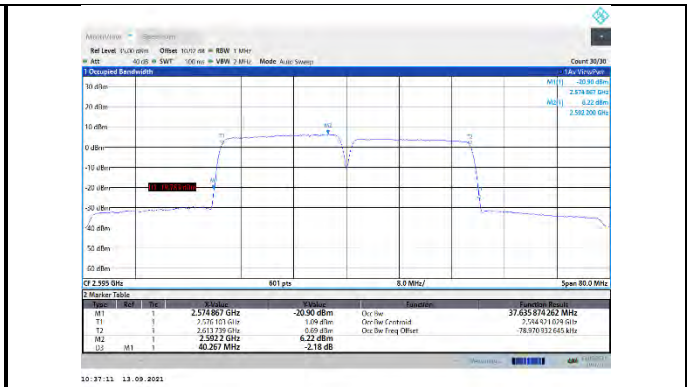
CA_38C-20MHz-20MHz-16QAM-16QAM-37901-38099-100#0-100#0
