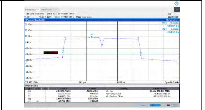
CA_41C-20MHz-20MHz-16QAM-16QAM-41292-41490-100RB#0-100RB#0
