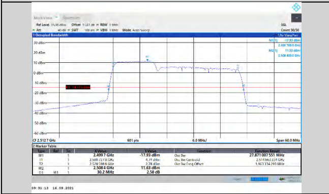
CA_7C-10MHz-20MHz-16QAM-16QAM-20805-20949-50RB#0-100RB#0
