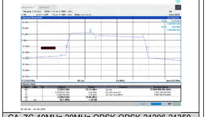
CA_7C-10MHz-20MHz-QPSK-QPSK-21206-21350-50RB#0-100RB#0
