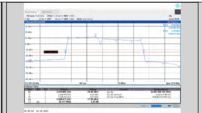
CA_7C-15MHz-20MHz-QPSK-QPSK-21179-21350-75RB#0-100RB#0
