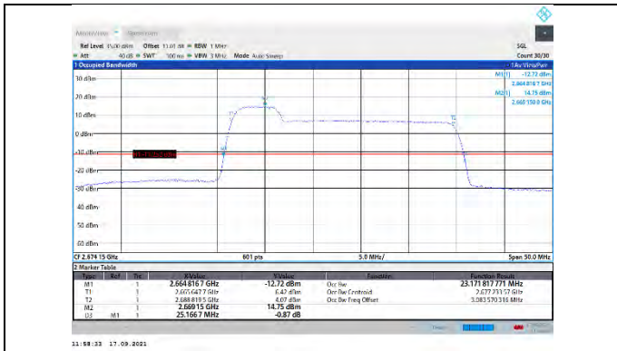
CA_41C-5MHz-20MHz-QPSK-QPSK-41373-41490-25RB#0-100RB#0
