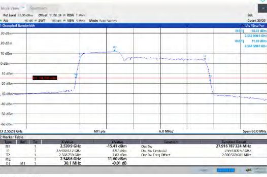
CA_7C-10MHz-20MHz-16QAM-16QAM-21206-21350-50RB#0-100RB#0
