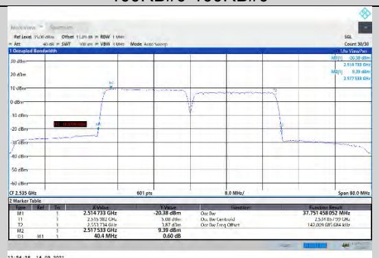
CA_7C-20MHz-20MHz-QPSK-QPSK-21001-21199-100RB#0-100RB#0
