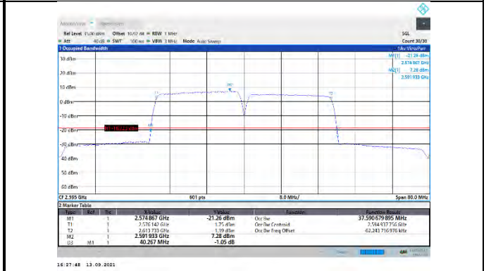
CA_38C-20MHz-20MHz-16QAM-16QAM-37901-38099-100RB#0-100RB#0
