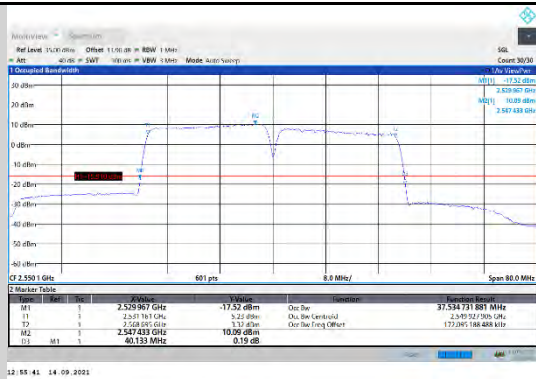
CA_7C-20MHz-20MHz-QPSK-QPSK-21152-21350-100RB#0-100RB#0
