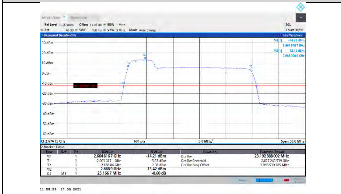
CA_41C-5MHz-20MHz-16QAM-16QAM-41373-41490-25RB#0-100RB#0
