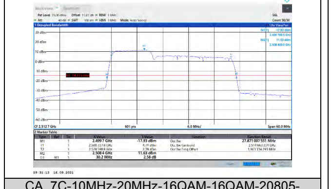
CA_7C-10MHz-20MHz-16QAM-16QAM-20805-20949-50RB#0-100RB#0
