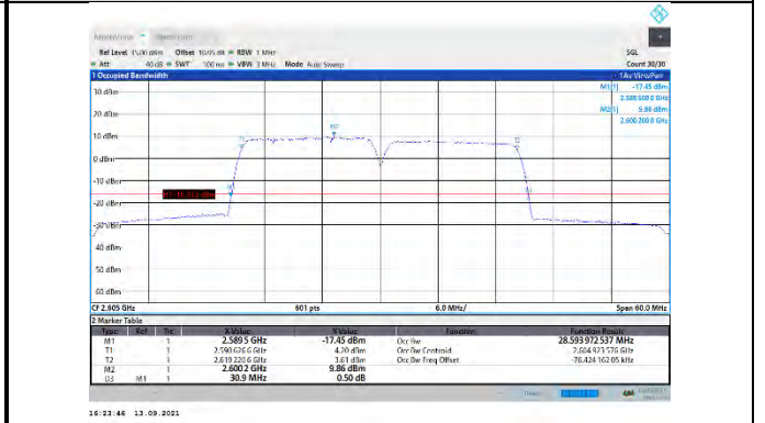
CA_38C-15MHz-15MHz-QPSK-QPSK-38025-38175-75RB#0-75RB#0
