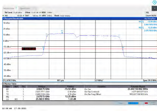
CA_41C-10MHz-15MHz-QPSK-QPSK-41395-41515-50RB#0-75RB#0
