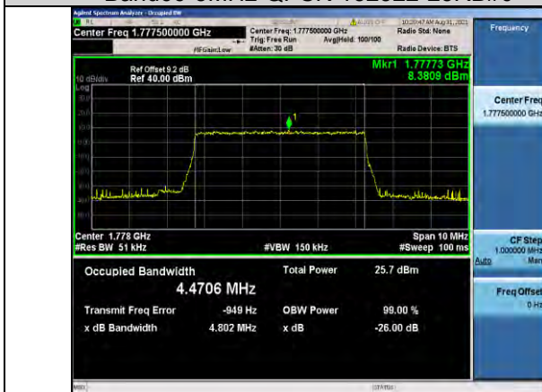
Band66-5MHz-QPSK-132647-25RB#0
