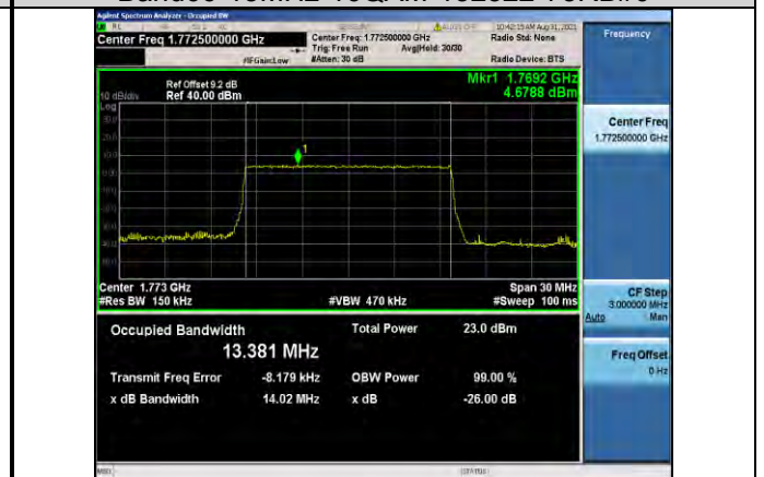
Band66-15MHz-16QAM-132597-75RB#0
