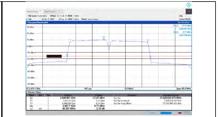
CA_41C-20MHz-20MHz-QPSK-QPSK-41292-41490-100RB#0-100RB#0
