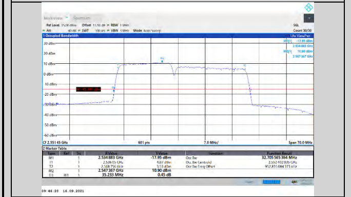
CA_7C-15MHz-20MHz-16QAM-16QAM-21179-21350-75RB#0-100RB#0
