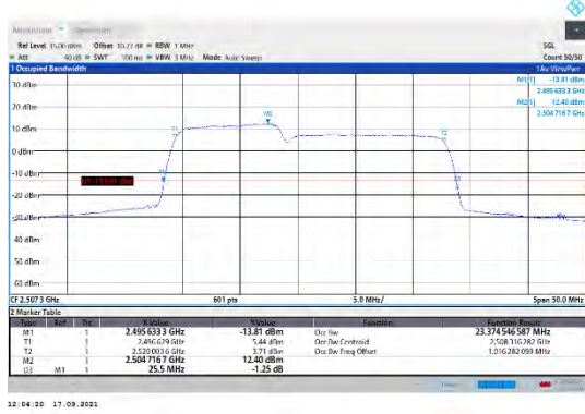
CA_41C-10MHz-15MHz-16QAM-16QAM-39703-39823-50RB#0-75RB#0
