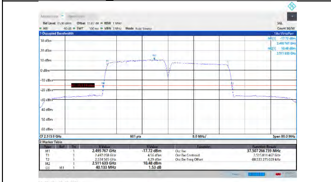
CA_41C-20MHz-20MHz-QPSK-QPSK-39750-39948-100RB#0-100RB#0
