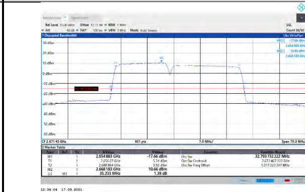
CA_41C-15MHz-20MHz-16QAM-16QAM-41319-41490-75RB#0-100RB#0
