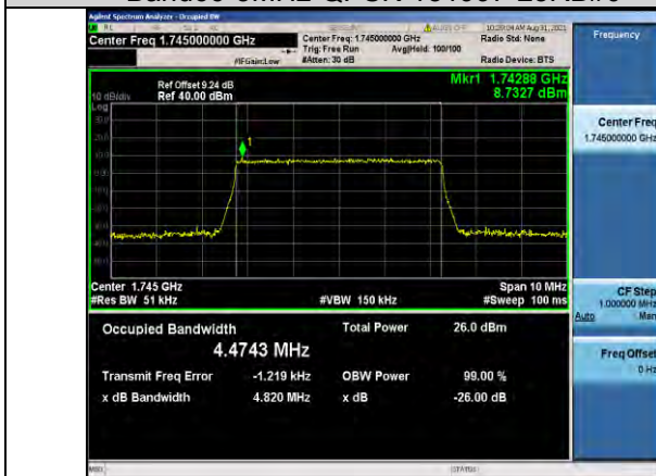
Band66-5MHz-QPSK-132322-25RB#0
