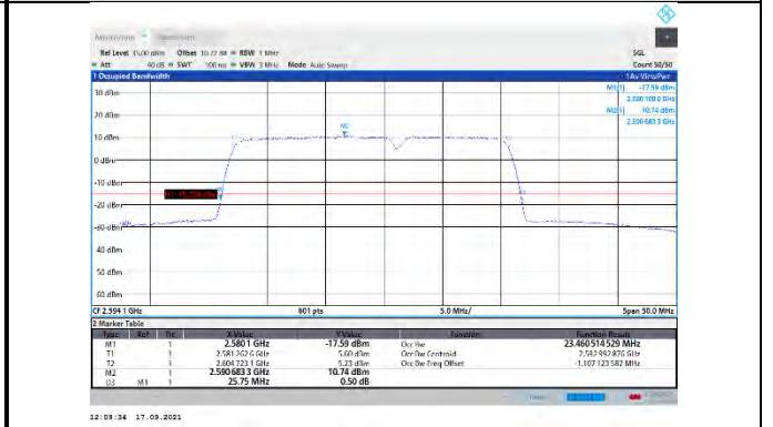
CA_41C-15MHz-10MHz-QPSK-QPSK-40571-40691-75RB#0-50RB#0
