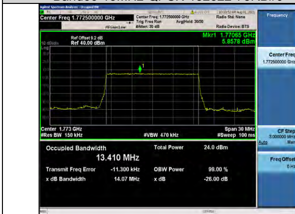
Band66-15MHz-QPSK-132597-75RB#0
