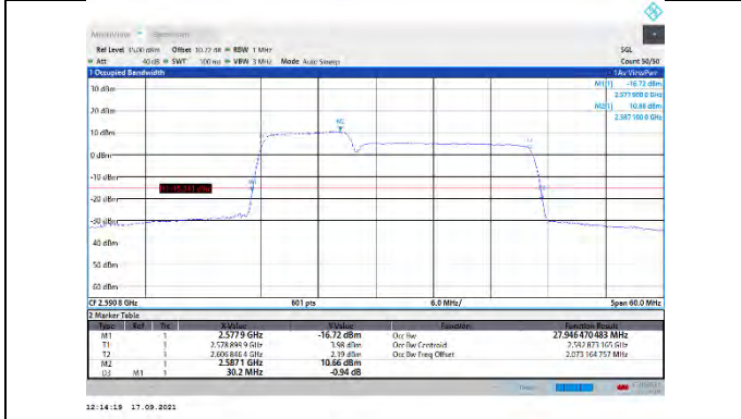
CA_41C-10MHz-20MHz-16QAM-16QAM-40526-40670-50RB#0-100RB#0
