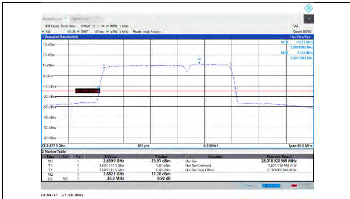
CA_41C-20MHz-10MHz-QPSK-QPSK-41391-41535-100RB#0-50RB#0
