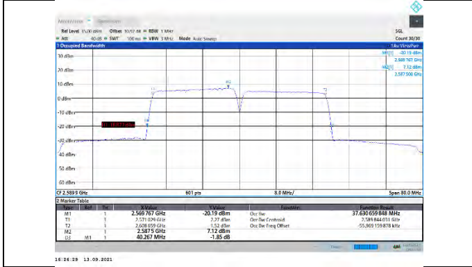
CA_38C-20MHz-20MHz-16QAM-16QAM-37850-38048-100RB#0-100RB#0
