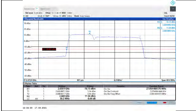
CA_41C-10MHz-20MHz-16QAM-16QAM-41346-41490-50RB#0-100RB#0
