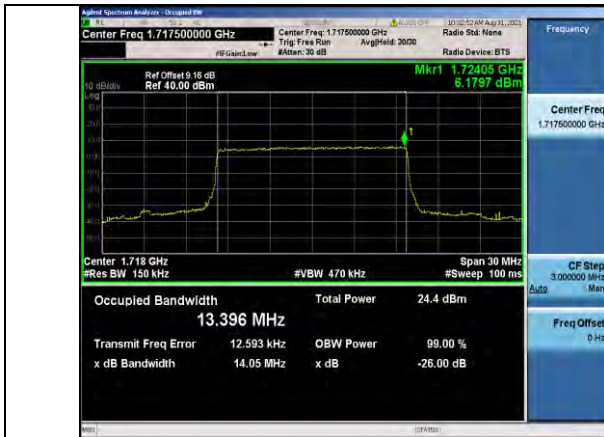
Band66-15MHz-QPSK-132047-75RB#0
