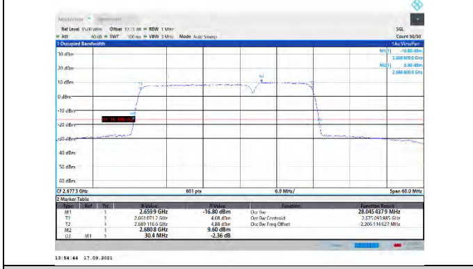
CA_41C-20MHz-10MHz-16QAM-16QAM-41391-41535-100RB#0-50RB#0
