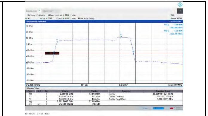
CA_41C-20MHz-5MHz-16QAM-16QAM-40595-40712-100RB#0-25RB#0
