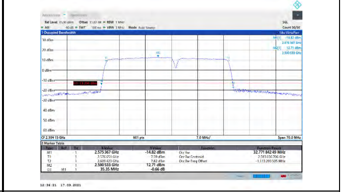
CA_41C-20MHz-15MHz-QPSK-QPSK-40546-40717-100RB#0-75RB#0
