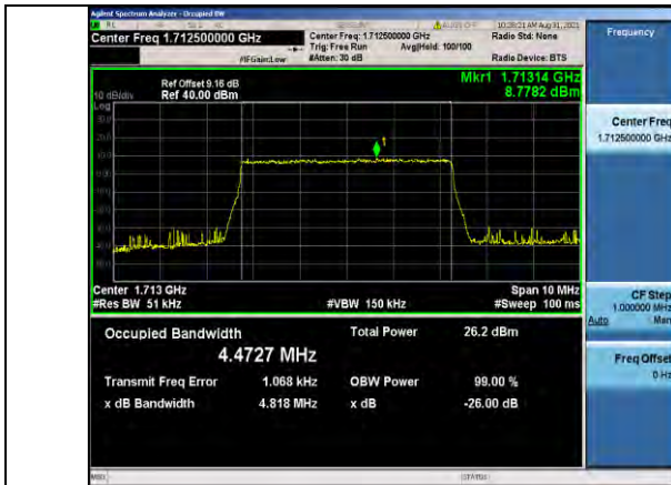
Band66-5MHz-QPSK-131997-25RB#0
