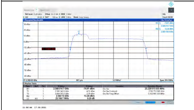
CA_41C-5MHz-20MHz-16QAM-16QAM-40528-40645-25RB#0-100RB#0
