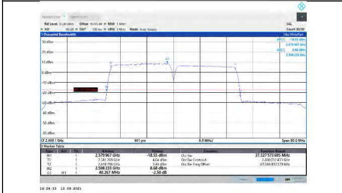
CA_38C-20MHz-20MHz-QPSK-QPSK-37952-38150-100RB#0-100RB#0
