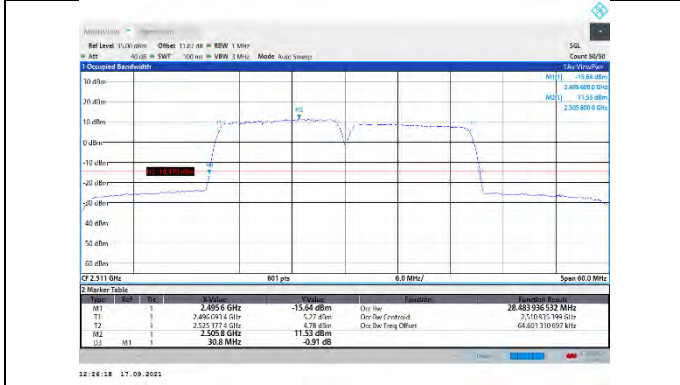
CA_41C-15MHz-15MHz-QPSK-QPSK-39725-39875-75RB#0-75RB#0
