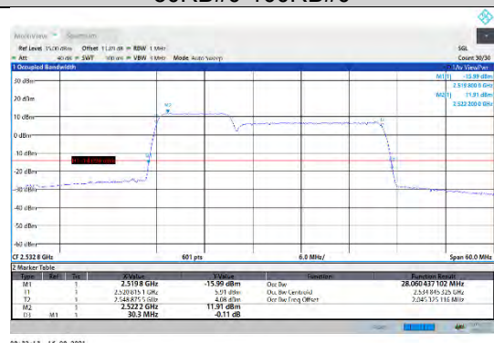
CA_7C-10MHz-20MHz-QPSK-QPSK-21006-21150-50RB#0-100RB#0
