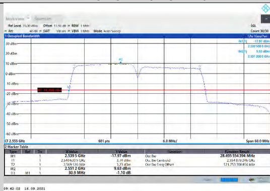
CA_7C-15MHz-15MHz-16QAM-16QAM-21225-21375-75RB#0-75RB#0
