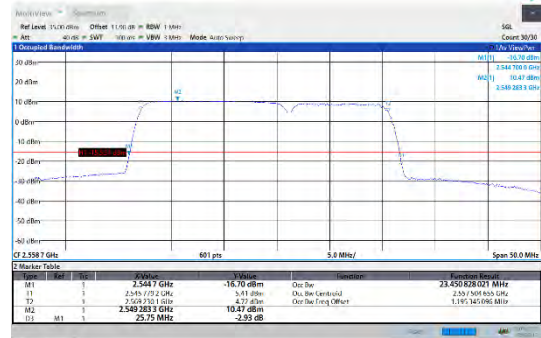
CA_7C-15MHz-10MHz-16QAM-16QAM-21277-2139CA_7C5RB#0-50RB#0
