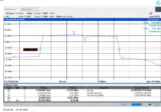
CA_7C-20MHz-15MHz-QPSK-QPSK-21201-21372-100RB#0-75RB#0
