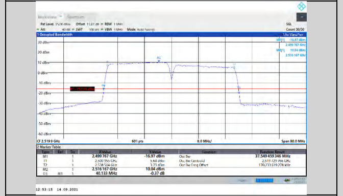
CA_7C-20MHz-20MHz-QPSK-QPSK-20850-21048-100RB#0-100RB#0
