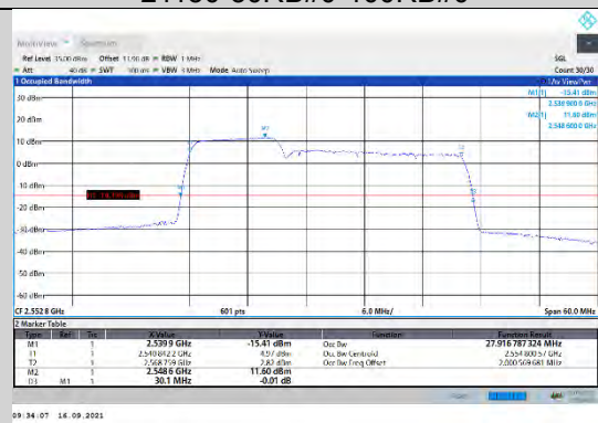
CA_7C-10MHz-20MHz-16QAM-16QAM-21206-21350-50RB#0-100RB#0
