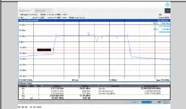
CA_7C-20MHz-15MHz-QPSK-QPSK-21026-21197-100RB#0-75RB#0
