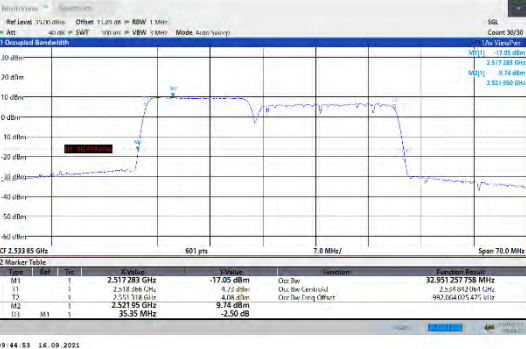
CA_7C-15MHz-20MHz-16QAM-16QAM-21003-21174-75RB#0-100RB#0
