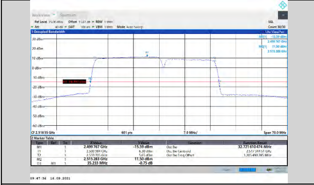
CA_7C-20MHz-15MHz-16QAM-16QAM-20850-21021-100RB#0-75RB#0
