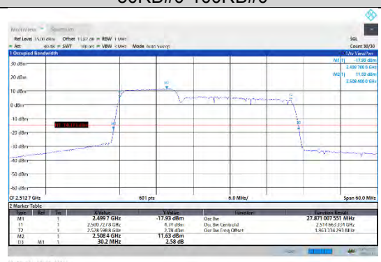
CA_7C-10MHz-20MHz-16QAM-16QAM-20805-20949-50RB#0-100RB#0
