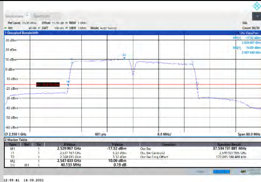
CA_7C-20MHz-20MHz-QPSK-QPSK-21152-21350-100RB#0-100RB#0
