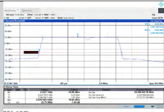
CA_7C-15MHz-10MHz-QPSK-QPSK-21051-21171-75RB#0-50RB#0
