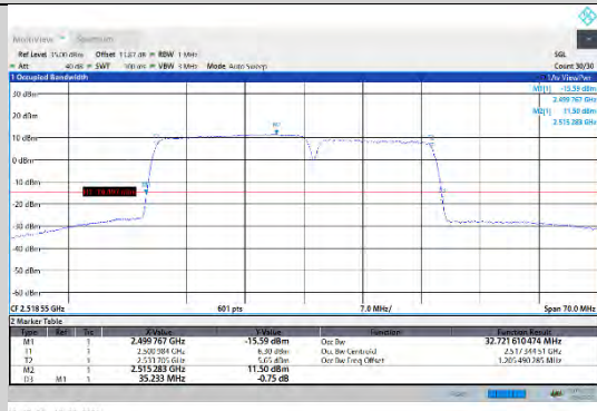
CA_7C-20MHz-15MHz-16QAM-16QAM-20850-21021-100RB#0-75RB#0
