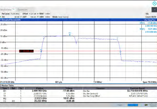
CA_7C-15MHz-20MHz-16QAM-16QAM-20828-20999-75RB#0-100RB#0
