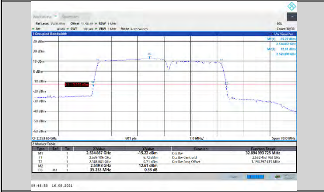
CA_7C-20MHz-15MHz-QPSK-QPSK-21201-21372-100RB#0-75RB#0
