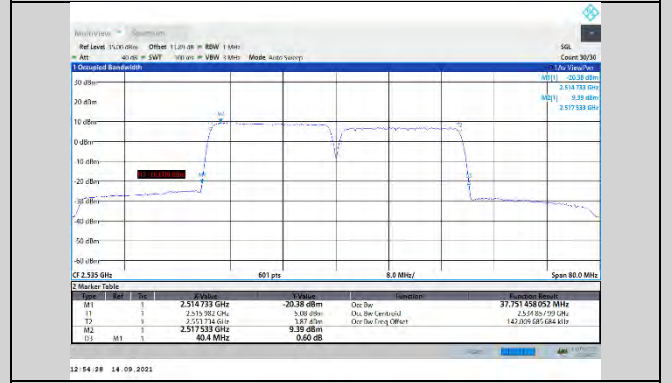
CA_7C-20MHz-20MHz-QPSK-QPSK-21001-21199-100RB#0-100RB#0
