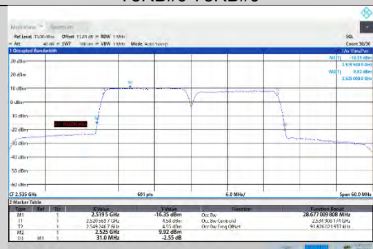
CA_7C-15MHz-15MHz-QPSK-QPSK-21025-21175-75RB#0-75RB#0
