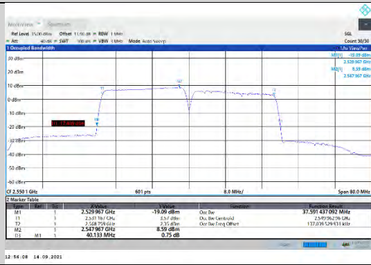
CA_7C-20MHz-20MHz-16QAM-16QAM-21152-21350-100RB#0-100RB#0
