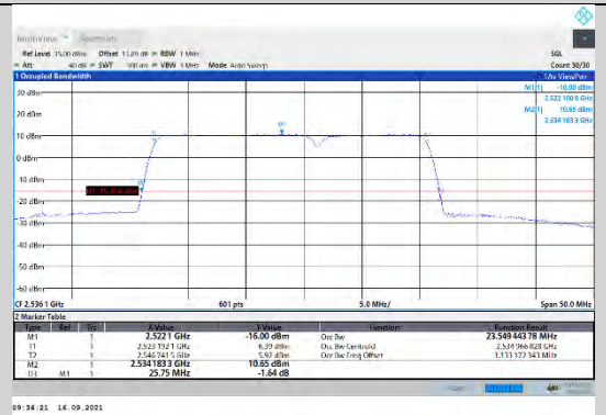
CA_7C-15MHz-10MHz-QPSK-QPSK-21051-21171-75RB#0-50RB#0
