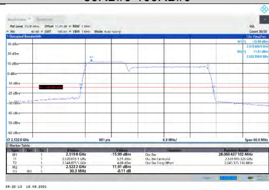
CA_7C-10MHz-20MHz-QPSK-QPSK-21006-21150-50RB#0-100RB#0
