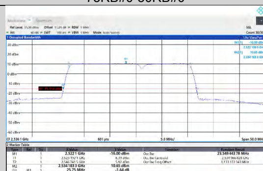
CA_7C-15MHz-10MHz-QPSK-QPSK-20825-20945-75RB#0-50RB#0
