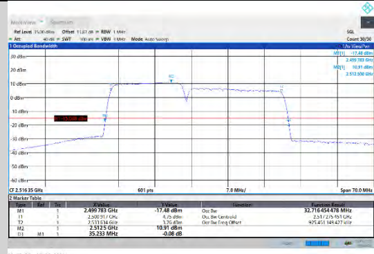
CA_7C-15MHz-20MHz-16QAM-16QAM-20828-20999-75RB#0-100RB#0
