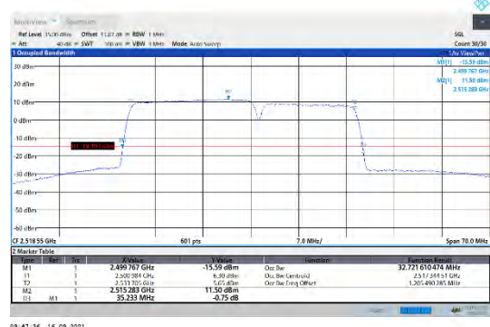
CA_7C-20MHz-15MHz-16QAM-16QAM-20850-21021-100RB#0-75RB#0
