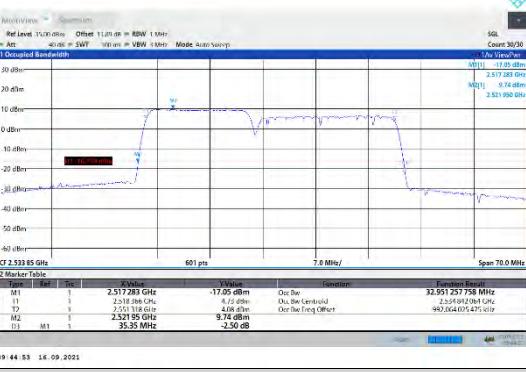
CA_7C-15MHz-20MHz-16QAM-16QAM-21003-21174-75RB#0-100RB#0
