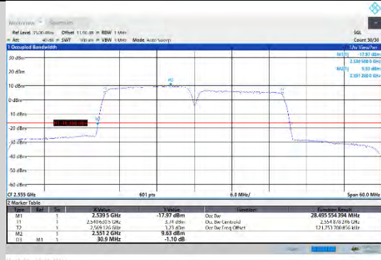
CA_7C-15MHz-15MHz-16QAM-16QAM-21225-21375-75RB#0-75RB#0
