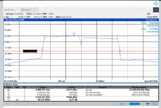
CA_7C-20MHz-20MHz-QPSK-QPSK-20850-21048-100RB#0-100RB#0
