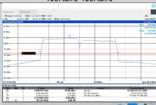
CA_7C-20MHz-20MHz-16QAM-16QAM-20850-21048-100RB#0-100RB#0
