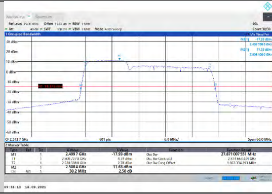
CA_7C-10MHz-20MHz-16QAM-16QAM-20805-20949-50RB#0-100RB#0
