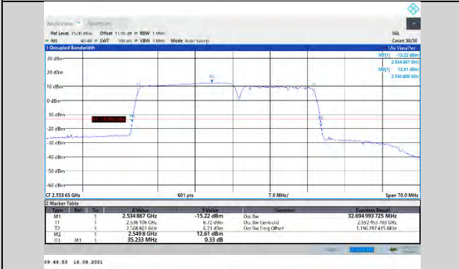
CA_7C-20MHz-15MHz-QPSK-QPSK-21201-21372-100RB#0-75RB#0
