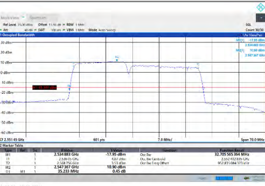
CA_7C-15MHz-20MHz-16QAM-16QAM-21179-21350-75RB#0-100RB#0
