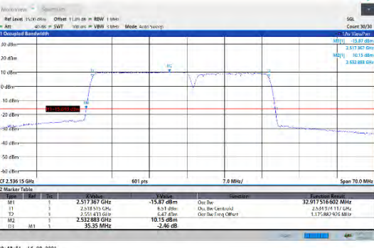
CA_7C-20MHz-15MHz-16QAM-16QAM-21026-21197-100RB#0-75RB#0
