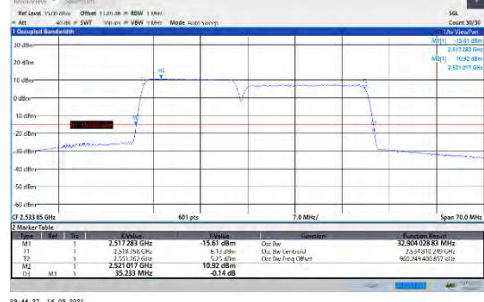
CA_7C-15MHz-20MHz-QPSK-QPSK-21003-21174-75RB#0-100RB#0
