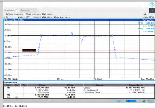
CA_7C-20MHz-15MHz-16QAM-16QAM-21026-21197-100RB#0-75RB#0
