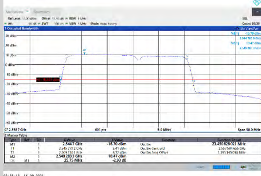
CA_7C-15MHz-10MHz-16QAM-16QAM-21277-2139CA_7C5RB#0-50RB#0
