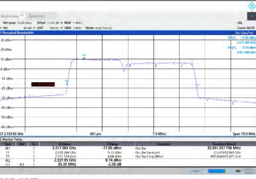
CA_7C-15MHz-20MHz-16QAM-16QAM-21003-21174-75RB#0-100RB#0
