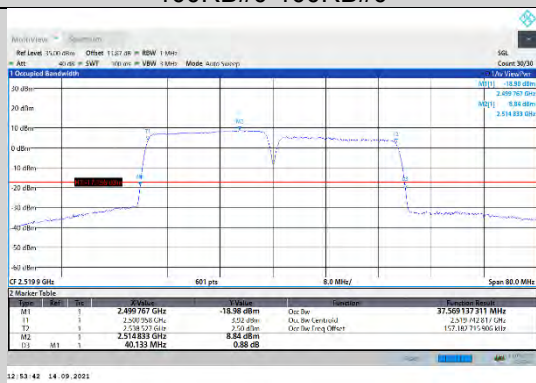
CA_7C-20MHz-20MHz-16QAM-16QAM-20850-21048-100RB#0-100RB#0
