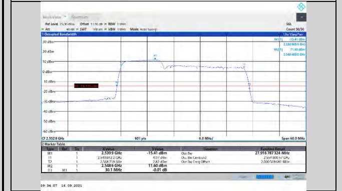
CA_7C-10MHz-20MHz-16QAM-16QAM-21206-21350-50RB#0-100RB#0
