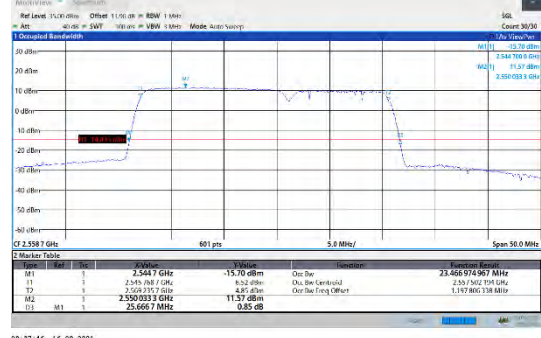
CA_7C-15MHz-10MHz-QPSK-QPSK-21277-2139CA_7C5RB#0-50RB#0
