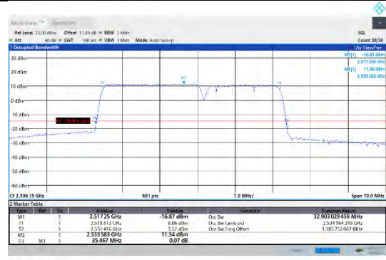
CA_7C-20MHz-15MHz-QPSK-QPSK-21026-21197-100RB#0-75RB#0
