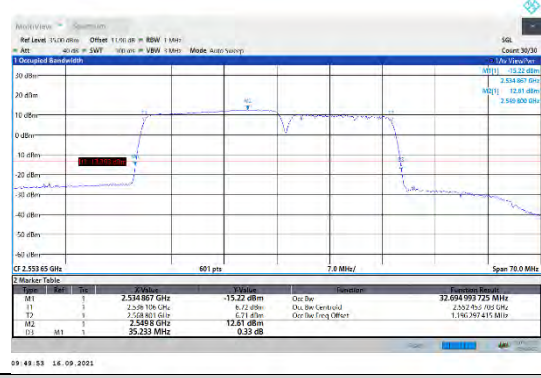
CA_7C-20MHz-15MHz-QPSK-QPSK-21201-21372-100RB#0-75RB#0
