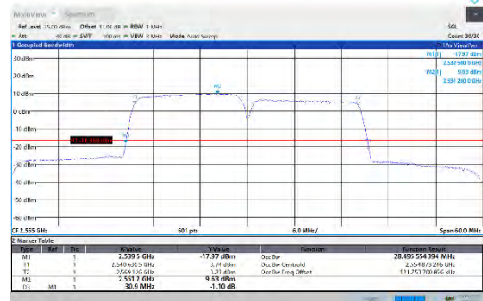
CA_7C-15MHz-15MHz-16QAM-16QAM-21225-21375-75RB#0-75RB#0
