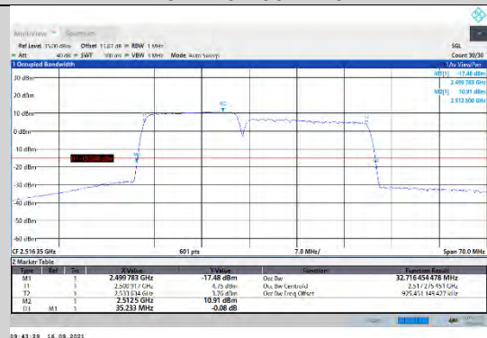
CA_7C-15MHz-20MHz-16QAM-16QAM-20828-20999-75RB#0-100RB#0
