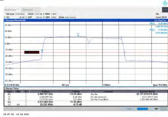
CA_7C-20MHz-15MHz-16QAM-16QAM-20850-21021-100RB#0-75RB#0
