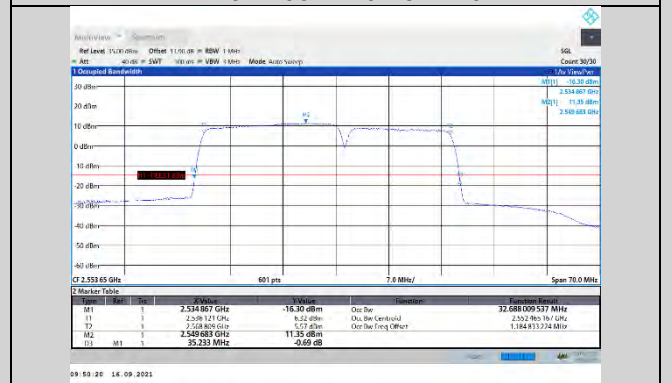
CA_7C-20MHz-15MHz-16QAM-16QAM-21201-21372-100RB#0-75RB#0
