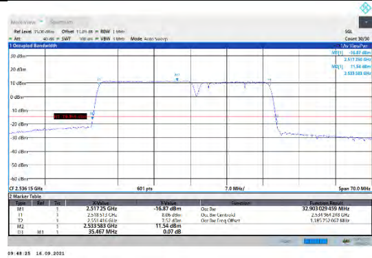
CA_7C-20MHz-15MHz-QPSK-QPSK-21026-21197-100RB#0-75RB#0
