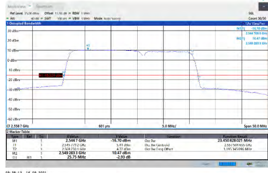
CA_7C-15MHz-10MHz-16QAM-16QAM-21277-2139CA_7C5RB#0-50RB#0
