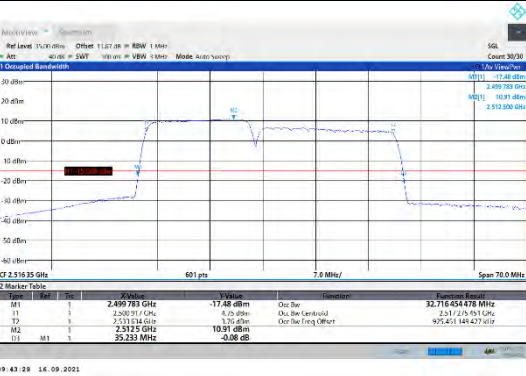
CA_7C-15MHz-20MHz-16QAM-16QAM-20828-20999-75RB#0-100RB#0
