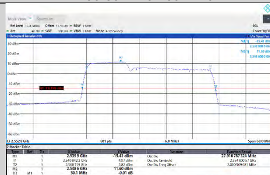
CA_7C-10MHz-20MHz-16QAM-16QAM-21150-50RB#0-100RB#0
