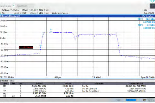
CA_7C-15MHz-20MHz-16QAM-16QAM-21003-21174-75RB#0-100RB#0
