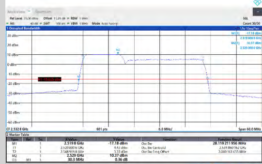
CA_7C-10MHz-20MHz-16QAM-16QAM-21150-50RB#0-100RB#0
