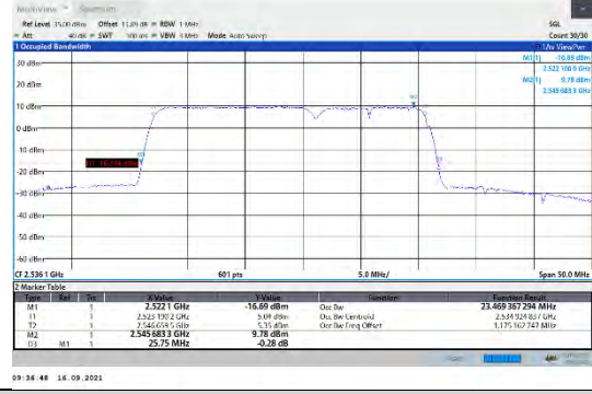
CA_7C-15MHz-10MHz-16QAM-16QAM-21051-21171-75RB#0-50RB#0
