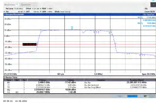
CA_7C-15MHz-10MHz-16QAM-16QAM-20825-20945-75RB#0-50RB#0
