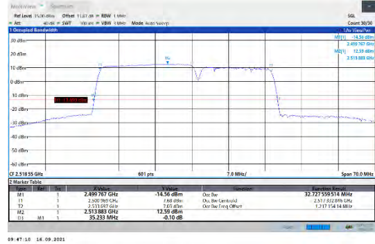
CA_7C-20MHz-15MHz-QPSK-QPSK-20850-21021-100RB#0-75RB#0
