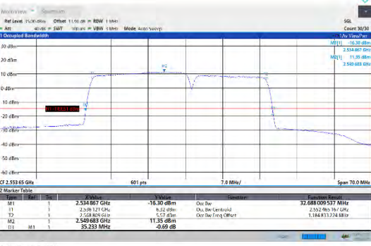
CA_7C-20MHz-15MHz-16QAM-16QAM-21201-21372-100RB#0-75RB#0
