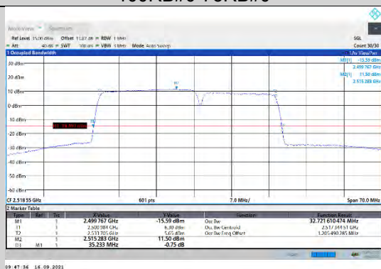
CA_7C-20MHz-15MHz-16QAM-16QAM-20850-21021-100RB#0-75RB#0
