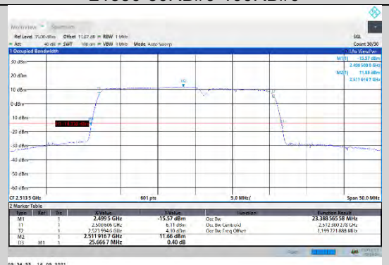
CA_7C-15MHz-10MHz-QPSK-QPSK-20825-20945-75RB#0-50RB#0
