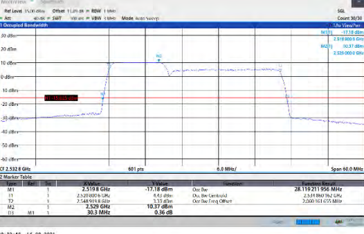
CA_7C-10MHz-20MHz-16QAM-16QAM-21006-21150-50RB#0-100RB#0
