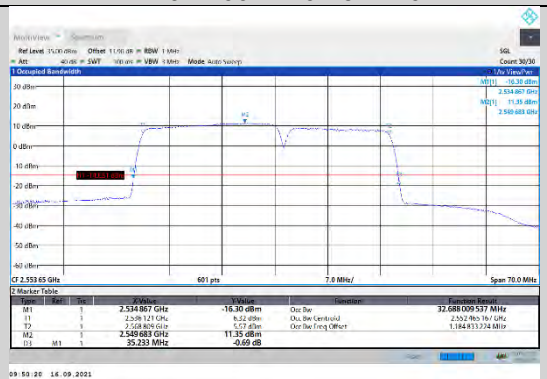
CA_7C-20MHz-15MHz-16QAM-16QAM-21201-21372-100RB#0-75RB#0
