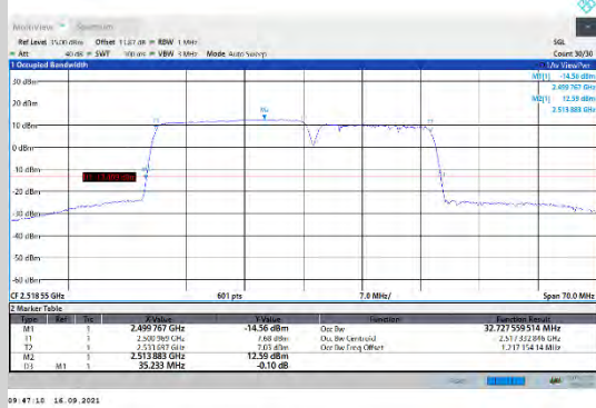
CA_7C-20MHz-15MHz-QPSK-QPSK-20850-21021-100RB#0-75RB#0
