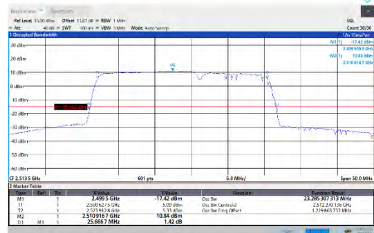
CA_7C-15MHz-10MHz-16QAM-16QAM-20825-20945-75RB#0-50RB#0
