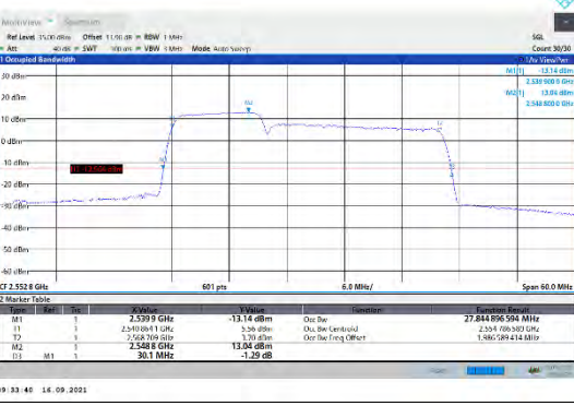
CA_7C-10MHz-20MHz-QPSK-QPSK-21206-21350-50RB#0-100RB#0
