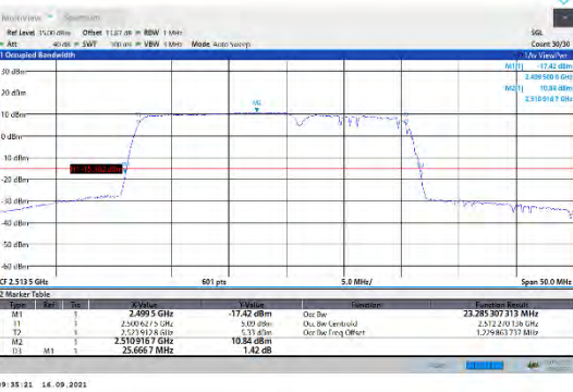
CA_7C-15MHz-10MHz-16QAM-16QAM-20825-20945-75RB#0-50RB#0
