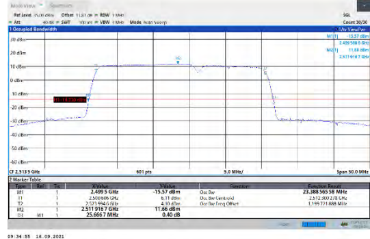
CA_7C-15MHz-10MHz-QPSK-QPSK-20825-20945-75RB#0-50RB#0
