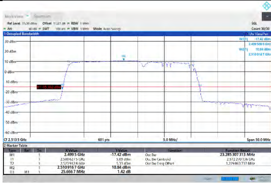
CA_7C-15MHz-10MHz-16QAM-16QAM-20825-20945-75RB#0-50RB#0
