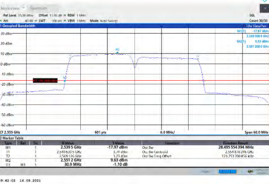
CA_7C-15MHz-15MHz-16QAM-16QAM-21225-21375-75RB#0-75RB#0
