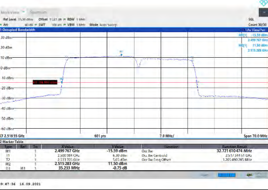
CA_7C-20MHz-15MHz-16QAM-16QAM-20850-21021-100RB#0-75RB#0
