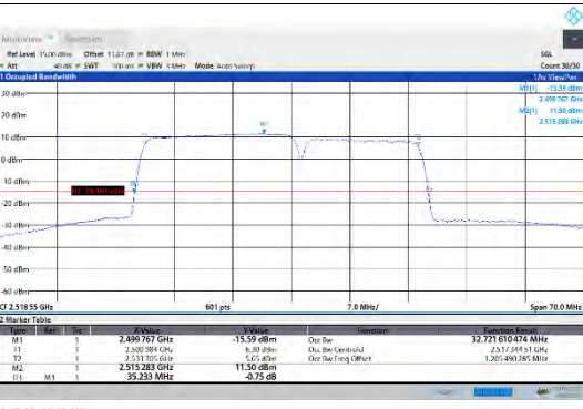
CA_7C-20MHz-15MHz-16QAM-16QAM-20850-21021-100RB#0-75RB#0
