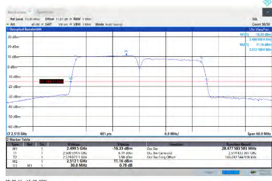
CA_7C-15MHz-15MHz-QPSK-QPSK-20825-20975-75RB#0-75RB#0
