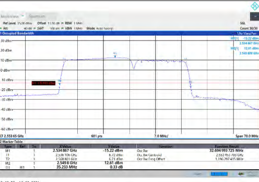
CA_7C-20MHz-15MHz-QPSK-QPSK-21201-21372-100RB#0-75RB#0
