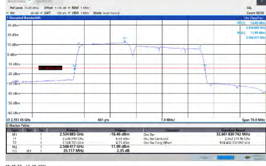
CA_7C-15MHz-20MHz-QPSK-QPSK-21179-21350-75RB#0-100RB#0
