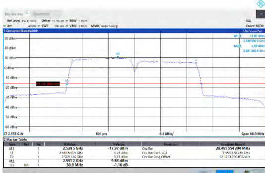
CA_7C-15MHz-15MHz-16QAM-16QAM-21225-21375-75RB#0-75RB#0
