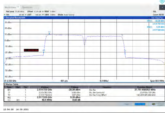
CA_7C-20MHz-20MHz-QPSK-QPSK-21001-21199-100RB#0-100RB#0
