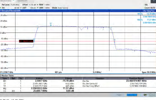
CA_7C-15MHz-10MHz-QPSK-QPSK-21277-2139CA_7C5RB#0-50RB#0
