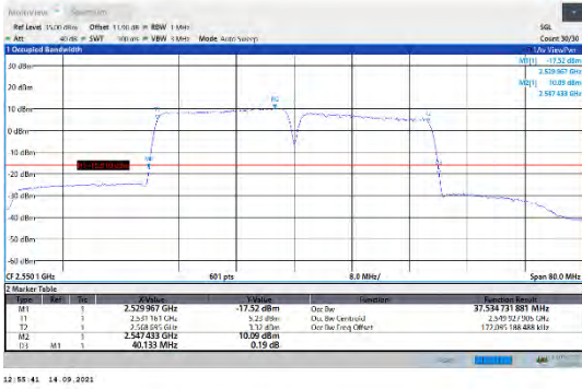
CA_7C-20MHz-20MHz-QPSK-QPSK-21152-21350-100RB#0-100RB#0
