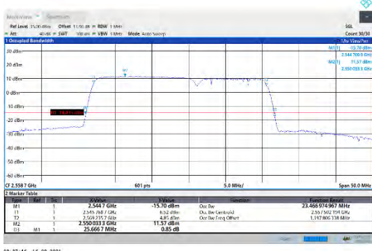
CA_7C-15MHz-10MHz-QPSK-QPSK-21277-2139CA_7C5RB#0-50RB#0
