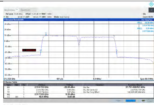
CA_7C-20MHz-20MHz-QPSK-QPSK-21001-21199-100RB#0-100RB#0
