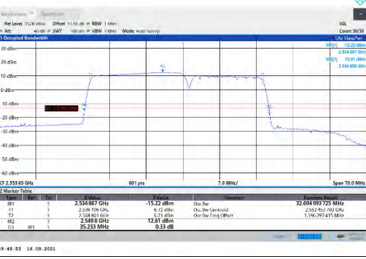
CA_7C-20MHz-15MHz-QPSK-QPSK-21201-21372-100RB#0-75RB#0
