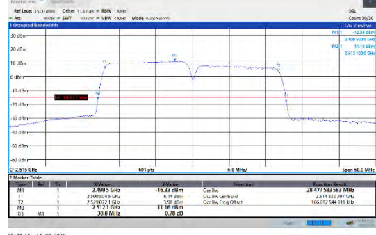
CA_7C-15MHz-15MHz-QPSK-QPSK-20825-20975-75RB#0-75RB#0
