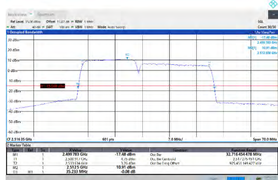
CA_7C-15MHz-20MHz-16QAM-16QAM-20828-20999-75RB#0-100RB#0
