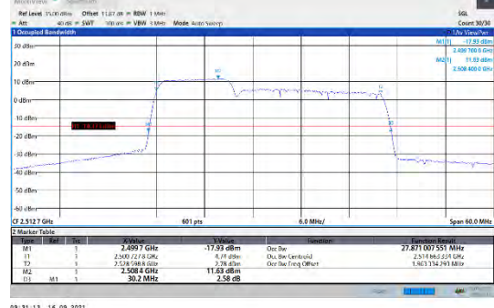
CA_7C-10MHz-20MHz-16QAM-16QAM-20805-20949-50RB#0-100RB#0
