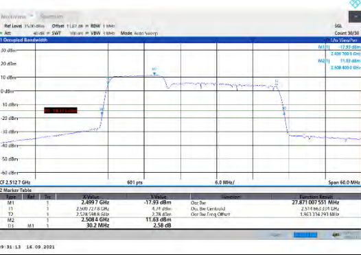
CA_7C-10MHz-20MHz-16QAM-16QAM-20805-20949-50RB#0-100RB#0
