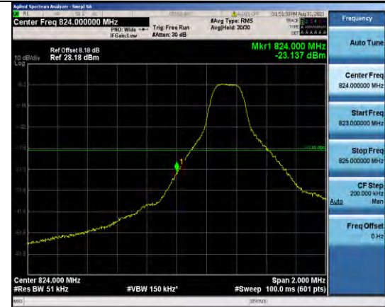
Band5-5MHz-QPSK-20425-25RB#0
