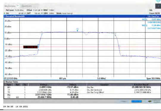
CA_7C-15MHz-10MHz-QPSK-QPSK-20825-20945-75RB#0-50RB#0
