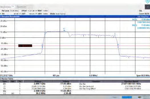
CA_7C-10MHz-20MHz-16QAM-16QAM-20805-20949-50RB#0-100RB#0
