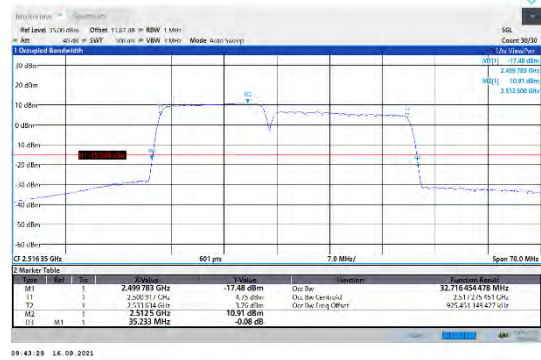
CA_7C-15MHz-20MHz-16QAM-16QAM-20828-20999-75RB#0-100RB#0
