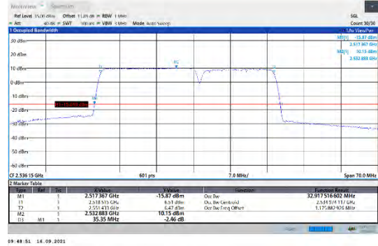
CA_7C-20MHz-15MHz-16QAM-16QAM-21026-21197-100RB#0-75RB#0
