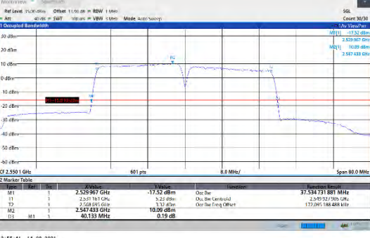
CA_7C-20MHz-20MHz-QPSK-QPSK-21152-21350-100RB#0-100RB#0
