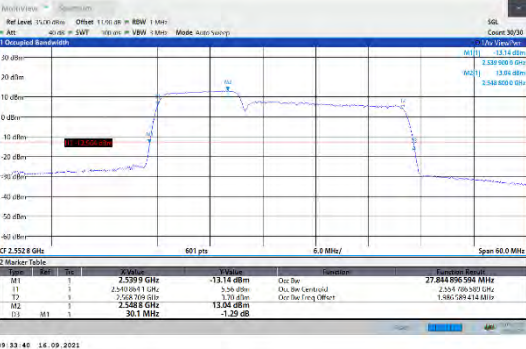
CA_7C-10MHz-20MHz-QPSK-QPSK-21206-21350-50RB#0-100RB#0
