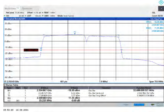
CA_7C-20MHz-15MHz-16QAM-16QAM-21201-21372-100RB#0-75RB#0
