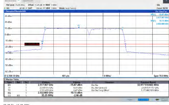
CA_7C-20MHz-15MHz-16QAM-16QAM-21026-21197-100RB#0-75RB#0
