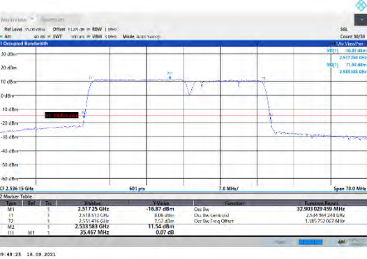
CA_7C-20MHz-15MHz-QPSK-QPSK-21026-21197-100RB#0-75RB#0
