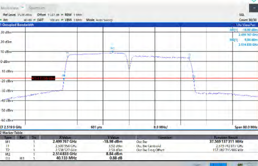
CA_7C-20MHz-20MHz-16QAM-16QAM-20850-21048-100RB#0-100RB#0
