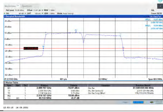
CA_7C-20MHz-20MHz-QPSK-QPSK-20850-21048-100RB#0-100RB#0
