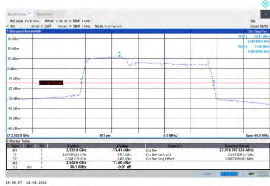
CA_7C-10MHz-20MHz-16QAM-16QAM-21206-21350-50RB#0-100RB#0
