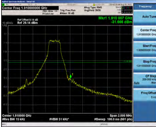
Band2-1.4MHz-16QAM-19193-6RB#0
