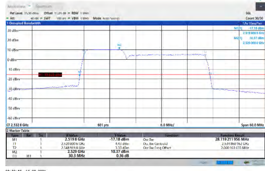
CA_7C-10MHz-20MHz-16QAM-16QAM-21150-50RB#0-100RB#0
