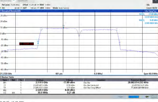
CA_7C-15MHz-15MHz-16QAM-16QAM-21025-21175-75RB#0-75RB#0
