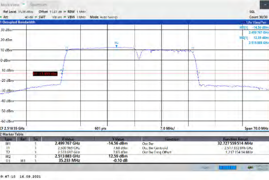
CA_7C-20MHz-15MHz-QPSK-QPSK-20850-21021-100RB#0-75RB#0
