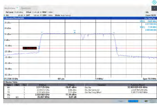
CA_7C-20MHz-15MHz-QPSK-QPSK-21026-21197-100RB#0-75RB#0
