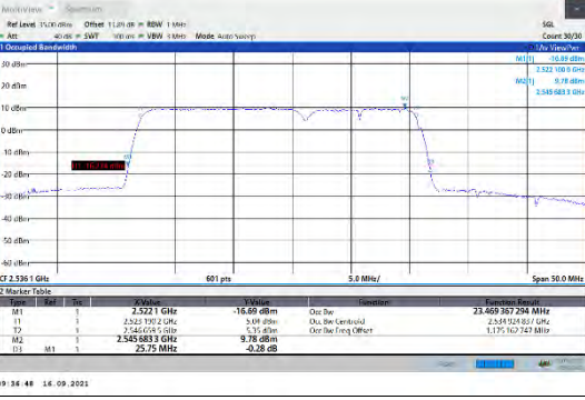
CA_7C-15MHz-10MHz-16QAM-16QAM-21051-21171-75RB#0-50RB#0
