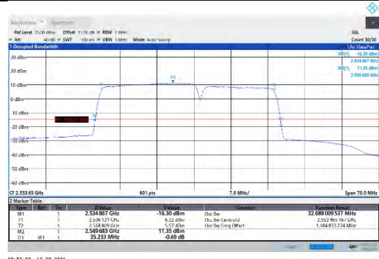
CA_7C-20MHz-15MHz-16QAM-16QAM-21201-21372-100RB#0-75RB#0
