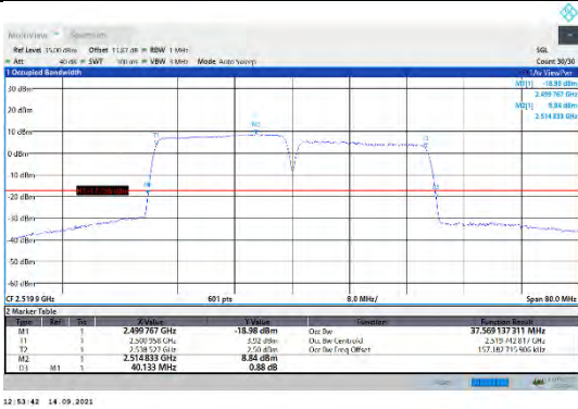
CA_7C-20MHz-20MHz-16QAM-16QAM-20850-21048-100RB#0-100RB#0
