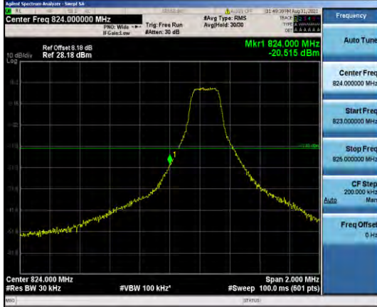
Band5-3MHz-16QAM-20415-15RB#0
