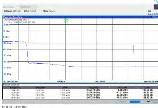
CA_7C-20MHz-20MHz-16QAM-16QAM-21152-21350-100RB#0-100RB#0
