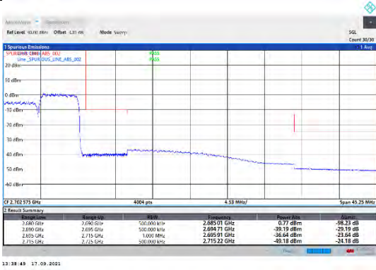
CA_41C-20MHz-5MHz-QPSK-QPSK-41440-41557-100RB#0-25RB#0
