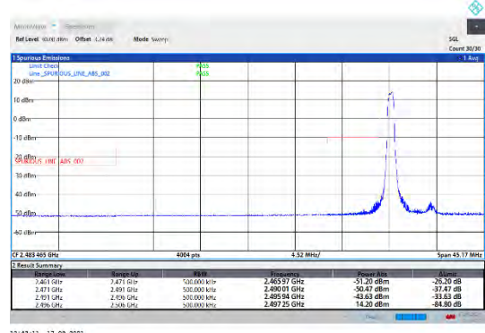
CA_41C-5MHz-20MHz-16QAM-16QAM-39683-39800-1RB#0-0RB#0
