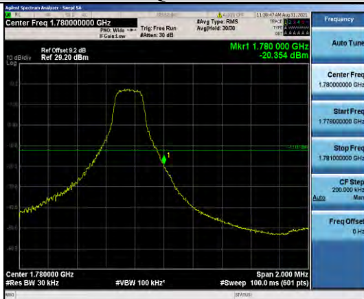
Band66-3MHz-QPSK-132657-1RB#14
