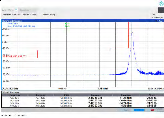
CA_41C-20MHz-5MHz-QPSK-QPSK-39750-39867-1RB#0-0RB#0
