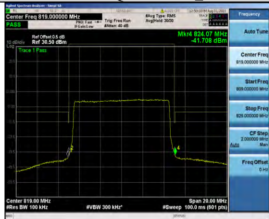
Band26-10MHz-16QAM-26740_Left-50RB#0
