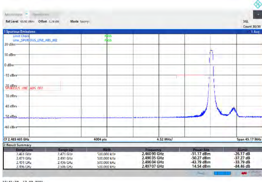
CA_41C-5MHz-20MHz-QPSK-QPSK-39683-39800-1RB#0-0RB#0
