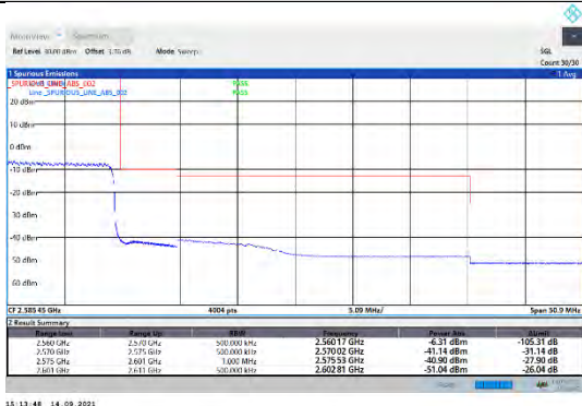
CA_7C-15MHz-15MHz-QPSK-QPSK-21225-21375-75RB#0-75RB#0
