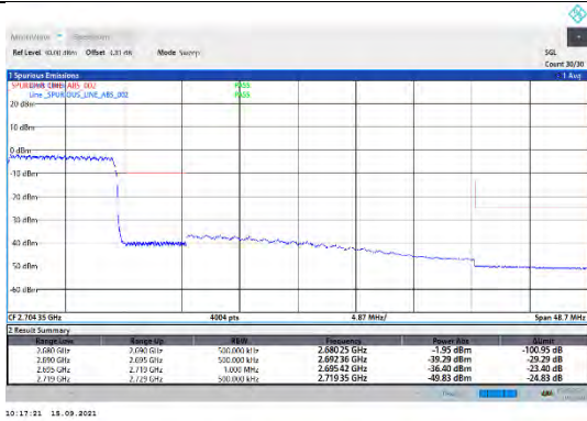
CA_41C-20MHz-10MHz-QPSK-QPSK-41391-41535-100RB#0-50RB#0
