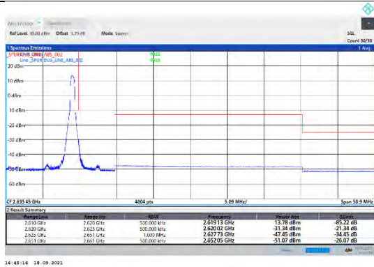
CA_38C-15MHz-15MHz-16QAM-16QAM-38025-38175-0RB#0-1RB#74
