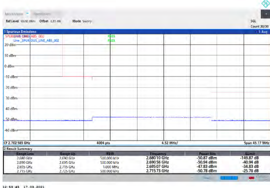
CA_41C-5MHz-20MHz-QPSK-QPSK-41373-41490-25RB#0-100RB#0
