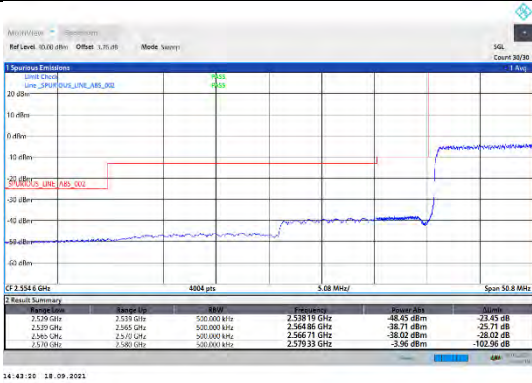
CA_38C-15MHz-15MHz-QPSK-QPSK-37825-37975-75RB#0-75RB#0
