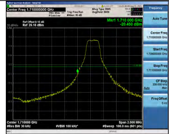
Band66-3MHz-16QAM-131987-15RB#0
