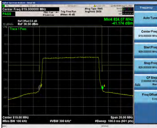
Band26-10MHz-QPSK-26740_Right-1RB#49
