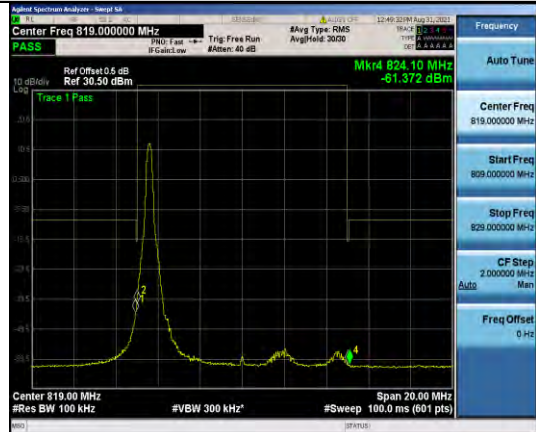
Band26-10MHz-16QAM-26740_Left-50RB#0
