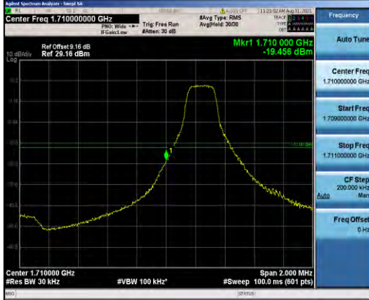
Band66-3MHz-QPSK-131987-15RB#0
