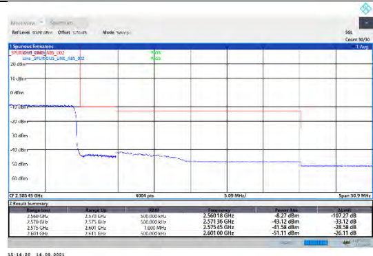
CA_7C-15MHz-15MHz-16QAM-16QAM-21225-21375-75RB#0-75RB#0
