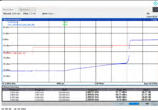
CA_7C-15MHz-15MHz-QPSK-QPSK-20825-20975-75RB#0-75RB#0
