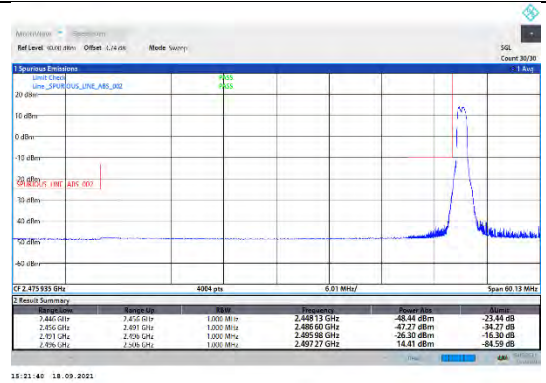
CA_41C-20MHz-20MHz-16QAM-16QAM-39750-39948-1RB#0-0RB#0
