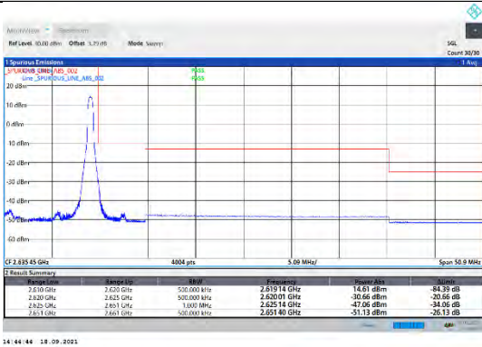
CA_38C-15MHz-15MHz-QPSK-QPSK-38025-38175-0RB#0-1RB#74
