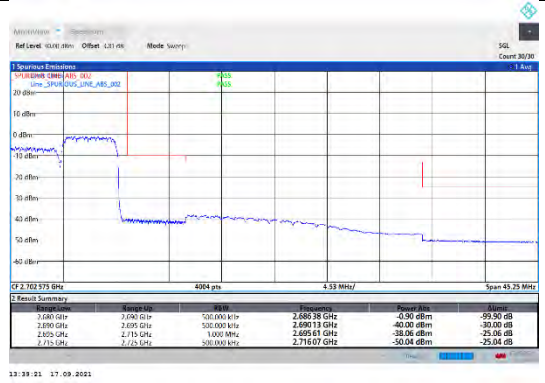
CA_41C-20MHz-5MHz-16QAM-16QAM-41440-41557-100RB#0-25RB#0
