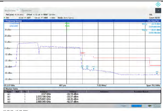
CA_7C-10MHz-20MHz-16QAM-16QAM-21206-21350-50RB#0-100RB#0
