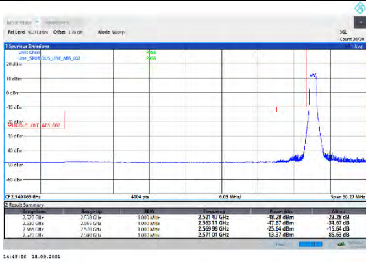
CA_38C-20MHz-20MHz-16QAM-16QAM-37850-38048-1RB#0-0RB#0
