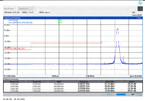
CA_38C-15MHz-15MHz-16QAM-16QAM-37825-37975-1RB#0-0RB#0
