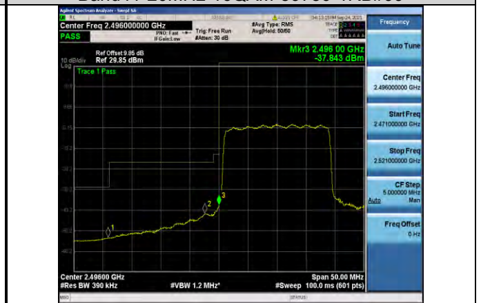
Band41-20MHz-16QAM-39750-1RB#0
