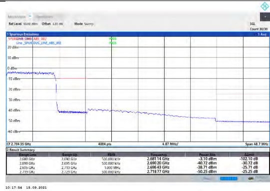
CA_41C-20MHz-10MHz-16QAM-16QAM-41391-41535-100RB#0-50RB#0
