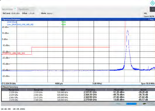
CA_38C-15MHz-15MHz-QPSK-QPSK-37825-37975-1RB#0-0RB#0
