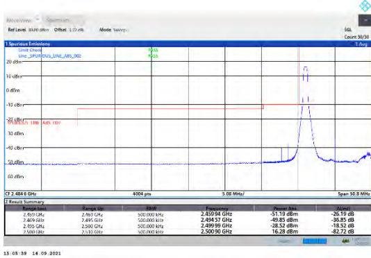
CA_7C-15MHz-15MHz-QPSK-QPSK-20825-20975-1RB#0-0RB#0
