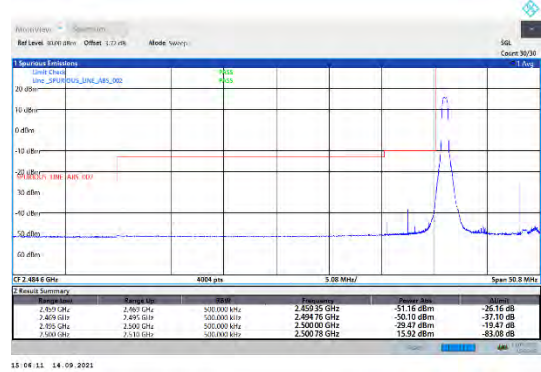
CA_7C-15MHz-15MHz-16QAM-16QAM-20825-20975-1RB#0-0RB#0
