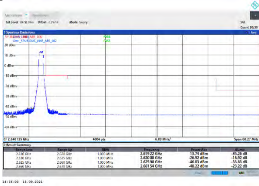
CA_38C-20MHz-20MHz-16QAM-16QAM-37952-38150-0RB#0-1RB#99
