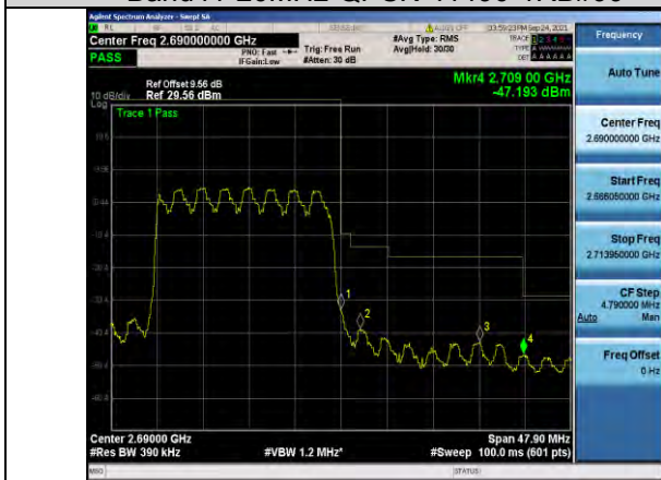
Band41-20MHz-QPSK-41490-100RB#0
