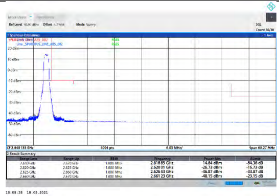
CA_38C-20MHz-20MHz-QPSK-QPSK-37952-38150-0RB#0-1RB#99
