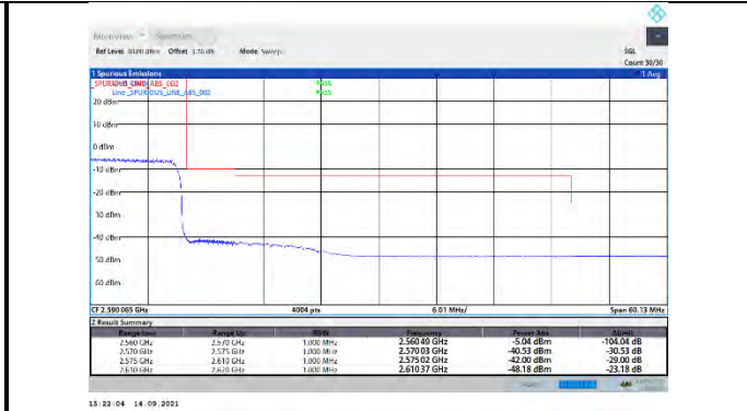
CA_7C-20MHz-20MHz-QPSK-QPSK-21152-21350-100RB#0-100RB#0
