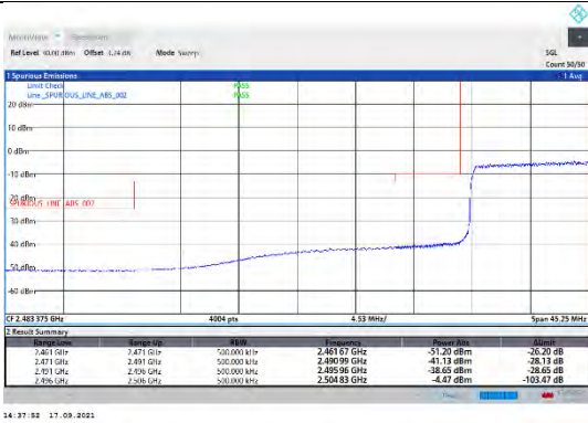
CA_41C-20MHz-5MHz-QPSK-QPSK-39750-39867-100RB#0-25RB#0
