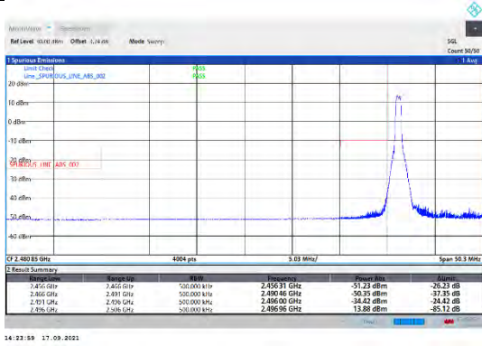
CA_41C-20MHz-10MHz-16QAM-16QAM-39750-39894-1RB#0-0RB#0
