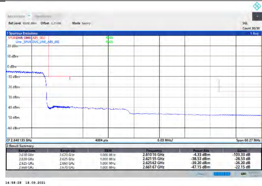
CA_38C-20MHz-20MHz-16QAM-16QAM-37952-38150-100RB#0-100RB#0
