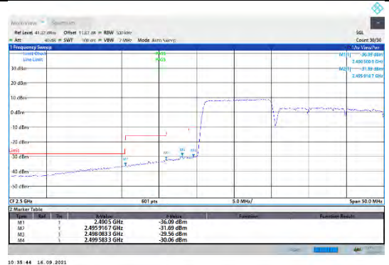
CA_7C-10MHz-20MHz-16QAM-16QAM-20805-20949-50RB#0-100RB#0
