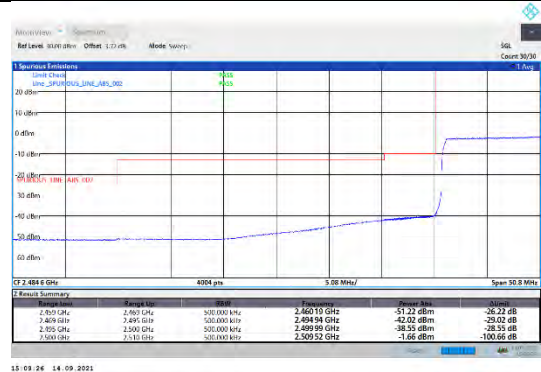
CA_7C-15MHz-15MHz-16QAM-16QAM-20825-20975-75RB#0-75RB#0
