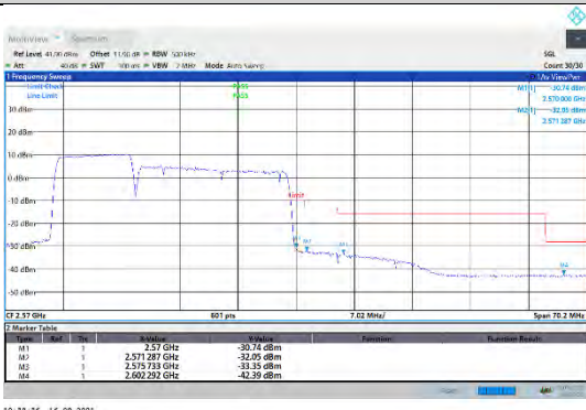
CA_7C-10MHz-20MHz-QPSK-QPSK-21206-21350-50RB#0-100RB#0
