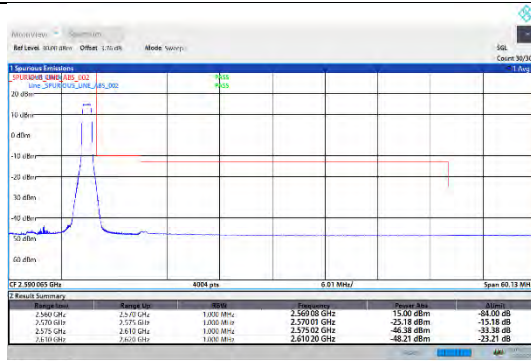
CA_7C-20MHz-20MHz-16QAM-16QAM-21152-21350-0RB#0-1RB#99
