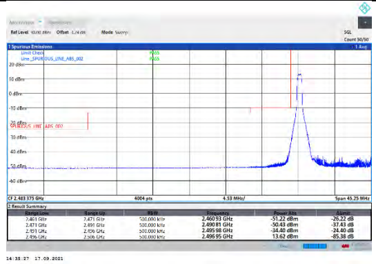
CA_41C-20MHz-5MHz-16QAM-16QAM-39750-39867-1RB#0-0RB#0
