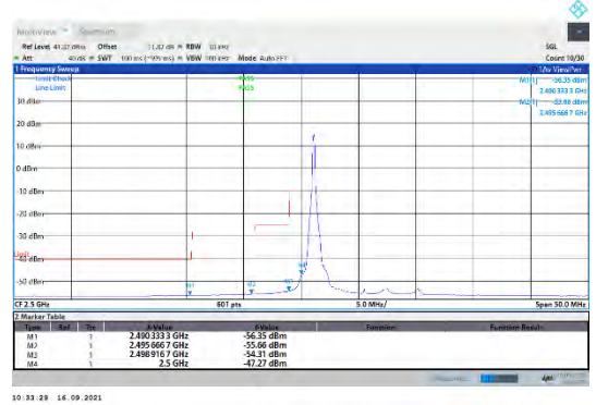
CA_7C-10MHz-20MHz-16QAM-16QAM-20805-20949-1RB#0-0RB#0
