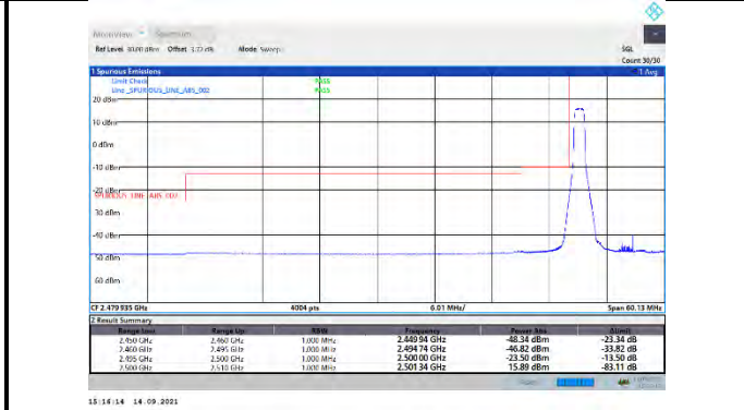
CA_7C-20MHz-20MHz-16QAM-16QAM-20850-21048-1RB#0-0RB#0
