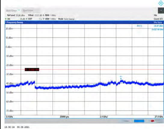
Band7-15MHz-16QAM-20825-1RB#0- Range3:3000~27000MHz
