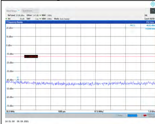
Band4-20MHz-QPSK-20175-1RB#0- Range1:30~1000MHz
