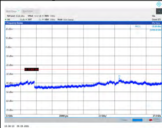
Band7-20MHz-16QAM-20850-1RB#0- Range3:3000~27000MHz
