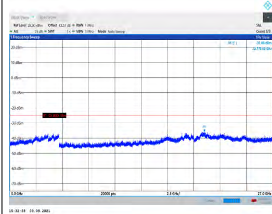
Band7-15MHz-QPSK-21375-1RB#0- Range3:3000~27000MHz
