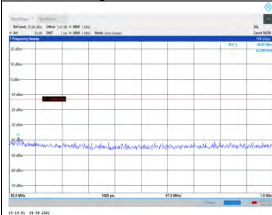
Band2-20MHz-QPSK-18900-1RB#0- Range1:30~1000MHz
