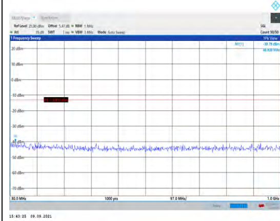
Band4-1.4MHz-QPSK-20175-1RB#0- Range1:30~1000MHz
