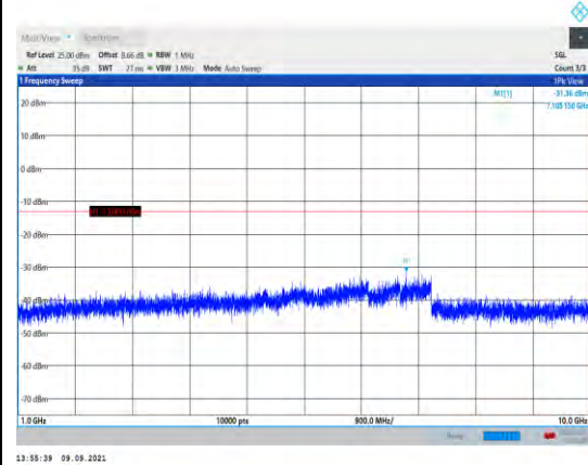
Band12-10MHz-16QAM-23130-1RB#0- Range2:1000~10000MHz
