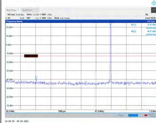
Band12-10MHz-16QAM-23095-1RB#0- Range1:30~1000MHz
