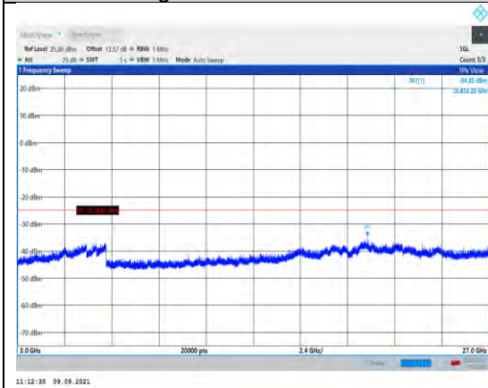
Band38-20MHz-16QAM-37850-1RB#0- Range3:3000~27000MHz
