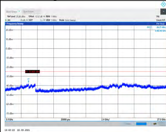
Band38-5MHz-16QAM-37775-1RB#0- Range3:3000~27000MHz
