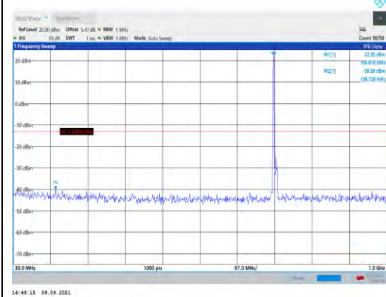
Band17-10MHz-16QAM-23790-1RB#0- Range1:30~1000MHz
