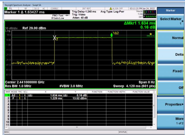
8-DPSK DH3
