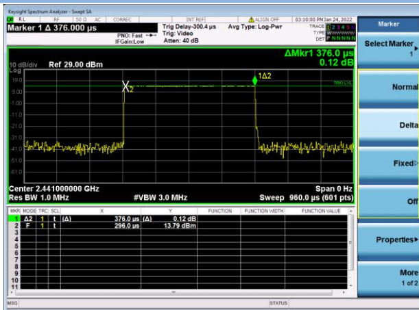
8-DPSK DH1
