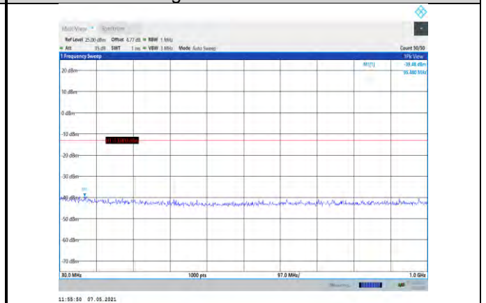
Band4-3MHz-QPSK-20385-1RB#0- Range1:30~1000MHz
