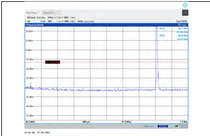
Band26-5MHz-16QAM-26715-1RB#0- Range1:30~1000MHz
