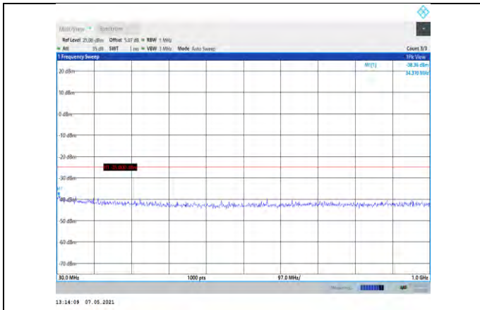
Band7-10MHz-16QAM-21100-1RB#0- Range1:30~1000MHz
