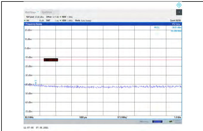
Band4-20MHz-16QAM-20050-1RB#0- Range1:30~1000MHz
