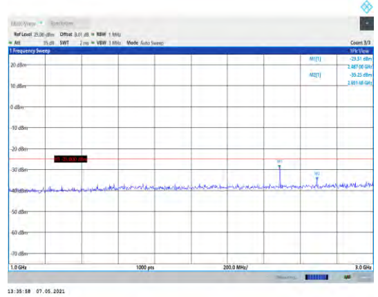
Band7-15MHz-16QAM-20825-1RB#0- Range2:1000~3000MHz
