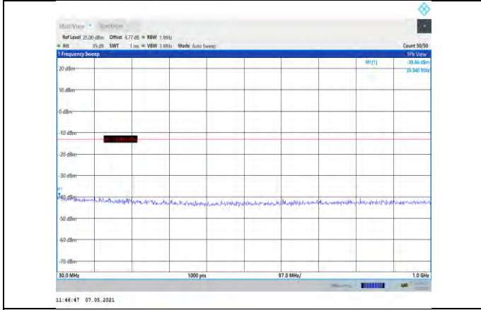
Band4-15MHz-16QAM-20175-1RB#0- Range1:30~1000MHz
