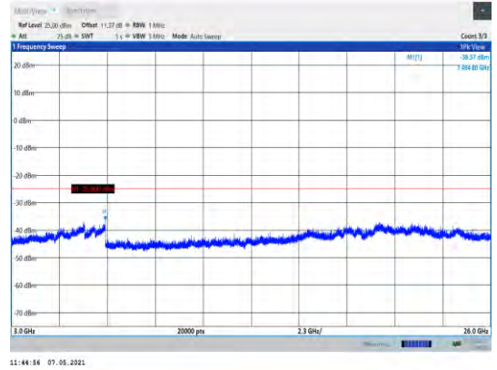
Band38-10MHz-16QAM-38200-1RB#0-Range3:3000~26000MHz
