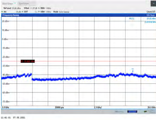
Band38-10MHz-QPSK-37800-1RB#0-Range3:3000~26000MHz
