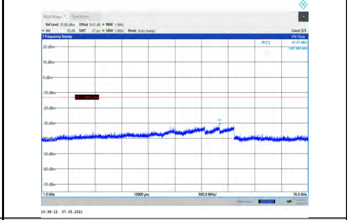
Band26-3MHz-16QAM-26775-1RB#0- Range2:1000~10000MHz
