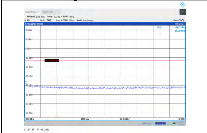
Band4-20MHz-16QAM-20175-1RB#0- Range1:30~1000MHz
