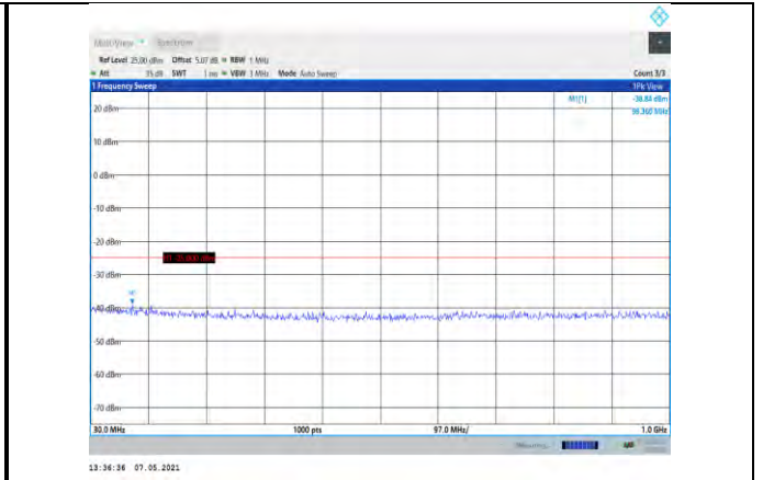
Band7-15MHz-QPSK-21100-1RB#0- Range1:30~1000MHz
