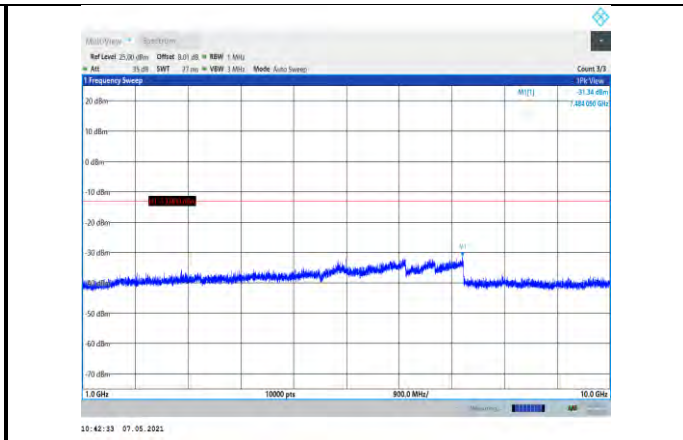
Band26-5MHz-16QAM-26740-1RB#0- Range2:1000~10000MHz
