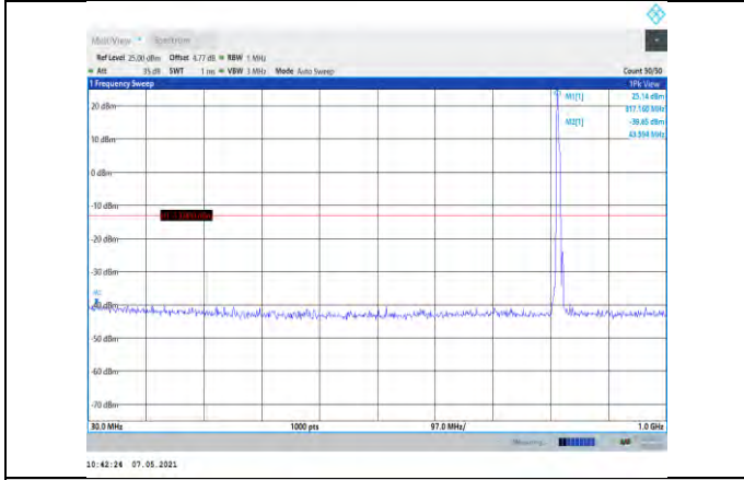
Band26-5MHz-16QAM-26740-1RB#0- Range1:30~1000MHz
