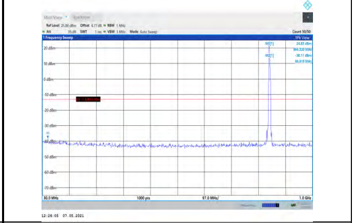
Band5-5MHz-QPSK-20625-1RB#0-Range1:30~1000MHz
