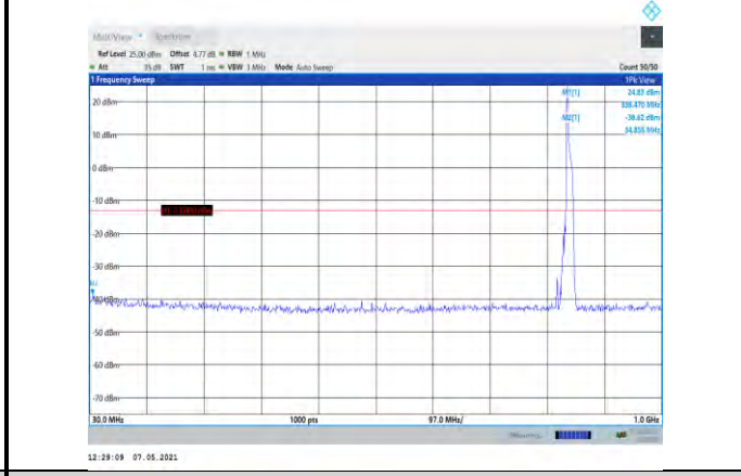
Band5-10MHz-16QAM-20600-1RB#0- Range1:30~1000MHz
