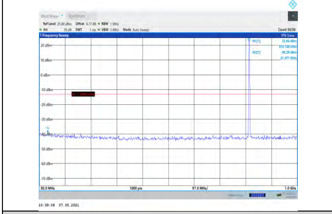
Band26-1.4MHz-QPSK-26740-1RB#0-Range1:30~1000MHz
