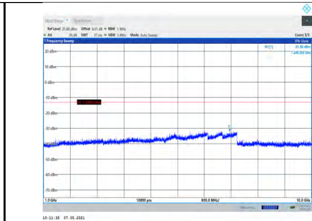
Band12-5MHz-QPSK-23095-1RB#0- Range2:1000~10000MHz
