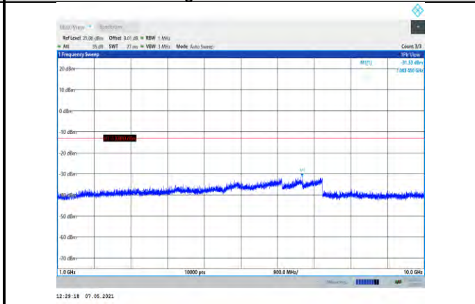
Band5-10MHz-16QAM-20600-1RB#0- Range2:1000~10000MHz
