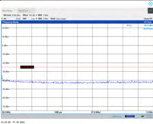
Band7-5MHz-QPSK-20775-1RB#0-Range1:30~1000MHz
