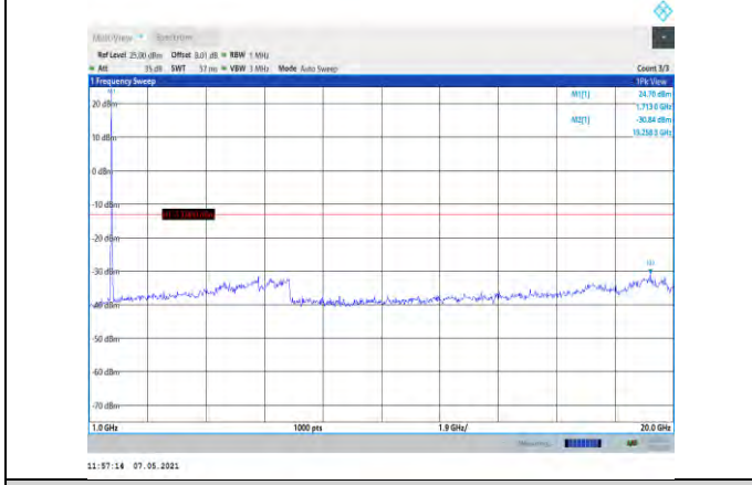
Band4-20MHz-16QAM-20050-1RB#0- Range2:1000~20000MHz
