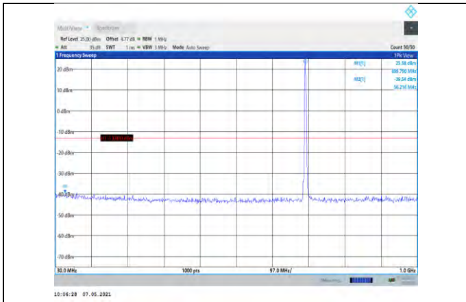
Band12-3MHz-16QAM-23025-1RB#0- Range1:30~1000MHz
