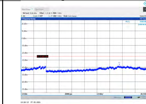
Band7-20MHz-16QAM-20850-1RB#0- Range3:3000~26000MHz
