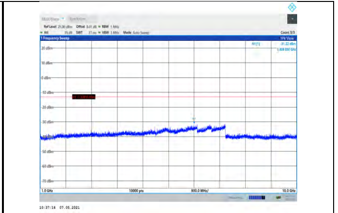
Band26-3MHz-QPSK-26740-1RB#0-Range2:1000~10000MHz
