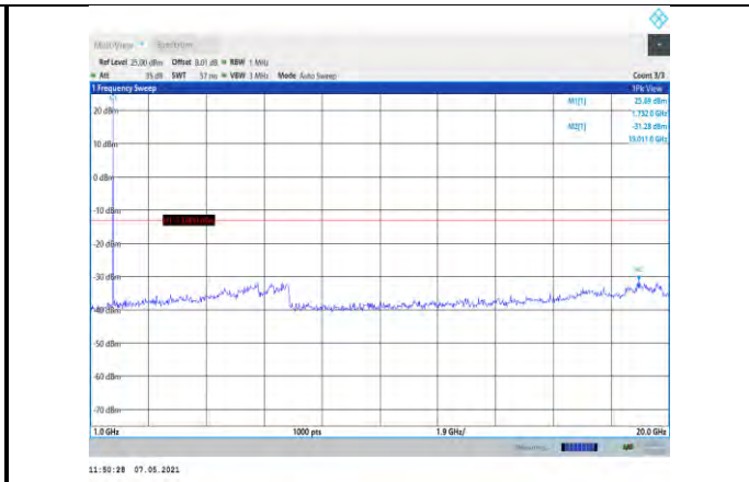
Band4-1.4MHz-16QAM-20175-1RB#0- Range2:1000~20000MHz
