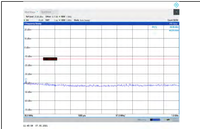
Band4-15MHz-16QAM-20025-1RB#0- Range1:30~1000MHz
