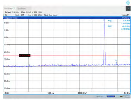
Band38-10MHz-16QAM-38000-1RB#0- Range2:1000~3000MHz
