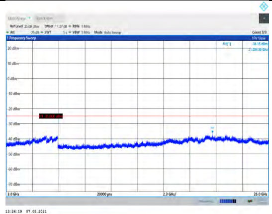
Band7-5MHz-16QAM-21425-1RB#0- Range3:3000~26000MHz
