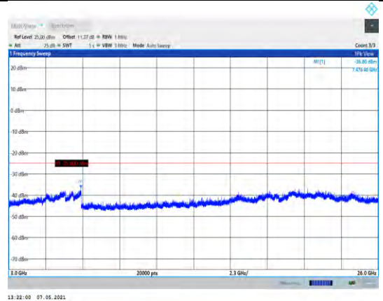
Band7-5MHz-QPSK-21100-1RB#0-Range3:3000~26000MHz
