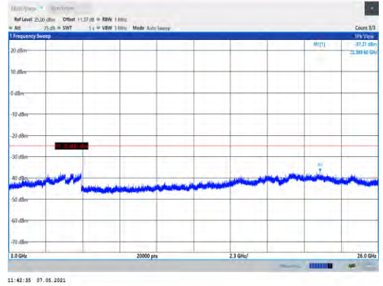
Band38-10MHz-QPSK-38000-1RB#0-Range3:3000~26000MHz
