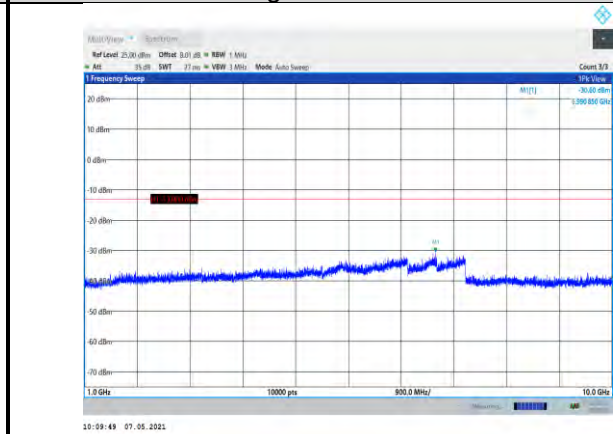
Band12-1.4MHz-16QAM-23173-1RB#0- Range2:1000~10000MHz
