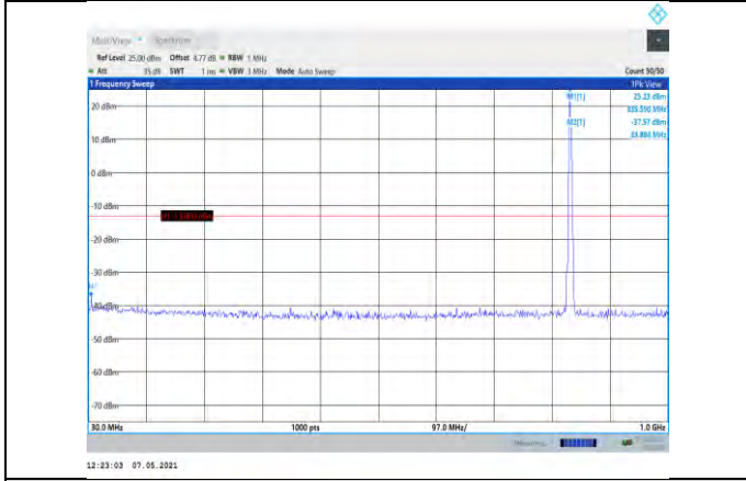
Band5-3MHz-16QAM-20525-1RB#0- Range1:30~1000MHz
