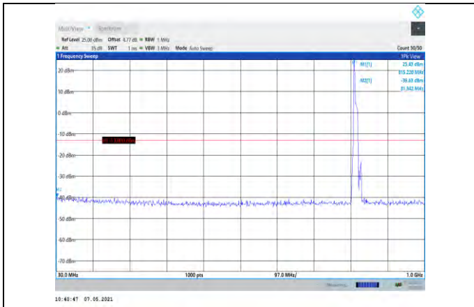
Band26-10MHz-QPSK-26740-1RB#0-Range1:30~1000MHz
