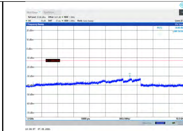
Band12-3MHz-QPSK-23095-1RB#0- Range2:1000~10000MHz
