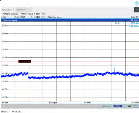
Band7-5MHz-QPSK-20775-1RB#0-Range3:3000~26000MHz
