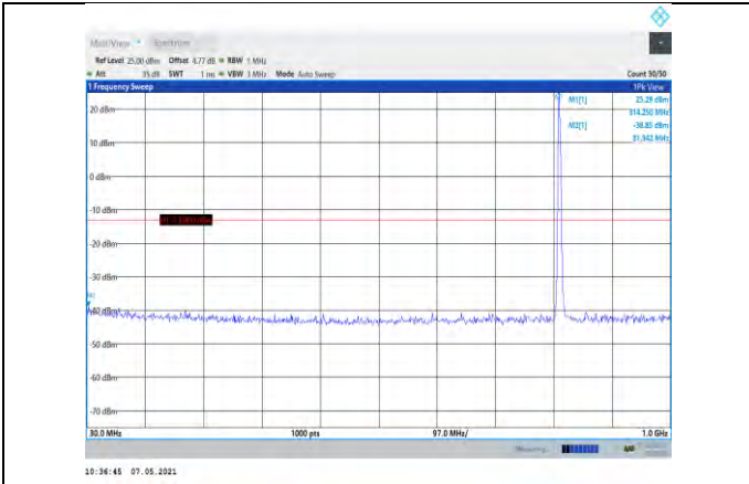
Band26-3MHz-16QAM-26705-1RB#0- Range1:30~1000MHz
