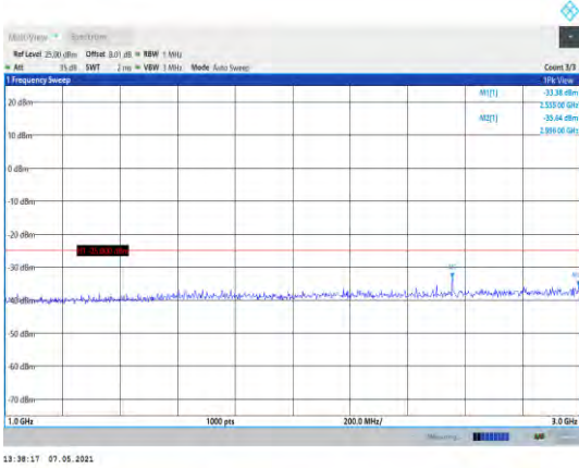
Band7-15MHz-QPSK-21375-1RB#0- Range2:1000~3000MHz
