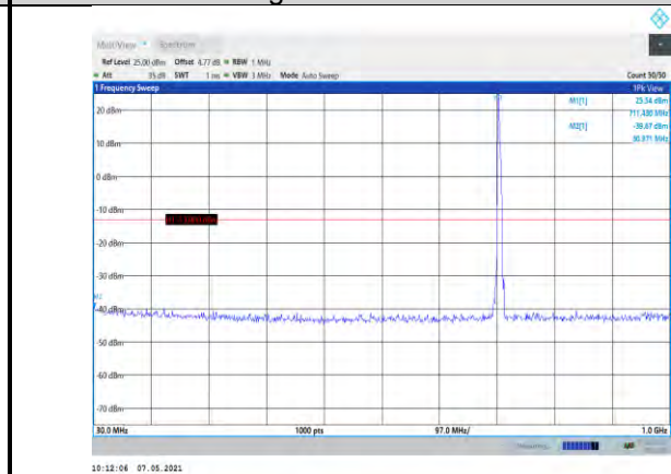
Band12-5MHz-QPSK-23155-1RB#0- Range1:30~1000MHz
