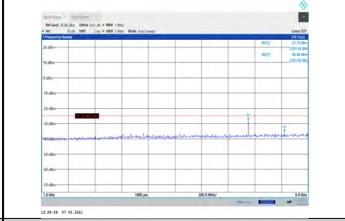
Band7-20MHz-16QAM-21350-1RB#0- Range2:1000~3000MHz
