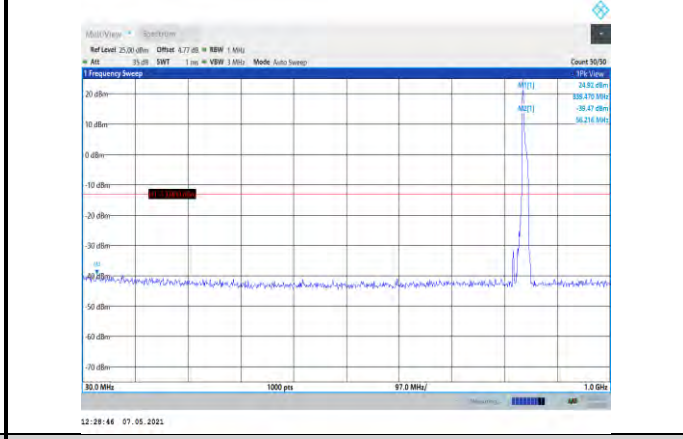
Band5-10MHz-QPSK-20600-1RB#0- Range1:30~1000MHz
