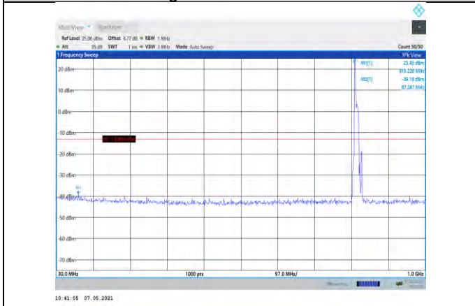
Band26-10MHz-16QAM-26740-1RB#0-Range1:30~1000MHz
