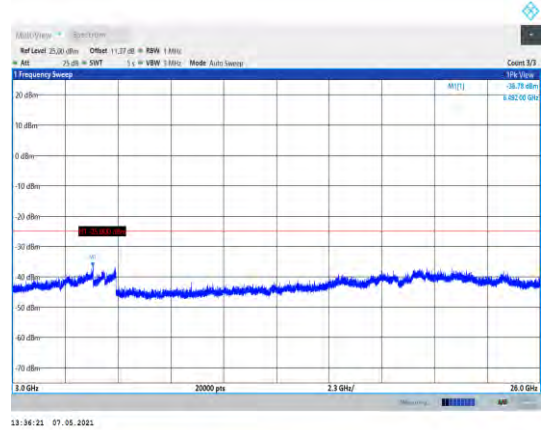
Band7-15MHz-16QAM-20825-1RB#0- Range3:3000~26000MHz
