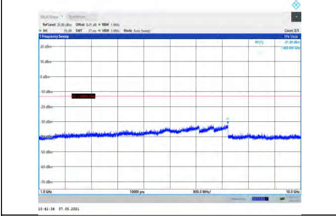
Band26-5MHz-QPSK-26715-1RB#0-Range2:1000~10000MHz
