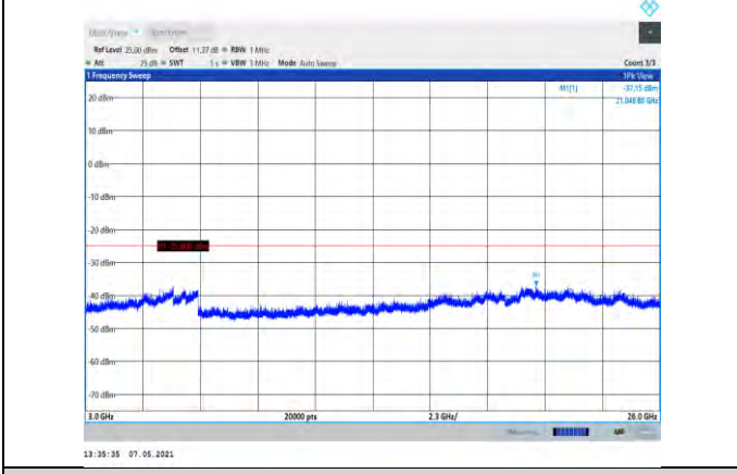
Band7-15MHz-QPSK-20825-1RB#0- Range3:3000~26000MHz
