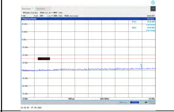
Band7-10MHz-16QAM-21400-1RB#0- Range2:1000~3000MHz
