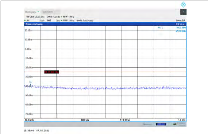
Band7-15MHz-QPSK-20825-1RB#0- Range1:30~1000MHz
