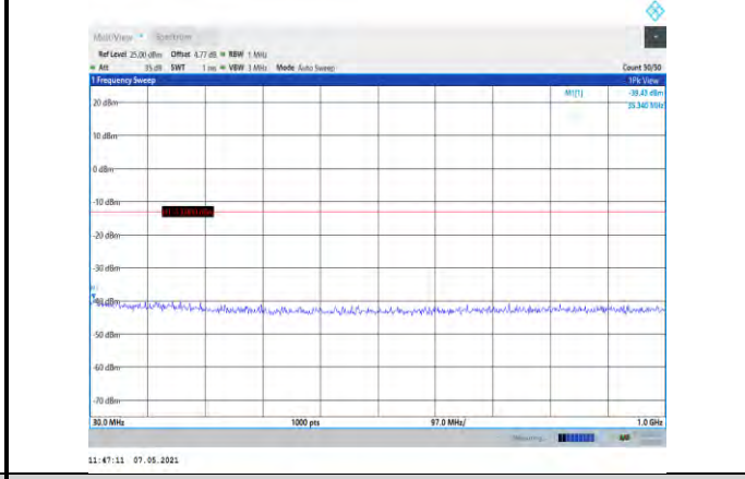
Band4-15MHz-QPSK-20325-1RB#0- Range1:30~1000MHz
