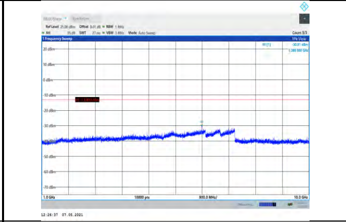
Band5-5MHz-16QAM-20625-1RB#0- Range2:1000~10000MHz
