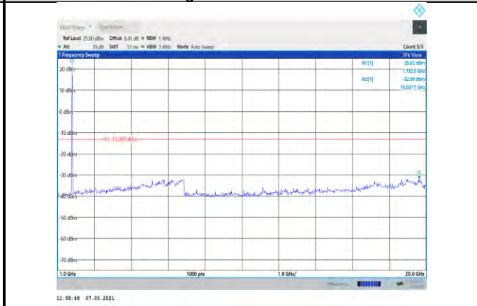
Band4-20MHz-16QAM-20300-1RB#0- Range2:1000~20000MHz
