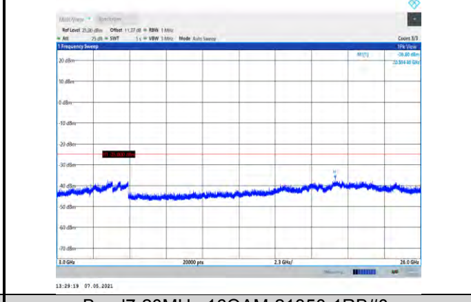
Band7-20MHz-16QAM-21350-1RB#0- Range3:3000~26000MHz
