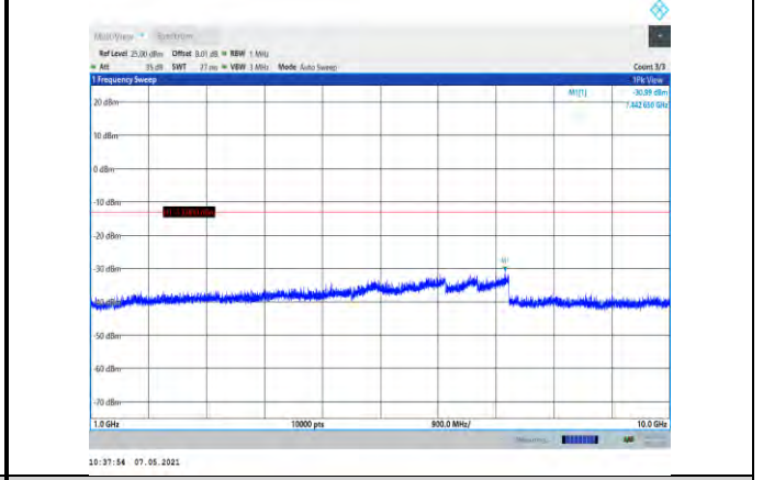
Band26-3MHz-QPSK-26775-1RB#0-Range2:1000~10000MHz
