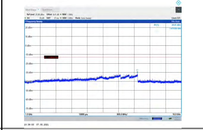
Band26-1.4MHz-QPSK-26783-1RB#0-Range2:1000~10000MHz
