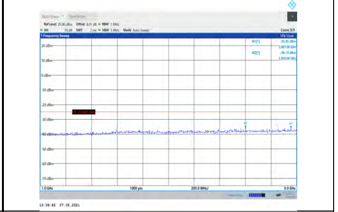
Band7-15MHz-QPSK-21100-1RB#0- Range2:1000~3000MHz
