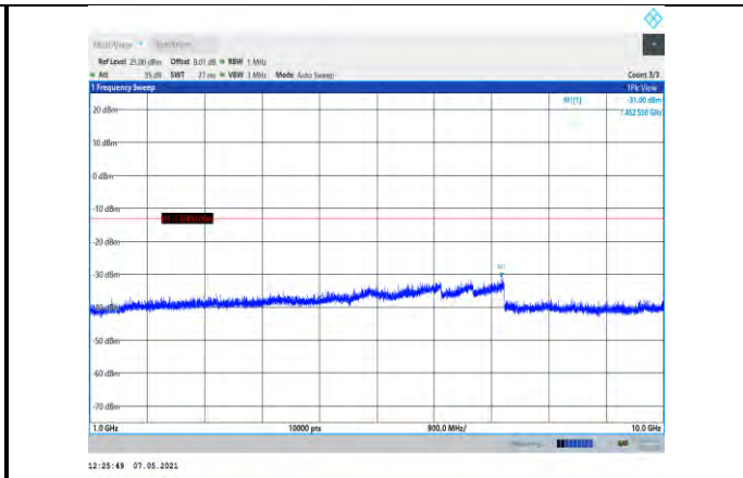
Band5-5MHz-16QAM-20525-1RB#0- Range2:1000~10000MHz
