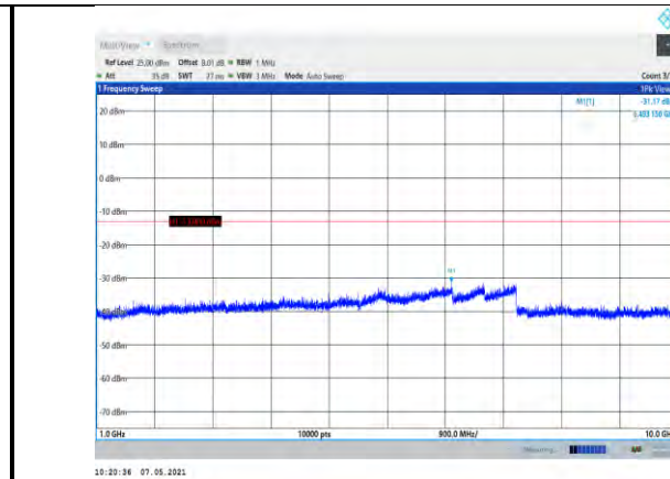
Band17-5MHz-QPSK-23790-1RB#0- Range2:1000~10000MHz
