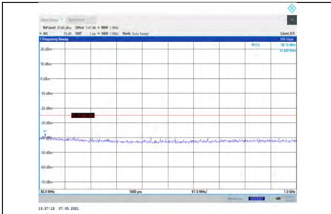
Band7-20MHz-16QAM-21100-1RB#0- Range1:30~1000MHz
