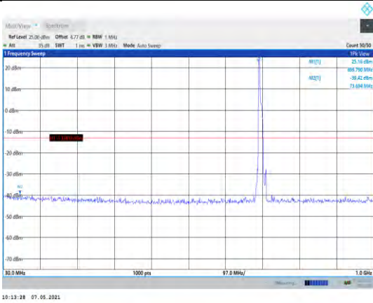
Band12-10MHz-16QAM-23060-1RB#0-Range1:30~1000MHz
