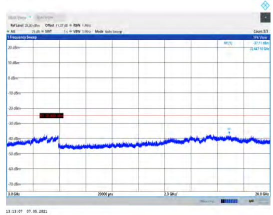
Band7-10MHz-16QAM-20800-1RB#0- Range3:3000~26000MHz
