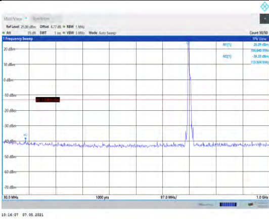
Band17-10MHz-16QAM-23780-1RB#0- Range1:30~1000MHz
