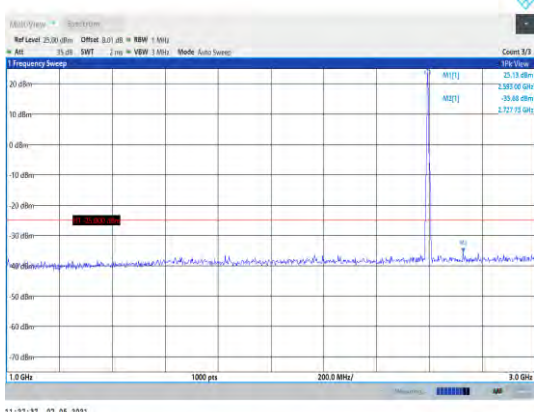
Band38-5MHz-QPSK-38000-1RB#0- Range2:1000~3000MHz
