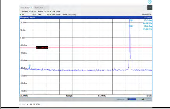
Band5-5MHz-QPSK-20525-1RB#0-Range1:30~1000MHz
