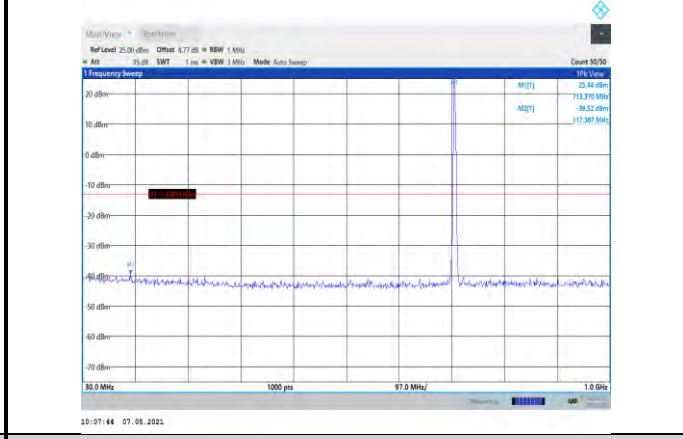
Band12-3MHz-16QAM-23165-1RB#0- Range1:30~1000MHz
