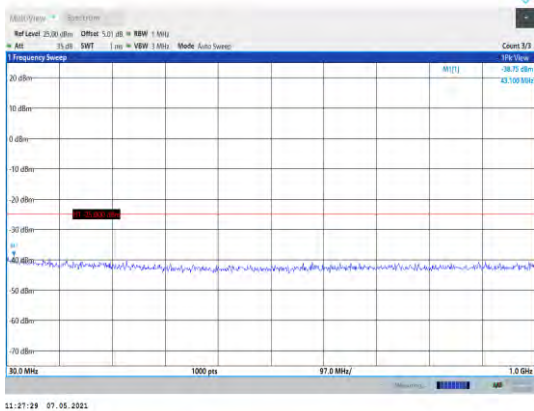
Band38-5MHz-QPSK-38000-1RB#0- Range1:30~1000MHz
