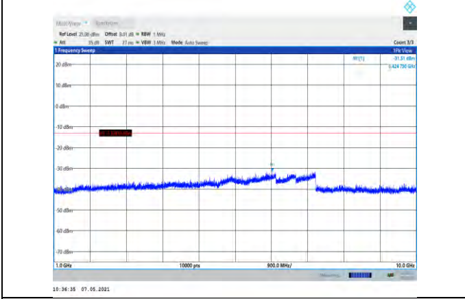
Band26-3MHz-QPSK-26705-1RB#0-Range2:1000~10000MHz
