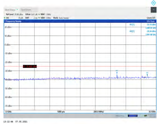
Band7-10MHz-16QAM-20800-1RB#0- Range2:1000~3000MHz
