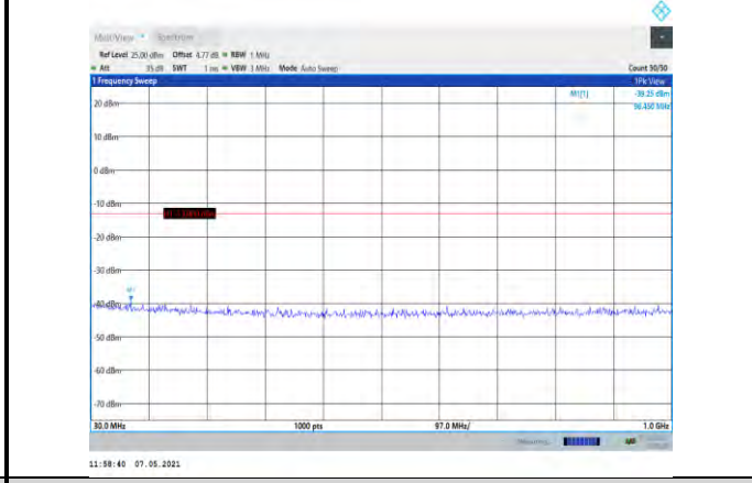
Band4-20MHz-16QAM-20300-1RB#0- Range1:30~1000MHz
