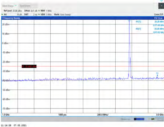
Band38-5MHz-16QAM-37775-1RB#0- Range2:1000~3000MHz
