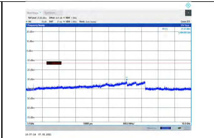
Band12-3MHz-16QAM-23095-1RB#0- Range2:1000~10000MHz
