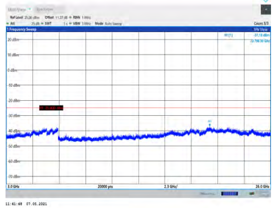
Band38-10MHz-16QAM-37800-1RB#0- Range3:3000~26000MHz
