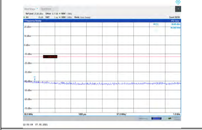
Band4-10MHz-QPSK-20175-1RB#0- Range1:30~1000MHz
