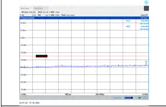
Band7-20MHz-16QAM-21100-1RB#0- Range2:1000~3000MHz
