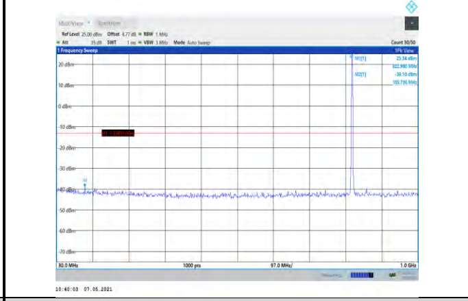
Band26-1.4MHz-16QAM-26783-1RB#0-Range1:30~1000MHz
