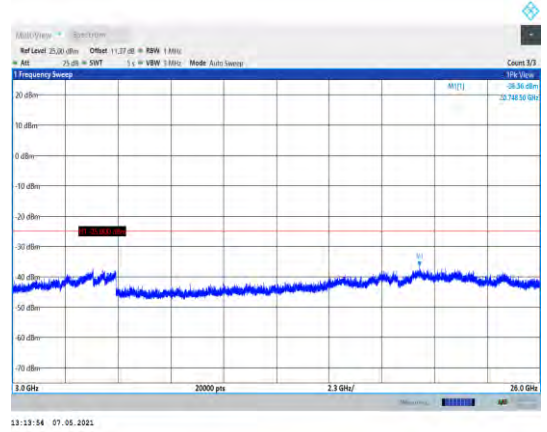
Band7-10MHz-QPSK-21100-1RB#0- Range3:3000~26000MHz
