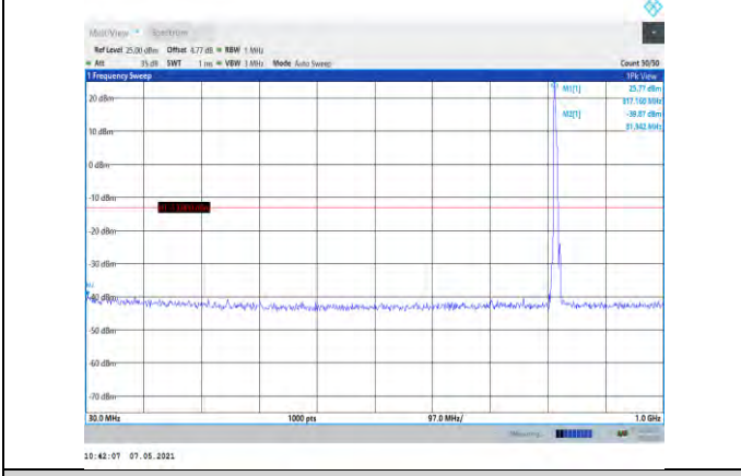
Band26-5MHz-QPSK-26740-1RB#0-Range1:30~1000MHz
