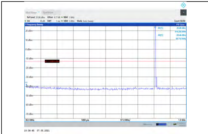
Band26-1.4MHz-16QAM-26697-1RB#0-Range1:30~1000MHz
