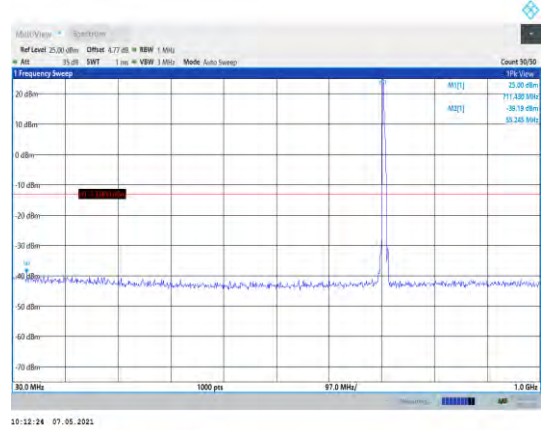
Band12-5MHz-16QAM-23155-1RB#0- Range1:30~1000MHz
