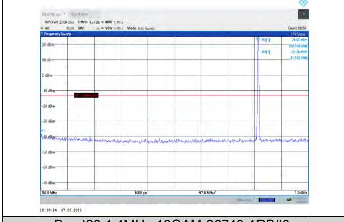
Band26-1.4MHz-16QAM-26740-1RB#0-Range1:30~1000MHz
