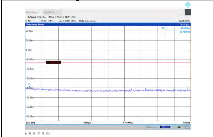
Band4-5MHz-QPSK-20175-1RB#0-Range1:30~1000MHz
