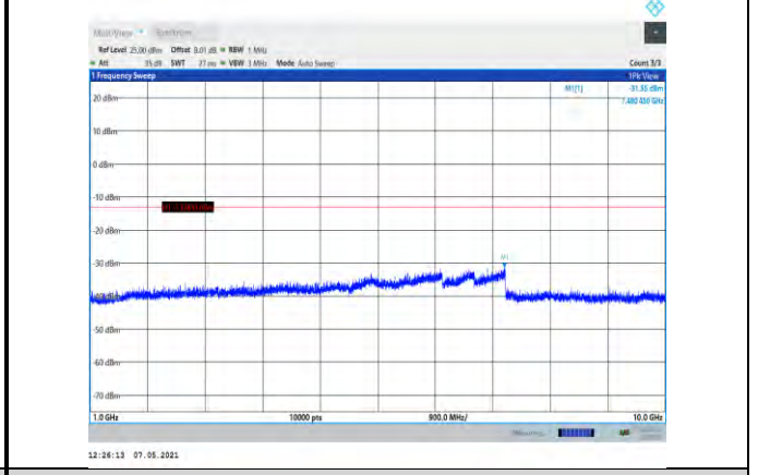
Band5-5MHz-QPSK-20625-1RB#0-Range2:1000~10000MHz
