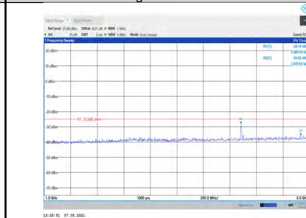
Band7-20MHz-16QAM-20850-1RB#0- Range2:1000~3000MHz
