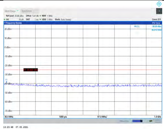
Band7-5MHz-16QAM-21425-1RB#0- Range1:30~1000MHz
