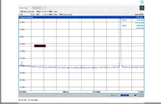
Band26-3MHz-16QAM-26740-1RB#0- Range1:30~1000MHz
