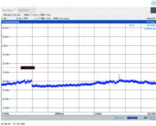
Band7-15MHz-QPSK-21375-1RB#0- Range3:3000~26000MHz
