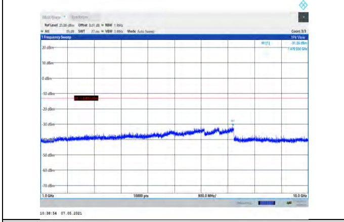
Band26-1.4MHz-16QAM-26697-1RB#0-Range2:1000~10000MHz
