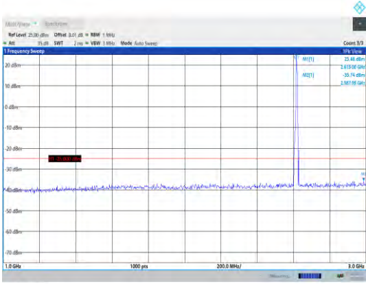
Band38-5MHz-16QAM-38225-1RB#0-Range2:1000~3000MHz
