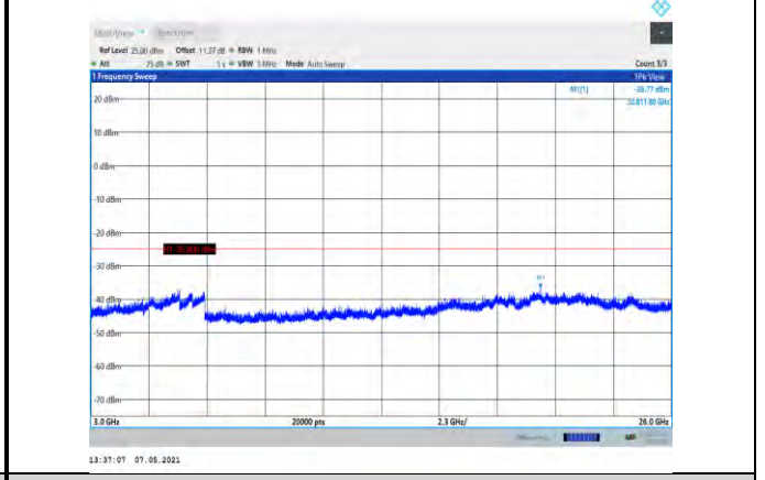
Band7-15MHz-QPSK-21100-1RB#0- Range3:3000~26000MHz
