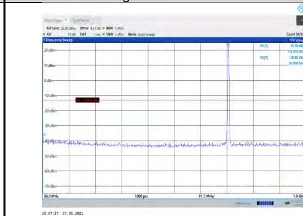
Band12-3MHz-QPSK-23165-1RB#0- Range1:30~1000MHz
