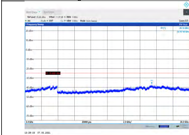
Band7-20MHz-QPSK-21350-1RB#0- Range3:3000~26000MHz
