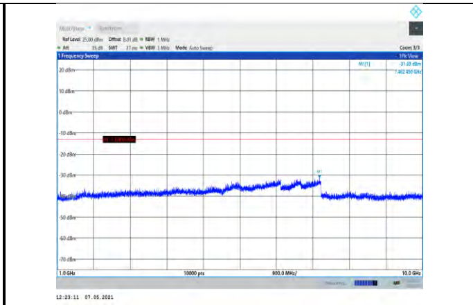
Band5-3MHz-16QAM-20525-1RB#0- Range2:1000~10000MHz
