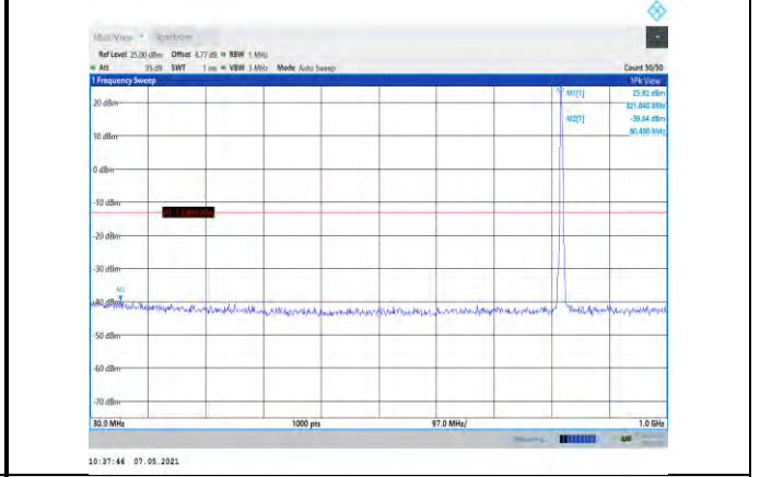
Band26-3MHz-QPSK-26775-1RB#0-Range1:30~1000MHz
