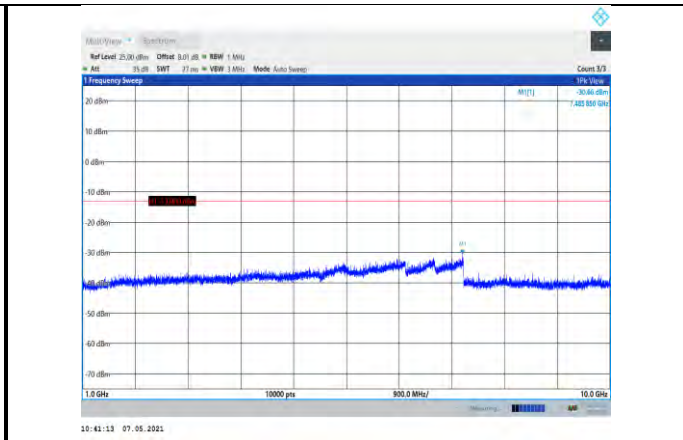
Band26-10MHz-16QAM-26740-1RB#0-Range2:1000~10000MHz
