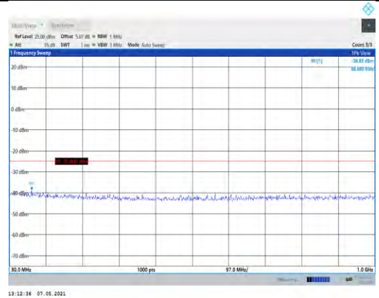
Band7-10MHz-16QAM-20800-1RB#0- Range1:30~1000MHz
