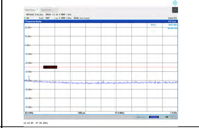
Band38-5MHz-QPSK-37775-1RB#0-Range1:30~1000MHz
