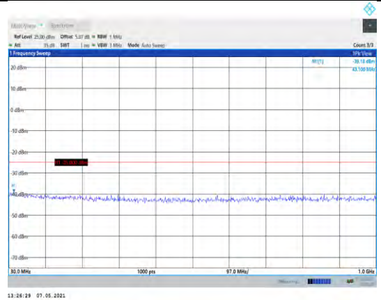
Band7-20MHz-QPSK-21100-1RB#0- Range1:30~1000MHz
