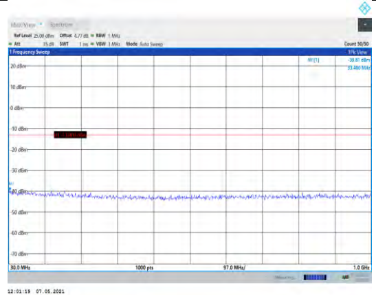
Band4-10MHz-16QAM-20350-1RB#0- Range1:30~1000MHz
