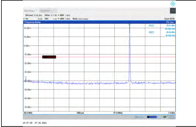
Band12-3MHz-16QAM-23095-1RB#0- Range1:30~1000MHz
