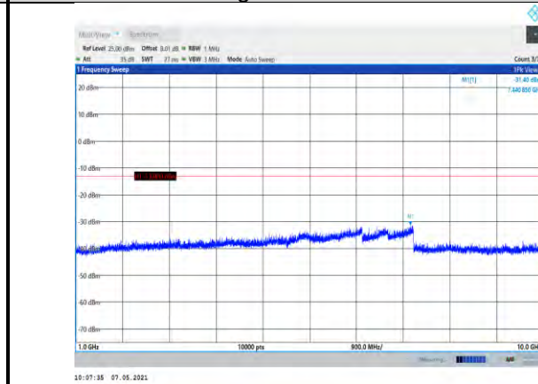
Band12-3MHz-QPSK-23165-1RB#0- Range2:1000~10000MHz
