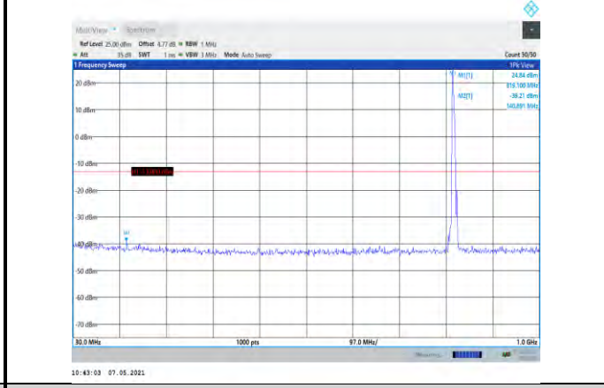
Band26-5MHz-16QAM-26765-1RB#0- Range1:30~1000MHz
