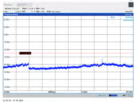
Band38-5MHz-16QAM-38225-1RB#0-Range3:3000~26000MHz
