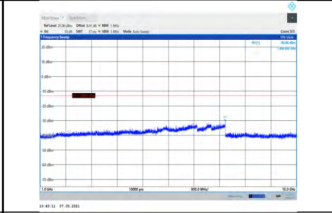
Band26-5MHz-16QAM-26765-1RB#0- Range2:1000~10000MHz
