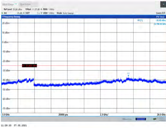
Band38-5MHz-QPSK-38225-1RB#0- Range3:3000~26000MHz
