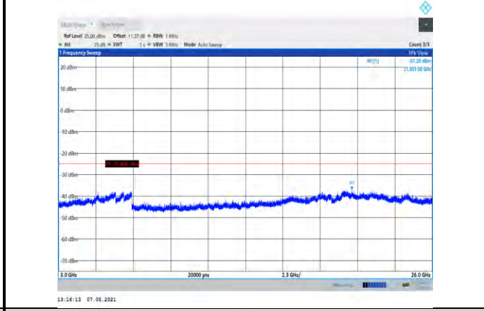
Band7-10MHz-16QAM-21400-1RB#0- Range3:3000~26000MHz
