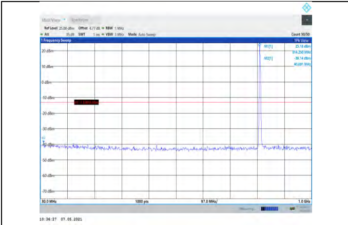
Band26-3MHz-QPSK-26705-1RB#0-Range1:30~1000MHz
