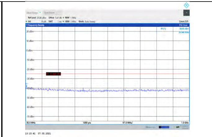
Band7-10MHz-16QAM-21400-1RB#0- Range1:30~1000MHz
