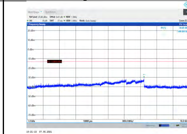
Band17-5MHz-QPSK-23825-1RB#0- Range2:1000~10000MHz
