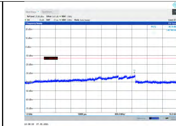
Band12-1.4MHz-QPSK-23095-1RB#0- Range2:1000~10000MHz
