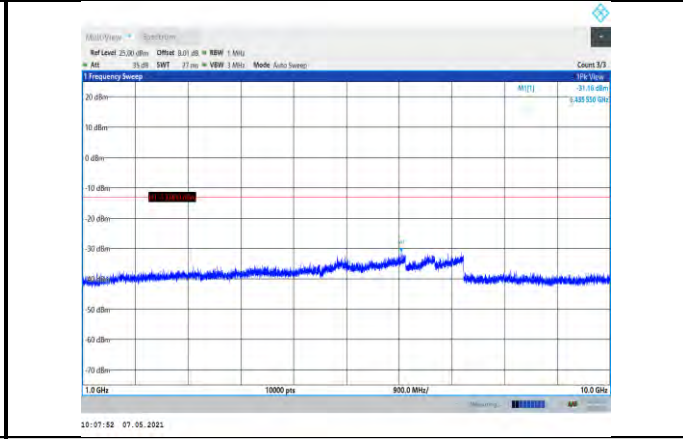
Band12-3MHz-16QAM-23165-1RB#0- Range2:1000~10000MHz
