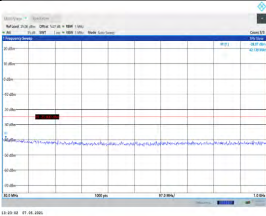
Band7-5MHz-QPSK-21425-1RB#0-Range1:30~1000MHz
