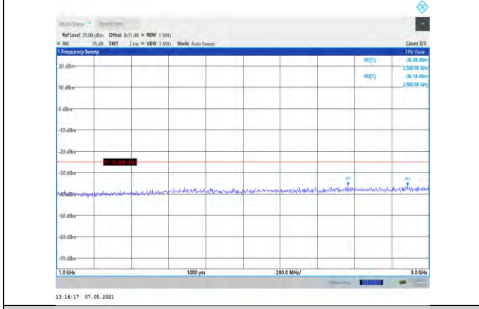
Band7-10MHz-16QAM-21100-1RB#0- Range2:1000~3000MHz
