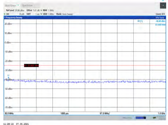
Band38-5MHz-16QAM-38000-1RB#0- Range1:30~1000MHz
