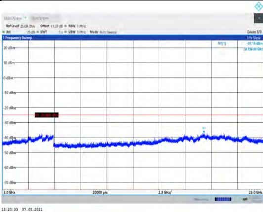
Band7-5MHz-QPSK-21425-1RB#0-Range3:3000~26000MHz
