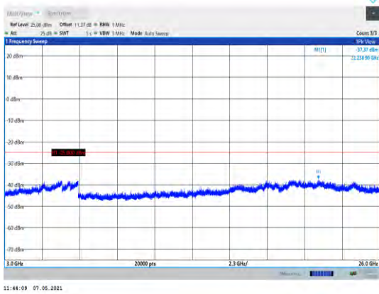
Band38-10MHz-QPSK-38200-1RB#0- Range3:3000~26000MHz
