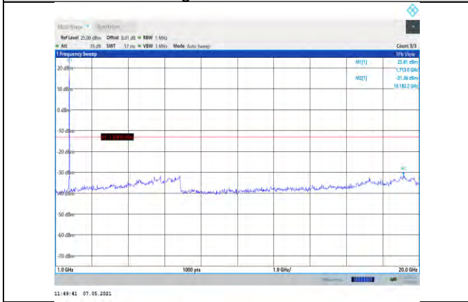
Band4-1.4MHz-16QAM-19957-1RB#0- Range2:1000~20000MHz
