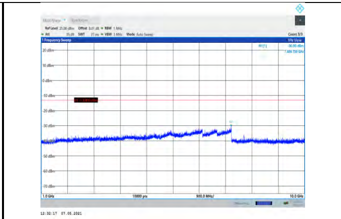
Band5-1.4MHz-16QAM-20525-1RB#0- Range2:1000~10000MHz
