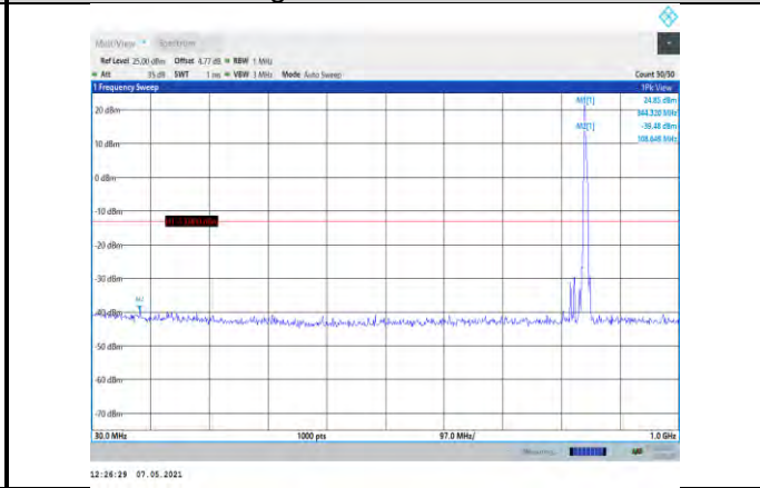
Band5-5MHz-16QAM-20625-1RB#0- Range1:30~1000MHz
