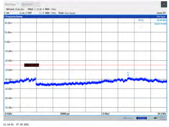
Band38-5MHz-16QAM-37775-1RB#0- Range3:3000~26000MHz
