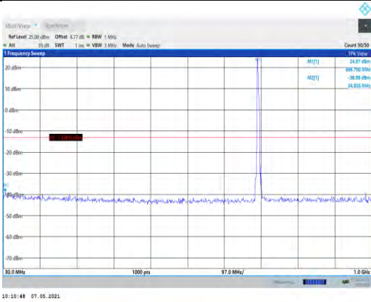
Band12-5MHz-16QAM-23035-1RB#0- Range1:30~1000MHz
