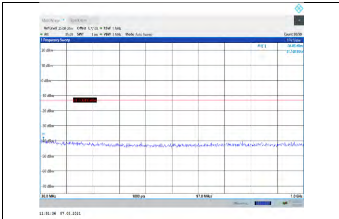
Band4-5MHz-QPSK-19975-1RB#0-Range1:30~1000MHz
