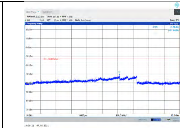
Band12-1.4MHz-16QAM-23095-1RB#0- Range2:1000~10000MHz
