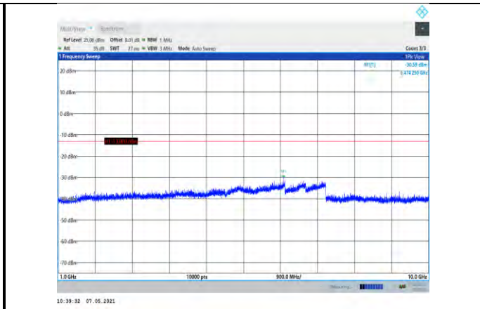
Band26-1.4MHz-16QAM-26740-1RB#0-Range2:1000~10000MHz
