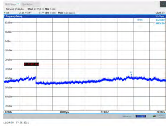
Band38-5MHz-QPSK-38000-1RB#0- Range3:3000~26000MHz
