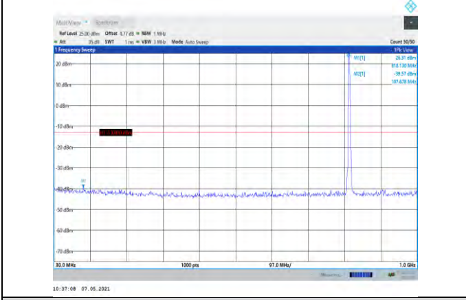
Band26-3MHz-QPSK-26740-1RB#0-Range1:30~1000MHz
