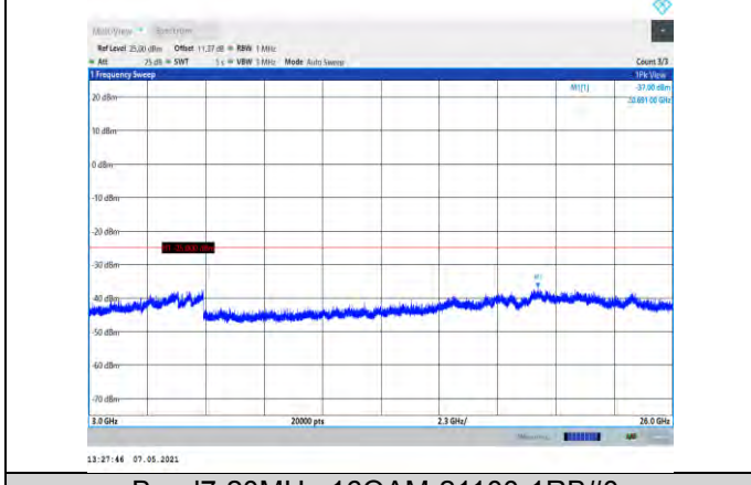
Band7-20MHz-16QAM-21100-1RB#0- Range3:3000~26000MHz
