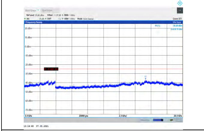
Band7-10MHz-16QAM-21100-1RB#0- Range3:3000~26000MHz
