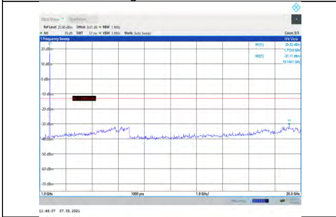
Band4-15MHz-16QAM-20025-1RB#0- Range2:1000~20000MHz
