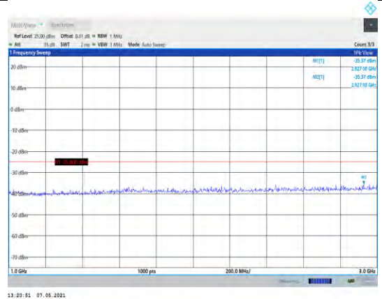
Band7-5MHz-16QAM-20775-1RB#0-Range2:1000~3000MHz
