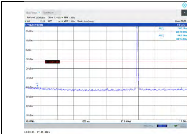
Band12-5MHz-QPSK-23035-1RB#0- Range1:30~1000MHz
