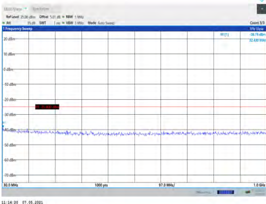
Band38-5MHz-16QAM-37775-1RB#0- Range1:30~1000MHz
