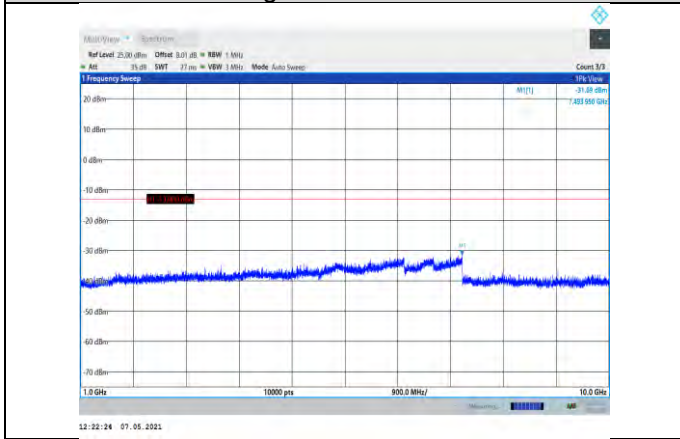
Band5-3MHz-16QAM-20415-1RB#0- Range2:1000~10000MHz
