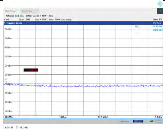
Band7-15MHz-16QAM-20825-1RB#0- Range1:30~1000MHz
