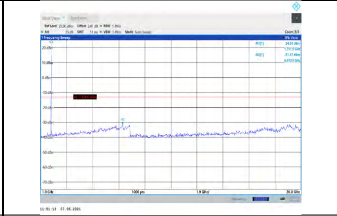
Band4-1.4MHz-16QAM-20393-1RB#0- Range2:1000~20000MHz
