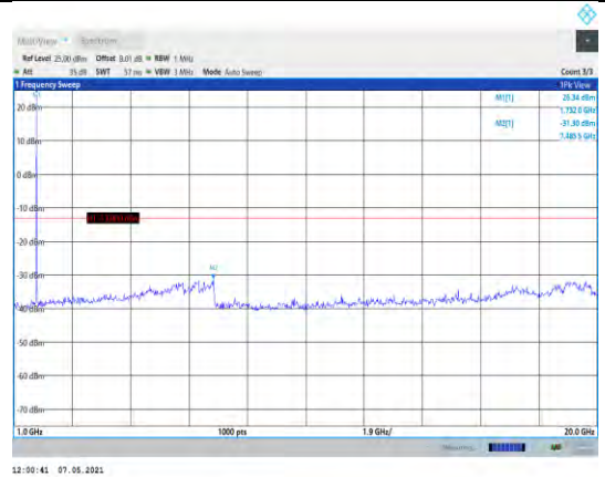
Band4-10MHz-16QAM-20175-1RB#0- Range2:1000~20000MHz
