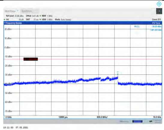
Band12-5MHz-16QAM-23095-1RB#0- Range2:1000~10000MHz
