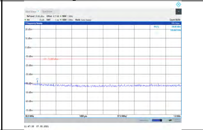
Band4-15MHz-16QAM-20325-1RB#0- Range1:30~1000MHz
