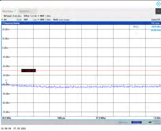
Band7-15MHz-QPSK-21375-1RB#0- Range1:30~1000MHz
