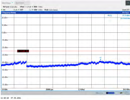
Band38-10MHz-16QAM-38000-1RB#0-Range3:3000~26000MHz
