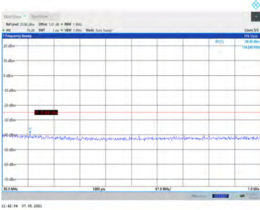
Band38-10MHz-QPSK-38000-1RB#0-Range1:30~1000MHz
