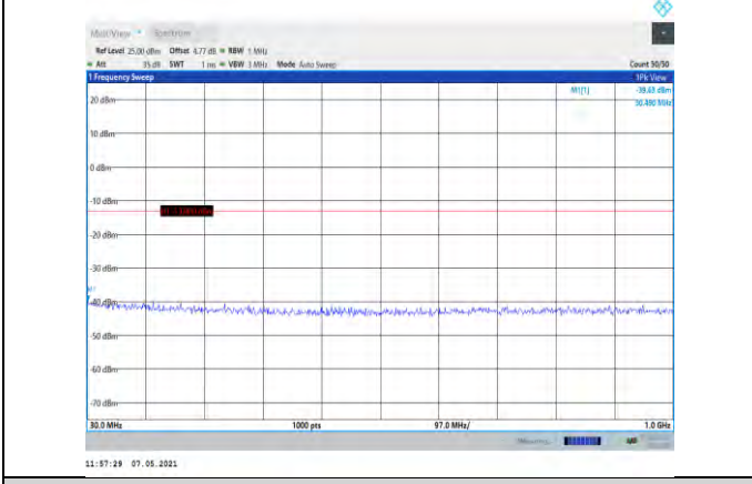
Band4-20MHz-QPSK-20175-1RB#0- Range1:30~1000MHz
