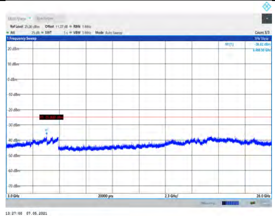
Band7-20MHz-QPSK-21100-1RB#0- Range3:3000~26000MHz
