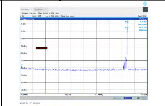
Band5-3MHz-16QAM-20635-1RB#0- Range1:30~1000MHz
