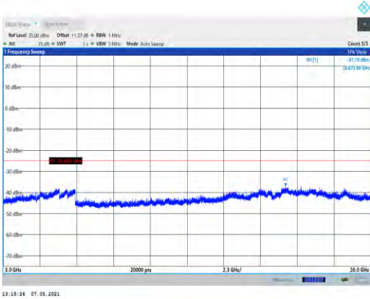
Band7-10MHz-QPSK-21400-1RB#0- Range3:3000~26000MHz
