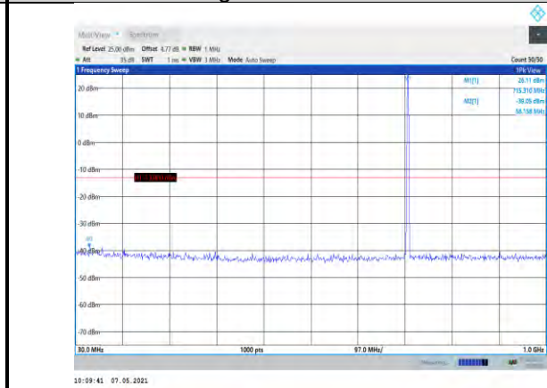
Band12-1.4MHz-16QAM-23173-1RB#0- Range1:30~1000MHz
