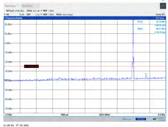
Band38-5MHz-16QAM-38000-1RB#0- Range2:1000~3000MHz
