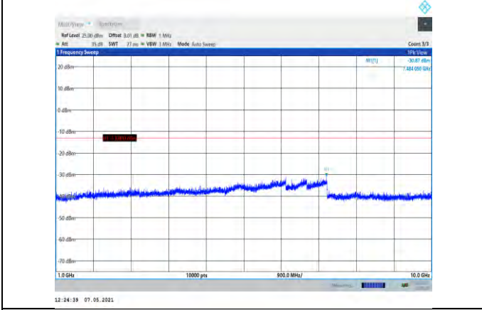
Band5-5MHz-QPSK-20425-1RB#0-Range2:1000~10000MHz
