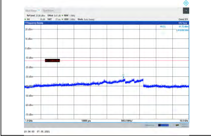
Band26-3MHz-16QAM-26705-1RB#0- Range2:1000~10000MHz
