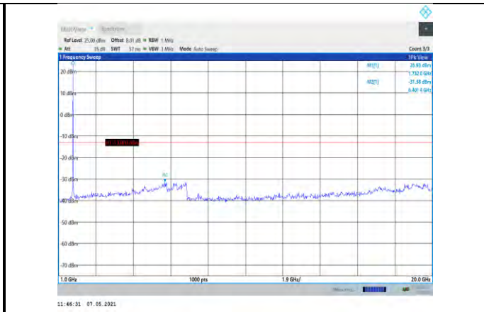
Band4-15MHz-QPSK-20175-1RB#0- Range2:1000~20000MHz
