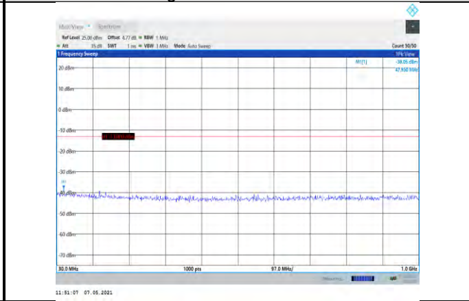
Band4-1.4MHz-16QAM-20393-1RB#0- Range1:30~1000MHz
