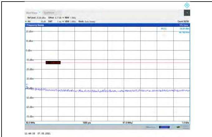
Band4-1.4MHz-16QAM-19957-1RB#0- Range1:30~1000MHz
