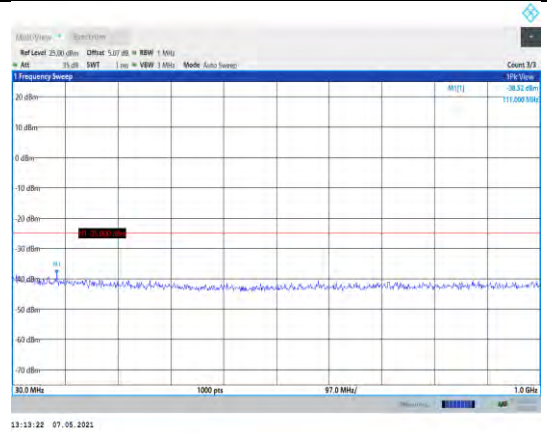
Band7-10MHz-QPSK-21100-1RB#0- Range1:30~1000MHz
