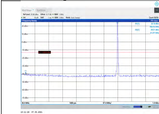
Band12-5MHz-QPSK-23095-1RB#0- Range1:30~1000MHz
