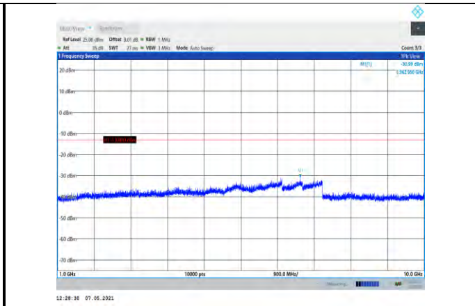
Band5-10MHz-16QAM-20525-1RB#0- Range2:1000~10000MHz
