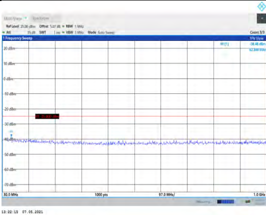
Band7-5MHz-16QAM-21100-1RB#0- Range1:30~1000MHz
