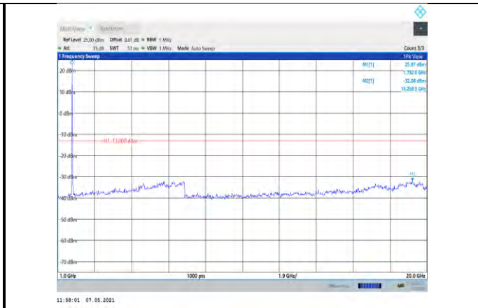
Band4-20MHz-16QAM-20175-1RB#0- Range2:1000~20000MHz
