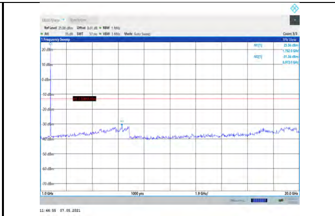
Band4-15MHz-16QAM-20175-1RB#0- Range2:1000~20000MHz
