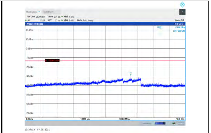
Band26-3MHz-16QAM-26740-1RB#0- Range2:1000~10000MHz
