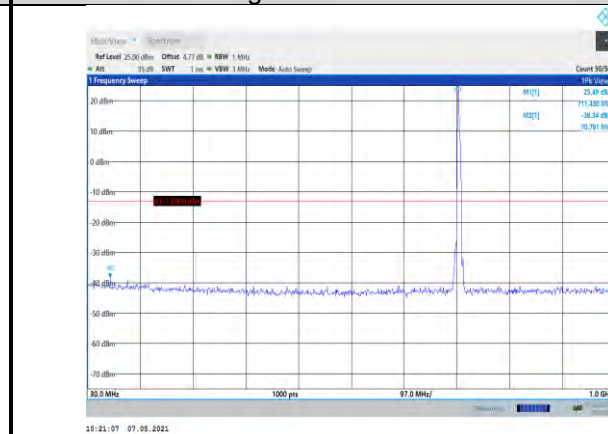
Band17-5MHz-QPSK-23825-1RB#0- Range1:30~1000MHz
