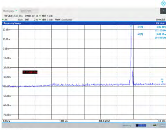
Band38-10MHz-16QAM-37800-1RB#0- Range2:1000~3000MHz
