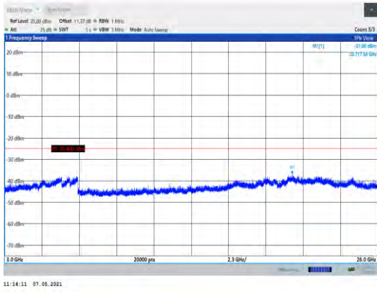
Band38-5MHz-QPSK-37775-1RB#0- Range3:3000~26000MHz
