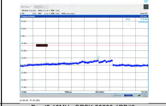
Band5-10MHz-QPSK-20600-1RB#0- Range2:1000~10000MHz
