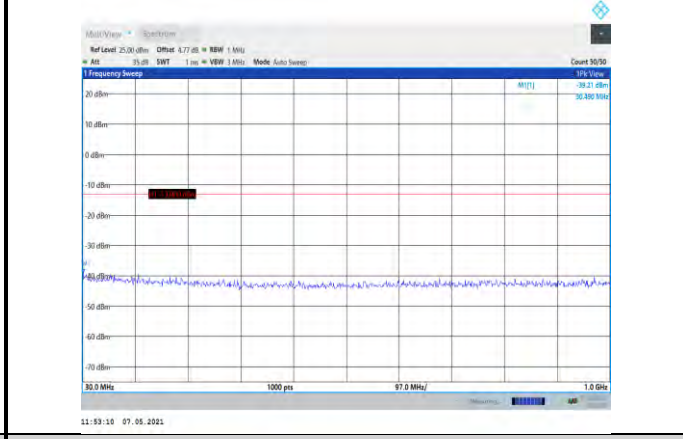
Band4-5MHz-QPSK-20375-1RB#0-Range1:30~1000MHz
