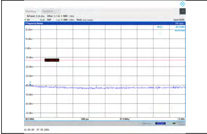
Band4-1.4MHz-16QAM-20175-1RB#0- Range1:30~1000MHz
