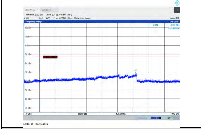
Band26-5MHz-16QAM-26715-1RB#0- Range2:1000~10000MHz
