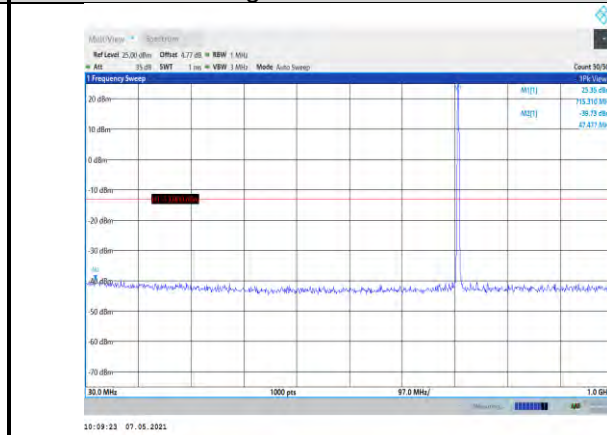
Band12-1.4MHz-QPSK-23173-1RB#0- Range1:30~1000MHz
