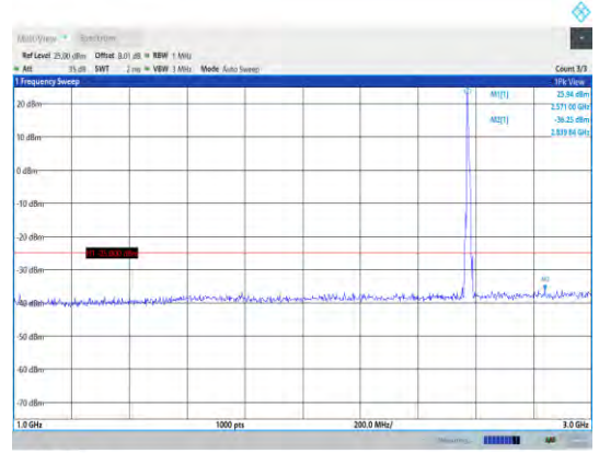
Band38-10MHz-QPSK-37800-1RB#0-Range2:1000~3000MHz
