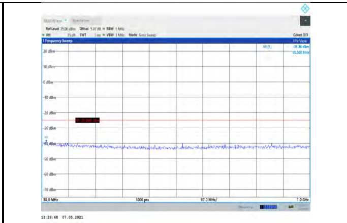
Band7-20MHz-16QAM-21350-1RB#0- Range1:30~1000MHz
