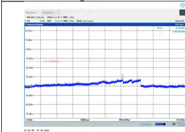
Band12-5MHz-QPSK-23035-1RB#0- Range2:1000~10000MHz
