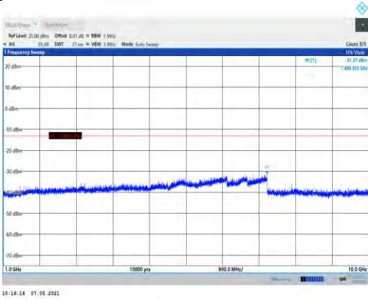
Band17-10MHz-16QAM-23780-1RB#0- Range2:1000~10000MHz
