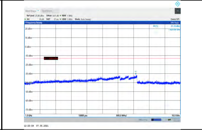
Band5-3MHz-16QAM-20635-1RB#0- Range2:1000~10000MHz
