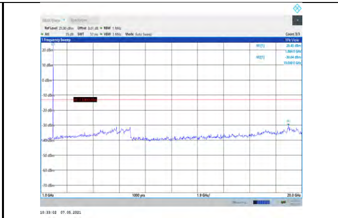
Band2-3MHz-16QAM-18900-1RB#0- Range2:1000~20000MHz
