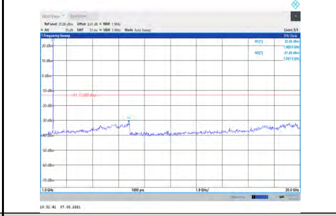
Band2-10MHz-16QAM-19150-1RB#0- Range2:1000~20000MHz
