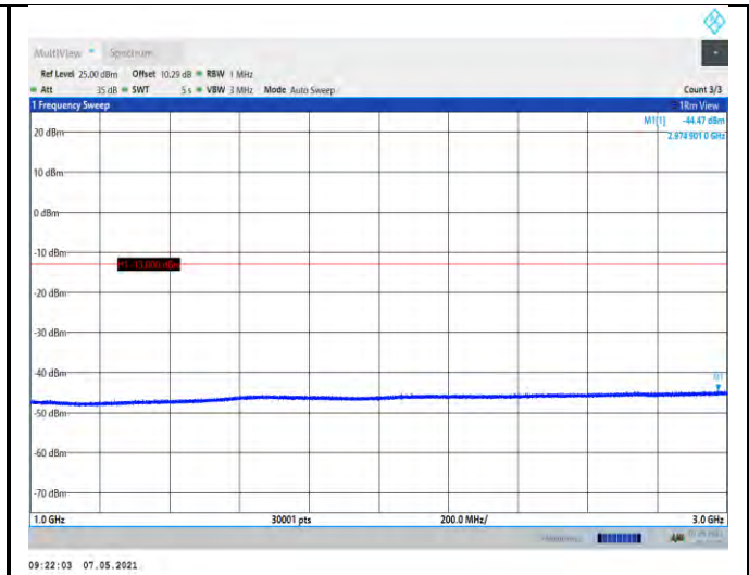
Band5-4132-1000~3000MHz
