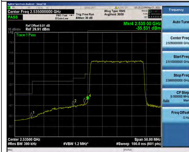
Band41-20MHz-QPSK-40140-100RB#0
