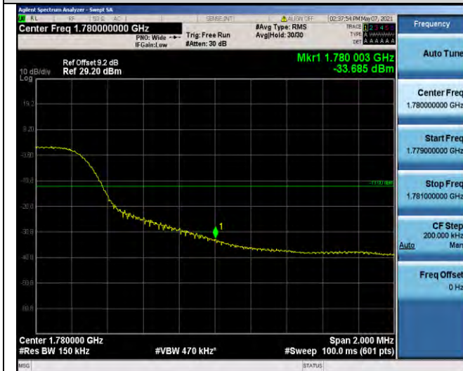
Band66-15MHz-QPSK-132597-75RB#0
