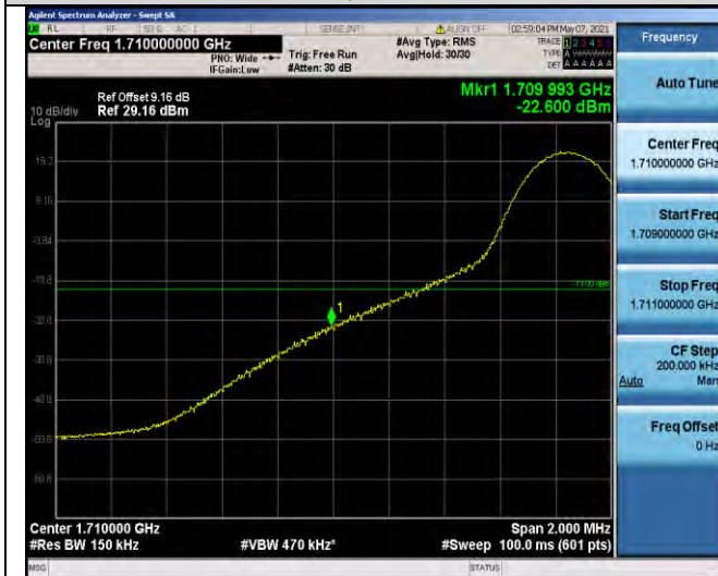
Band66-15MHz-16QAM-132047-1RB#0
