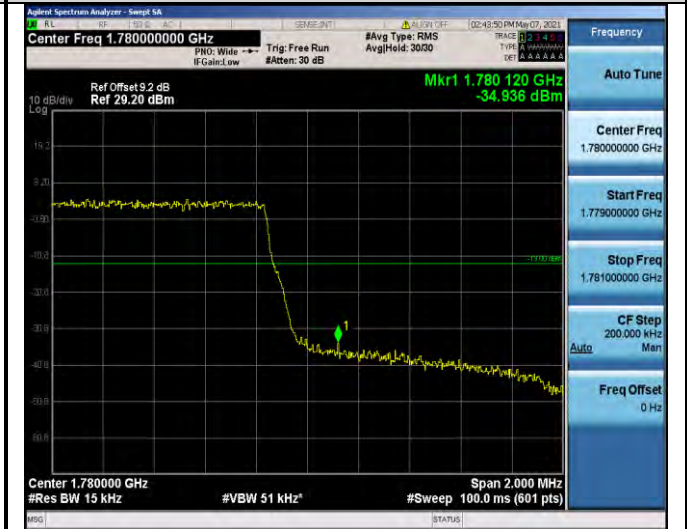
Band66-1.4MHz-QPSK-132665-6RB#0
