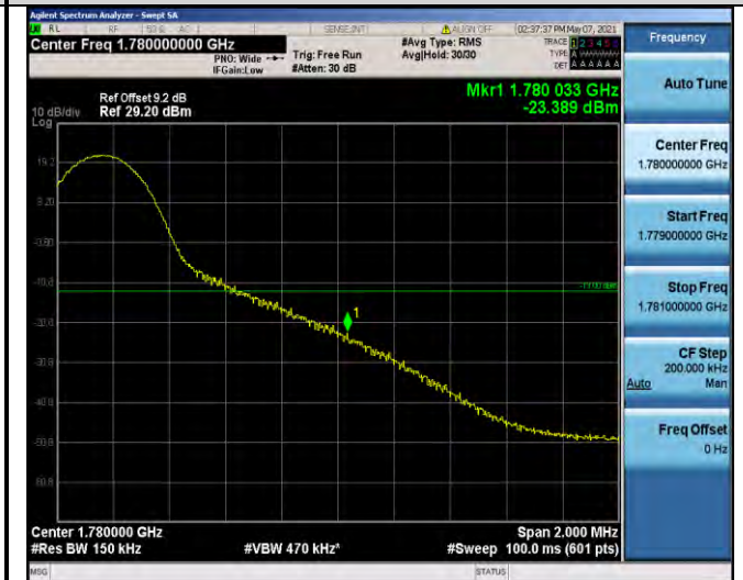
Band66-15MHz-16QAM-132047-75RB#0
