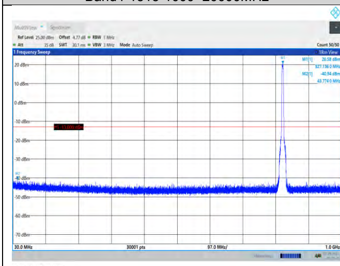
Band5-4132-30~1000MHz
