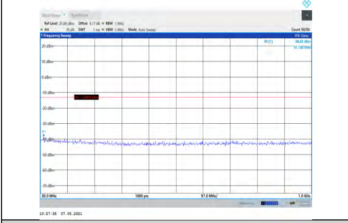
Band2-15MHz-16QAM-18900-1RB#0- Range1:30~1000MHz
