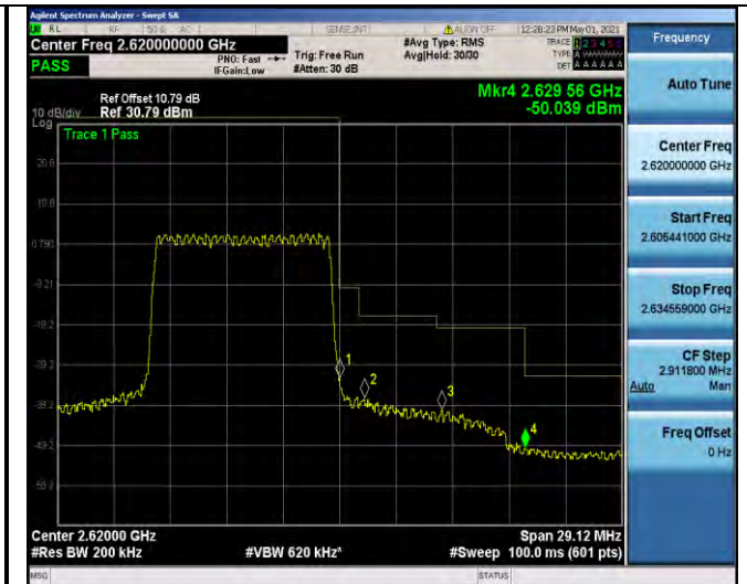
Band38-10MHz-QPSK-38200-50RB#0
