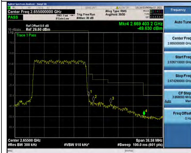
Band41-15MHz-QPSK-41165-75RB#0
