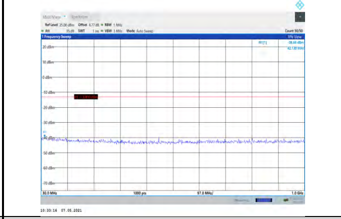
Band2-3MHz-QPSK-19185-1RB#0-Range1:30~1000MHz
