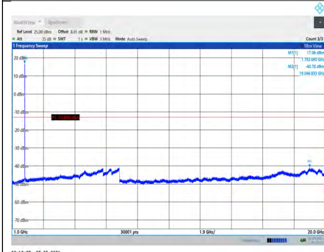
Band4-1513-1000~20000MHz
