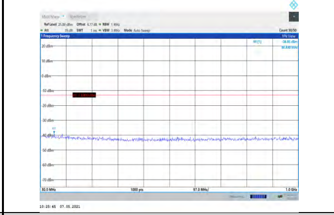
Band2-20MHz-QPSK-19100-1RB#0- Range1:30~1000MHz
