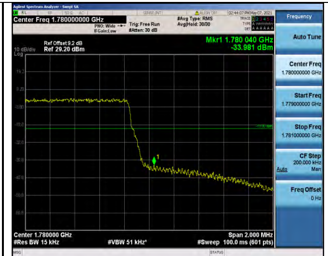
Band66-1.4MHz-16QAM-132665-6RB#0
