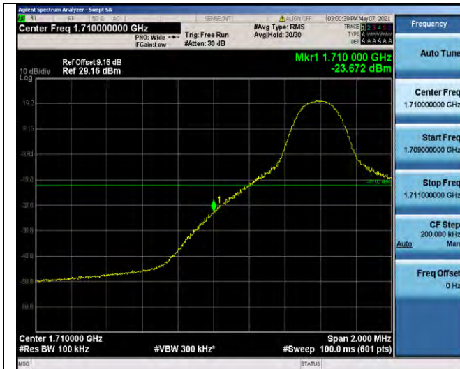
Band66-10MHz-16QAM-132022-1RB#0
