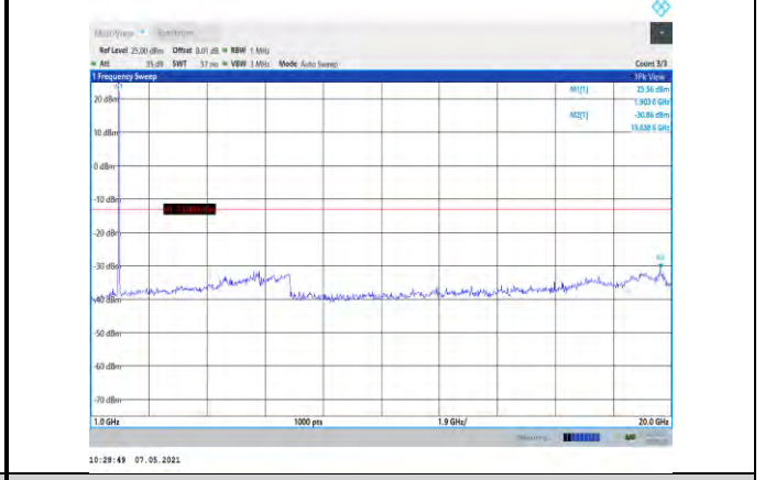
Band2-15MHz-16QAM-19125-1RB#0- Range2:1000~20000MHz
