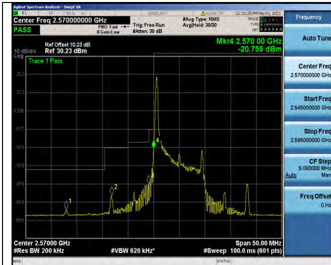
Band38-10MHz-QPSK-37800-1RB#0
