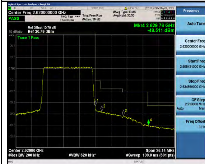
Band38-10MHz-16QAM-38200-50RB#0
