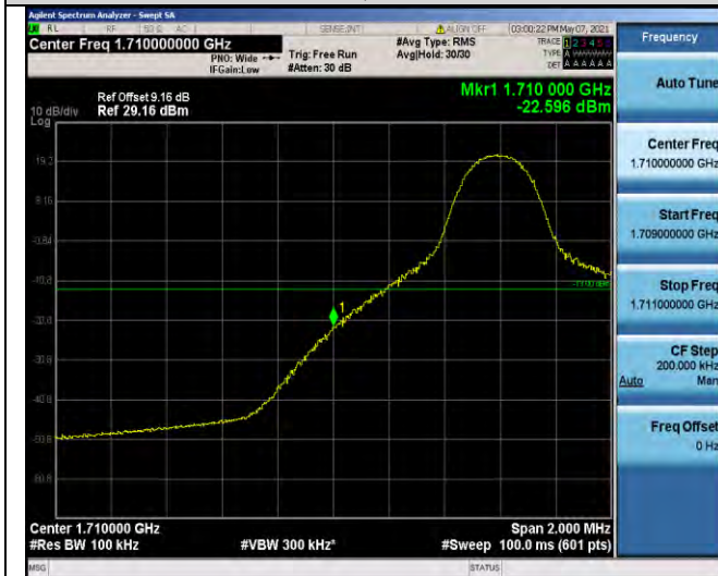
Band66-10MHz-QPSK-132022-1RB#0
