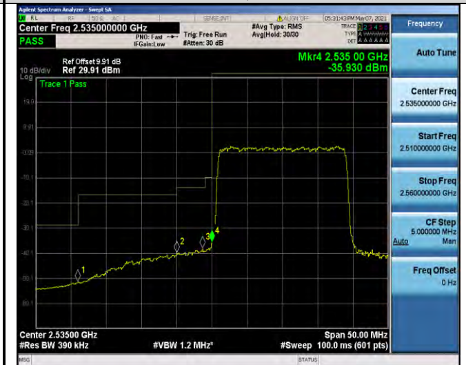
Band41-20MHz-16QAM-40140-100RB#0
