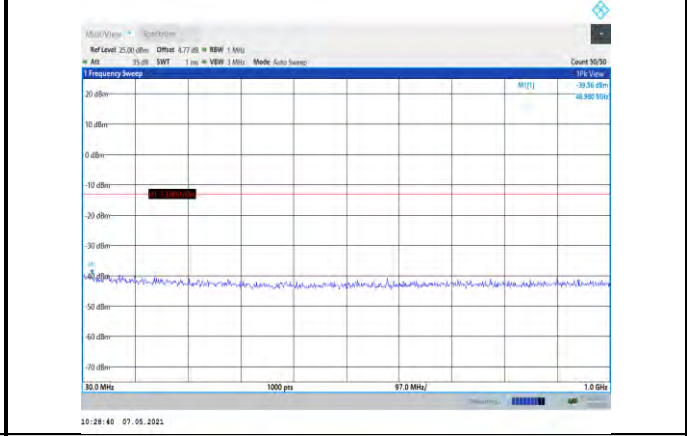
Band2-15MHz-16QAM-19125-1RB#0- Range1:30~1000MHz
