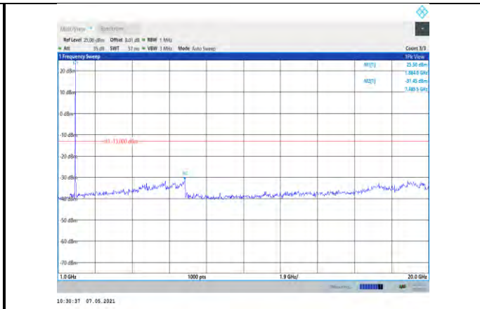
Band2-10MHz-16QAM-18900-1RB#0- Range2:1000~20000MHz
