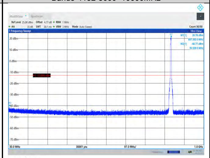
Band5-4182-30~1000MHz
