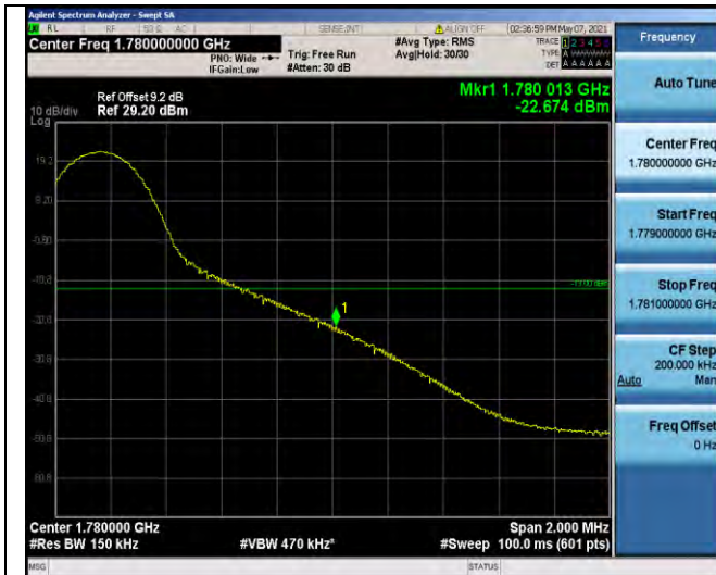
Band66-15MHz-QPSK-132597-1RB#74
