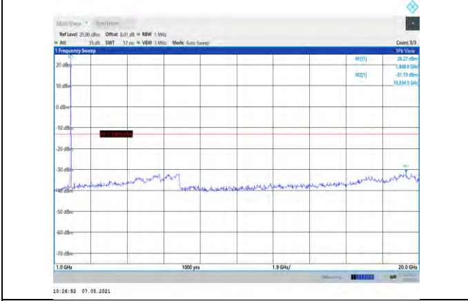
Band2-15MHz-16QAM-18675-1RB#0- Range2:1000~20000MHz
