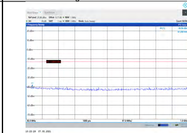
Band2-1.4MHz-16QAM-19193-1RB#0- Range1:30~1000MHz
