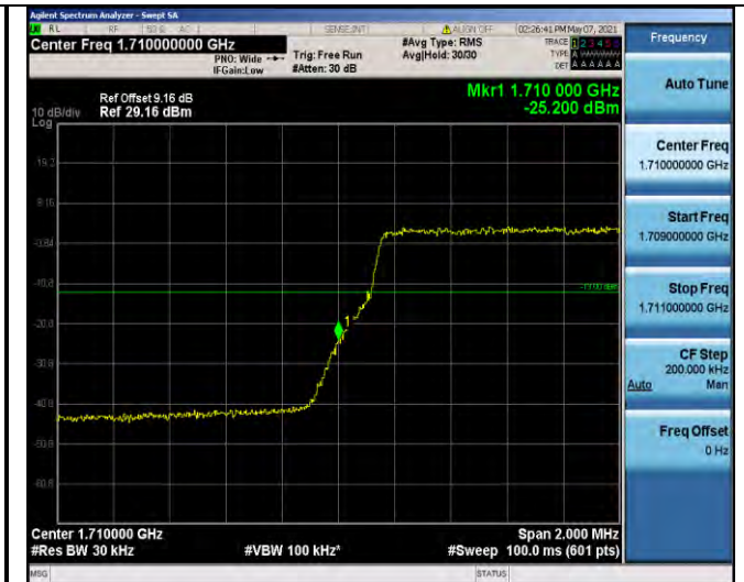
Band66-3MHz-16QAM-131987-15RB#0
