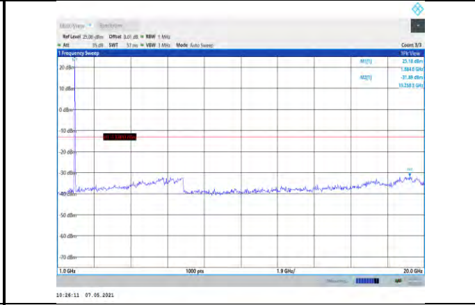
Band2-20MHz-16QAM-19100-1RB#0- Range2:1000~20000MHz
