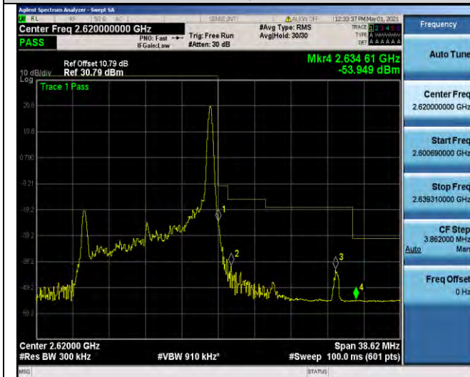
Band38-15MHz-16QAM-38175-1RB#74
