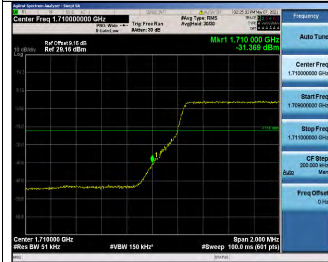
Band66-5MHz-QPSK-131997-25RB#0
