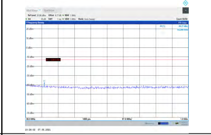
Band2-20MHz-16QAM-19100-1RB#0- Range1:30~1000MHz
