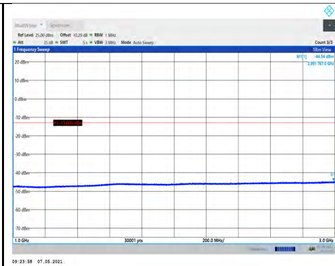
Band5-4233-1000~3000MHz
