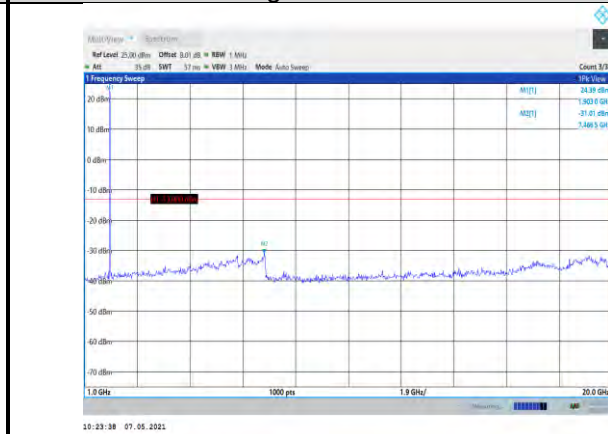
Band2-1.4MHz-16QAM-19193-1RB#0- Range2:1000~20000MHz
