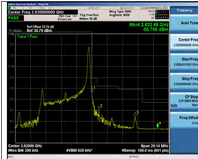
Band38-10MHz-16QAM-38200-1RB#49
