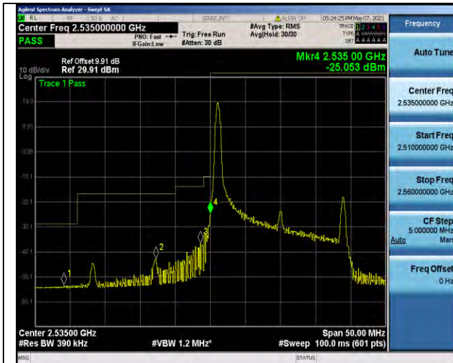
Band41-20MHz-QPSK-40140-1RB#0
