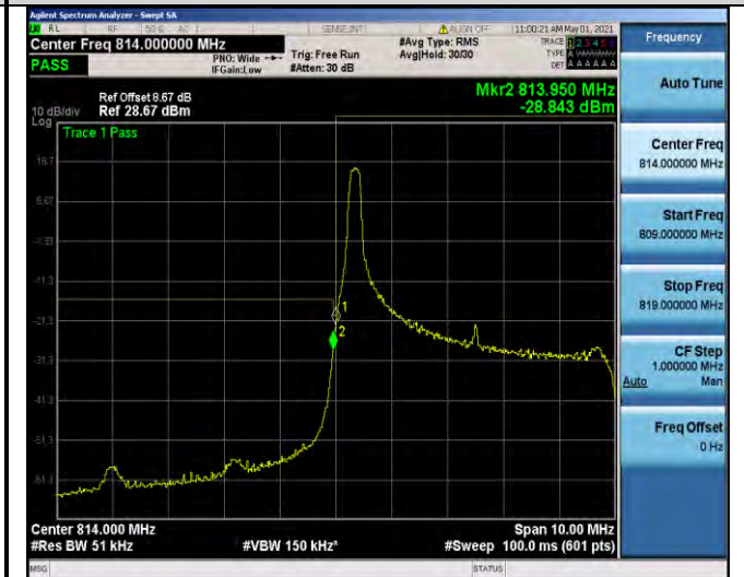
Band26-5MHz-16QAM-26715-1RB#0
