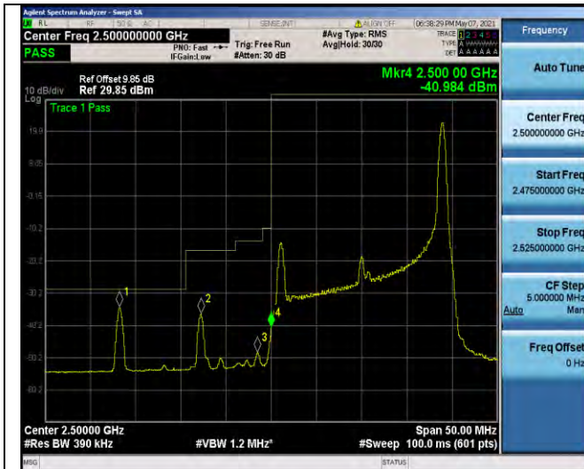
Band7-20MHz-QPSK-20850-1RB#99
