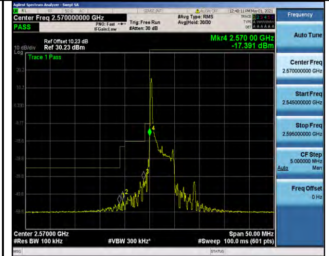
Band38-5MHz-QPSK-37775-1RB#0
