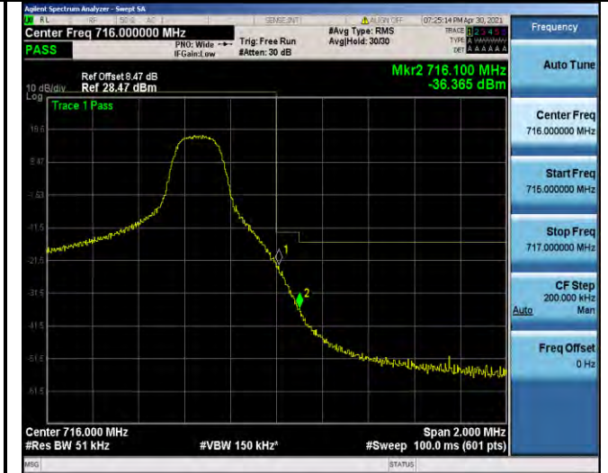
Band17-5MHz-16QAM-23825-1RB#24
