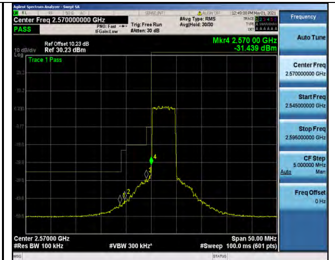
Band38-5MHz-16QAM-37775-25RB#0
