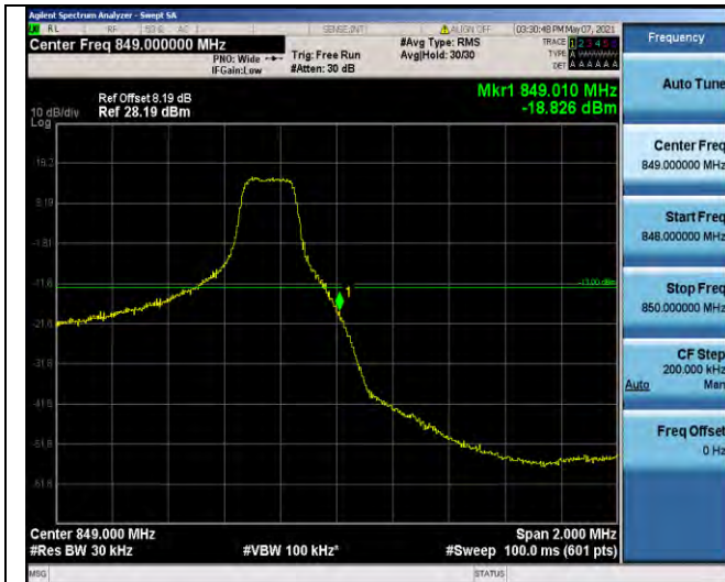
Band5-3MHz-16QAM-20635-1RB#14
