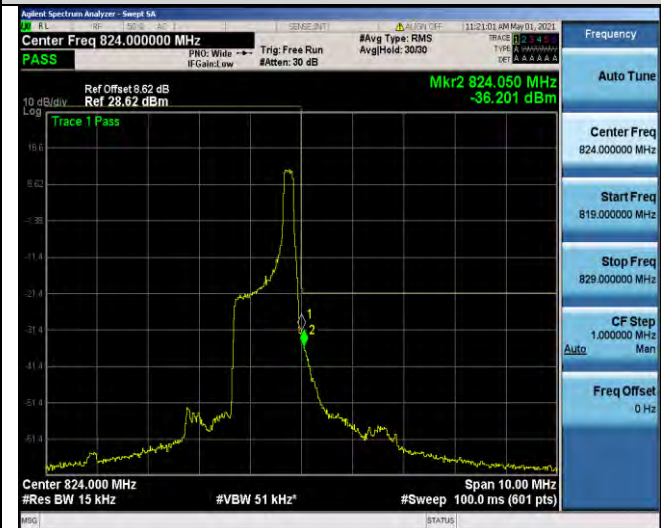
Band26-1.4MHz-QPSK-26783-1RB#5
