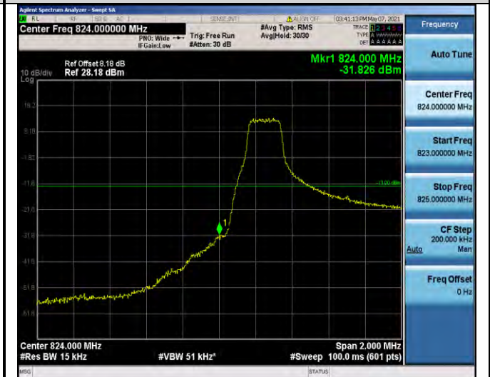
Band5-1.4MHz-QPSK-20407-1RB#0
