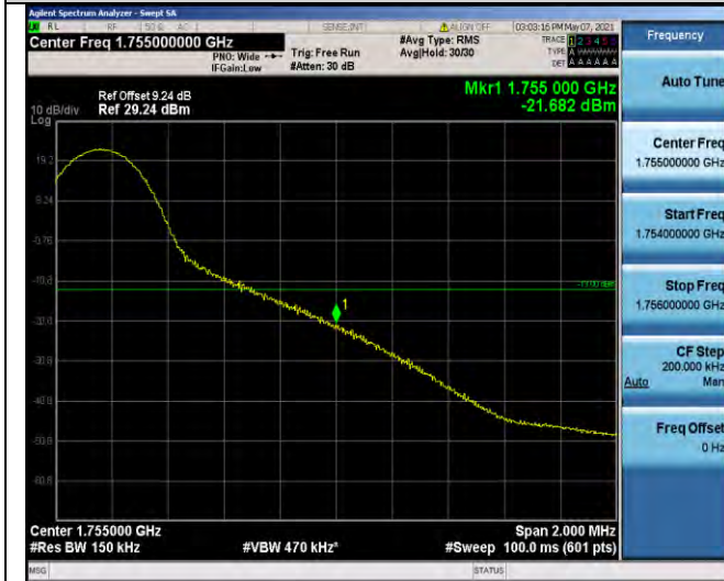
Band4-15MHz-QPSK-20325-1RB#74
