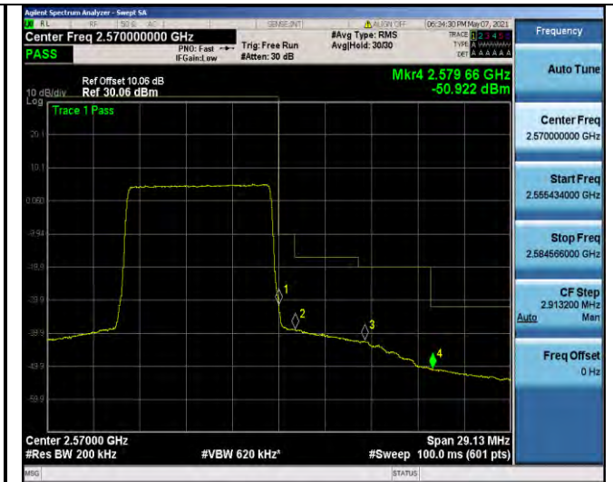
Band7-10MHz-16QAM-21400-50RB#0
