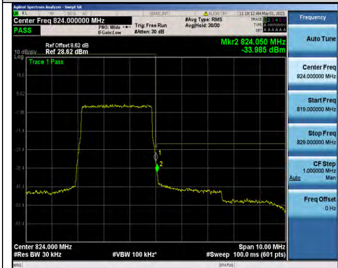
Band26-3MHz-QPSK-26775-15RB#0
