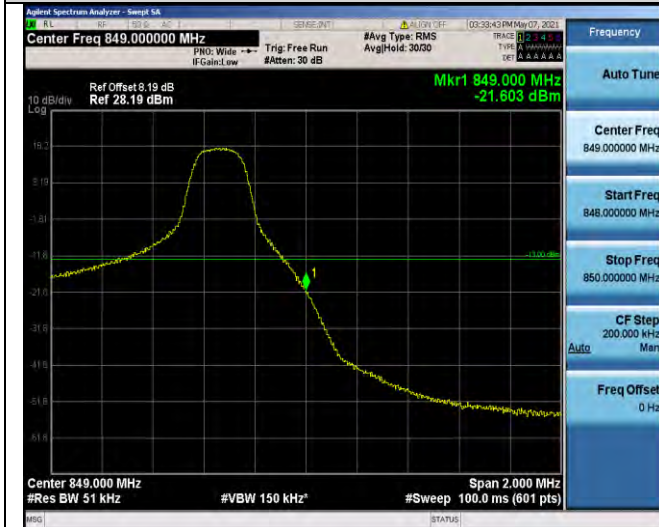
Band5-5MHz-16QAM-20625-1RB#24
