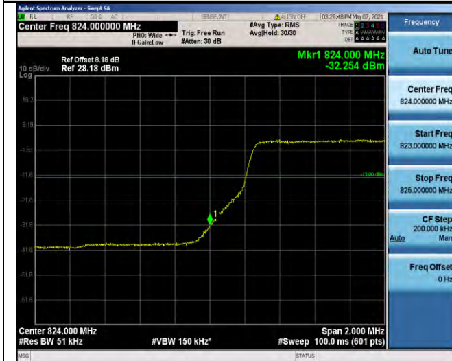
Band5-5MHz-16QAM-20425-25RB#0
