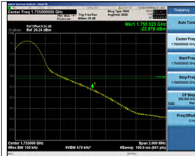
Band4-15MHz-16QAM-20325-1RB#74
