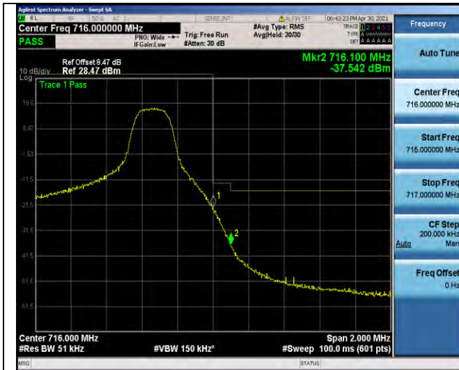
Band12-5MHz-16QAM-23155-1RB#24
