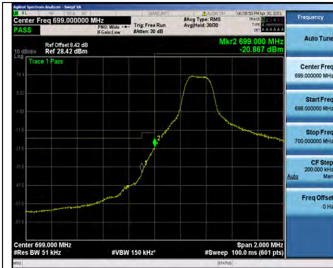
Band12-5MHz-QPSK-23035-1RB#0
