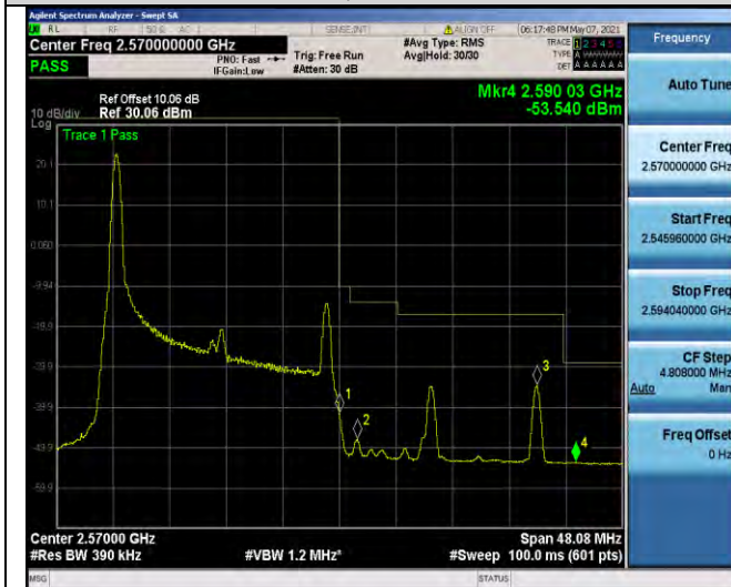
Band7-20MHz-QPSK-21350-1RB#0
