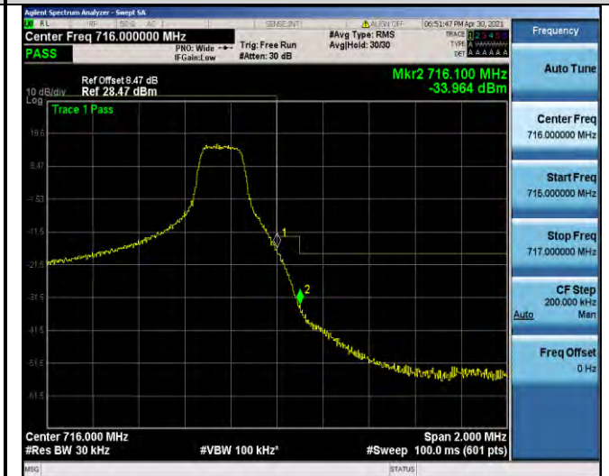
Band12-3MHz-16QAM-23165-1RB#14
