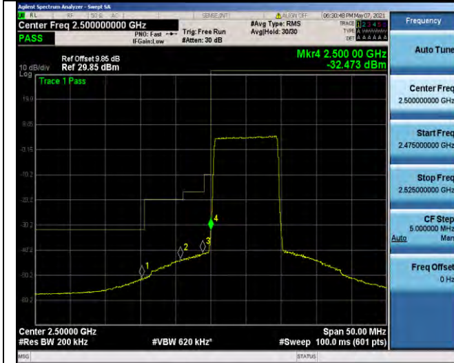
Band7-10MHz-16QAM-20800-50RB#0
