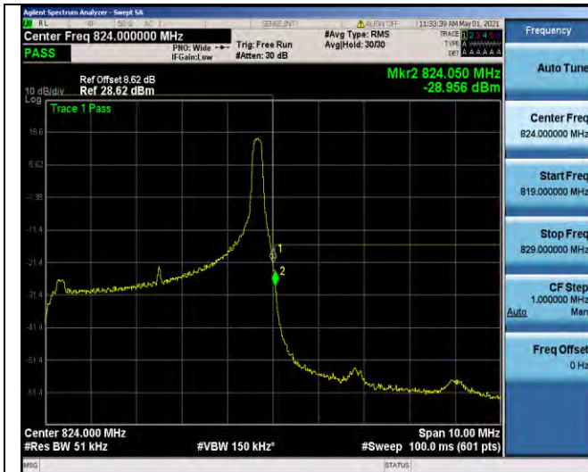
Band26-5MHz-16QAM-26765-1RB#24
