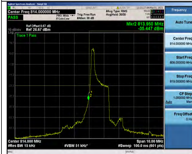
Band26-1.4MHz-QPSK-26697-1RB#0
