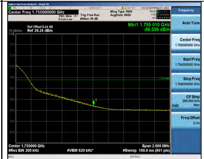
Band4-20MHz-QPSK-20300-100RB#0
