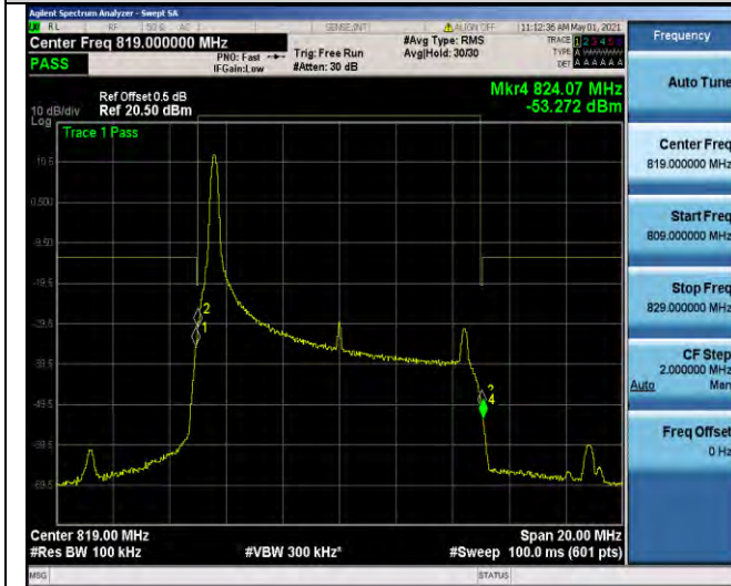
Band26-10MHz-QPSK-26740 Left-1RB#0
