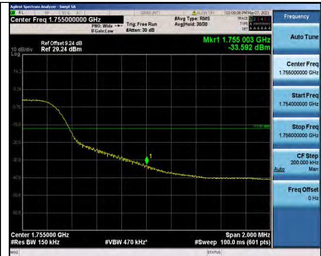
Band4-15MHz-QPSK-20325-75RB#0
