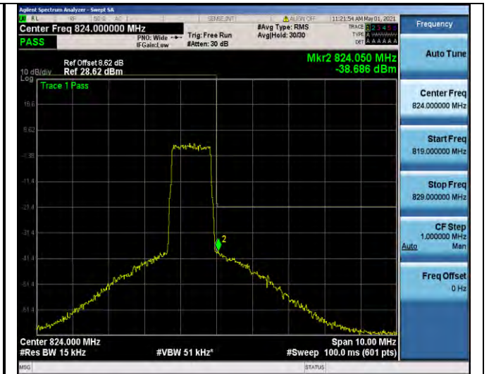
Band26-1.4MHz-16QAM-26783-6RB#0
