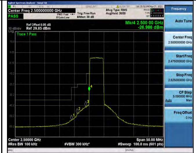
Band7-5MHz-16QAM-20775-25RB#0
