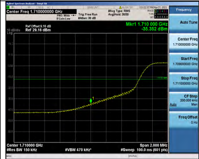
Band4-15MHz-16QAM-20025-75RB#0
