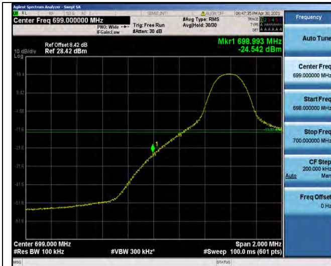
Band12-10MHz-16QAM-23060-1RB#0
