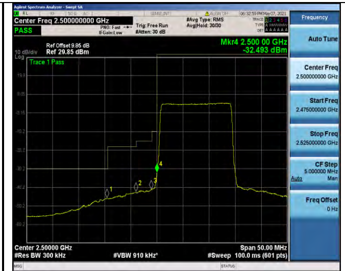
Band7-15MHz-16QAM-20825-75RB#0
