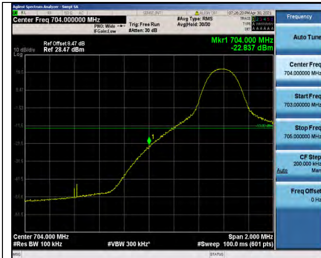
Band17-10MHz-QPSK-23780-1RB#0
