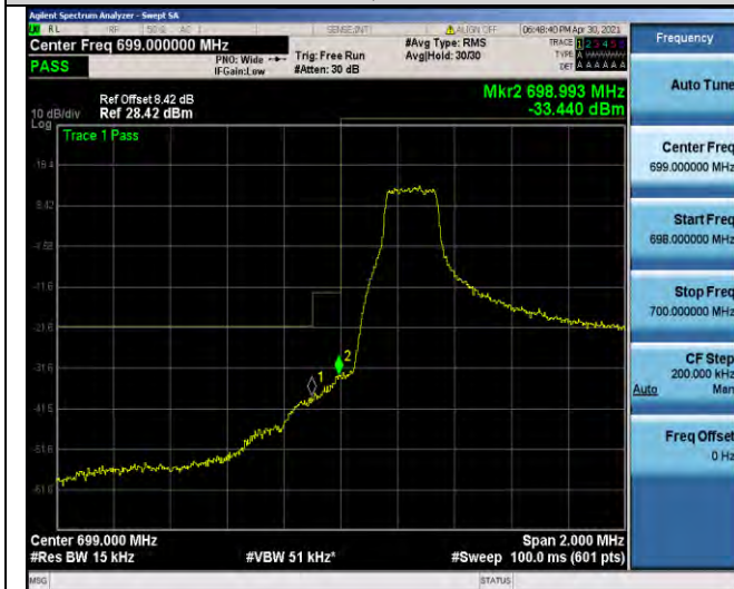
Band12-1.4MHz-QPSK-23017-1RB#0
