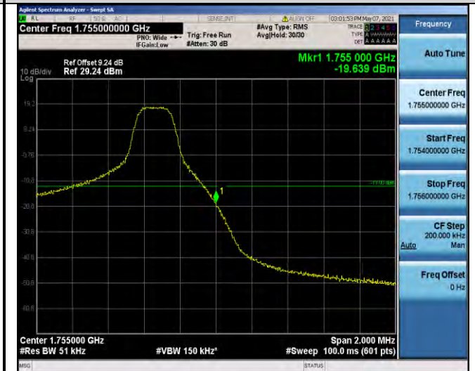
Band4-5MHz-QPSK-20375-1RB#24
