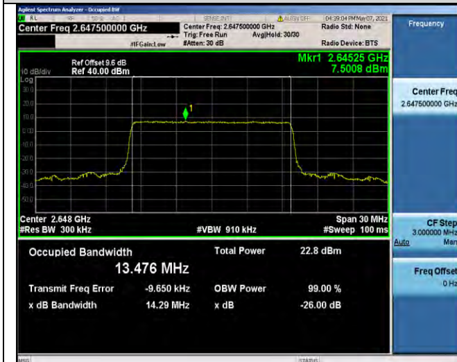
Band41-15MHz-QPSK-41165-75RB#0-13.476
