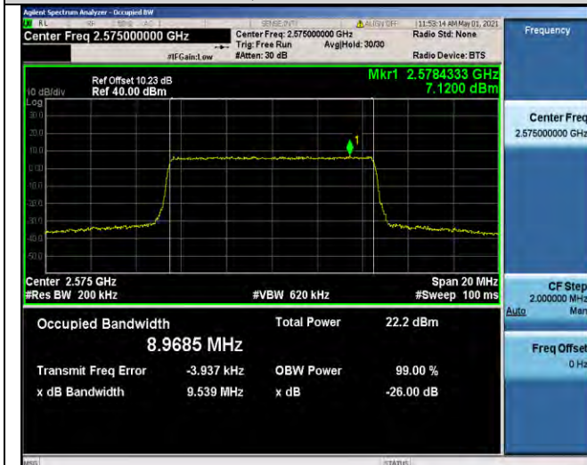
Band38-10MHz-16QAM-37800-50RB#0-8.9685
