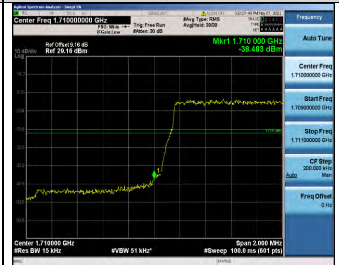
Band4-1.4MHz-QPSK-19957-6RB#0
