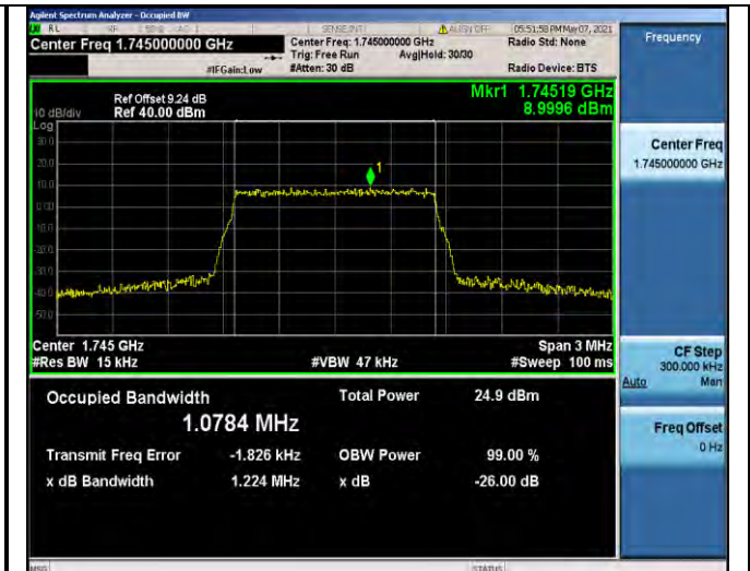
Band66-1.4MHz-16QAM-132322-6RB#0-1.0784
