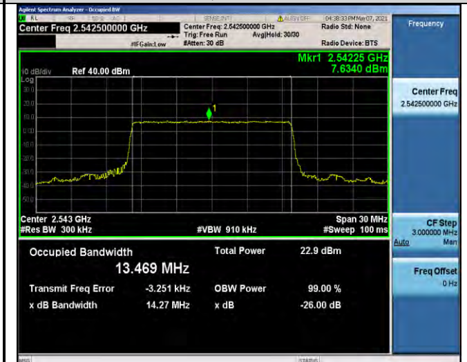
Band41-15MHz-QPSK-40115-75RB#0-13.469
