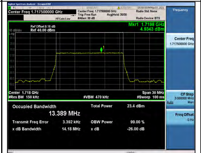
Band66-15MHz-QPSK-132047-75RB#0-13.389
