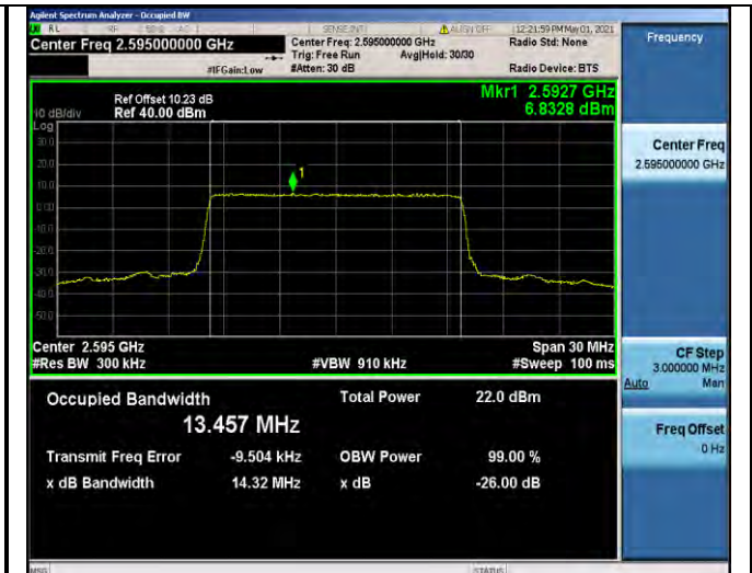
Band38-15MHz-16QAM-38000-75RB#0-13.457
