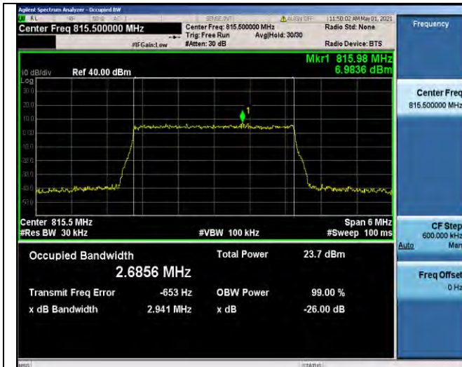
Band26-3MHz-16QAM-26705-15RB#0-2.6856
