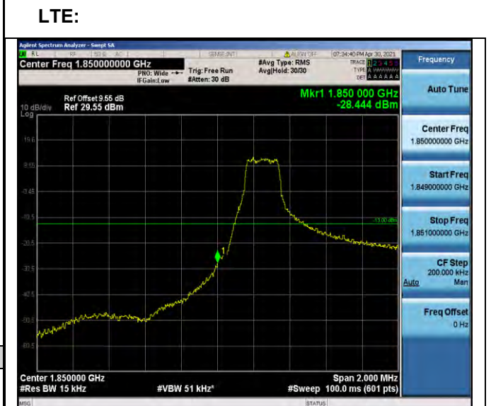
Band2-1.4MHz-QPSK-18607-1RB#0
