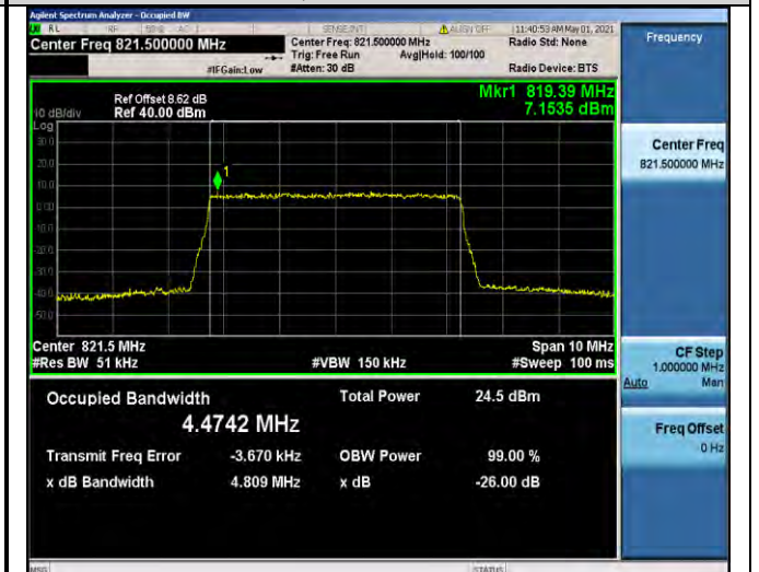
Band26-5MHz-QPSK-26765-25RB#0-4.4742
