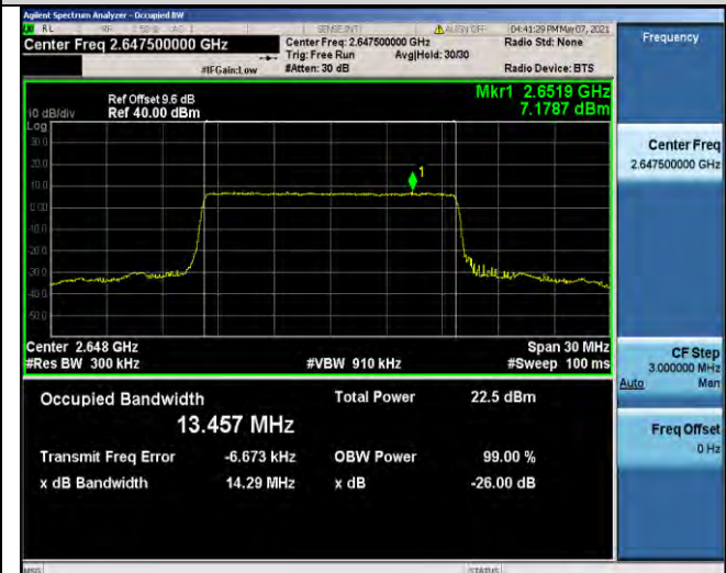
Band41-15MHz-16QAM-41165-75RB#0-13.457
