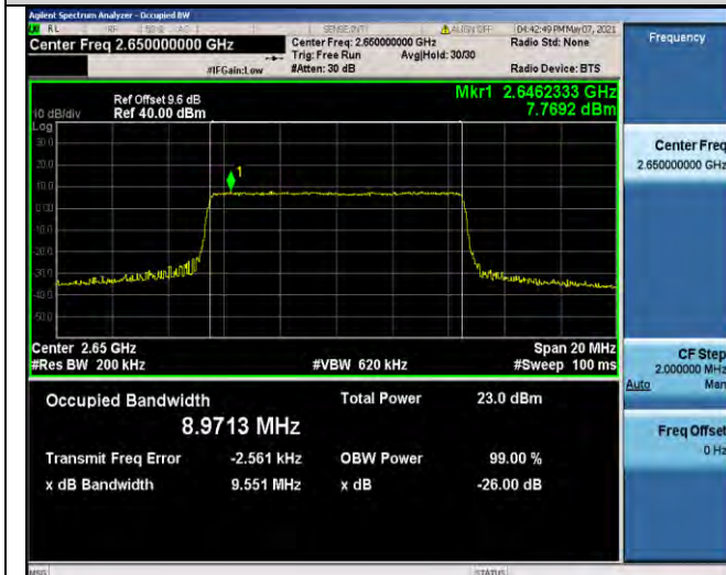
Band41-10MHz-QPSK-41190-50RB#0-8.9713
