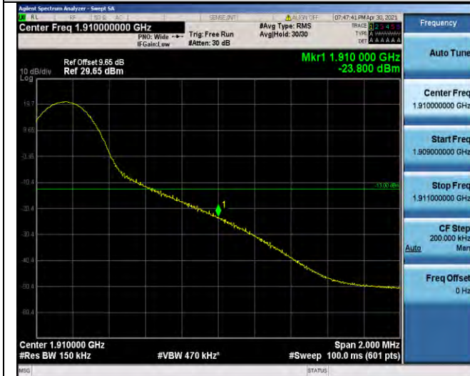
Band2-15MHz-QPSK-19125-1RB#74
