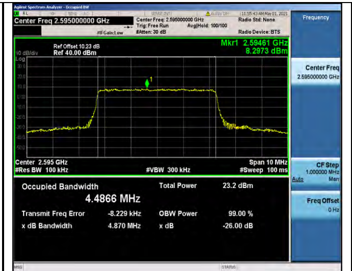
Band38-5MHz-16QAM-38000-25RB#0-4.4866
