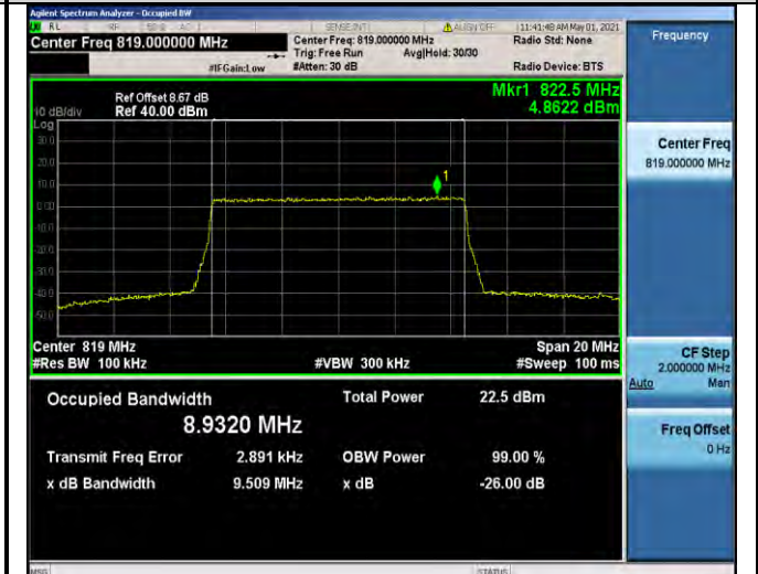
Band26-10MHz-16QAM-26740-50RB#0-8.9320
