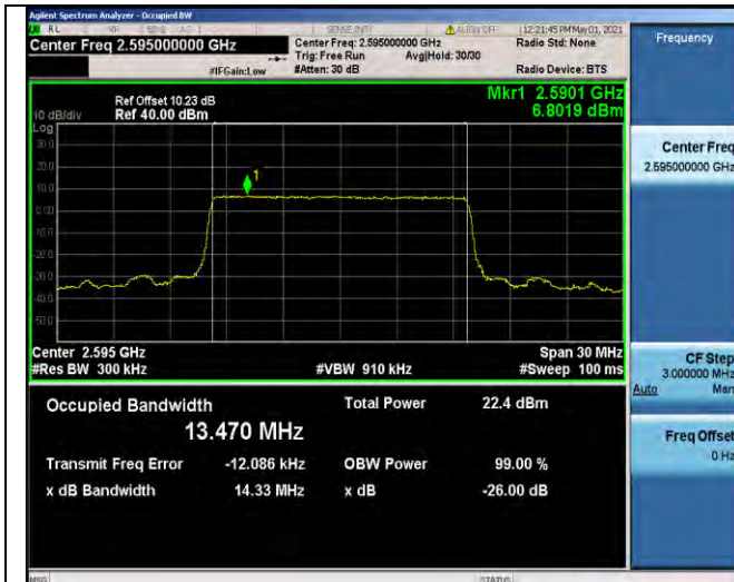
Band38-15MHz-QPSK-38000-75RB#0-13.470
