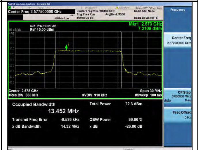
Band38-15MHz-QPSK-37825-75RB#0-13.452
