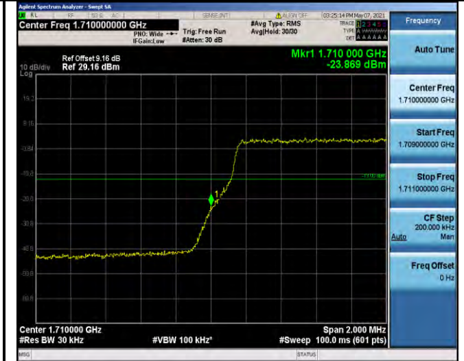
Band4-3MHz-16QAM-19965-15RB#0
