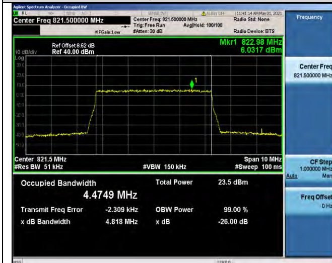
Band26-5MHz-16QAM-26765-25RB#0-4.4749
