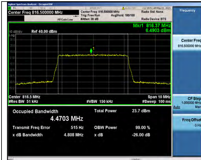
Band26-5MHz-16QAM-26715-25RB#0-4.4703
