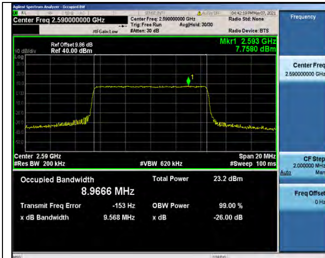
Band41-10MHz-QPSK-40590-50RB#0-8.9666
