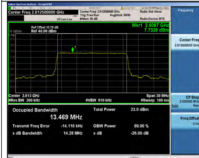
Band38-15MHz-QPSK-38175-75RB#0-13.469
