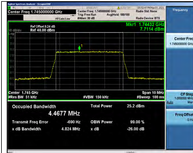
Band66-5MHz-QPSK-132322-25RB#0-4.4677
