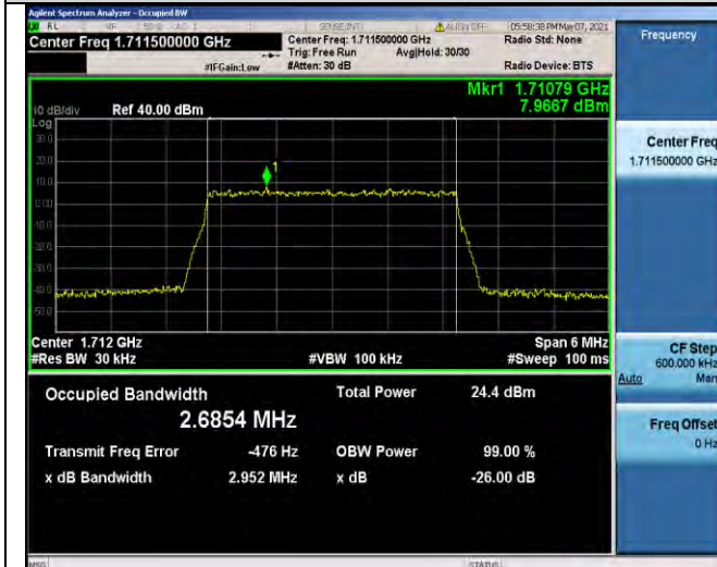
Band66-3MHz-16QAM-131987-15RB#0-2.6854
