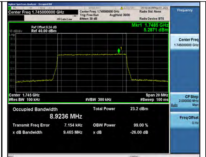
Band66-10MHz-16QAM-132322-50RB#0-8.9236
