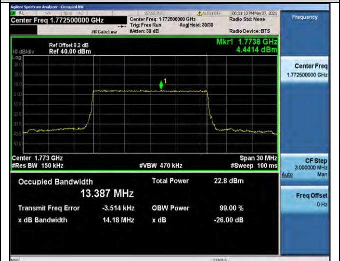
Band66-15MHz-16QAM-132597-75RB#0-13.387
