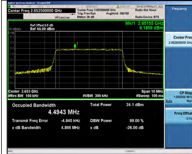
Band41-5MHz-QPSK-41215-25RB#0-4.4943
