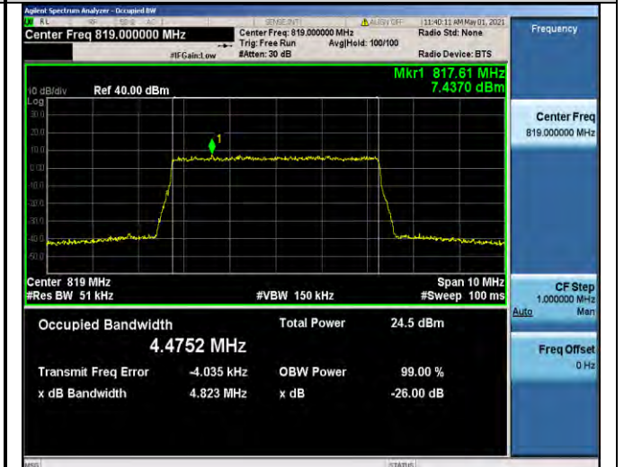
Band26-5MHz-QPSK-26740-25RB#0-4.4752
