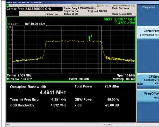
Band41-5MHz-16QAM-40065-25RB#0-4.4941
