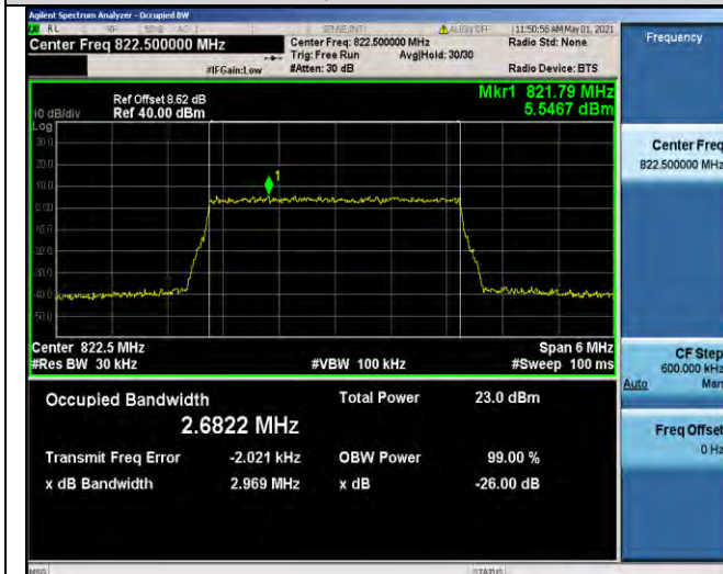
Band26-3MHz-16QAM-26775-15RB#0-2.6822
