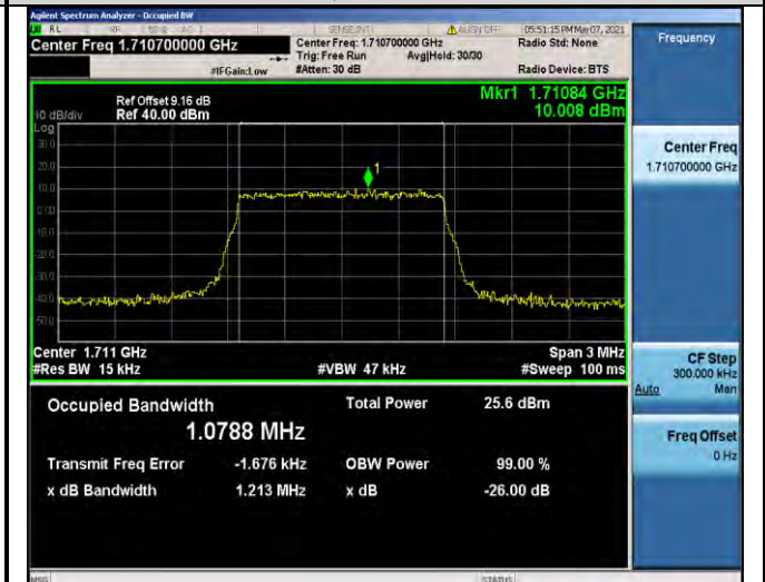
Band66-1.4MHz-QPSK-131979-6RB#0-1.0788
