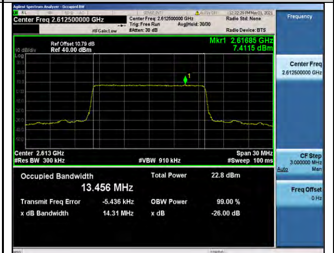
Band38-15MHz-16QAM-38175-75RB#0-13.456
