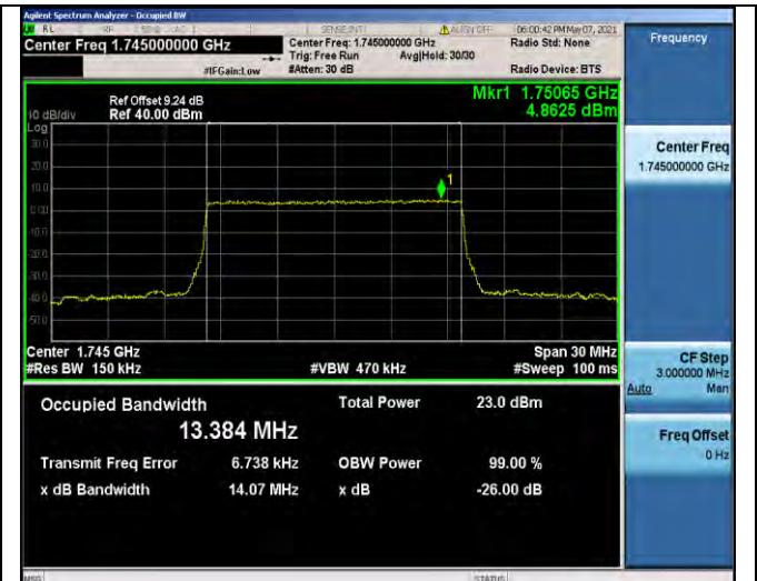
Band66-15MHz-16QAM-132322-75RB#0-13.384
