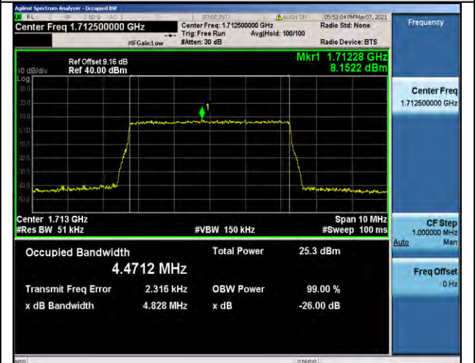
Band66-5MHz-QPSK-131997-25RB#0-4.4712
