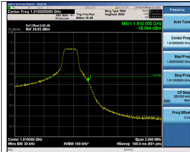
Band2-3MHz-16QAM-19185-1RB#14
