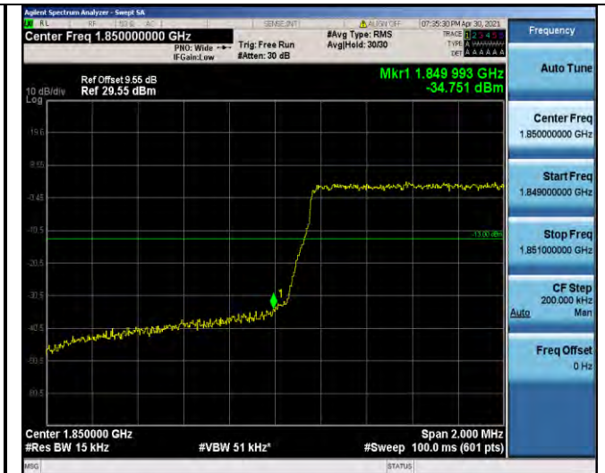
Band2-1.4MHz-16QAM-18607-6RB#0
