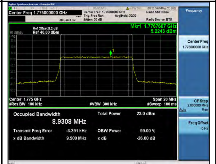
Band66-10MHz-16QAM-132622-50RB#0-8.9308
