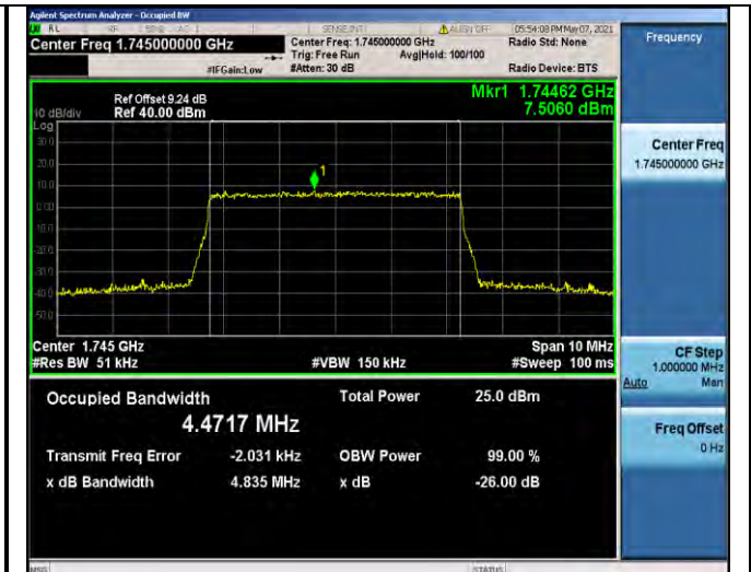
Band66-5MHz-16QAM-132322-25RB#0-4.4717
