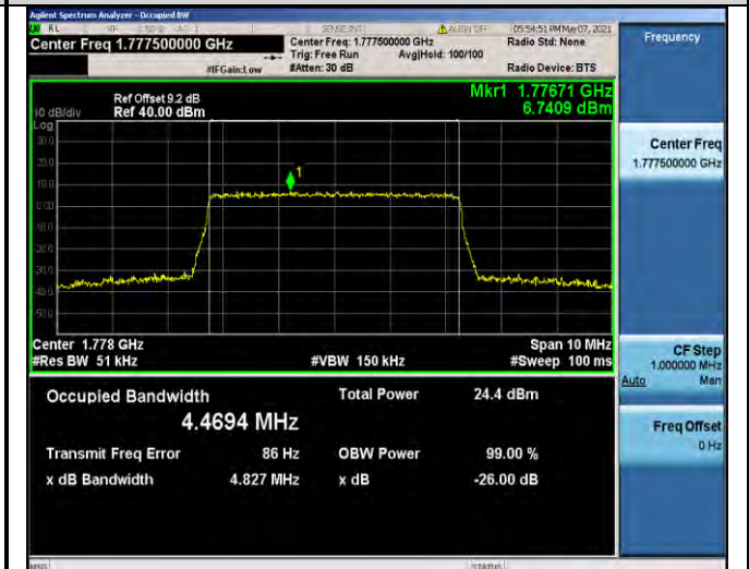
Band66-5MHz-16QAM-132647-25RB#0-4.4694
