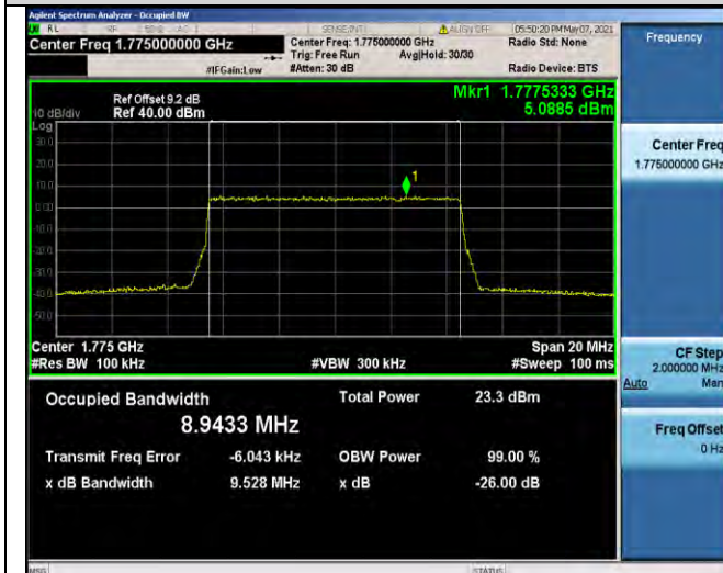
Band66-10MHz-QPSK-132622-50RB#0-8.9433
