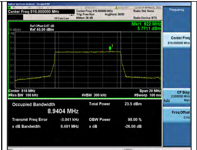
Band26-10MHz-QPSK-26740-50RB#0-8.9404
