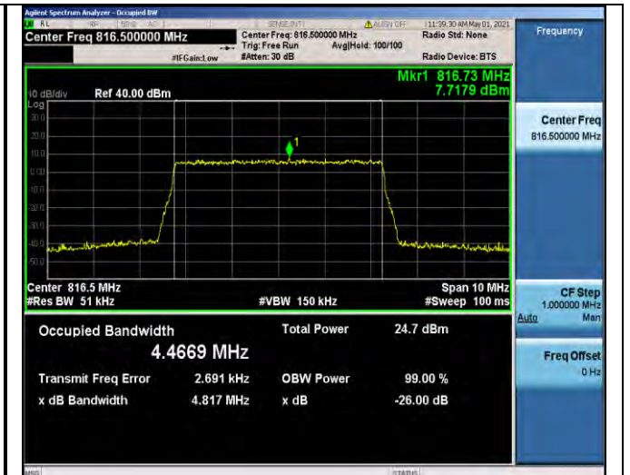
Band26-5MHz-QPSK-26715-25RB#0-4.4669
