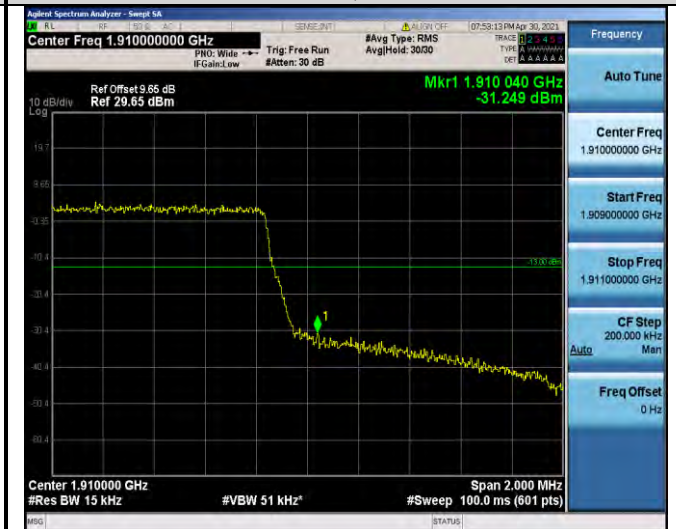
Band2-1.4MHz-16QAM-19193-6RB#0
