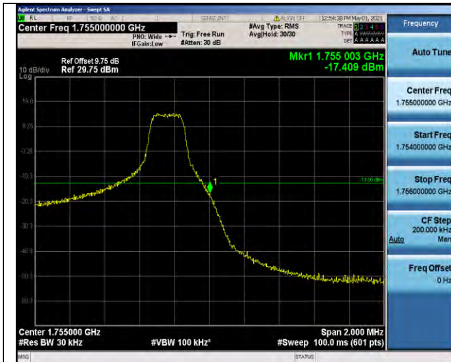
Band4-3MHz-16QAM-20385-1RB#14
