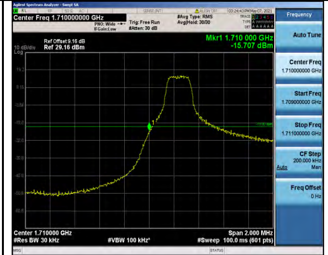
Band4-3MHz-16QAM-19965-1RB#0
