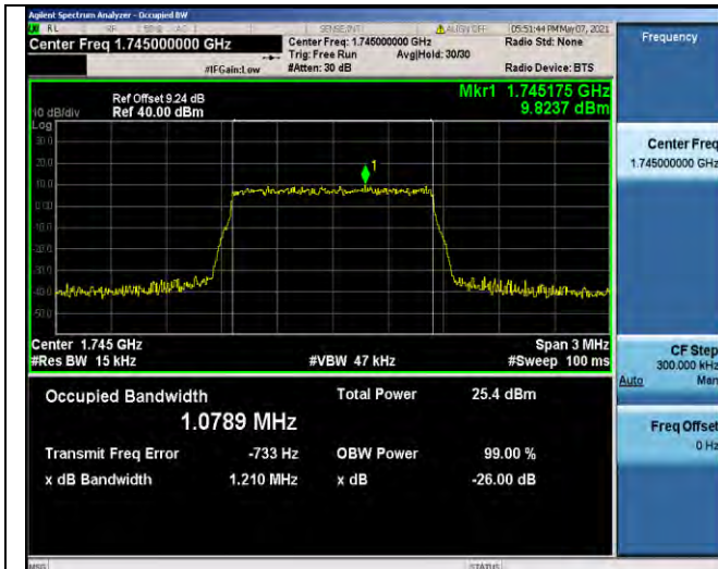
Band66-1.4MHz-QPSK-132322-6RB#0-1.0789
