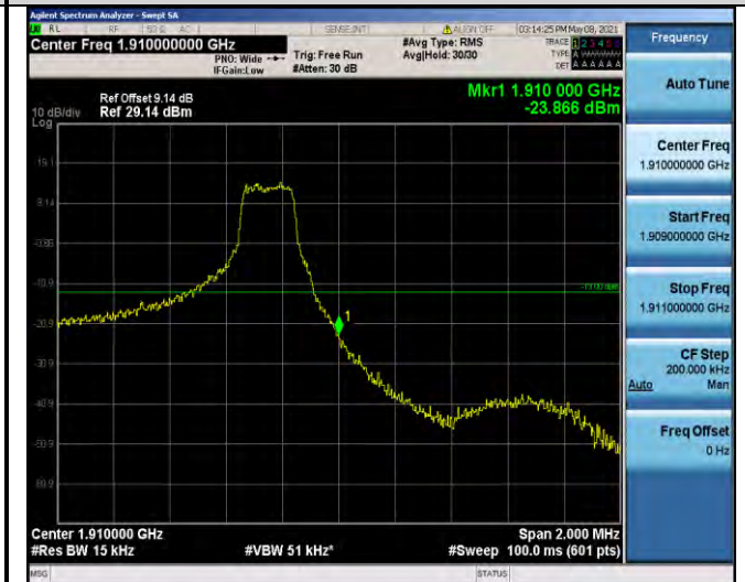
Band2-1.4MHz-16QAM-19193-1RB#5
