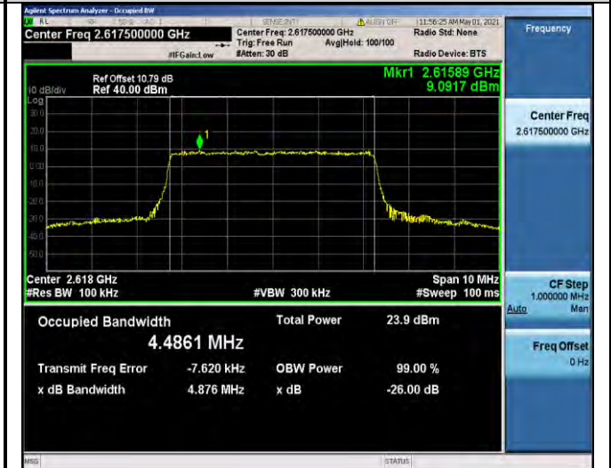
Band38-5MHz-16QAM-38225-25RB#0-4.4861
