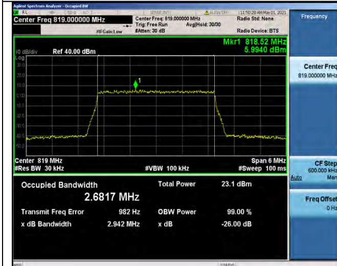
Band26-3MHz-16QAM-26740-15RB#0-2.6817
