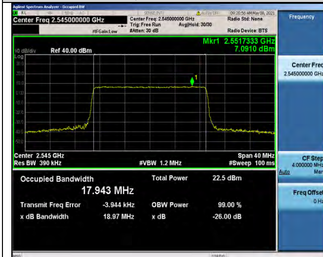
Band41-20MHz-16QAM-40140-100RB#0-17.943
