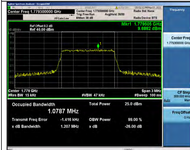
Band66-1.4MHz-QPSK-132665-6RB#0-1.0787
