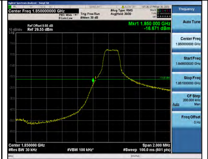
Band2-3MHz-16QAM-18615-1RB#0
