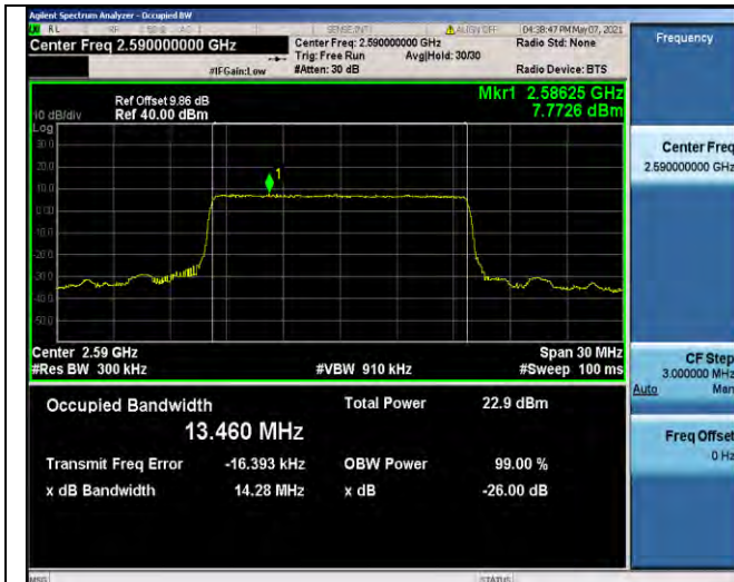
Band41-15MHz-QPSK-40590-75RB#0-13.460
