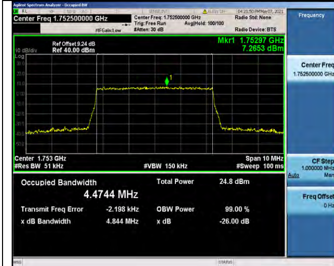
Band4-5MHz-16QAM-20375-25RB#0-4.4744
