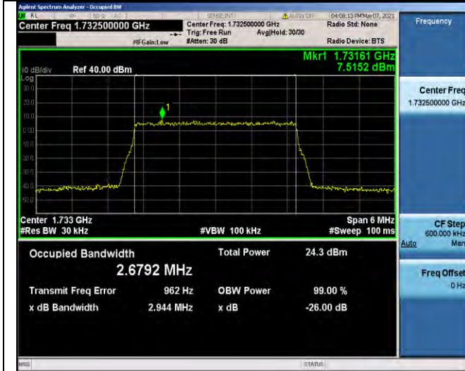
Band4-3MHz-16QAM-20175-15RB#0-2.6792
