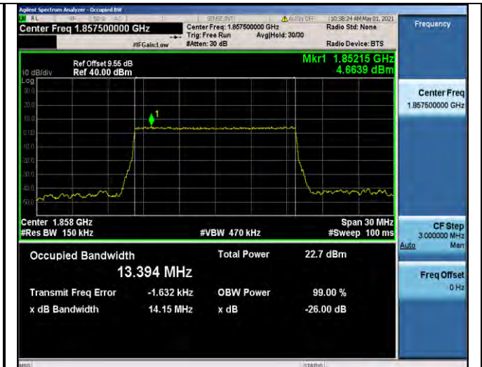
Band2-15MHz-QPSK-18675-75RB#0-13.394
