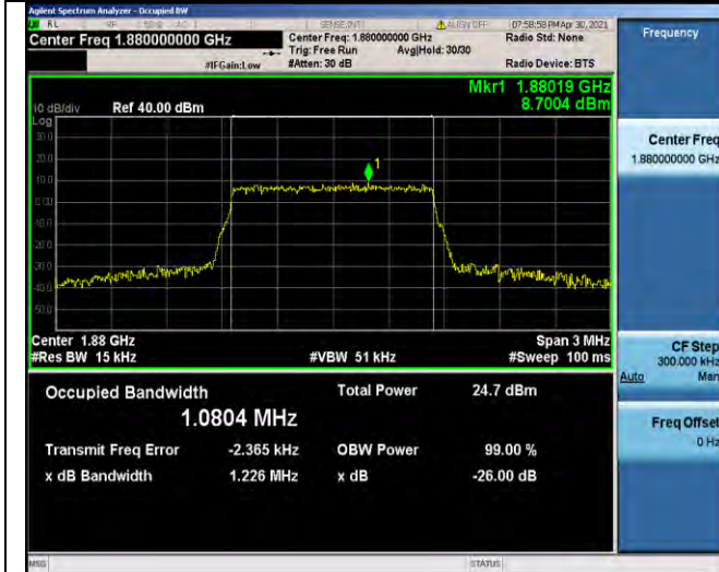
Band2-1.4MHz-16QAM-18900-6RB#0-1.0804
