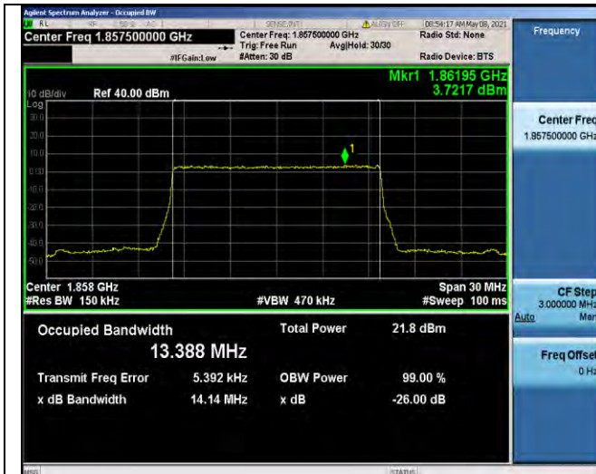
Band2-15MHz-16QAM-18675-75RB#0-13.388
