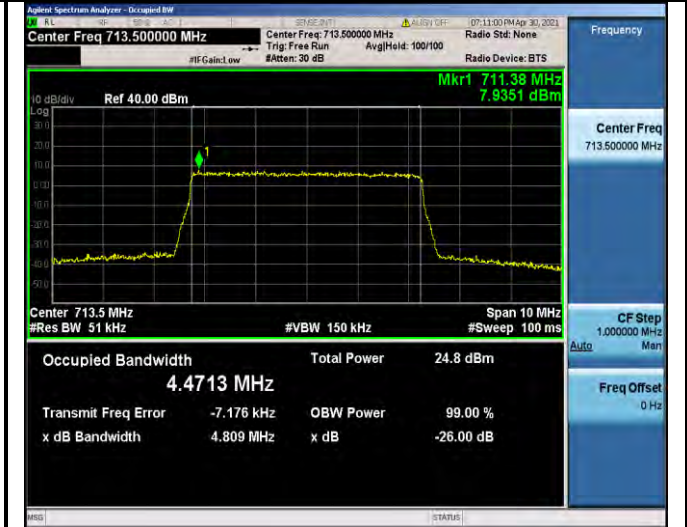
Band12-5MHz-QPSK-23155-25RB#0-4.4713
