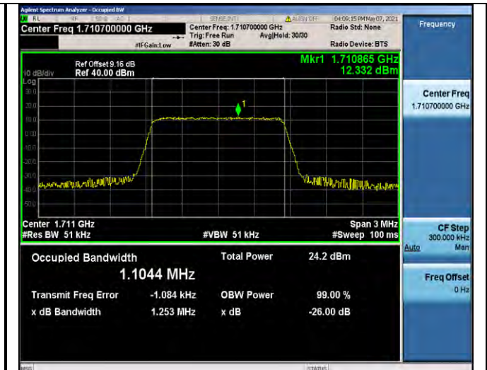
Band4-1.4MHz-QPSK-19957-6RB#0-1.1044
