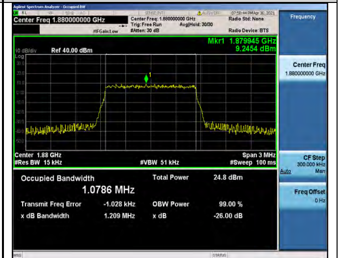
Band2-1.4MHz-QPSK-18900-6RB#0-1.0786
