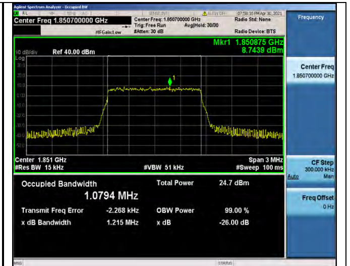
Band2-1.4MHz-QPSK-18607-6RB#0-1.0794
