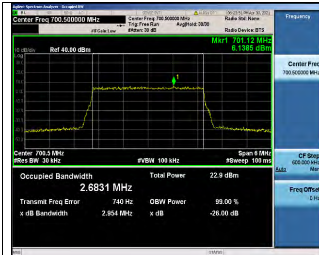
Band12-3MHz-16QAM-23025-15RB#0-2.6831
