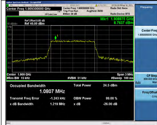
Band2-1.4MHz-16QAM-19193-6RB#0-1.0807
