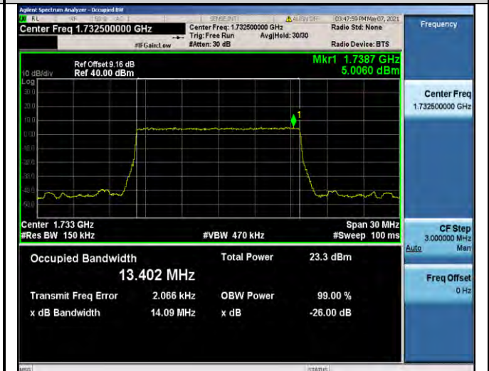
Band4-15MHz-QPSK-20175-75RB#0-13.402
