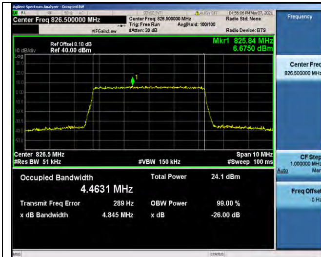
Band5-5MHz-16QAM-20425-25RB#0-4.4631
