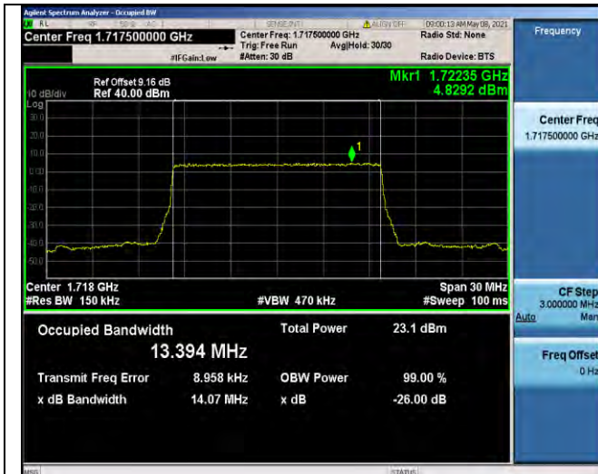
Band4-15MHz-16QAM-20025-75RB#0-13.394
