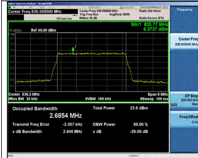
Band5-3MHz-16QAM-20525-15RB#0-2.6854
