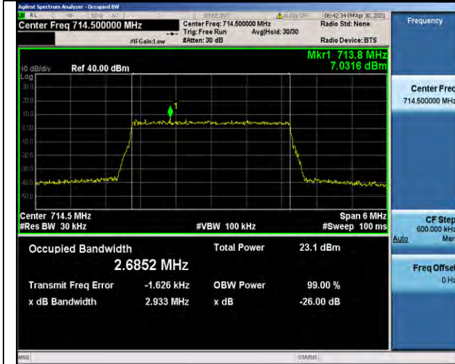
Band12-3MHz-16QAM-23165-15RB#0-2.6852
