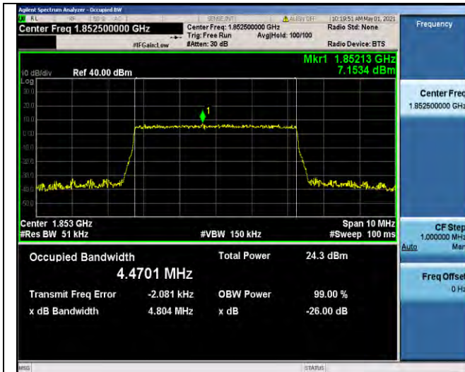
Band2-5MHz-16QAM-18625-25RB#0-4.4701
