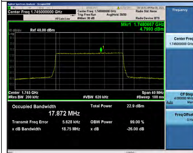
Band4-20MHz-16QAM-20300-100RB#0-17.872
