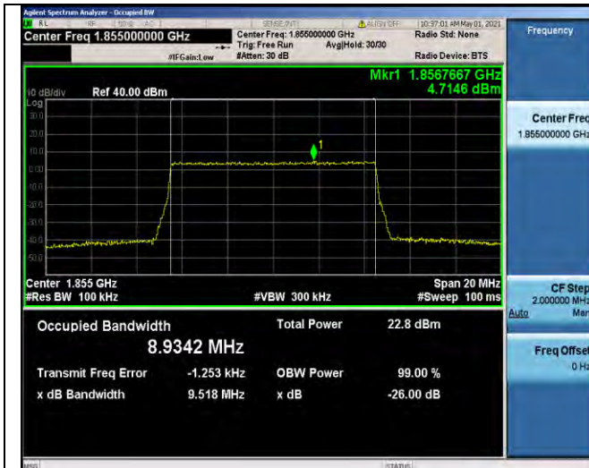
Band2-10MHz-16QAM-18650-50RB#0-8.9342
