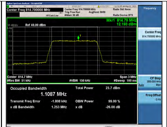
Band26-1.4MHz-QPSK-26697-6RB#0-1.1087
