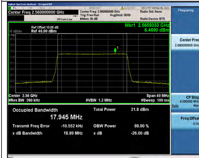
Band7-20MHz-16QAM-21350-100RB#0-17.945
