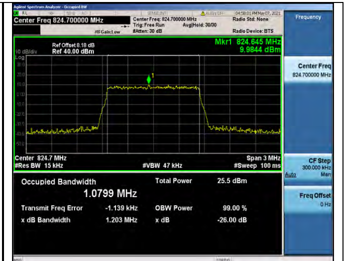
Band5-1.4MHz-QPSK-20407-6RB#0-1.0799
