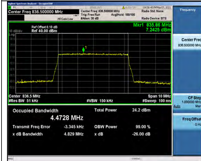
Band5-5MHz-16QAM-20525-25RB#0-4.4728
