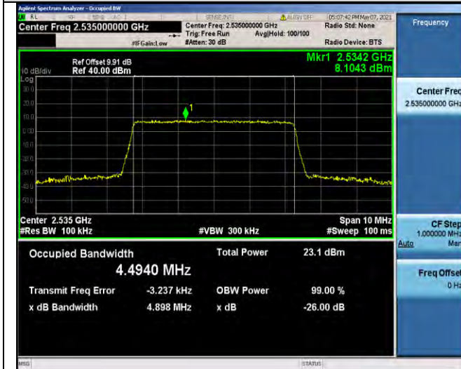
Band7-5MHz-16QAM-21100-25RB#0-4.4940
