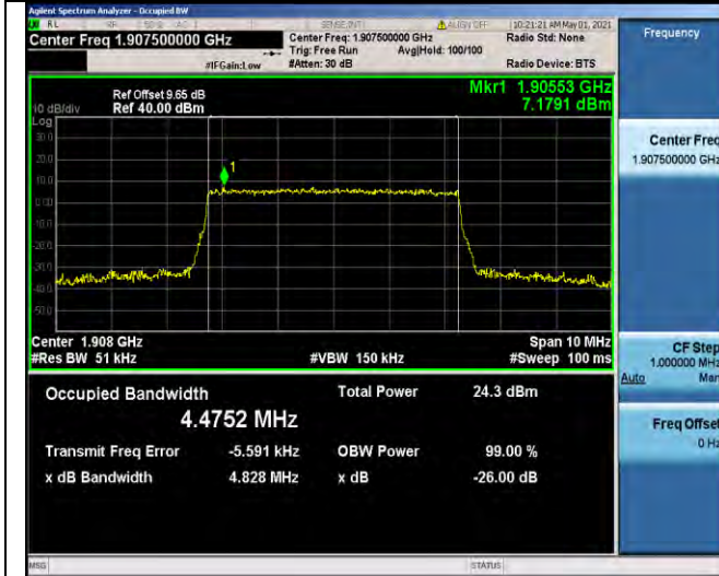
Band2-5MHz-16QAM-19175-25RB#0-4.4752
