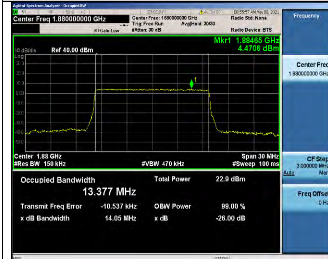
Band2-15MHz-16QAM-18900-75RB#0-13.377
