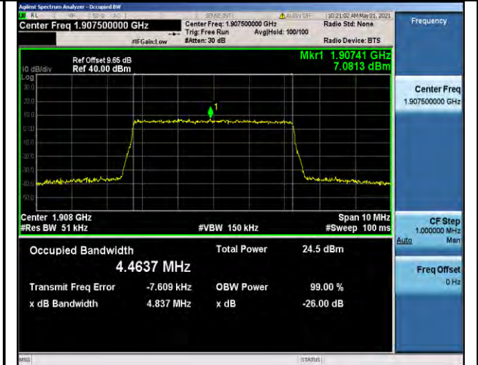
Band2-5MHz-QPSK-19175-25RB#0-4.4637
