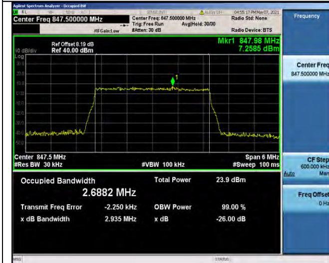
Band5-3MHz-16QAM-20635-15RB#0-2.6882
