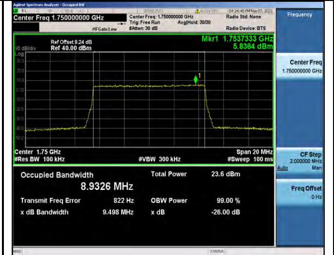
Band4-10MHz-QPSK-20350-50RB#0-8.9326
