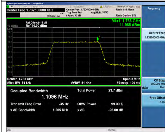
Band4-1.4MHz-16QAM-20175-6RB#0-1.1096
