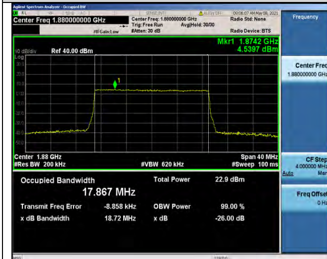
Band2-20MHz-16QAM-18900-100RB#0-17.867
