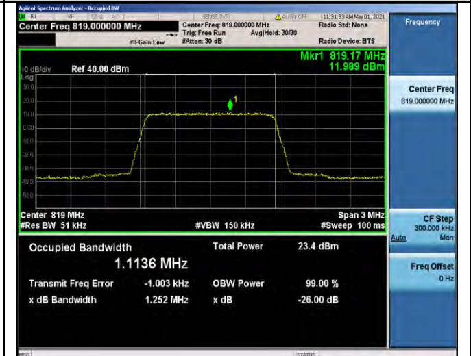
Band26-1.4MHz-QPSK-26740-6RB#0-1.1136
