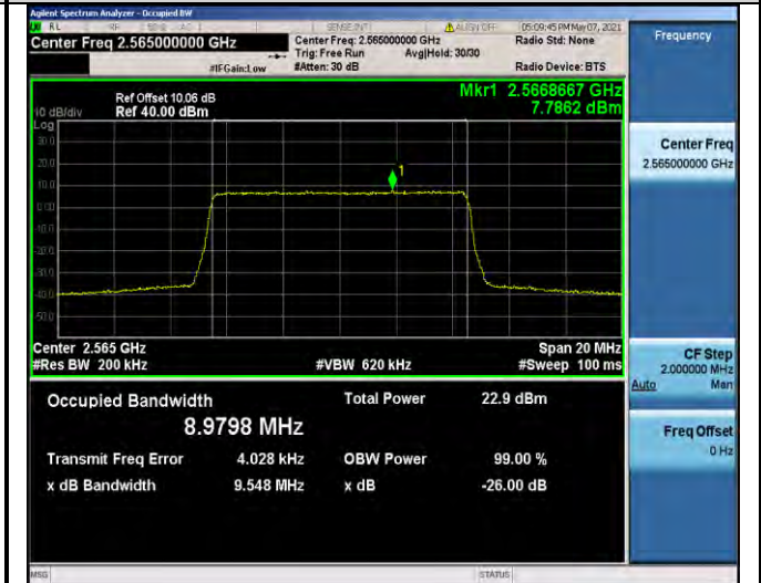
Band7-10MHz-QPSK-21400-50RB#0-8.9798
