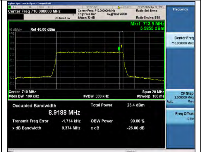
Band17-10MHz-QPSK-23790-50RB#0-8.9188
