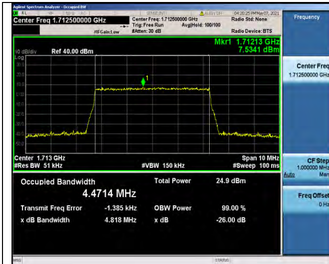
Band4-5MHz-16QAM-19975-25RB#0-4.4714
