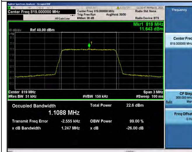
Band26-1.4MHz-16QAM-26740-6RB#0-1.1088
