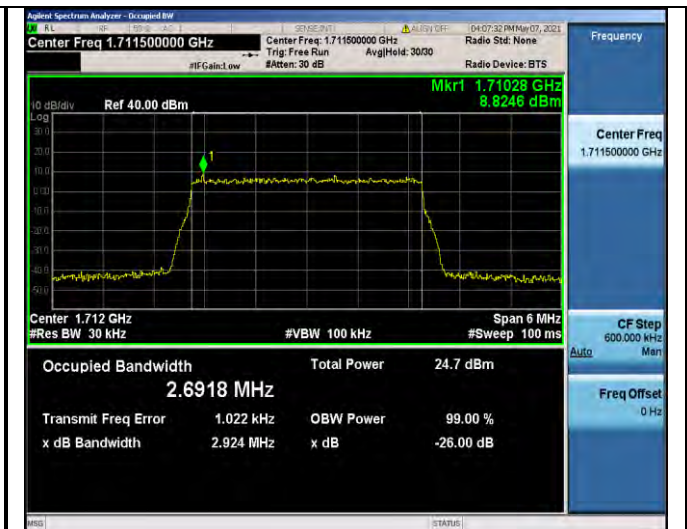
Band4-3MHz-QPSK-19965-15RB#0-2.6918
