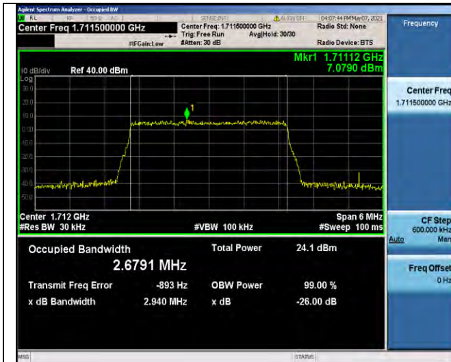
Band4-3MHz-16QAM-19965-15RB#0-2.6791
