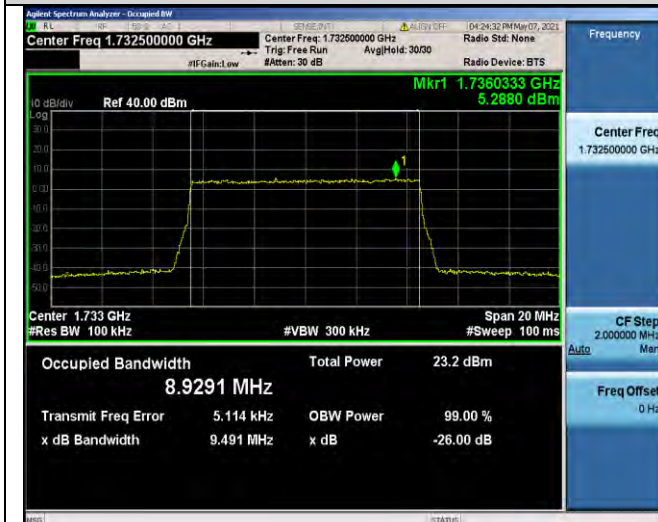
Band4-10MHz-16QAM-20175-50RB#0-8.9291
