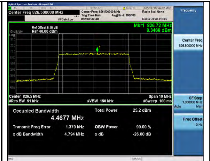
Band5-5MHz-QPSK-20425-25RB#0-4.4677
