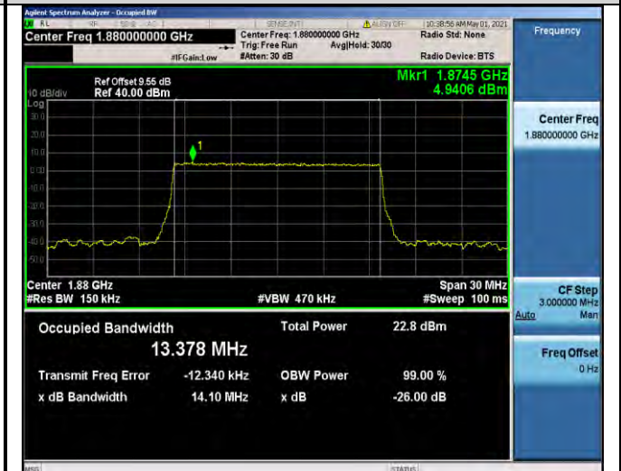
Band2-15MHz-QPSK-18900-75RB#0-13.378
