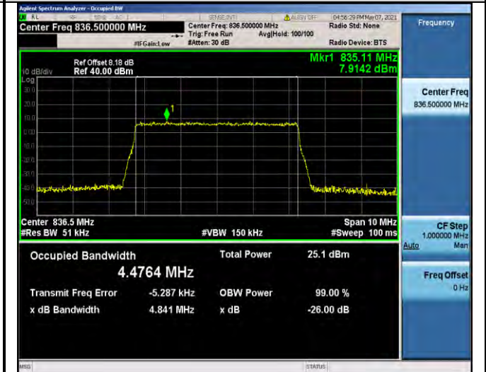
Band5-5MHz-QPSK-20525-25RB#0-4.4764
