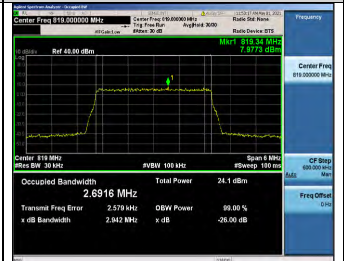
Band26-3MHz-QPSK-26740-15RB#0-2.6916
