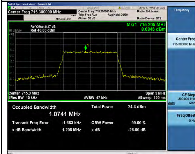
Band12-1.4MHz-16QAM-23173-6RB#0-1.0741
