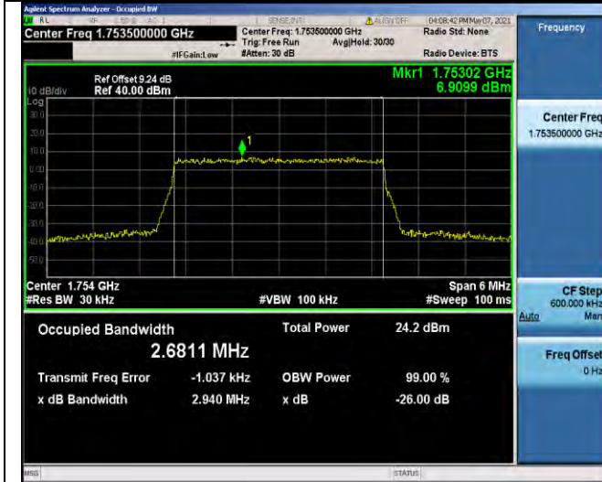
Band4-3MHz-16QAM-20385-15RB#0-2.6811
