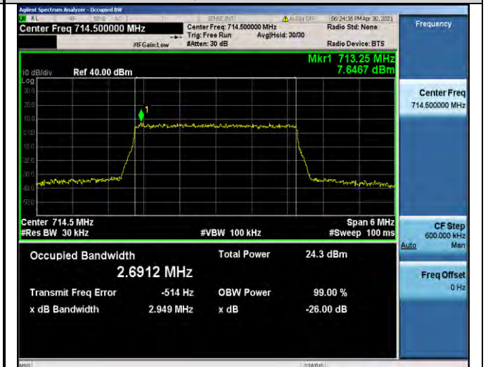
Band12-3MHz-QPSK-23165-15RB#0-2.6912
