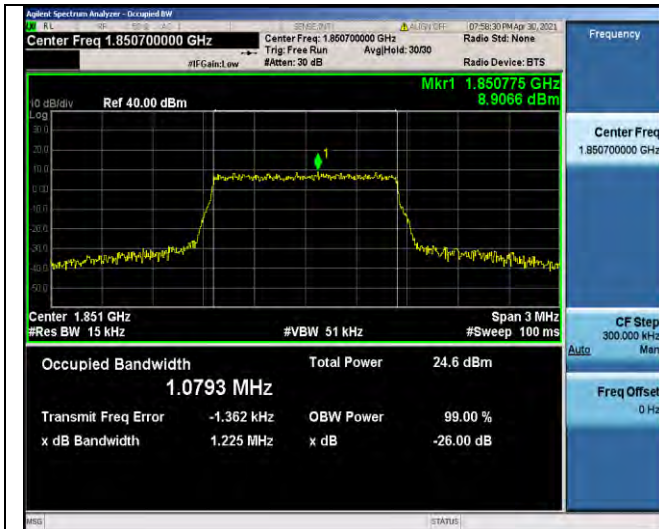
Band2-1.4MHz-16QAM-18607-6RB#0-1.0793
