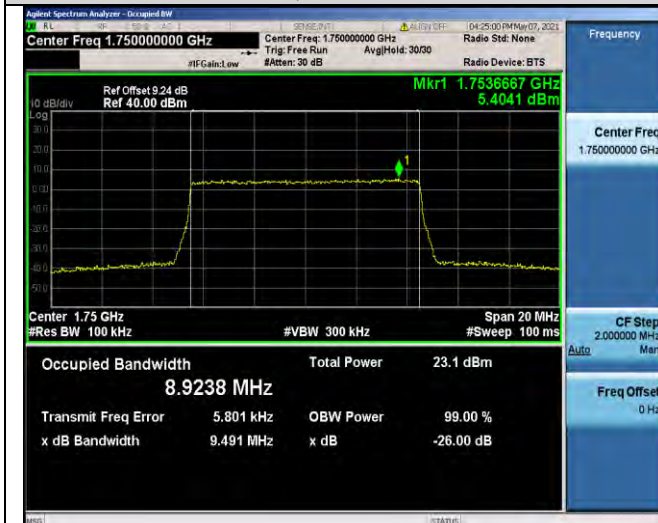
Band4-10MHz-16QAM-20350-50RB#0-8.9238
