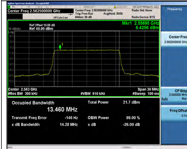
Band7-15MHz-16QAM-21375-75RB#0-13.460
