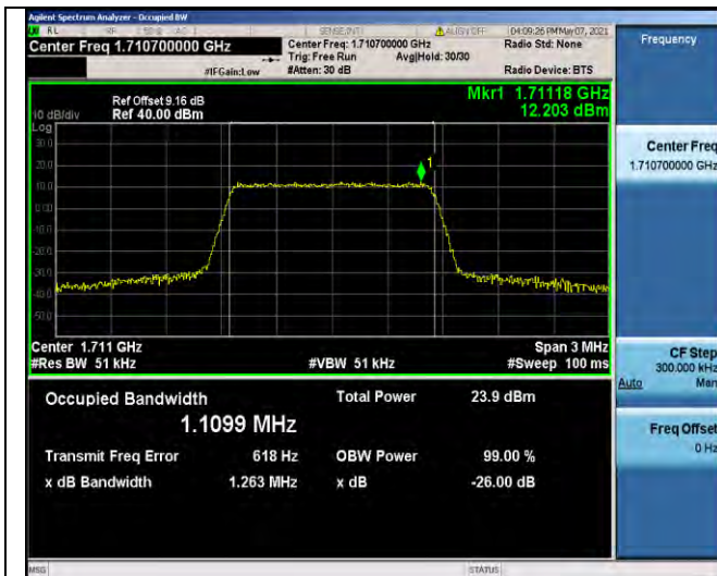
Band4-1.4MHz-16QAM-19957-6RB#0-1.1099
