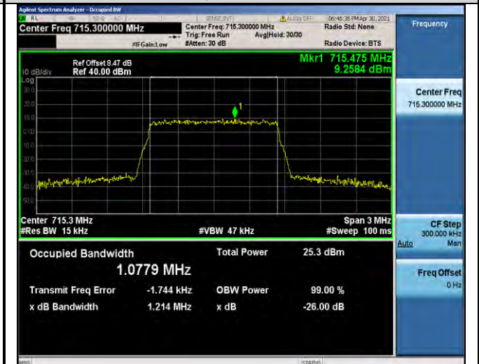
Band12-1.4MHz-QPSK-23173-6RB#0-1.0779
