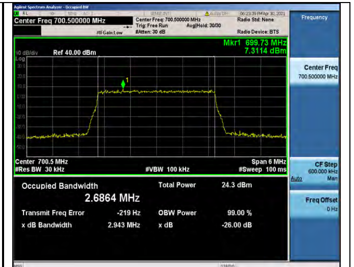
Band12-3MHz-QPSK-23025-15RB#0-2.6864
