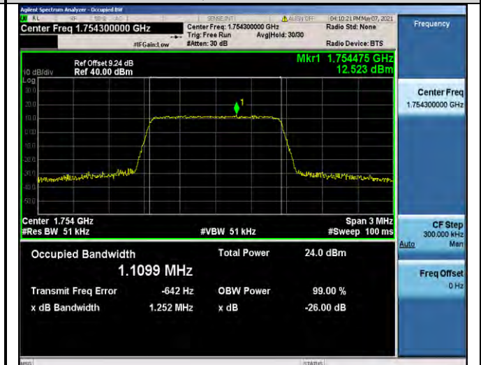
Band4-1.4MHz-QPSK-20393-6RB#0-1.1099
