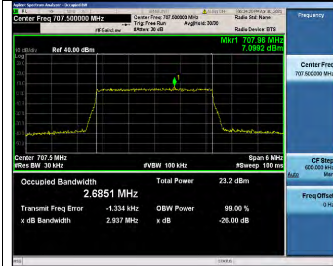
Band12-3MHz-16QAM-23095-15RB#0-2.6851
