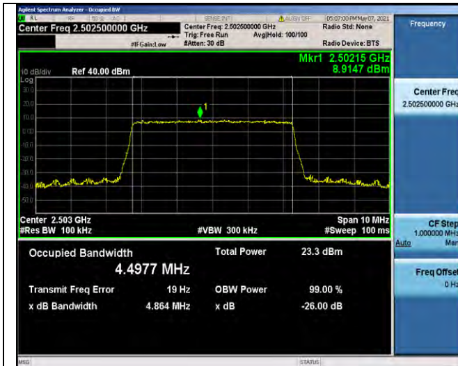
Band7-5MHz-16QAM-20775-25RB#0-4.4977
