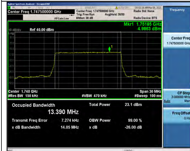
Band4-15MHz-16QAM-20325-75RB#0-13.390
