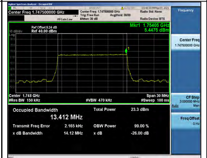
Band4-15MHz-QPSK-20325-75RB#0-13.412
