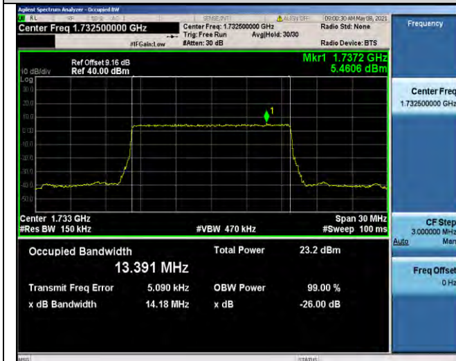
Band4-15MHz-16QAM-20175-75RB#0-13.391
