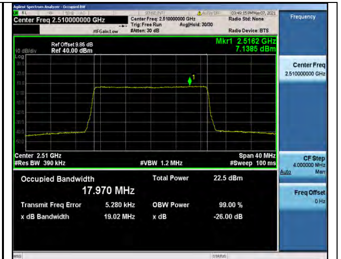
Band7-20MHz-QPSK-20850-100RB#0-17.970
