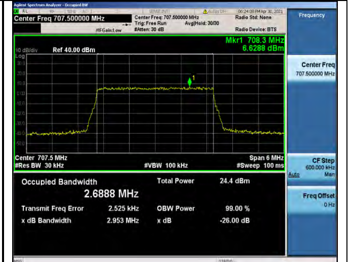
Band12-3MHz-QPSK-23095-15RB#0-2.6888
