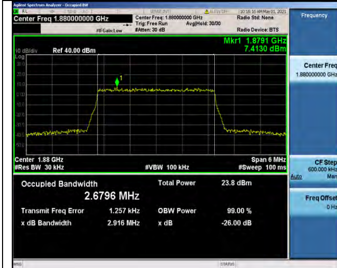
Band2-3MHz-16QAM-18900-15RB#0-2.6796
