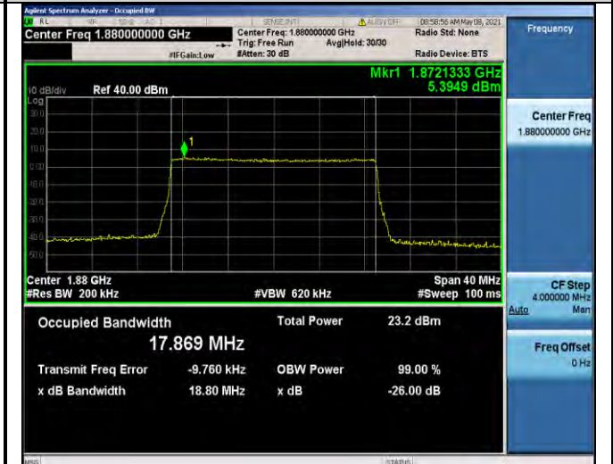
Band2-20MHz-QPSK-18900-100RB#0-17.869
