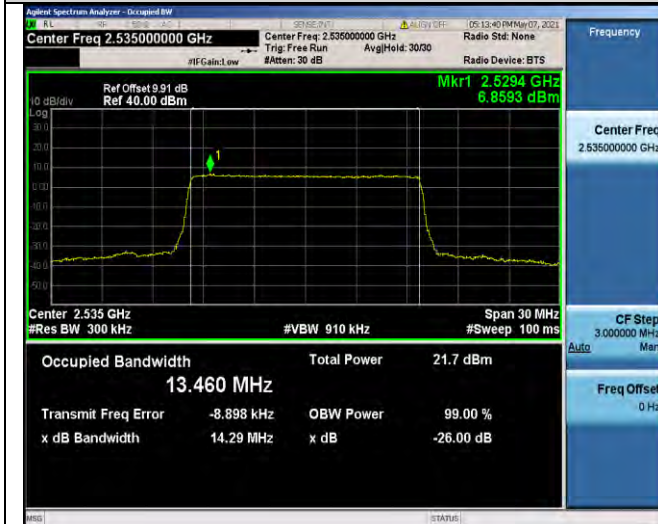
Band7-15MHz-16QAM-21100-75RB#0-13.460
