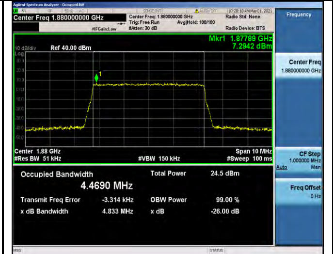
Band2-5MHz-QPSK-18900-25RB#0-4.4690
