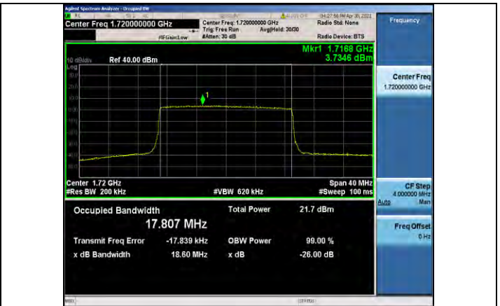
Band66-20MHz-16QAM-132072-100RB#0-17.807
