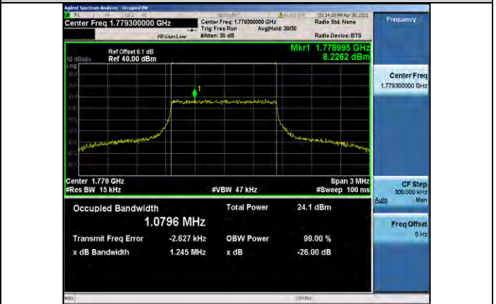
Band66-1.4MHz-16QAM-132665-6RB#0-1.0796
