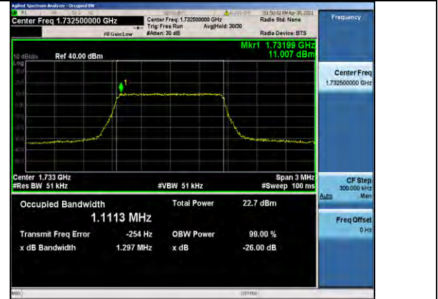
Band4-1.4MHz-16QAM-20175-6RB#0-1.1113
