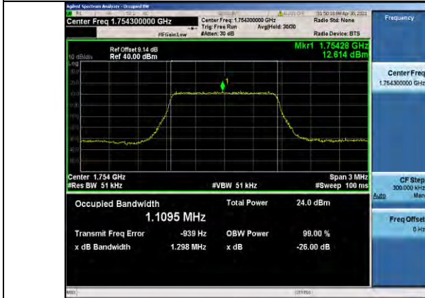
Band4-1.4MHz-QPSK-20393-6RB#0-1.1095
