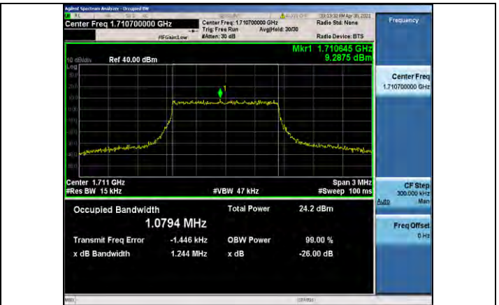
Band66-1.4MHz-16QAM-131979-6RB#0-1.0794
