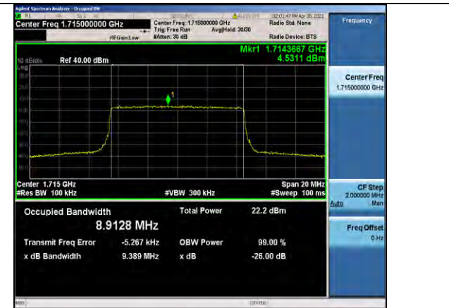
Band4-10MHz-16QAM-20000-50RB#0-8.9128
