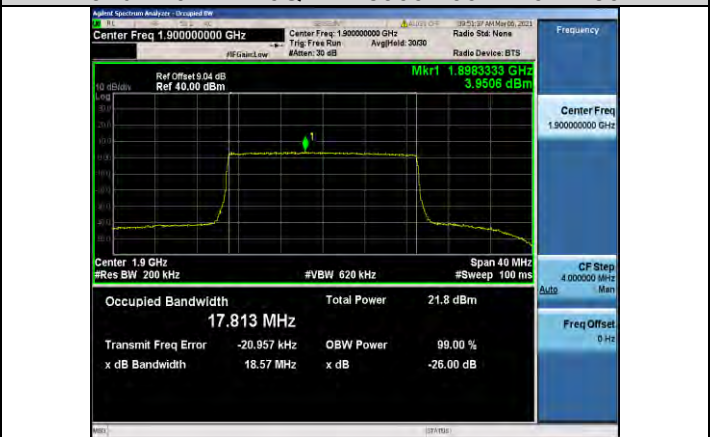
Band2-20MHz-16QAM-19100-100RB#0-17.813
