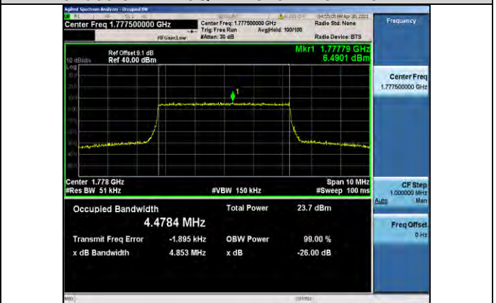
Band66-5MHz-16QAM-132647-25RB#0-4.4784
