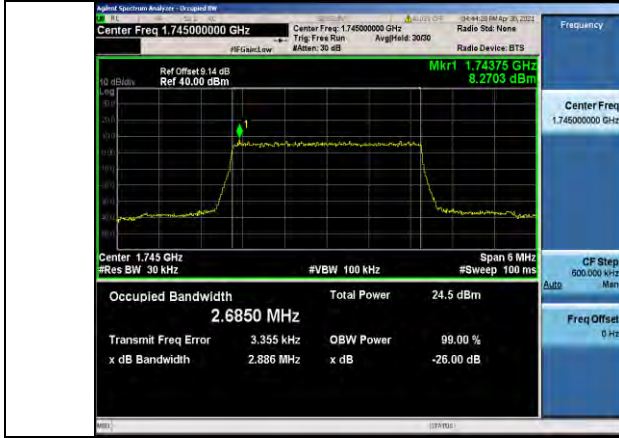
Band66-3MHz-QPSK-132322-15RB#0-2.6850
