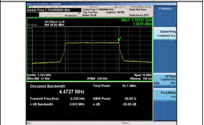
Band66-5MHz-16QAM-132322-25RB#0-4.4727
