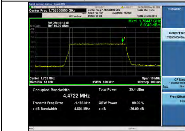
Band4-5MHz-QPSK-20375-25RB#0-4.4722
