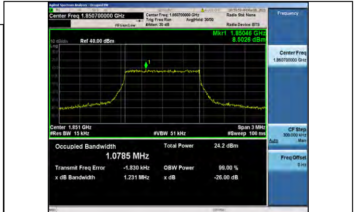
Band2-1.4MHz-16QAM-18607-6RB#0-1.0785
