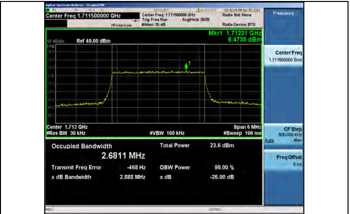
Band4-3MHz-16QAM-19965-15RB#0-2.6811
