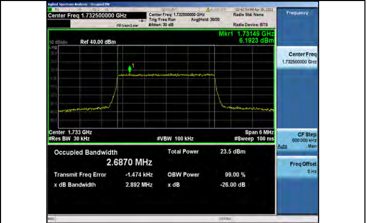
Band4-3MHz-16QAM-20175-15RB#0-2.6870
