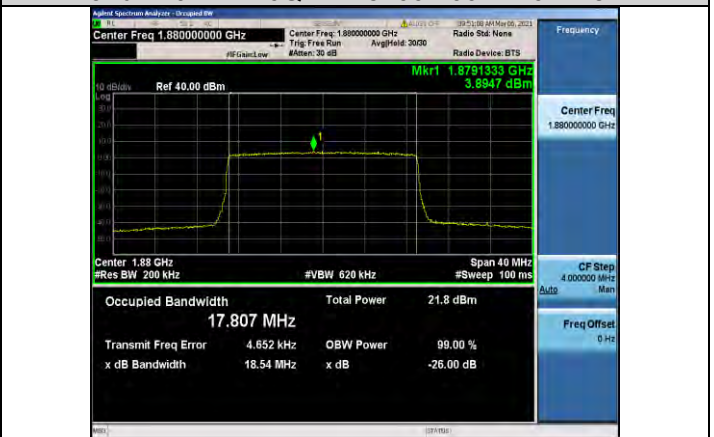
Band2-20MHz-16QAM-18900-100RB#0-17.807
