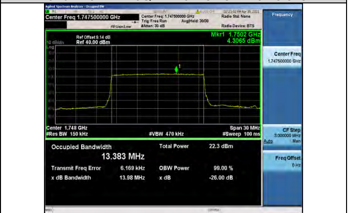
Band4-15MHz-16QAM-20325-75RB#0-13.383
