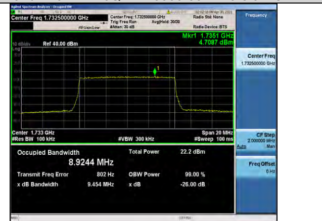
Band4-10MHz-16QAM-20175-50RB#0-8.9244
