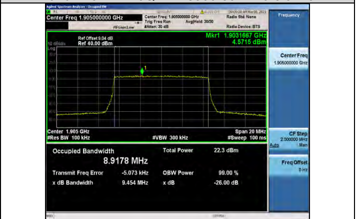
Band2-10MHz-16QAM-19150-50RB#0-8.9178
