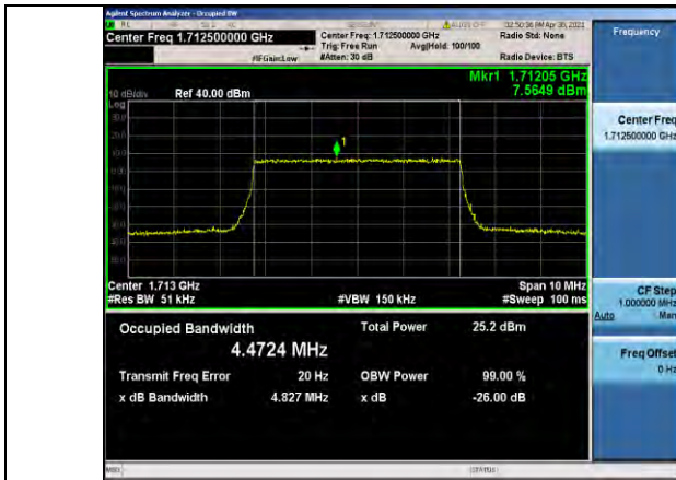
Band4-5MHz-QPSK-19975-25RB#0-4.4724
