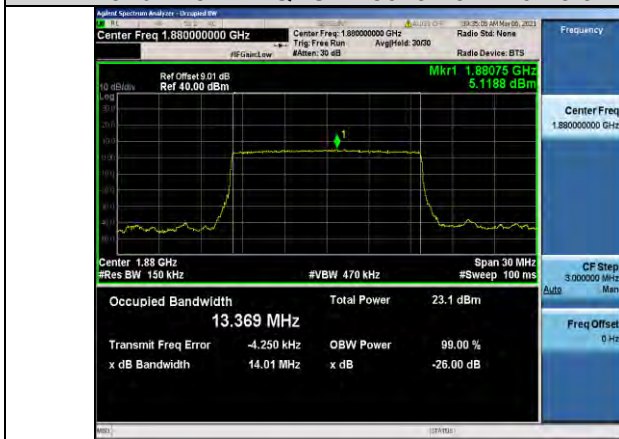
Band2-15MHz-QPSK-18900-75RB#0-13.369
