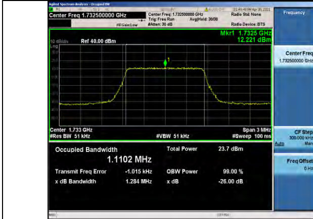
Band4-1.4MHz-QPSK-20175-6RB#0-1.1102
