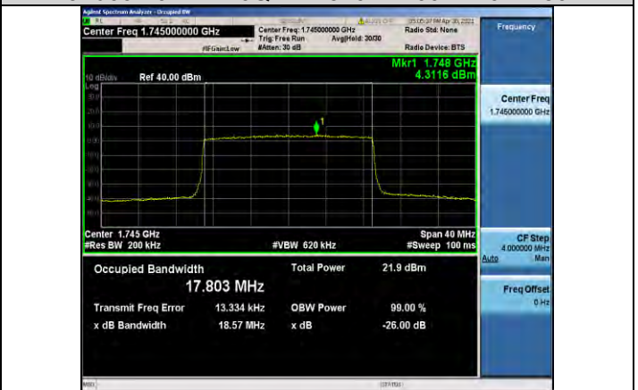
Band66-20MHz-16QAM-132322-100RB#0-17.803
