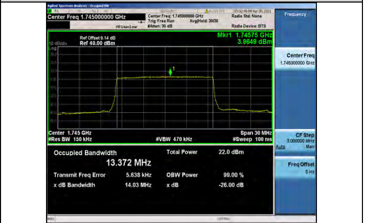
Band66-15MHz-16QAM-132322-75RB#0-13.372
