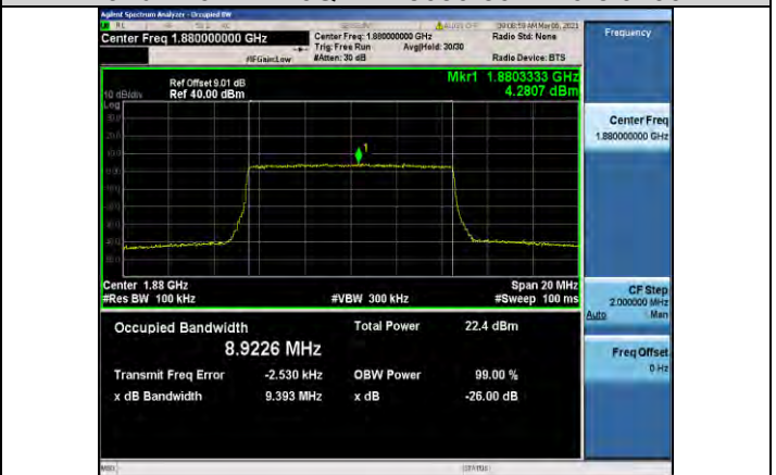
Band2-10MHz-16QAM-18900-50RB#0-8.9226
