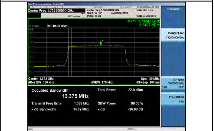
Band4-15MHz-16QAM-20175-75RB#0-13.375
