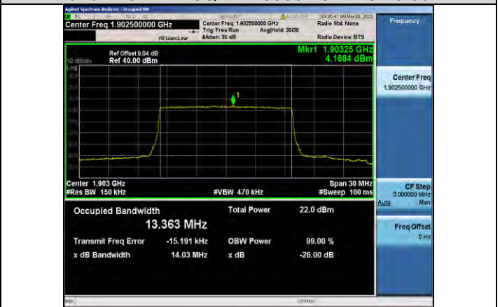
Band2-15MHz-16QAM-19125-75RB#0-13.363
