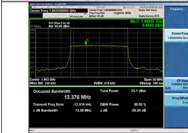
Band2-15MHz-QPSK-19125-75RB#0-13.376
