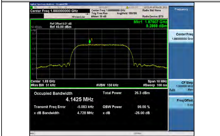
Band2-9400
