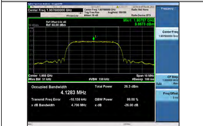
Band2-9538
