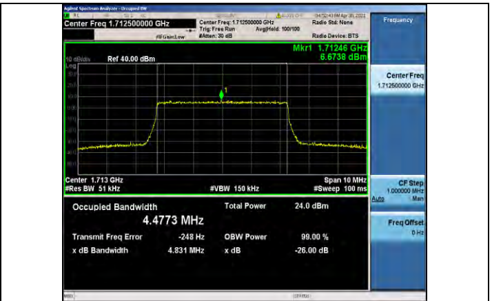
Band66-5MHz-16QAM-131997-25RB#0-4.4773
