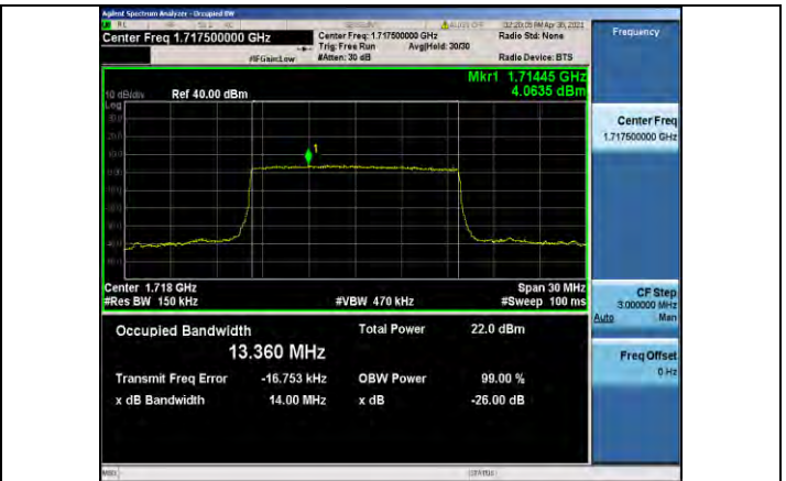
Band4-15MHz-16QAM-20025-75RB#0-13.360
