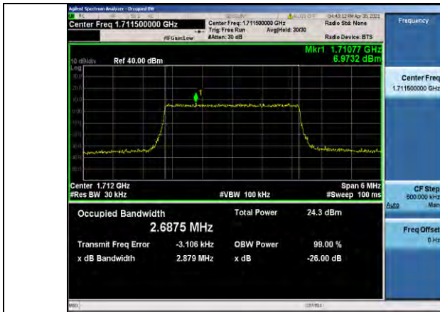
Band66-3MHz-QPSK-131987-15RB#0-2.6875
