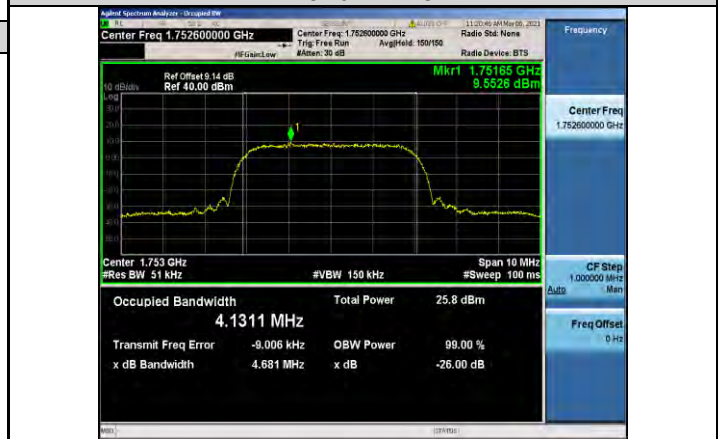
Band4-1513
