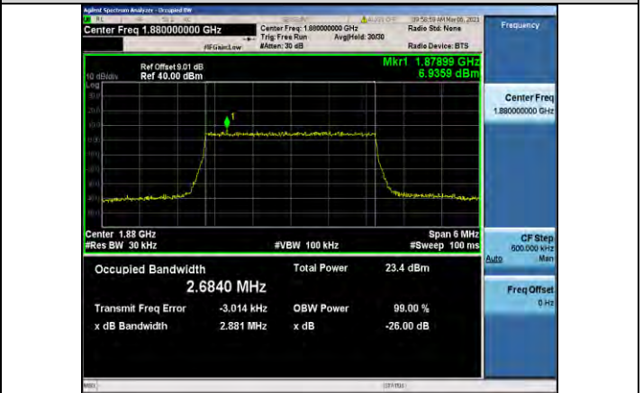
Band2-3MHz-16QAM-18900-15RB#0-2.6840
