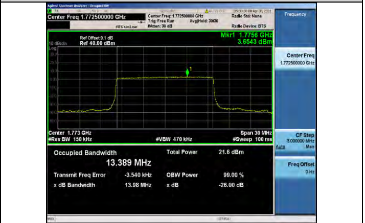
Band66-15MHz-16QAM-132597-75RB#0-13.389
