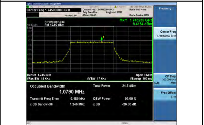
Band66-1.4MHz-16QAM-132322-6RB#0-1.0790
