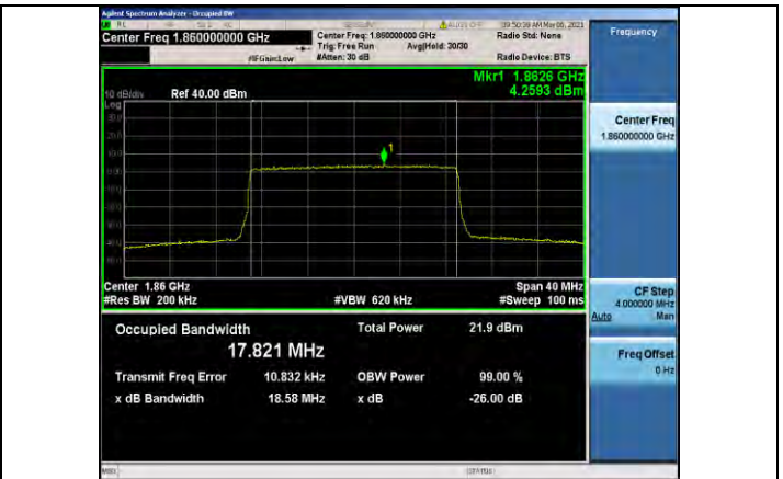
Band2-20MHz-16QAM-18700-100RB#0-17.821
