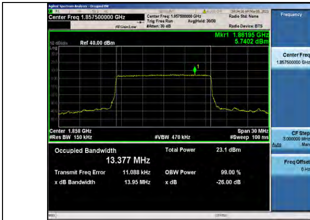
Band2-15MHz-QPSK-18675-75RB#0-13.377
