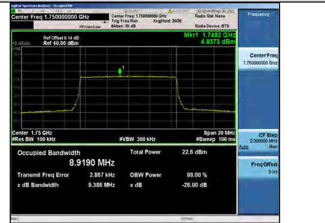
Band4-10MHz-16QAM-20350-50RB#0-8.9190
