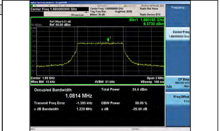
Band2-1.4MHz-16QAM-18900-6RB#0-1.0814
