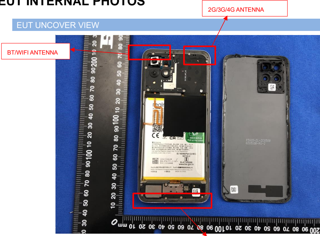
2G/3G/4G Dev ANTENNA
