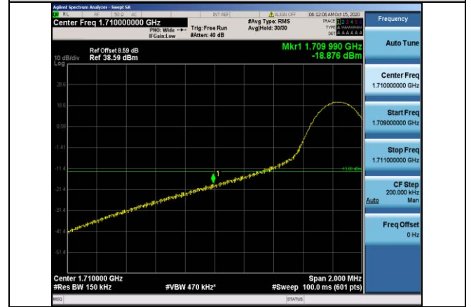
Band66-15MHz-16QAM-132047-1RB#0
