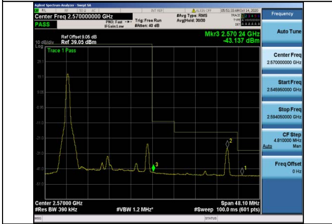
Band7-20MHz-16QAM-21350-1RB#0
