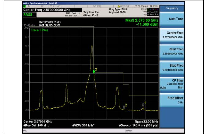
Band7-5MHz-16QAM-21425-1RB#24
