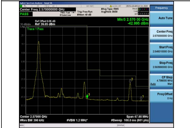
Band7-20MHz-QPSK-21350-1RB#0
