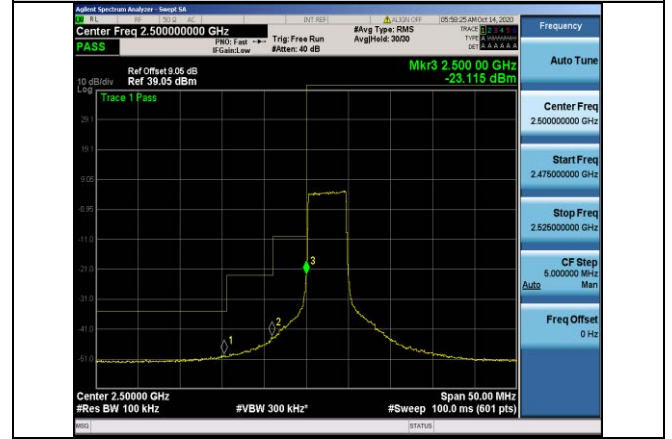
Band7-5MHz-16QAM-20775-25RB#0
