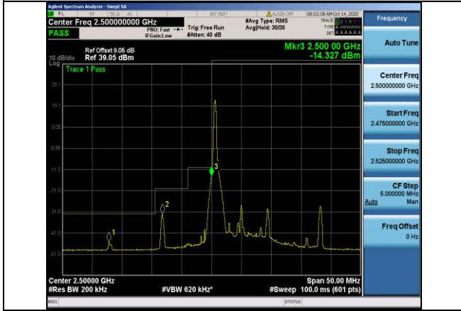
Band7-10MHz-QPSK-20800-1RB#0
