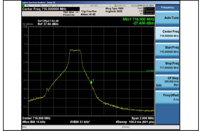
Band12-1.4MHz-16QAM-23173-1RB#5
