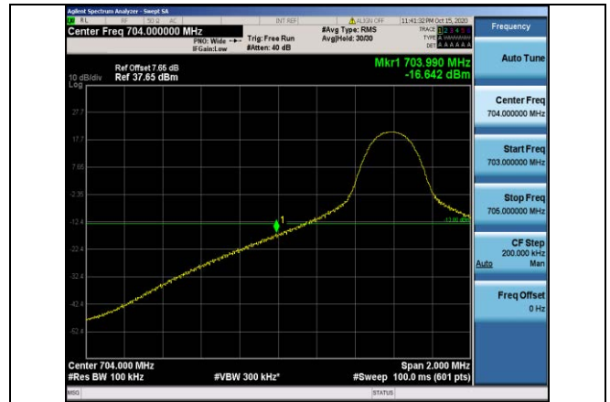
Band17-10MHz-QPSK-23780-1RB#0
