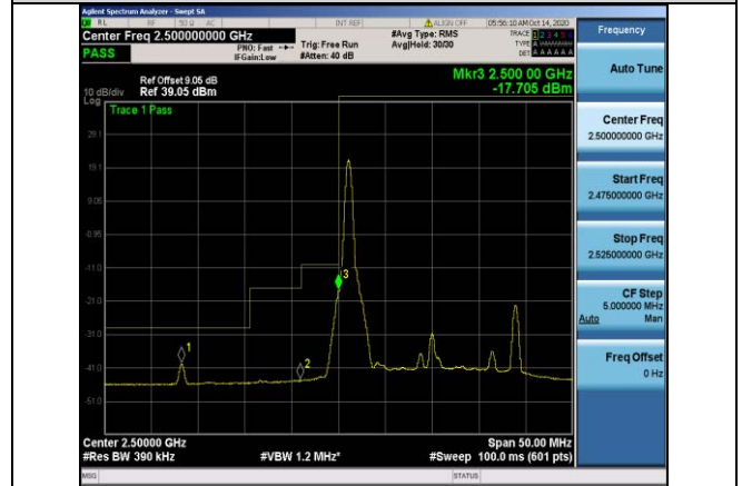
Band7-20MHz-16QAM-20850-1RB#0
