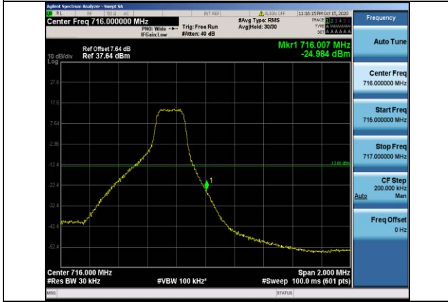
Band12-3MHz-16QAM-23165-1RB#14
