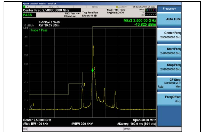
Band7-5MHz-16QAM-20775-1RB#0
