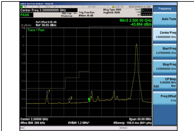
Band7-20MHz-16QAM-20850-1RB#99
