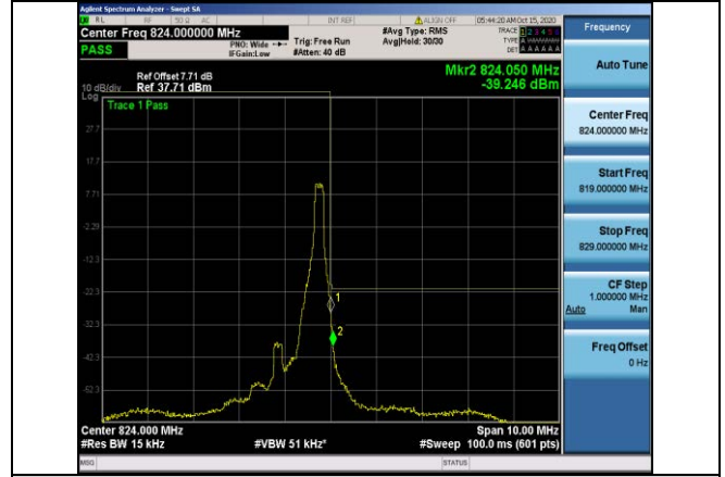
Band26-1.4MHz-16QAM-26783-1RB#5
