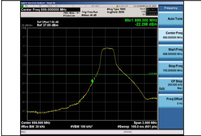
Band12-3MHz-QPSK-23025-1RB#0
