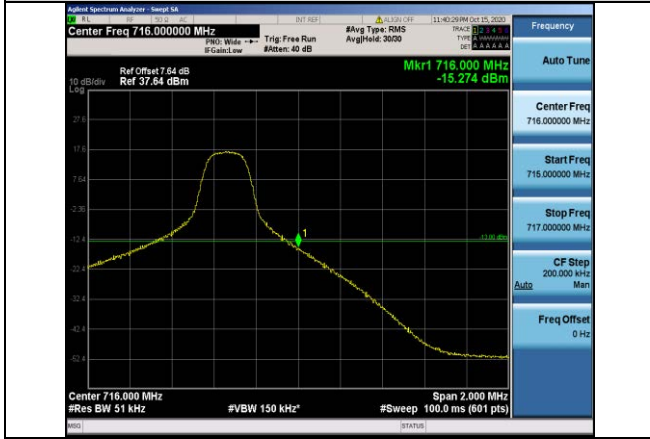
Band17-5MHz-16QAM-23825-1RB#24
