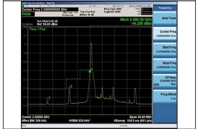
Band7-10MHz-16QAM-20800-1RB#0
