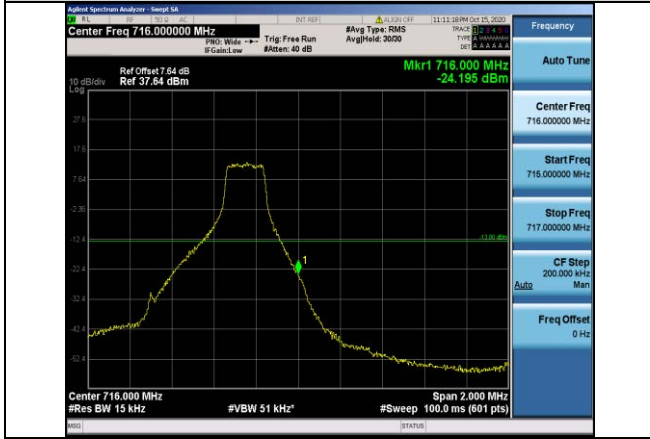
Band12-1.4MHz-QPSK-23173-1RB#5
