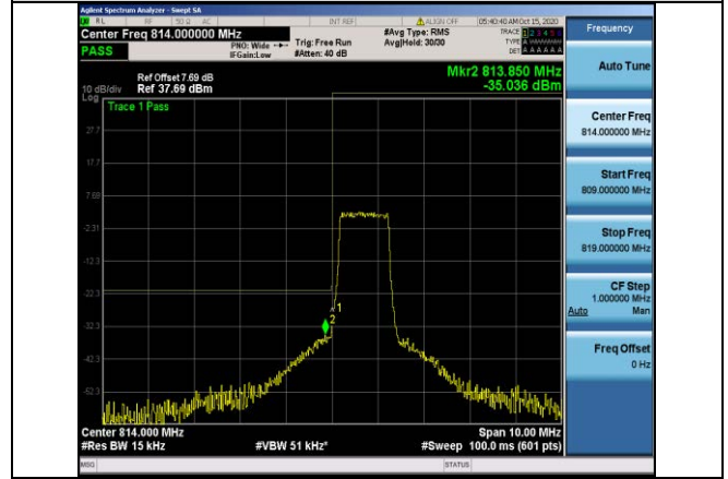
Band26-1.4MHz-16QAM-26697-6RB#0
