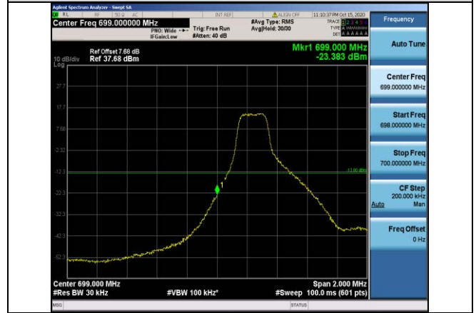
Band12-3MHz-16QAM-23025-1RB#0
