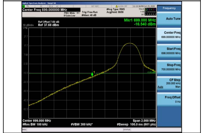
Band12-10MHz-QPSK-23060-1RB#0
