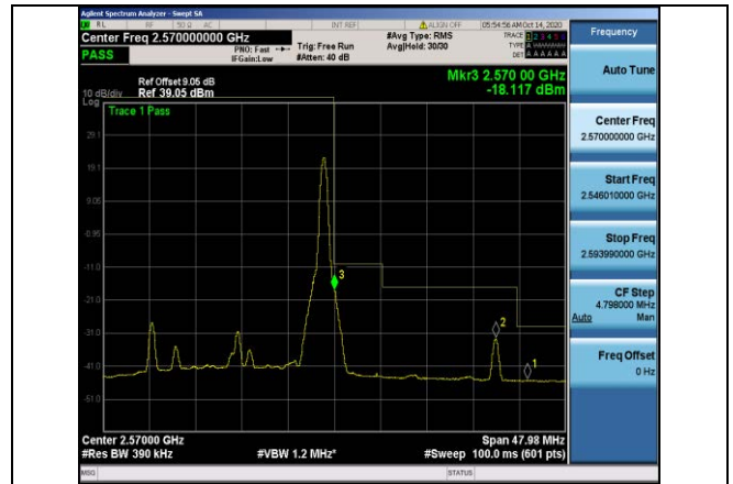
Band7-20MHz-QPSK-21350-1RB#99
