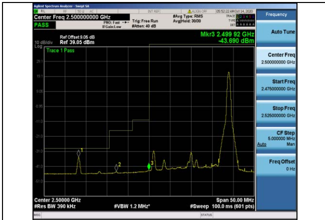
Band7-20MHz-QPSK-20850-1RB#99
