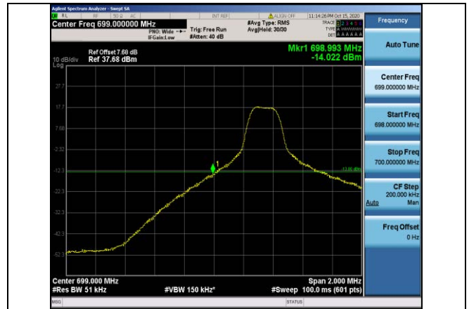
Band12-5MHz-QPSK-23035-1RB#0
