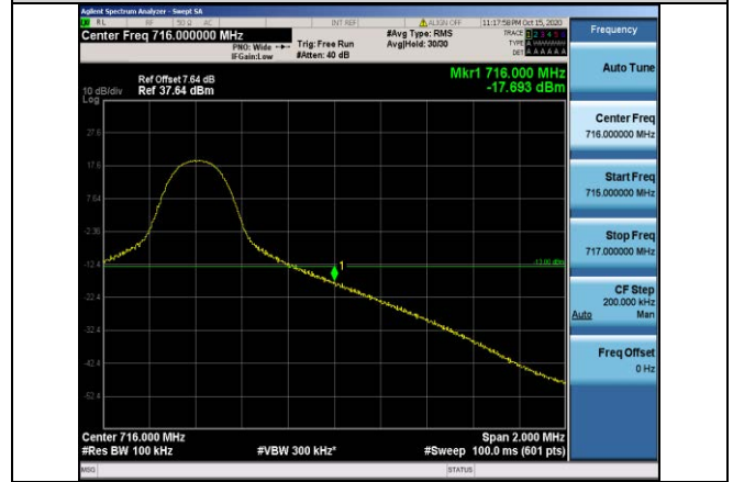
Band12-10MHz-16QAM-23130-1RB#49
