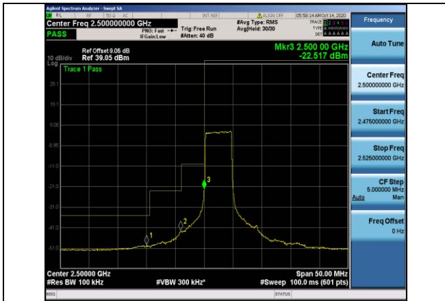
Band7-5MHz-QPSK-20775-25RB#0
