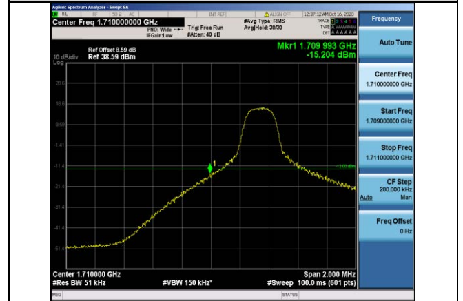
Band4-5MHz-16QAM-19975-1RB#0
