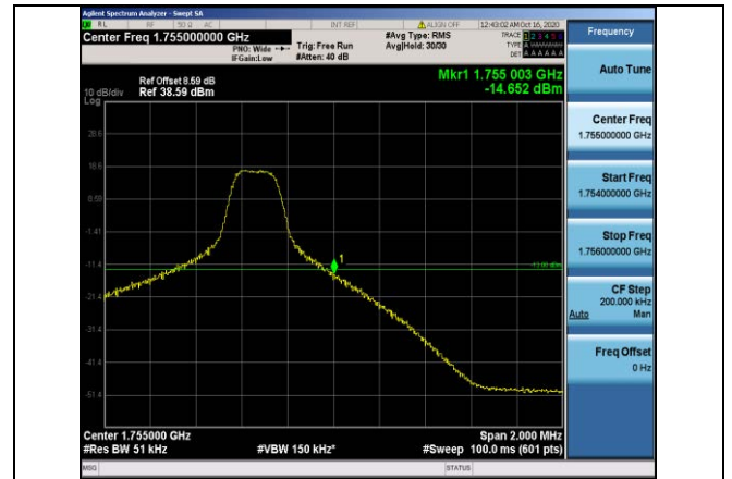
Band4-5MHz-QPSK-20375-1RB#24
