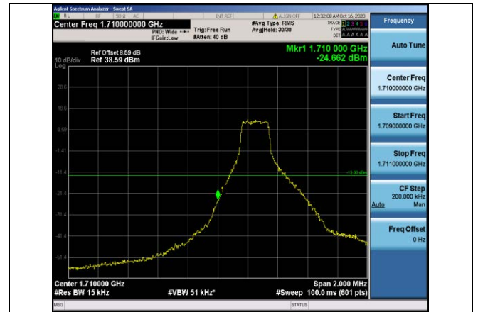
Band4-1.4MHz-QPSK-19957-1RB#0
