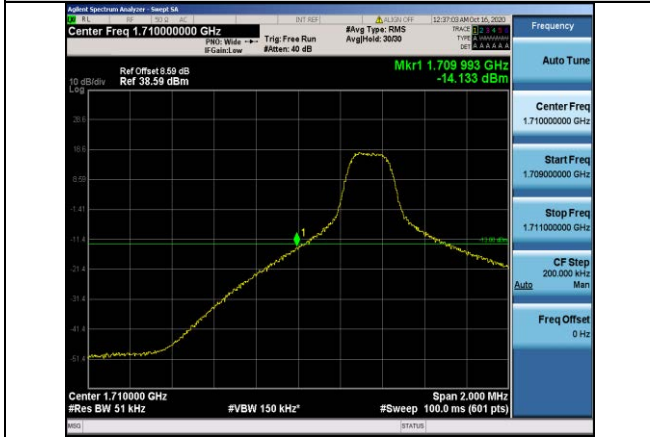
Band4-5MHz-QPSK-19975-1RB#0
