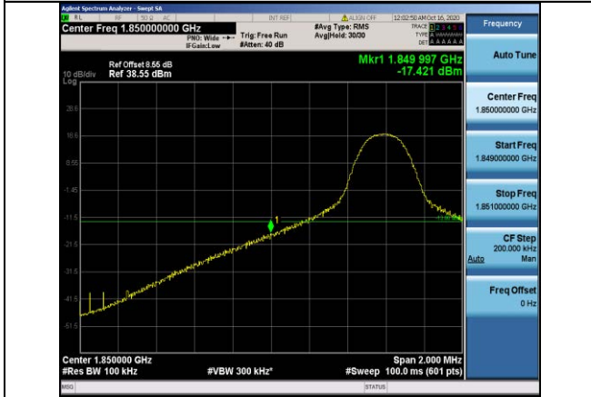
Band2-10MHz-16QAM-18650-1RB#0
