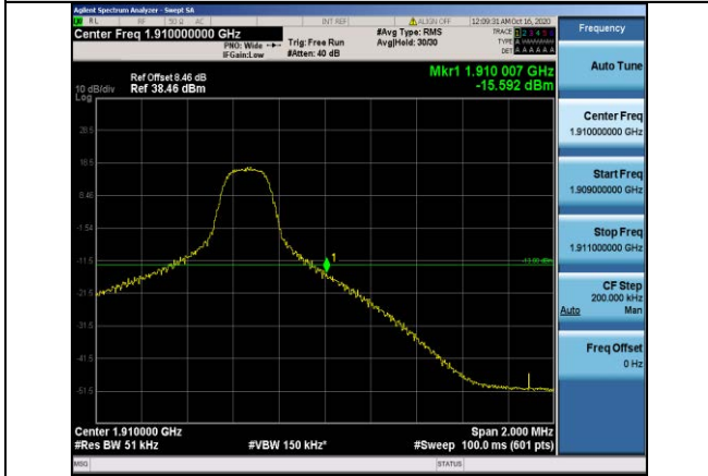
Band2-5MHz-16QAM-19175-1RB#24
