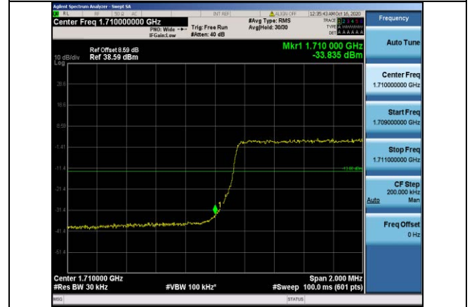
Band4-3MHz-16QAM-19965-15RB#0
