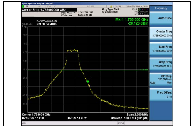
Band4-1.4MHz-16QAM-20393-1RB#5
