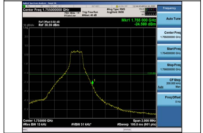
Band4-1.4MHz-QPSK-20393-1RB#5
