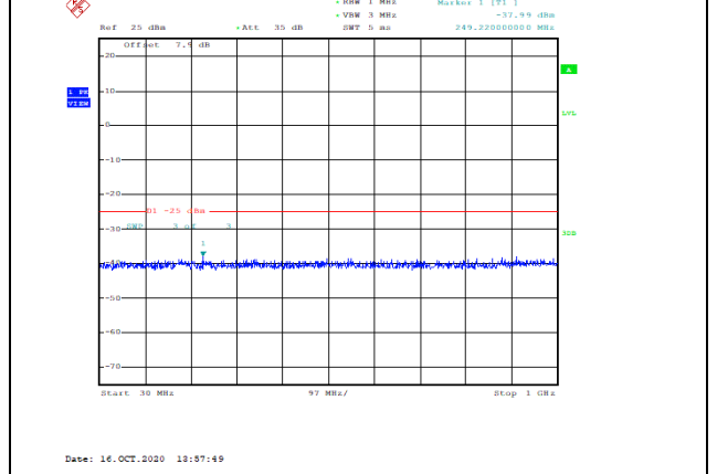
Band41-5MHz-16QAM-41215-1RB#0-Range1:30~1000MHz--37.99-PASS
