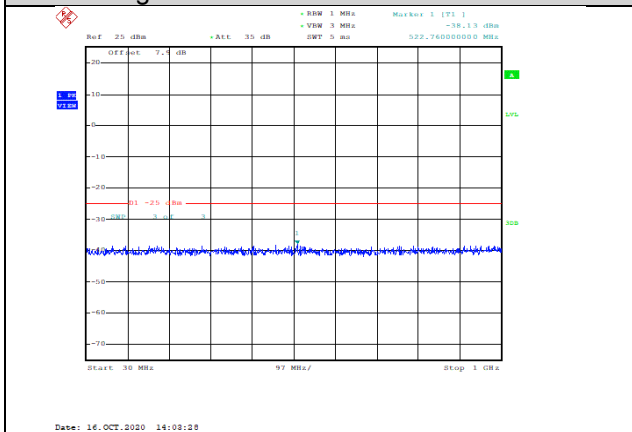
Band41-15MHz-QPSK-40115-1RB#0-Range1:30~1000MHz--38.13-PASS
