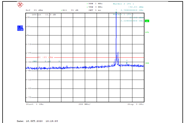
Band7-20MHz-16QAM-21100-1RB#0-Range2:1000~3000MHz--32.05-PASS
