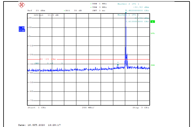
Band38-10MHz-QPSK-38200-1RB#0-Range2:1000~3000MHz--31.92-PASS
