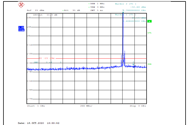
Band38-15MHz-QPSK-38175-1RB#0-Range2:1000~3000MHz--32.48-PASS
