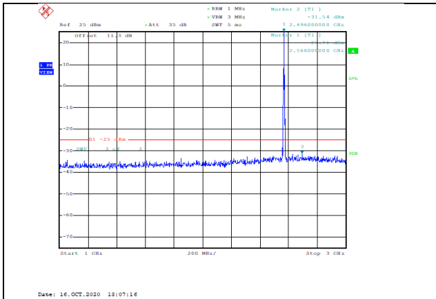
Band7-5MHz-16QAM-21425-1RB#0-Range2:1000~3000MHz--31.54-PASS
