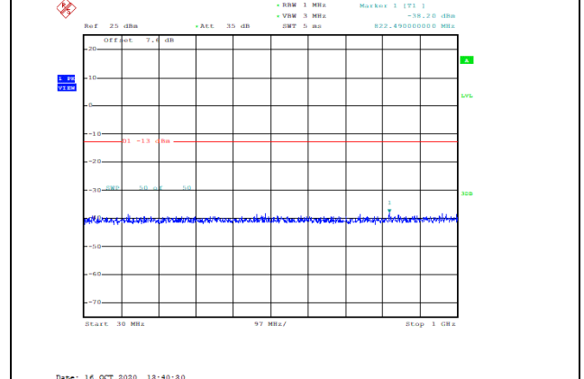
Band66-1.4MHz-QPSK-132322-1RB#0-Range1:30~1000MHz--38.2-PASS
