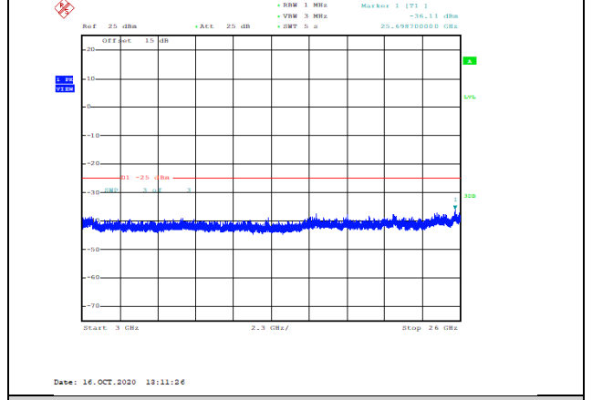
Band7-10MHz-QPSK-21400-1RB#0-Range3:3000~26000MHz--36.11-PASS
