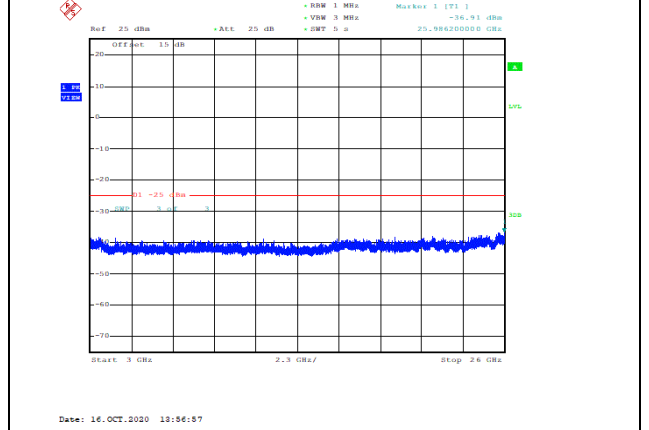
Band41-5MHz-16QAM-40590-1RB#0-Range3:3000~26000MHz--36.91-PASS
