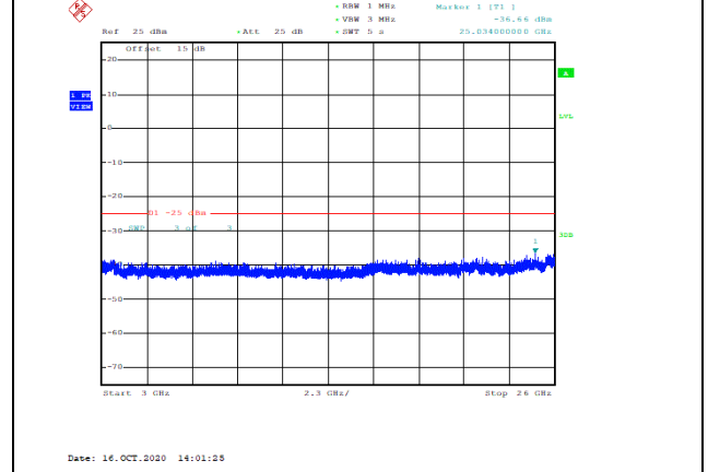
Band41-10MHz-16QAM-40590-1RB#0-Range3:3000~26000MHz--36.66-PASS
