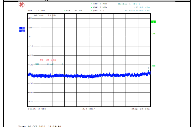
Band38-10MHz-QPSK-38200-1RB#0-Range3:3000~26000MHz--37-PASS
