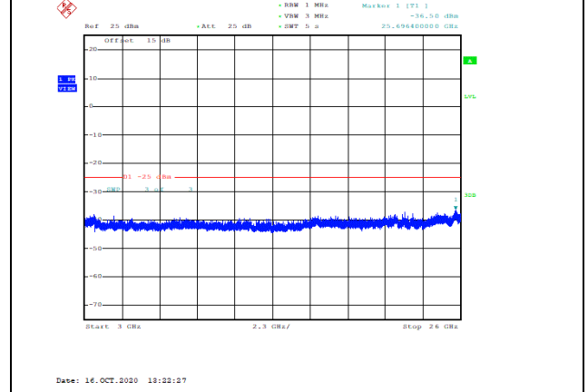
Band38-5MHz-QPSK-37775-1RB#0-Range3:3000~26000MHz--36.5-PASS
