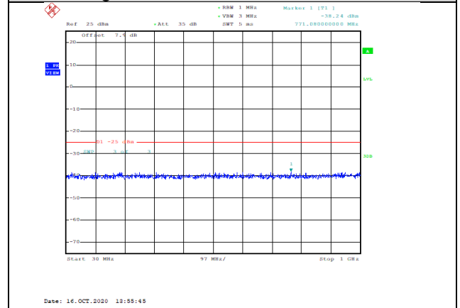
Band41-5MHz-QPSK-40590-1RB#0-Range1:30~1000MHz--38.24-PASS
