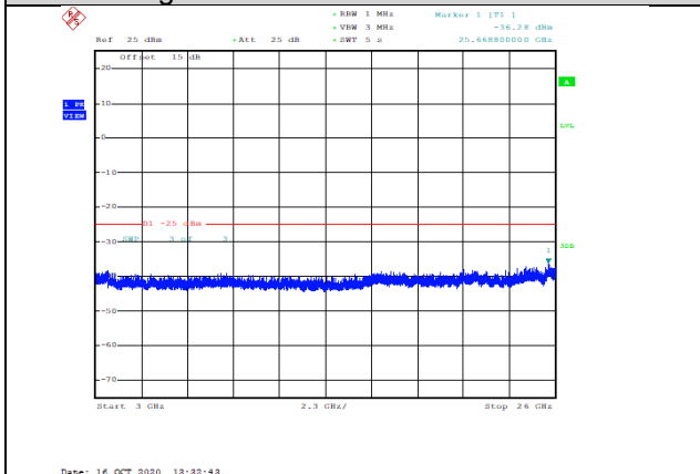
Band38-15MHz-QPSK-38000-1RB#0-Range3:3000~26000MHz--36.28-PASS
