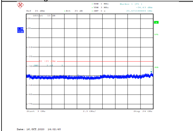
Band41-10MHz-16QAM-41190-1RB#0-Range3:3000~26000MHz--36.63-PASS
