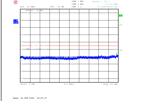
Band38-20MHz-QPSK-38000-1RB#0-Range3:3000~26000MHz--37-PASS
