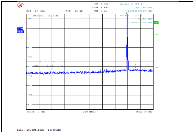
Band41-10MHz-QPSK-40590-1RB#0-Range2:1000~3000MHz--31.8-PASS
