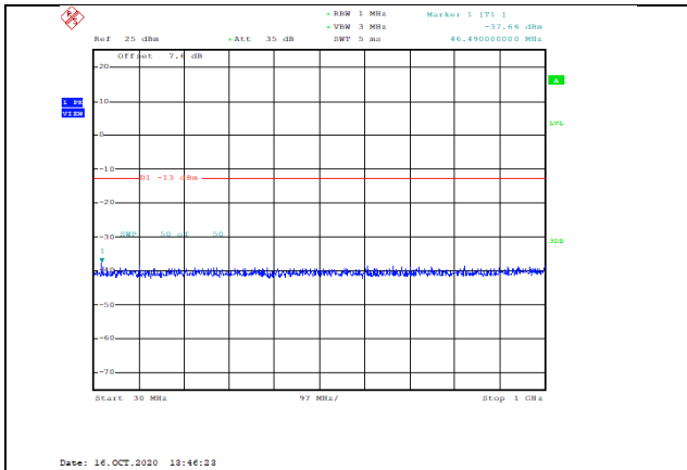
Band66-5MHz-QPSK-132647-1RB#0-Range1:30~1000MHz--37.66-PASS
