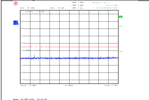
Band7-15MHz-QPSK-20825-1RB#0-Range1:30~1000MHz--38.16-PASS
