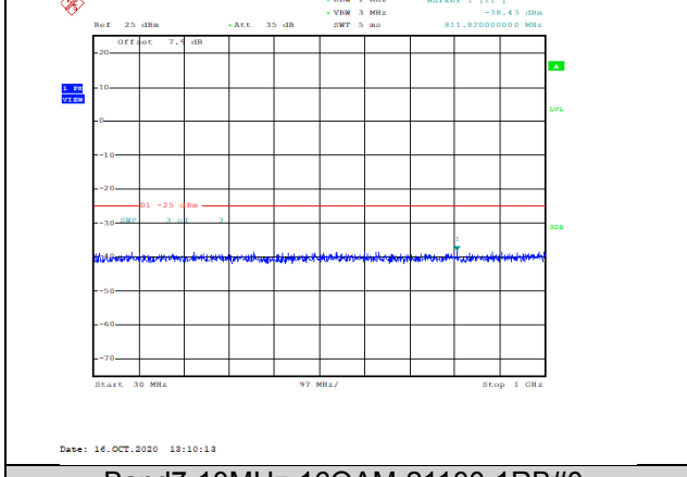
Band7-10MHz-16QAM-21100-1RB#0-Range1:30~1000MHz--38.43-PASS
