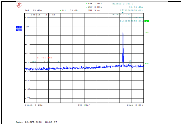
Band41-5MHz-16QAM-41215-1RB#0-Range2:1000~3000MHz--31.86-PASS
