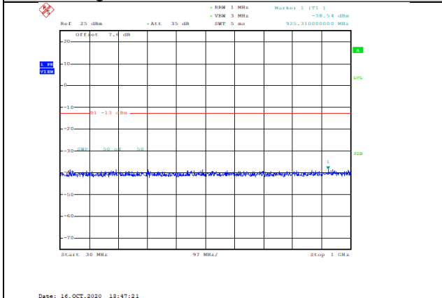
Band66-10MHz-QPSK-132322-1RB#0-Range1:30~1000MHz--38.54-PASS
