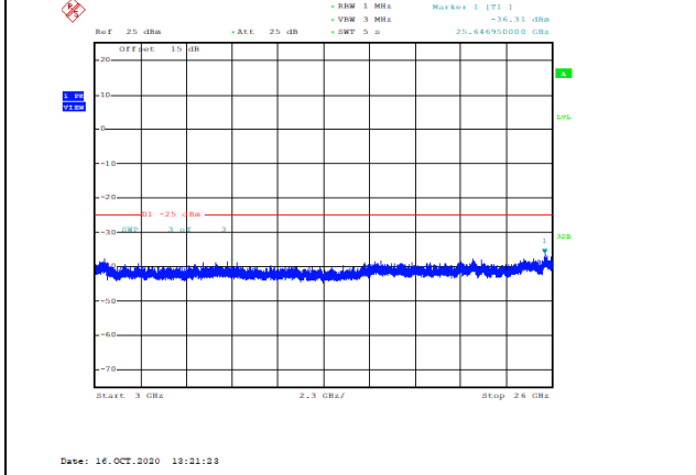
Band7-20MHz-16QAM-21350-1RB#0-Range3:3000~26000MHz--36.31-PASS
