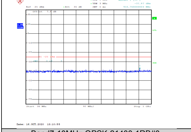
Band7-10MHz-QPSK-21400-1RB#0-Range1:30~1000MHz--37.97-PASS
