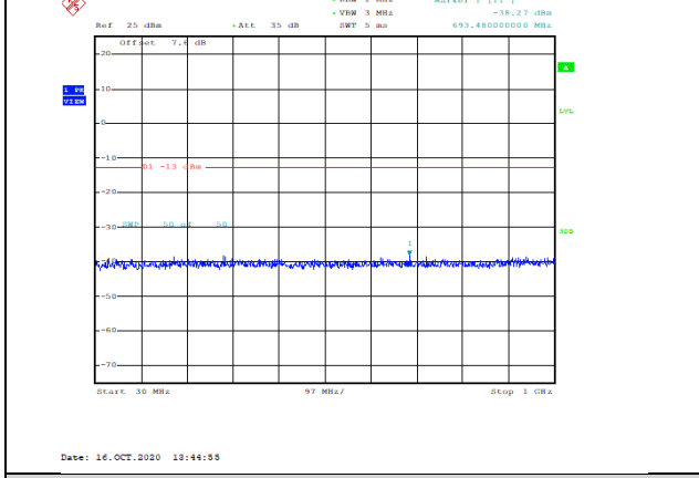
Band66-5MHz-QPSK-131997-1RB#0-Range1:30~1000MHz--38.27-PASS
