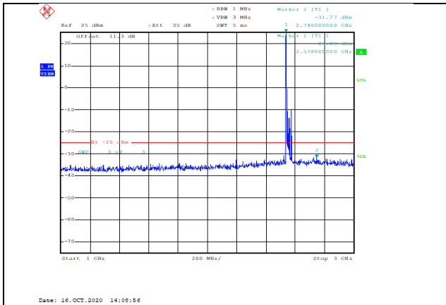
Band41-20MHz-16QAM-40140-1RB#0-Range2:1000~3000MHz--31.77-PASS
