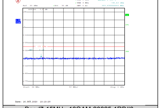
Band7-15MHz-16QAM-20825-1RB#0-Range1:30~1000MHz--38.62-PASS
