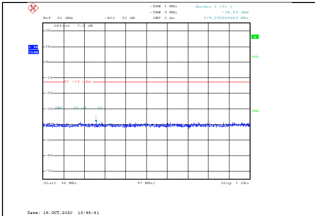
Band66-5MHz-16QAM-132647-1RB#0-Range1:30~1000MHz--38.49-PASS
