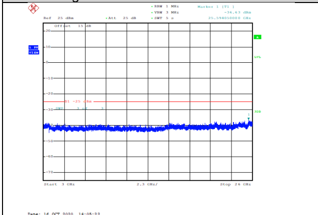
Band41-15MHz-QPSK-40590-1RB#0-Range3:3000~26000MHz--36.63-PASS
