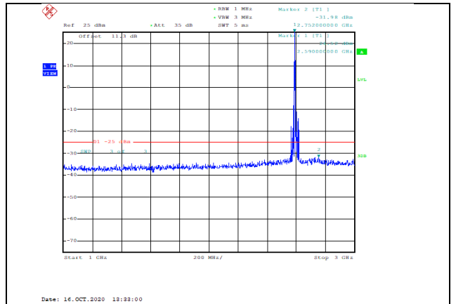
Band38-15MHz-16QAM-38000-1RB#0-Range2:1000~3000MHz--31.98-PASS
