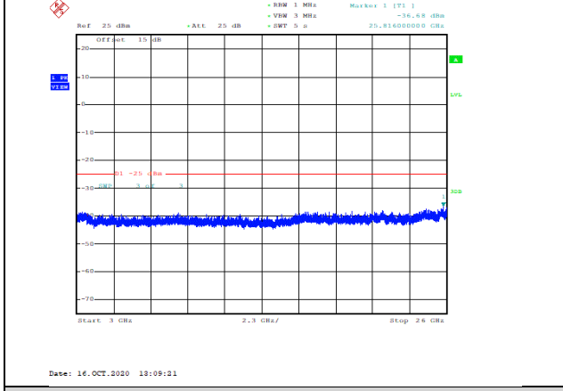
Band7-10MHz-16QAM-20800-1RB#0-Range3:3000~26000MHz--36.68-PASS
