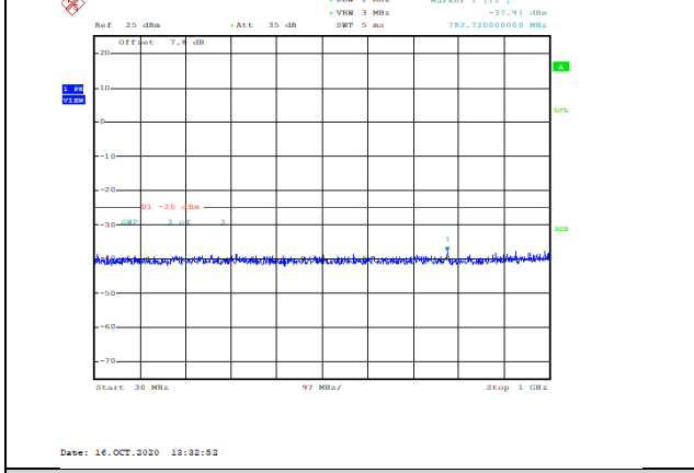
Band38-15MHz-16QAM-38000-1RB#0-Range1:30~1000MHz--37.91-PASS
