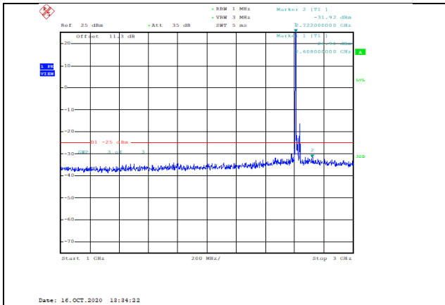
Band38-15MHz-16QAM-38175-1RB#0-Range2:1000~3000MHz--31.92-PASS
