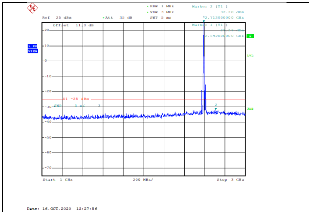
Band38-10MHz-QPSK-38000-1RB#0-Range2:1000~3000MHz--32.2-PASS
