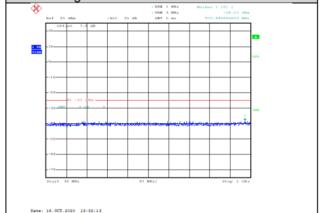
Band38-15MHz-QPSK-38000-1RB#0-Range1:30~1000MHz--38.25-PASS
