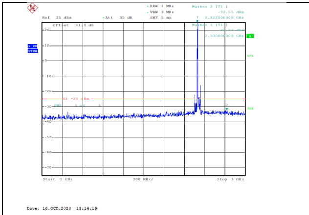
Band7-15MHz-QPSK-21100-1RB#0-Range2:1000~3000MHz--32.55-PASS
