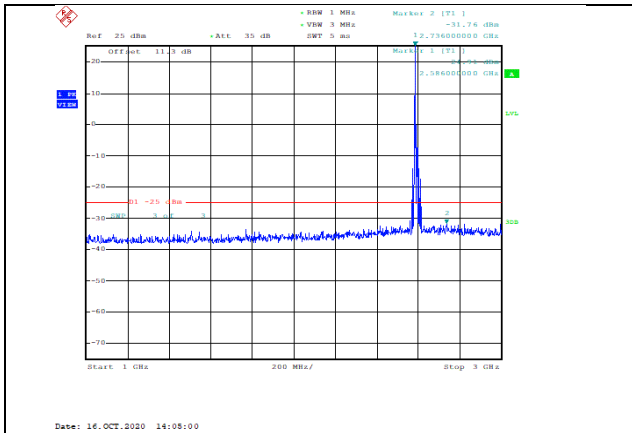
Band41-15MHz-QPSK-40590-1RB#0-Range2:1000~3000MHz--31.76-PASS
