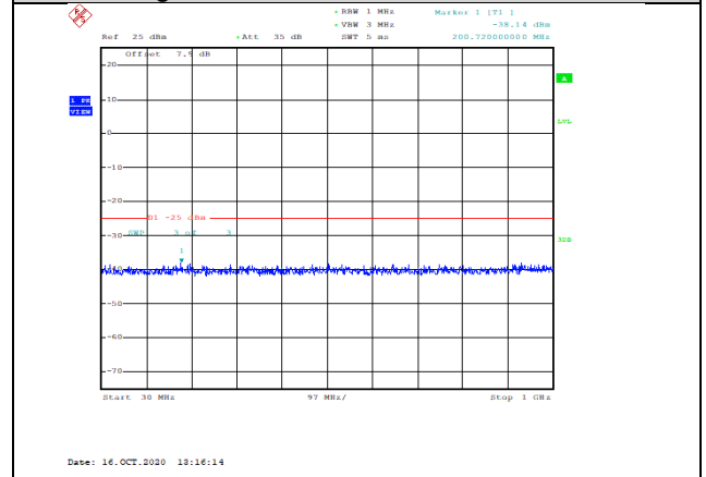
Band7-15MHz-16QAM-21375-1RB#0-Range1:30~1000MHz--38.14-PASS
