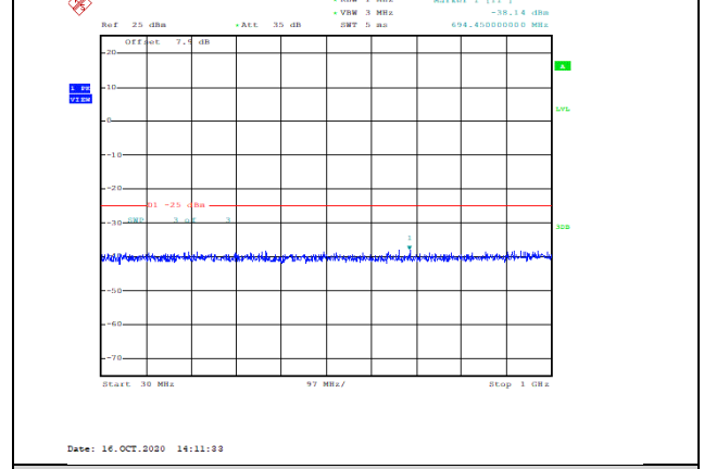
Band41-20MHz-16QAM-41140-1RB#0-Range1:30~1000MHz--38.14-PASS
