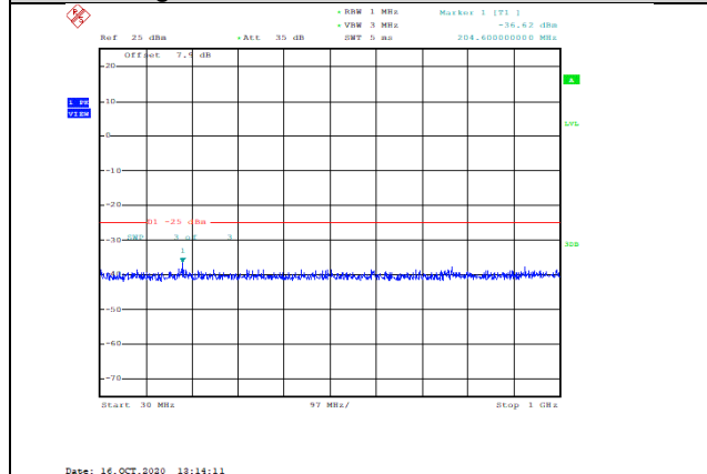
Band7-15MHz-QPSK-21100-1RB#0-Range1:30~1000MHz--36.62-PASS
