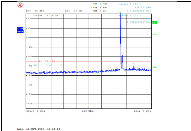
Band7-20MHz-16QAM-20850-1RB#0-Range2:1000~3000MHz--31.00-PASS
