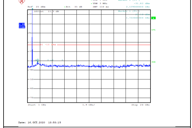
Band66-20MHz-16QAM-132322-1RB#0-Range2:1000~20000MHz--31.82-PASS
