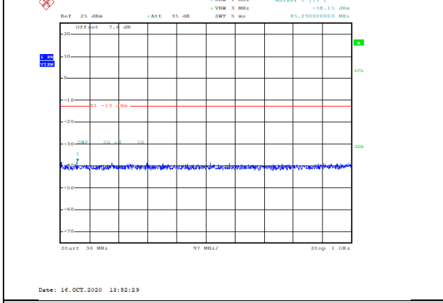
Band66-20MHz-16QAM-132072-1RB#0-Range1:30~1000MHz--38.15-PASS
