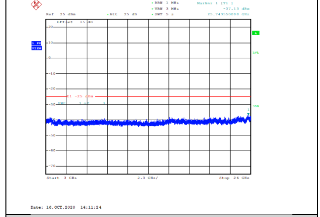
Band41-20MHz-QPSK-41140-1RB#0-Range3:3000~26000MHz--37.13-PASS
