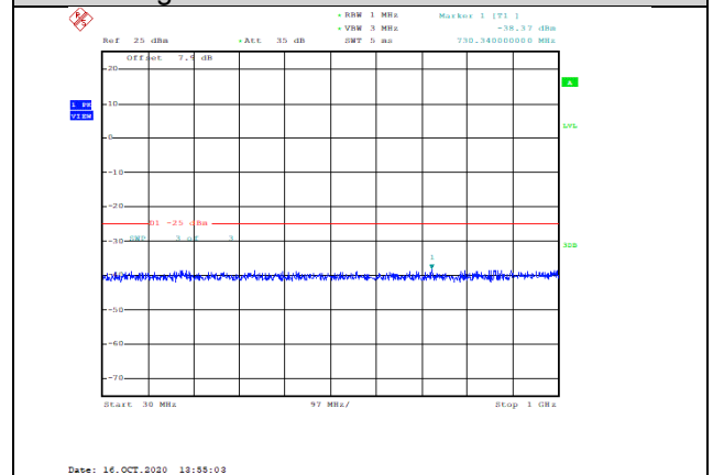
Band41-5MHz-16QAM-40065-1RB#0-Range1:30~1000MHz--38.37-PASS
