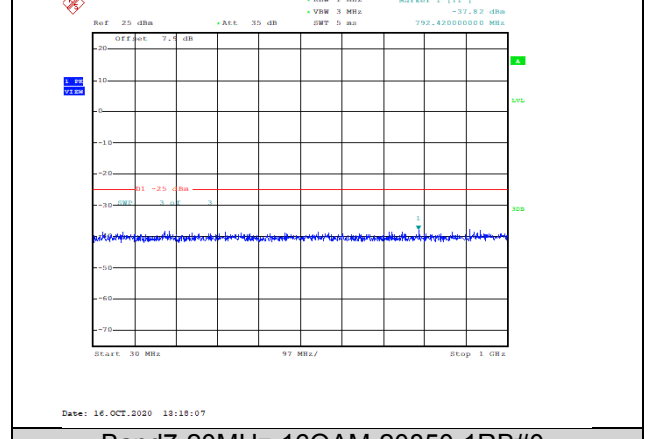
Band7-20MHz-16QAM-20850-1RB#0-Range1:30~1000MHz--37.82-PASS
