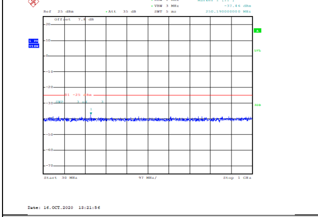
Band38-5MHz-QPSK-37775-1RB#0-Range1:30~1000MHz--37.46-PASS
