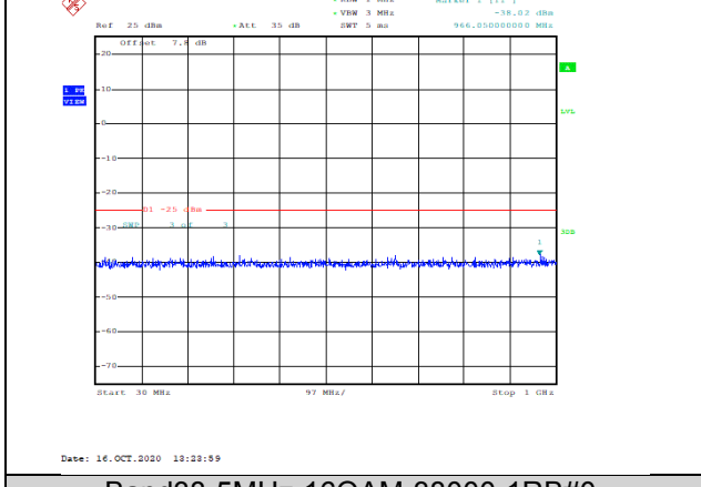
Band38-5MHz-16QAM-38000-1RB#0-Range1:30~1000MHz--38.02-PASS
