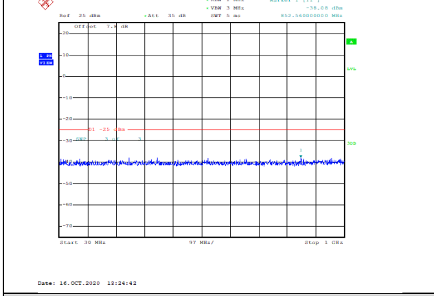
Band38-5MHz-QPSK-38225-1RB#0-Range1:30~1000MHz--38.08-PASS
