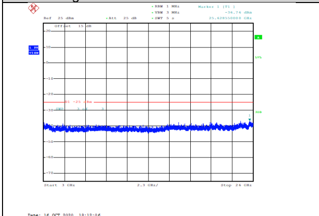
Band7-10MHz-16QAM-21400-1RB#0-Range3:3000~26000MHz--36.76-PASS
