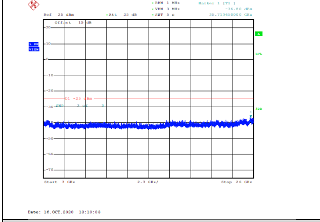
Band7-10MHz-QPSK-21100-1RB#0-Range3:3000~26000MHz--36.8-PASS
