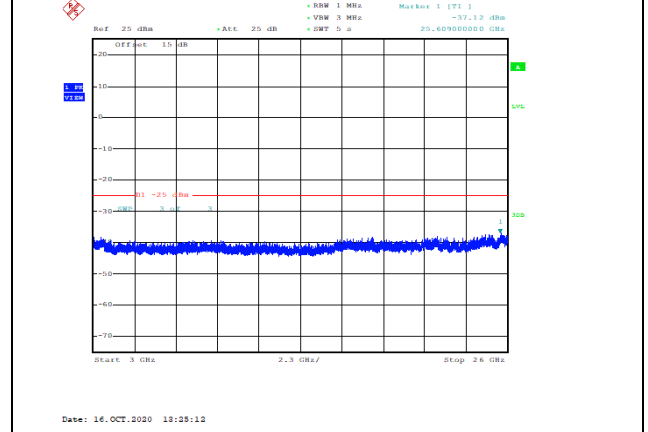
Band38-5MHz-QPSK-38225-1RB#0-Range3:3000~26000MHz--37.12-PASS
