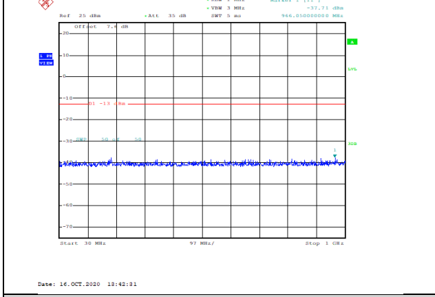
Band66-3MHz-QPSK-131987-1RB#0-Range1:30~1000MHz--37.71-PASS
