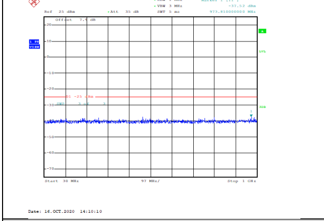
Band41-20MHz-16QAM-40590-1RB#0-Range1:30~1000MHz--37.52-PASS
