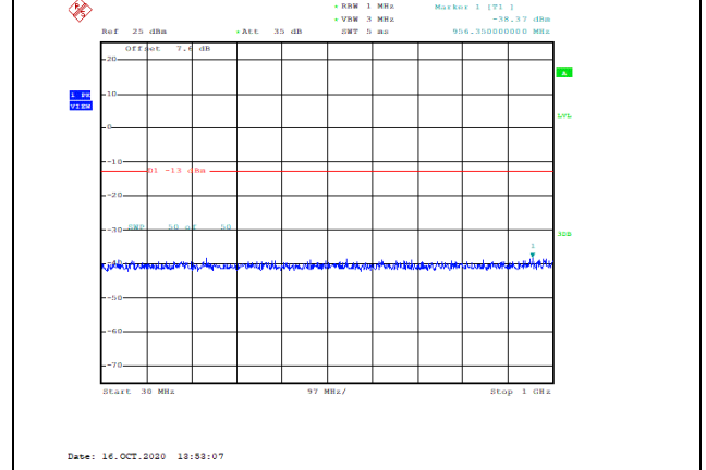
Band66-20MHz-16QAM-132322-1RB#0-Range1:30~1000MHz--38.37-PASS
