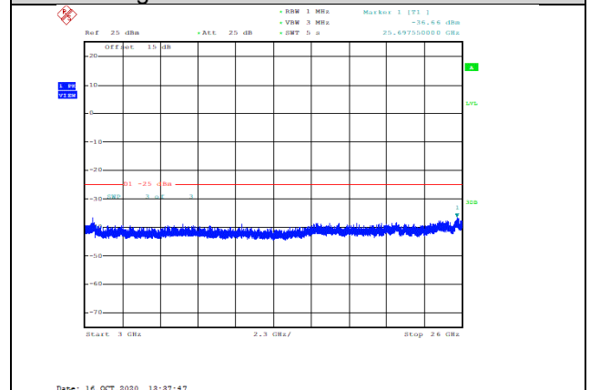
Band38-20MHz-16QAM-38000-1RB#0-Range3:3000~26000MHz--36.66-PASS
