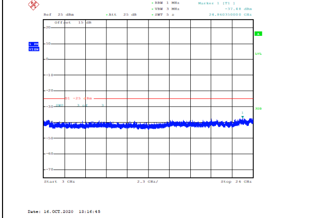
Band7-15MHz-16QAM-21375-1RB#0-Range3:3000~26000MHz--37.48-PASS
