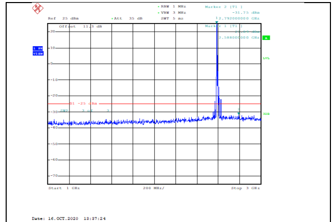
Band38-20MHz-16QAM-38000-1RB#0-Range2:1000~3000MHz--31.75-PASS
