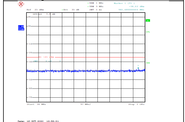
Band41-10MHz-16QAM-40090-1RB#0-Range1:30~1000MHz--38.02-PASS
