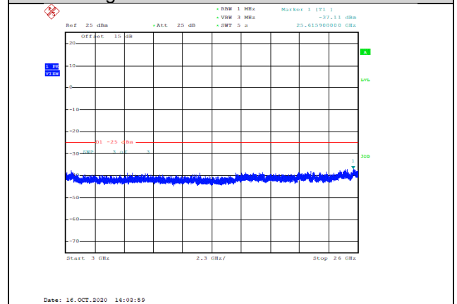
Band41-15MHz-QPSK-40115-1RB#0-Range3:3000~26000MHz--37.11-PASS
