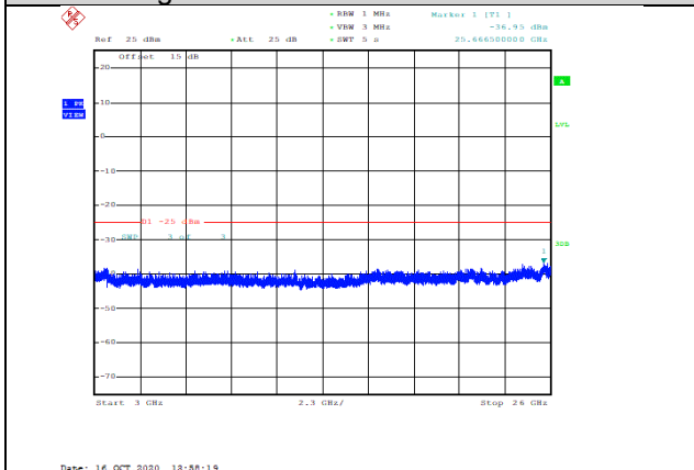
Band41-5MHz-16QAM-41215-1RB#0-Range3:3000~26000MHz--36.95-PASS
