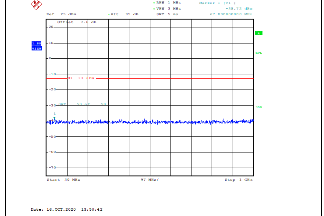
Band66-15MHz-16QAM-132322-1RB#0-Range1:30~1000MHz--38.72-PASS
