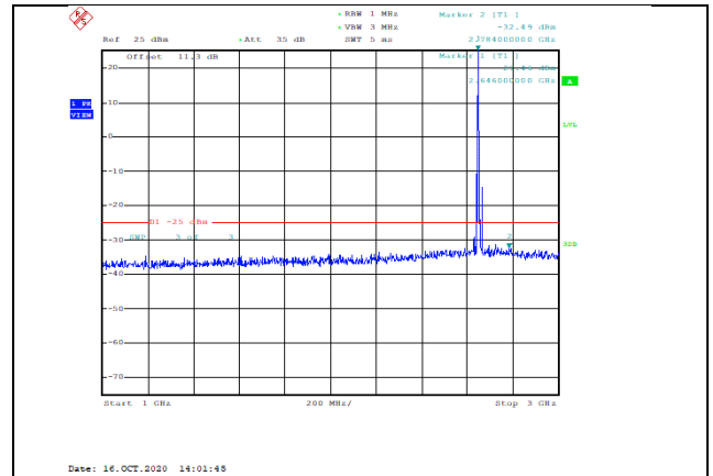
Band41-10MHz-QPSK-41190-1RB#0-Range2:1000~3000MHz--32.49-PASS
