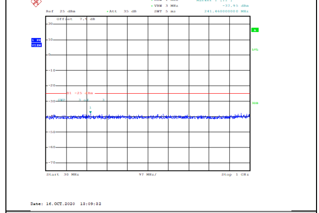
Band7-10MHz-QPSK-21100-1RB#0-Range1:30~1000MHz--37.95-PASS
