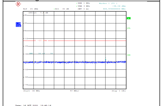
Band66-10MHz-16QAM-132322-1RB#0-Range1:30~1000MHz--38.34-PASS
