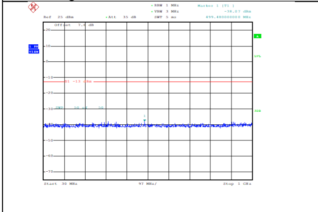
Band66-1.4MHz-QPSK-131979-1RB#0-Range1:30~1000MHz--38.07-PASS
