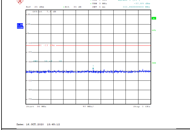
Band66-5MHz-16QAM-131997-1RB#0-Range1:30~1000MHz--37.89-PASS
