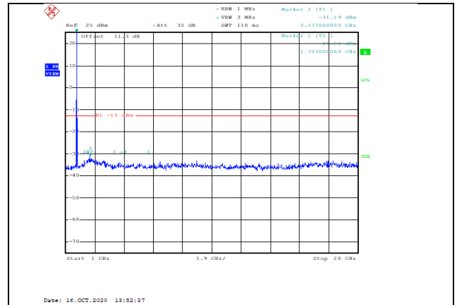
Band66-20MHz-16QAM-132072-1RB#0-Range2:1000~20000MHz--31.19-PASS
