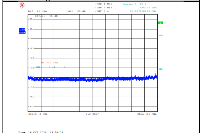
Band7-20MHz-16QAM-21100-1RB#0-Range3:3000~26000MHz--36.57-PASS
