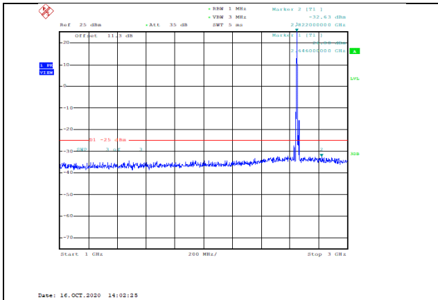
Band41-10MHz-16QAM-41190-1RB#0-Range2:1000~3000MHz--32.63-PASS
