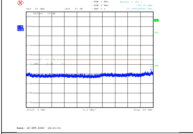
Band41-20MHz-QPSK-40590-1RB#0-Range3:3000~26000MHz--36.18-PASS
