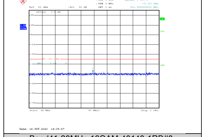
Band41-20MHz-16QAM-40140-1RB#0-Range1:30~1000MHz--37.83-PASS
