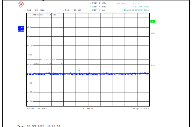
Band7-20MHz-16QAM-21350-1RB#0-Range1:30~1000MHz--37.98-PASS
