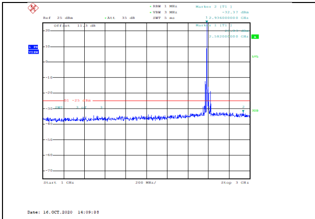
Band41-20MHz-QPSK-40590-1RB#0-Range2:1000~3000MHz--32.37-PASS
