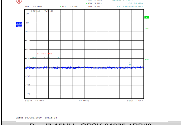
Band7-15MHz-QPSK-21375-1RB#0-Range1:30~1000MHz--38.24-PASS
