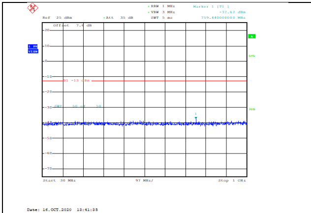
Band66-1.4MHz-QPSK-132665-1RB#0-Range1:30~1000MHz--37.62-PASS
