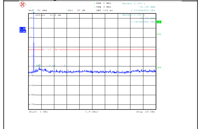
Band66-1.4MHz-QPSK-132322-1RB#0-Range2:1000~20000MHz--31.94-PASS
