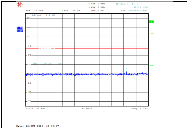
Band66-10MHz-16QAM-132622-1RB#0-Range1:30~1000MHz--38.16-PASS
