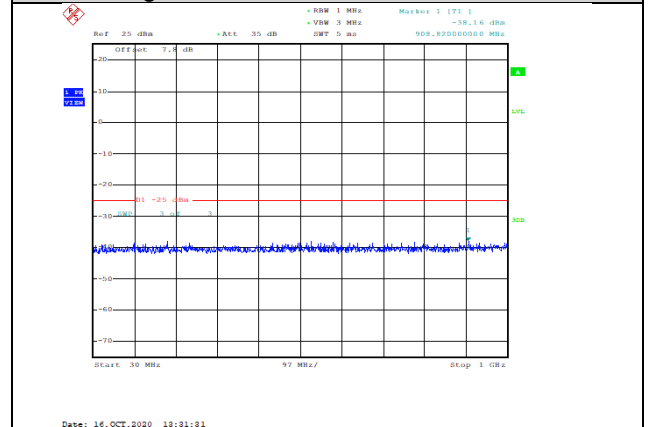
Band38-15MHz-16QAM-37825-1RB#0-Range1:30~1000MHz--38.16-PASS
