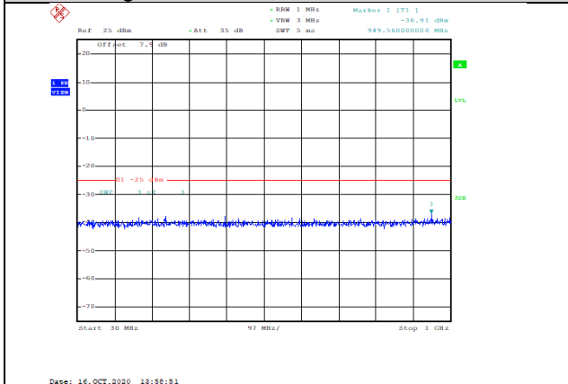
Band41-10MHz-QPSK-40090-1RB#0-Range1:30~1000MHz--36.91-PASS
