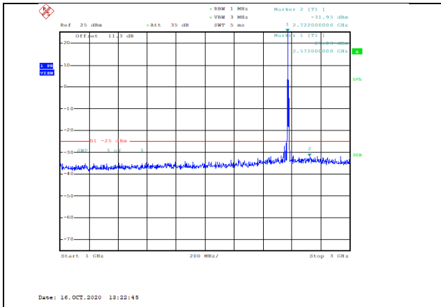
Band38-5MHz-16QAM-37775-1RB#0-Range2:1000~3000MHz--31.95-PASS
