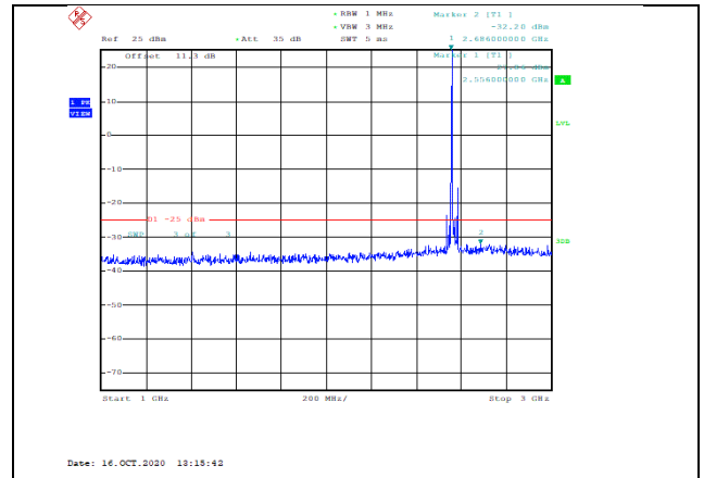
Band7-15MHz-QPSK-21375-1RB#0-Range2:1000~3000MHz--32.28-PASS
