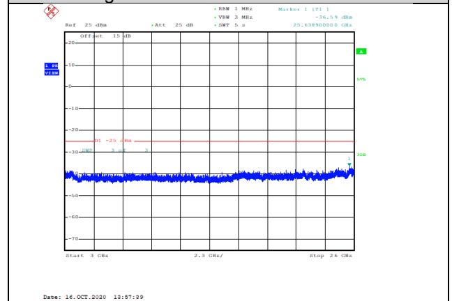
Band41-5MHz-QPSK-41215-1RB#0-Range3:3000~26000MHz--36.59-PASS
