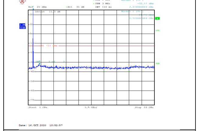
Band66-20MHz-QPSK-132322-1RB#0-Range2:1000~20000MHz--32.37-PASS
