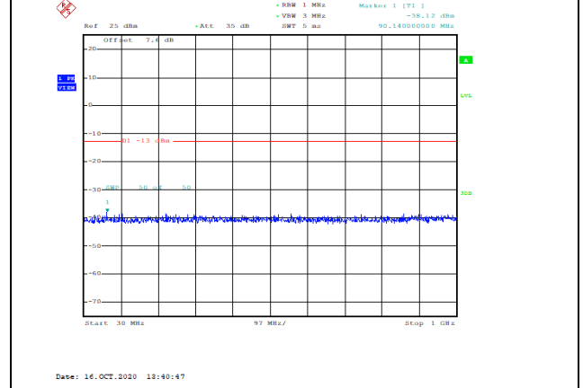
Band66-1.4MHz-16QAM-132322-1RB#0-Range1:30~1000MHz--38.12-PASS
