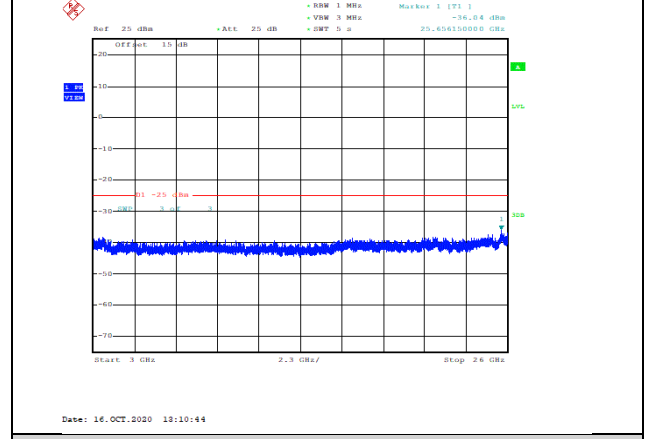
Band7-10MHz-16QAM-21100-1RB#0-Range3:3000~26000MHz--36.04-PASS
