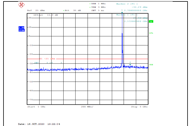
Band38-5MHz-QPSK-37775-1RB#0-Range2:1000~3000MHz--32.29-PASS
