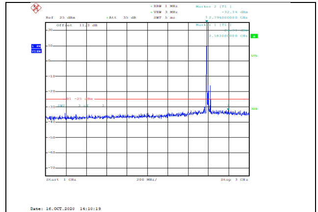
Band41-20MHz-16QAM-40590-1RB#0-Range2:1000~3000MHz--32.36-PASS
