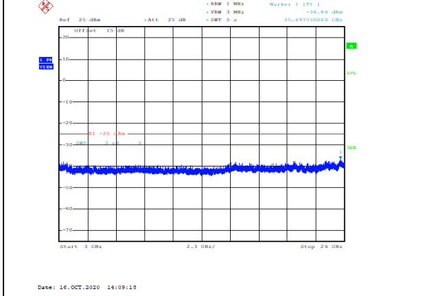
Band41-20MHz-16QAM-40140-1RB#0-Range3:3000~26000MHz--36.86-PASS
