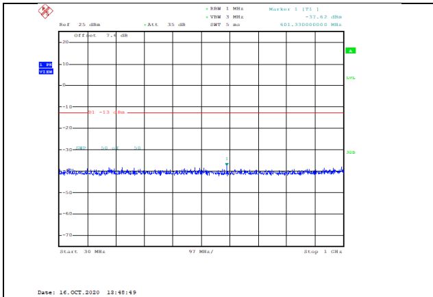
Band66-10MHz-QPSK-132622-1RB#0-Range1:30~1000MHz--37.62-PASS
