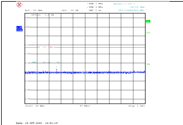
Band66-15MHz-QPSK-132597-1RB#0-Range1:30~1000MHz--38.2-PASS
