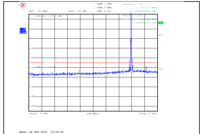
Band41-15MHz-16QAM-40590-1RB#0-Range2:1000~3000MHz--31.72-PASS
