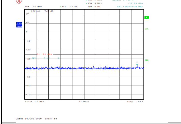
Band38-20MHz-QPSK-38150-1RB#0-Range1:30~1000MHz--36.99-PASS
