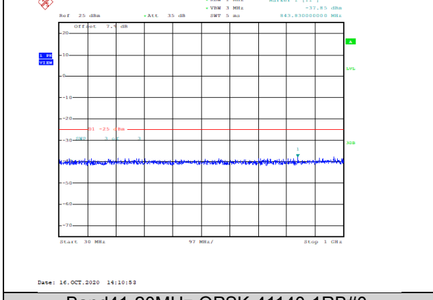
Band41-20MHz-QPSK-41140-1RB#0-Range1:30~1000MHz--37.85-PASS
