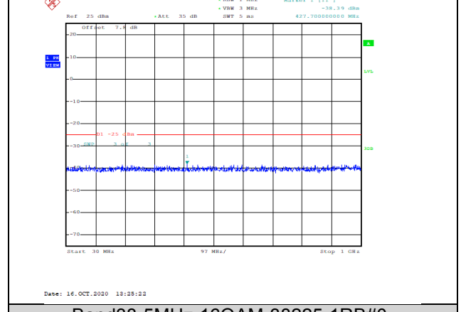
Band38-5MHz-16QAM-38225-1RB#0-Range1:30~1000MHz--38.39-PASS
