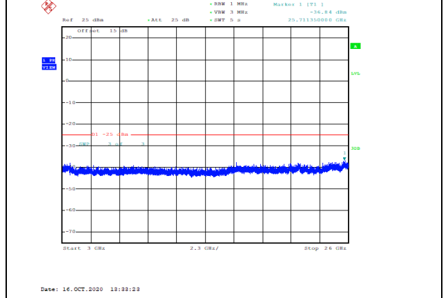
Band38-15MHz-16QAM-38000-1RB#0-Range3:3000~26000MHz--36.84-PASS
