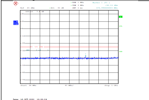
Band38-15MHz-QPSK-38175-1RB#0-Range1:30~1000MHz--38.16-PASS
