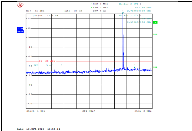
Band41-5MHz-16QAM-40065-1RB#0-Range2:1000~3000MHz--32.3-PASS
