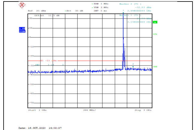
Band41-15MHz-QPSK-40115-1RB#0-Range2:1000~3000MHz--32.02-PASS
