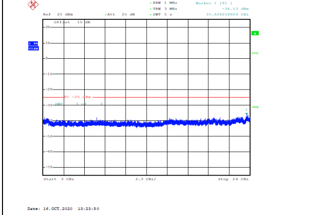
Band38-5MHz-QPSK-38000-1RB#0-Range3:3000~26000MHz--36.53-PASS
