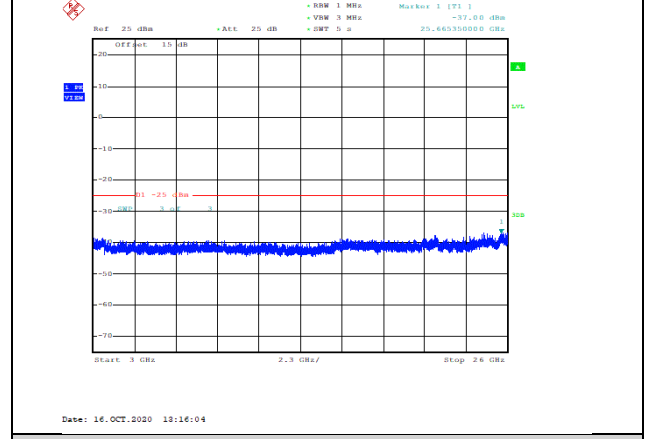
Band7-15MHz-QPSK-21375-1RB#0-Range3:3000~26000MHz--37-PASS
