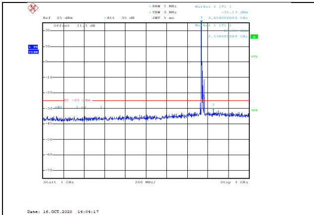
Band41-15MHz-16QAM-40115-1RB#0-Range2:1000~3000MHz--31.13-PASS
