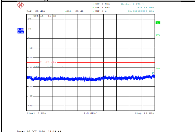
Band38-15MHz-16QAM-38175-1RB#0-Range3:3000~26000MHz--36.88-PASS
