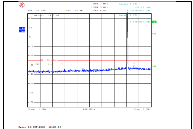
Band38-5MHz-QPSK-38225-1RB#0-Range2:1000~3000MHz--32.18-PASS
