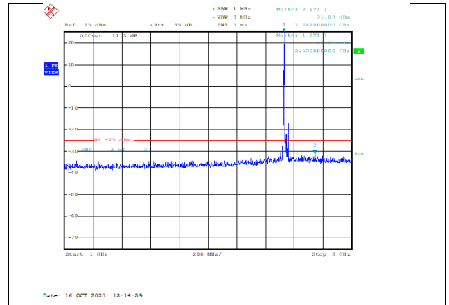
Band7-15MHz-16QAM-21100-1RB#0-Range2:1000~3000MHz--31.03-PASS
