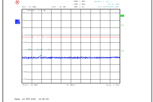
Band66-5MHz-16QAM-132322-1RB#0-Range1:30~1000MHz--38.47-PASS
