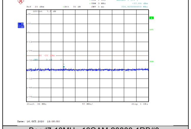
Band7-10MHz-16QAM-20800-1RB#0-Range1:30~1000MHz--37.86-PASS
