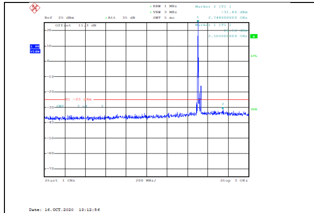
Band7-15MHz-QPSK-20825-1RB#0-Range2:1000~3000MHz--31.48-PASS
