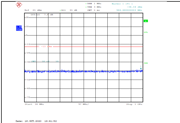
Band66-1.4MHz-16QAM-132665-1RB#0-Range1:30~1000MHz--38.38-PASS
