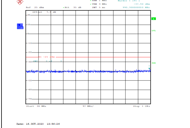
Band41-5MHz-16QAM-40590-1RB#0-Range1:30~1000MHz--37.9-PASS
