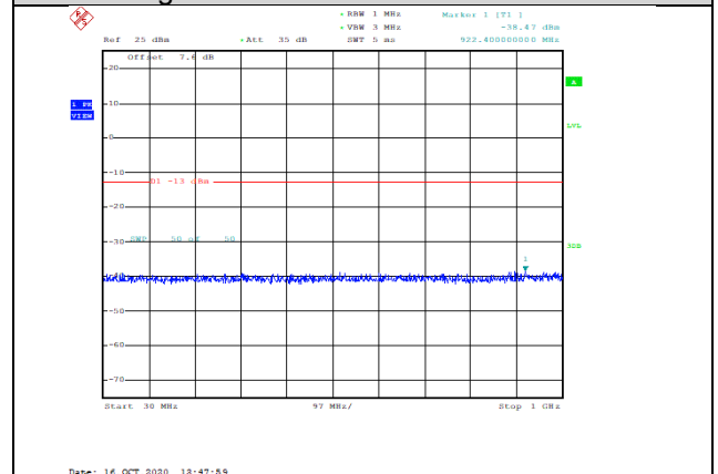
Band66-10MHz-QPSK-132322-1RB#0-Range1:30~1000MHz--38.47-PASS
