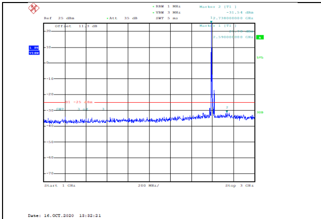
Band38-15MHz-QPSK-38000-1RB#0-Range2:1000~3000MHz--31.54-PASS
