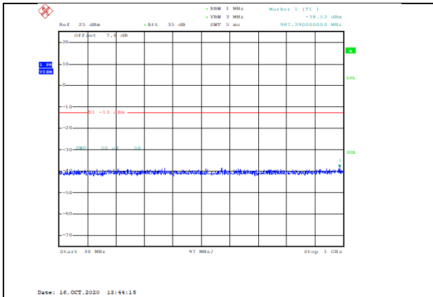
Band66-3MHz-16QAM-132657-1RB#0-Range1:30~1000MHz--38.52-PASS
