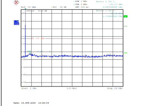
Band66-3MHz-QPSK-132657-1RB#0-Range2:1000~20000MHz--32.57-PASS
