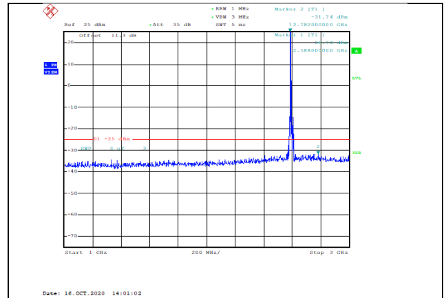
Band41-10MHz-16QAM-40590-1RB#0-Range2:1000~3000MHz--31.74-PASS
