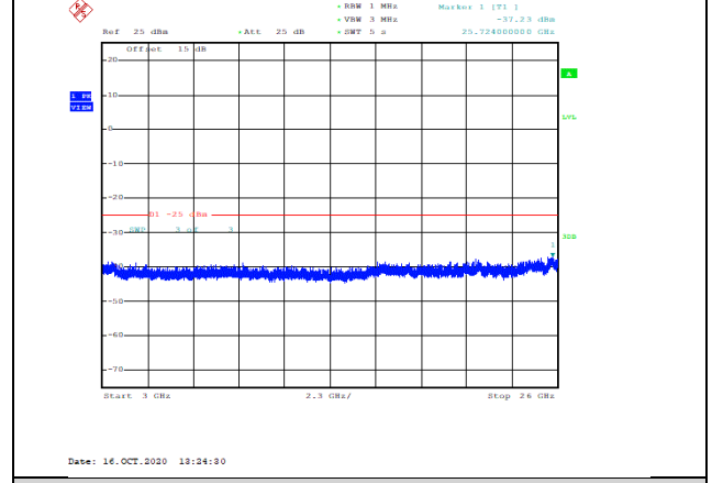
Band38-5MHz-16QAM-38000-1RB#0-Range3:3000~26000MHz--37.23-PASS
