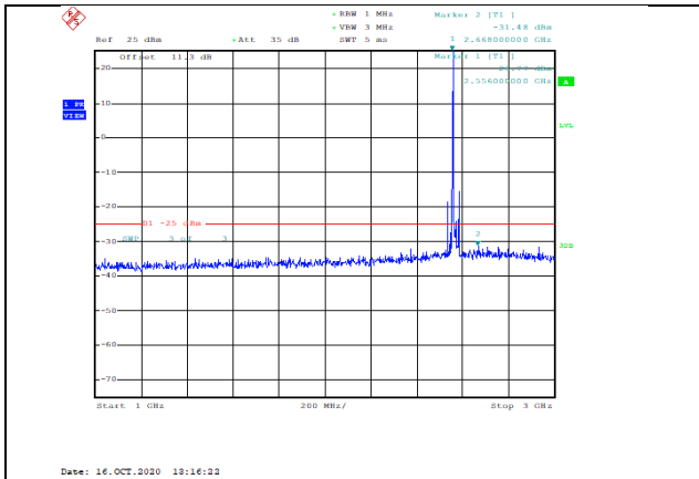
Band7-15MHz-16QAM-21375-1RB#0-Range2:1000~3000MHz--31.48-PASS
