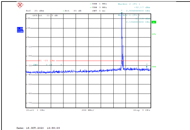
Band41-10MHz-16QAM-40090-1RB#0-Range2:1000~3000MHz--32.17-PASS
