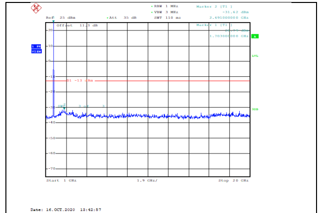
Band66-3MHz-16QAM-131987-1RB#0-Range2:1000~20000MHz--31.62-PASS
