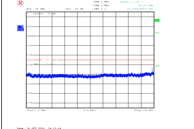
Band41-20MHz-16QAM-41140-1RB#0-Range3:3000~26000MHz--36.01-PASS
