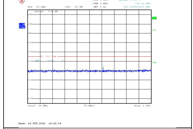
Band38-5MHz-QPSK-38000-1RB#0-Range1:30~1000MHz--38.16-PASS
