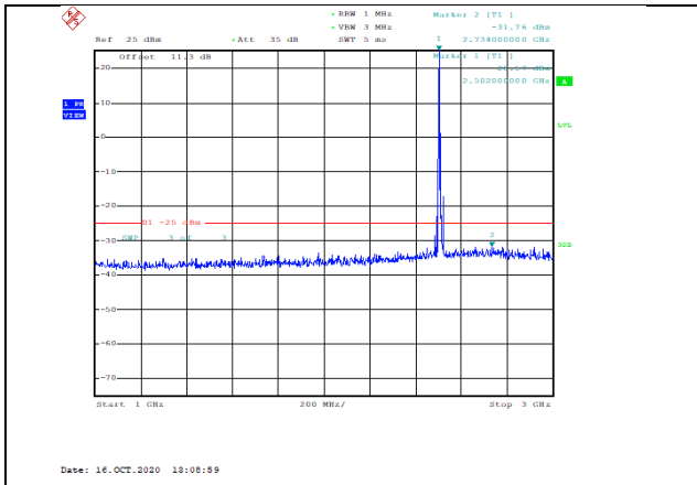
Band7-10MHz-16QAM-20800-1RB#0-Range2:1000~3000MHz--31.76-PASS
