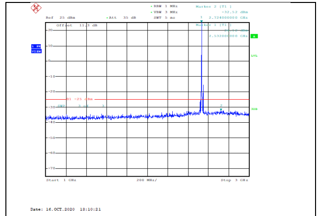
Band7-10MHz-16QAM-21100-1RB#0-Range2:1000~3000MHz--32.52-PASS
