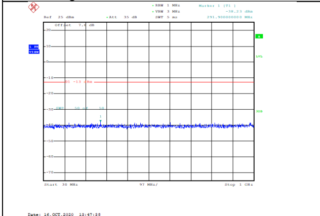
Band66-10MHz-16QAM-132022-1RB#0-Range1:30~1000MHz--38.23-PASS
