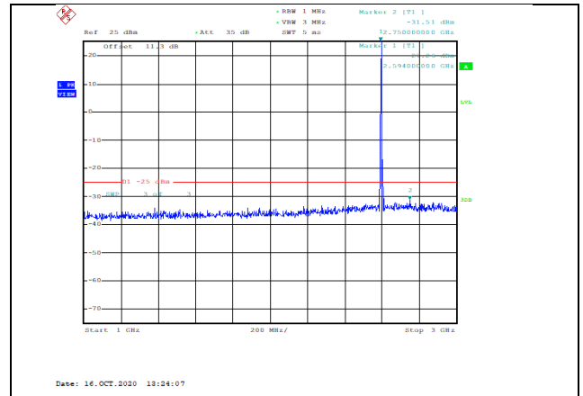
Band38-5MHz-16QAM-38000-1RB#0-Range2:1000~3000MHz--31.51-PASS
