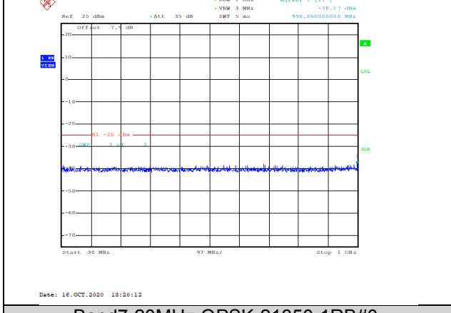
Band7-20MHz-QPSK-21350-1RB#0-Range1:30~1000MHz--38.17-PASS
