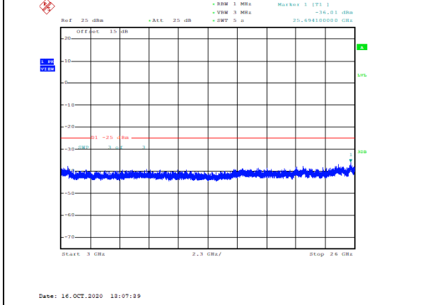
Band7-5MHz-16QAM-21425-1RB#0-Range3:3000~26000MHz--36.01-PASS
