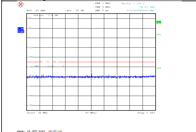
Band38-20MHz-16QAM-38000-1RB#0-Range1:30~1000MHz--38.03-PASS
