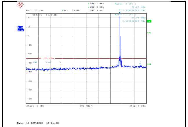
Band7-10MHz-QPSK-21400-1RB#0-Range2:1000~3000MHz--32.05-PASS
