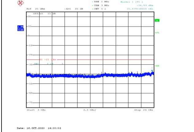
Band41-10MHz-16QAM-40090-1RB#0-Range3:3000~26000MHz--36.99-PASS
