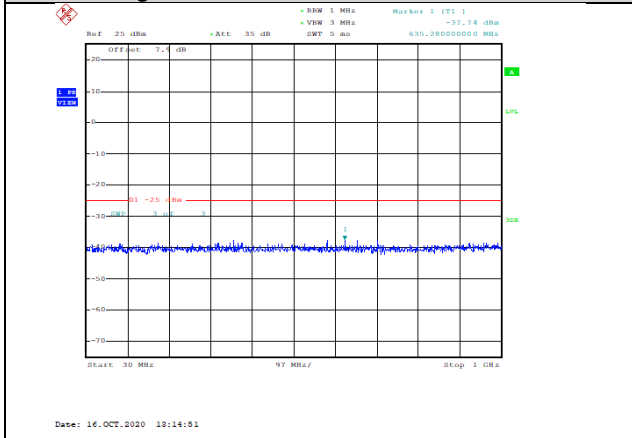
Band7-15MHz-16QAM-21100-1RB#0-Range1:30~1000MHz--37.74-PASS
