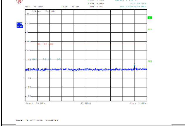
Band66-15MHz-QPSK-132047-1RB#0-Range1:30~1000MHz--37.5-PASS
