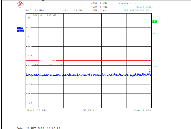
Band41-15MHz-QPSK-41165-1RB#0-Range1:30~1000MHz--37.71-PASS
