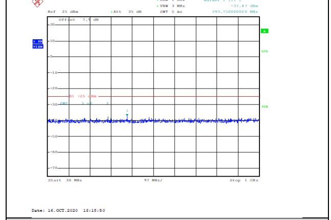
Band7-20MHz-QPSK-21100-1RB#0-Range1:30~1000MHz--37.47-PASS
