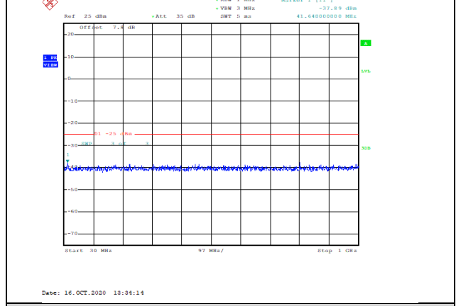
Band38-15MHz-16QAM-38175-1RB#0-Range1:30~1000MHz--37.89-PASS
