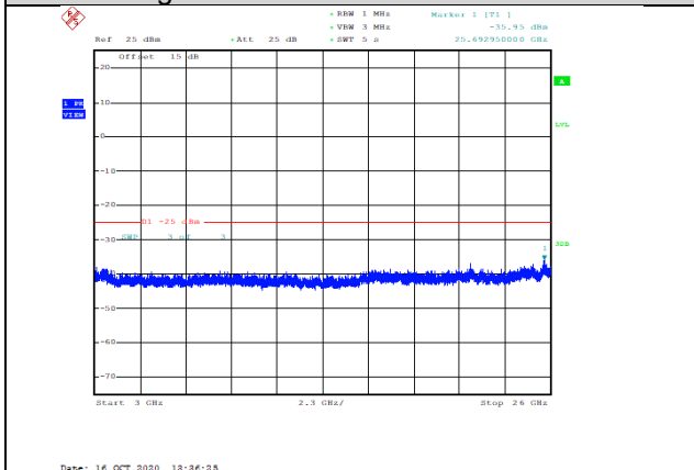
Band38-20MHz-16QAM-37850-1RB#0-Range3:3000~26000MHz--35.95-PASS
