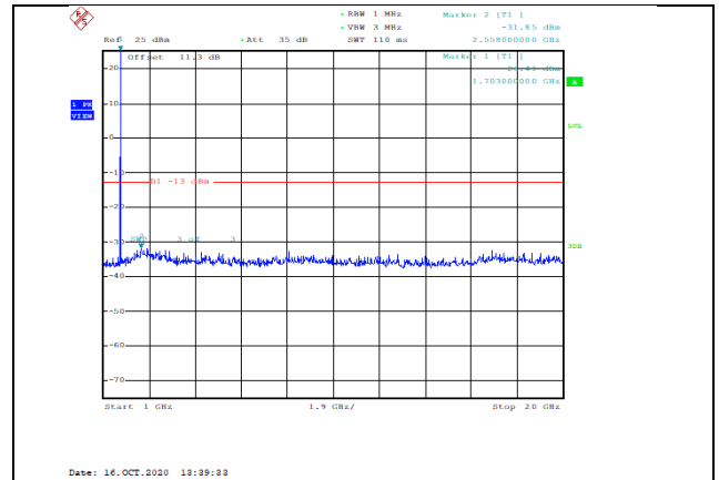
Band66-1.4MHz-QPSK-131979-1RB#0-Range2:1000~20000MHz--31.85-PASS
