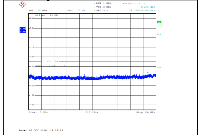
Band7-15MHz-16QAM-21100-1RB#0-Range3:3000~26000MHz--36.83-PASS
