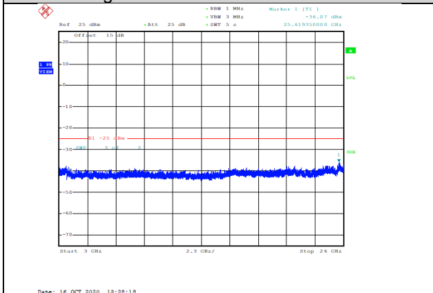
Band38-10MHz-QPSK-38000-1RB#0-Range3:3000~26000MHz--36.07-PASS
