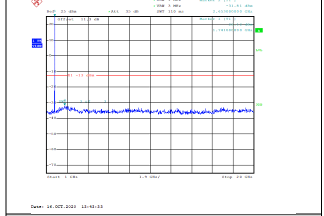
Band66-3MHz-16QAM-132322-1RB#0-Range2:1000~20000MHz--31.81-PASS
