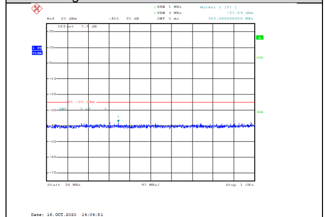
Band41-15MHz-QPSK-40590-1RB#0-Range1:30~1000MHz--37.69-PASS
