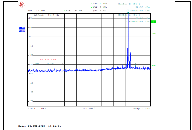
Band41-20MHz-QPSK-41140-1RB#0-Range2:1000~3000MHz--32.37-PASS
