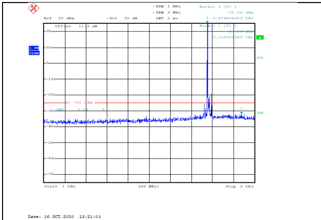
Band7-20MHz-16QAM-21350-1RB#0-Range2:1000~3000MHz--32.3-PASS
