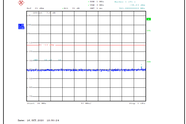
Band66-15MHz-QPSK-132322-1RB#0-Range1:30~1000MHz--38.03-PASS
