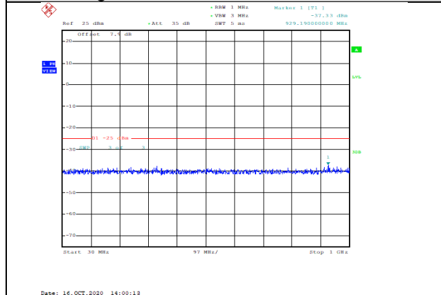
Band41-10MHz-QPSK-40590-1RB#0-Range1:30~1000MHz--37.33-PASS
