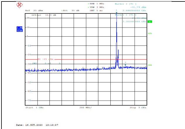
Band7-15MHz-16QAM-20825-1RB#0-Range2:1000~3000MHz--31.79-PASS
