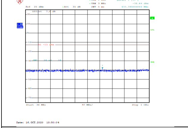
Band66-15MHz-16QAM-132047-1RB#0-Range1:30~1000MHz--38.46-PASS
