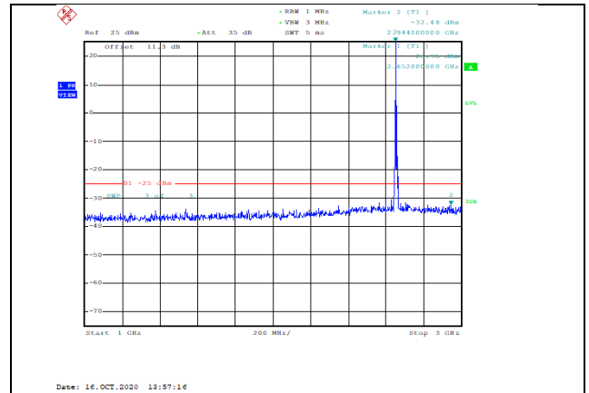
Band41-5MHz-QPSK-41215-1RB#0-Range2:1000~3000MHz--32.48-PASS
