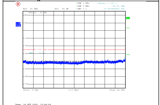
Band38-15MHz-QPSK-38175-1RB#0-Range3:3000~26000MHz--36.95-PASS
