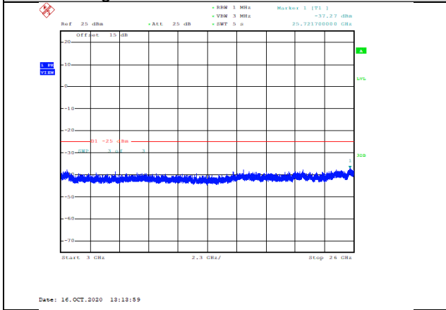
Band7-15MHz-16QAM-20825-1RB#0-Range3:3000~26000MHz--37.27-PASS
