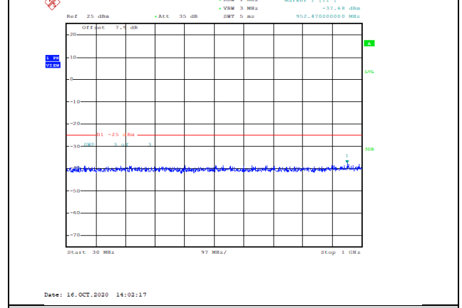
Band41-10MHz-16QAM-41190-1RB#0-Range1:30~1000MHz--37.68-PASS
