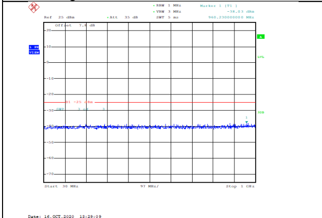
Band38-10MHz-QPSK-38200-1RB#0-Range1:30~1000MHz--38.03-PASS
