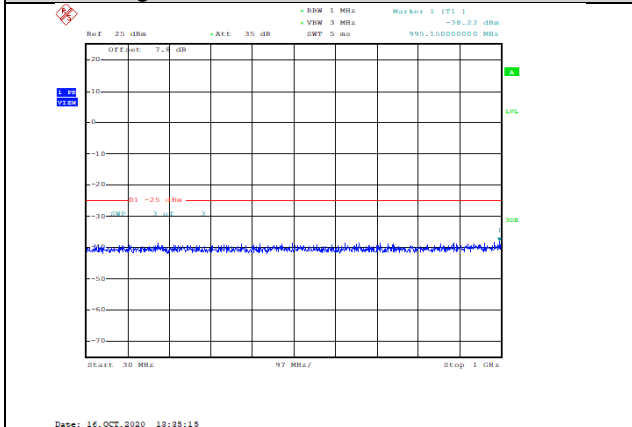
Band38-20MHz-QPSK-37850-1RB#0-Range1:30~1000MHz--38.22-PASS
