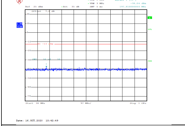
Band66-3MHz-16QAM-131987-1RB#0-Range1:30~1000MHz--38.06-PASS
