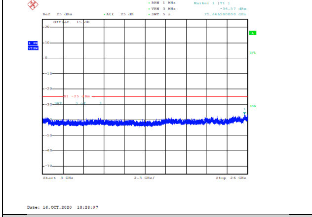
Band38-5MHz-16QAM-37775-1RB#0-Range3:3000~26000MHz--36.57-PASS
