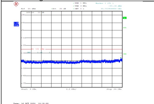
Band7-20MHz-16QAM-20850-1RB#0-Range3:3000~26000MHz--37.14-PASS
