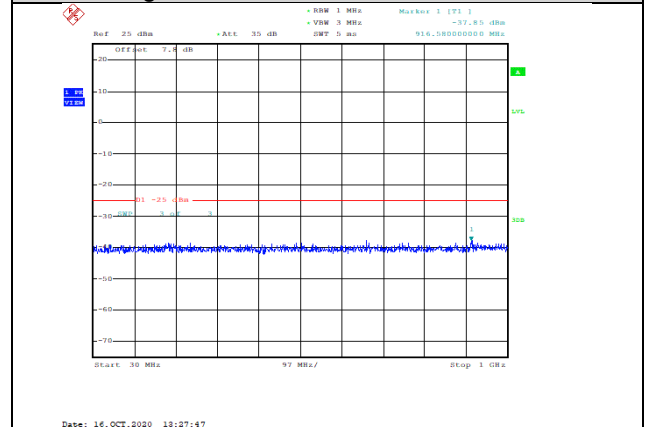
Band38-10MHz-QPSK-38000-1RB#0-Range1:30~1000MHz--37.85-PASS
