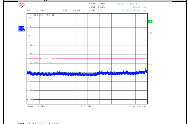
Band41-10MHz-QPSK-41190-1RB#0-Range3:3000~26000MHz--36.62-PASS
