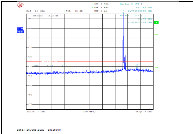
Band7-20MHz-QPSK-21100-1RB#0-Range2:1000~3000MHz--31.83-PASS
