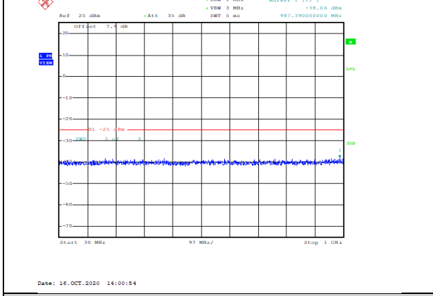
Band41-10MHz-16QAM-40590-1RB#0-Range1:30~1000MHz--38.06-PASS
