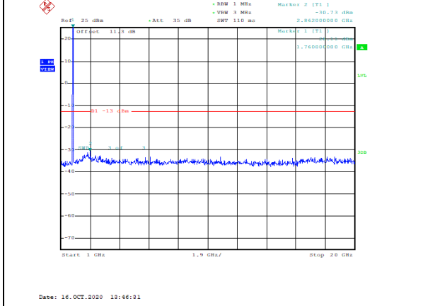
Band66-5MHz-QPSK-132647-1RB#0-Range2:1000~20000MHz--30.73-PASS
