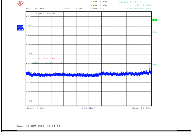
Band7-15MHz-QPSK-21100-1RB#0-Range3:3000~26000MHz--36.52-PASS
