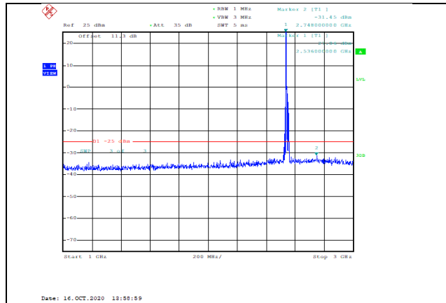
Band41-10MHz-QPSK-40090-1RB#0-Range2:1000~3000MHz--31.45-PASS
