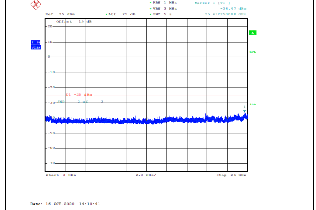
Band41-20MHz-16QAM-40590-1RB#0-Range3:3000~26000MHz--36.47-PASS
