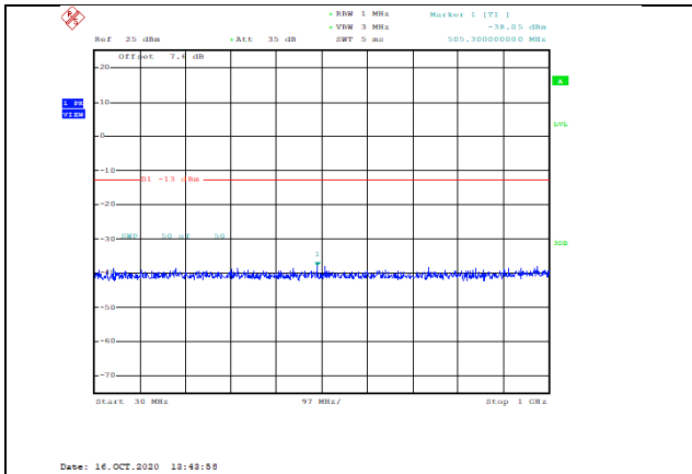
Band66-3MHz-QPSK-132657-1RB#0-Range1:30~1000MHz--38.05-PASS
