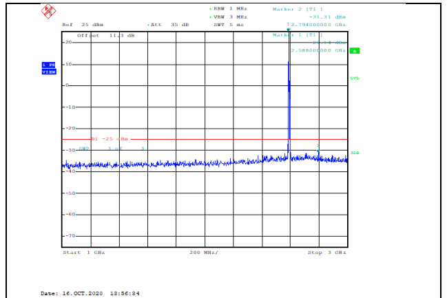
Band41-5MHz-16QAM-40590-1RB#0-Range2:1000~3000MHz--31.31-PASS
