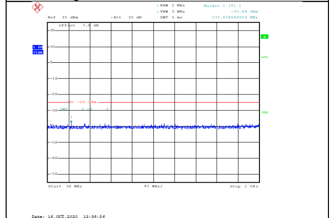
Band38-20MHz-QPSK-38000-1RB#0-Range1:30~1000MHz--37.98-PASS
