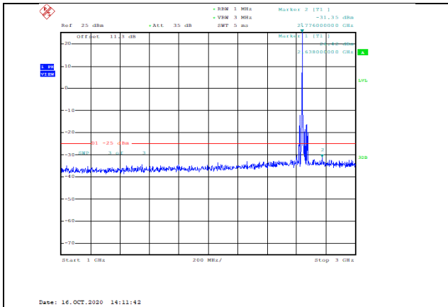
Band41-20MHz-16QAM-41140-1RB#0-Range2:1000~3000MHz--31.35-PASS
