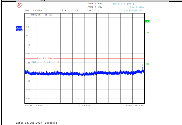
Band38-20MHz-16QAM-38150-1RB#0-Range3:3000~26000MHz--36.1-PASS
