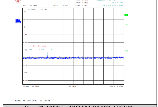
Band7-10MHz-16QAM-21400-1RB#0-Range1:30~1000MHz--37.53-PASS
