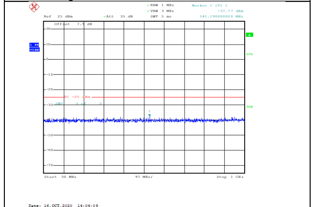
Band41-15MHz-16QAM-40115-1RB#0-Range1:30~1000MHz--37.77-PASS
