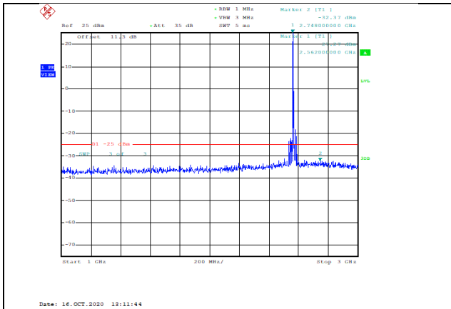
Band7-10MHz-16QAM-21400-1RB#0-Range2:1000~3000MHz--32.37-PASS
