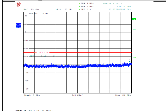
Band41-10MHz-QPSK-40090-1RB#0-Range3:3000~26000MHz--37.12-PASS
