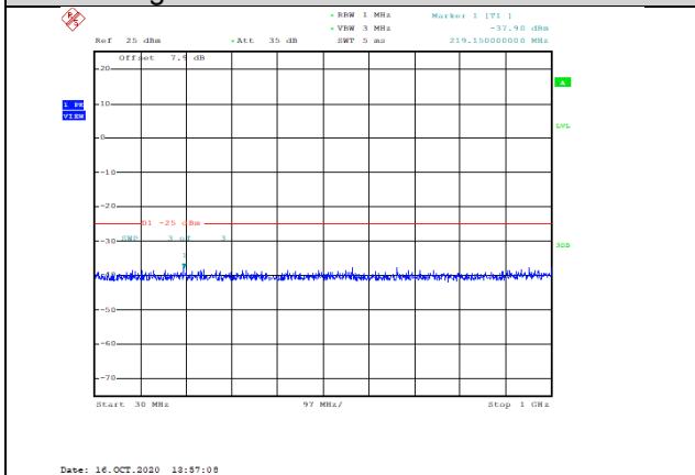
Band41-5MHz-QPSK-41215-1RB#0-Range1:30~1000MHz--37.9-PASS
