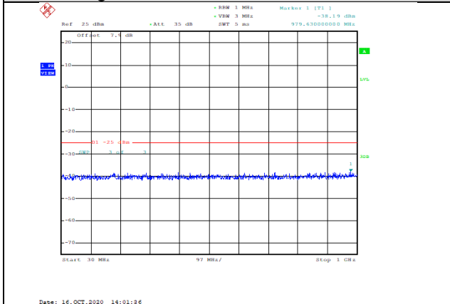
Band41-10MHz-QPSK-41190-1RB#0-Range1:30~1000MHz--38.19-PASS
