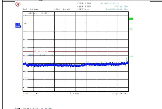
Band7-15MHz-QPSK-20825-1RB#0-Range3:3000~26000MHz--36.68-PASS
