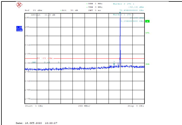
Band38-5MHz-QPSK-38000-1RB#0-Range2:1000~3000MHz--32.18-PASS
