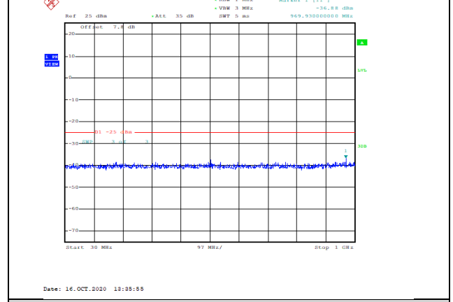
Band38-20MHz-16QAM-37850-1RB#0-Range1:30~1000MHz--36.88-PASS
