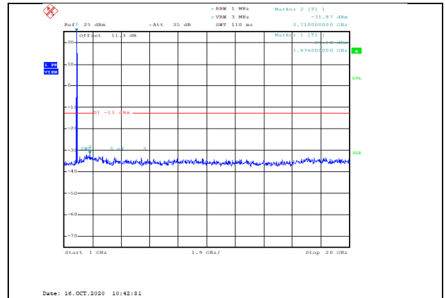
Band2-20MHz-16QAM-18700-1RB#0-Range2:1000~20000MHz--31.87-PASS
