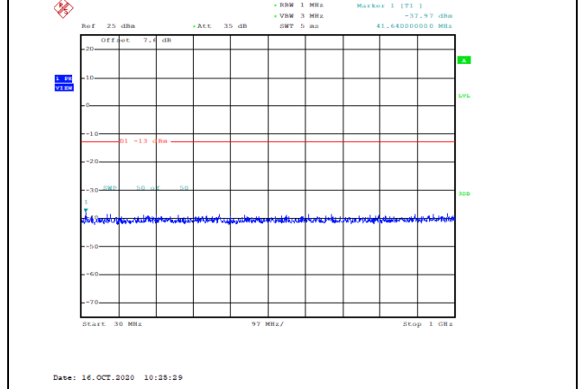
Band2-5MHz-16QAM-18900-1RB#0-Range1:30~1000MHz--37.97-PASS
