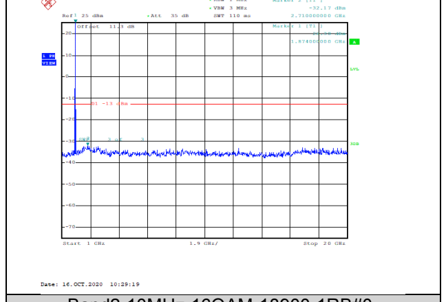
Band2-10MHz-16QAM-18900-1RB#0-Range2:1000~20000MHz--32.17-PASS
