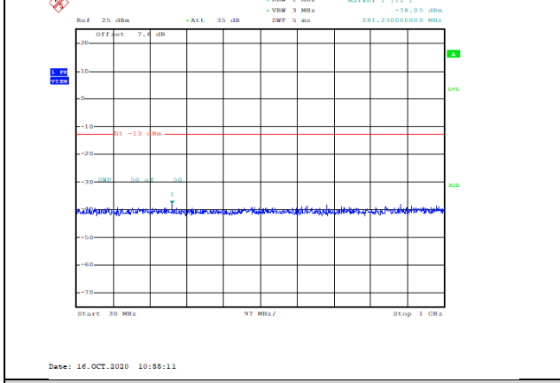
Band4-20MHz-QPSK-20050-1RB#0-Range1:30~1000MHz--38.05-PASS
