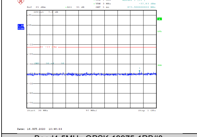
Band4-5MHz-QPSK-19975-1RB#0-Range1:30~1000MHz--37.83-PASS
