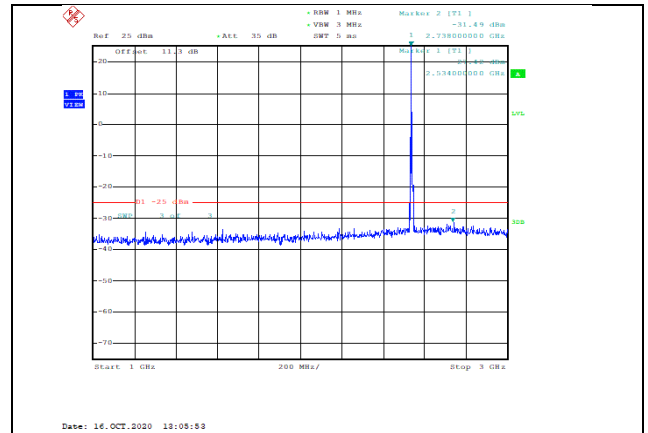
Band7-5MHz-16QAM-21100-1RB#0-Range2:1000~3000MHz--31.49-PASS
