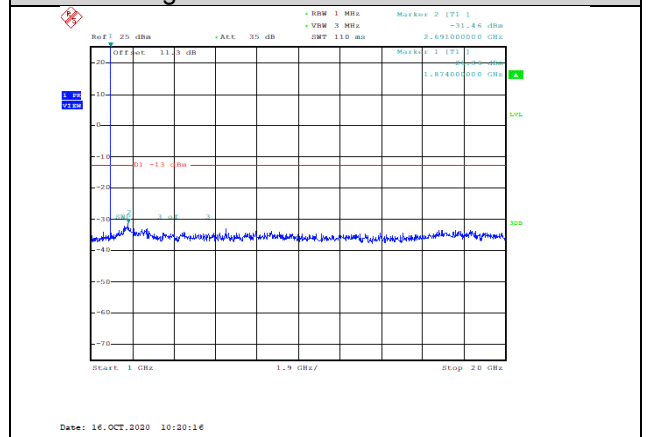
Band2-1.4MHz-QPSK-18900-1RB#0- Range2:1000~20000MHz--31.46-PASS
