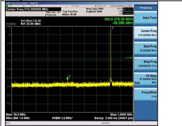
Band26-3MHz-QPSK-26775-1RB#0-Range1:30~1000MHz
