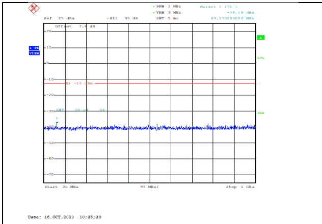
Band2-15MHz-QPSK-19125-1RB#0-Range1:30~1000MHz--38.18-PASS
