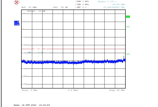
Band7-5MHz-16QAM-20775-1RB#0-Range3:3000~26000MHz--36.06-PASS
