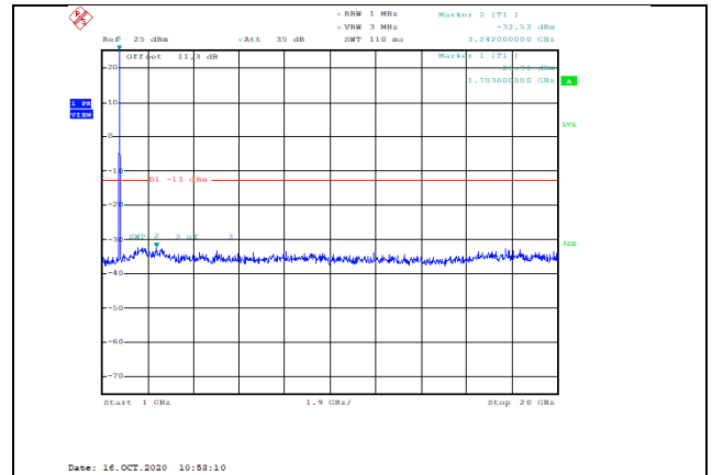
Band4-15MHz-QPSK-20025-1RB#0-Range2:1000~20000MHz--32.52-PASS
