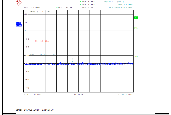
Band4-5MHz-QPSK-20175-1RB#0-Range1:30~1000MHz--38.08-PASS
