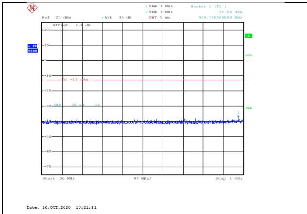
Band2-1.4MHz-16QAM-19193-1RB#0-Range1:30~1000MHz--37.8-PASS
