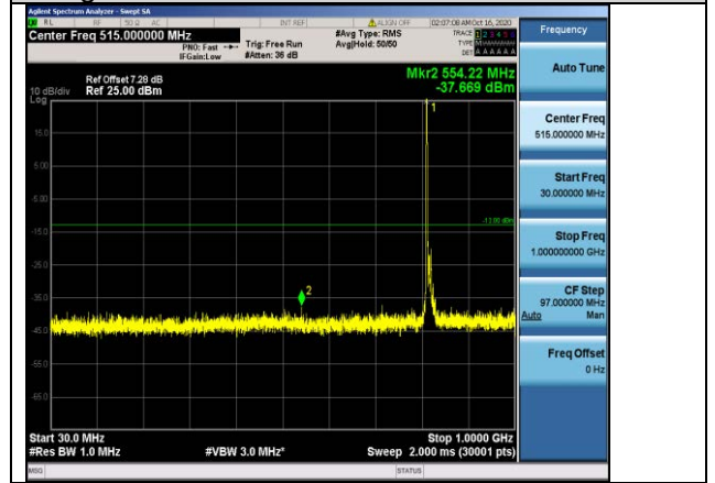
Band26-10MHz-QPSK-26740-1RB#0-Range1:30~1000MHz
