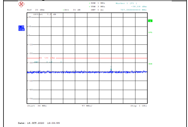
Band7-5MHz-16QAM-20775-1RB#0-Range1:30~1000MHz--38.08-PASS
