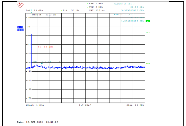
Band2-3MHz-QPSK-18615-1RB#0-Range2:1000~20000MHz--32.4-PASS
