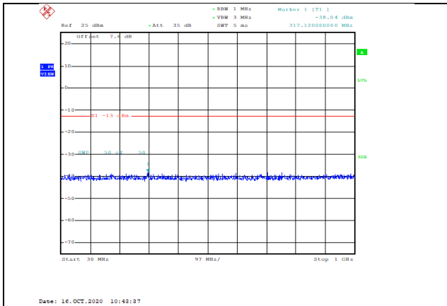
Band2-20MHz-16QAM-19100-1RB#0-Range1:30~1000MHz--38.04-PASS
