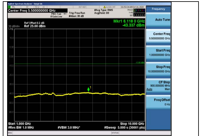
Band17-10MHz-QPSK-23800-1RB#0-Range2:1000~10000MHz
