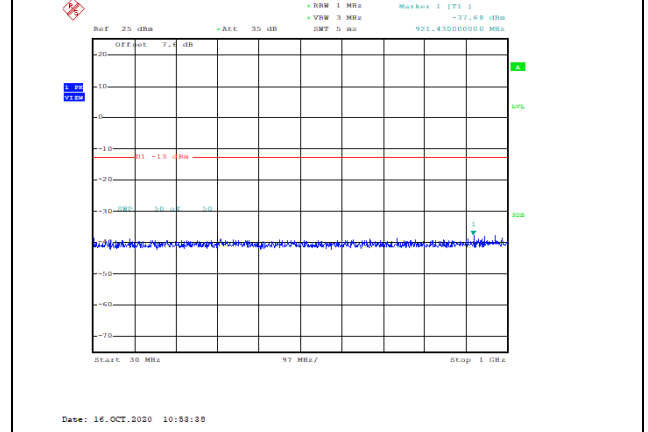
Band4-15MHz-QPSK-20175-1RB#0-Range1:30~1000MHz--37.68-PASS
