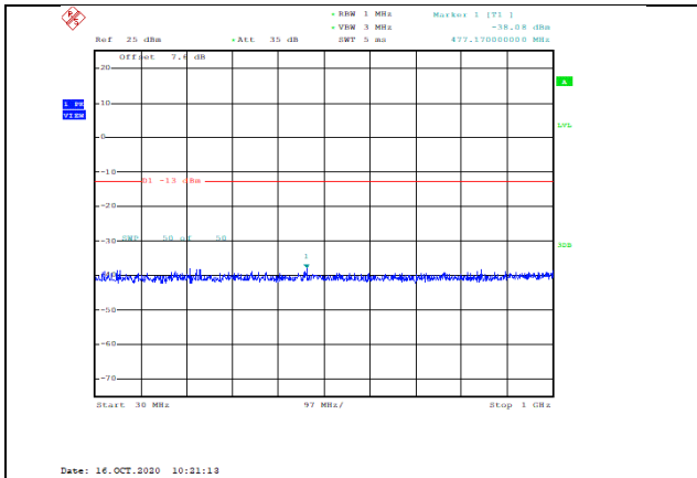
Band2-1.4MHz-QPSK-19193-1RB#0-Range1:30~1000MHz--38.08-PASS
