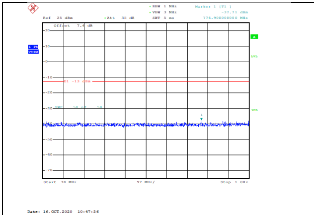
Band4-3MHz-QPSK-20385-1RB#0-Range1:30~1000MHz--37.71-PASS
