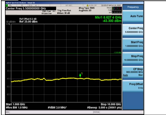
Band26-5MHz-QPSK-26740-1RB#0-Range2:1000~10000MHz
