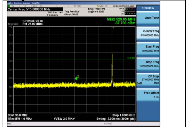
Band26-3MHz-16QAM-26705-1RB#0-Range1:30~1000MHz
