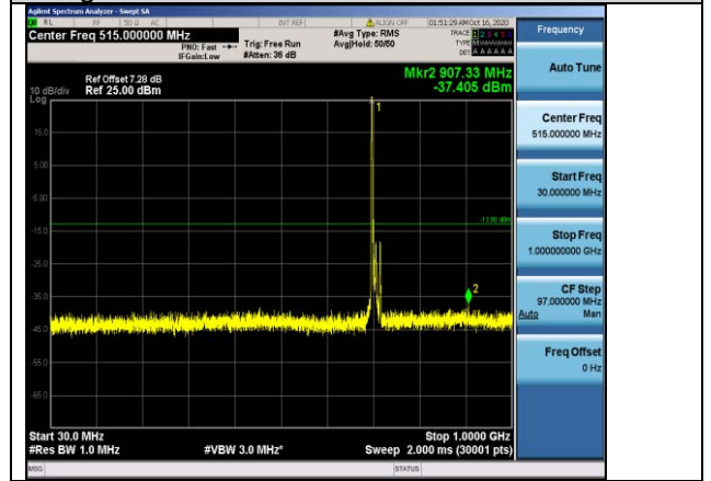
Band17-10MHz-16QAM-23780-1RB#0-Range1:30~1000MHz
