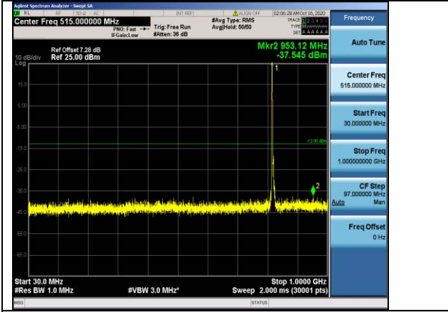
Band26-5MHz-16QAM-26765-1RB#0-Range1:30~1000MHz
