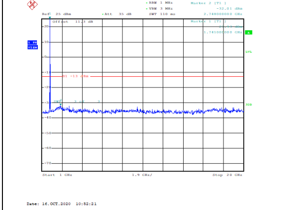
Band4-10MHz-16QAM-20350-1RB#0-Range2:1000~20000MHz--32.01-PASS
