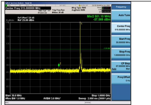
Band17-10MHz-16QAM-23790-1RB#0- Range1:30~1000MHz
