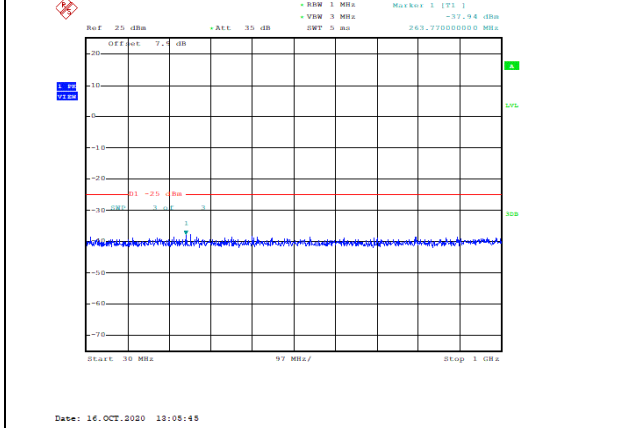
Band7-5MHz-16QAM-21100-1RB#0-Range1:30~1000MHz--37.94-PASS
