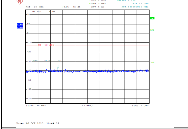
Band4-1.4MHz-QPSK-19957-1RB#0-Range1:30~1000MHz--38.37-PASS
