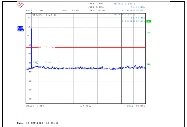
Band2-10MHz-16QAM-18650-1RB#0-Range2:1000~20000MHz--31.59-PASS
