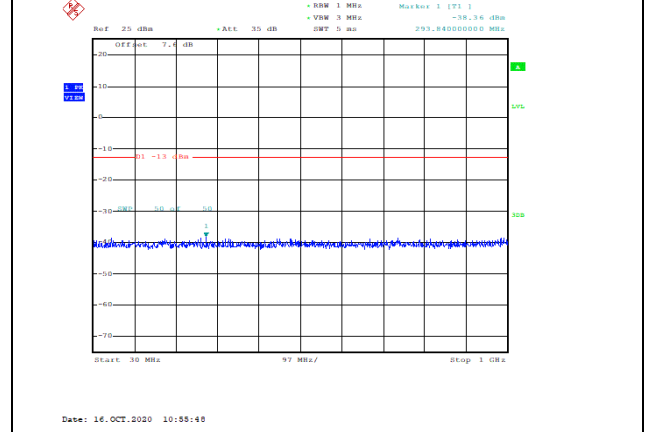
Band4-20MHz-QPSK-20175-1RB#0-Range1:30~1000MHz--38.36-PASS
