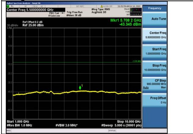
Band17-10MHz-16QAM-23790-1RB#0- Range2:1000~10000MHz
