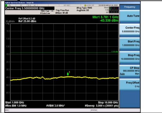
Band26-1.4MHz-QPSK-26740-1RB#0-Range2:1000~10000MHz
