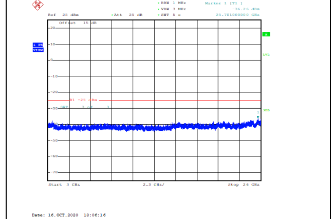
Band7-5MHz-16QAM-21100-1RB#0-Range3:3000~26000MHz--36.26-PASS
