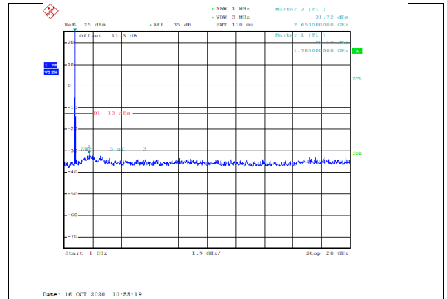
Band4-20MHz-QPSK-20050-1RB#0-Range2:1000~20000MHz--31.72-PASS
