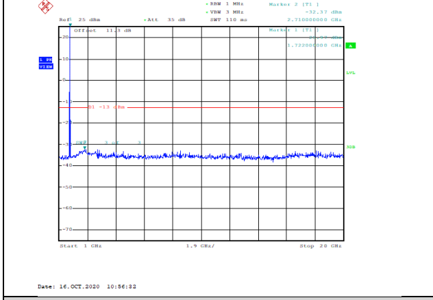
Band4-20MHz-QPSK-20300-1RB#0-Range2:1000~20000MHz--32.37-PASS
