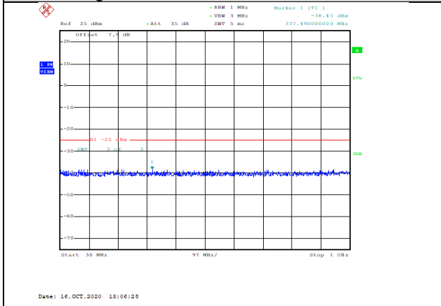
Band7-5MHz-QPSK-21425-1RB#0-Range1:30~1000MHz--38.45-PASS
