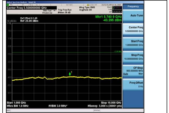
Band17-10MHz-16QAM-23780-1RB#0-Range2:1000~10000MHz
