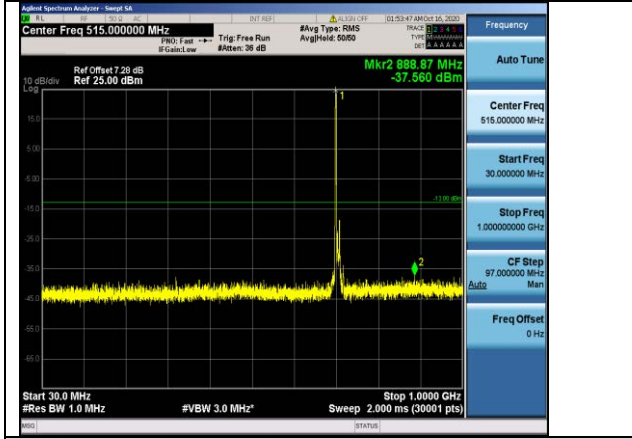
Band17-10MHz-16QAM-23800-1RB#0- Range1:30~1000MHz
