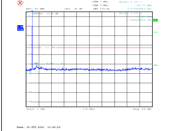
Band2-20MHz-QPSK-19100-1RB#0-Range2:1000~20000MHz--32.37-PASS
