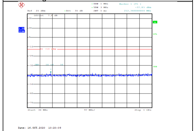
Band2-1.4MHz-QPSK-18900-1RB#0- Range1:30~1000MHz--37.85-PASS
