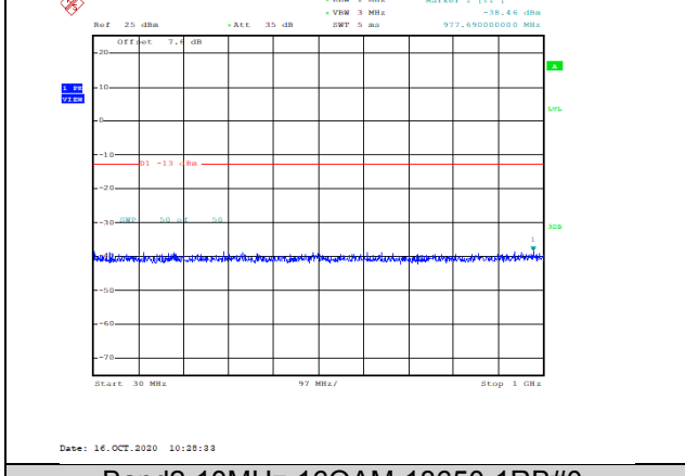
Band2-10MHz-16QAM-18650-1RB#0-Range1:30~1000MHz--38.46-PASS
