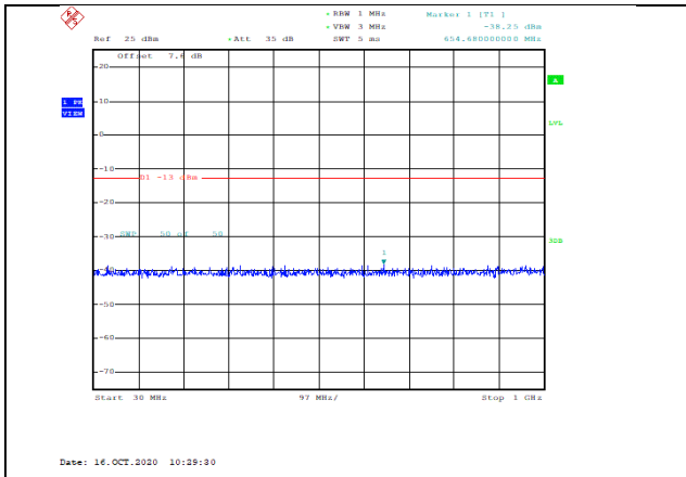
Band2-10MHz-QPSK-19150-1RB#0-Range1:30~1000MHz--38.25-PASS
