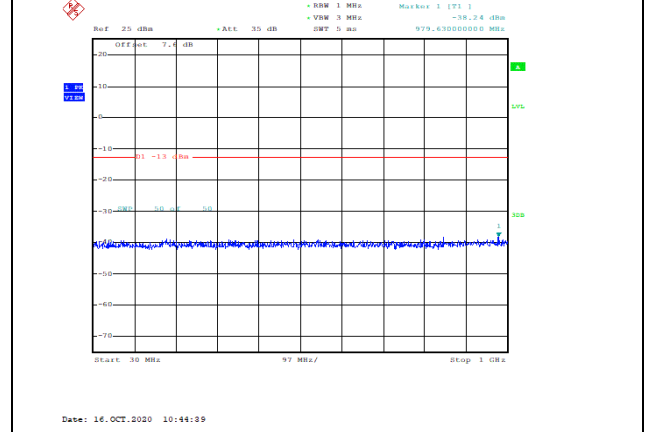
Band4-1.4MHz-QPSK-20175-1RB#0-Range1:30~1000MHz--38.24-PASS
