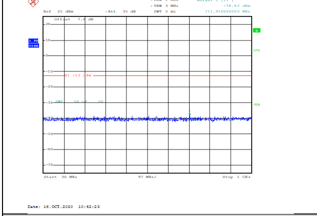
Band2-20MHz-16QAM-18700-1RB#0-Range1:30~1000MHz--38.62-PASS
