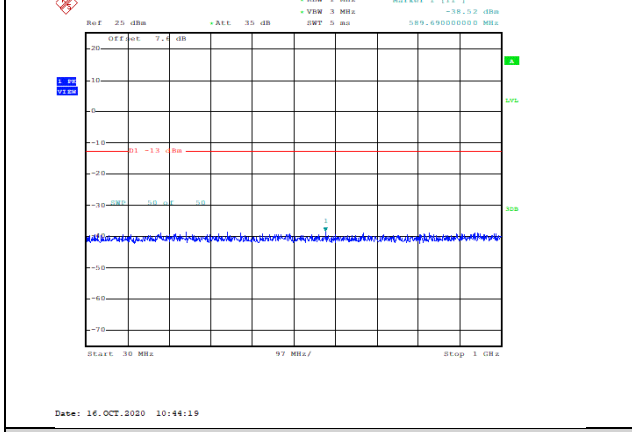
Band4-1.4MHz-16QAM-19957-1RB#0-Range1:30~1000MHz--38.52-PASS
