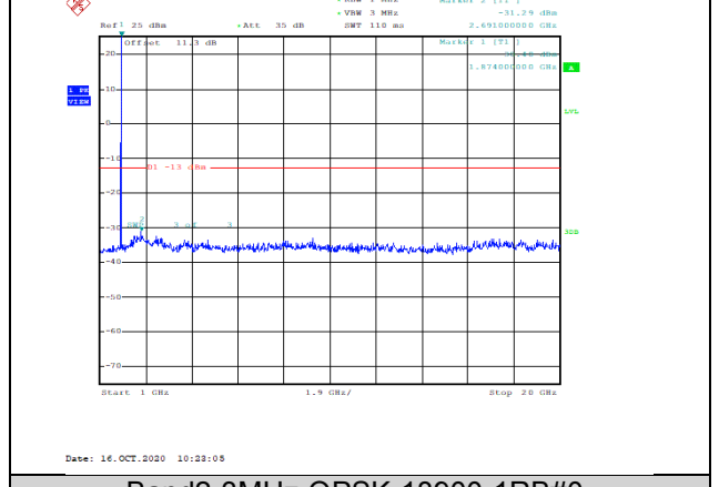
Band2-3MHz-QPSK-18900-1RB#0-Range2:1000~20000MHz--31.29-PASS
