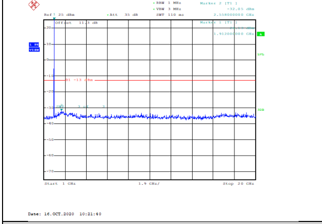
Band2-1.4MHz-16QAM-19193-1RB#0-Range2:1000~20000MHz--32.05-PASS
