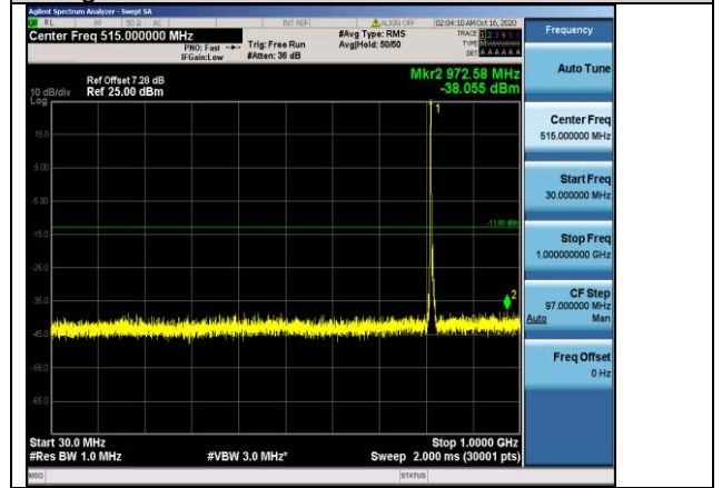
Band26-5MHz-16QAM-26715-1RB#0-Range1:30~1000MHz
