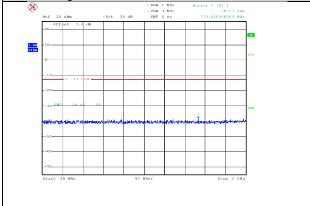
Band4-3MHz-16QAM-19965-1RB#0-Range1:30~1000MHz--38.63-PASS
