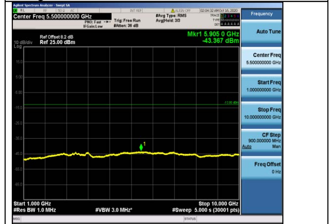
Band26-5MHz-16QAM-26715-1RB#0-Range2:1000~10000MHz
