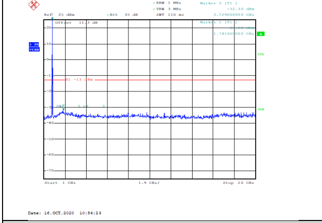
Band4-15MHz-QPSK-20325-1RB#0-Range2:1000~20000MHz--32.3-PASS
