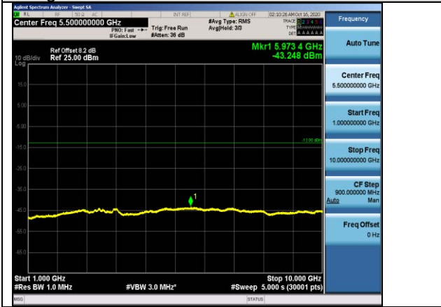
Band26-1.4MHz-16QAM-26740-1RB#0-Range2:1000~10000MHz
