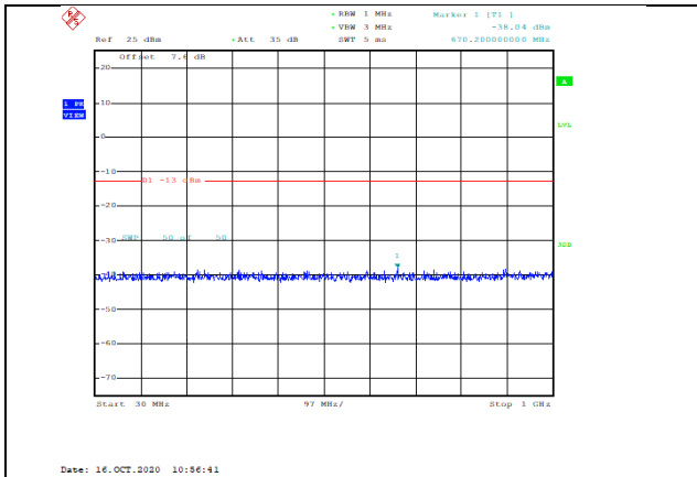
Band4-20MHz-16QAM-20300-1RB#0-Range1:30~1000MHz--38.04-PASS
