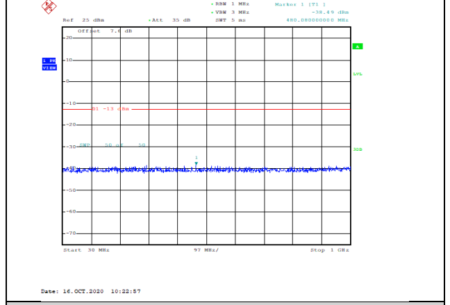
Band2-3MHz-QPSK-18900-1RB#0-Range1:30~1000MHz--38.49-PASS
