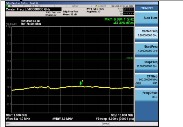
Band26-3MHz-QPSK-26740-1RB#0-Range2:1000~10000MHz
