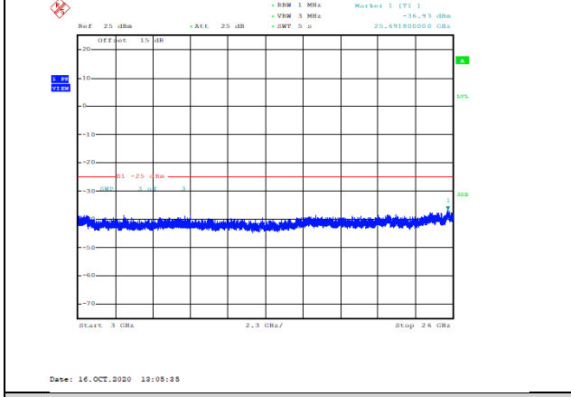
Band7-5MHz-QPSK-21100-1RB#0-Range3:3000~26000MHz--36.93-PASS
