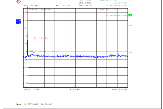
Band4-15MHz-QPSK-20175-1RB#0-Range2:1000~20000MHz--32.28-PASS
