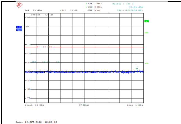
Band2-5MHz-QPSK-19175-1RB#0-Range1:30~1000MHz--37.96-PASS
