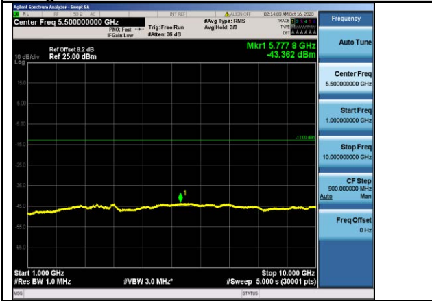
Band26-3MHz-16QAM-26740-1RB#0-Range2:1000~10000MHz
