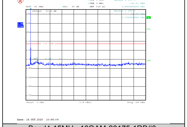
Band4-15MHz-16QAM-20175-1RB#0-Range2:1000~20000MHz--32.01-PASS
