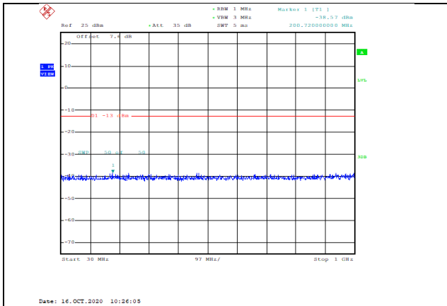
Band2-5MHz-16QAM-19175-1RB#0-Range1:30~1000MHz--38.57-PASS
