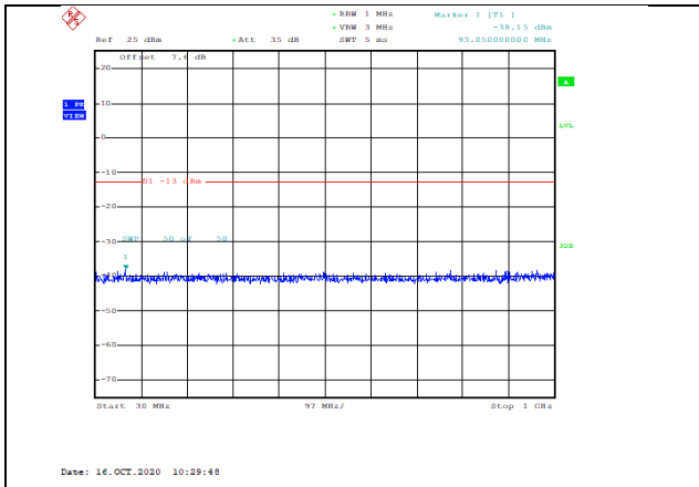
Band2-10MHz-16QAM-19150-1RB#0-Range1:30~1000MHz--38.15-PASS
