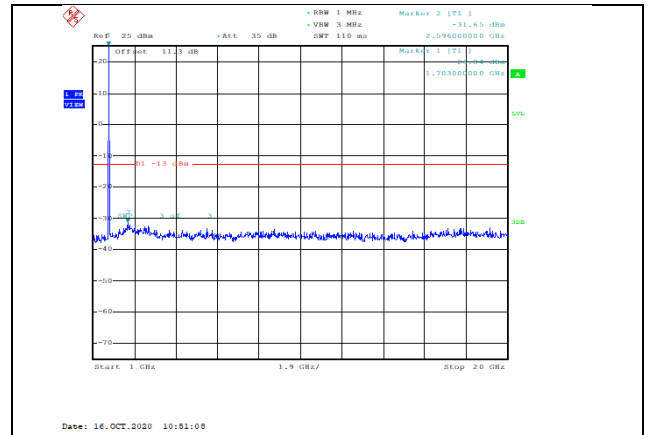
Band4-10MHz-16QAM-20000-1RB#0-Range2:1000~20000MHz--31.65-PASS
