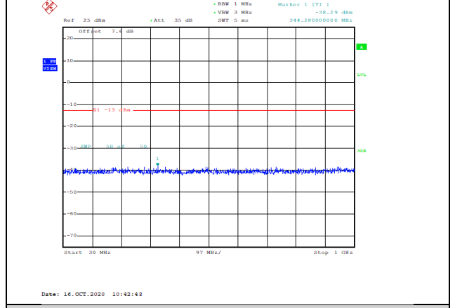
Band2-20MHz-QPSK-18900-1RB#0-Range1:30~1000MHz--38.29-PASS
