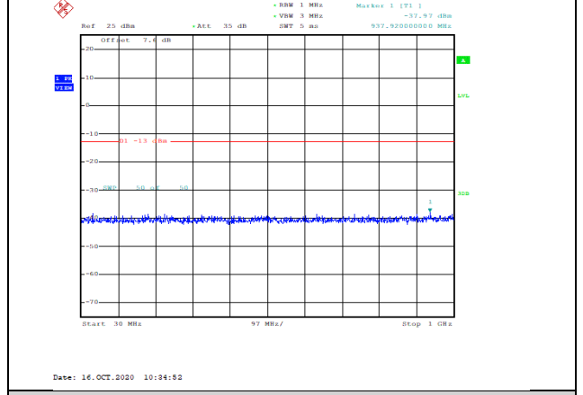
Band2-15MHz-QPSK-18900-1RB#0-Range1:30~1000MHz--37.97-PASS
