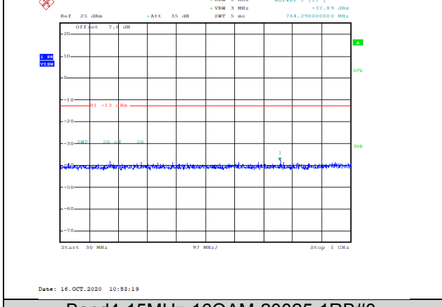
Band4-15MHz-16QAM-20025-1RB#0-Range1:30~1000MHz--37.89-PASS
