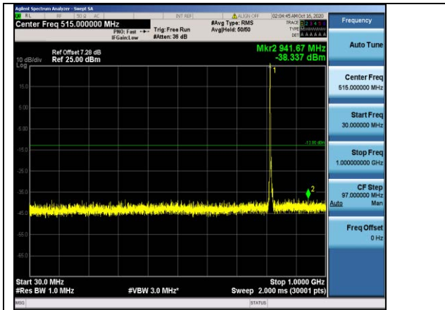
Band26-5MHz-QPSK-26740-1RB#0-Range1:30~1000MHz
