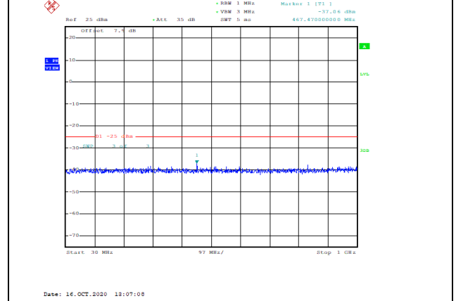
Band7-5MHz-16QAM-21425-1RB#0-Range1:30~1000MHz--37.06-PASS
