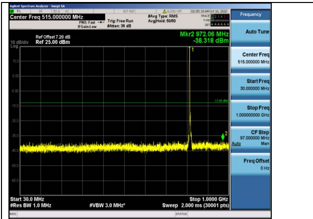
Band26-5MHz-16QAM-26740-1RB#0-Range1:30~1000MHz
