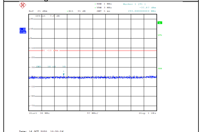
Band2-1.4MHz-16QAM-18900-1RB#0-Range1:30~1000MHz--37.87-PASS
