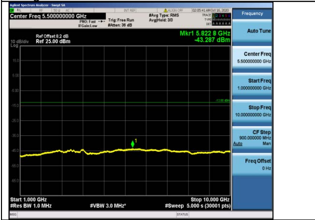
Band26-5MHz-16QAM-26740-1RB#0-Range2:1000~10000MHz
