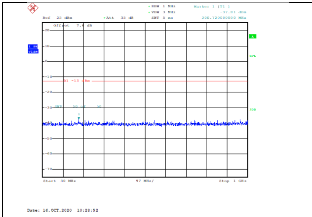
Band2-3MHz-16QAM-19185-1RB#0-Range1:30~1000MHz--37.81-PASS
