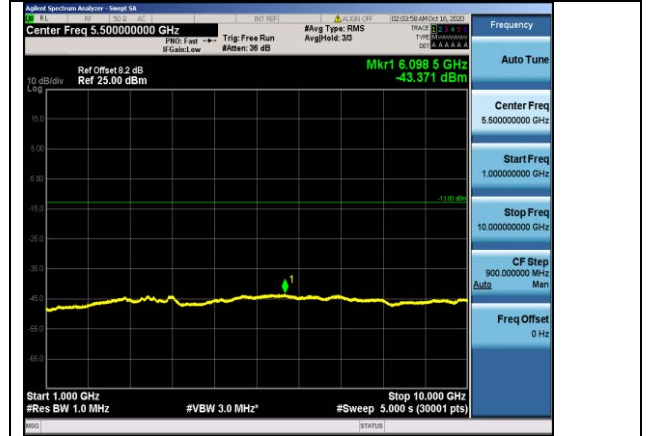
Band26-5MHz-QPSK-26715-1RB#0-Range2:1000~10000MHz
