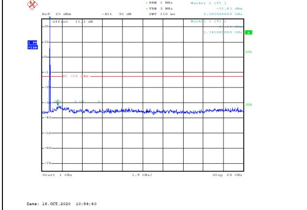
Band4-15MHz-16QAM-20325-1RB#0-Range2:1000~20000MHz--31.85-PASS
