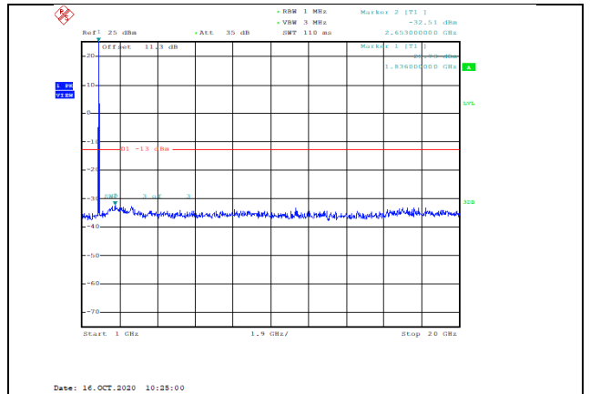
Band2-5MHz-16QAM-18625-1RB#0-Range2:1000~20000MHz--32.51-PASS
