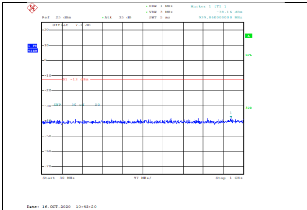
Band2-20MHz-QPSK-19100-1RB#0-Range1:30~1000MHz--38.16-PASS
