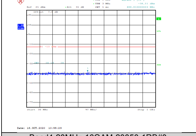
Band4-20MHz-16QAM-20050-1RB#0-Range1:30~1000MHz--38.31-PASS
