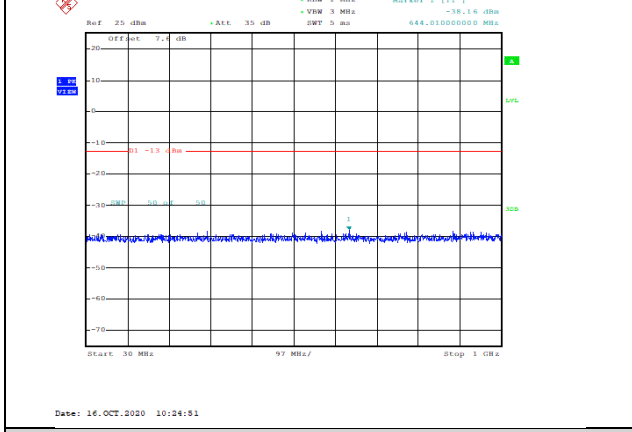
Band2-5MHz-16QAM-18625-1RB#0-Range1:30~1000MHz--38.16-PASS
