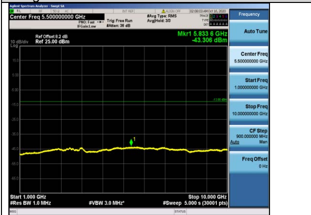
Band26-10MHz-16QAM-26740-1RB#0- Range2:1000~10000MHz
