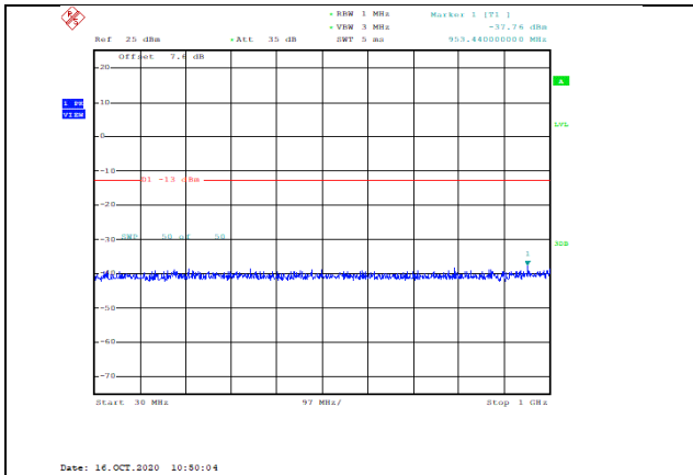
Band4-5MHz-16QAM-20375-1RB#0-Range1:30~1000MHz--37.76-PASS
