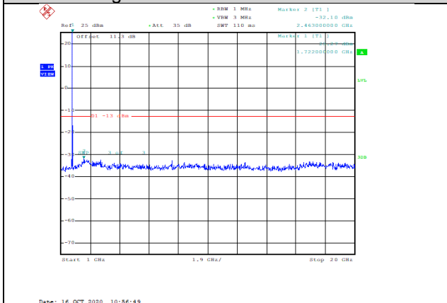
Band4-20MHz-16QAM-20300-1RB#0-Range2:1000~20000MHz--32.1-PASS
