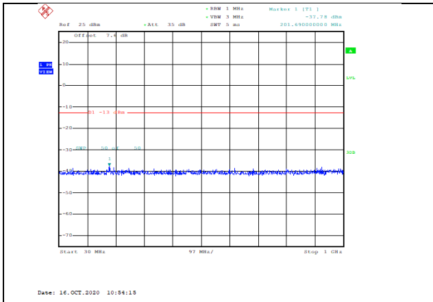
Band4-15MHz-QPSK-20325-1RB#0-Range1:30~1000MHz--37.78-PASS
