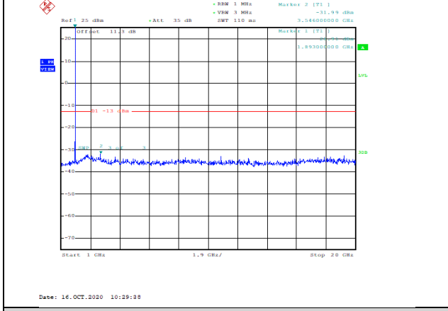
Band2-10MHz-QPSK-19150-1RB#0-Range2:1000~20000MHz--31.99-PASS
