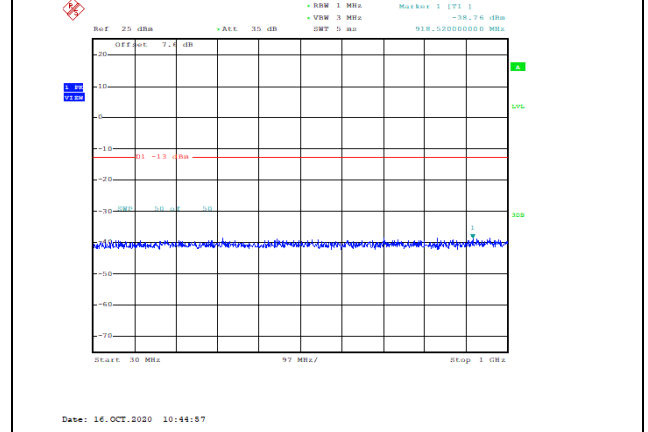
Band4-1.4MHz-16QAM-20175-1RB#0-Range1:30~1000MHz--38.76-PASS
