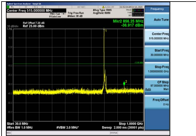
Band17-10MHz-QPSK-23790-1RB#0-Range1:30~1000MHz
