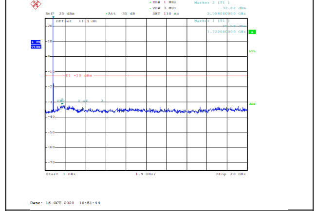
Band4-10MHz-16QAM-20175-1RB#0-Range2:1000~20000MHz--32.02-PASS
