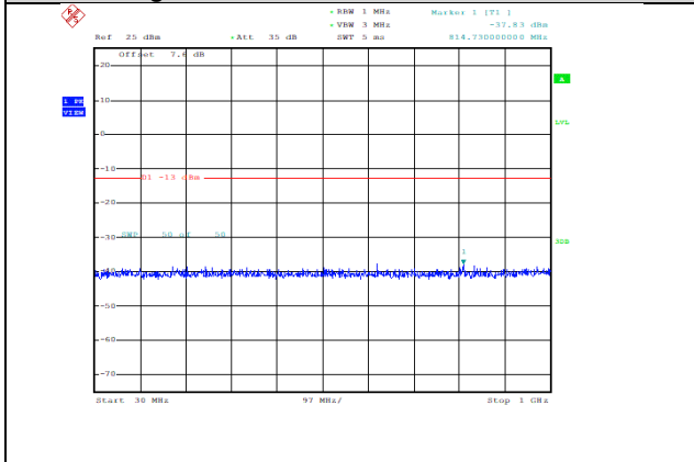
Band4-5MHz-16QAM-19975-1RB#0-Range1:30~1000MHz--37.83-PASS
