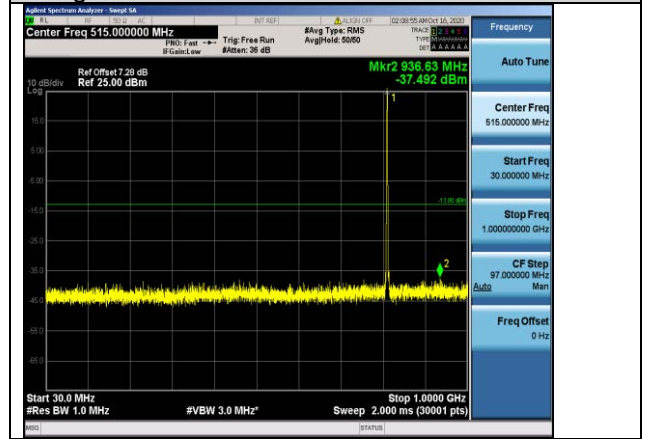
Band26-1.4MHz-16QAM-26697-1RB#0-Range1:30~1000MHz
