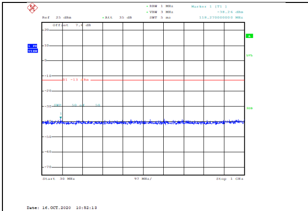
Band4-10MHz-16QAM-20350-1RB#0-Range1:30~1000MHz--38.26-PASS
