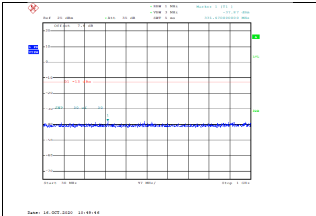
Band4-5MHz-QPSK-20375-1RB#0-Range1:30~1000MHz--37.87-PASS
