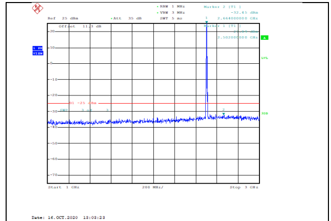
Band7-5MHz-QPSK-20775-1RB#0-Range2:1000~3000MHz--32.45-PASS
