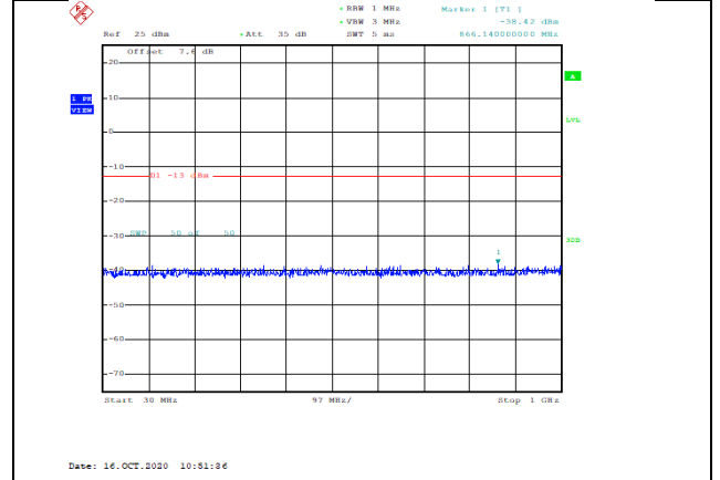
Band4-10MHz-16QAM-20175-1RB#0-Range1:30~1000MHz--38.42-PASS
