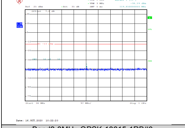
Band2-3MHz-QPSK-18615-1RB#0-Range1:30~1000MHz--38.39-PASS
