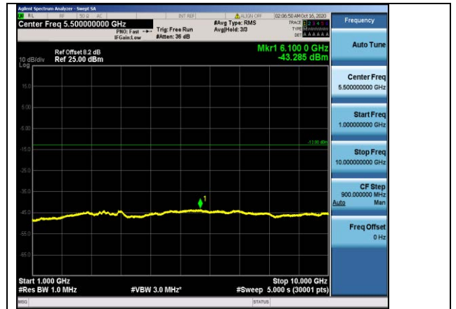
Band26-5MHz-16QAM-26765-1RB#0-Range2:1000~10000MHz
