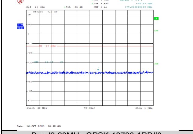
Band2-20MHz-QPSK-18700-1RB#0-Range1:30~1000MHz--38.45-PASS
