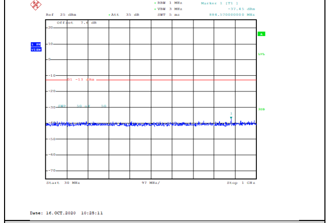
Band2-5MHz-QPSK-18900-1RB#0-Range1:30~1000MHz--37.45-PASS
