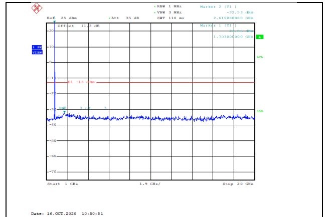
Band4-10MHz-QPSK-20000-1RB#0-Range2:1000~20000MHz--32.53-PASS
