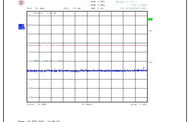
Band4-5MHz-16QAM-20175-1RB#0-Range1:30~1000MHz--38.19-PASS
