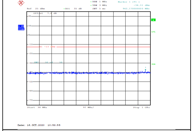
Band4-15MHz-16QAM-20175-1RB#0-Range1:30~1000MHz--38.31-PASS
