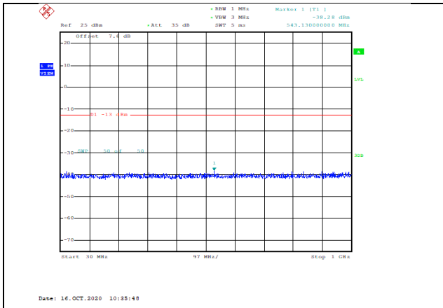
Band2-15MHz-16QAM-19125-1RB#0-Range1:30~1000MHz--38.28-PASS
