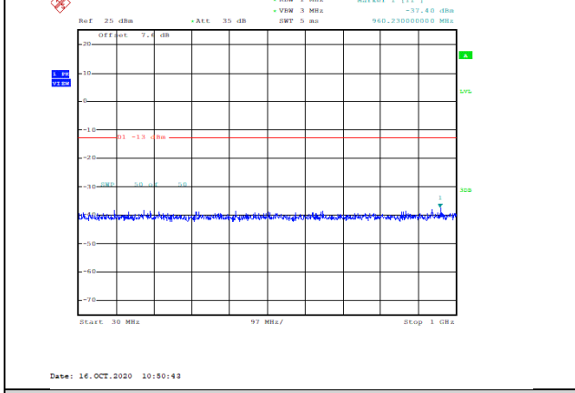
Band4-10MHz-QPSK-20000-1RB#0-Range1:30~1000MHz--37.4-PASS
