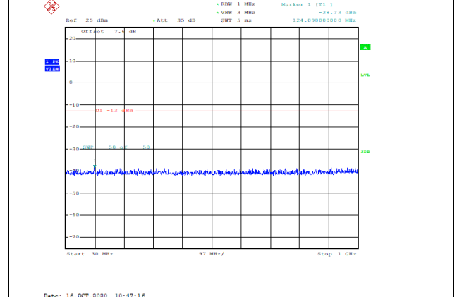
Band4-3MHz-16QAM-20175-1RB#0-Range1:30~1000MHz--38.73-PASS
