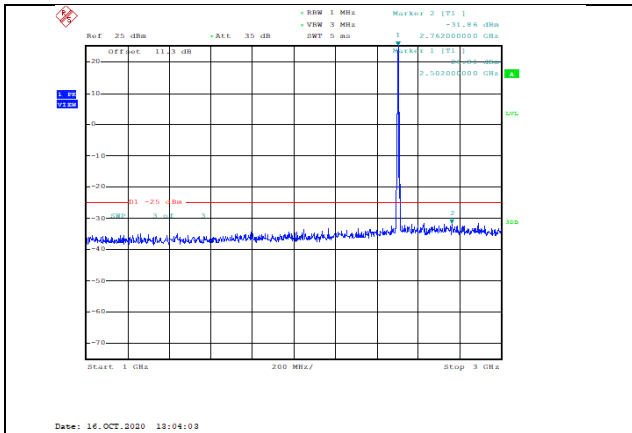
Band7-5MHz-16QAM-20775-1RB#0-Range2:1000~3000MHz--31.86-PASS
