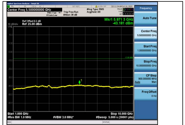
Band26-1.4MHz-16QAM-26783-1RB#0-Range2:1000~10000MHz
