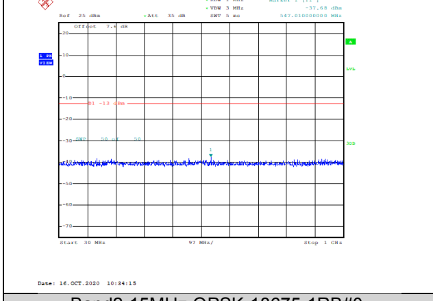
Band2-15MHz-QPSK-18675-1RB#0-Range1:30~1000MHz--37.68-PASS
