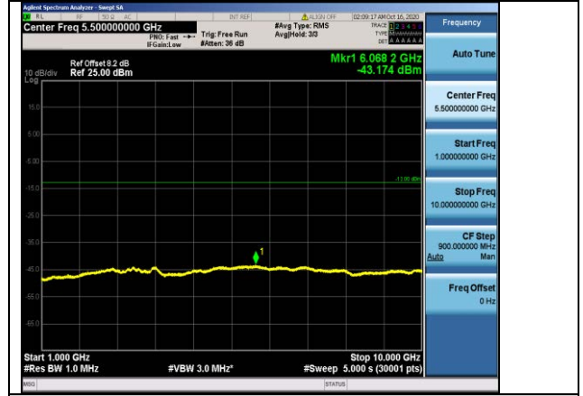
Band26-1.4MHz-16QAM-26697-1RB#0-Range2:1000~10000MHz
