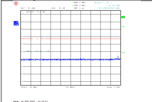
Band2-1.4MHz-16QAM-18607-1RB#0-Range1:30~1000MHz--37.88-PASS
