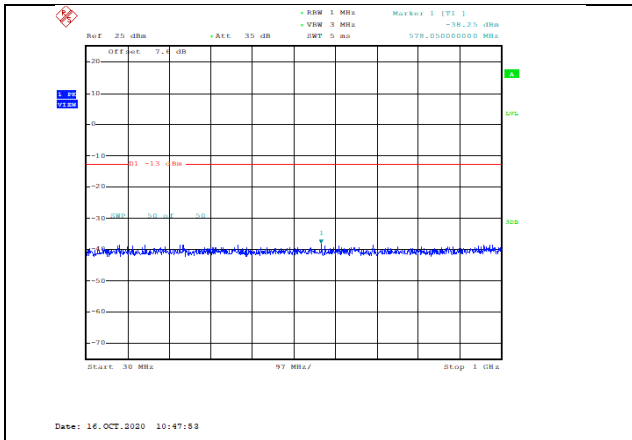
Band4-3MHz-16QAM-20385-1RB#0-Range1:30~1000MHz--38.25-PASS
