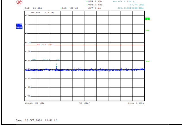
Band4-10MHz-16QAM-20000-1RB#0-Range1:30~1000MHz--37.74-PASS
