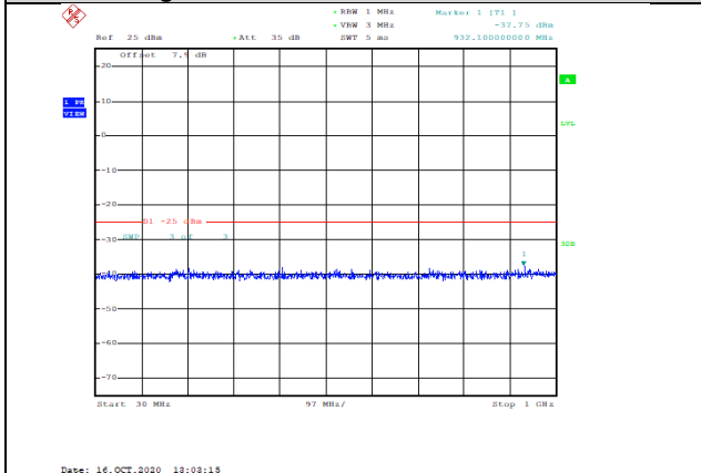
Band7-5MHz-QPSK-20775-1RB#0-Range1:30~1000MHz--37.75-PASS
