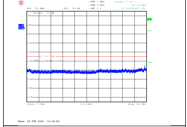
Band7-5MHz-QPSK-21425-1RB#0-Range3:3000~26000MHz--36.28-PASS
