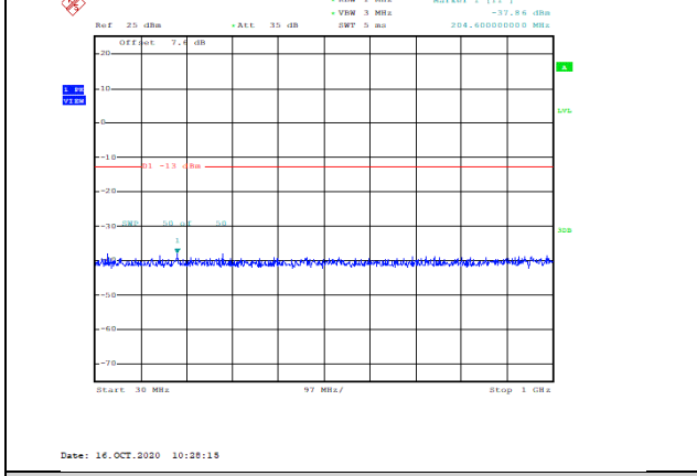
Band2-10MHz-QPSK-18650-1RB#0-Range1:30~1000MHz--37.86-PASS
