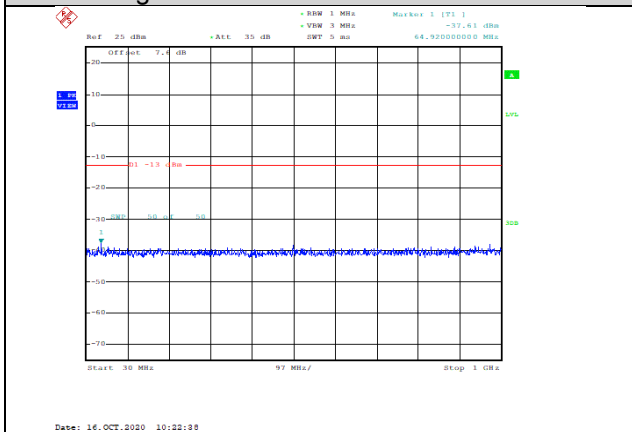
Band2-3MHz-16QAM-18615-1RB#0-Range1:30~1000MHz--37.61-PASS
