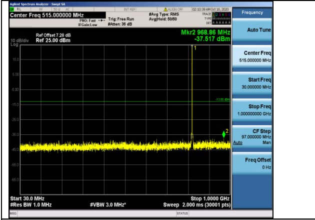
Band26-1.4MHz-QPSK-26783-1RB#0-Range1:30~1000MHz
