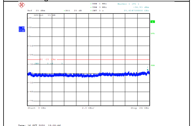
Band7-5MHz-QPSK-20775-1RB#0-Range3:3000~26000MHz--36.95-PASS
