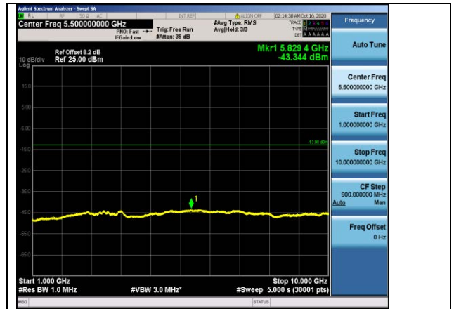
Band26-3MHz-QPSK-26775-1RB#0-Range2:1000~10000MHz
