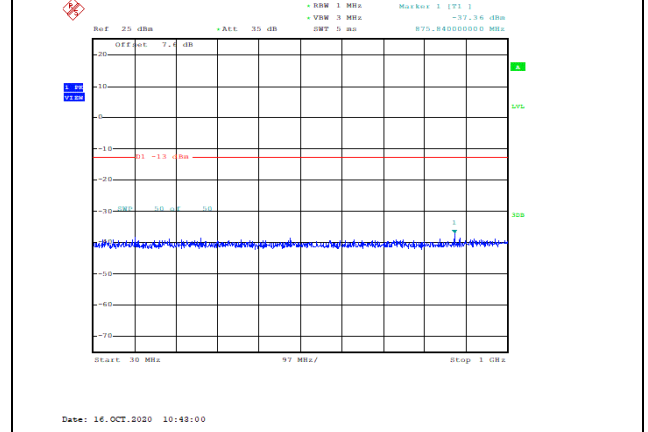
Band2-20MHz-16QAM-18900-1RB#0-Range1:30~1000MHz--37.36-PASS
