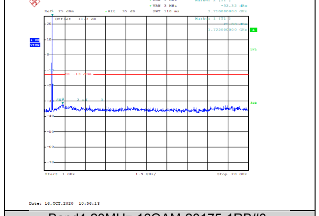
Band4-20MHz-16QAM-20175-1RB#0-Range2:1000~20000MHz--32.32-PASS
