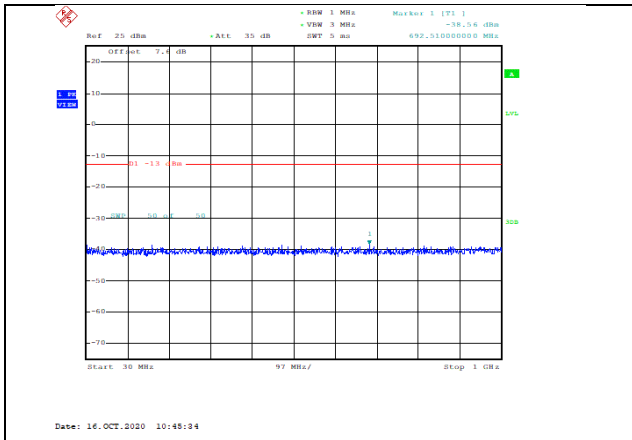
Band4-1.4MHz-16QAM-20393-1RB#0-Range1:30~1000MHz--38.56-PASS
