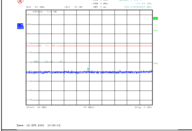
Band4-15MHz-QPSK-20025-1RB#0-Range1:30~1000MHz--37.93-PASS
