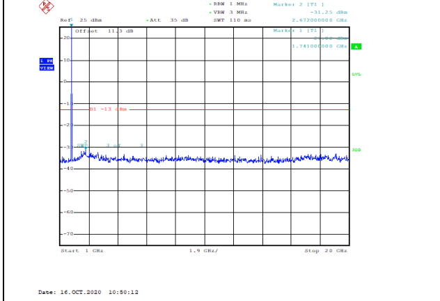
Band4-5MHz-16QAM-20375-1RB#0-Range2:1000~20000MHz--31.25-PASS
