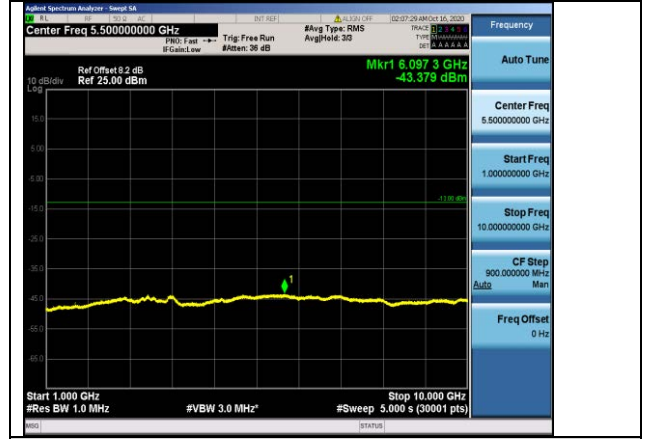
Band26-10MHz-QPSK-26740-1RB#0-Range2:1000~10000MHz
