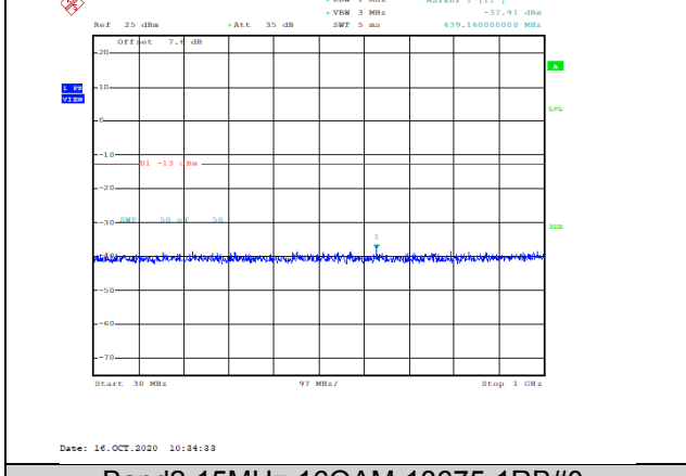
Band2-15MHz-16QAM-18675-1RB#0-Range1:30~1000MHz--37.91-PASS
