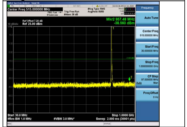
Band26-5MHz-QPSK-26715-1RB#0-Range1:30~1000MHz
