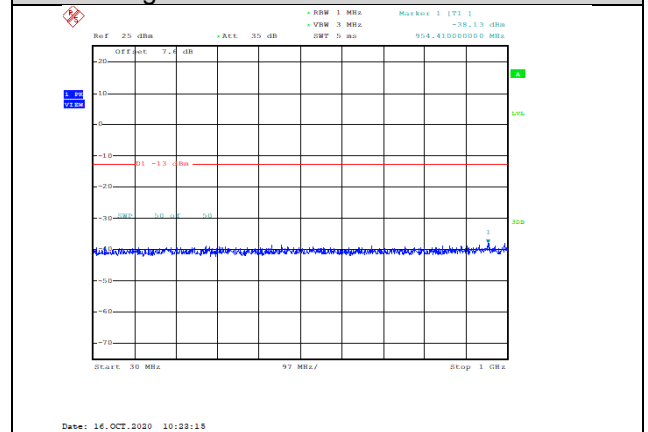
Band2-3MHz-16QAM-18900-1RB#0-Range1:30~1000MHz--38.13-PASS
