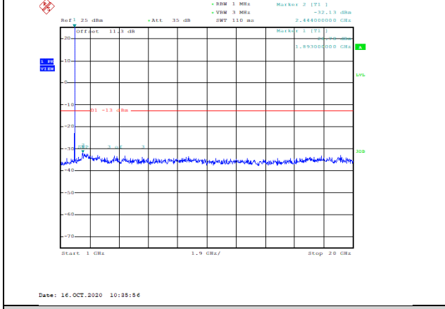
Band2-15MHz-16QAM-19125-1RB#0-Range2:1000~20000MHz--32.13-PASS
