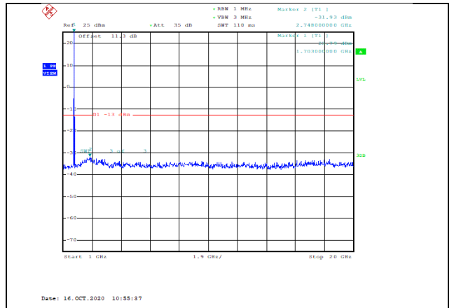
Band4-20MHz-16QAM-20050-1RB#0-Range2:1000~20000MHz--31.93-PASS
