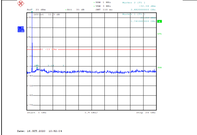
Band4-10MHz-QPSK-20350-1RB#0-Range2:1000~20000MHz--32.38-PASS
