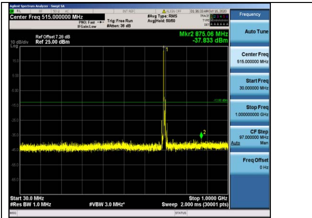
Band12-5MHz-QPSK-23035-1RB#0-Range1:30~1000MHz
