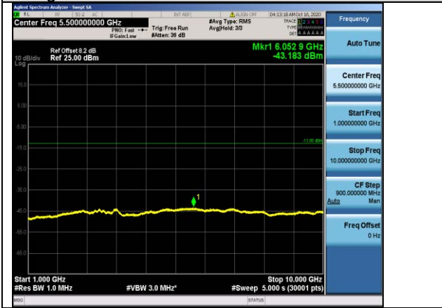
Band5-5MHz-QPSK-20425-1RB#0-Range2:1000~10000MHz
