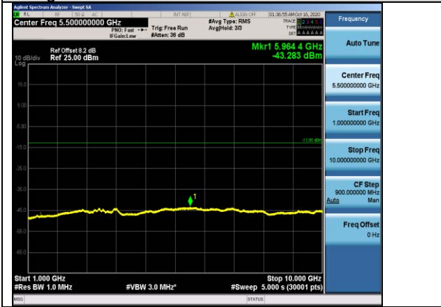
Band12-5MHz-QPSK-23035-1RB#0-Range2:1000~10000MHz
