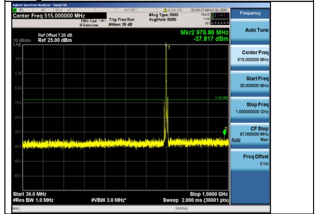
Band17-5MHz-QPSK-23755-1RB#0-Range1:30~1000MHz
