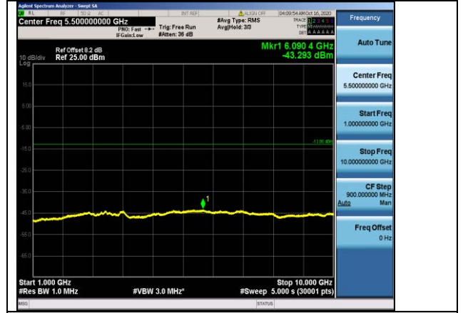
Band5-3MHz-16QAM-20635-1RB#0-Range2:1000~10000MHz
