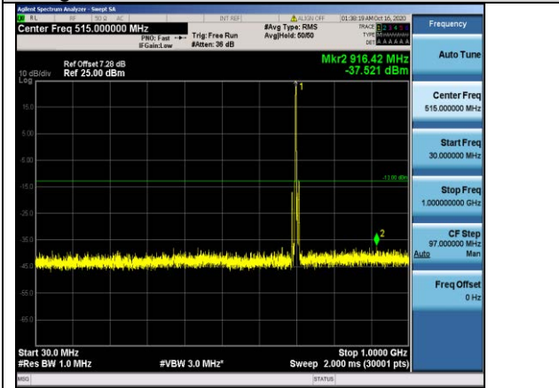
Band12-5MHz-16QAM-23095-1RB#0-Range1:30~1000MHz
