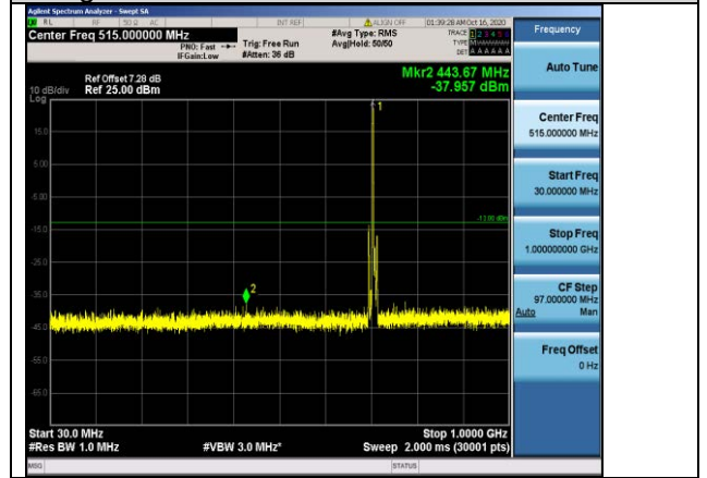
Band12-5MHz-16QAM-23155-1RB#0-Range1:30~1000MHz
