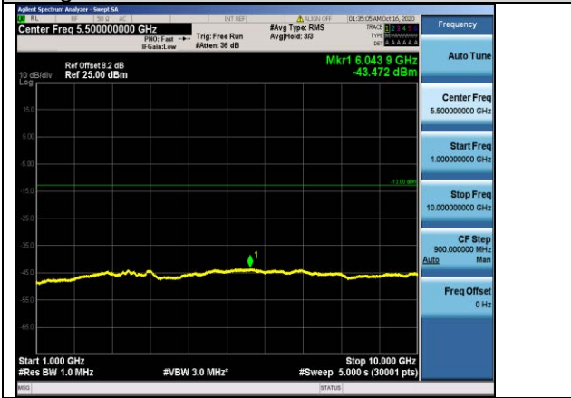
Band12-10MHz-16QAM-23095-1RB#0-Range2:1000~10000MHz
