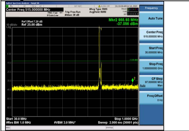
Band12-10MHz-QPSK-23060-1RB#0-Range1:30~1000MHz
