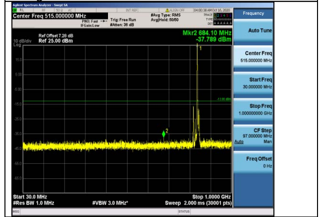
Band5-10MHz-QPSK-20600-1RB#0-Range1:30~1000MHz
