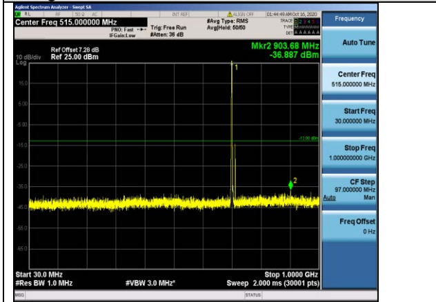
Band12-1.4MHz-QPSK-23095-1RB#0-Range1:30~1000MHz
