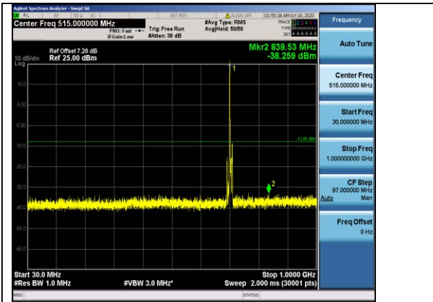
Band17-5MHz-QPSK-23790-1RB#0-Range1:30~1000MHz
