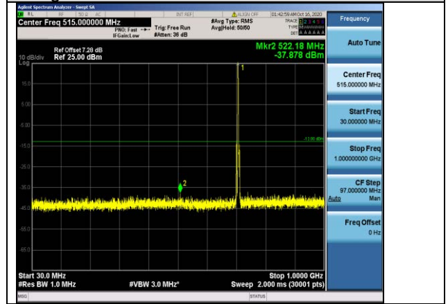
Band12-3MHz-16QAM-23165-1RB#0-Range1:30~1000MHz
