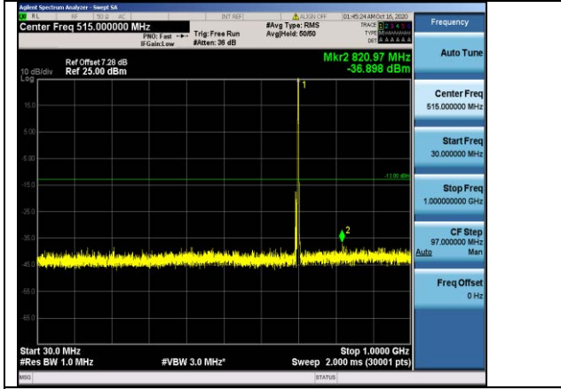
Band12-1.4MHz-16QAM-23095-1RB#0-Range1:30~1000MHz
