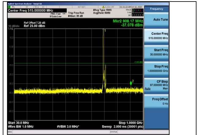
Band12-10MHz-16QAM-23060-1RB#0-Range2:30~1000MHz
