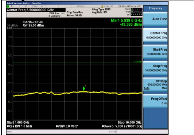
Band12-10MHz-QPSK-23130-1RB#0-Range2:1000~10000MHz
