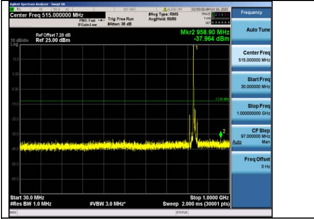
Band5-10MHz-QPSK-20525-1RB#0-Range1:30~1000MHz
