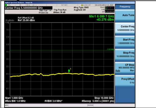
Band5-5MHz-16QAM-20425-1RB#0-Range2:1000~10000MHz
