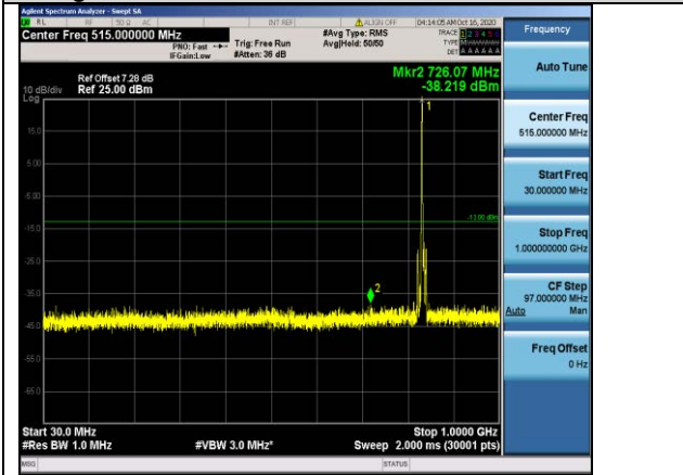
Band5-5MHz-QPSK-20525-1RB#0-Range1:30~1000MHz
