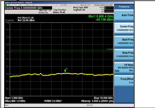
Band5-10MHz-QPSK-20450-1RB#0-Range2:1000~10000MHz
