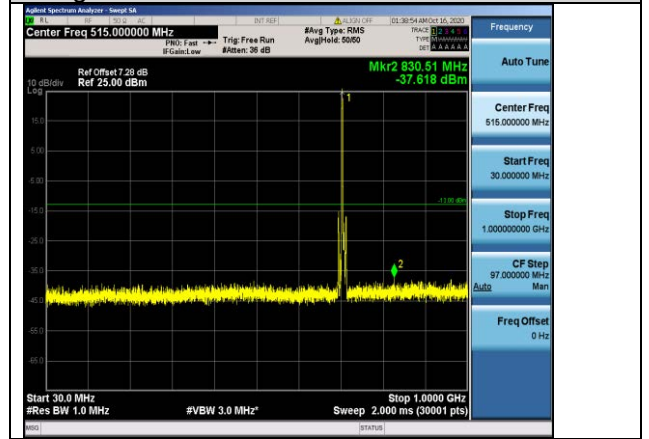
Band12-5MHz-QPSK-23095-1RB#0-Range1:30~1000MHz
