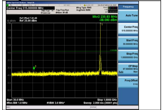
Band5-5MHz-16QAM-20625-1RB#0-Range1:30~1000MHz
