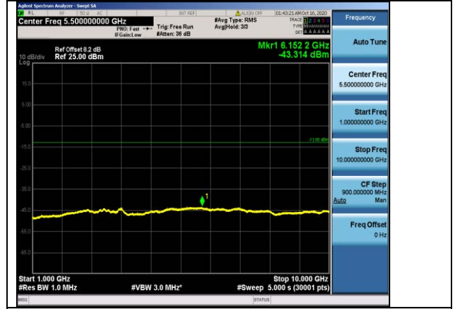
Band12-3MHz-16QAM-23165-1RB#0-Range2:1000~10000MHz
