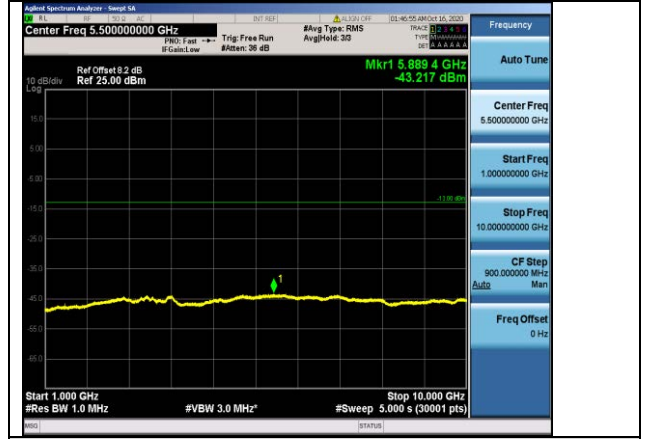
Band12-1.4MHz-16QAM-23173-1RB#0-Range2:1000~10000MHz
