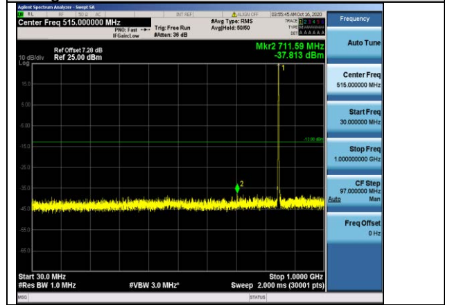
Band5-1.4MHz-16QAM-20643-1RB#0-Range1:30~1000MHz
