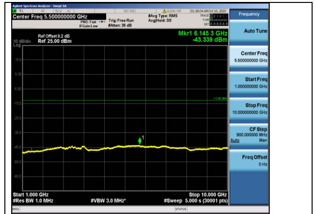
Band12-5MHz-QPSK-23095-1RB#0-Range2:1000~10000MHz
