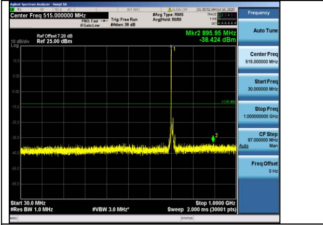
Band12-10MHz-16QAM-23130-1RB#0-Range1:30~1000MHz
