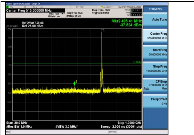
Band12-5MHz-16QAM-23035-1RB#0-Range1:30~1000MHz
