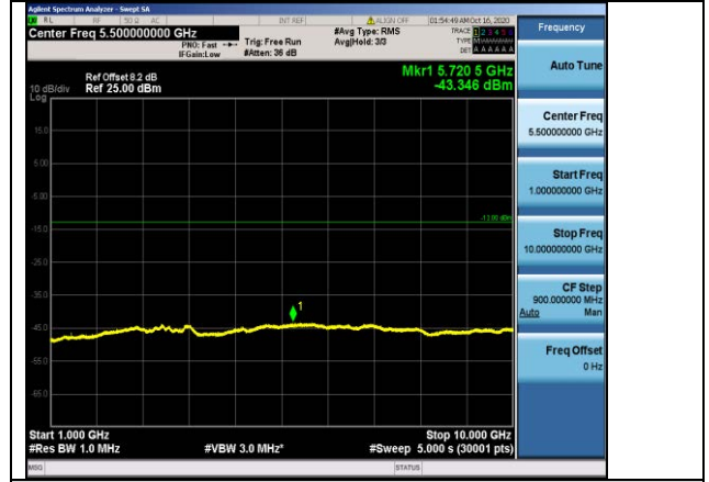
Band17-5MHz-QPSK-23755-1RB#0-Range2:1000~10000MHz
