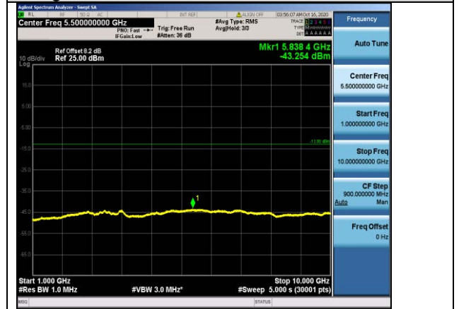
Band5-1.4MHz-16QAM-20643-1RB#0-Range2:1000~10000MHz
