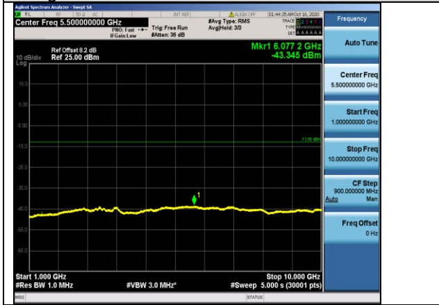
Band12-1.4MHz-16QAM-23017-1RB#0-Range2:1000~10000MHz
