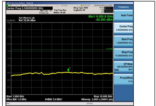
Band5-10MHz-QPSK-20525-1RB#0-Range2:1000~10000MHz
