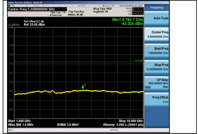
Band5-10MHz-QPSK-20600-1RB#0-Range2:1000~10000MHz
