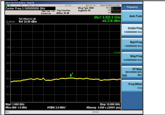
Band5-3MHz-16QAM-20525-1RB#0-Range2:1000~10000MHz
