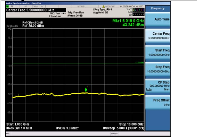
Band17-5MHz-QPSK-23790-1RB#0-Range2:1000~10000MHz
