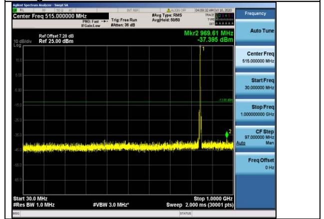
Band5-3MHz-16QAM-20635-1RB#0-Range1:30~1000MHz
