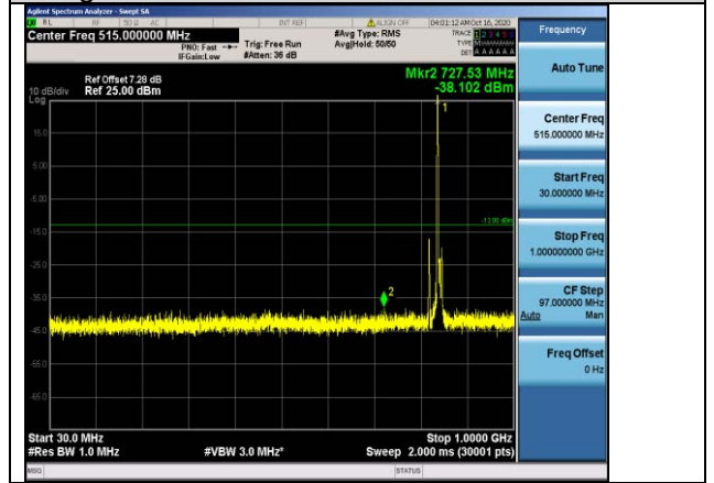
Band5-10MHz-16QAM-20600-1RB#0-Range1:30~1000MHz
