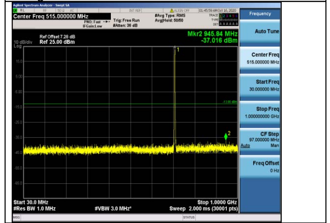
Band12-1.4MHz-QPSK-23173-1RB#0-Range1:30~1000MHz
