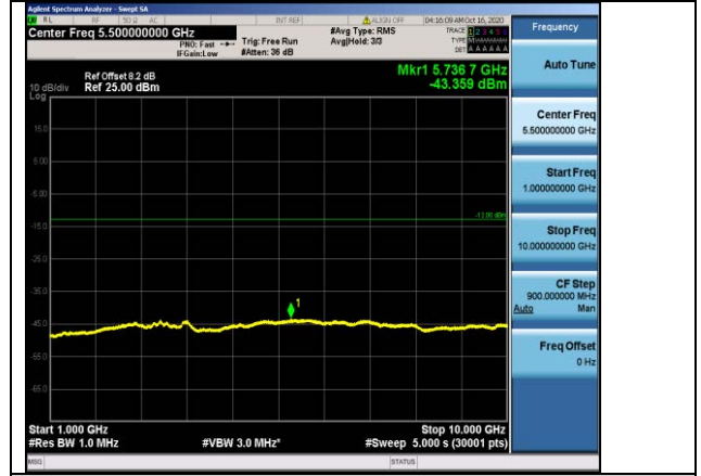
Band5-5MHz-16QAM-20625-1RB#0-Range2:1000~10000MHz
