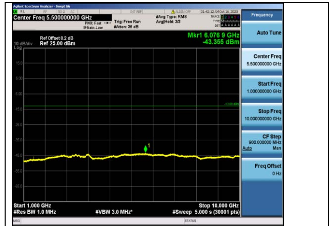
Band12-3MHz-16QAM-23095-1RB#0-Range2:1000~10000MHz
