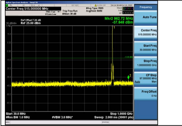
Band5-5MHz-16QAM-20525-1RB#0-Range1:30~1000MHz
