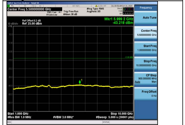
Band12-5MHz-16QAM-23155-1RB#0-Range2:1000~10000MHz
