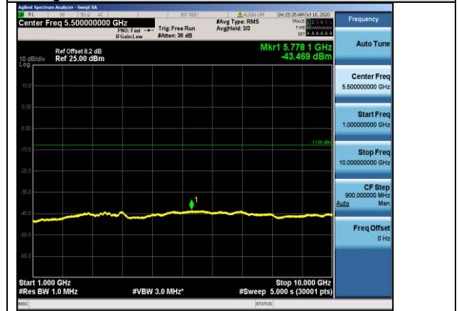
Band5-5MHz-QPSK-20625-1RB#0-Range2:1000~10000MHz
