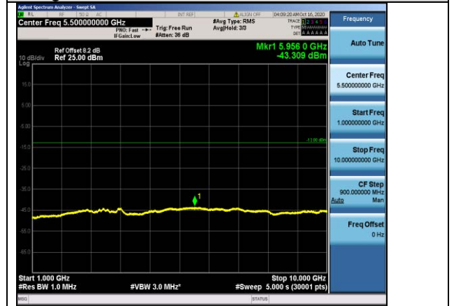
Band5-3MHz-QPSK-20635-1RB#0- Range2:1000~10000MHz
