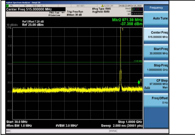
Band5-3MHz-16QAM-20525-1RB#0-Range1:30~1000MHz
