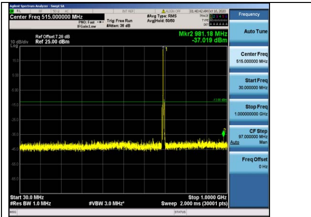
Band12-3MHz-16QAM-23025-1RB#0-Range1:30~1000MHz
