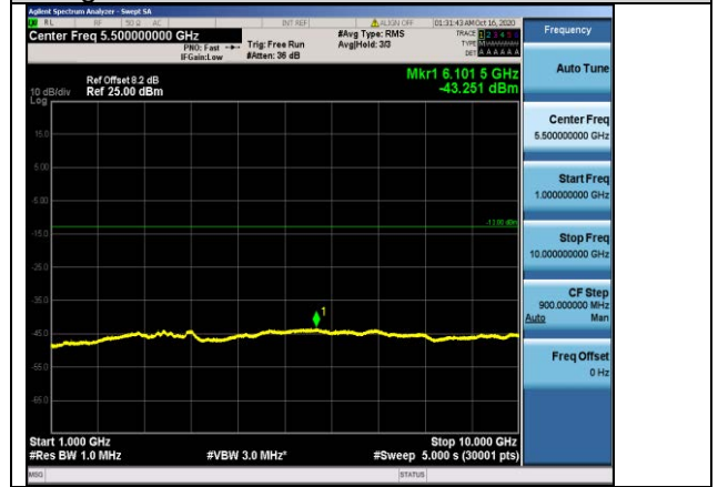
Band12-10MHz-16QAM-23060-1RB#0-Range3:1000~10000MHz
