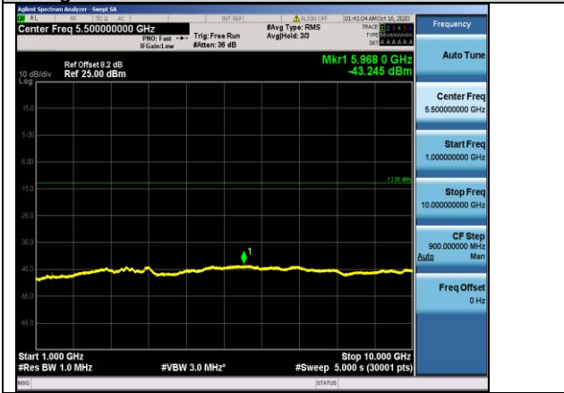
Band12-3MHz-16QAM-23025-1RB#0-Range2:1000~10000MHz
