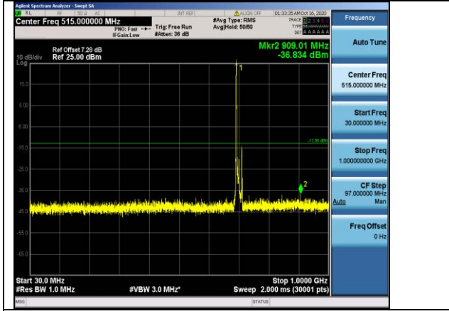
Band12-10MHz-16QAM-23060-1RB#0-Range1:30~1000MHz
