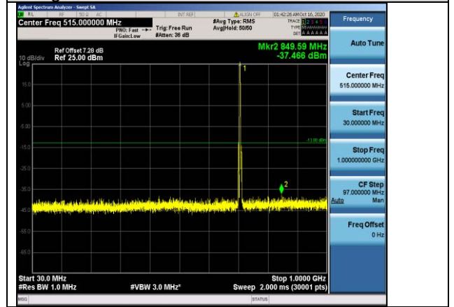
Band12-3MHz-QPSK-23095-1RB#0-Range1:30~1000MHz
