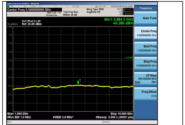
Band5-10MHz-16QAM-20525-1RB#0-Range2:1000~10000MHz
