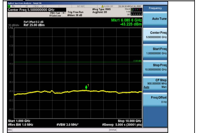
Band12-10MHz-QPSK-23095-1RB#0-Range2:1000~10000MHz
