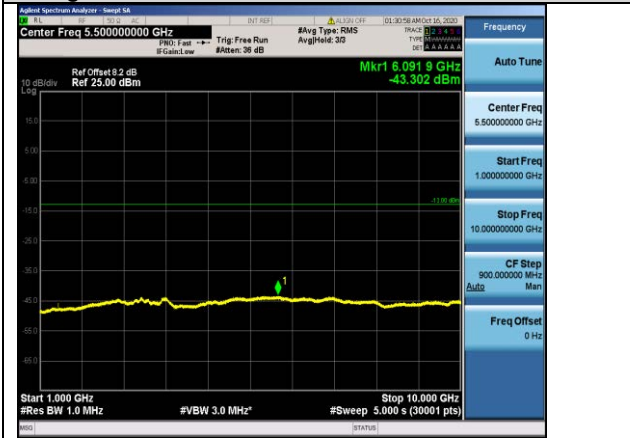
Band12-10MHz-QPSK-23060-1RB#0-Range3:1000~10000MHz
