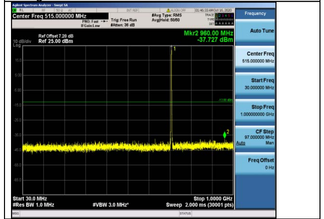
Band12-1.4MHz-16QAM-23173-1RB#0-Range1:30~1000MHz
