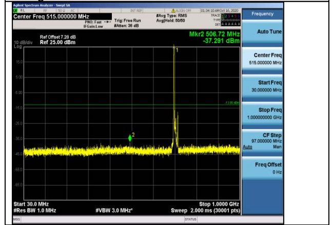
Band12-10MHz-QPSK-23095-1RB#0-Range1:30~1000MHz
