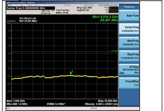
Band5-10MHz-16QAM-20600-1RB#0-Range2:1000~10000MHz
