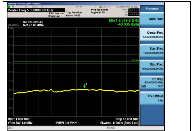
Band12-5MHz-16QAM-23095-1RB#0-Range2:1000~10000MHz
