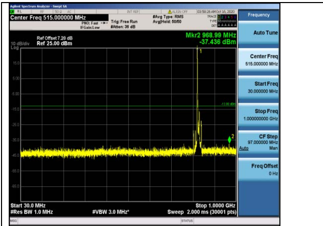
Band5-10MHz-16QAM-20450-1RB#0-Range1:30~1000MHz
