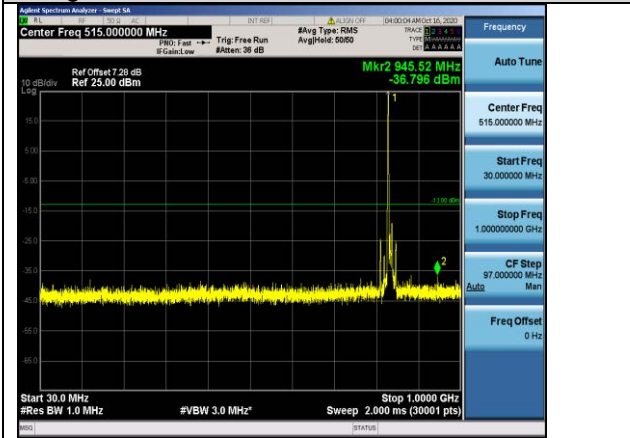
Band5-10MHz-16QAM-20525-1RB#0-Range1:30~1000MHz
