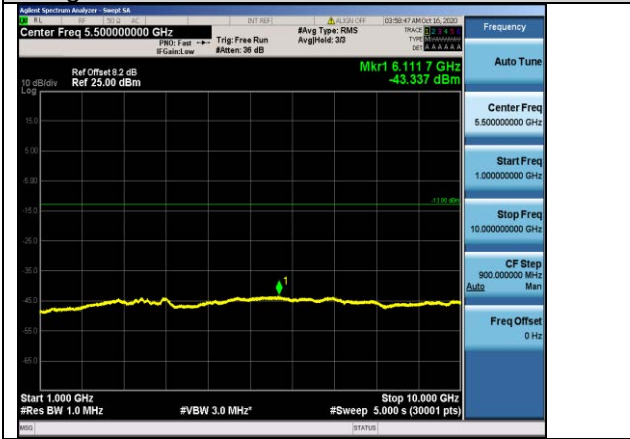
Band5-10MHz-16QAM-20450-1RB#0-Range2:1000~10000MHz
