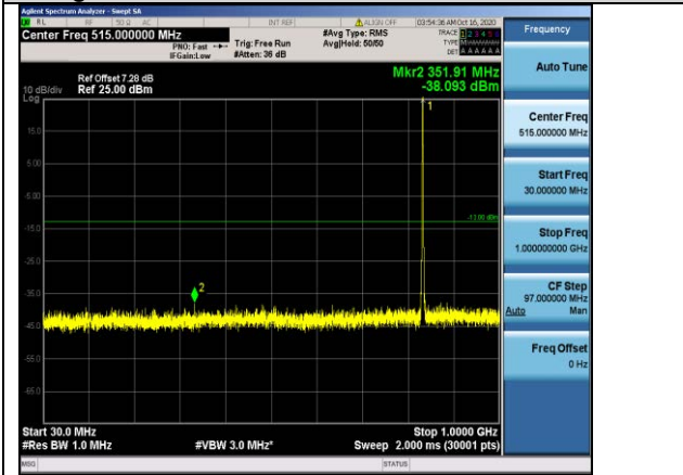
Band5-1.4MHz-16QAM-20643-1RB#0-Range1:30~1000MHz
