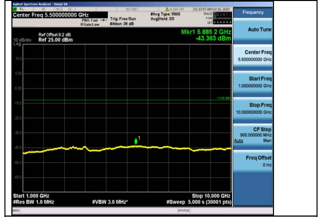
Band12-10MHz-16QAM-23060-1RB#0-Range2:1000~10000MHz
