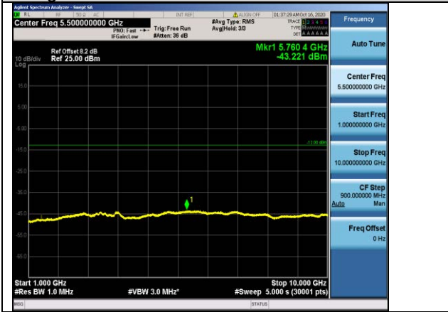
Band12-5MHz-16QAM-23035-1RB#0-Range2:1000~10000MHz
