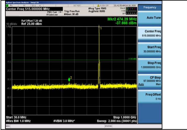
Band12-3MHz-16QAM-23095-1RB#0-Range1:30~1000MHz
