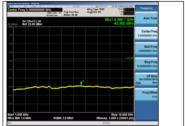
Band12-10MHz-16QAM-23130-1RB#0-Range2:1000~10000MHz
