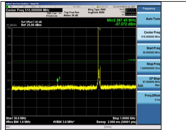
Band12-10MHz-16QAM-23095-1RB#0-Range1:30~1000MHz
