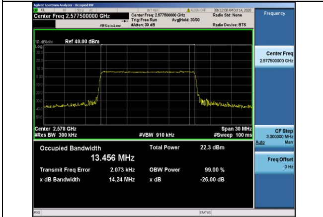
Band38-15MHz-16QAM-37825-75RB#0-13.456
