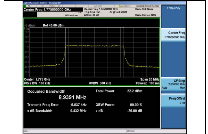
Band66-10MHz-16QAM-132622-50RB#0-8.9391
