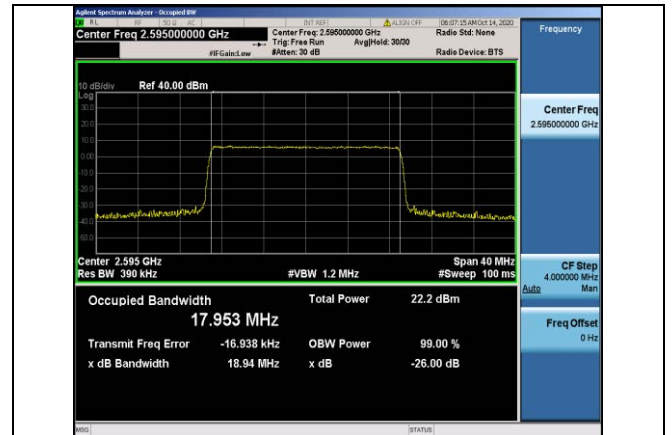
Band38-20MHz-16QAM-38000-100RB#0-17.953
