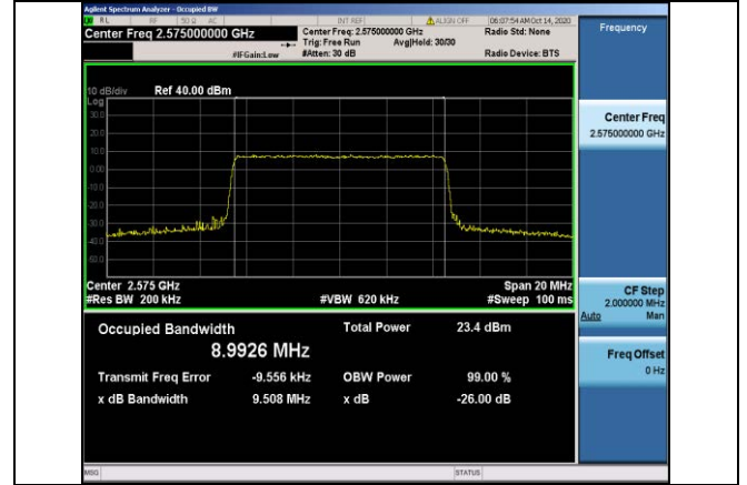
Band38-10MHz-QPSK-37800-50RB#0-8.9926
