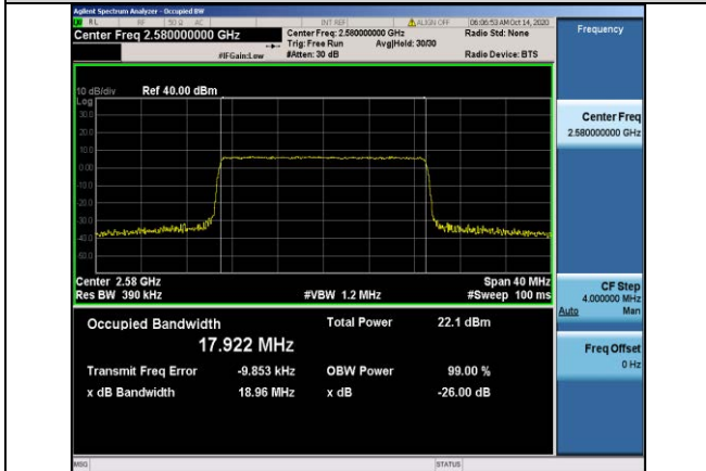
Band38-20MHz-16QAM-37850-100RB#0-17.922
