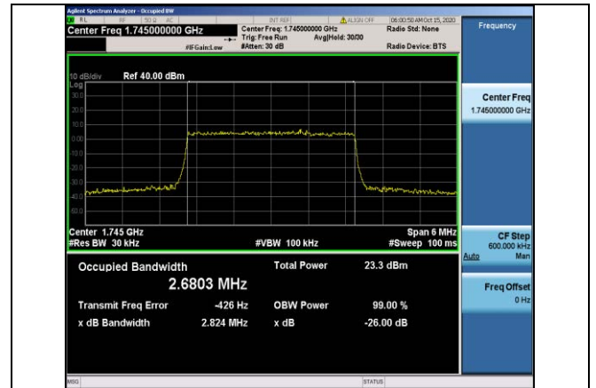
Band66-3MHz-16QAM-132322-15RB#0-2.6803
