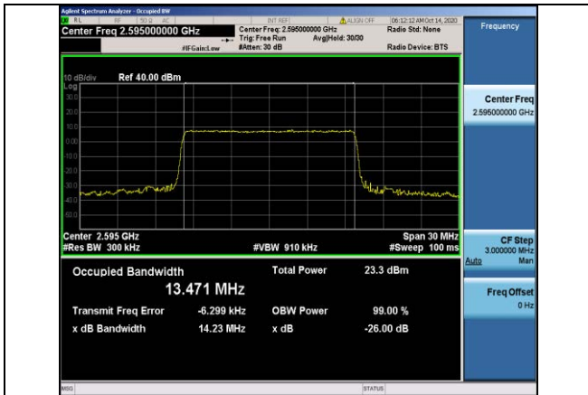
Band38-15MHz-QPSK-38000-75RB#0-13.471
