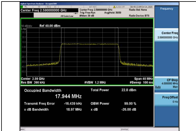
Band41-20MHz-QPSK-40590-100RB#0-17.944
