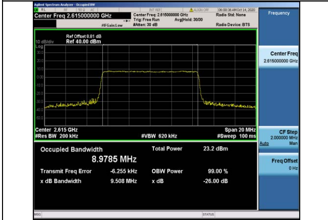
Band38-10MHz-QPSK-38200-50RB#0-8.9785
