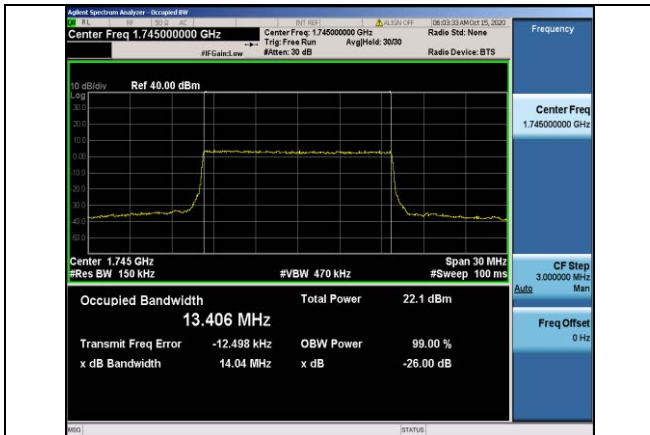
Band66-15MHz-QPSK-132322-75RB#0-13.406
