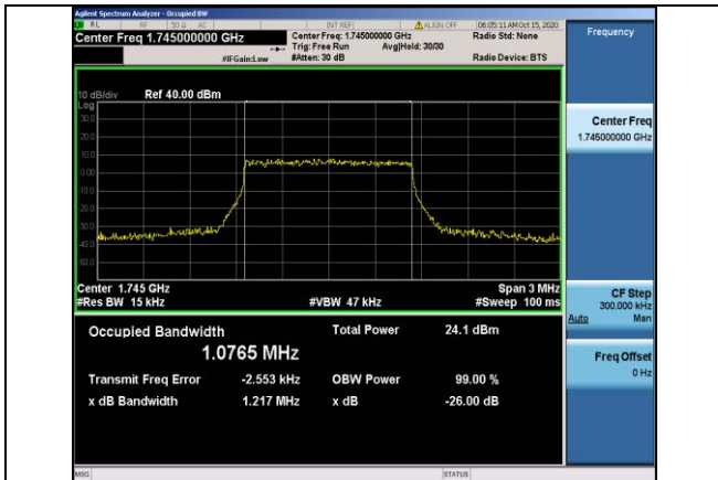
Band66-1.4MHz-QPSK-132322-6RB#0-1.0765
