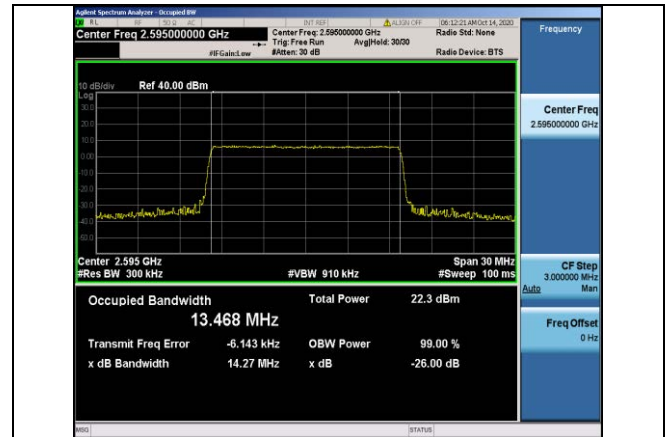
Band38-15MHz-16QAM-38000-75RB#0-13.468
