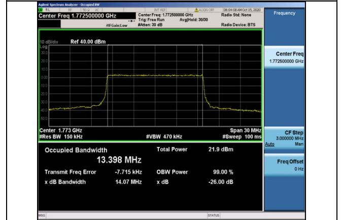
Band66-15MHz-16QAM-132597-75RB#0-13.398
