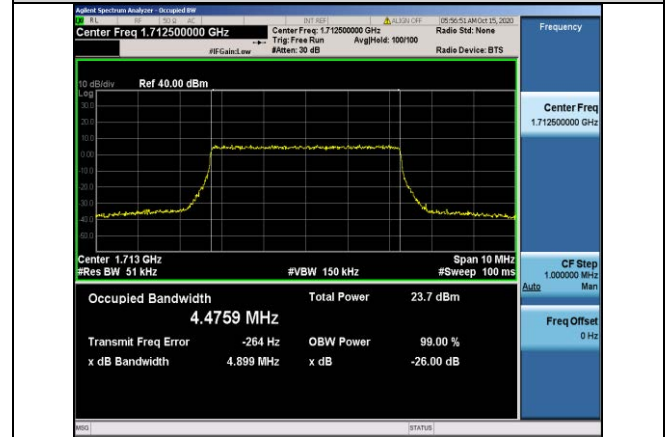
Band66-5MHz-QPSK-131997-25RB#0-4.4759
