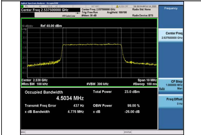
Band41-5MHz-16QAM-40065-25RB#0-4.5034
