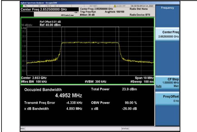
Band41-5MHz-QPSK-41215-25RB#0-4.4952
