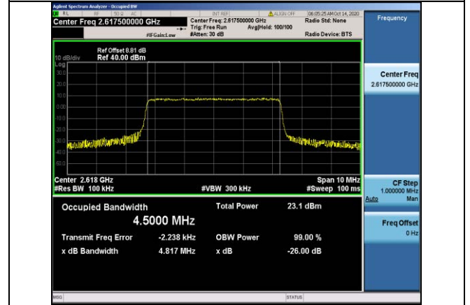
Band38-5MHz-16QAM-38225-25RB#0-4.5000
