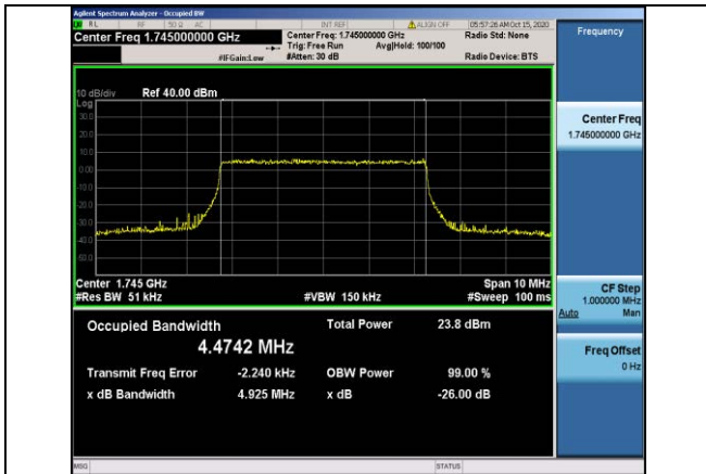
Band66-5MHz-QPSK-132322-25RB#0-4.4742
