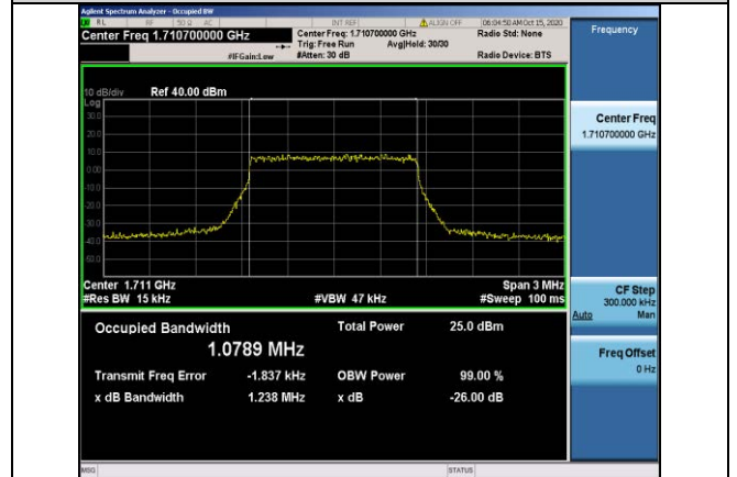
Band66-1.4MHz-QPSK-131979-6RB#0-1.0789
