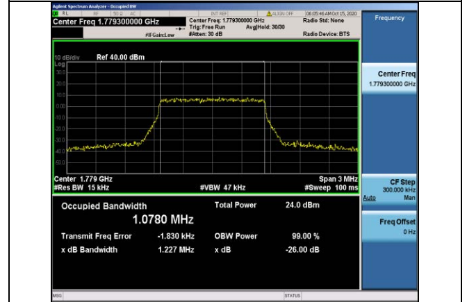
Band66-1.4MHz-16QAM-132665-6RB#0-1.0780
