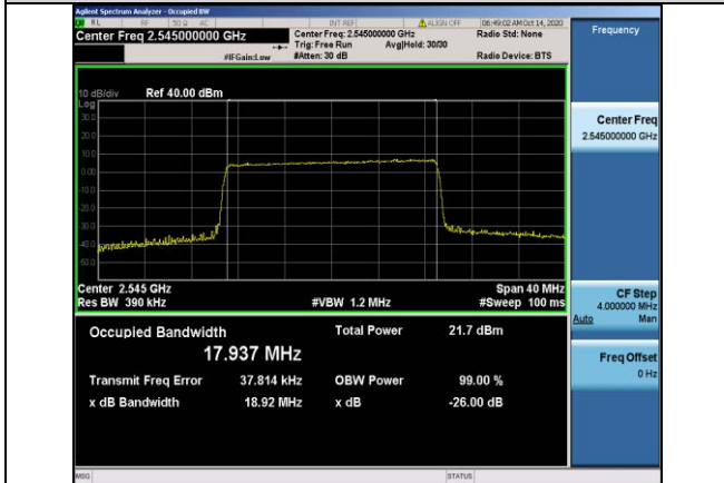
Band41-20MHz-16QAM-40140-100RB#0-17.937
