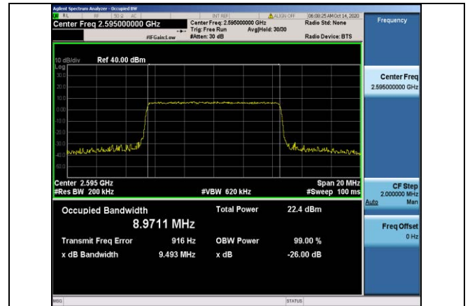
Band38-10MHz-16QAM-38000-50RB#0-8.9711
