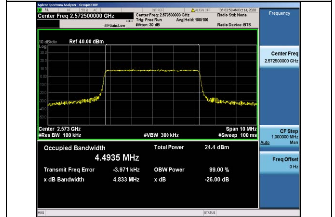
Band38-5MHz-QPSK-37775-25RB#0-4.4935
