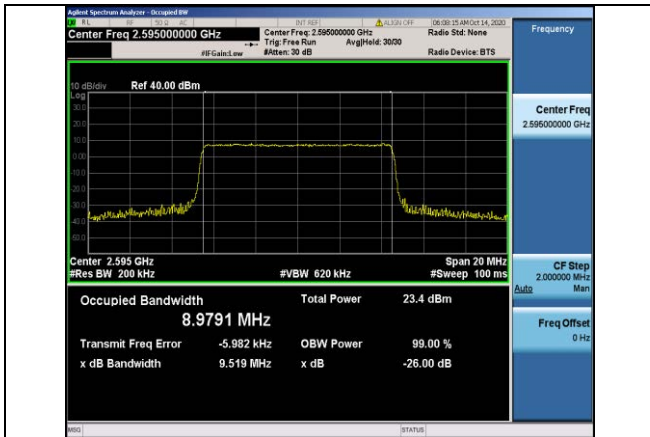
Band38-10MHz-QPSK-38000-50RB#0-8.9791
