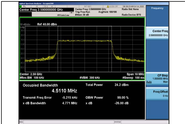
Band41-5MHz-QPSK-40590-25RB#0-4.5110
