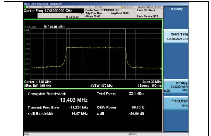
Band66-15MHz-16QAM-132322-75RB#0-13.403
