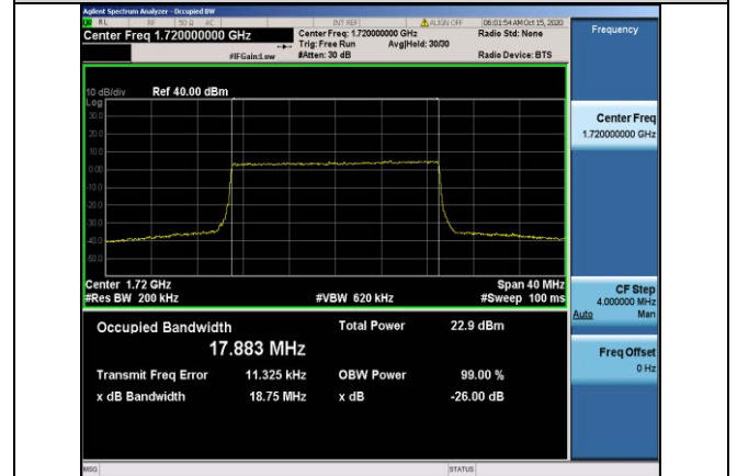
Band66-20MHz-QPSK-132072-100RB#0-17.883
