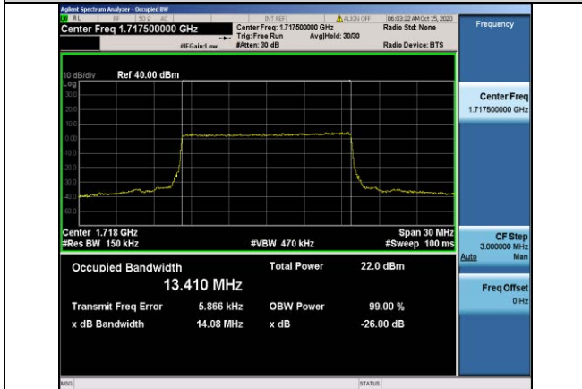
Band66-15MHz-16QAM-132047-75RB#0-13.410
