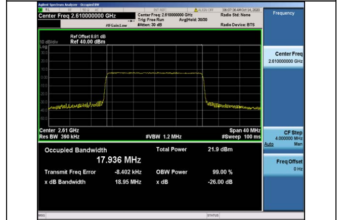
Band38-20MHz-16QAM-38150-100RB#0-17.936
