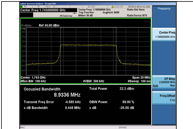
Band66-10MHz-QPSK-132322-50RB#0-8.9336
