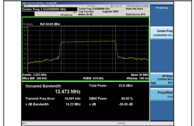
Band41-15MHz-QPSK-40115-75RB#0-13.473
