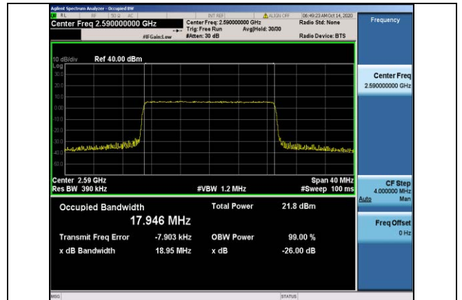
Band41-20MHz-16QAM-40590-100RB#0-17.946
