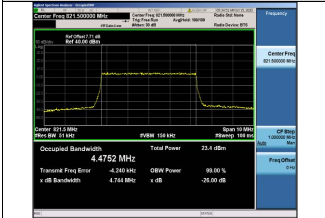
Band26-5MHz-16QAM-26765-25RB#0-4.4752
