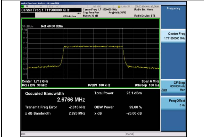
Band66-3MHz-16QAM-131987-15RB#0-2.6766
