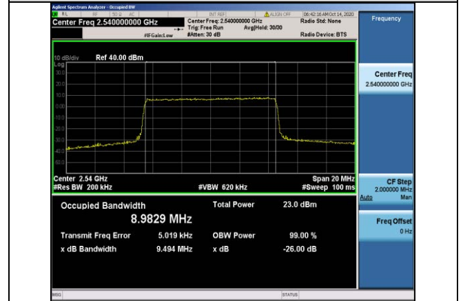
Band41-10MHz-QPSK-40090-50RB#0-8.9829
