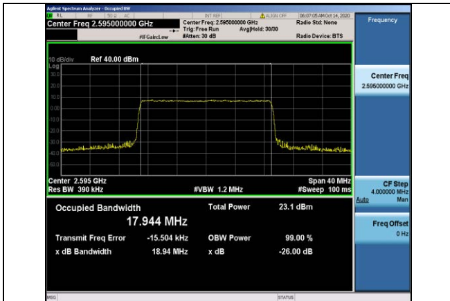
Band38-20MHz-QPSK-38000-100RB#0-17.944
