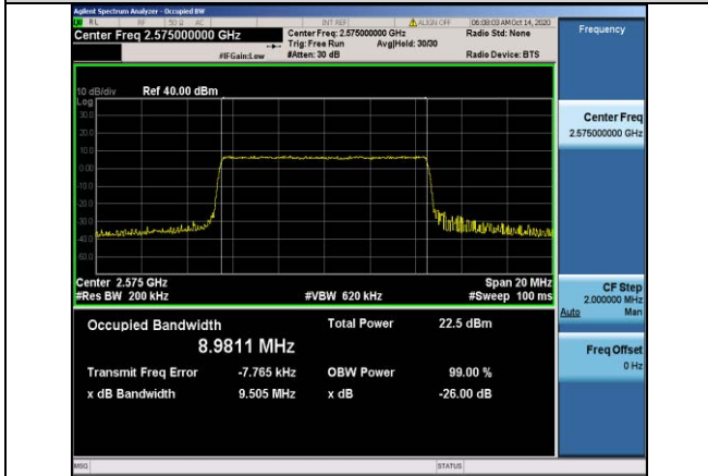
Band38-10MHz-16QAM-37800-50RB#0-8.9811
