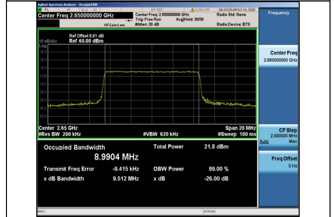
Band41-10MHz-16QAM-41190-50RB#0-8.9904
