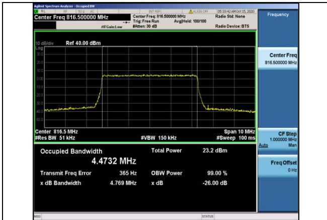
Band26-5MHz-16QAM-26715-25RB#0-4.4732
