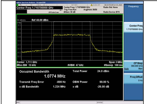
Band66-1.4MHz-16QAM-131979-6RB#0-1.0774
