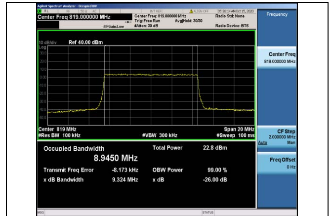
Band26-10MHz-QPSK-26740-50RB#0-8.9450
