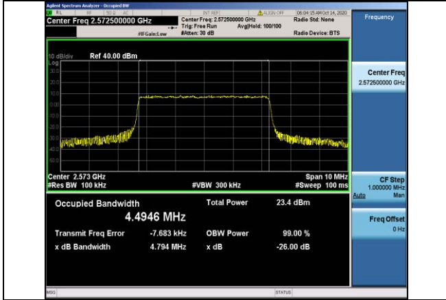
Band38-5MHz-16QAM-37775-25RB#0-4.4946
