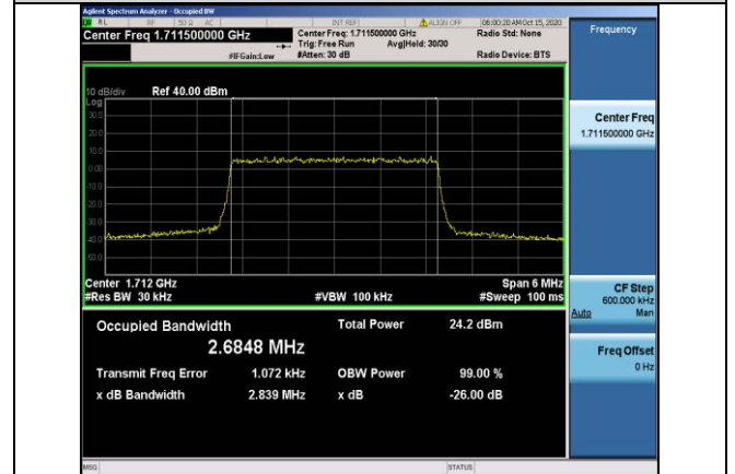
Band66-3MHz-QPSK-131987-15RB#0-2.6848
