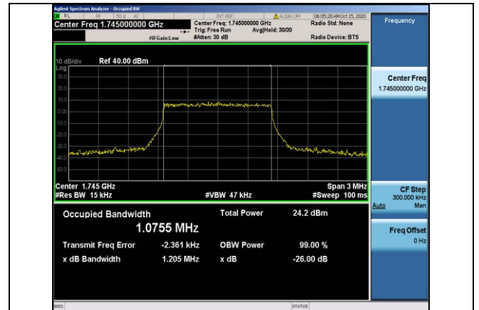
Band66-1.4MHz-16QAM-132322-6RB#0-1.0755
