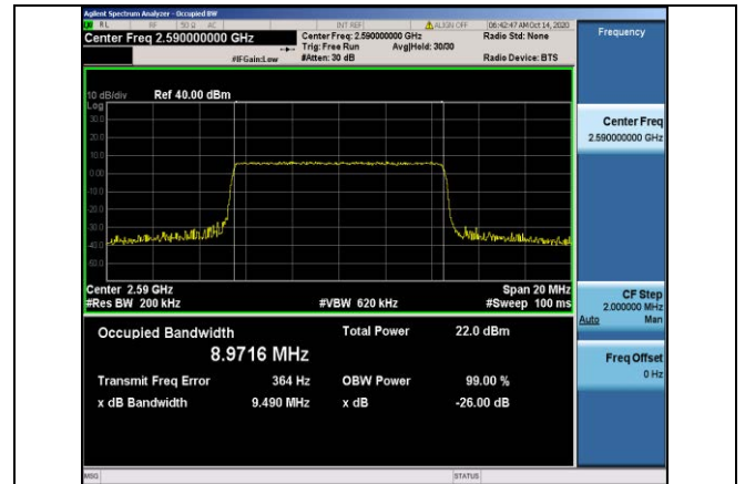
Band41-10MHz-16QAM-40590-50RB#0-8.9716
