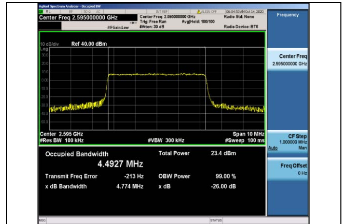
Band38-5MHz-16QAM-38000-25RB#0-4.4927
