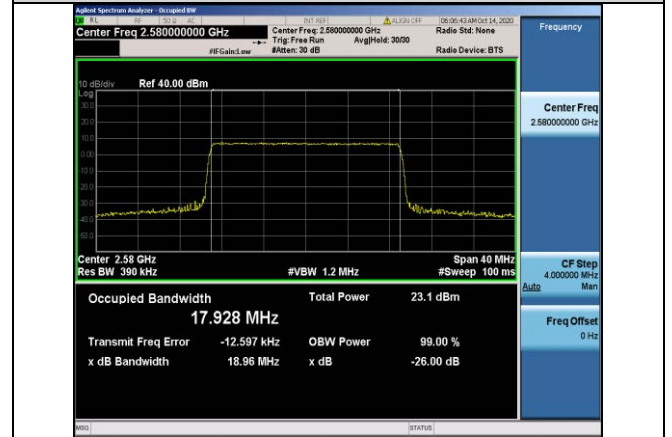
Band38-20MHz-QPSK-37850-100RB#0-17.928
