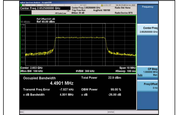
Band41-5MHz-16QAM-41215-25RB#0-4.4901
