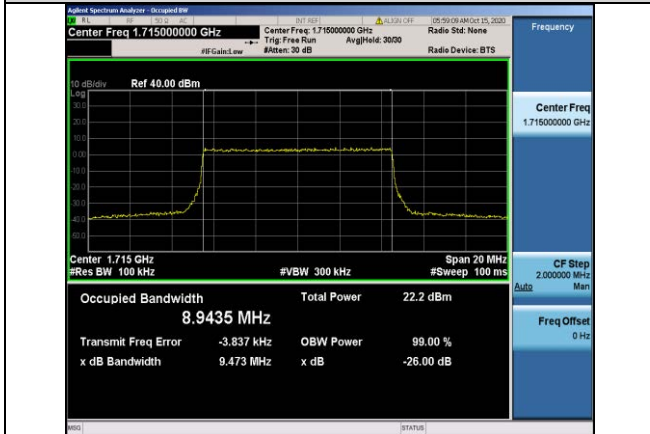
Band66-10MHz-16QAM-132022-50RB#0-8.9435
