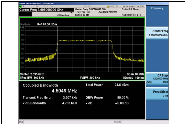
Band38-5MHz-QPSK-38000-25RB#0-4.5046
