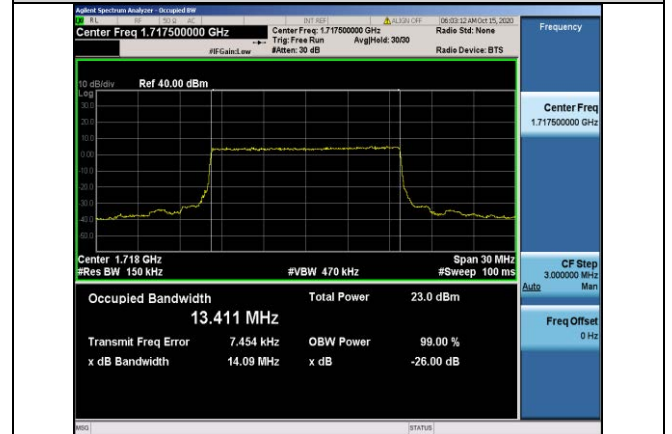
Band66-15MHz-QPSK-132047-75RB#0-13.411
