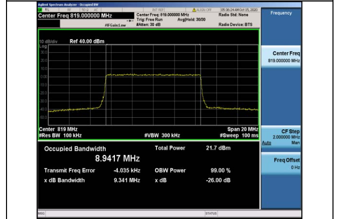
Band26-10MHz-16QAM-26740-50RB#0-8.9417
