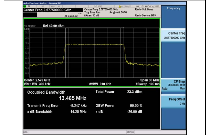
Band38-15MHz-QPSK-37825-75RB#0-13.465
