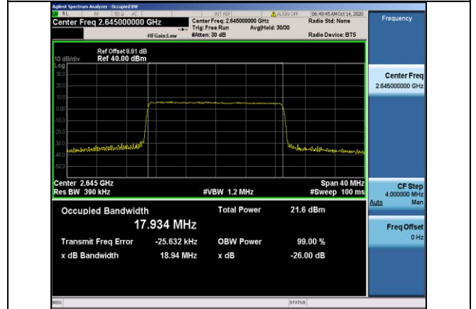
Band41-20MHz-16QAM-41140-100RB#0-17.934
