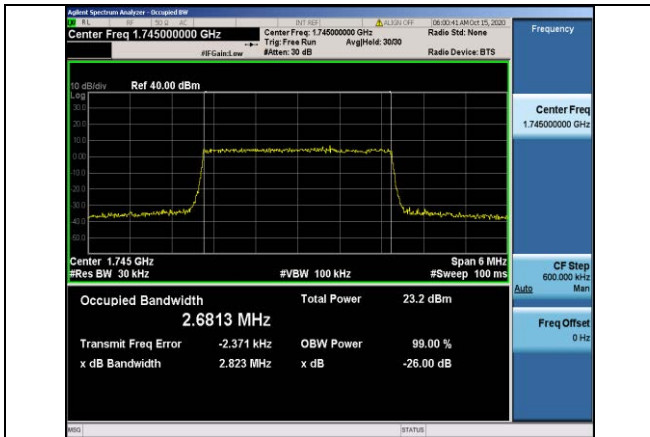
Band66-3MHz-QPSK-132322-15RB#0-2.6813
