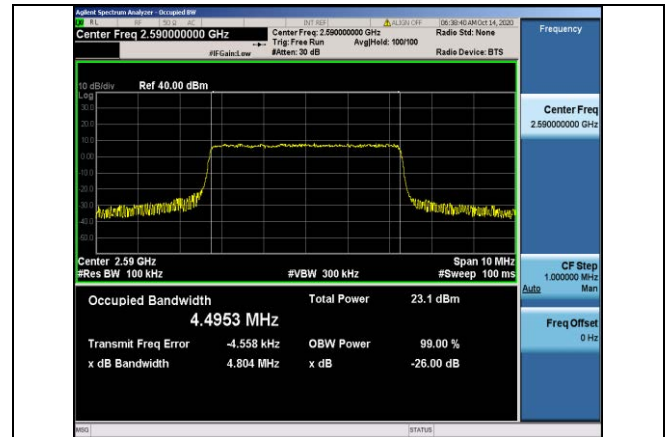
Band41-5MHz-16QAM-40590-25RB#0-4.4953
