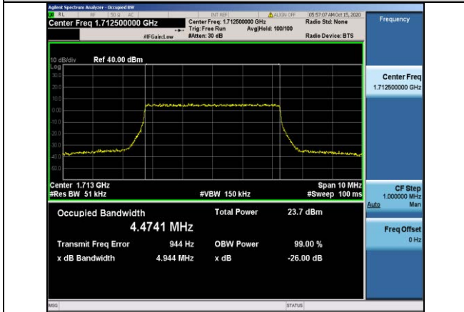
Band66-5MHz-16QAM-131997-25RB#0-4.4741
