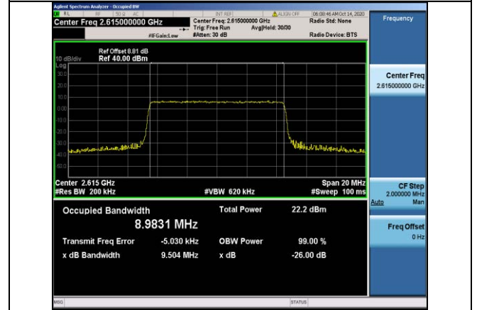
Band38-10MHz-16QAM-38200-50RB#0-8.9831
