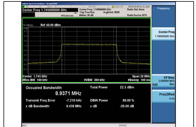
Band66-10MHz-16QAM-132322-50RB#0-8.9371
