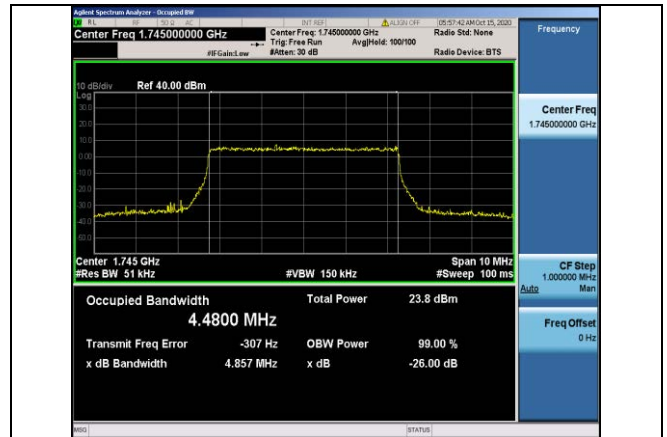
Band66-5MHz-16QAM-132322-25RB#0-4.4800
