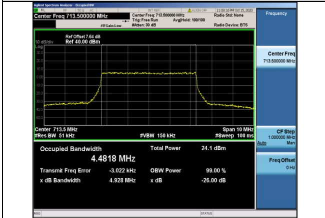
Band12-5MHz-16QAM-23155-25RB#0-4.4818
