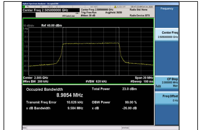
Band7-10MHz-QPSK-20800-50RB#0-8.9854
