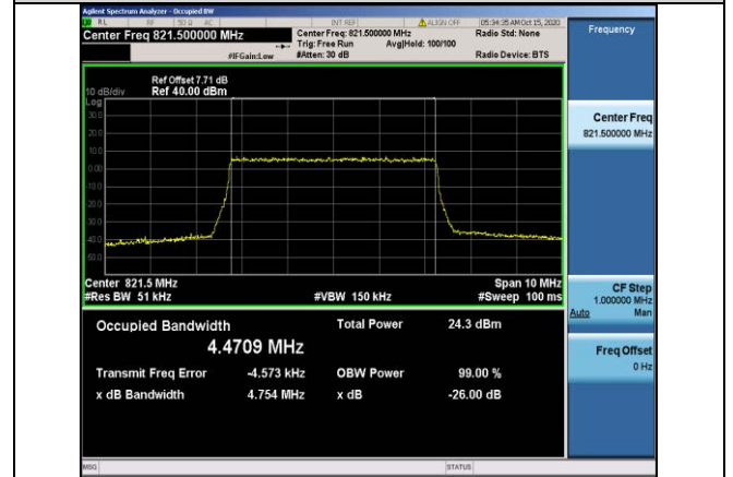
Band26-5MHz-QPSK-26765-25RB#0-4.4709
