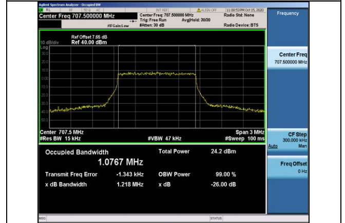
Band12-1.4MHz-QPSK-23095-6RB#0-1.0767
