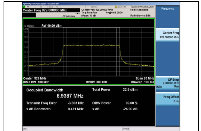
Band5-10MHz-QPSK-20450-50RB#0-8.9387
