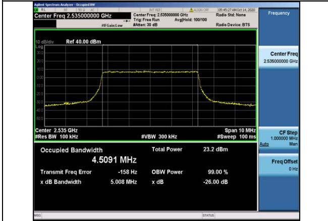
Band7-5MHz-16QAM-21100-25RB#0-4.5091
