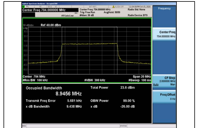
Band12-10MHz-QPSK-23060-50RB#0-8.9456
