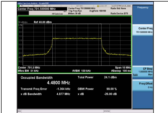
Band12-5MHz-16QAM-23035-25RB#0-4.4800
