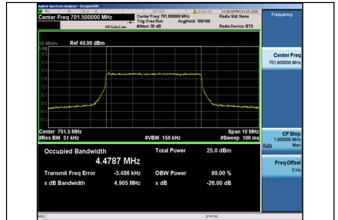
Band12-5MHz-QPSK-23035-25RB#0-4.4787
