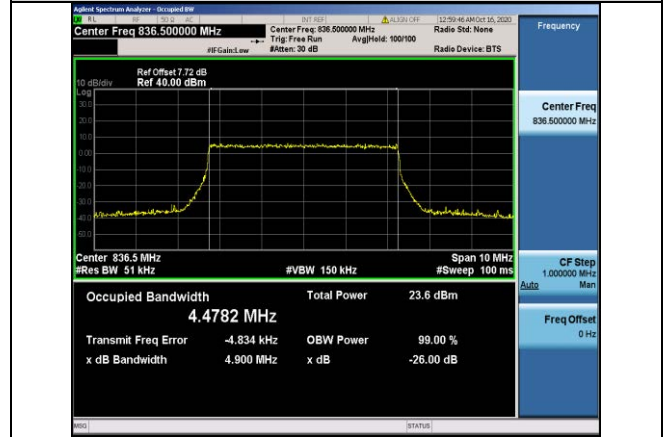
Band5-5MHz-QPSK-20525-25RB#0-4.4782
