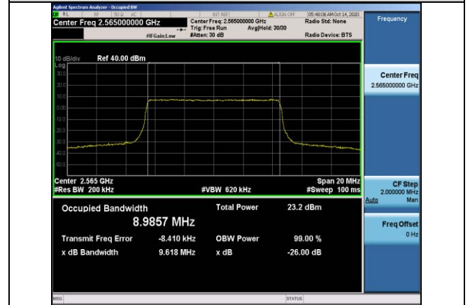
Band7-10MHz-QPSK-21400-50RB#0-8.9857
