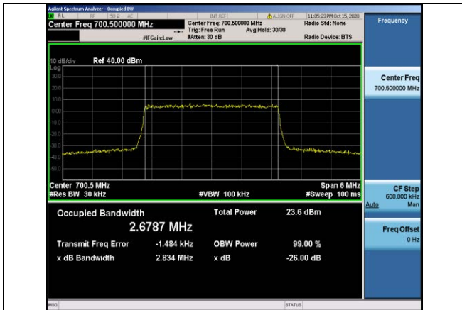
Band12-3MHz-16QAM-23025-15RB#0-2.6787
