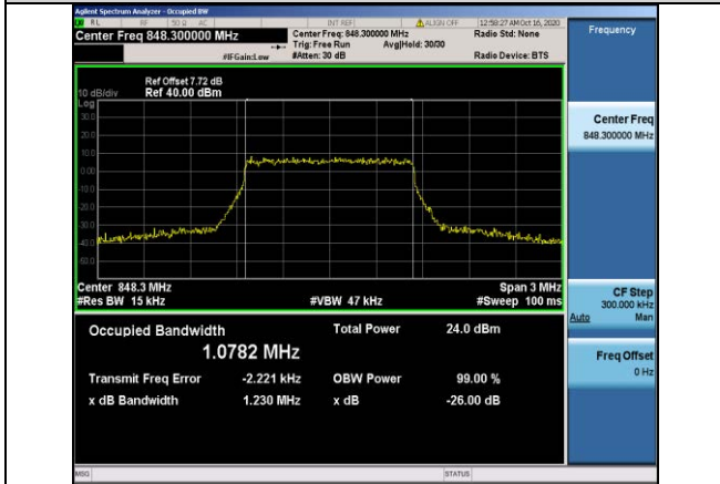
Band5-1.4MHz-16QAM-20643-6RB#0-1.0782
