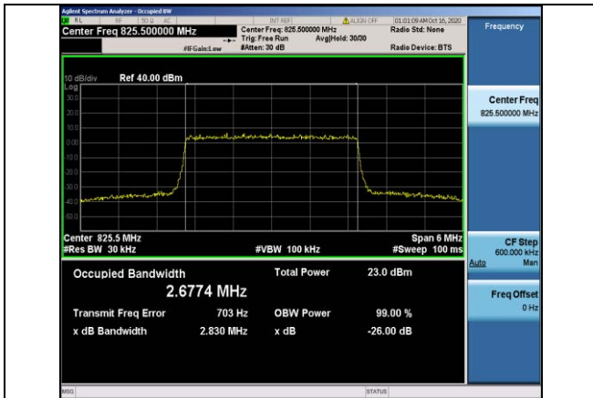
Band5-3MHz-16QAM-20415-15RB#0-2.6774
