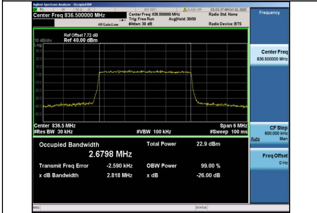
Band5-3MHz-16QAM-20525-15RB#0-2.6798
