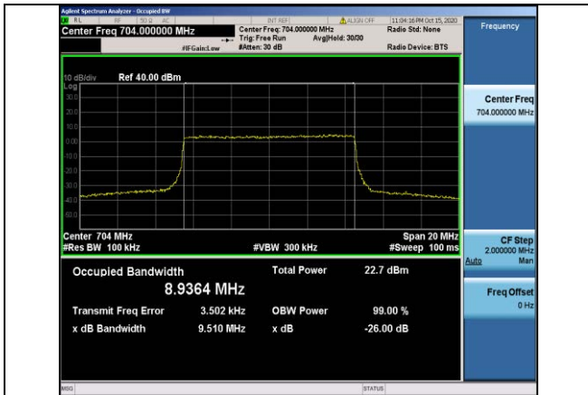
Band12-10MHz-16QAM-23060-50RB#0-8.9364
