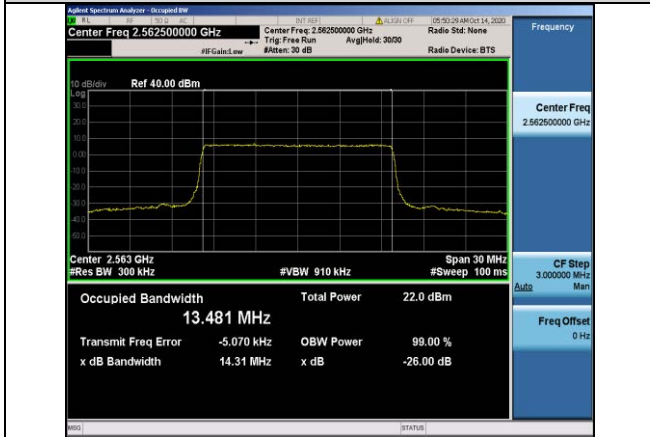
Band7-15MHz-16QAM-21375-75RB#0-13.481
