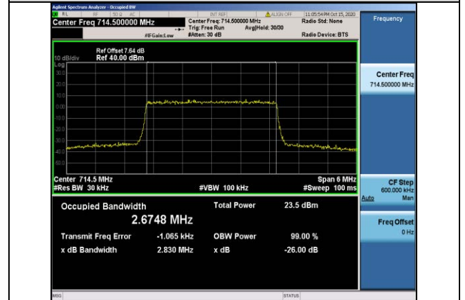
Band12-3MHz-QPSK-23165-15RB#0-2.6748
