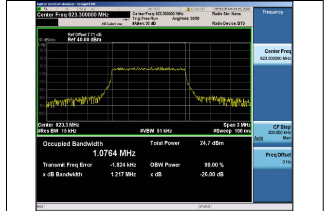
Band26-1.4MHz-QPSK-26783-6RB#0-1.0764
