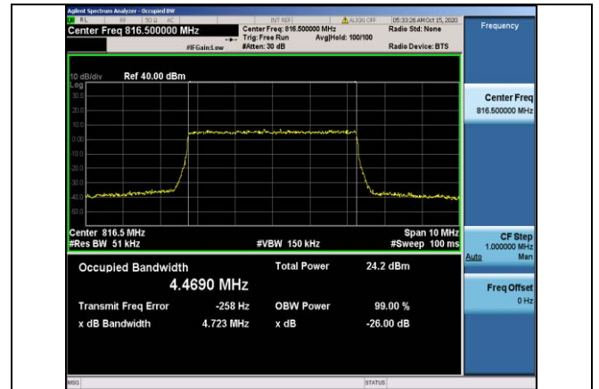
Band26-5MHz-QPSK-26715-25RB#0-4.4690
