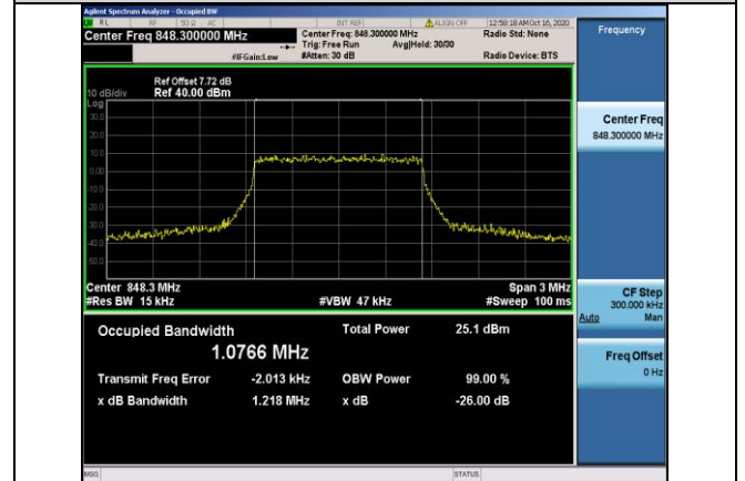
Band5-1.4MHz-QPSK-20643-6RB#0-1.0766
