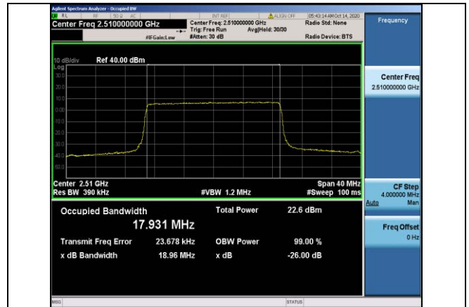
Band7-20MHz-QPSK-20850-100RB#0-17.931
