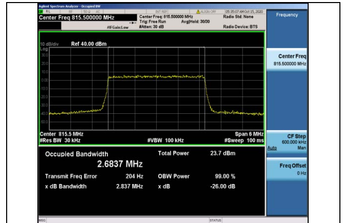
Band26-3MHz-QPSK-26705-15RB#0-2.6837
