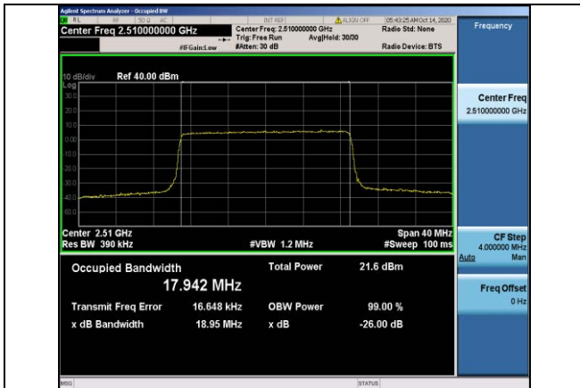
Band7-20MHz-16QAM-20850-100RB#0-17.942
