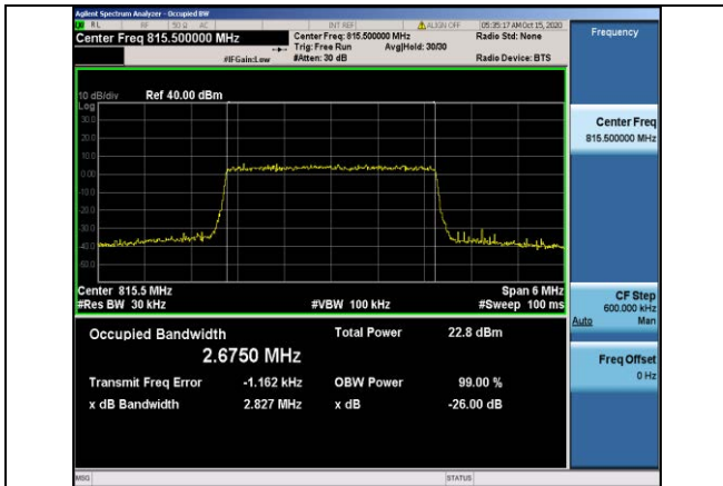
Band26-3MHz-16QAM-26705-15RB#0-2.6750
