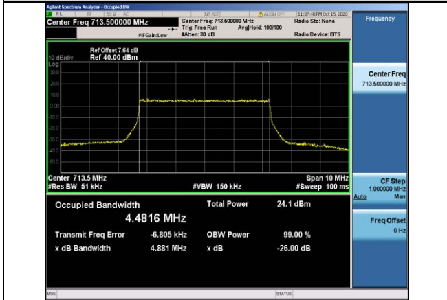
Band17-5MHz-16QAM-23825-25RB#0-4.4816
