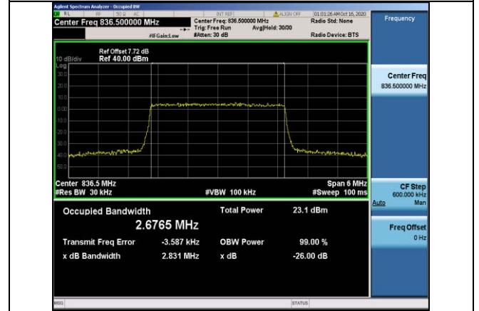
Band5-3MHz-QPSK-20525-15RB#0-2.6765
