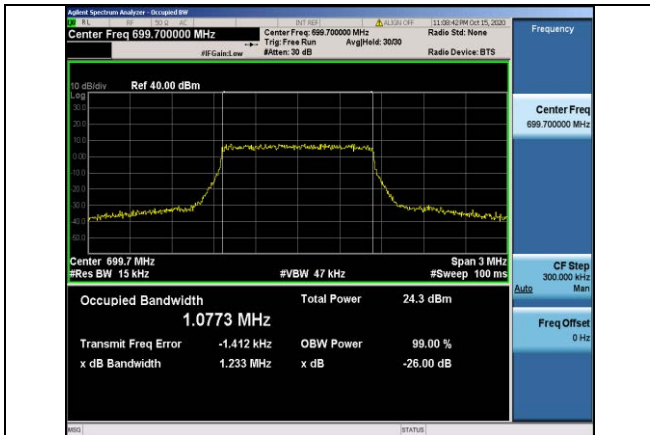
Band12-1.4MHz-16QAM-23017-6RB#0-1.0773
