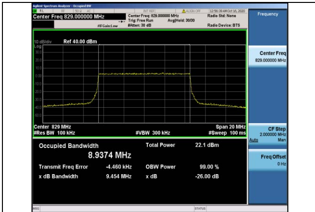
Band5-10MHz-16QAM-20450-50RB#0-8.9374
