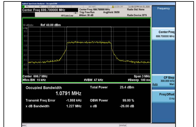
Band12-1.4MHz-QPSK-23017-6RB#0-1.0791
