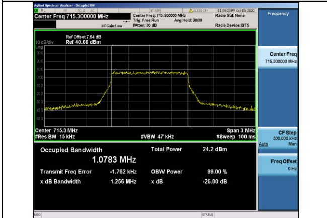
Band12-1.4MHz-16QAM-23173-6RB#0-1.0783
