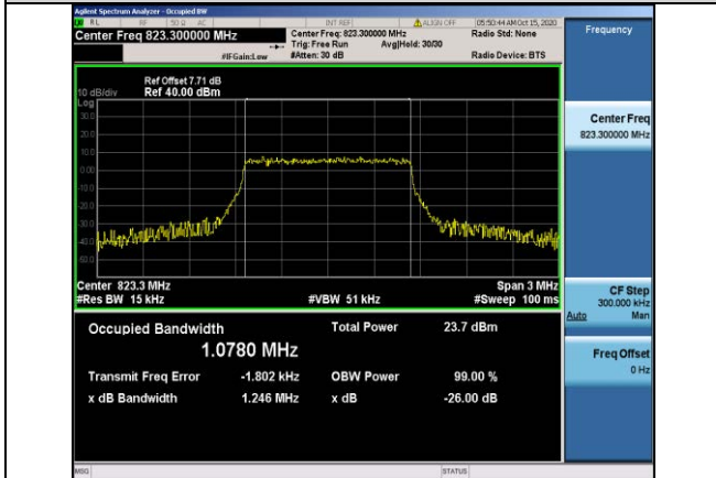
Band26-1.4MHz-16QAM-26783-6RB#0-1.0780
