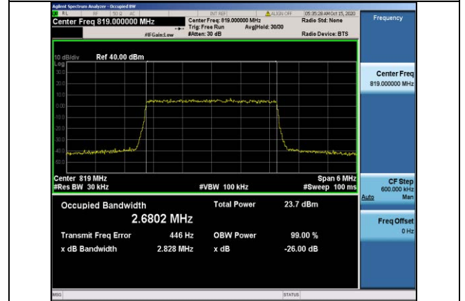
Band26-3MHz-QPSK-26740-15RB#0-2.6802
