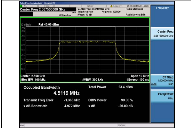
Band7-5MHz-16QAM-21425-25RB#0-4.5119
