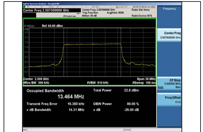
Band7-15MHz-QPSK-20825-75RB#0-13.464
