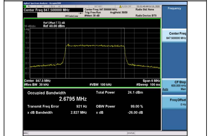
Band5-3MHz-QPSK-20635-15RB#0-2.6795
