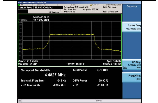
Band12-5MHz-QPSK-23155-25RB#0-4.4827
