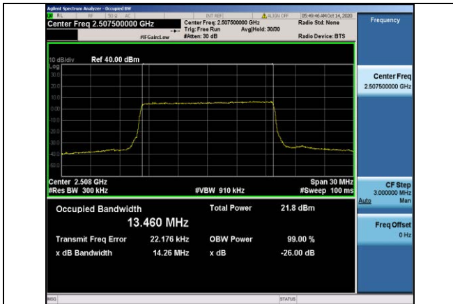
Band7-15MHz-16QAM-20825-75RB#0-13.460
