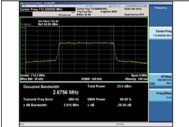
Band12-3MHz-16QAM-23165-15RB#0-2.6756
