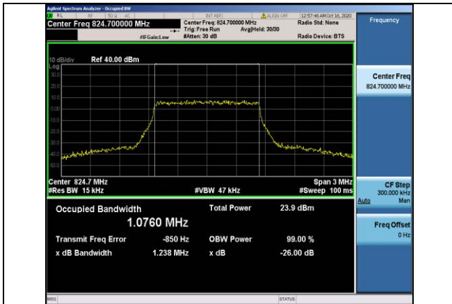
Band5-1.4MHz-16QAM-20407-6RB#0-1.0760
