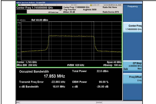
Band4-20MHz-16QAM-20300-100RB#0-17.853
