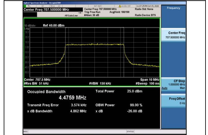
Band12-5MHz-QPSK-23095-25RB#0-4.4759
