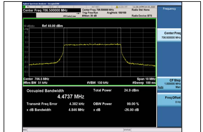
Band17-5MHz-QPSK-23755-25RB#0-4.4737
