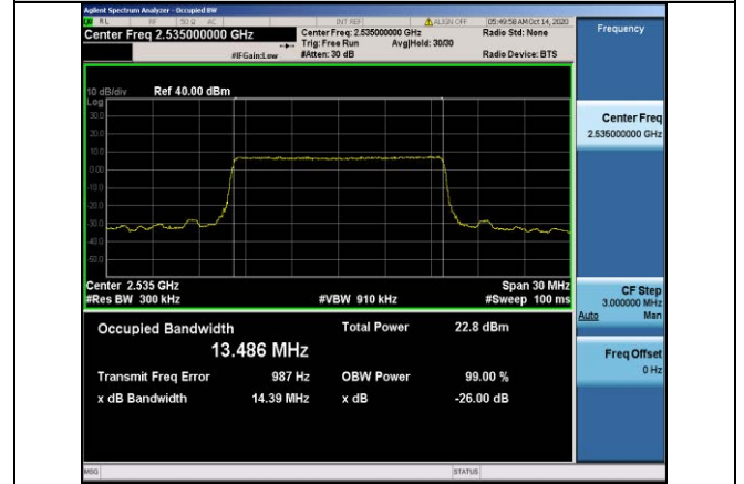
Band7-15MHz-QPSK-21100-75RB#0-13.486
