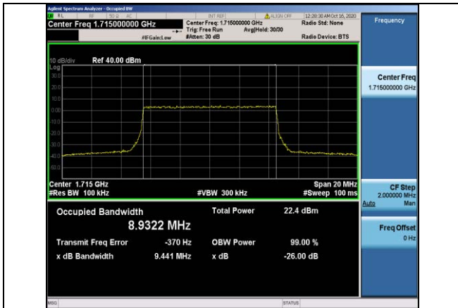
Band4-10MHz-16QAM-20000-50RB#0-8.9322
