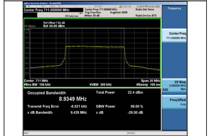
Band12-10MHz-QPSK-23130-50RB#0-8.9349
