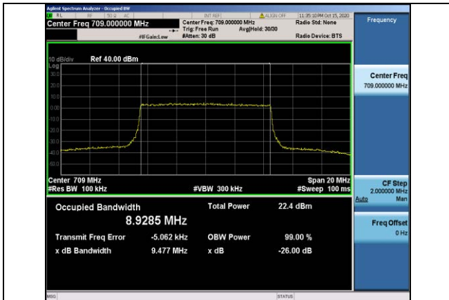
Band17-10MHz-16QAM-23780-50RB#0-8.9285
