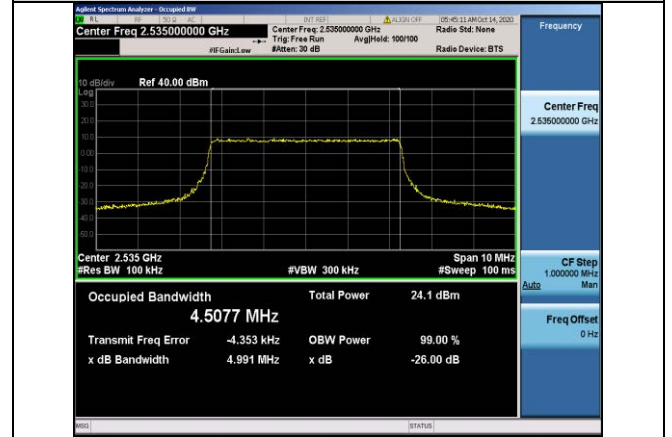
Band7-5MHz-QPSK-21100-25RB#0-4.5077
