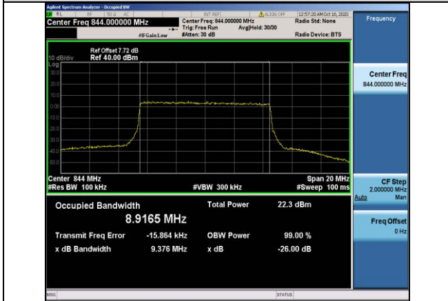
Band5-10MHz-16QAM-20600-50RB#0-8.9165
