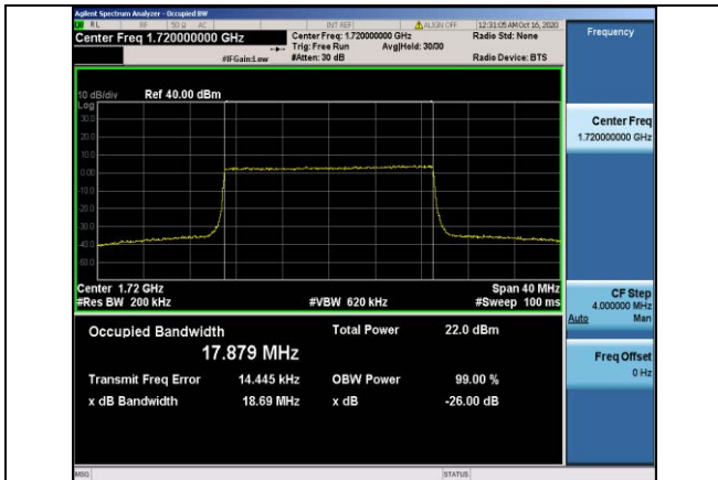
Band4-20MHz-16QAM-20050-100RB#0-17.879
