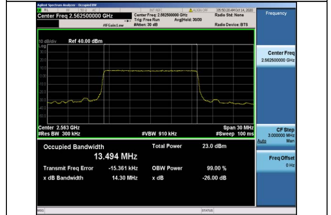
Band7-15MHz-QPSK-21375-75RB#0-13.494
