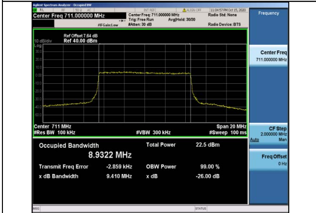
Band12-10MHz-16QAM-23130-50RB#0-8.9322
