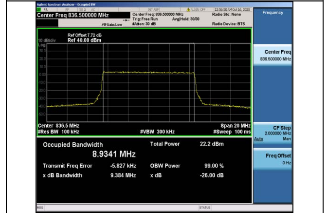
Band5-10MHz-QPSK-20525-50RB#0-8.9341
