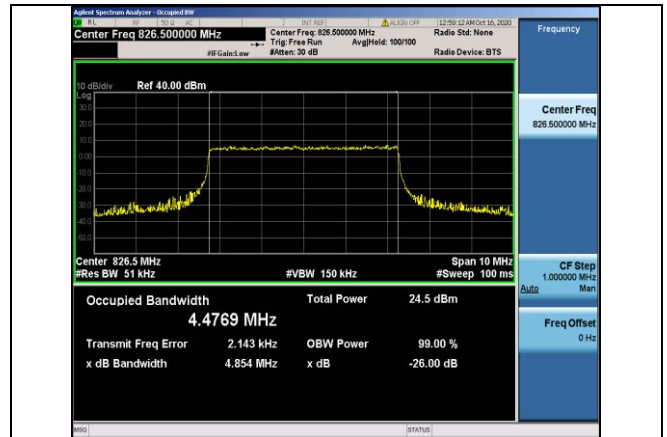
Band5-5MHz-QPSK-20425-25RB#0-4.4769
