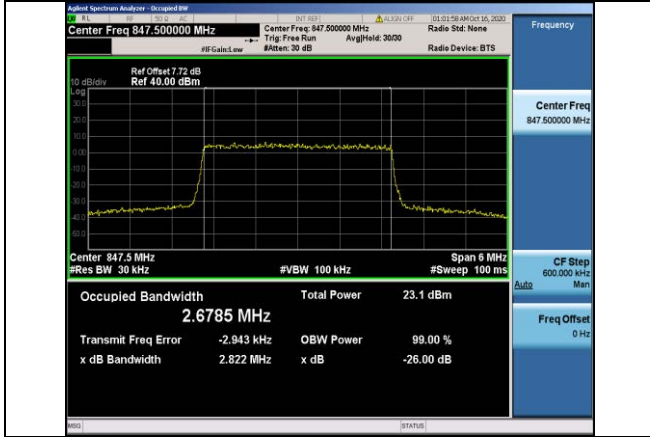
Band5-3MHz-16QAM-20635-15RB#0-2.6785
