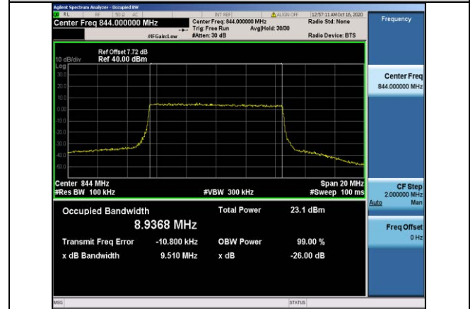
Band5-10MHz-QPSK-20600-50RB#0-8.9368
