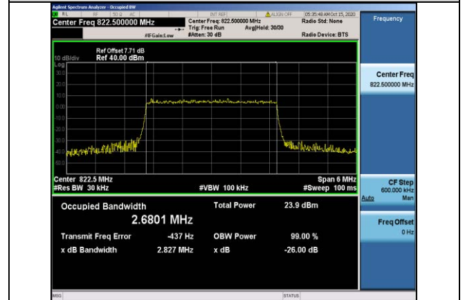
Band26-3MHz-QPSK-26775-15RB#0-2.6801
