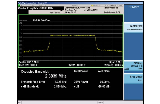
Band5-3MHz-QPSK-20415-15RB#0-2.6839
