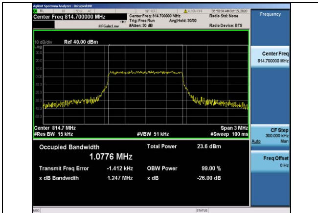
Band26-1.4MHz-16QAM-26697-6RB#0-1.0776
