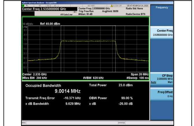
Band7-10MHz-QPSK-21100-50RB#0-9.0014
