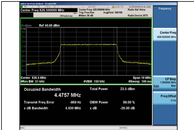
Band5-5MHz-16QAM-20425-25RB#0-4.4757
