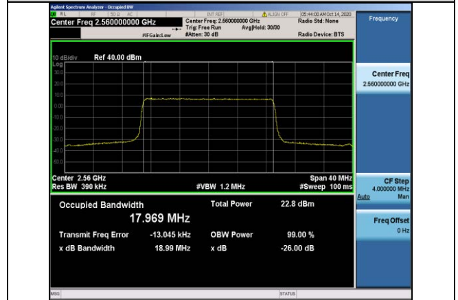
Band7-20MHz-QPSK-21350-100RB#0-17.969
