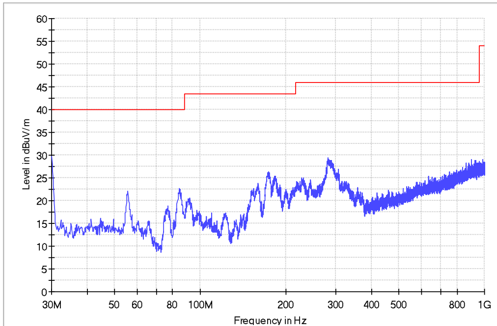
Copy of Field strength 30M-1GHz
