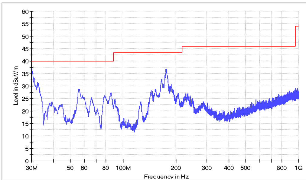
Copy of Field strength 30M-1GHz
