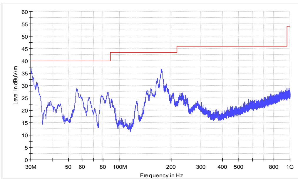
Copy of Field strength 30M-1GHz
