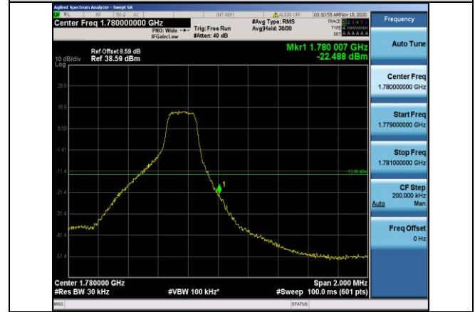
Band66-3MHz-QPSK-132657-1RB#14
