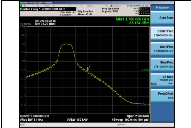
Band66-5MHz-QPSK-132647-1RB#24
