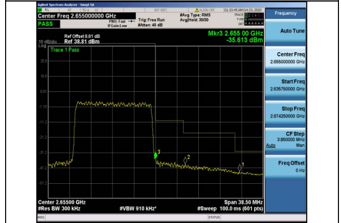
Band41-15MHz-16QAM-41165-75RB#0
