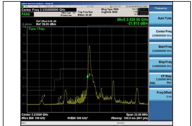
Band41-5MHz-16QAM-40065-1RB#0
