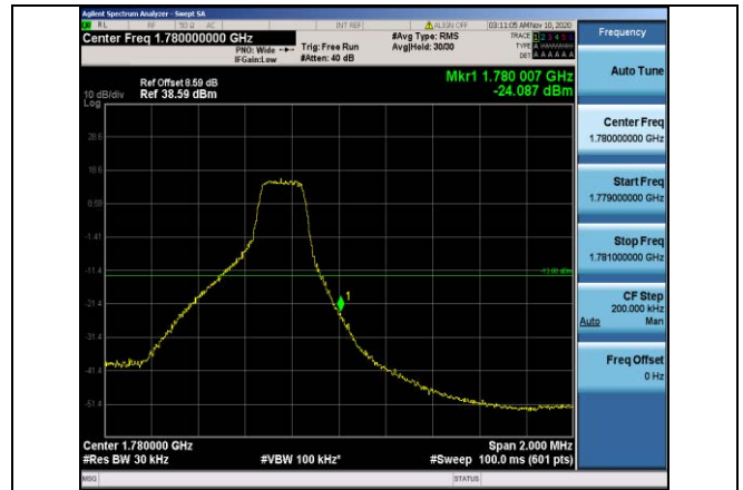
Band66-3MHz-16QAM-132657-1RB#14
