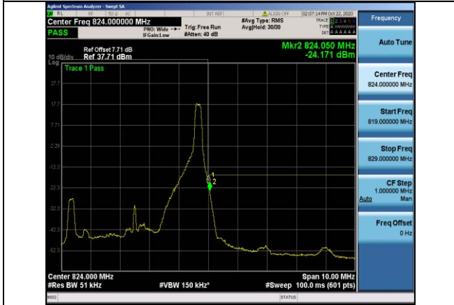
Band26-5MHz-QPSK-26765-1RB#24
