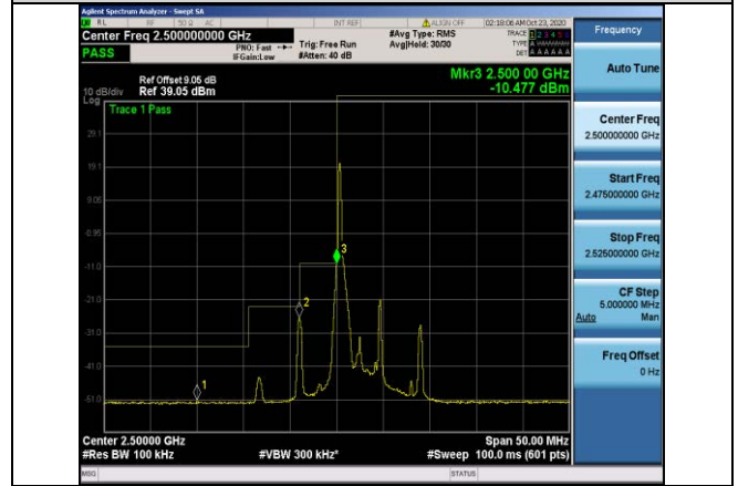
Band7-5MHz-QPSK-20775-1RB#0
