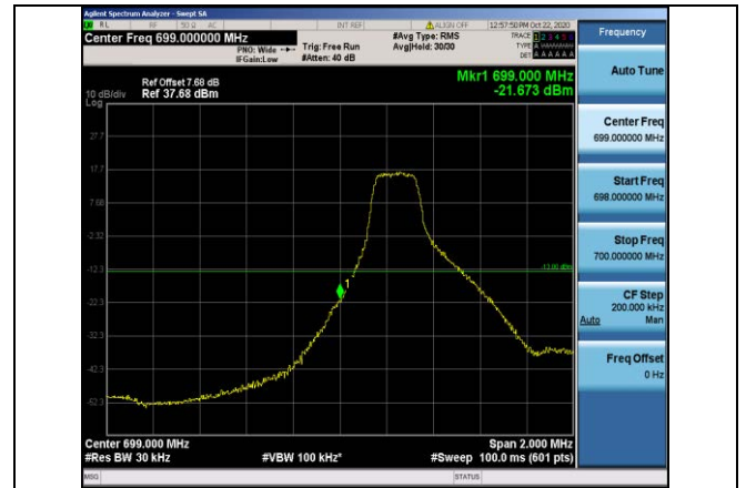
Band12-3MHz-QPSK-23025-1RB#0
