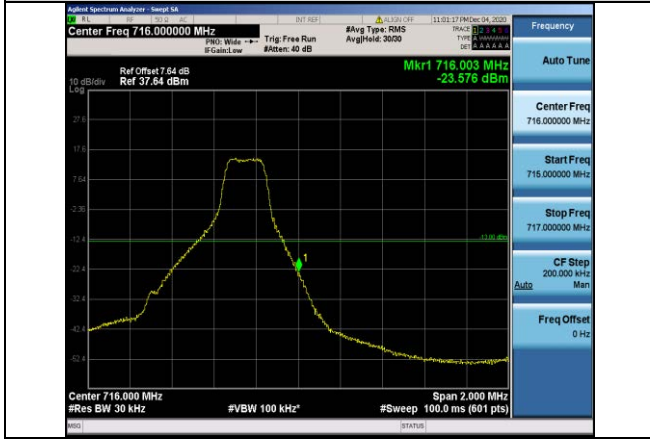
Band12-1.4MHz-16QAM-23173-1RB#5
