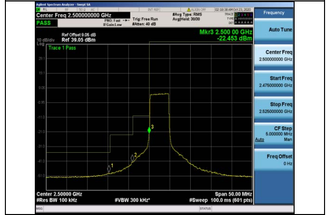
Band7-5MHz-16QAM-20775-25RB#0
