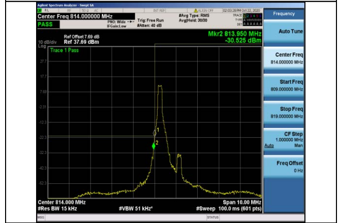
Band26-1.4MHz-16QAM-26697-1RB#0
