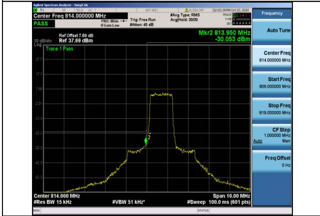
Band26-1.4MHz-QPSK-26697-6RB#0
