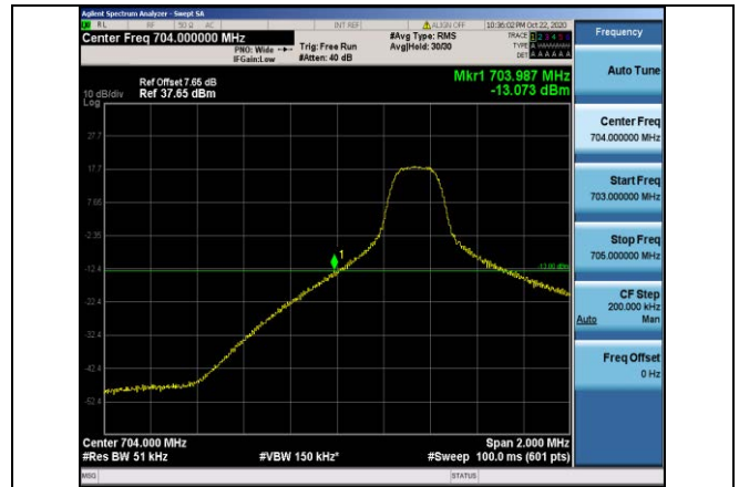
Band17-5MHz-QPSK-23755-1RB#0
