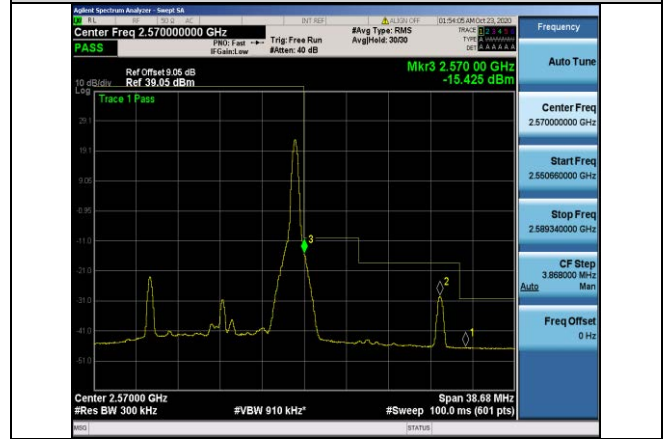
Band7-15MHz-QPSK-21375-1RB#74
