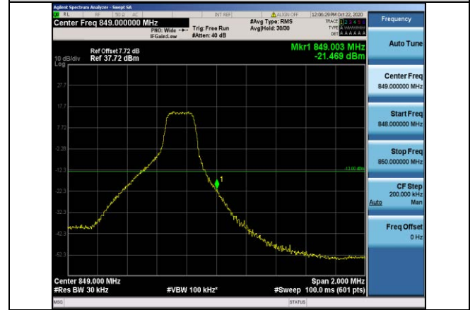
Band5-3MHz-16QAM-20635-1RB#14
