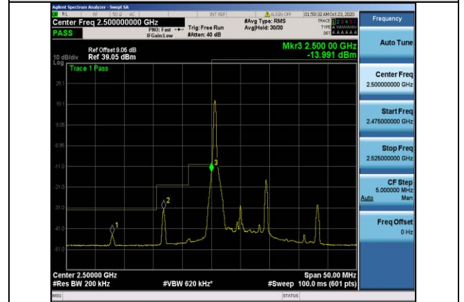
Band7-10MHz-16QAM-20800-1RB#0
