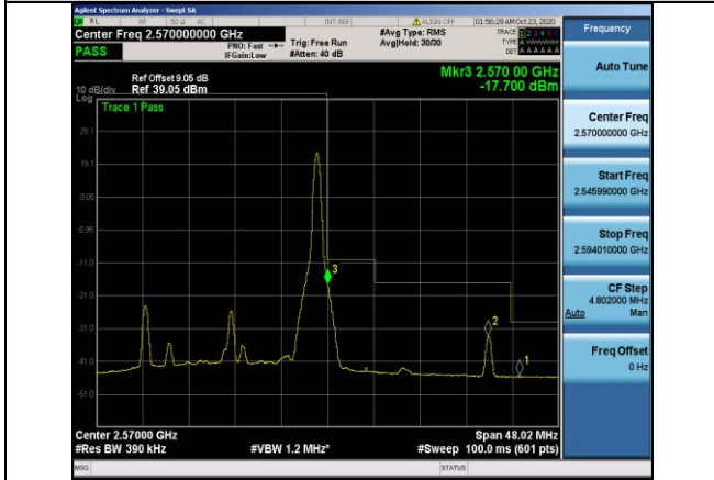
Band7-20MHz-QPSK-21350-1RB#99
