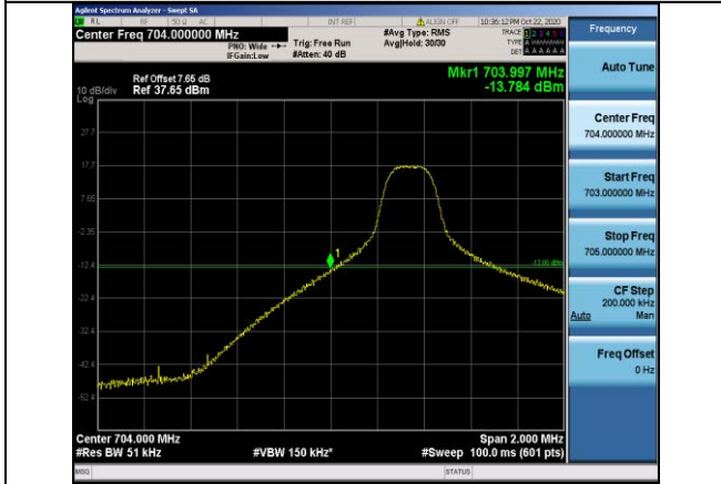
Band17-5MHz-16QAM-23755-1RB#0
