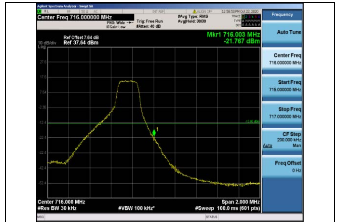
Band12-3MHz-16QAM-23165-1RB#14
