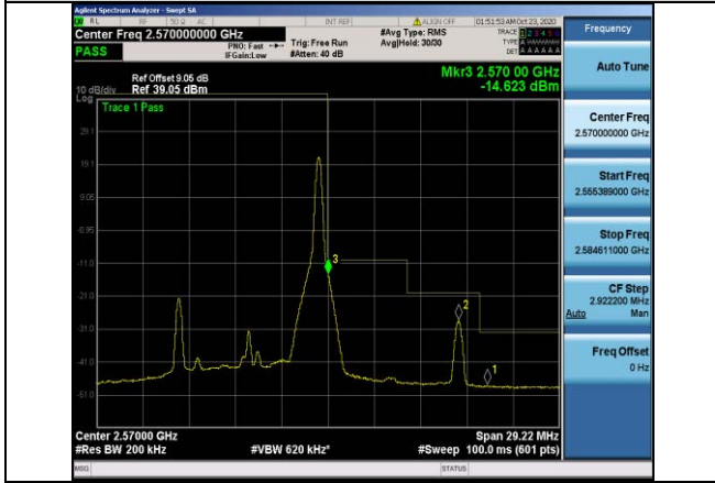
Band7-10MHz-16QAM-21400-1RB#49
