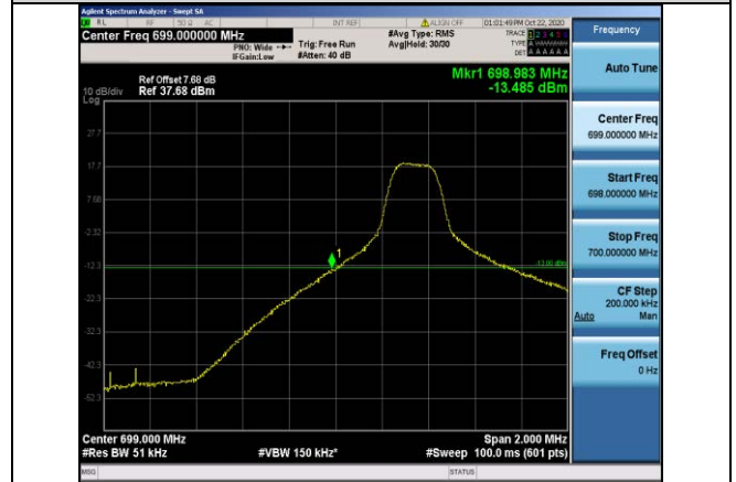
Band12-5MHz-QPSK-23035-1RB#0
