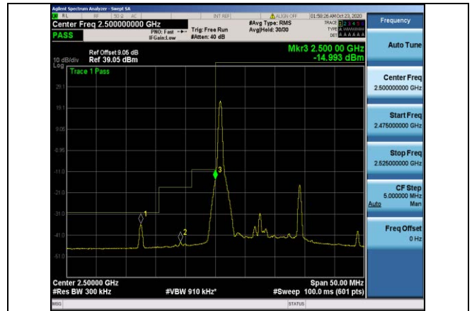
Band7-15MHz-QPSK-20825-1RB#0
