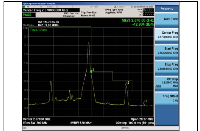
Band7-10MHz-QPSK-21400-1RB#49
