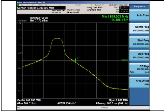
Band5-5MHz-16QAM-20625-1RB#24
