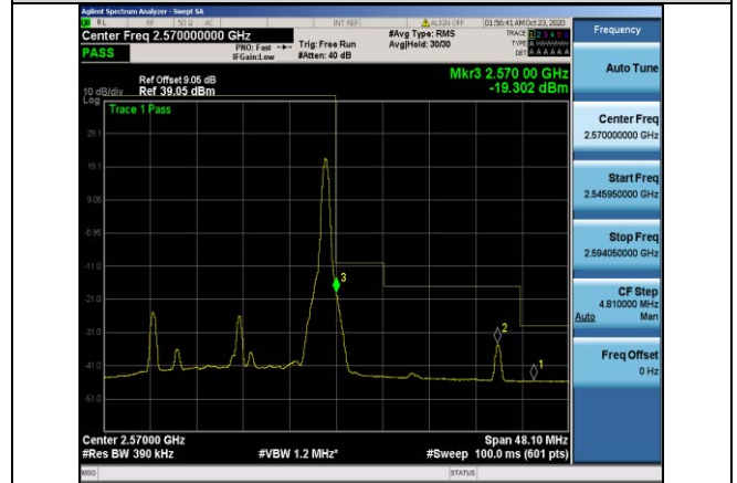
Band7-20MHz-16QAM-21350-1RB#99
