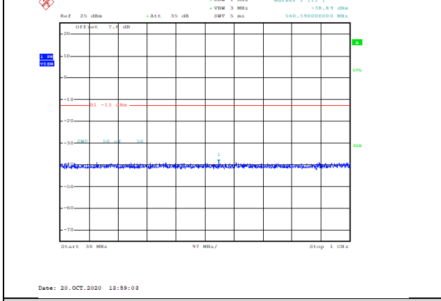
Band66-15MHz-QPSK-132597-1RB#0-Range1:30~1000MHz--38.89-PASS
