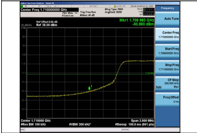
Band4-10MHz-16QAM-20000-50RB#0
