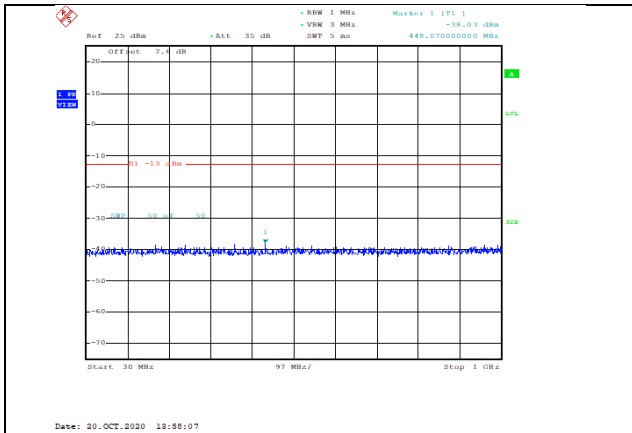
Band66-15MHz-QPSK-132322-1RB#0-Range1:30~1000MHz--38.03-PASS
