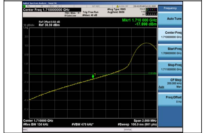
Band4-15MHz-QPSK-20025-1RB#0
