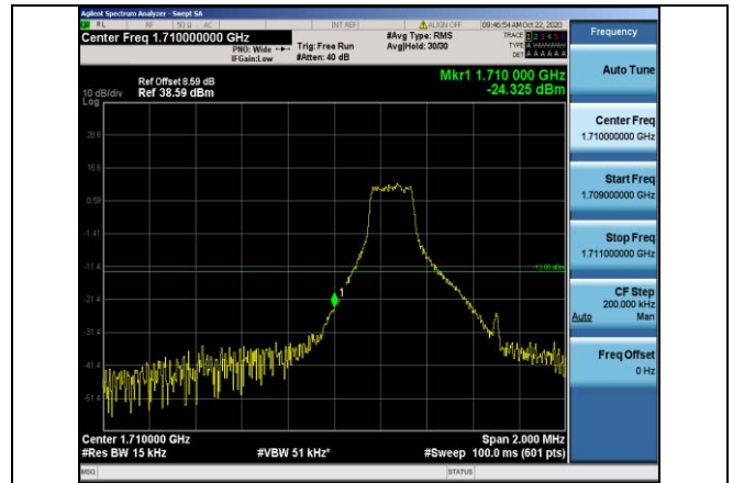
Band4-1.4MHz-QPSK-19957-1RB#0
