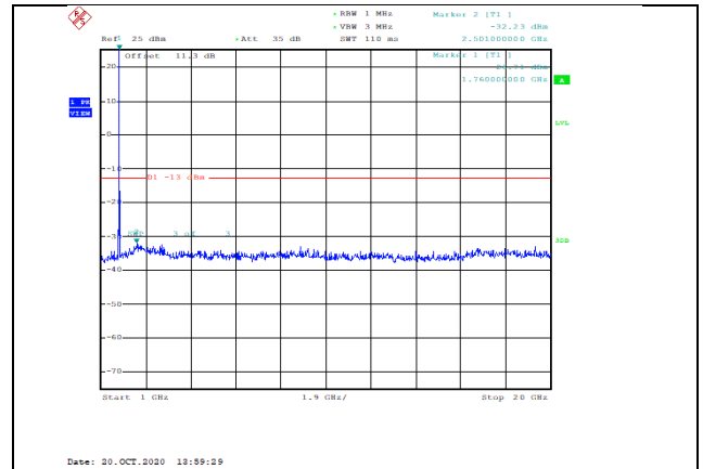
Band66-15MHz-16QAM-132597-1RB#0-Range2:1000~20000MHz--32.23-PASS
