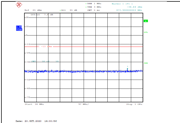
Band66-20MHz-16QAM-132322-1RB#0-Range1:30~1000MHz--38.48-PASS
