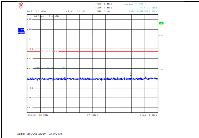
Band66-20MHz-QPSK-132322-1RB#0-Range1:30~1000MHz--38.37-PASS
