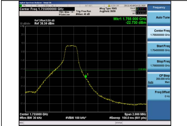
Band4-3MHz-QPSK-20385-1RB#14
