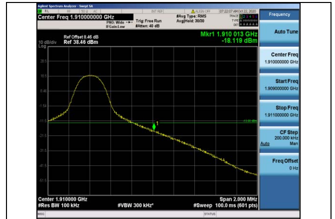
Band2-10MHz-16QAM-19150-1RB#49
