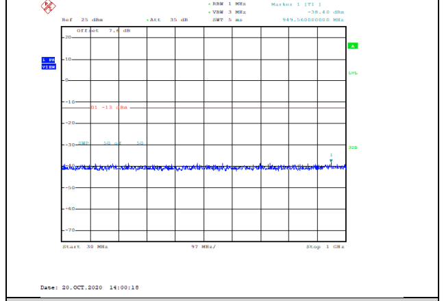
Band66-20MHz-16QAM-132072-1RB#0-Range1:30~1000MHz--38.4-PASS
