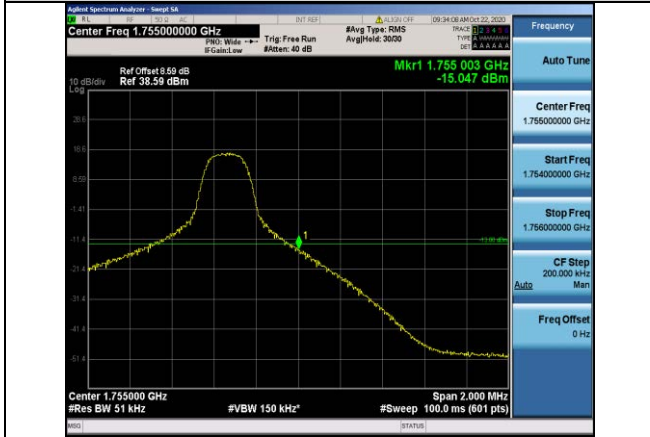
Band4-5MHz-16QAM-20375-1RB#24
