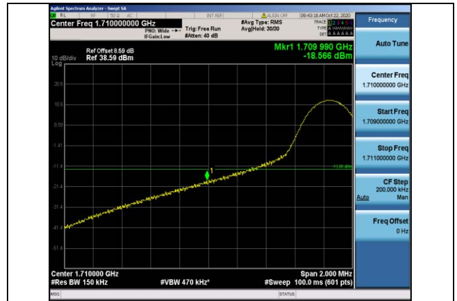
Band4-15MHz-16QAM-20025-1RB#0
