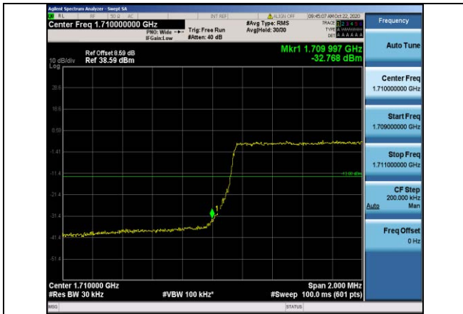
Band4-3MHz-QPSK-19965-15RB#0
