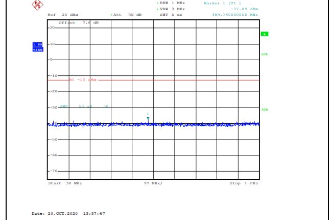
Band66-15MHz-16QAM-132047-1RB#0-Range1:30~1000MHz--37.49-PASS
