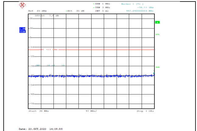
Band66-20MHz-16QAM-132572-1RB#0-Range1:30~1000MHz--38.55-PASS
