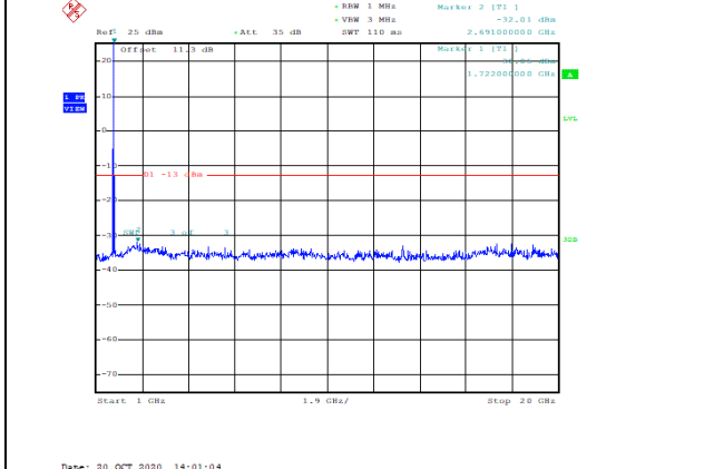
Band66-20MHz-16QAM-132322-1RB#0-Range2:1000~20000MHz--32.01-PASS
