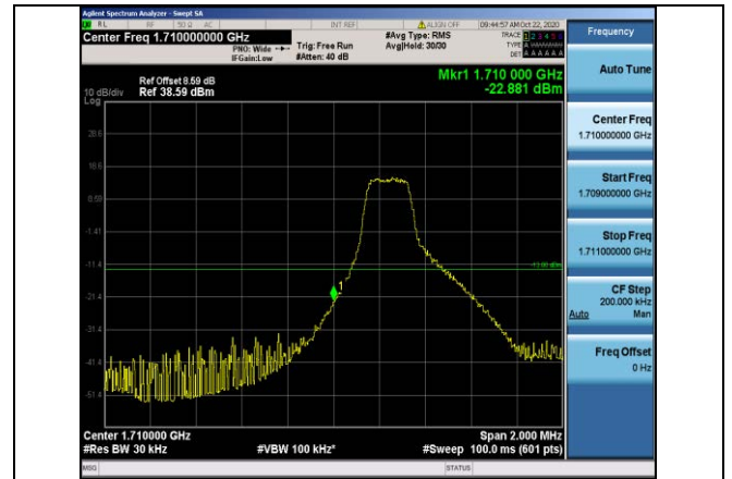
Band4-3MHz-16QAM-19965-1RB#0
