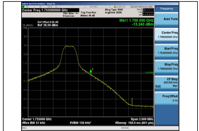
Band4-5MHz-QPSK-20375-1RB#24
