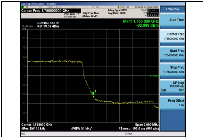
Band4-1.4MHz-QPSK-20393-6RB#0
