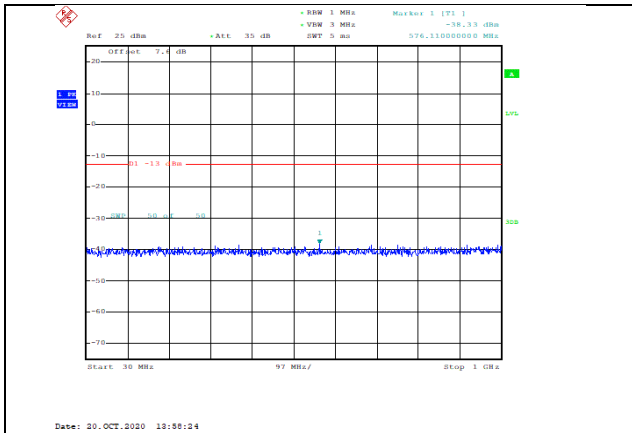
Band66-15MHz-16QAM-132322-1RB#0-Range1:30~1000MHz--38.33-PASS
