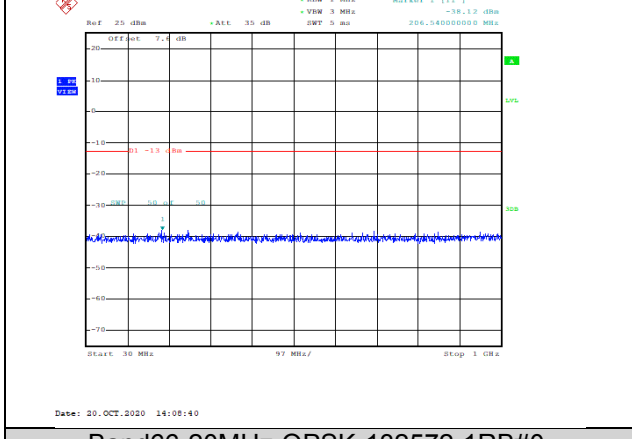
Band66-20MHz-QPSK-132572-1RB#0-Range1:30~1000MHz--38.12-PASS
