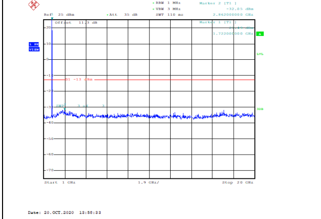
Band66-15MHz-16QAM-132322-1RB#0-Range2:1000~20000MHz--32.05-PASS
