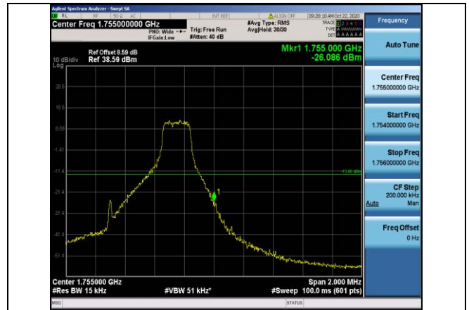
Band4-1.4MHz-16QAM-20393-1RB#5
