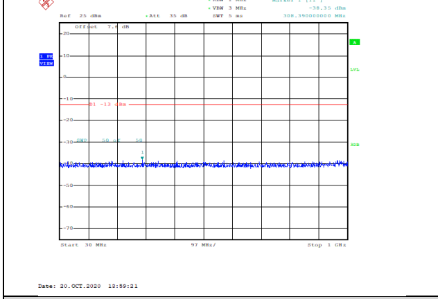
Band66-15MHz-16QAM-132597-1RB#0-Range1:30~1000MHz--38.35-PASS
