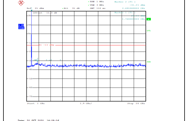
Band66-20MHz-16QAM-132572-1RB#0-Range2:1000~20000MHz--31.25-PASS
