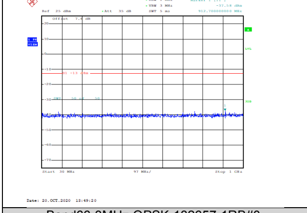
Band66-3MHz-QPSK-132657-1RB#0-Range1:30~1000MHz--37.58-PASS
