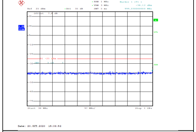
Band38-15MHz-QPSK-38175-1RB#0-Range1:30~1000MHz--38.12-PASS
