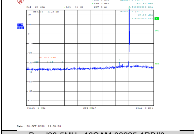
Band38-5MHz-16QAM-38225-1RB#0-Range2:1000~3000MHz--30.63-PASS
