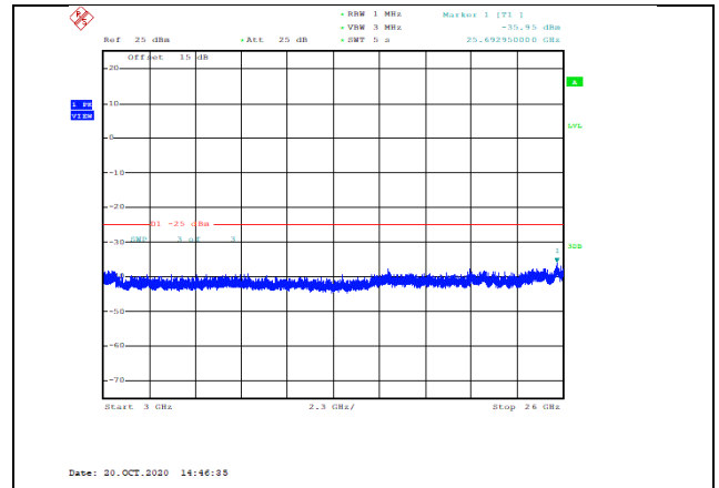
Band7-15MHz-16QAM-21375-1RB#0-Range3:3000~26000MHz--35.95-PASS
