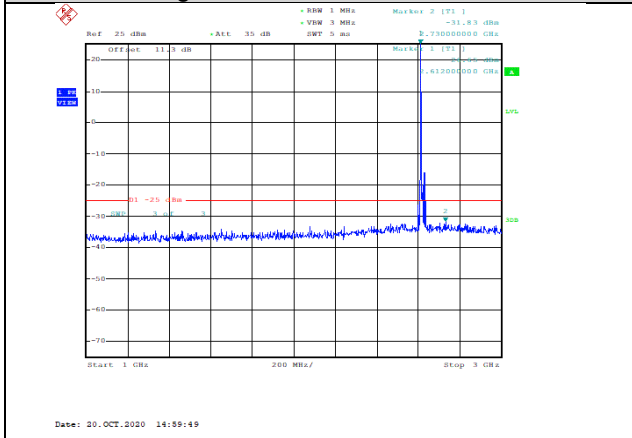
Band38-10MHz-16QAM-38200-1RB#0-Range2:1000~3000MHz--31.83-PASS
