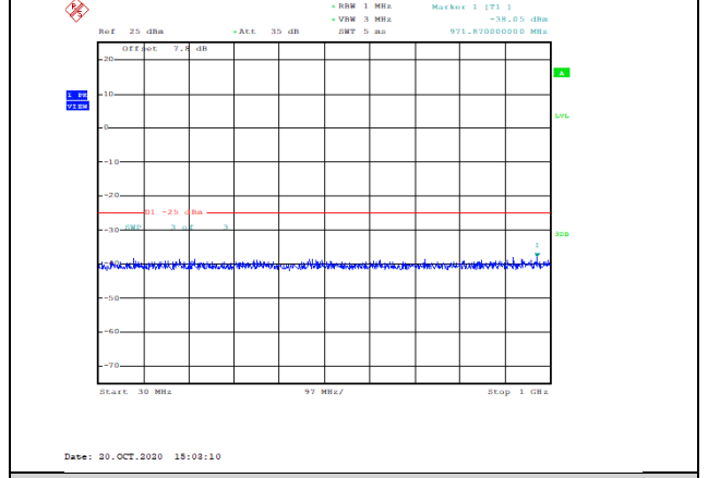
Band38-15MHz-16QAM-38000-1RB#0-Range1:30~1000MHz--38.05-PASS
