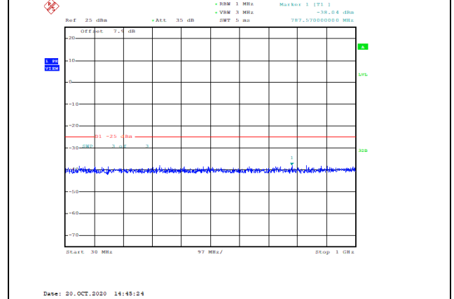
Band7-15MHz-QPSK-21375-1RB#0-Range1:30~1000MHz--38.04-PASS
