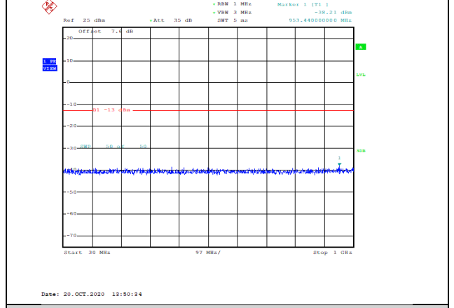
Band66-5MHz-16QAM-131997-1RB#0-Range1:30~1000MHz--38.21-PASS
