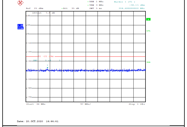
Band7-15MHz-16QAM-21100-1RB#0-Range1:30~1000MHz--38.15-PASS
