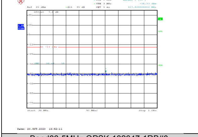
Band66-5MHz-QPSK-132647-1RB#0-Range1:30~1000MHz--38.33-PASS
