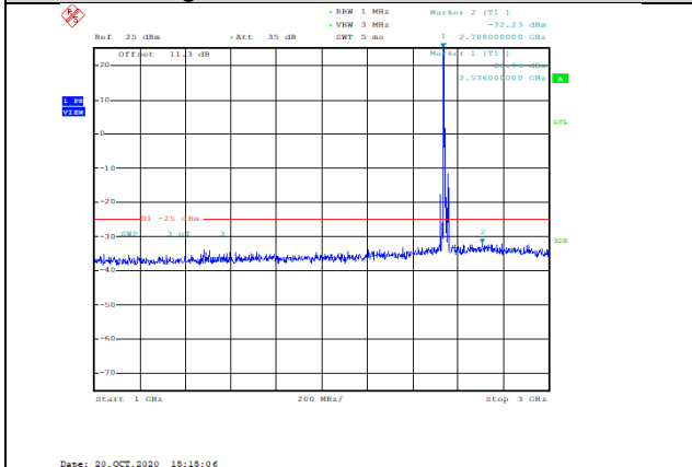
Band41-10MHz-16QAM-40090-1RB#0-Range2:1000~3000MHz--32.23-PASS
