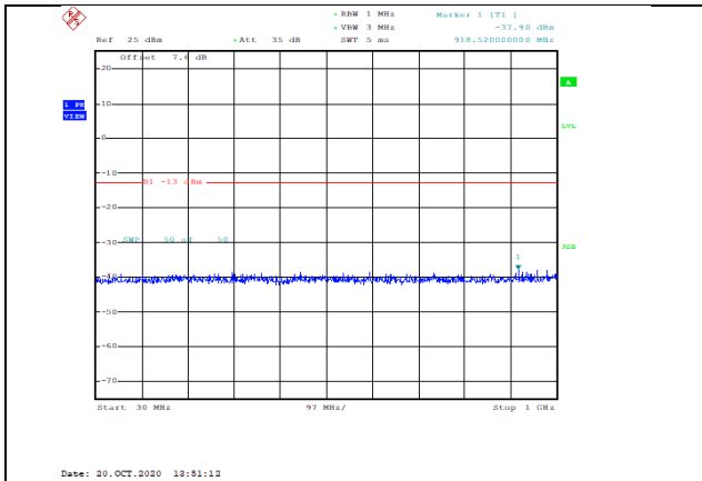
Band66-5MHz-16QAM-132322-1RB#0-Range1:30~1000MHz--37.9-PASS
