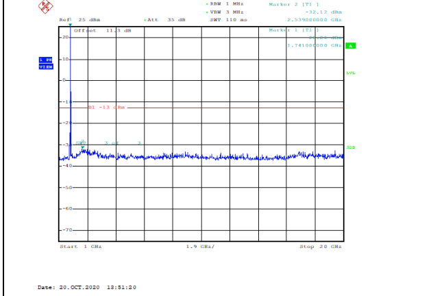
Band66-5MHz-16QAM-132322-1RB#0-Range2:1000~20000MHz--32.12-PASS
