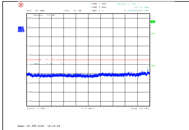
Band41-5MHz-16QAM-41215-1RB#0-Range3:3000~26000MHz--36.53-PASS
