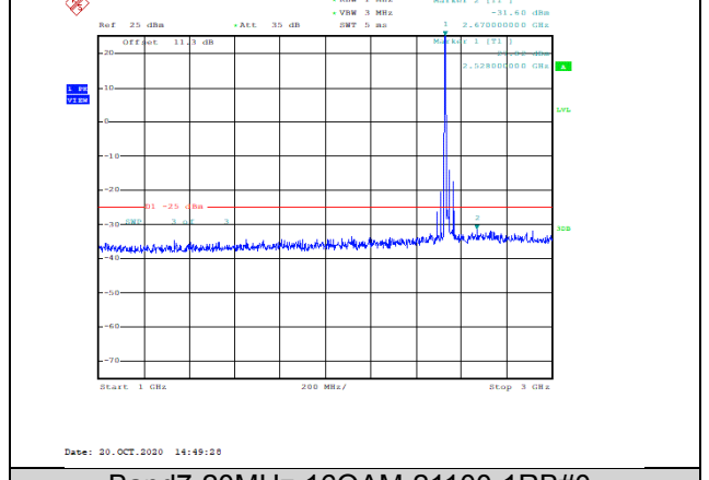
Band7-20MHz-16QAM-21100-1RB#0-Range2:1000~3000MHz--31.6-PASS
