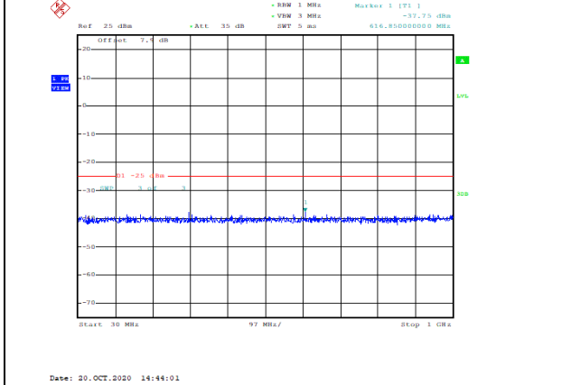
Band7-15MHz-QPSK-21100-1RB#0-Range1:30~1000MHz--37.75-PASS
