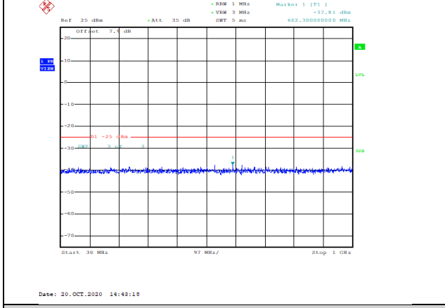
Band7-15MHz-16QAM-20825-1RB#0-Range1:30~1000MHz--37.81-PASS
