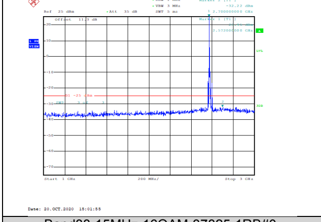
Band38-15MHz-16QAM-37825-1RB#0-Range2:1000~3000MHz--32.22-PASS
