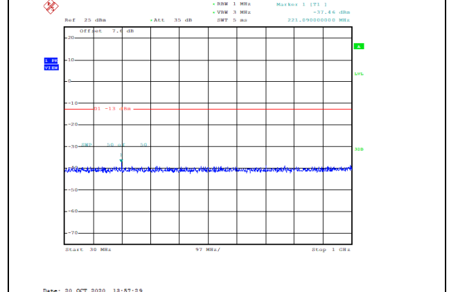
Band66-15MHz-QPSK-132047-1RB#0-Range1:30~1000MHz--37.46-PASS
