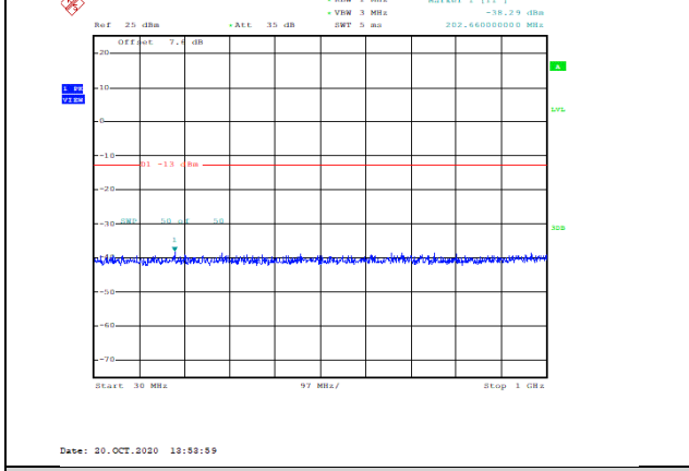
Band66-5MHz-16QAM-132647-1RB#0-Range1:30~1000MHz--38.29-PASS
