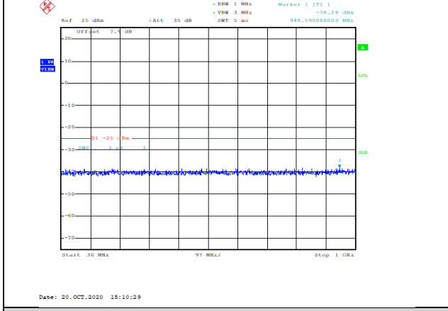
Band41-5MHz-16QAM-40065-1RB#0-Range1:30~1000MHz--38.28-PASS
