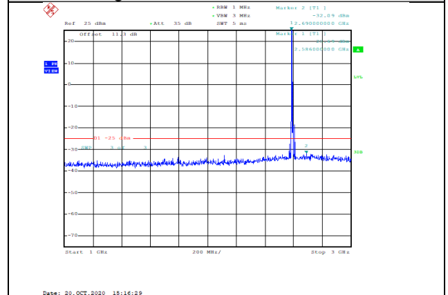
Band41-10MHz-16QAM-40590-1RB#0-Range2:1000~3000MHz--32.09-PASS
