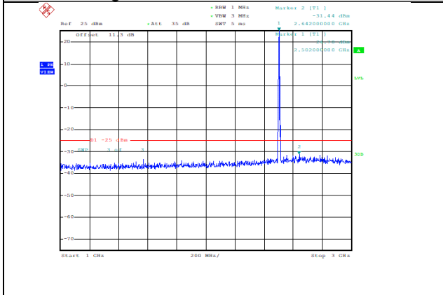
Band7-5MHz-16QAM-20775-1RB#0-Range2:1000~3000MHz--31.44-PASS
