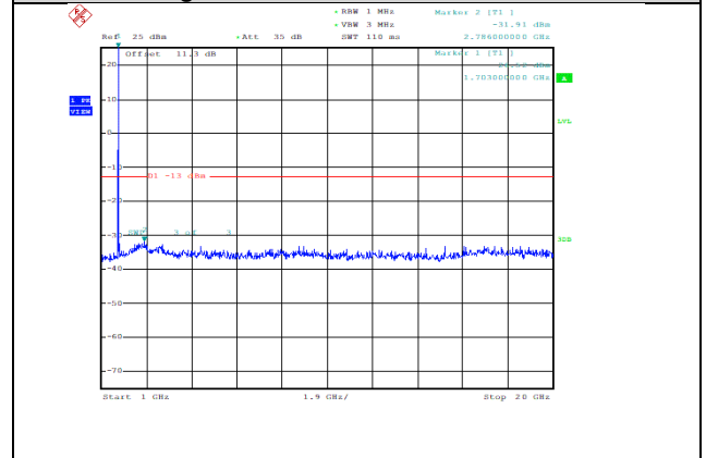
Band66-15MHz-QPSK-132047-1RB#0-Range2:1000~20000MHz--31.91-PASS
