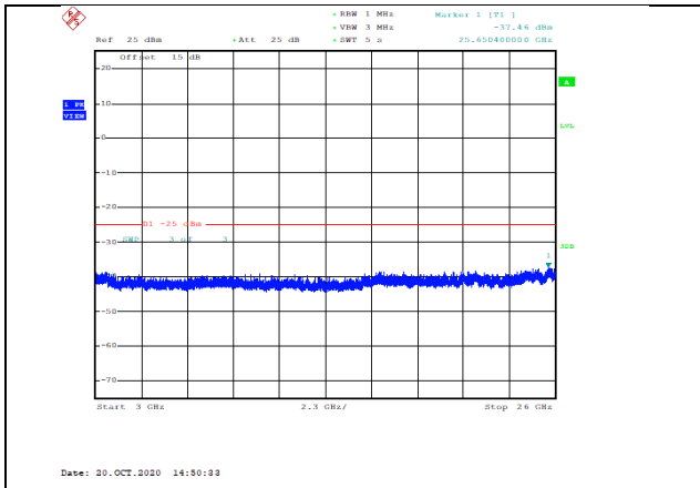
Band7-20MHz-QPSK-21350-1RB#0-Range3:3000~26000MHz--37.46-PASS
