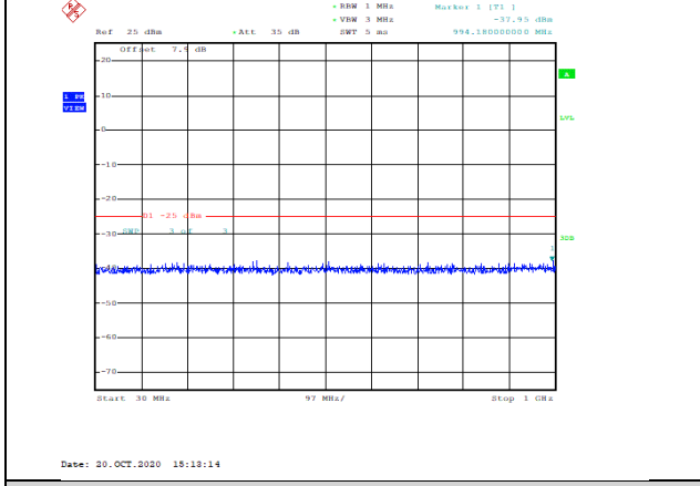
Band41-5MHz-16QAM-41215-1RB#0-Range1:30~1000MHz--37.95-PASS
