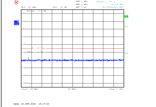
Band41-10MHz-16QAM-41190-1RB#0-Range1:30~1000MHz--38.3-PASS
