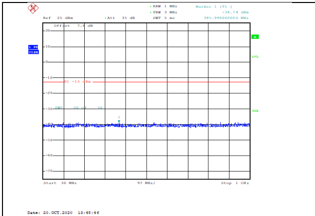
Band66-3MHz-16QAM-132322-1RB#0-Range1:30~1000MHz--38.74-PASS
