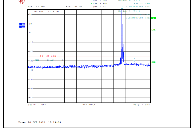
Band41-15MHz-QPSK-40115-1RB#0-Range2:1000~3000MHz--31.22-PASS
