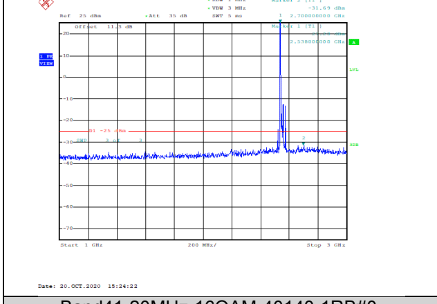
Band41-20MHz-16QAM-40140-1RB#0-Range2:1000~3000MHz--31.69-PASS
