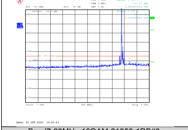
Band7-20MHz-16QAM-21350-1RB#0-Range2:1000~3000MHz--31.37-PASS
