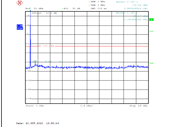
Band66-10MHz-QPSK-132322-1RB#0-Range2:1000~20000MHz--32.03-PASS
