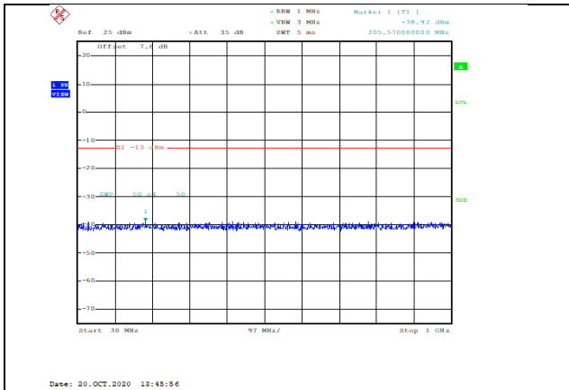
Band66-1.4MHz-QPSK-132322-1RB#0-Range1:30~1000MHz--38.92-PASS
