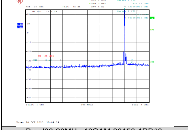
Band38-20MHz-16QAM-38150-1RB#0-Range2:1000~3000MHz--32.39-PASS
