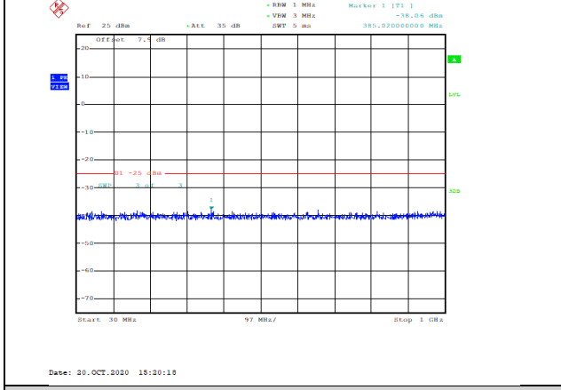
Band41-15MHz-QPSK-40590-1RB#0-Range1:30~1000MHz--38.06-PASS
