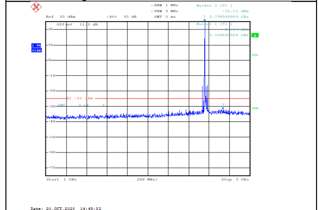
Band7-15MHz-QPSK-21375-1RB#0-Range2:1000~3000MHz--32.15-PASS
