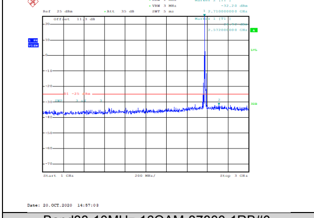
Band38-10MHz-16QAM-37800-1RB#0-Range2:1000~3000MHz--32.2-PASS
