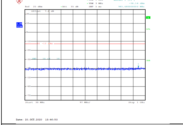
Band66-1.4MHz-QPSK-132665-1RB#0-Range1:30~1000MHz--38.54-PASS
