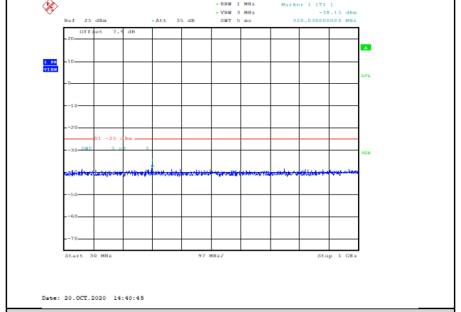
Band7-10MHz-QPSK-21400-1RB#0-Range1:30~1000MHz--38.15-PASS
