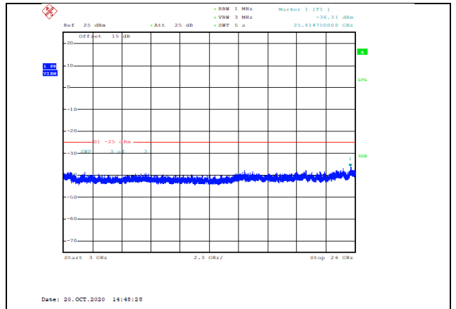
Band7-20MHz-16QAM-20850-1RB#0-Range3:3000~26000MHz--36.31-PASS
