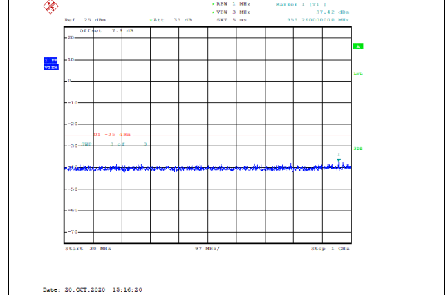
Band41-10MHz-16QAM-40590-1RB#0-Range1:30~1000MHz--37.42-PASS
