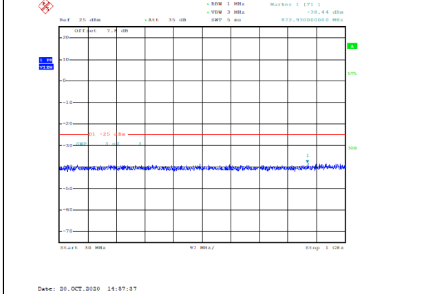
Band38-10MHz-QPSK-38000-1RB#0-Range1:30~1000MHz--38.44-PASS
