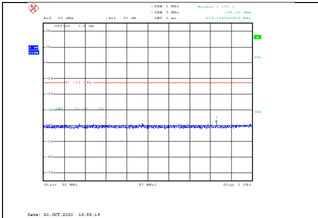
Band66-10MHz-QPSK-132322-1RB#0-Range1:30~1000MHz--38.3-PASS
