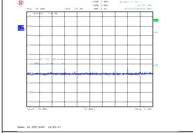
Band38-10MHz-16QAM-38000-1RB#0-Range1:30~1000MHz--37.8-PASS
