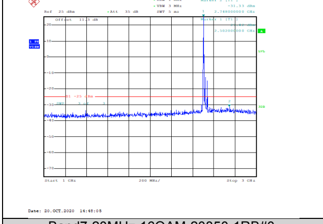
Band7-20MHz-16QAM-20850-1RB#0-Range2:1000~3000MHz--31.33-PASS
