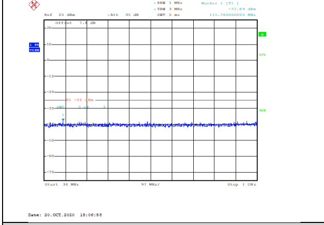
Band38-20MHz-QPSK-38000-1RB#0-Range1:30~1000MHz--37.89-PASS
