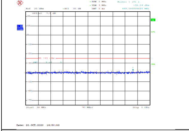
Band7-20MHz-16QAM-21350-1RB#0-Range1:30~1000MHz--38.24-PASS
