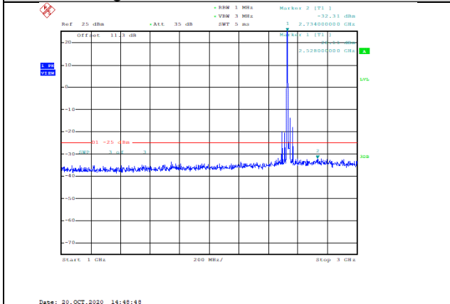
Band7-20MHz-QPSK-21100-1RB#0-Range2:1000~3000MHz--32.31-PASS
