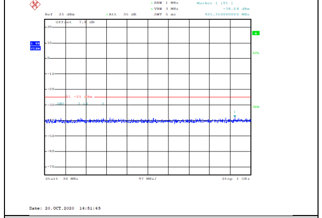
Band7-20MHz-16QAM-21350-1RB#0-Range1:30~1000MHz--38.04-PASS
