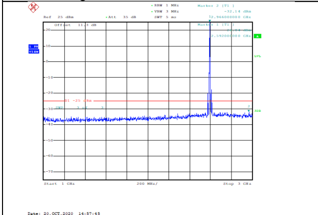
Band38-10MHz-QPSK-38000-1RB#0-Range2:1000~3000MHz--32.14-PASS
