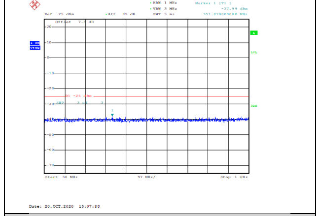
Band38-20MHz-16QAM-38000-1RB#0-Range1:30~1000MHz--37.99-PASS
