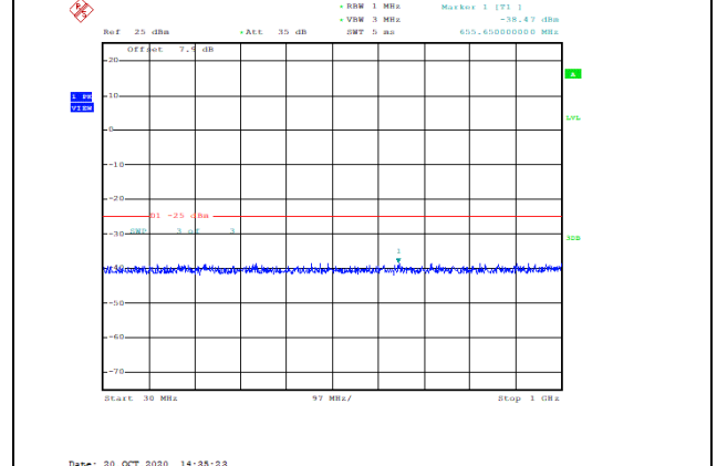
Band7-5MHz-16QAM-21100-1RB#0-Range1:30~1000MHz--38.47-PASS
