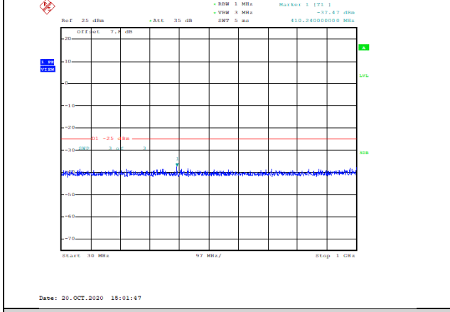
Band38-15MHz-16QAM-37825-1RB#0-Range1:30~1000MHz--37.47-PASS
