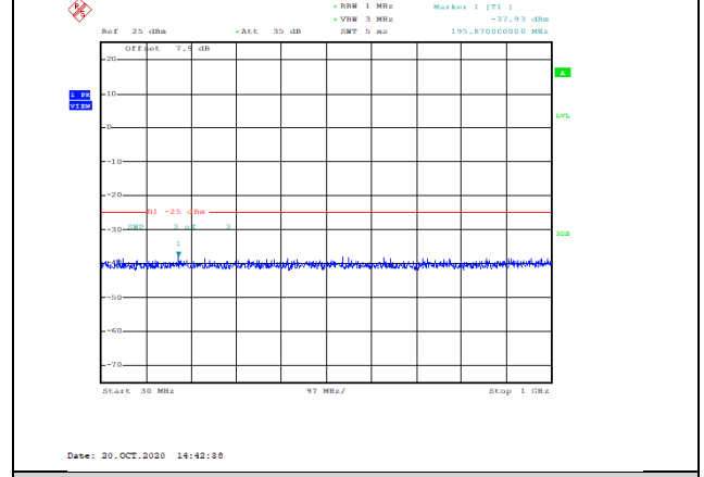
Band7-15MHz-QPSK-20825-1RB#0-Range1:30~1000MHz--37.93-PASS
