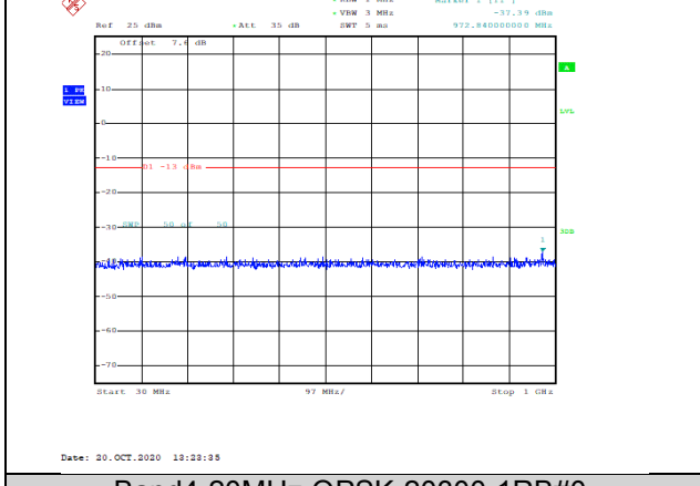
Band4-20MHz-QPSK-20300-1RB#0-Range1:30~1000MHz--37.39-PASS
