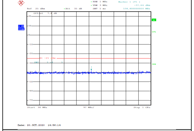
Band38-10MHz-QPSK-37800-1RB#0-Range1:30~1000MHz--37.66-PASS
