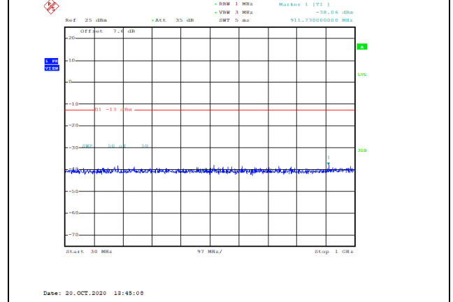
Band66-1.4MHz-16QAM-131979-1RB#0-Range1:30~1000MHz--38.06-PASS
