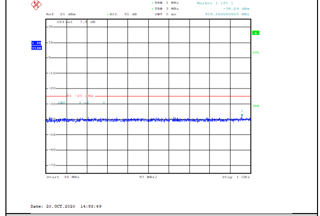
Band38-5MHz-16QAM-38000-1RB#0-Range1:30~1000MHz--38.08-PASS
