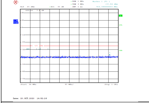
Band38-5MHz-16QAM-37775-1RB#0-Range1:30~1000MHz--37.94-PASS
