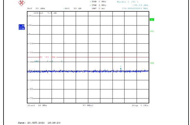
Band41-20MHz-QPSK-41140-1RB#0-Range1:30~1000MHz--38.29-PASS
