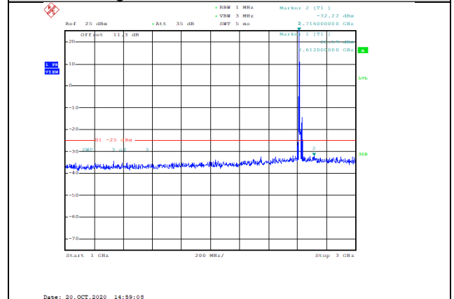
Band38-10MHz-QPSK-38200-1RB#0-Range2:1000~3000MHz--32.22-PASS
