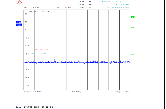
Band41-5MHz-QPSK-41215-1RB#0-Range1:30~1000MHz--38.46-PASS
