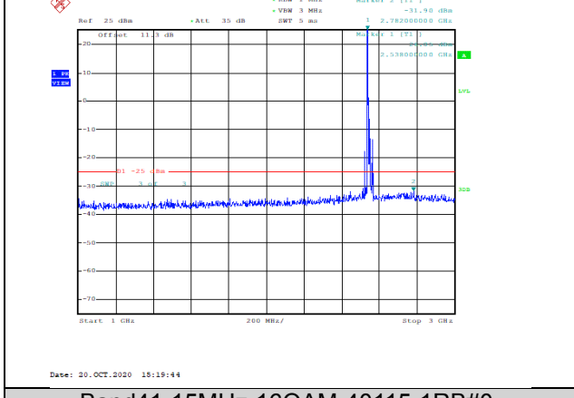
Band41-15MHz-16QAM-40115-1RB#0-Range2:1000~3000MHz--31.9-PASS
