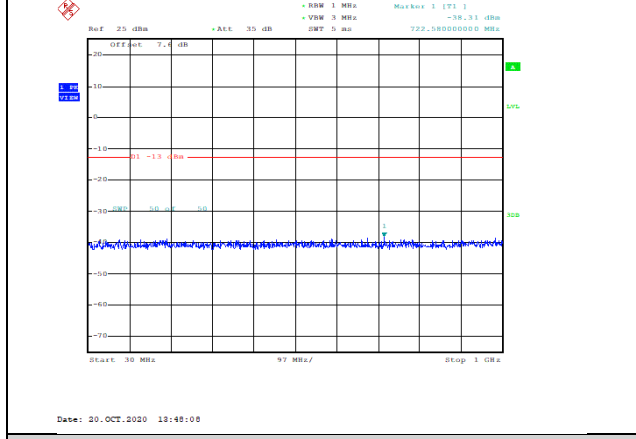
Band66-3MHz-16QAM-131987-1RB#0-Range1:30~1000MHz--38.31-PASS
