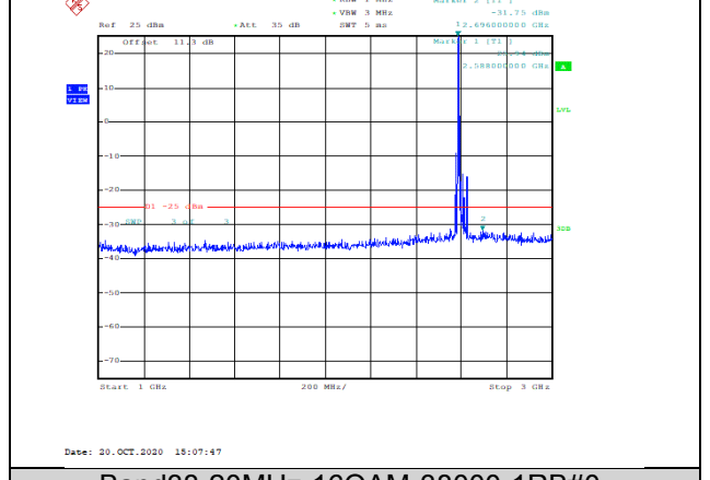
Band38-20MHz-16QAM-38000-1RB#0-Range2:1000~3000MHz--31.75-PASS
