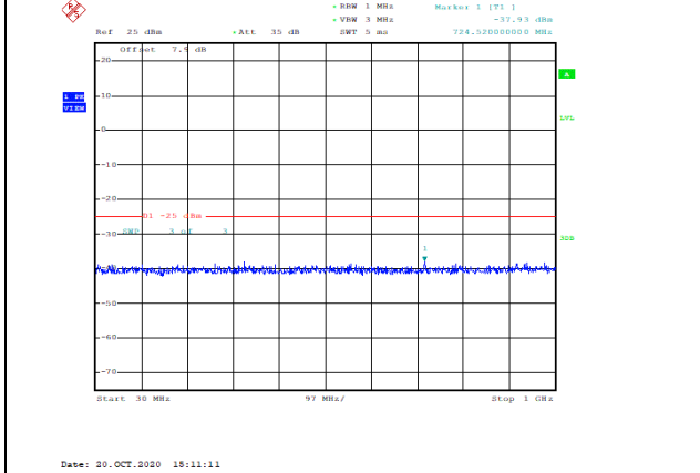
Band41-5MHz-QPSK-40590-1RB#0-Range1:30~1000MHz--37.93-PASS
