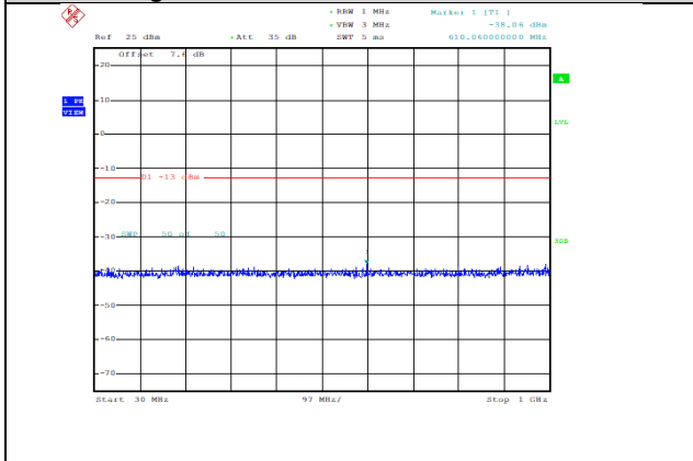
Band66-10MHz-16QAM-132622-1RB#0-Range1:30~1000MHz--38.06-PASS
