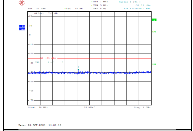
Band7-5MHz-QPSK-21425-1RB#0-Range1:30~1000MHz--37.97-PASS
