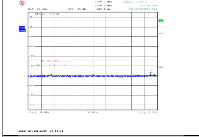
Band38-5MHz-QPSK-38225-1RB#0-Range1:30~1000MHz--37.88-PASS
