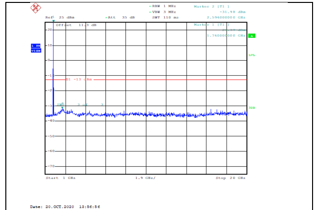
Band66-10MHz-16QAM-132622-1RB#0-Range2:1000~20000MHz--31.98-PASS
