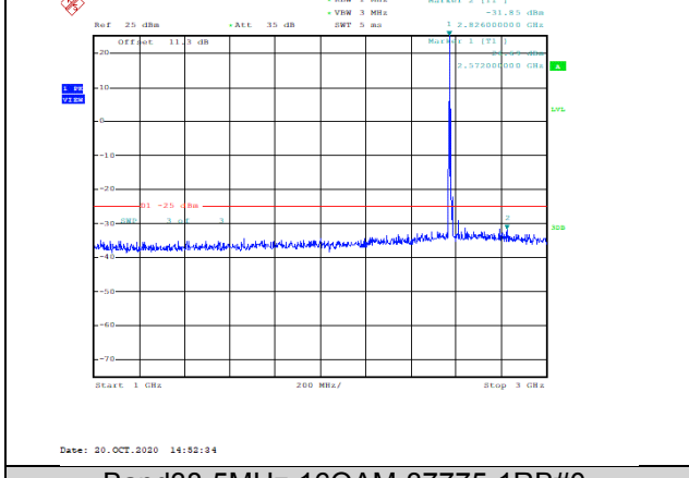
Band38-5MHz-16QAM-37775-1RB#0-Range2:1000~3000MHz--31.85-PASS
