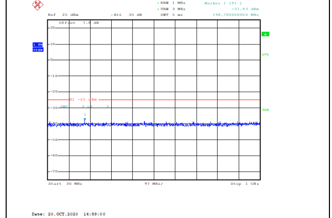
Band38-10MHz-QPSK-38200-1RB#0-Range1:30~1000MHz--37.93-PASS
