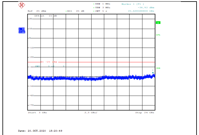
Band41-15MHz-QPSK-40590-1RB#0-Range3:3000~26000MHz--36.92-PASS
