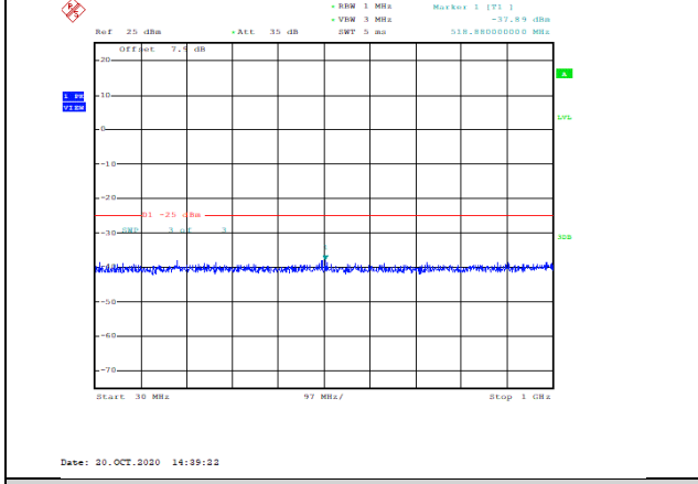
Band7-10MHz-QPSK-21100-1RB#0-Range1:30~1000MHz--37.89-PASS
