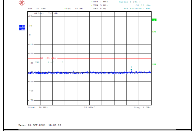
Band41-20MHz-16QAM-40590-1RB#0-Range1:30~1000MHz--37.99-PASS
