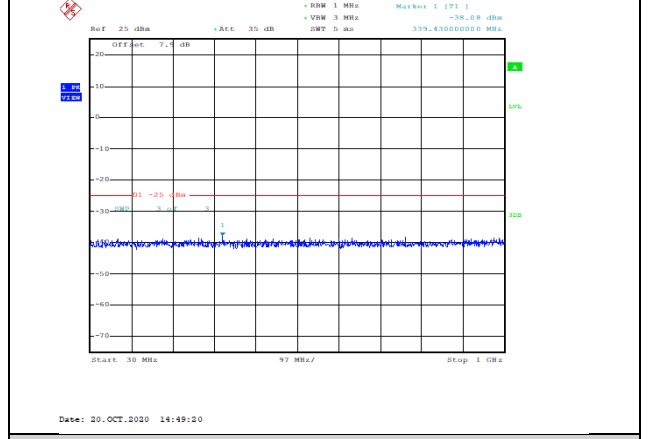
Band7-20MHz-16QAM-21100-1RB#0-Range1:30~1000MHz--38.08-PASS
