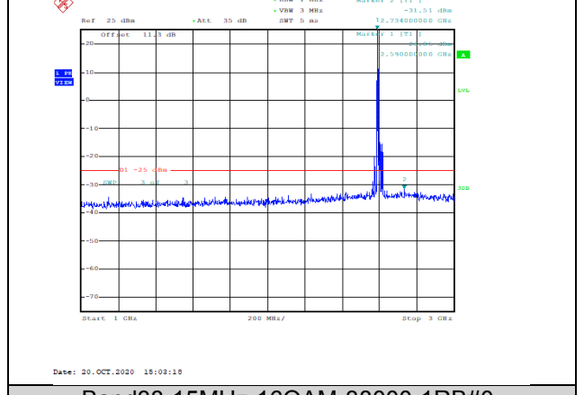
Band38-15MHz-16QAM-38000-1RB#0-Range2:1000~3000MHz--31.51-PASS
