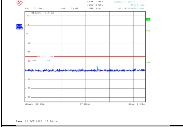
Band41-20MHz-16QAM-40140-1RB#0-Range1:30~1000MHz--37.46-PASS
