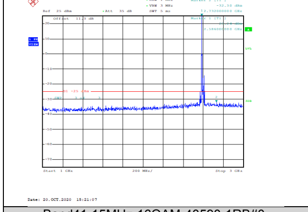
Band41-15MHz-16QAM-40590-1RB#0-Range2:1000~3000MHz--32.3-PASS
