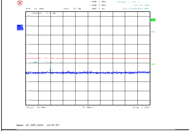
Band7-20MHz-16QAM-20850-1RB#0-Range1:30~1000MHz--37.96-PASS
