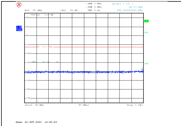
Band66-3MHz-QPSK-132322-1RB#0-Range1:30~1000MHz--38.53-PASS
