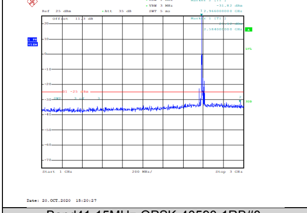
Band41-15MHz-QPSK-40590-1RB#0-Range2:1000~3000MHz--31.82-PASS
