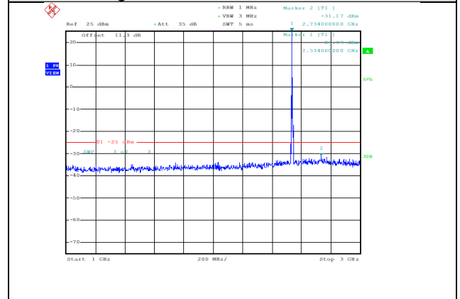
Band7-5MHz-16QAM-21100-1RB#0-Range2:1000~3000MHz--31.17-PASS
