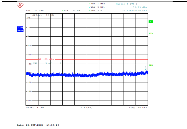
Band7-10MHz-16QAM-20800-1RB#0-Range3:3000~26000MHz--36.75-PASS
