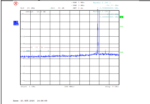
Band7-5MHz-16QAM-21425-1RB#0-Range2:1000~3000MHz--31.77-PASS
