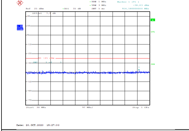
Band41-20MHz-16QAM-41140-1RB#0-Range1:30~1000MHz--38.03-PASS
