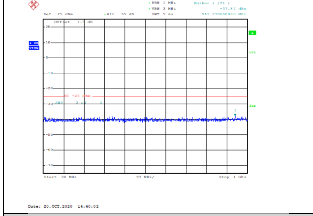
Band7-10MHz-16QAM-21100-1RB#0-Range1:30~1000MHz--37.87-PASS
