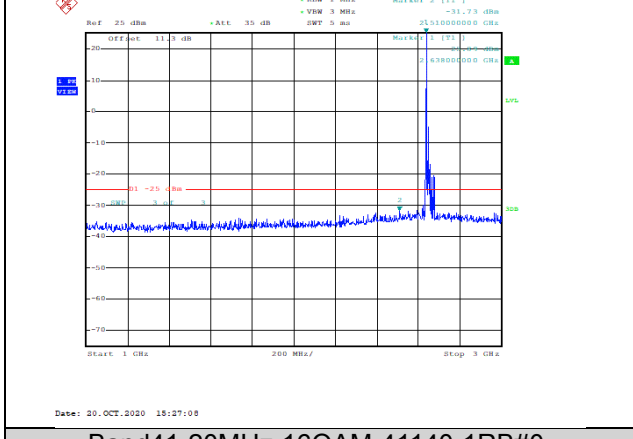
Band41-20MHz-16QAM-41140-1RB#0-Range2:1000~3000MHz--31.73-PASS
