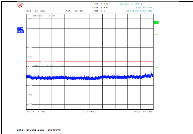
Band38-20MHz-16QAM-38000-1RB#0-Range3:3000~26000MHz--36.9-PASS
