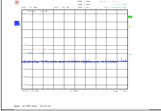
Band38-20MHz-16QAM-37850-1RB#0-Range1:30~1000MHz--37.27-PASS
