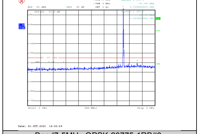
Band7-5MHz-QPSK-20775-1RB#0-Range2:1000~3000MHz--31.4-PASS
