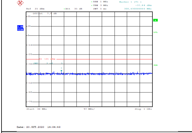
Band7-5MHz-QPSK-21100-1RB#0-Range1:30~1000MHz--37.84-PASS
