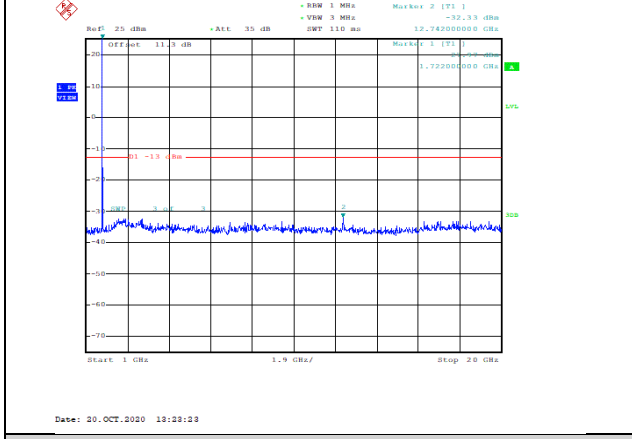
Band4-20MHz-16QAM-20175-1RB#0-Range2:1000~20000MHz--32.33-PASS
