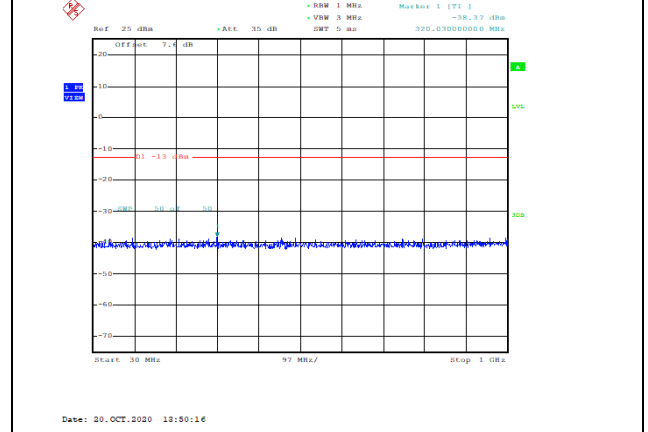
Band66-5MHz-QPSK-131997-1RB#0-Range1:30~1000MHz--38.37-PASS
