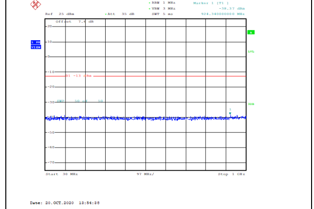
Band66-10MHz-QPSK-132022-1RB#0-Range1:30~1000MHz--38.37-PASS
