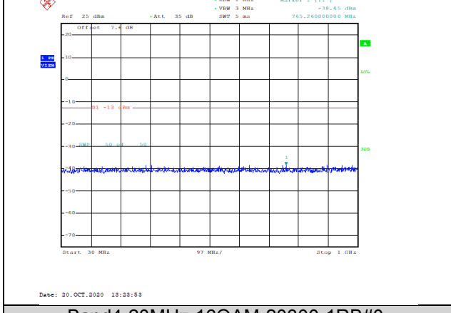
Band4-20MHz-16QAM-20300-1RB#0-Range1:30~1000MHz--38.45-PASS
