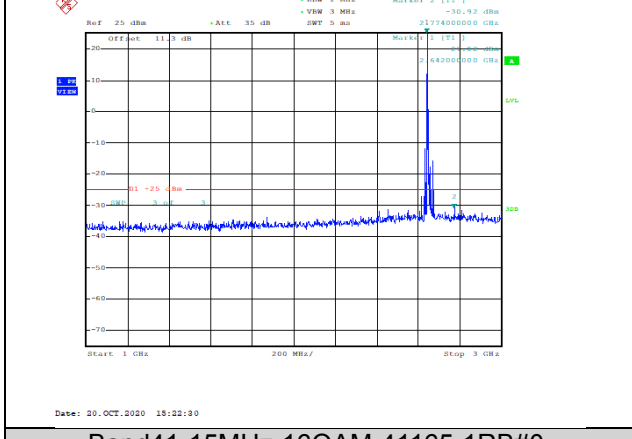
Band41-15MHz-16QAM-41165-1RB#0-Range2:1000~3000MHz--30.92-PASS
