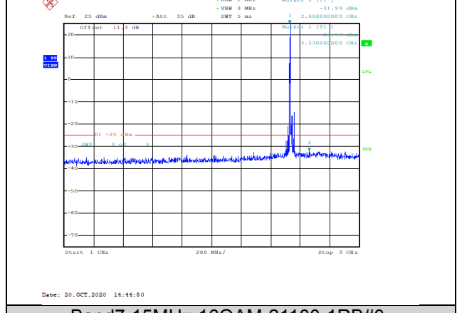
Band7-15MHz-16QAM-21100-1RB#0-Range2:1000~3000MHz--31.99-PASS
