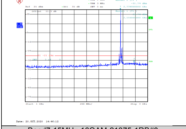
Band7-15MHz-16QAM-21375-1RB#0-Range2:1000~3000MHz--31.79-PASS
