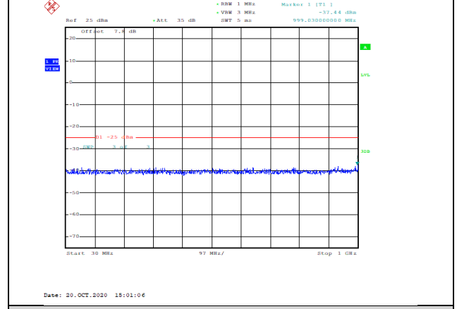
Band38-15MHz-QPSK-37825-1RB#0-Range1:30~1000MHz--37.44-PASS
