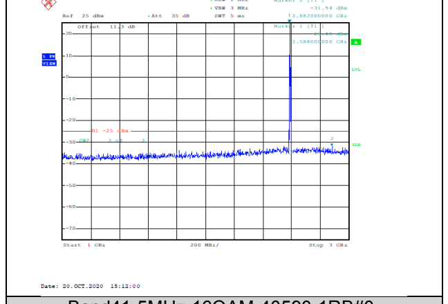
Band41-5MHz-16QAM-40590-1RB#0-Range2:1000~3000MHz--31.94-PASS
