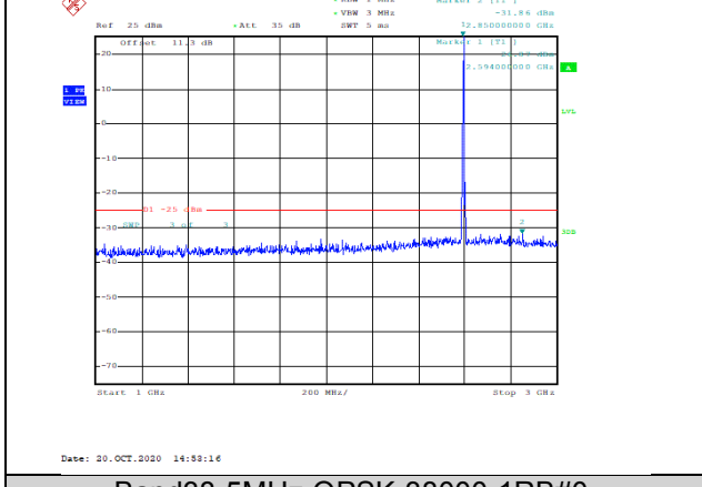
Band38-5MHz-QPSK-38000-1RB#0-Range2:1000~3000MHz--31.86-PASS
