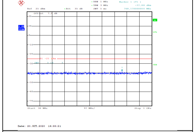
Band7-5MHz-QPSK-20775-1RB#0-Range1:30~1000MHz--37.88-PASS
