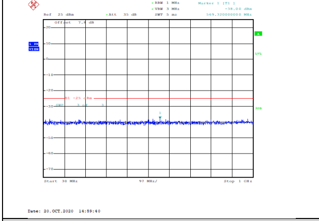
Band38-10MHz-16QAM-38200-1RB#0-Range1:30~1000MHz--38-PASS
