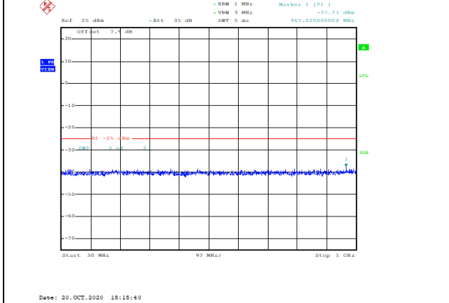
Band41-10MHz-QPSK-40590-1RB#0-Range1:30~1000MHz--37.71-PASS
