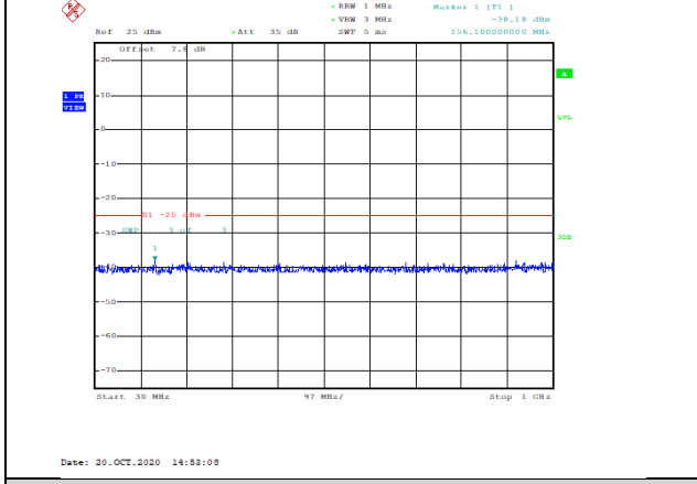
Band38-5MHz-QPSK-38000-1RB#0-Range1:30~1000MHz--38.18-PASS
