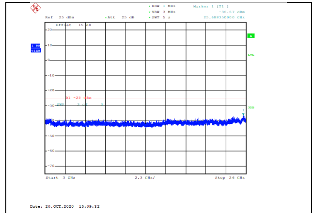
Band38-20MHz-16QAM-38150-1RB#0-Range3:3000~26000MHz--36.67-PASS
