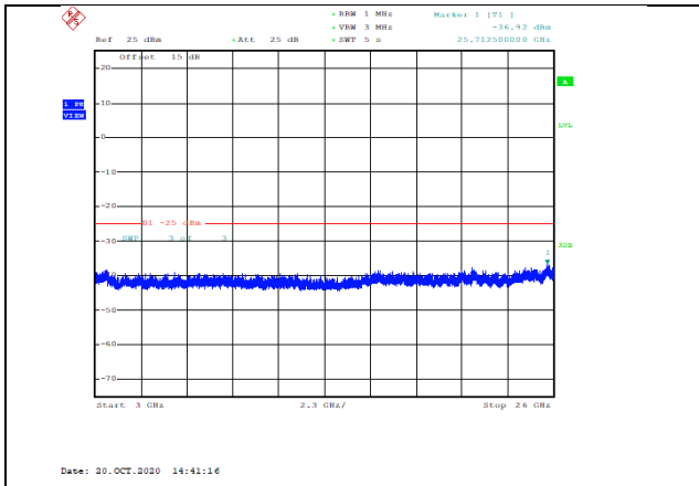
Band7-10MHz-QPSK-21400-1RB#0-Range3:3000~26000MHz--36.92-PASS
