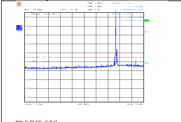
Band7-15MHz-QPSK-21100-1RB#0-Range2:1000~3000MHz--31.63-PASS
