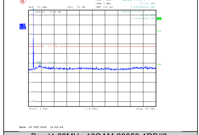
Band4-20MHz-16QAM-20050-1RB#0-Range2:1000~20000MHz--31.92-PASS
