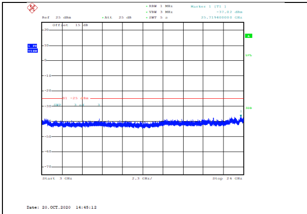
Band7-15MHz-16QAM-21100-1RB#0-Range3:3000~26000MHz--37.02-PASS
