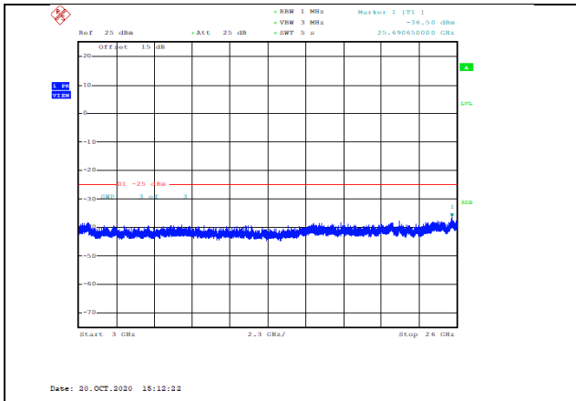
Band41-5MHz-16QAM-40590-1RB#0-Range3:3000~26000MHz--36.5-PASS
