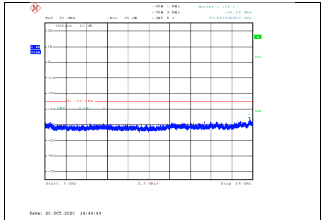
Band7-15MHz-16QAM-20825-1RB#0-Range3:3000~26000MHz--36.38-PASS
