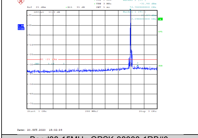
Band38-15MHz-QPSK-38000-1RB#0-Range2:1000~3000MHz--31.98-PASS
