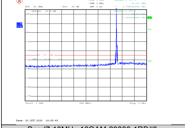
Band7-10MHz-16QAM-20800-1RB#0-Range2:1000~3000MHz--32.02-PASS
