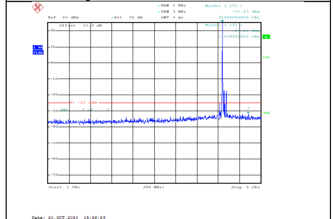
Band41-20MHz-QPSK-41140-1RB#0-Range2:1000~3000MHz--31.93-PASS
