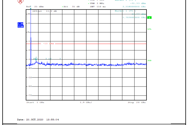
Band66-10MHz-16QAM-132022-1RB#0-Range2:1000~20000MHz--31.33-PASS
