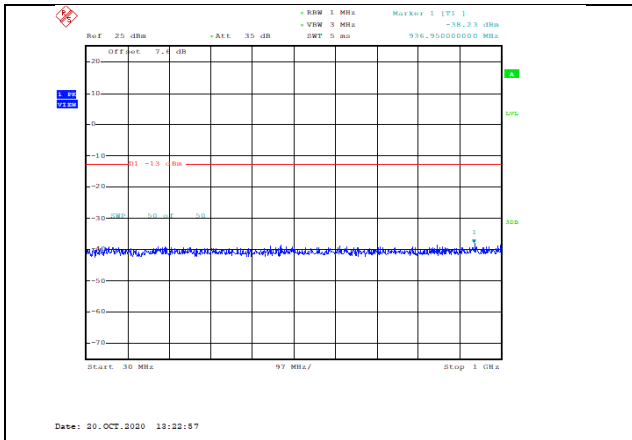
Band4-20MHz-QPSK-20175-1RB#0-Range1:30~1000MHz--38.23-PASS
