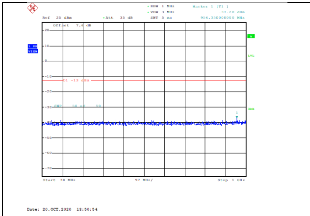
Band66-5MHz-QPSK-132322-1RB#0-Range1:30~1000MHz--37.28-PASS
