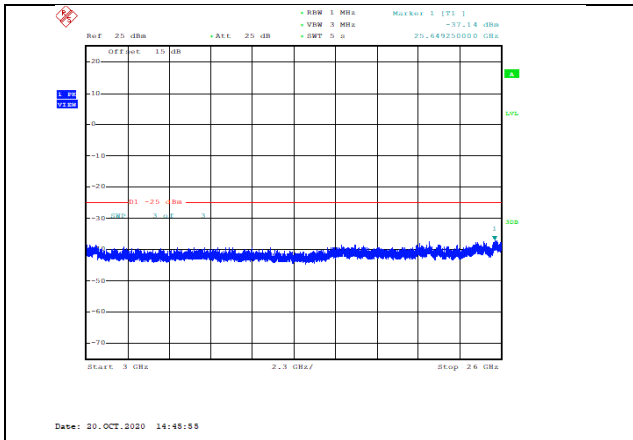
Band7-15MHz-QPSK-21375-1RB#0-Range3:3000~26000MHz--37.14-PASS
