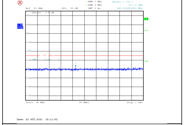
Band41-5MHz-16QAM-40590-1RB#0-Range1:30~1000MHz--37.13-PASS
