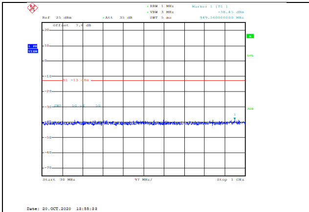
Band66-10MHz-16QAM-132322-1RB#0-Range1:30~1000MHz--38.45-PASS
