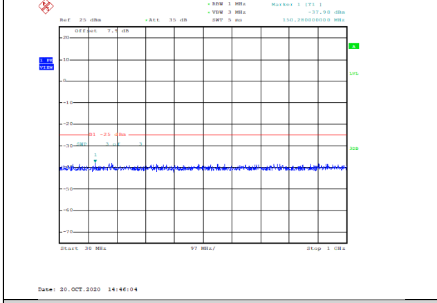
Band7-15MHz-16QAM-21375-1RB#0-Range1:30~1000MHz--37.9-PASS
