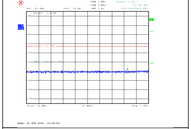
Band66-1.4MHz-QPSK-131979-1RB#0-Range1:30~1000MHz--37.96-PASS
