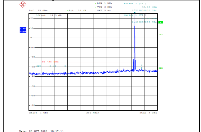
Band41-10MHz-QPSK-41190-1RB#0-Range2:1000~3000MHz--32.02-PASS
