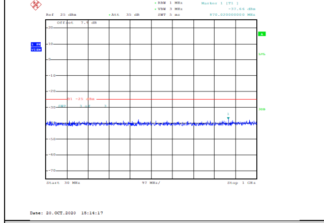
Band41-10MHz-QPSK-40090-1RB#0-Range1:30~1000MHz--37.66-PASS
