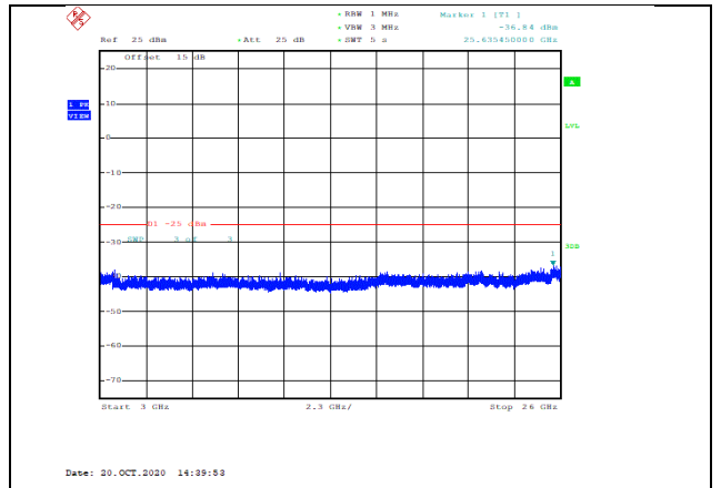
Band7-10MHz-QPSK-21100-1RB#0-Range3:3000~26000MHz--36.84-PASS
