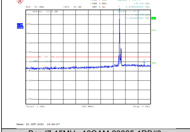
Band7-15MHz-16QAM-20825-1RB#0-Range2:1000~3000MHz--31.66-PASS
