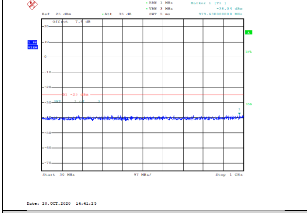
Band7-10MHz-16QAM-21400-1RB#0-Range1:30~1000MHz--38.04-PASS
