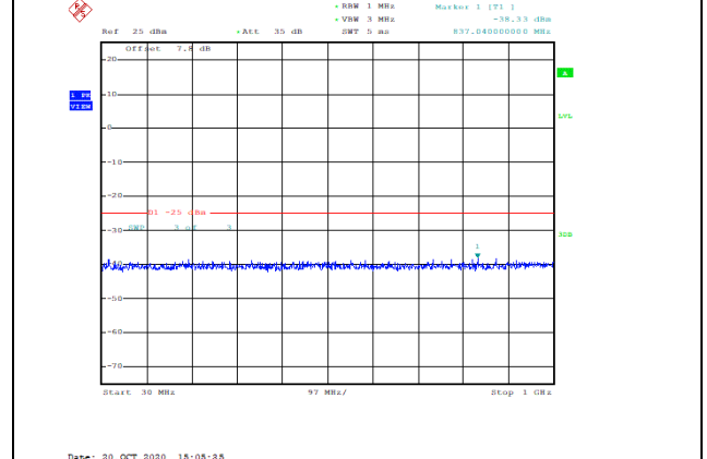
Band38-20MHz-QPSK-37850-1RB#0-Range1:30~1000MHz--38.33-PASS
