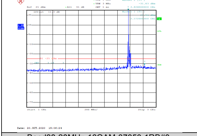
Band38-20MHz-16QAM-37850-1RB#0-Range2:1000~3000MHz--31.43-PASS
