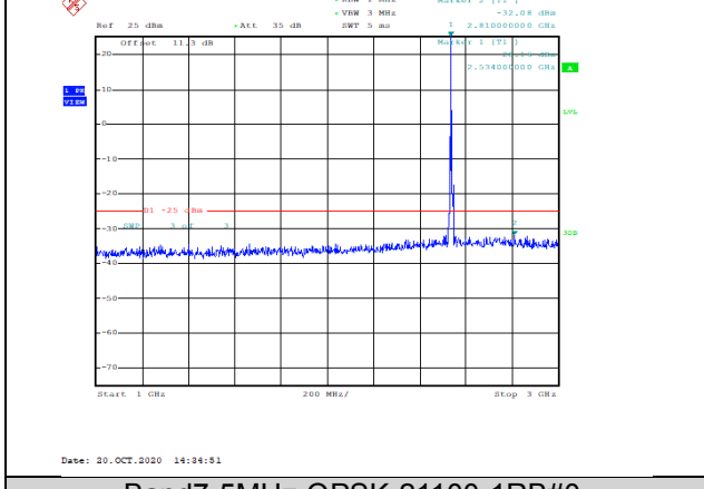
Band7-5MHz-QPSK-21100-1RB#0-Range2:1000~3000MHz--32.08-PASS
