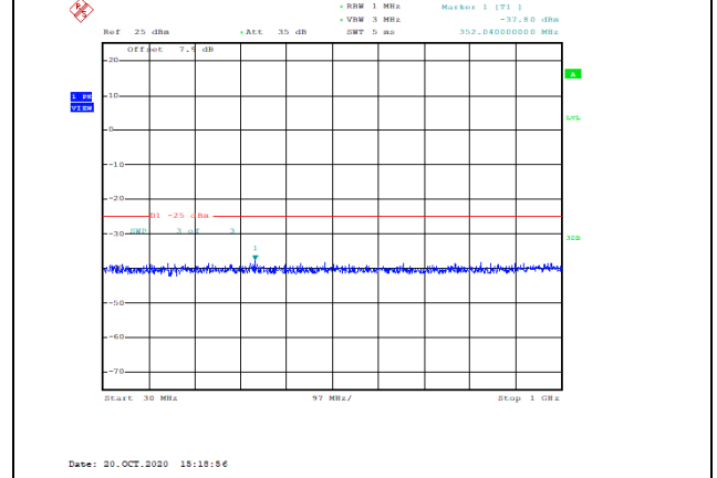
Band41-15MHz-QPSK-40115-1RB#0-Range1:30~1000MHz--37.8-PASS
