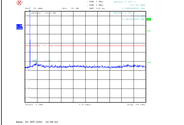
Band66-1.4MHz-16QAM-132322-1RB#0-Range2:1000~20000MHz--31.95-PASS
