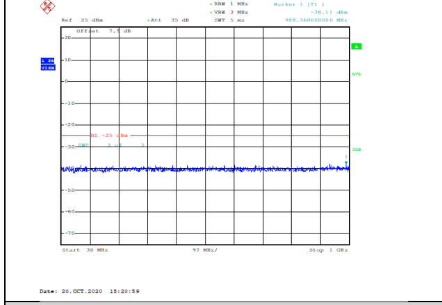
Band41-15MHz-16QAM-40590-1RB#0-Range1:30~1000MHz--38.11-PASS
