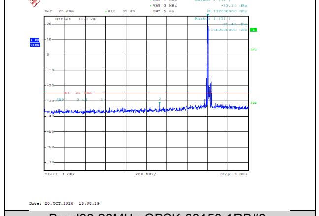
Band38-20MHz-QPSK-38150-1RB#0-Range2:1000~3000MHz--32.15-PASS
