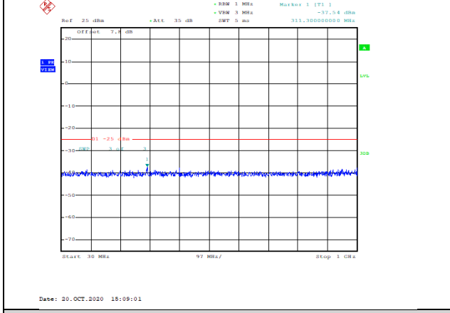
Band38-20MHz-16QAM-38150-1RB#0-Range1:30~1000MHz--37.54-PASS
