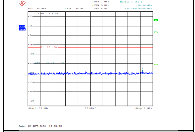
Band4-20MHz-16QAM-20050-1RB#0-Range1:30~1000MHz--38.56-PASS
