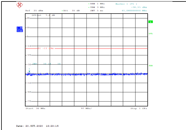
Band4-20MHz-16QAM-20175-1RB#0-Range1:30~1000MHz--38.35-PASS
