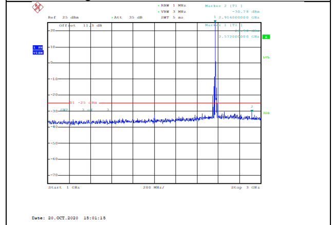
Band38-15MHz-QPSK-37825-1RB#0-Range2:1000~3000MHz--30.78-PASS
