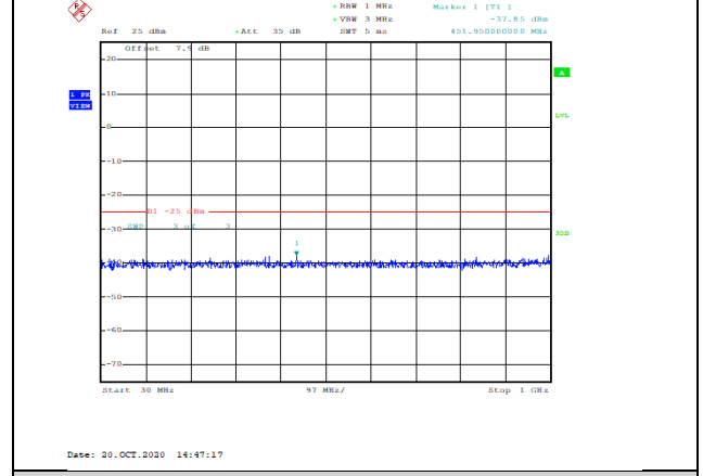
Band7-20MHz-QPSK-20850-1RB#0-Range1:30~1000MHz--37.85-PASS
