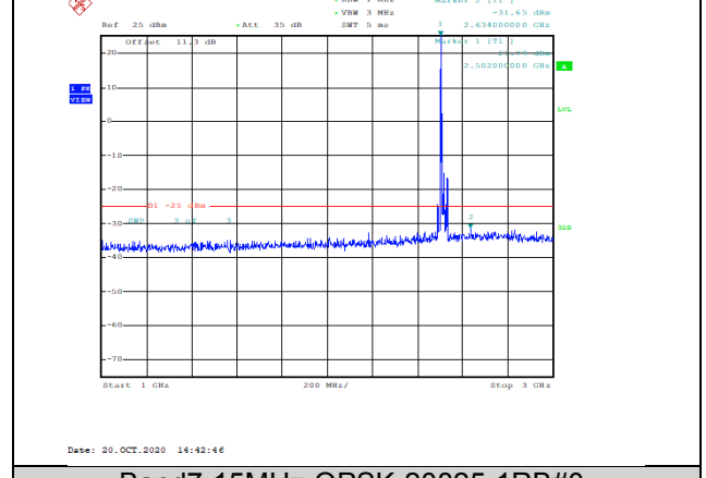
Band7-15MHz-QPSK-20825-1RB#0-Range2:1000~3000MHz--31.65-PASS
