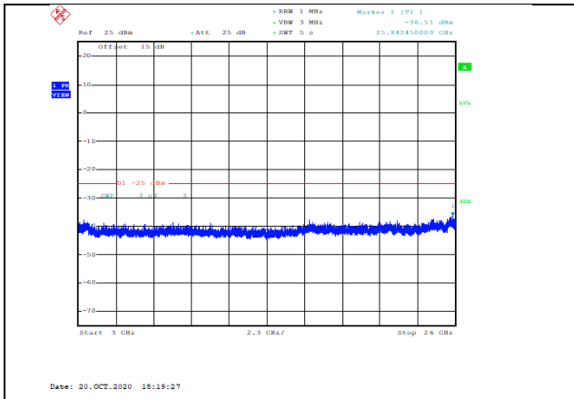
Band41-15MHz-QPSK-40115-1RB#0-Range3:3000~26000MHz--36.51-PASS
