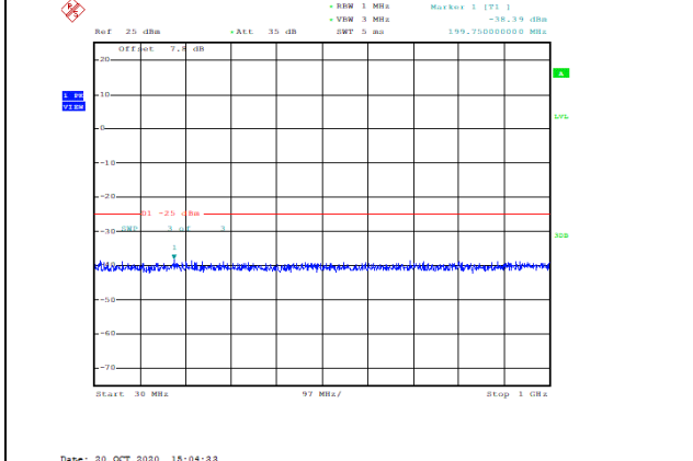
Band38-15MHz-16QAM-38175-1RB#0-Range1:30~1000MHz--38.39-PASS
