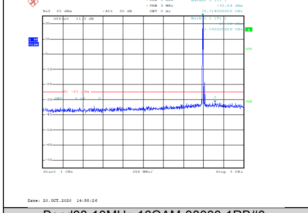
Band38-10MHz-16QAM-38000-1RB#0-Range2:1000~3000MHz--32.04-PASS
