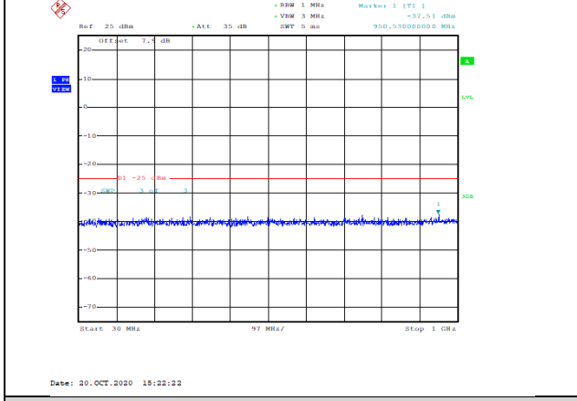
Band41-15MHz-16QAM-41165-1RB#0-Range1:30~1000MHz--37.51-PASS
