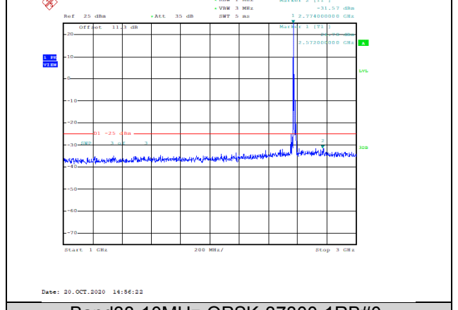
Band38-10MHz-QPSK-37800-1RB#0-Range2:1000~3000MHz--31.57-PASS
