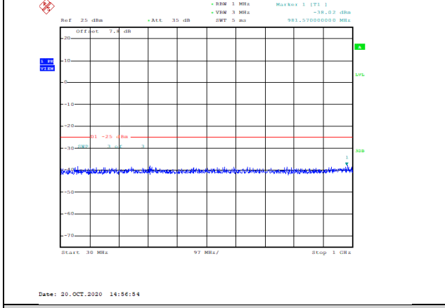
Band38-10MHz-16QAM-37800-1RB#0-Range1:30~1000MHz--38.02-PASS
