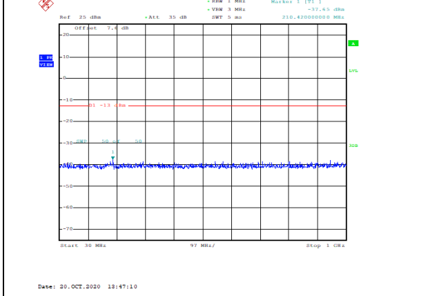
Band66-1.4MHz-16QAM-132665-1RB#0-Range1:30~1000MHz--37.65-PASS
