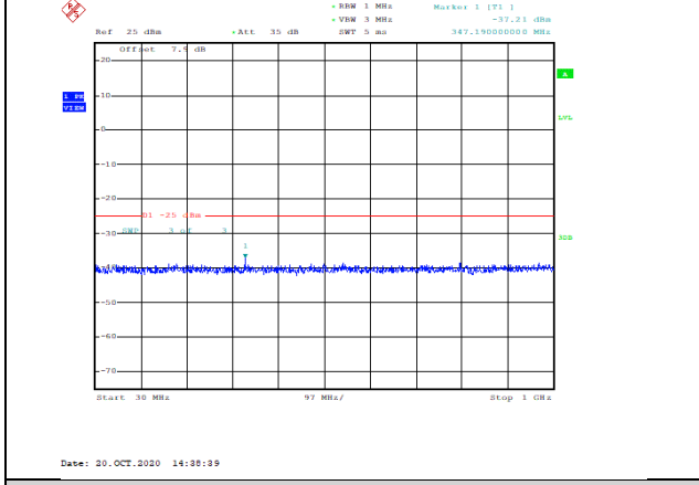
Band7-10MHz-16QAM-20800-1RB#0-Range1:30~1000MHz--37.21-PASS
