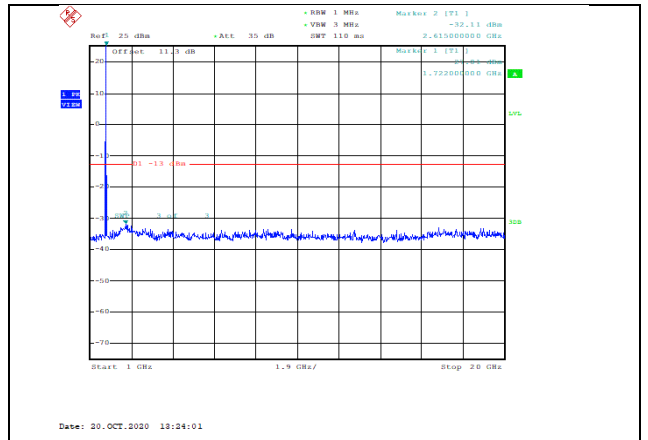
Band4-20MHz-16QAM-20300-1RB#0-Range2:1000~20000MHz--32.11-PASS
