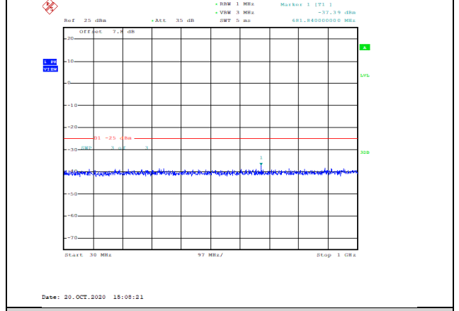
Band38-20MHz-QPSK-38150-1RB#0-Range1:30~1000MHz--37.39-PASS
