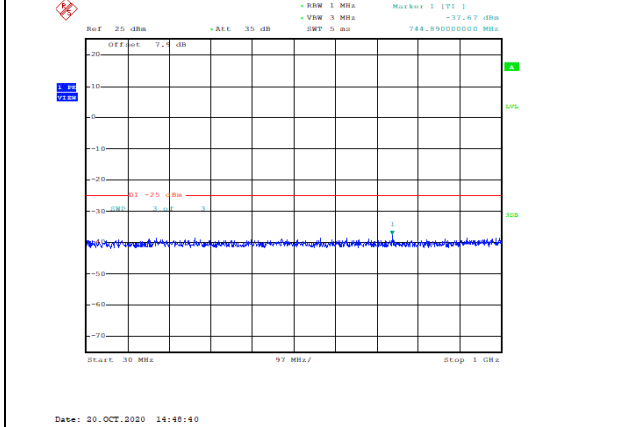
Band7-20MHz-QPSK-21100-1RB#0-Range1:30~1000MHz--37.67-PASS
