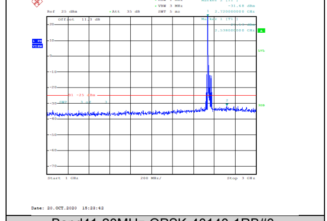
Band41-20MHz-QPSK-40140-1RB#0-Range2:1000~3000MHz--31.68-PASS
