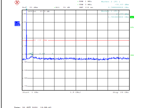
Band66-10MHz-16QAM-132322-1RB#0-Range2:1000~20000MHz--31.63-PASS
