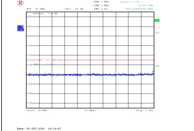
Band41-10MHz-16QAM-40090-1RB#0-Range1:30~1000MHz--37.8-PASS
