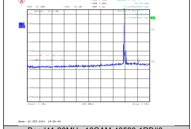
Band41-20MHz-16QAM-40590-1RB#0-Range2:1000~3000MHz--32.09-PASS
