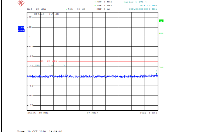
Band7-5MHz-16QAM-20775-1RB#0-Range1:30~1000MHz--38.05-PASS
