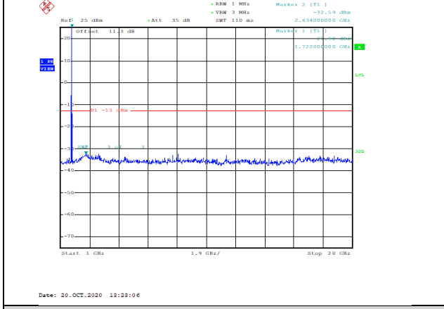
Band4-20MHz-QPSK-20175-1RB#0-Range2:1000~20000MHz--32.59-PASS
