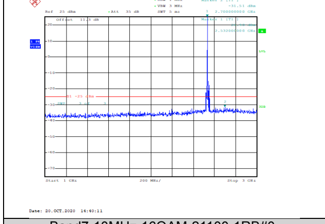
Band7-10MHz-16QAM-21100-1RB#0-Range2:1000~3000MHz--31.51-PASS
