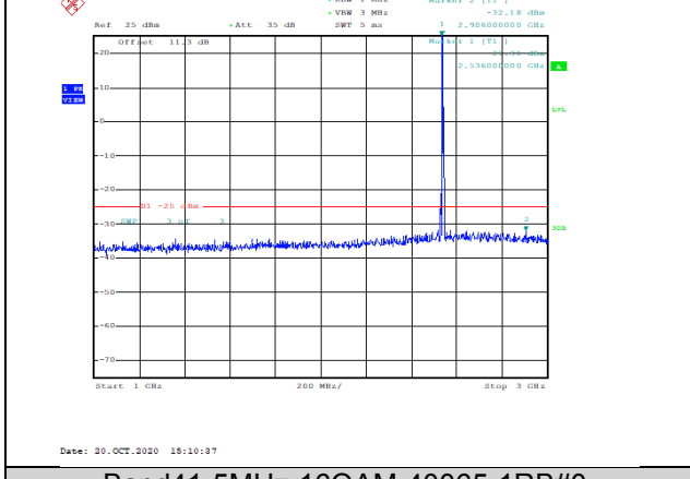
Band41-5MHz-16QAM-40065-1RB#0-Range2:1000~3000MHz--32.18-PASS
