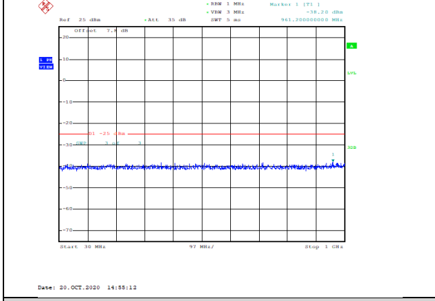
Band38-5MHz-16QAM-38225-1RB#0-Range1:30~1000MHz--38.2-PASS
