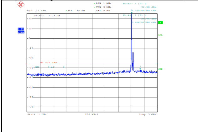
Band38-15MHz-16QAM-38175-1RB#0-Range2:1000~3000MHz--32.3-PASS
