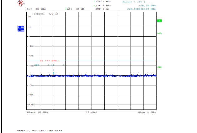
Band41-20MHz-QPSK-40590-1RB#0-Range1:30~1000MHz--38.18-PASS
