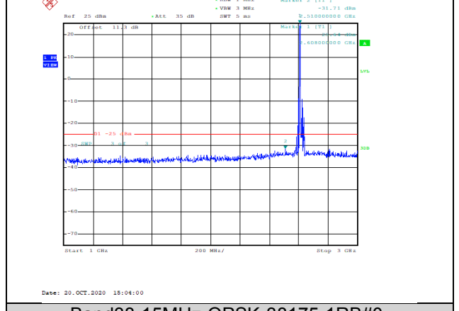
Band38-15MHz-QPSK-38175-1RB#0-Range2:1000~3000MHz--31.71-PASS
