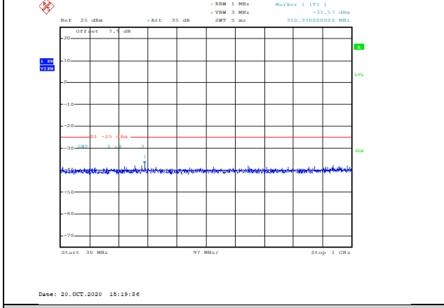
Band41-15MHz-16QAM-40115-1RB#0-Range1:30~1000MHz--37.57-PASS
