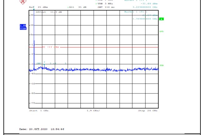
Band66-10MHz-QPSK-132022-1RB#0-Range2:1000~20000MHz--31.48-PASS
