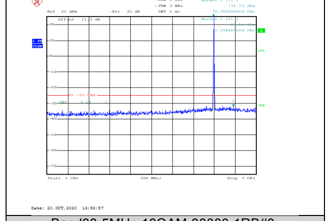
Band38-5MHz-16QAM-38000-1RB#0-Range2:1000~3000MHz--32.33-PASS
