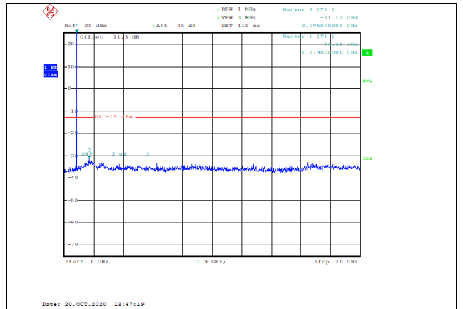
Band66-1.4MHz-16QAM-132665-1RB#0-Range2:1000~20000MHz--31.12-PASS
