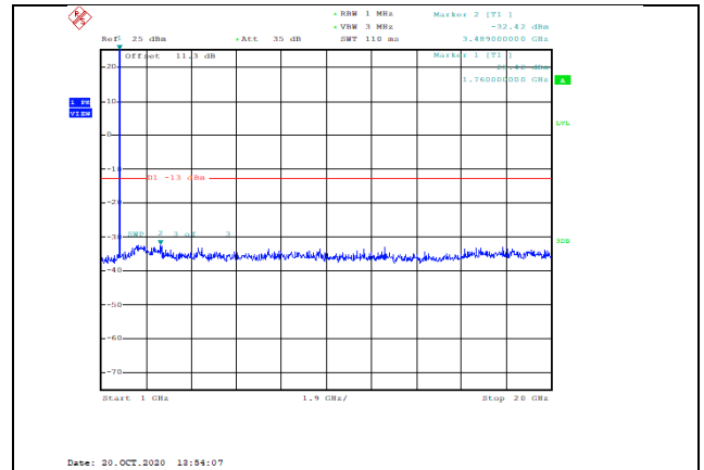
Band66-5MHz-16QAM-132647-1RB#0-Range2:1000~20000MHz--32.42-PASS
