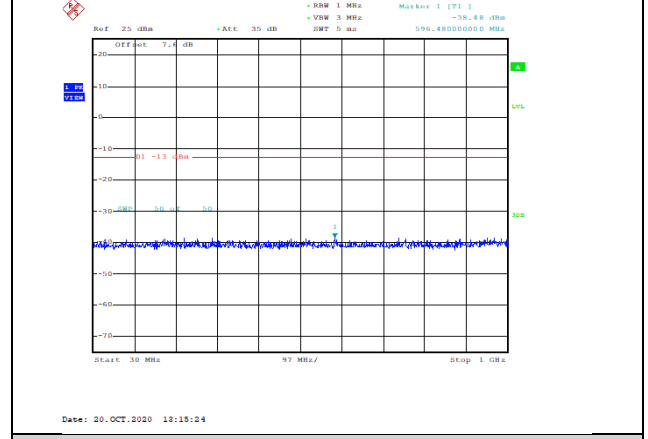
Band4-5MHz-QPSK-19975-1RB#0-Range1:30~1000MHz--38.48-PASS
