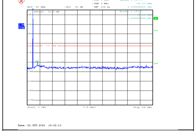
Band2-15MHz-QPSK-18675-1RB#0-Range2:1000~20000MHz--32.33-PASS
