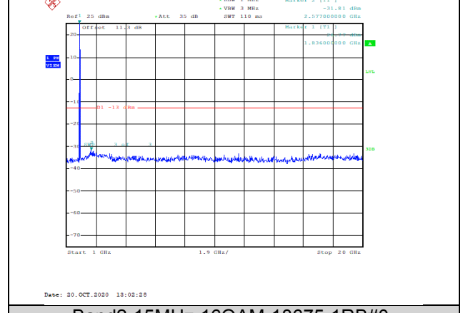
Band2-15MHz-16QAM-18675-1RB#0-Range2:1000~20000MHz--31.81-PASS
