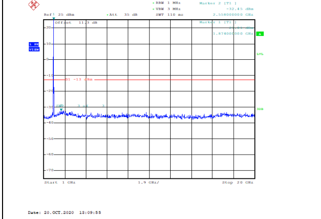
Band2-20MHz-16QAM-18900-1RB#0-Range2:1000~20000MHz--32.45-PASS
