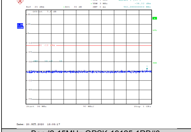
Band2-15MHz-QPSK-19125-1RB#0-Range1:30~1000MHz--38.32-PASS
