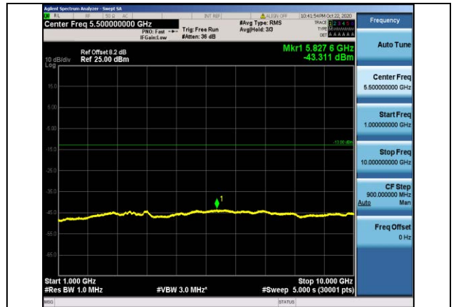
Band26-5MHz-16QAM-26740-1RB#0- Range2:1000~10000MHz
