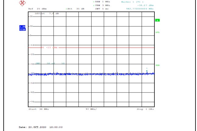
Band2-10MHz-16QAM-18650-1RB#0-Range1:30~1000MHz--38.07-PASS
