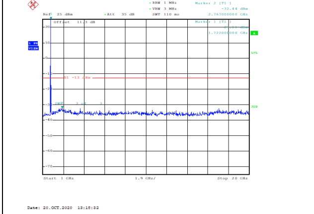
Band4-10MHz-QPSK-20175-1RB#0-Range2:1000~20000MHz--32.44-PASS
