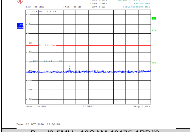
Band2-5MHz-16QAM-19175-1RB#0-Range1:30~1000MHz--38.4-PASS
