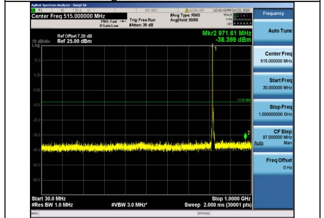
Band26-5MHz-16QAM-26765-1RB#0- Range1:30~1000MHz
