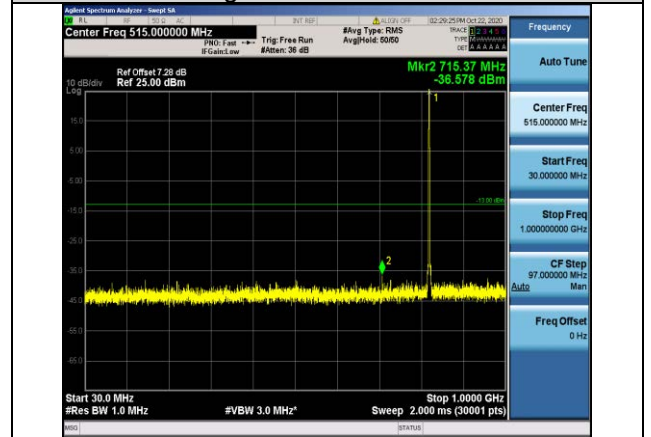
Band26-1.4MHz-16QAM-26783-1RB#0- Range1:30~1000MHz
