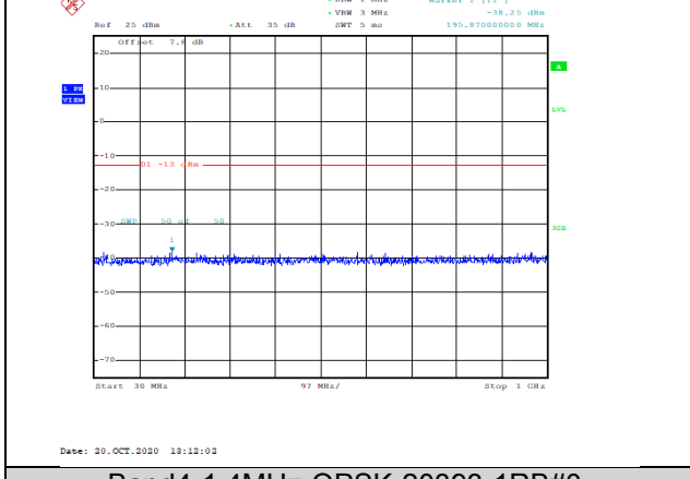
Band4-1.4MHz-QPSK-20393-1RB#0-Range1:30~1000MHz--38.25-PASS
