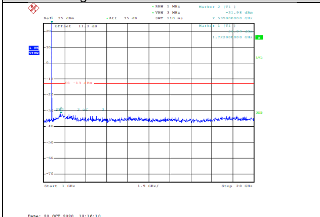
Band4-5MHz-QPSK-20175-1RB#0-Range2:1000~20000MHz--31.98-PASS
