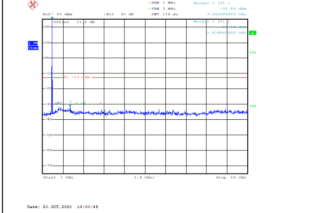
Band2-10MHz-16QAM-18900-1RB#0-Range2:1000~20000MHz--31.9-PASS
