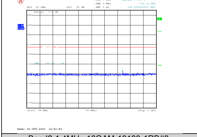
Band2-1.4MHz-16QAM-19193-1RB#0-Range1:30~1000MHz--38.14-PASS
