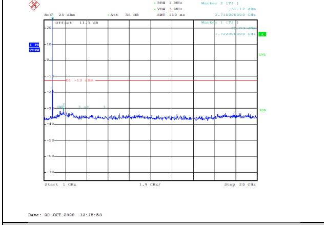
Band4-10MHz-16QAM-20175-1RB#0-Range2:1000~20000MHz--31.12-PASS
