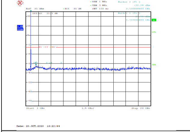
Band4-15MHz-QPSK-20175-1RB#0-Range2:1000~20000MHz--32.28-PASS
