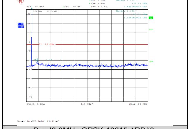
Band2-3MHz-QPSK-18615-1RB#0-Range2:1000~20000MHz--31.75-PASS
