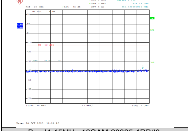
Band4-15MHz-16QAM-20325-1RB#0-Range1:30~1000MHz--38.34-PASS
