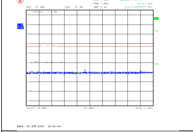
Band2-1.4MHz-QPSK-19193-1RB#0-Range1:30~1000MHz--38.03-PASS
