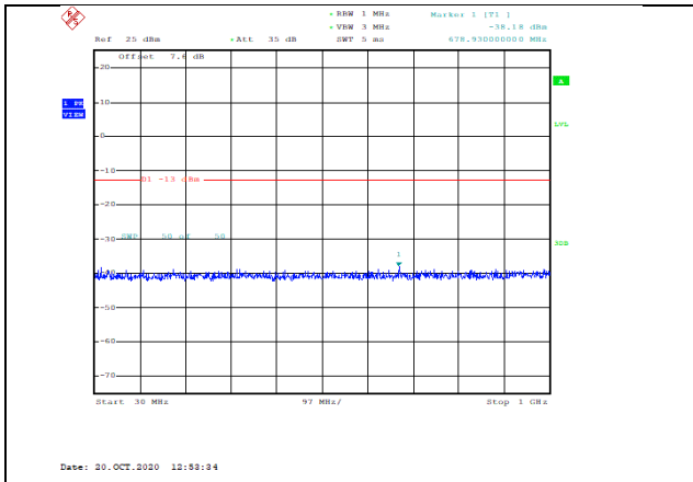
Band2-3MHz-16QAM-18900-1RB#0-Range1:30~1000MHz--38.18-PASS
