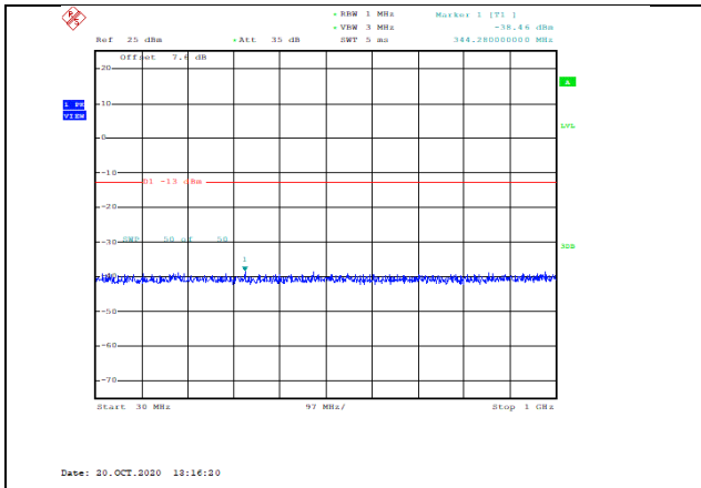
Band4-5MHz-16QAM-20175-1RB#0-Range1:30~1000MHz--38.46-PASS
