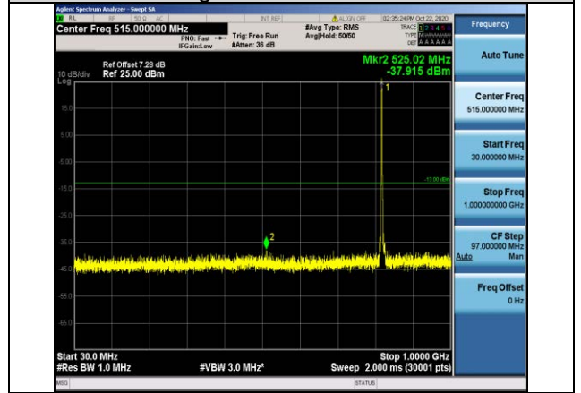
Band26-3MHz-QPSK-26775-1RB#0-Range1:30~1000MHz
