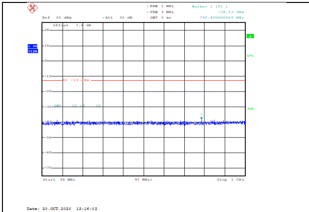
Band4-5MHz-QPSK-20175-1RB#0-Range1:30~1000MHz--38.33-PASS
