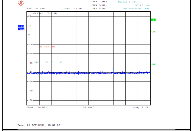
Band2-3MHz-QPSK-18615-1RB#0-Range1:30~1000MHz--38.45-PASS
