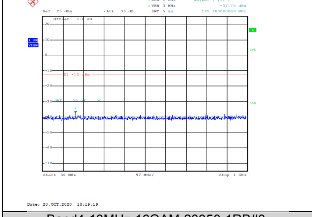
Band4-10MHz-16QAM-20350-1RB#0-Range1:30~1000MHz--37.72-PASS
