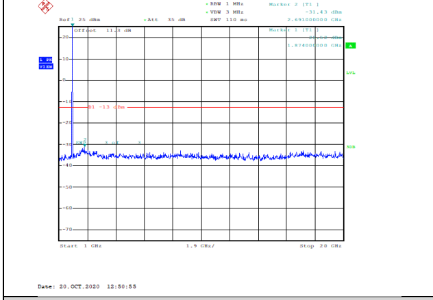
Band2-1.4MHz-16QAM-18900-1RB#0-Range2:1000~20000MHz--31.43-PASS
