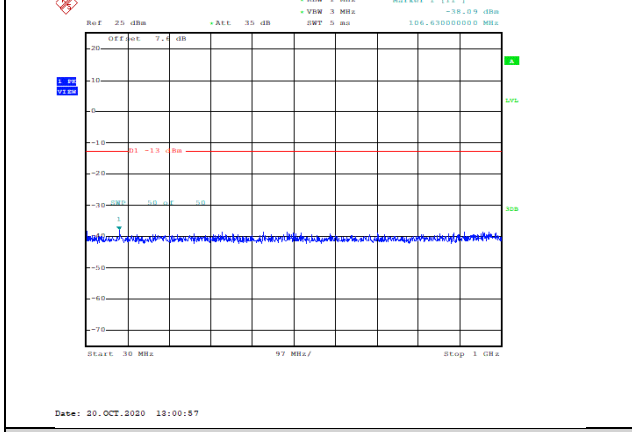
Band2-10MHz-QPSK-19150-1RB#0-Range1:30~1000MHz--38.09-PASS
