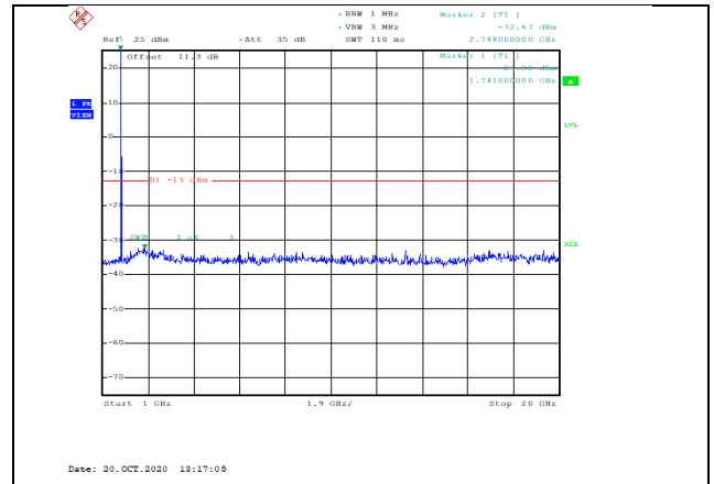
Band4-5MHz-16QAM-20375-1RB#0-Range2:1000~20000MHz--32.67-PASS
