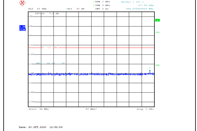
Band2-3MHz-16QAM-18615-1RB#0-Range1:30~1000MHz--37.98-PASS
