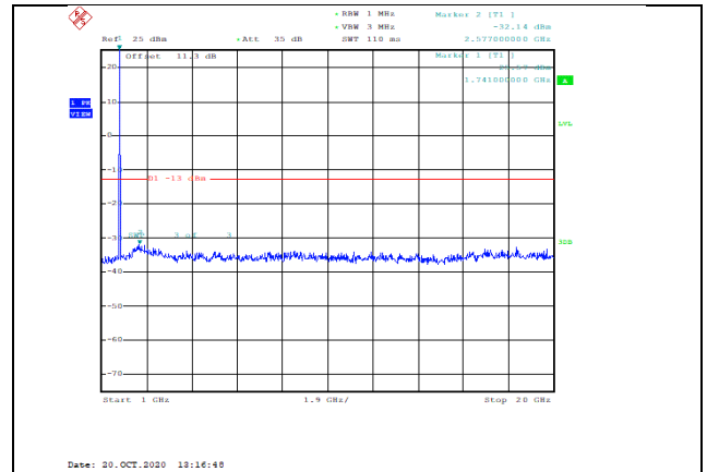
Band4-5MHz-QPSK-20375-1RB#0-Range2:1000~20000MHz--32.14-PASS
