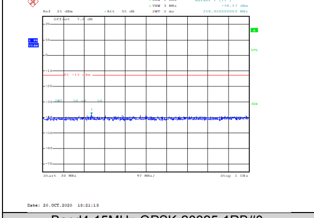
Band4-15MHz-QPSK-20325-1RB#0-Range1:30~1000MHz--38.37-PASS
