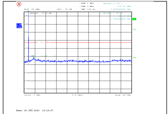
Band4-10MHz-16QAM-20350-1RB#0-Range2:1000~20000MHz--32.16-PASS
