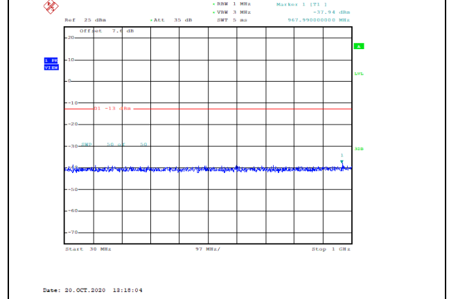
Band4-10MHz-16QAM-20000-1RB#0-Range1:30~1000MHz--37.94-PASS
