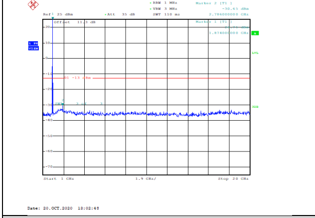
Band2-15MHz-QPSK-18900-1RB#0-Range2:1000~20000MHz--30.65-PASS
