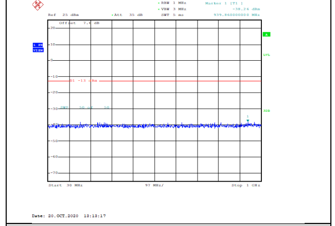
Band4-3MHz-16QAM-19965-1RB#0-Range1:30~1000MHz--38.26-PASS
