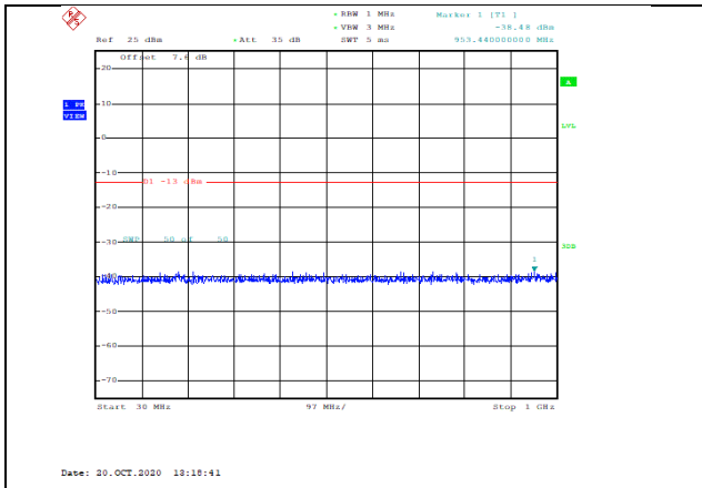
Band4-10MHz-16QAM-20175-1RB#0-Range1:30~1000MHz--38.48-PASS
