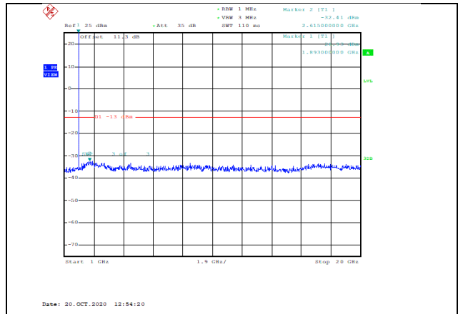
Band2-3MHz-16QAM-19185-1RB#0-Range2:1000~20000MHz--32.41-PASS
