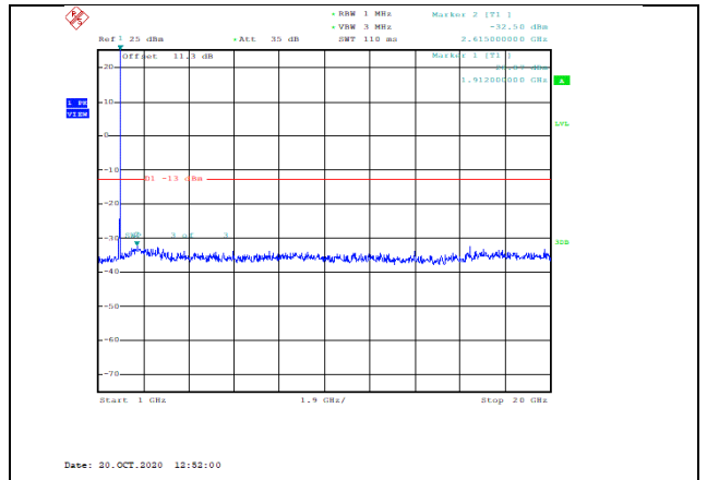
Band2-1.4MHz-16QAM-19193-1RB#0-Range2:1000~20000MHz--32.5-PASS
