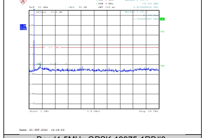
Band4-5MHz-QPSK-19975-1RB#0-Range2:1000~20000MHz--31.68-PASS
