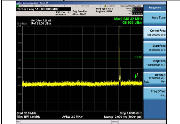
Band26-1.4MHz-QPSK-26740-1RB#0- Range1:30~1000MHz
