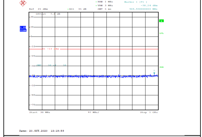
Band4-15MHz-QPSK-20025-1RB#0-Range1:30~1000MHz--38.24-PASS
