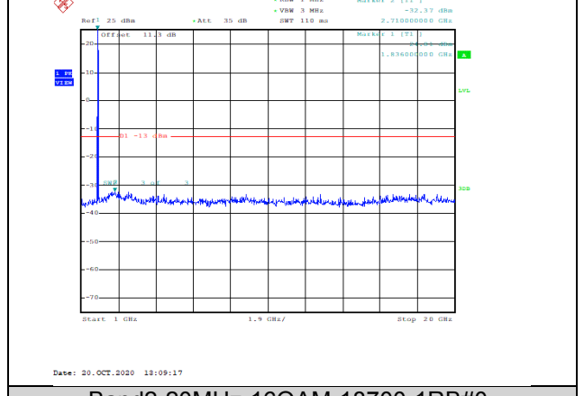
Band2-20MHz-16QAM-18700-1RB#0-Range2:1000~20000MHz--32.37-PASS
