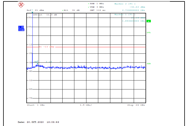
Band2-15MHz-16QAM-19125-1RB#0-Range2:1000~20000MHz--32.02-PASS
