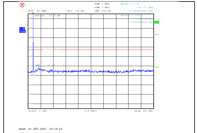
Band4-3MHz-QPSK-20385-1RB#0-Range2:1000~20000MHz--32.55-PASS
