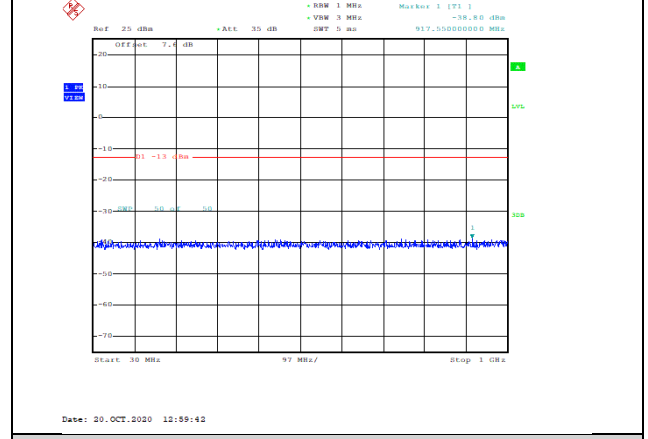
Band2-10MHz-QPSK-18650-1RB#0-Range1:30~1000MHz--38.8-PASS
