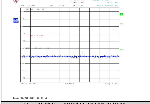
Band2-3MHz-16QAM-19185-1RB#0-Range1:30~1000MHz--38.13-PASS
