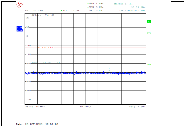
Band2-3MHz-QPSK-18900-1RB#0-Range1:30~1000MHz--38.57-PASS
