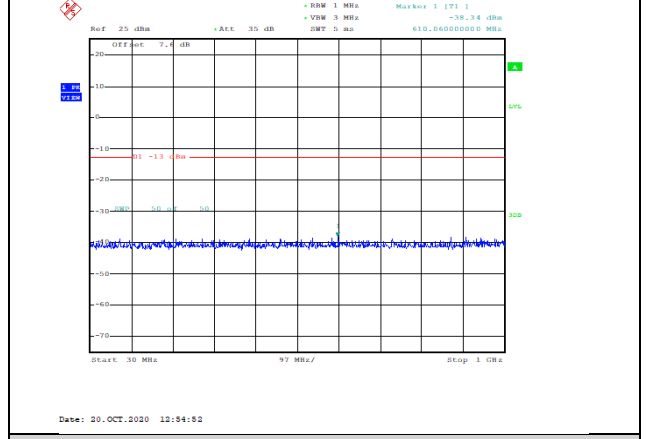
Band2-5MHz-QPSK-18625-1RB#0-Range1:30~1000MHz--38.34-PASS
