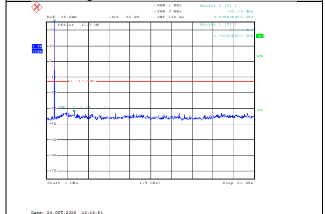
Band4-5MHz-16QAM-19975-1RB#0-Range2:1000~20000MHz--32.56-PASS
