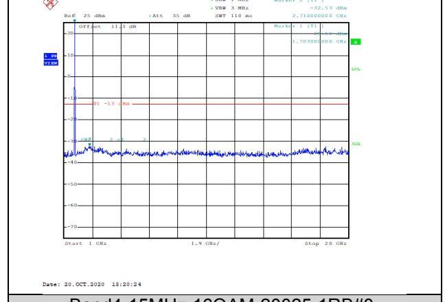
Band4-15MHz-16QAM-20025-1RB#0-Range2:1000~20000MHz--32.53-PASS
