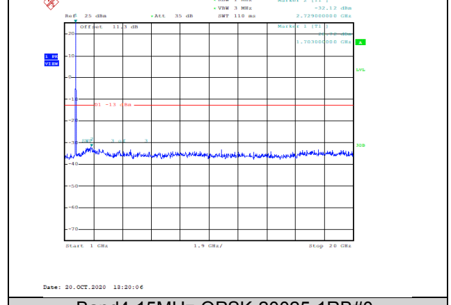
Band4-15MHz-QPSK-20025-1RB#0-Range2:1000~20000MHz--32.12-PASS
