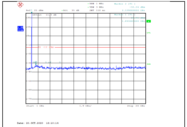
Band2-20MHz-QPSK-19100-1RB#0-Range2:1000~20000MHz--32.26-PASS
