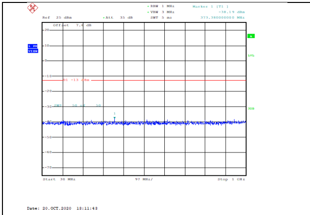
Band4-1.4MHz-16QAM-20175-1RB#0-Range1:30~1000MHz--38.19-PASS
