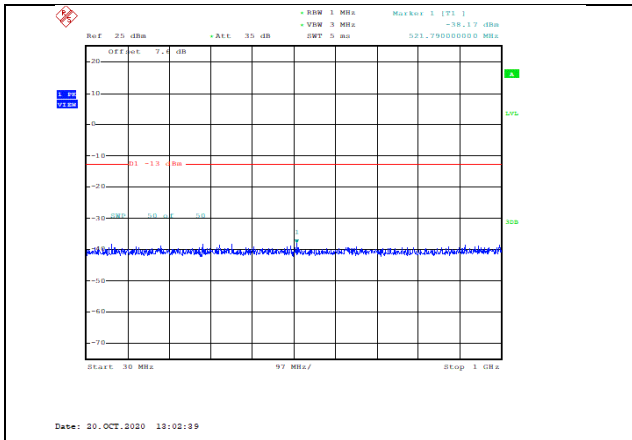
Band2-15MHz-QPSK-18900-1RB#0-Range1:30~1000MHz--38.17-PASS
