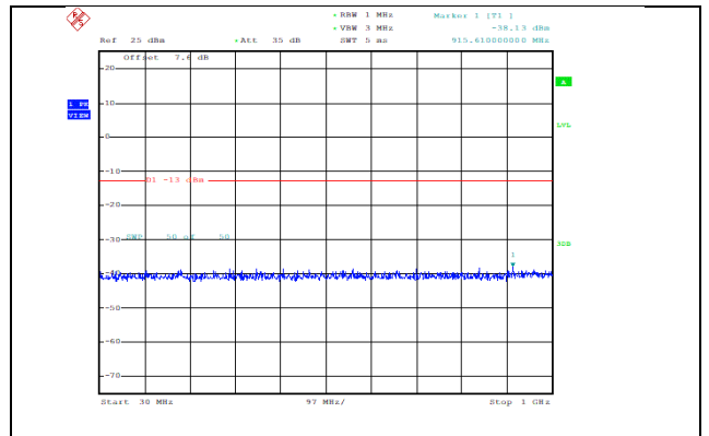
Band2-1.4MHz-QPSK-18607-1RB#0- Range1:30~1000MHz--38.13-PASS
