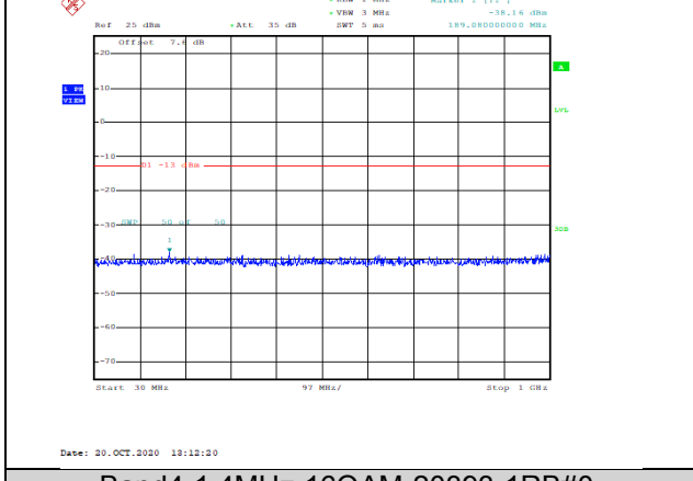
Band4-1.4MHz-16QAM-20393-1RB#0-Range1:30~1000MHz--38.16-PASS
