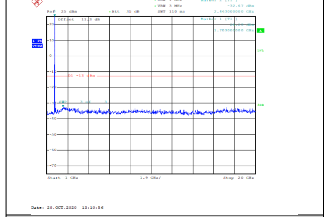
Band4-1.4MHz-QPSK-19957-1RB#0-Range2:1000~20000MHz--32.67-PASS
