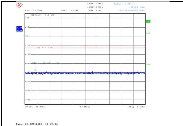
Band2-20MHz-16QAM-18900-1RB#0-Range1:30~1000MHz--38.06-PASS
