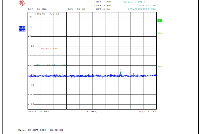
Band2-15MHz-QPSK-18675-1RB#0-Range1:30~1000MHz--37.75-PASS
