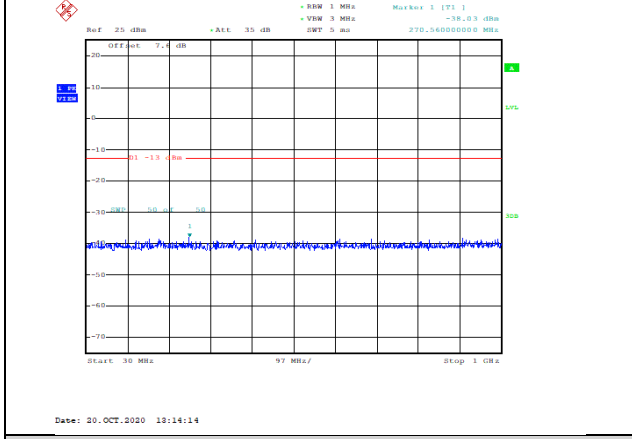
Band4-3MHz-QPSK-20385-1RB#0-Range1:30~1000MHz--38.03-PASS
