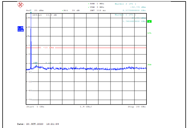
Band4-15MHz-16QAM-20325-1RB#0-Range2:1000~20000MHz--32.79-PASS
