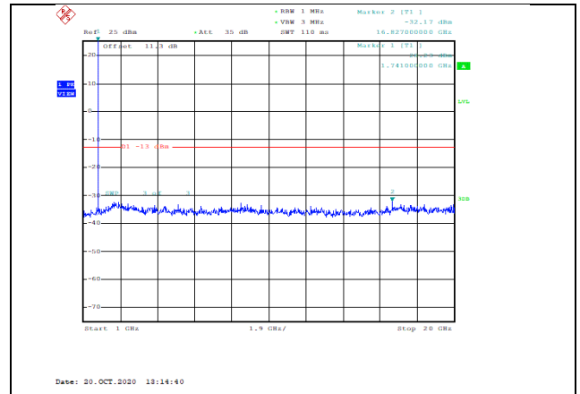
Band4-3MHz-16QAM-20385-1RB#0-Range2:1000~20000MHz--32.17-PASS
