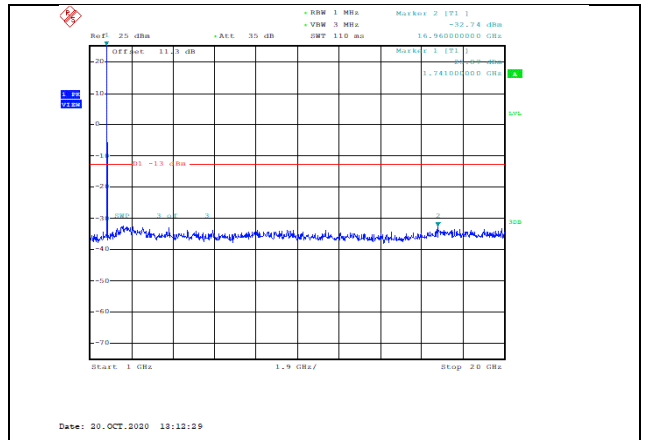
Band4-1.4MHz-16QAM-20393-1RB#0-Range2:1000~20000MHz--32.74-PASS
