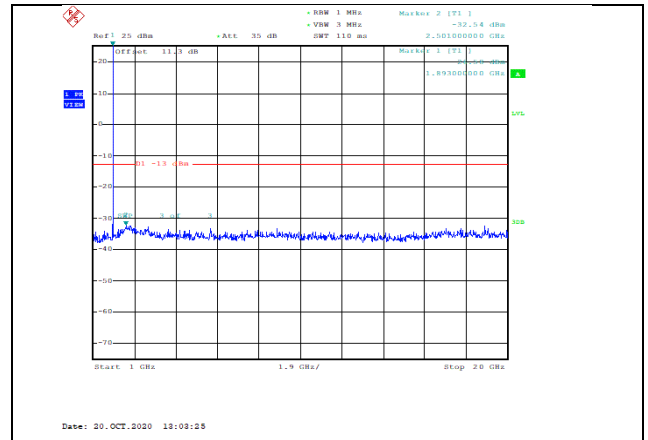
Band2-15MHz-QPSK-19125-1RB#0-Range2:1000~20000MHz--32.54-PASS
