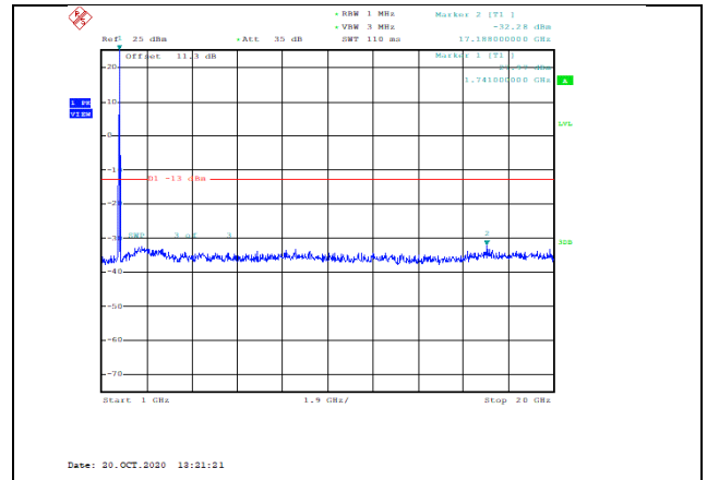
Band4-15MHz-QPSK-20325-1RB#0-Range2:1000~20000MHz--32.28-PASS
