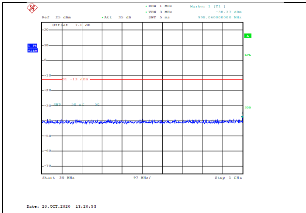
Band4-15MHz-16QAM-20175-1RB#0-Range1:30~1000MHz--38.37-PASS
