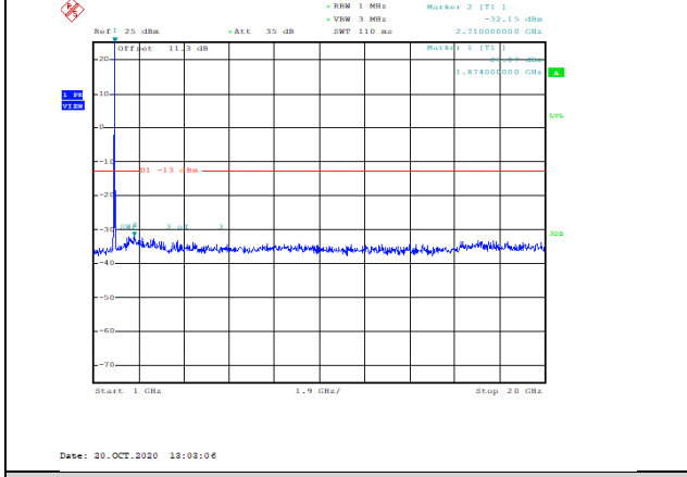
Band2-15MHz-16QAM-18900-1RB#0-Range2:1000~20000MHz--32.15-PASS
