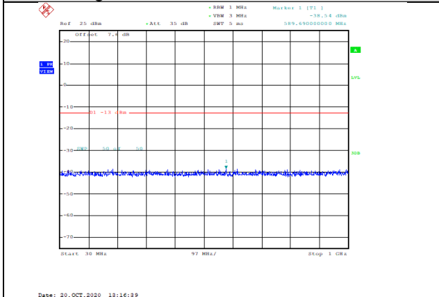
Band4-5MHz-QPSK-20375-1RB#0-Range1:30~1000MHz--38.54-PASS
