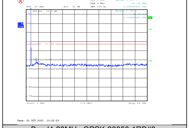
Band4-20MHz-QPSK-20050-1RB#0-Range2:1000~20000MHz--31.98-PASS
