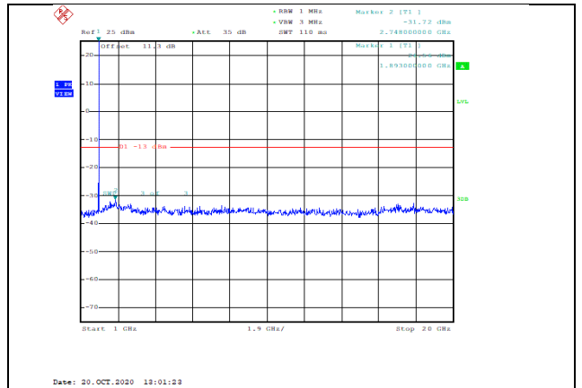
Band2-10MHz-16QAM-19150-1RB#0-Range2:1000~20000MHz--31.72-PASS
