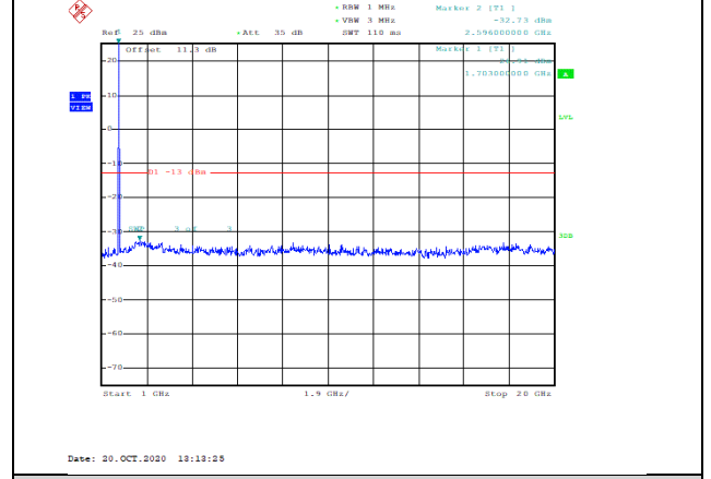
Band4-3MHz-16QAM-19965-1RB#0-Range2:1000~20000MHz--32.73-PASS
