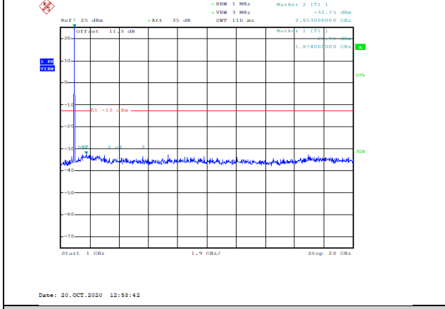
Band2-3MHz-16QAM-18900-1RB#0-Range2:1000~20000MHz--32.75-PASS
