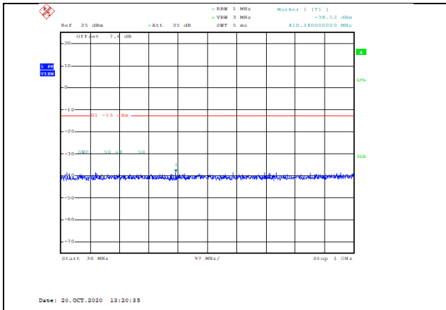
Band4-15MHz-QPSK-20175-1RB#0-Range1:30~1000MHz--38.52-PASS
