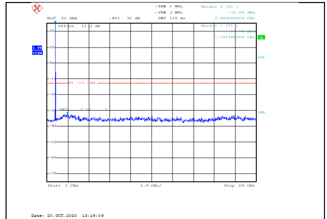
Band4-10MHz-QPSK-20350-1RB#0-Range2:1000~20000MHz--32.38-PASS
