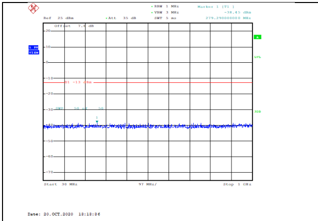
Band4-3MHz-QPSK-20175-1RB#0-Range1:30~1000MHz--38.45-PASS
