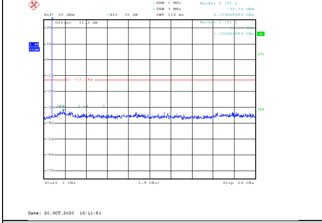
Band4-1.4MHz-16QAM-20175-1RB#0-Range2:1000~20000MHz--32.76-PASS
