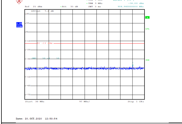
Band2-3MHz-QPSK-19185-1RB#0-Range1:30~1000MHz--38-PASS
