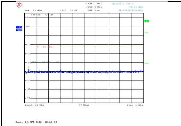
Band2-5MHz-16QAM-18900-1RB#0-Range1:30~1000MHz--38.66-PASS
