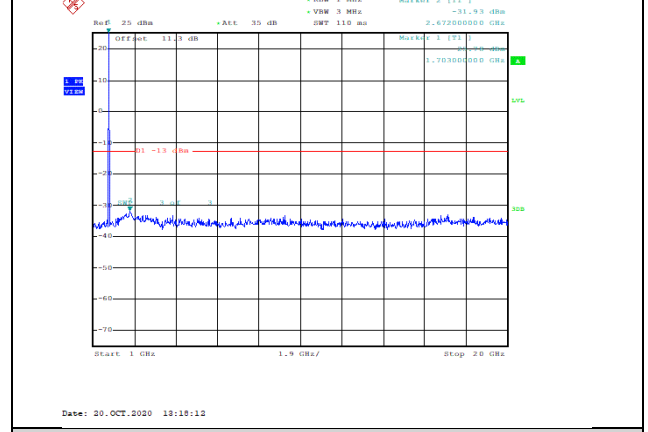
Band4-10MHz-16QAM-20000-1RB#0-Range2:1000~20000MHz--31.93-PASS
