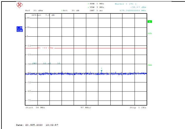
Band2-15MHz-16QAM-18900-1RB#0-Range1:30~1000MHz--38.27-PASS
