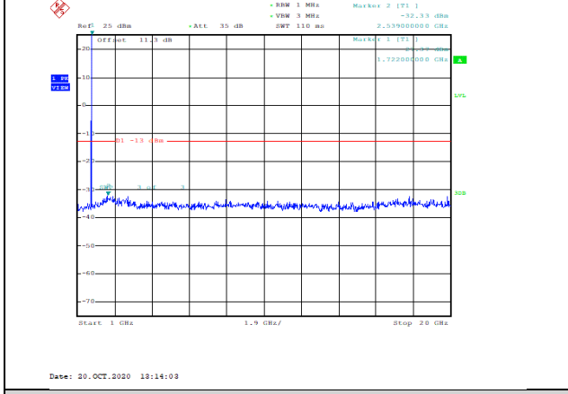
Band4-3MHz-16QAM-20175-1RB#0-Range2:1000~20000MHz--32.33-PASS
