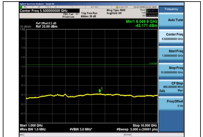
Band26-10MHz-16QAM-26740-1RB#0- Range2:1000~10000MHz
