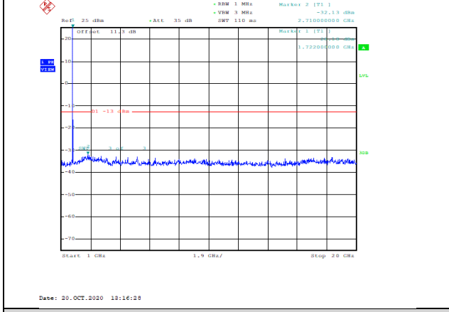
Band4-5MHz-16QAM-20175-1RB#0-Range2:1000~20000MHz--32.13-PASS
