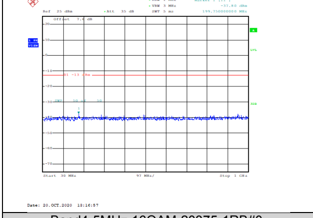
Band4-5MHz-16QAM-20375-1RB#0-Range1:30~1000MHz--37.8-PASS
