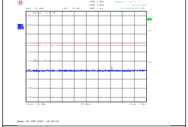
Band2-20MHz-16QAM-18700-1RB#0-Range1:30~1000MHz--38.36-PASS
