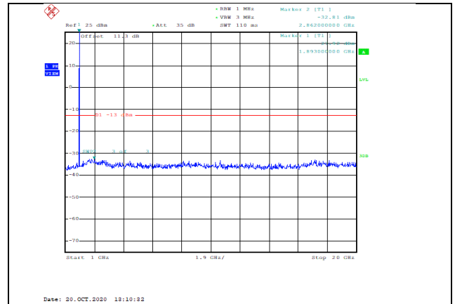
Band2-20MHz-16QAM-19100-1RB#0-Range2:1000~20000MHz--32.81-PASS
