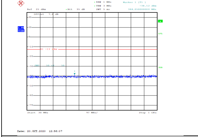
Band2-5MHz-QPSK-19175-1RB#0-Range1:30~1000MHz--38.52-PASS
