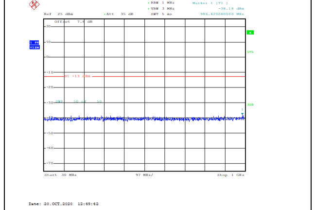
Band2-1.4MHz-16QAM-18607-1RB#0-Range1:30~1000MHz--38.18-PASS
