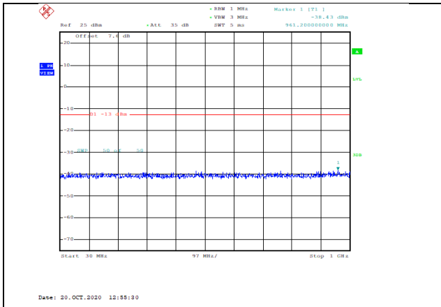
Band2-5MHz-QPSK-18900-1RB#0-Range1:30~1000MHz--38.43-PASS
