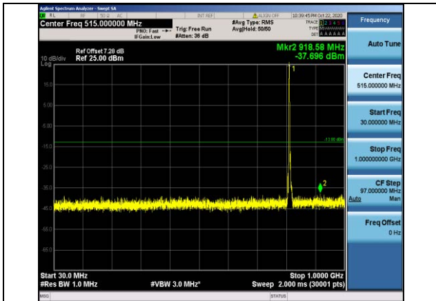
Band26-5MHz-QPSK-26715-1RB#0- Range1:30~1000MHz
