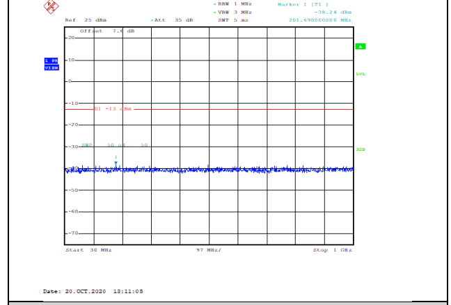
Band4-1.4MHz-16QAM-19957-1RB#0-Range1:30~1000MHz--38.24-PASS
