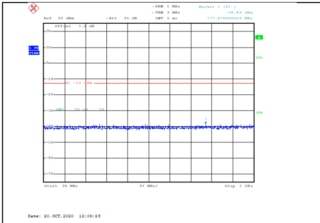
Band2-20MHz-QPSK-18900-1RB#0-Range1:30~1000MHz--38.46-PASS
