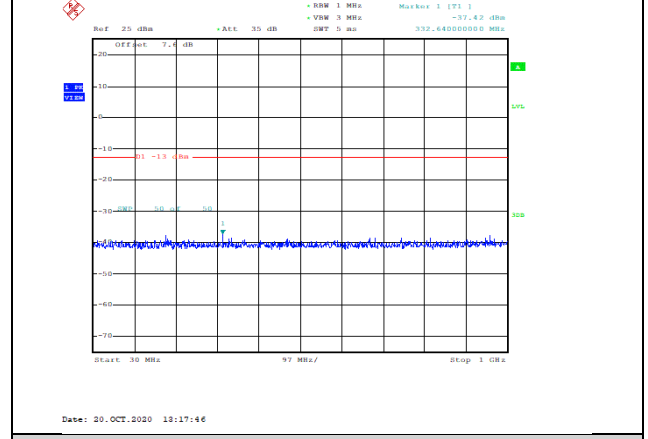
Band4-10MHz-QPSK-20000-1RB#0-Range1:30~1000MHz--37.42-PASS
