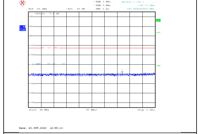
Band2-5MHz-16QAM-18625-1RB#0-Range1:30~1000MHz--38.72-PASS
