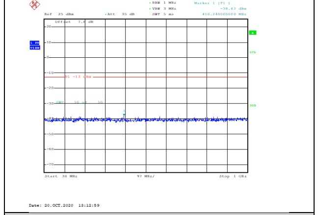
Band4-3MHz-QPSK-19965-1RB#0-Range1:30~1000MHz--38.42-PASS
