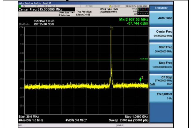
Band17-10MHz-16QAM-23800-1RB#0- Range1:30~1000MHz
