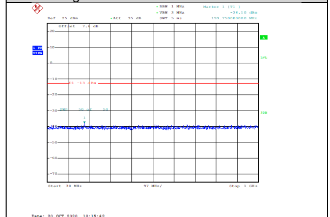
Band4-5MHz-16QAM-19975-1RB#0-Range1:30~1000MHz--38.1-PASS
