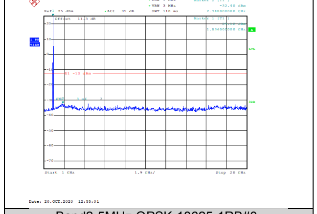
Band2-5MHz-QPSK-18625-1RB#0-Range2:1000~20000MHz--32.4-PASS
