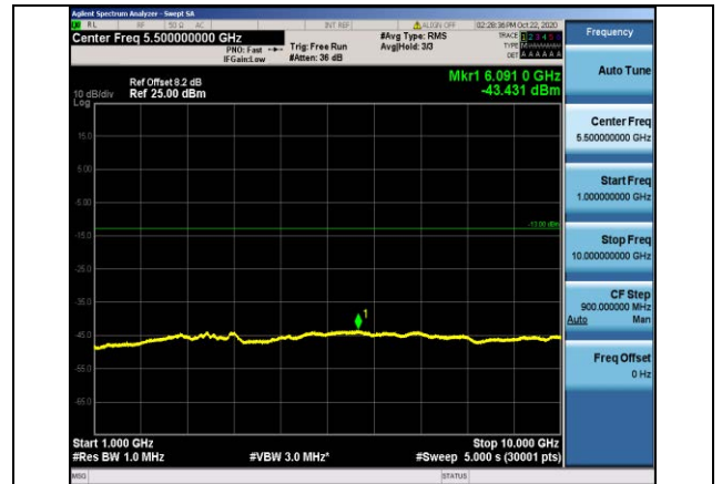
Band26-1.4MHz-16QAM-26740-1RB#0- Range2:1000~10000MHz
