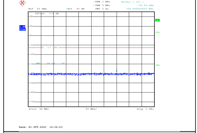
Band2-15MHz-16QAM-18675-1RB#0-Range1:30~1000MHz--38.49-PASS
