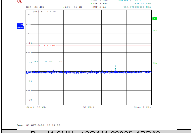
Band4-3MHz-16QAM-20385-1RB#0-Range1:30~1000MHz--38-PASS
