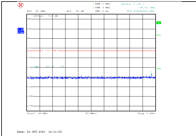
Band4-1.4MHz-QPSK-20175-1RB#0-Range1:30~1000MHz--38.42-PASS
