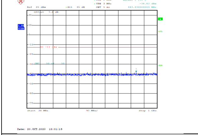
Band2-10MHz-16QAM-19150-1RB#0-Range1:30~1000MHz--38.42-PASS
