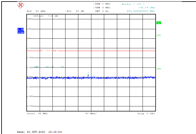
Band4-10MHz-QPSK-20175-1RB#0-Range1:30~1000MHz--38.74-PASS
