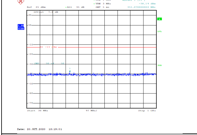
Band4-10MHz-QPSK-20350-1RB#0-Range1:30~1000MHz--38.19-PASS
