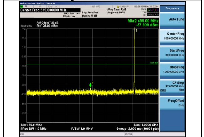
Band26-1.4MHz-QPSK-26783-1RB#0- Range1:30~1000MHz
