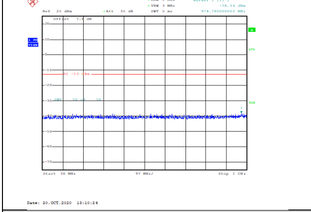
Band2-20MHz-16QAM-19100-1RB#0-Range1:30~1000MHz--38.36-PASS
