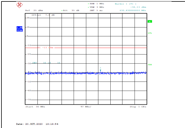
Band4-3MHz-16QAM-20175-1RB#0-Range1:30~1000MHz--38.33-PASS
