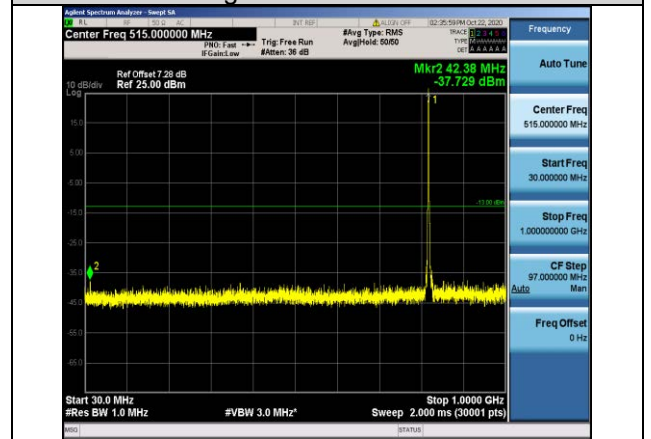
Band26-3MHz-16QAM-26775-1RB#0- Range1:30~1000MHz
