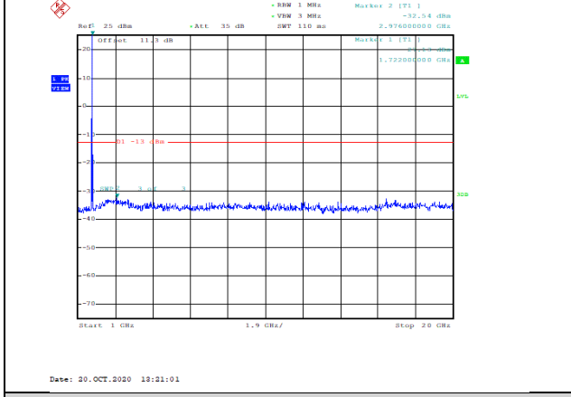
Band4-15MHz-16QAM-20175-1RB#0-Range2:1000~20000MHz--32.54-PASS
