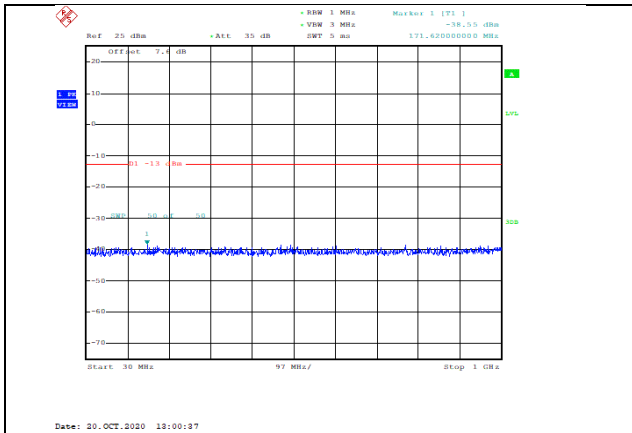
Band2-10MHz-16QAM-18900-1RB#0-Range1:30~1000MHz--38.55-PASS
