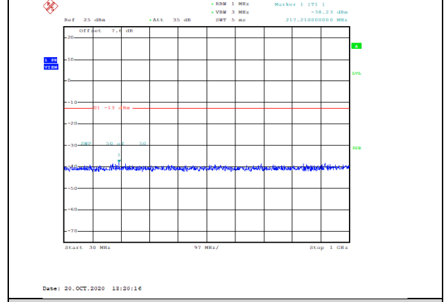
Band4-15MHz-16QAM-20025-1RB#0-Range1:30~1000MHz--38.23-PASS
