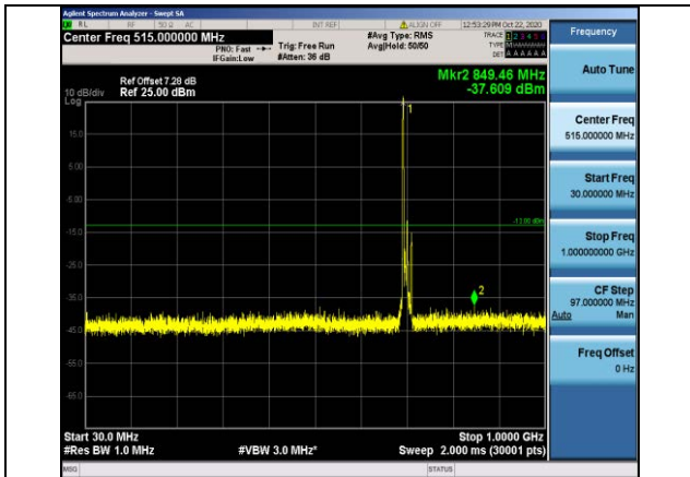
Band12-10MHz-16QAM-23060-1RB#0- Range1:30~1000MHz
