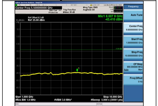
Band12-3MHz-16QAM-23165-1RB#0-Range2:1000~10000MHz
