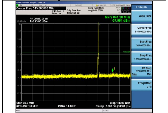
Band12-3MHz-16QAM-23165-1RB#0-Range1:30~1000MHz
