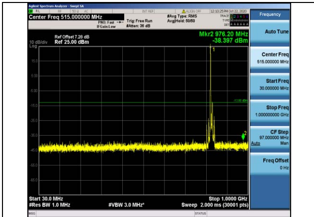
Band5-10MHz-QPSK-20450-1RB#0-Range1:30~1000MHz
