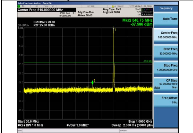
Band12-3MHz-16QAM-23095-1RB#0-Range1:30~1000MHz
