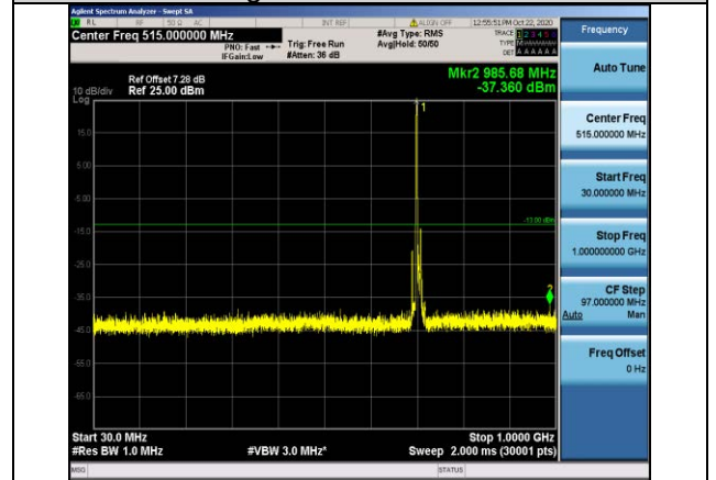
Band12-10MHz-16QAM-23130-1RB#0- Range1:30~1000MHz
