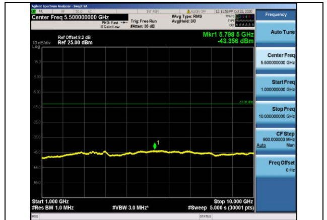
Band5-10MHz-QPSK-20525-1RB#0-Range2:1000~10000MHz
