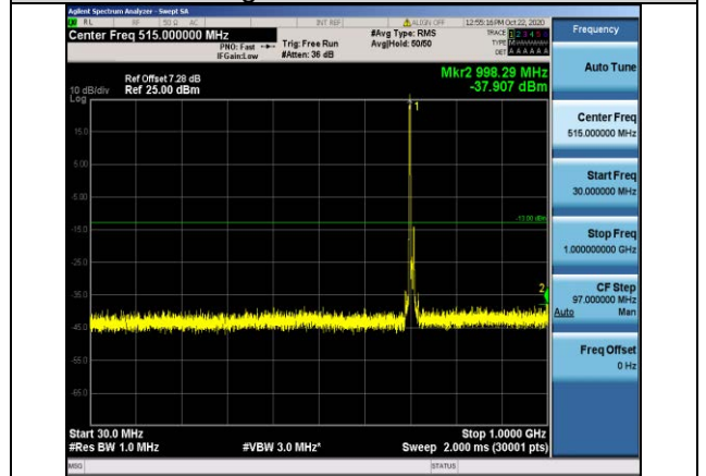
Band12-10MHz-QPSK-23130-1RB#0- Range1:30~1000MHz
