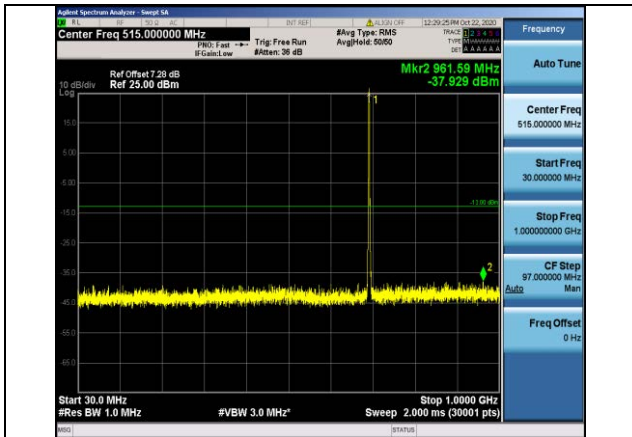
Band12-1.4MHz-16QAM-23017-1RB#0- Range1:30~1000MHz
