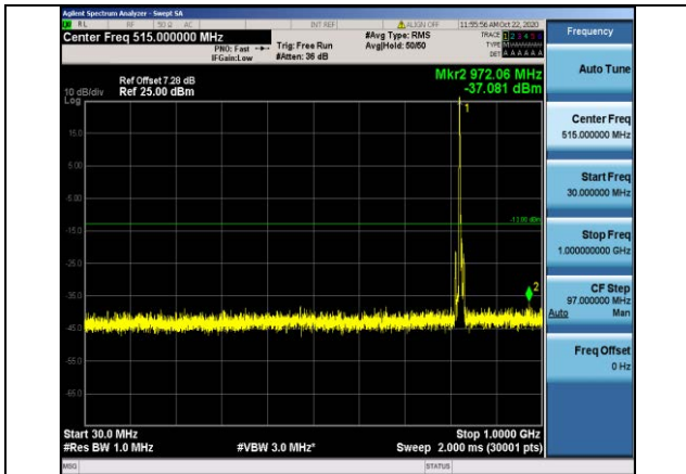
Band5-5MHz-16QAM-20425-1RB#0- Range1:30~1000MHz
