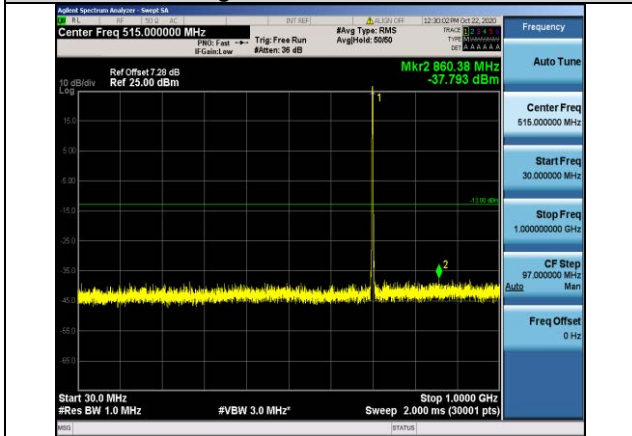
Band12-1.4MHz-QPSK-23095-1RB#0- Range1:30~1000MHz
