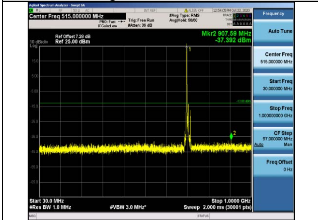
Band12-10MHz-QPSK-23095-1RB#0- Range1:30~1000MHz
