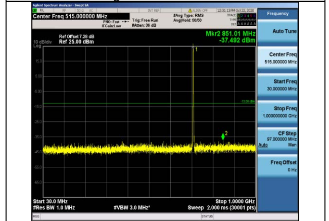
Band12-1.4MHz-QPSK-23173-1RB#0- Range1:30~1000MHz
