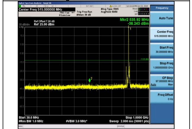
Band5-10MHz-16QAM-20600-1RB#0- Range1:30~1000MHz
