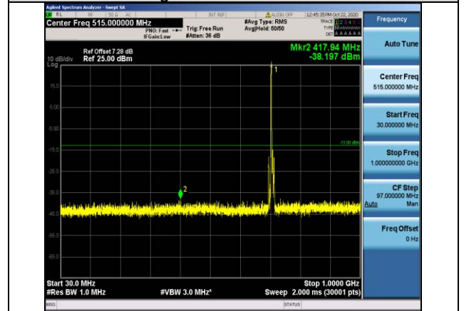
Band12-5MHz-QPSK-23155-1RB#0- Range1:30~1000MHz
