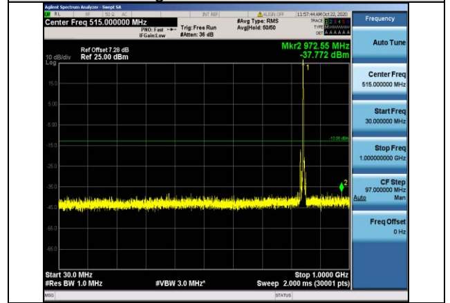
Band5-5MHz-QPSK-20625-1RB#0-Range1:30~1000MHz
