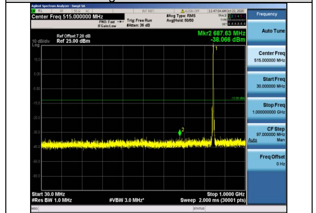
Band5-3MHz-16QAM-20635-1RB#0- Range1:30~1000MHz
