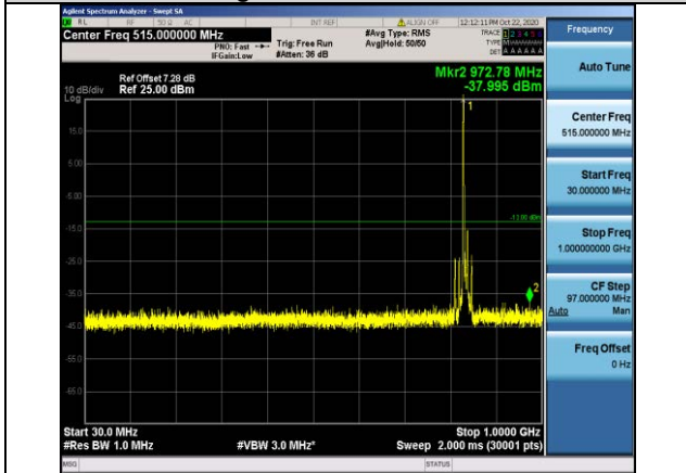
Band5-10MHz-16QAM-20525-1RB#0- Range1:30~1000MHz
