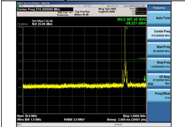
Band5-10MHz-QPSK-20525-1RB#0-Range1:30~1000MHz
