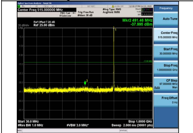
Band12-1.4MHz-16QAM-23095-1RB#0- Range1:30~1000MHz
