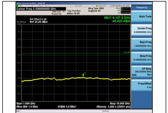
Band5-5MHz-16QAM-20525-1RB#0- Range2:1000~10000MHz
