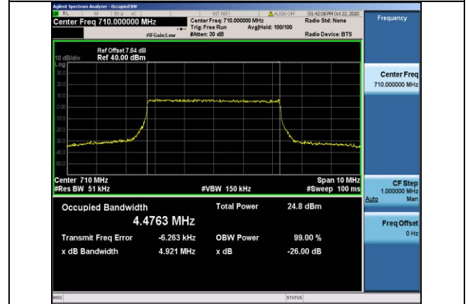
Band17-5MHz-QPSK-23790-25RB#0-4.4763
