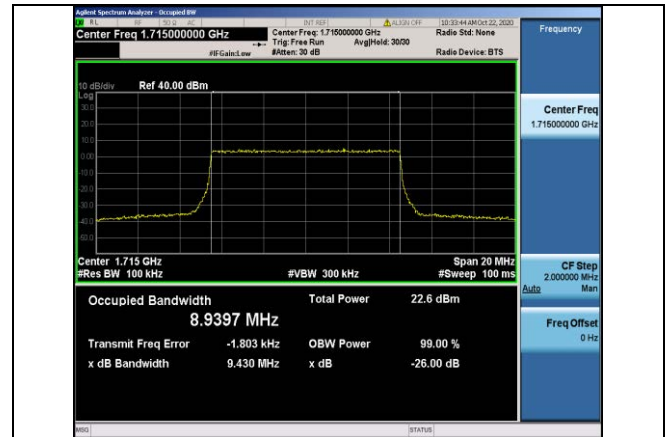
Band4-10MHz-QPSK-20000-50RB#0-8.9397
