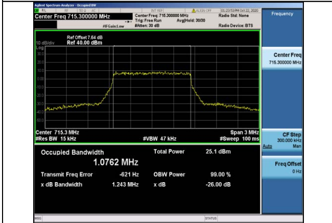
Band12-1.4MHz-16QAM-23173-6RB#0-1.0762
