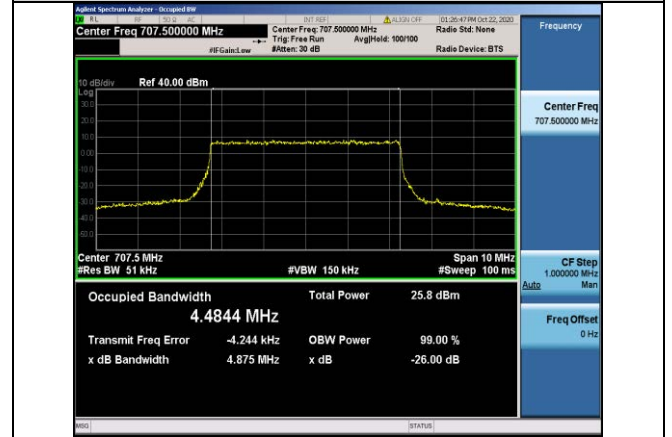
Band12-5MHz-QPSK-23095-25RB#0-4.4844
