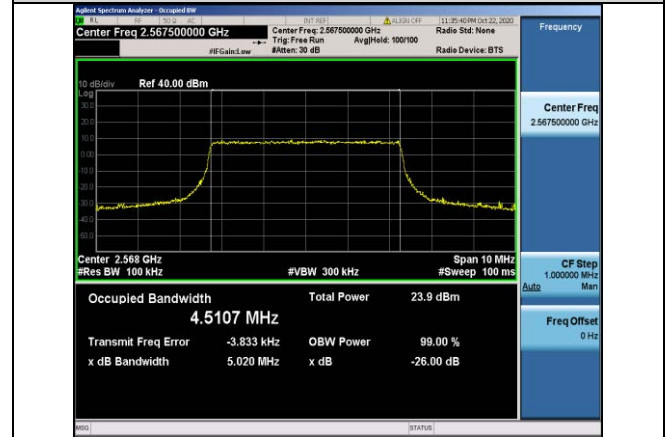
Band7-5MHz-QPSK-21425-25RB#0-4.5107
