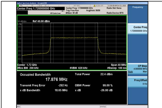
Band4-20MHz-16QAM-20050-100RB#0-17.876
