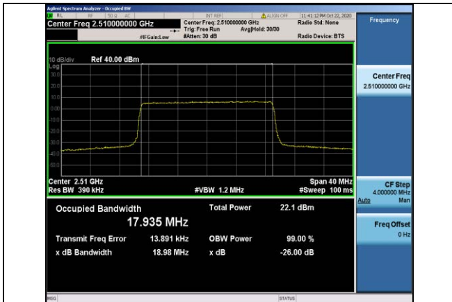
Band7-20MHz-16QAM-20850-100RB#0-17.935
