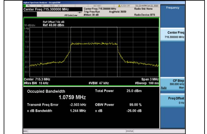
Band12-1.4MHz-QPSK-23173-6RB#0-1.0759
