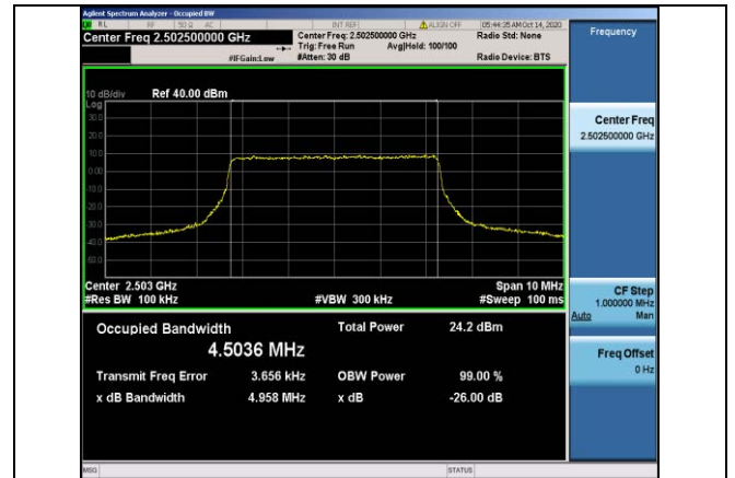
Band7-5MHz-QPSK-20775-25RB#0-4.5036
