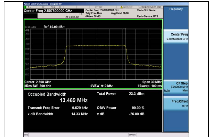
Band7-15MHz-QPSK-20825-75RB#0-13.469
