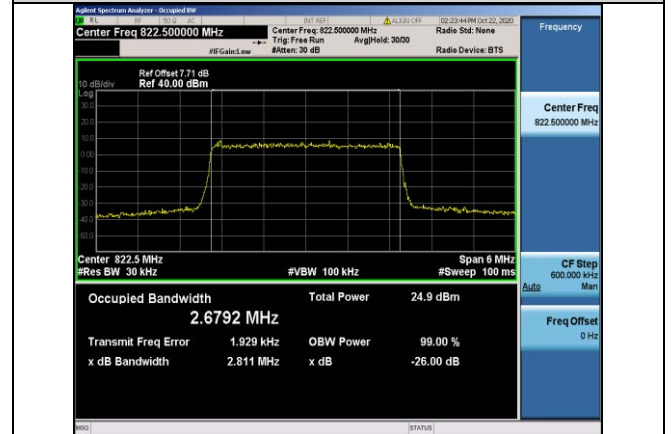
Band26-3MHz-QPSK-26775-15RB#0-2.6792
