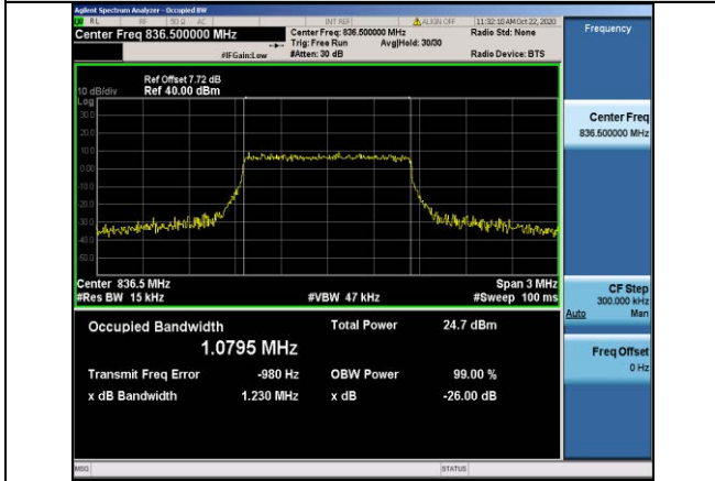
Band5-1.4MHz-16QAM-20525-6RB#0-1.0795
