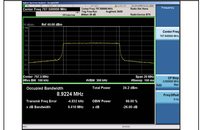
Band12-10MHz-QPSK-23095-50RB#0-8.9224
