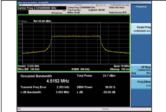
Band7-5MHz-16QAM-21100-25RB#0-4.5152
