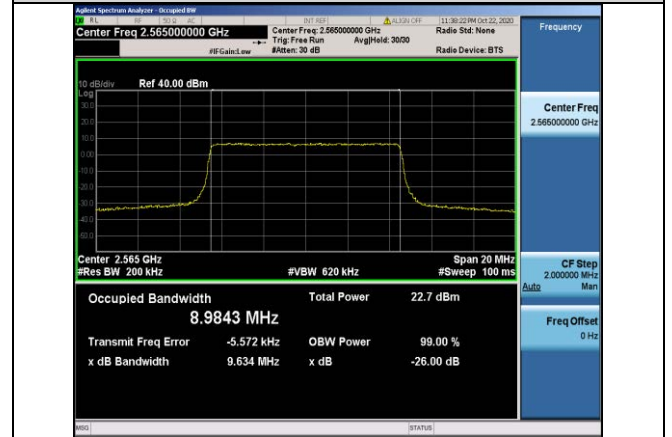
Band7-10MHz-QPSK-21400-50RB#0-8.9843
