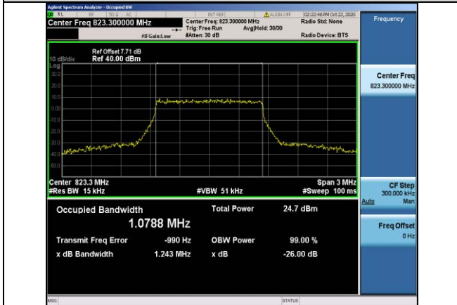
Band26-1.4MHz-16QAM-26783-6RB#0-1.0788
