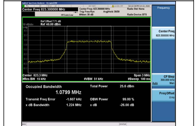
Band26-1.4MHz-QPSK-26783-6RB#0-1.0799
