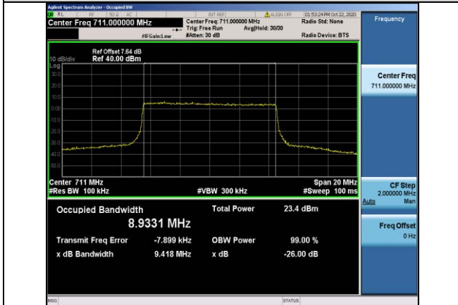
Band17-10MHz-16QAM-23800-50RB#0-8.9331
