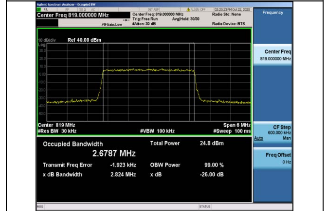
Band26-3MHz-QPSK-26740-15RB#0-2.6787
