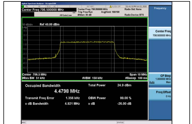
Band17-5MHz-QPSK-23755-25RB#0-4.4798
