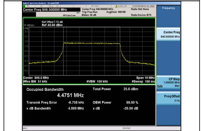
Band5-5MHz-QPSK-20625-25RB#0-4.4751
