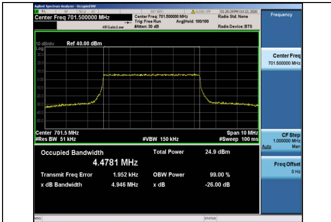
Band12-5MHz-16QAM-23035-25RB#0-4.4781
