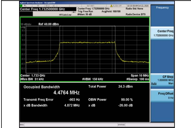
Band4-5MHz-16QAM-20175-25RB#0-4.4764
