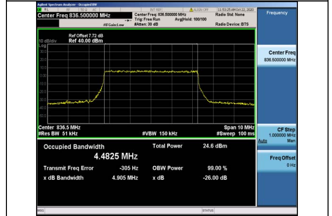
Band5-5MHz-QPSK-20525-25RB#0-4.4825
