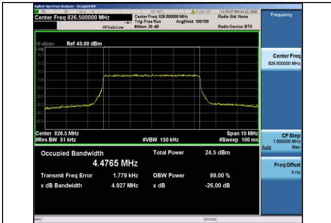
Band5-5MHz-16QAM-20425-25RB#0-4.4765
