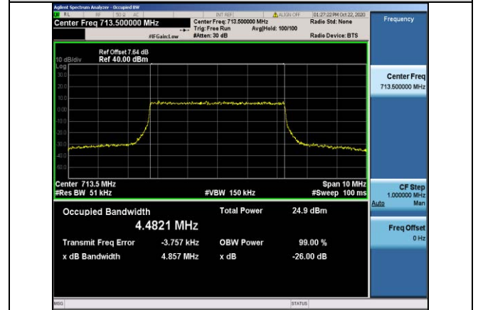
Band12-5MHz-QPSK-23155-25RB#0-4.4821
