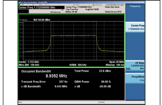
Band4-10MHz-QPSK-20175-50RB#0-8.9352
