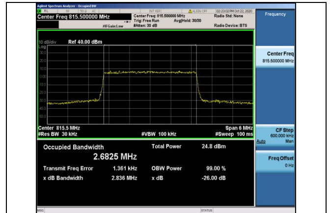
Band26-3MHz-QPSK-26705-15RB#0-2.6825
