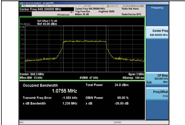
Band5-1.4MHz-16QAM-20643-6RB#0-1.0755
