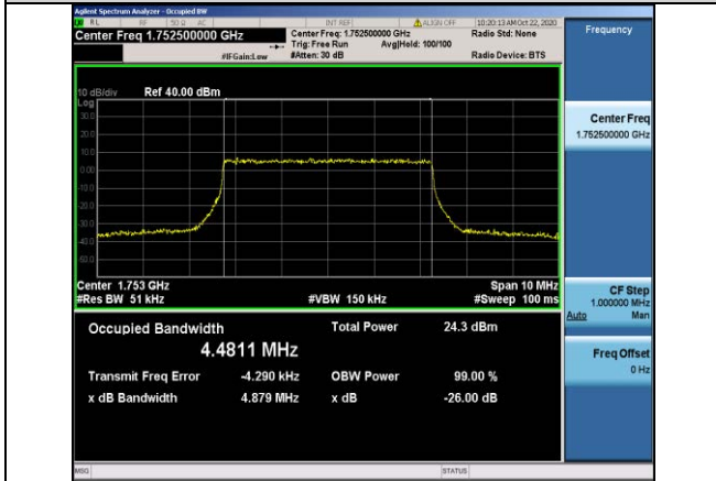
Band4-5MHz-16QAM-20375-25RB#0-4.4811
