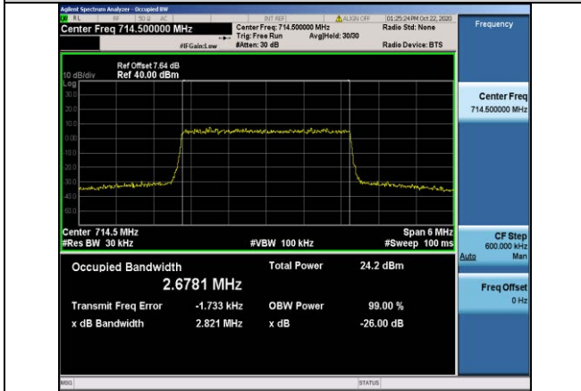
Band12-3MHz-16QAM-23165-15RB#0-2.6781
