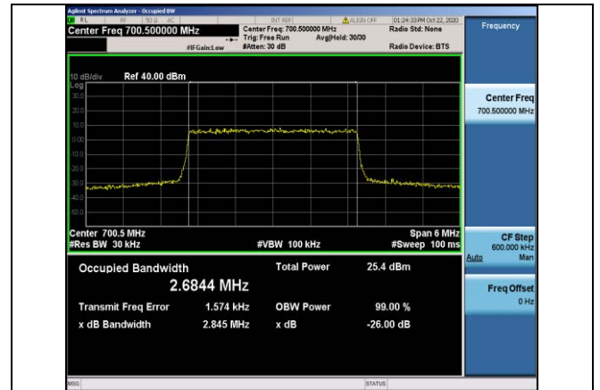
Band12-3MHz-QPSK-23025-15RB#0-2.6844
