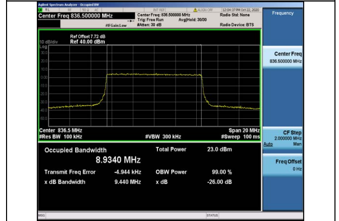
Band5-10MHz-QPSK-20525-50RB#0-8.9340
