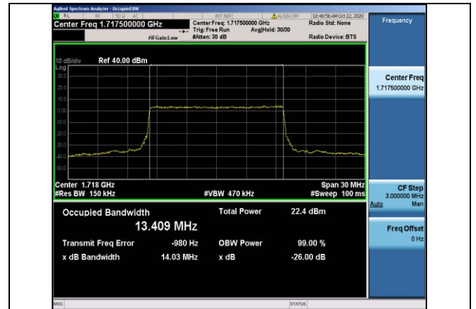
Band4-15MHz-QPSK-20025-75RB#0-13.409
