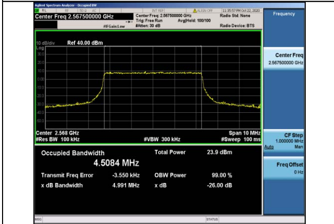
Band7-5MHz-16QAM-21425-25RB#0-4.5084
