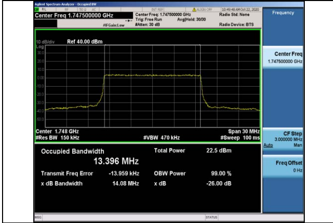
Band4-15MHz-16QAM-20325-75RB#0-13.396
