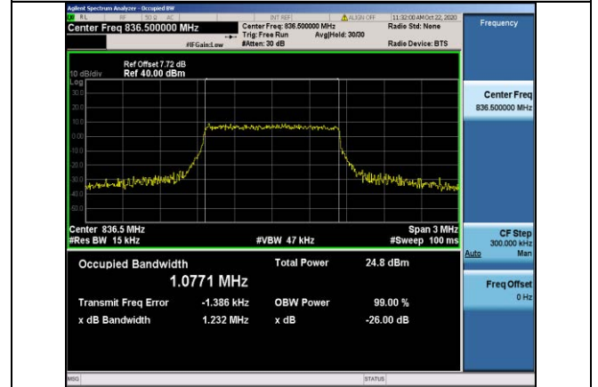
Band5-1.4MHz-QPSK-20525-6RB#0-1.0771
