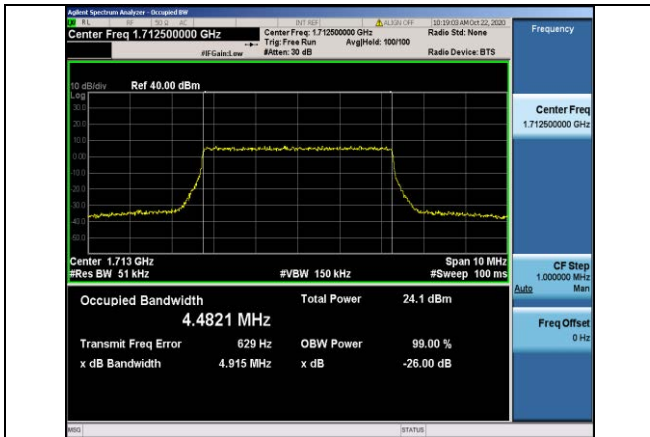
Band4-5MHz-16QAM-19975-25RB#0-4.4821
