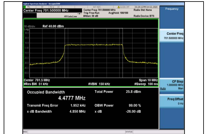
Band12-5MHz-QPSK-23035-25RB#0-4.4777
