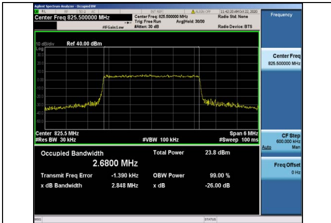
Band5-3MHz-16QAM-20415-15RB#0-2.6800
