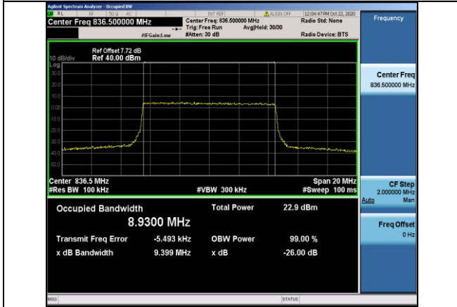
Band5-10MHz-16QAM-20525-50RB#0-8.9300
