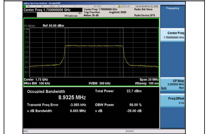
Band4-10MHz-QPSK-20350-50RB#0-8.9325
