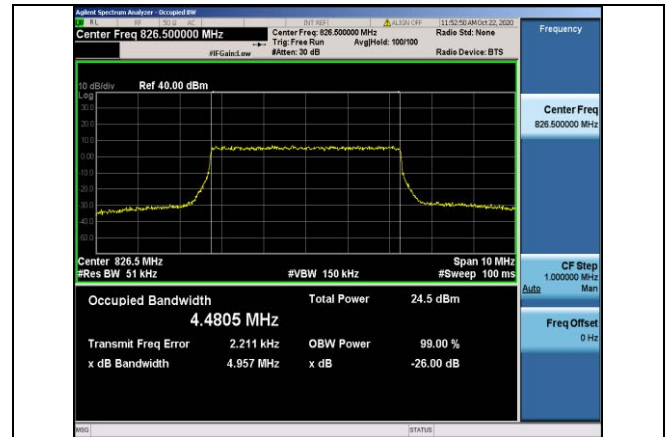
Band5-5MHz-QPSK-20425-25RB#0-4.4805
