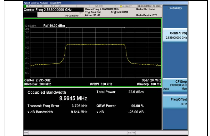
Band7-10MHz-QPSK-21100-50RB#0-8.9945
