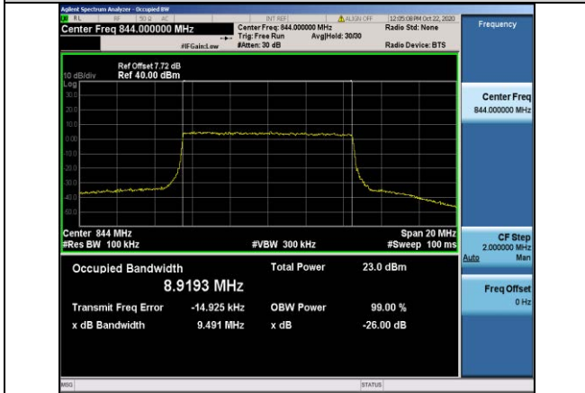
Band5-10MHz-16QAM-20600-50RB#0-8.9193
