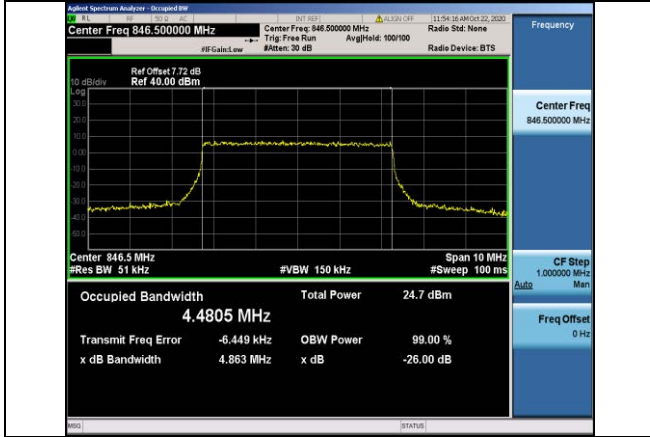
Band5-5MHz-16QAM-20625-25RB#0-4.4805
