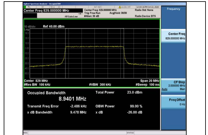
Band5-10MHz-QPSK-20450-50RB#0-8.9401
