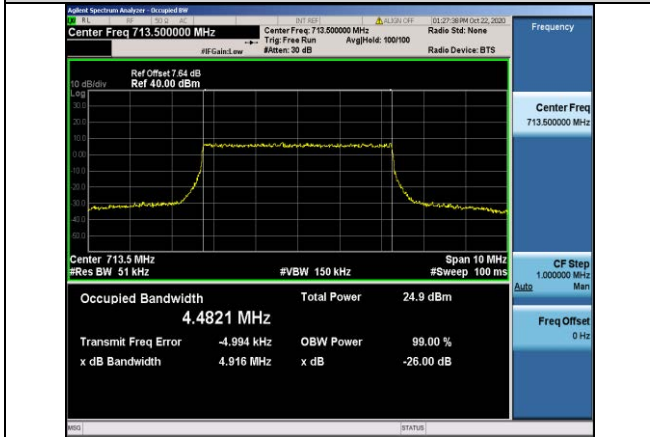
Band12-5MHz-16QAM-23155-25RB#0-4.4821
