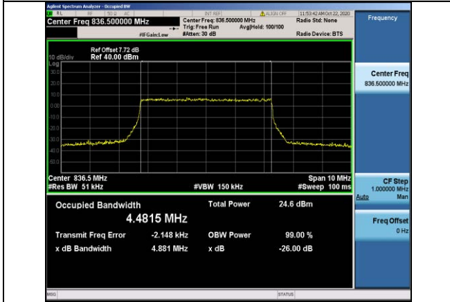
Band5-5MHz-16QAM-20525-25RB#0-4.4815
