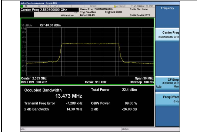
Band7-15MHz-16QAM-21375-75RB#0-13.473
