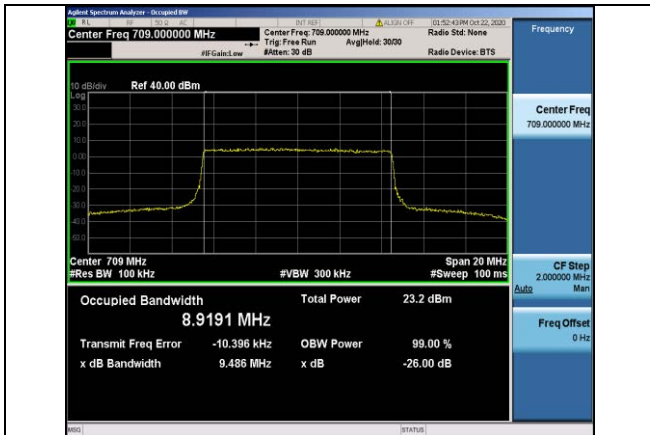
Band17-10MHz-16QAM-23780-50RB#0-8.9191
