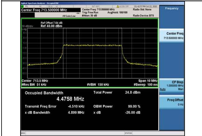
Band17-5MHz-16QAM-23825-25RB#0-4.4758
