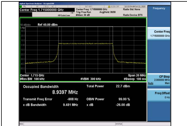
Band4-10MHz-16QAM-20000-50RB#0-8.9397
