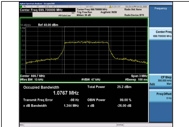
Band12-1.4MHz-16QAM-23017-6RB#0-1.0767
