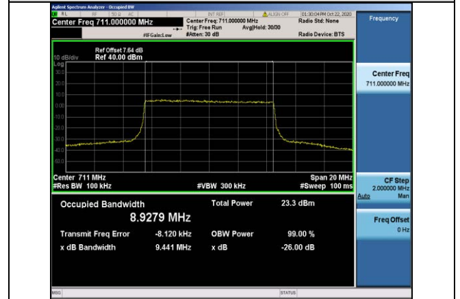
Band12-10MHz-QPSK-23130-50RB#0-8.9279
