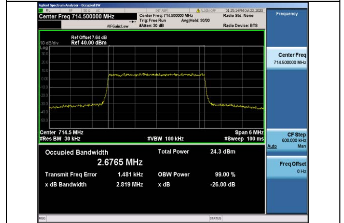
Band12-3MHz-QPSK-23165-15RB#0-2.6765
