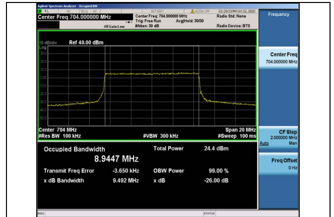
Band12-10MHz-QPSK-23060-50RB#0-8.9447
