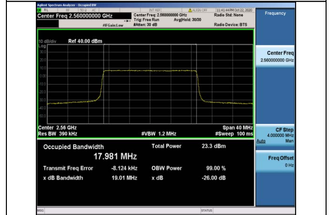
Band7-20MHz-QPSK-21350-100RB#0-17.981
