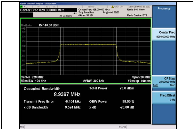
Band5-10MHz-16QAM-20450-50RB#0-8.9397
