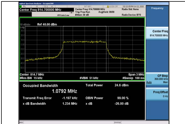
Band26-1.4MHz-16QAM-26697-6RB#0-1.0792
