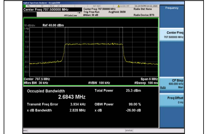
Band12-3MHz-QPSK-23095-15RB#0-2.6843
