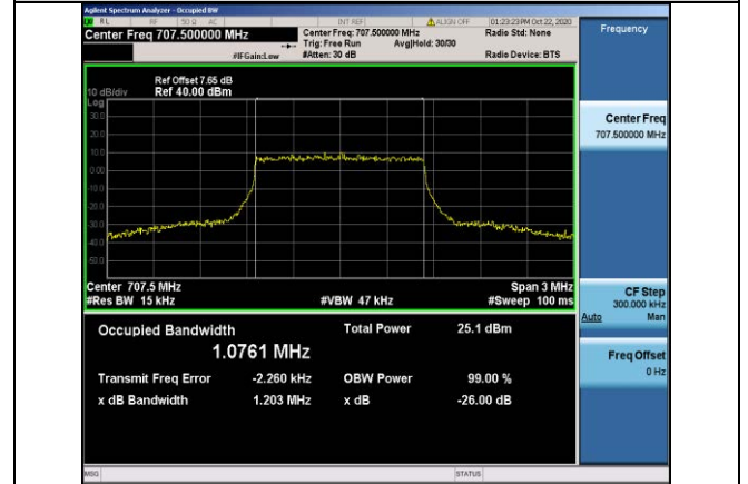
Band12-1.4MHz-QPSK-23095-6RB#0-1.0761
