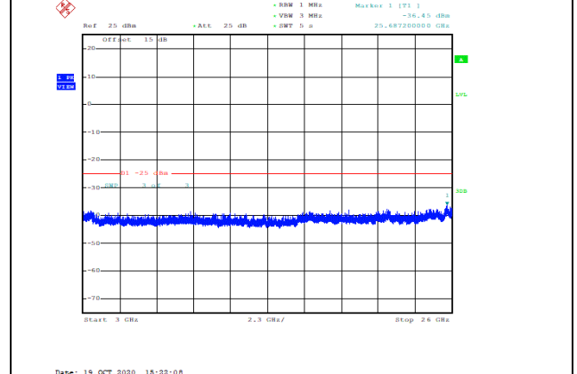
Band38-5MHz-QPSK-38000-1RB#0-Range3:3000~26000MHz--36.45-PASS
