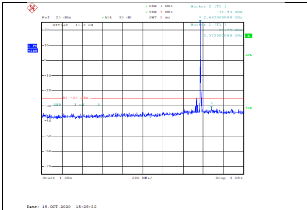
Band38-15MHz-QPSK-37825-1RB#0-Range2:1000~3000MHz--31.93-PASS
