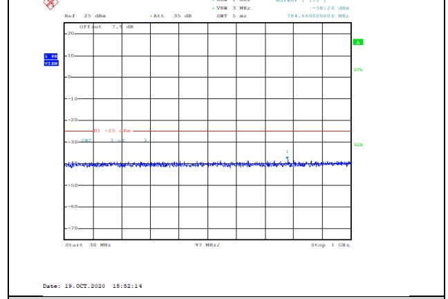
Band41-10MHz-16QAM-40590-1RB#0-Range1:30~1000MHz--38.2-PASS
