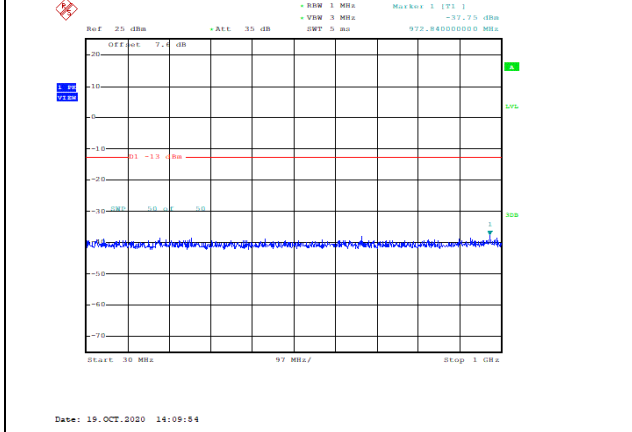
Band66-1.4MHz-QPSK-132322-1RB#0-Range1:30~1000MHz--37.75-PASS
