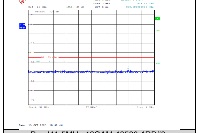
Band41-5MHz-16QAM-40590-1RB#0-Range1:30~1000MHz--38.14-PASS
