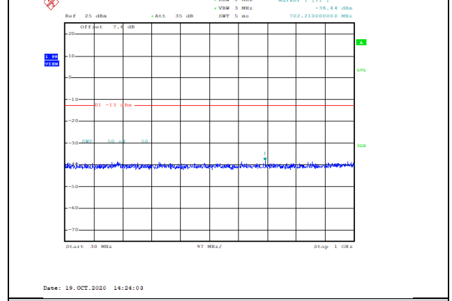
Band66-10MHz-QPSK-132022-1RB#0-Range1:30~1000MHz--38.44-PASS
