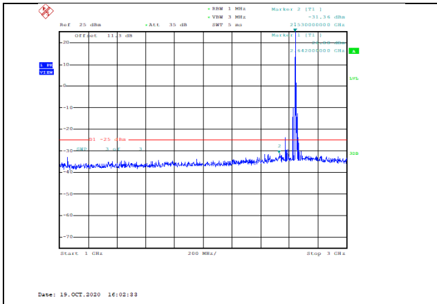
Band41-15MHz-QPSK-41165-1RB#0-Range2:1000~3000MHz--31.36-PASS
