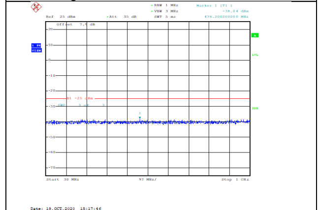
Band7-20MHz-16QAM-21100-1RB#0-Range1:30~1000MHz--38.04-PASS
