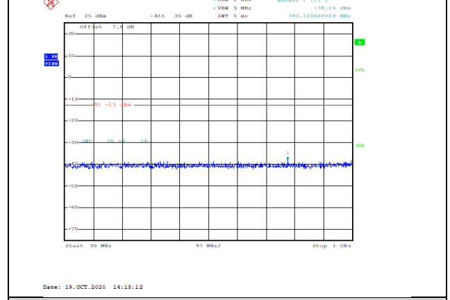
Band66-3MHz-QPSK-131987-1RB#0-Range1:30~1000MHz--38.26-PASS
