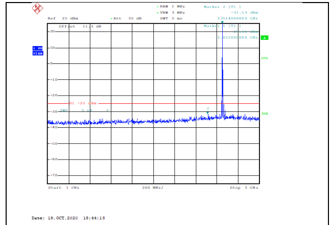
Band41-5MHz-16QAM-41215-1RB#0-Range2:1000~3000MHz--31.53-PASS
