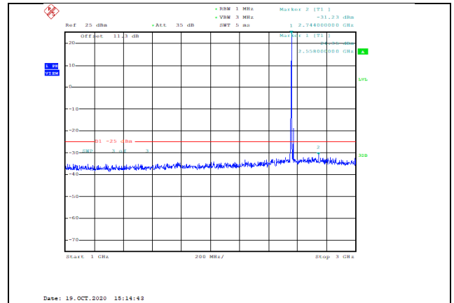
Band7-15MHz-16QAM-21375-1RB#0-Range2:1000~3000MHz--31.23-PASS
