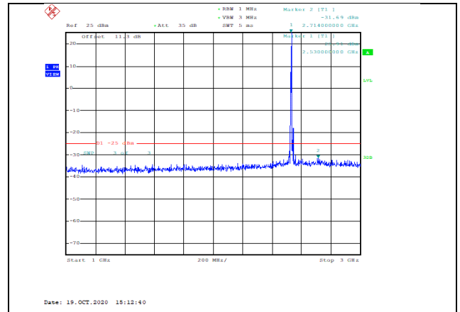
Band7-15MHz-QPSK-21100-1RB#0-Range2:1000~3000MHz--31.69-PASS
