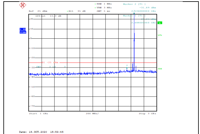
Band41-10MHz-16QAM-41190-1RB#0-Range2:1000~3000MHz--31.49-PASS
