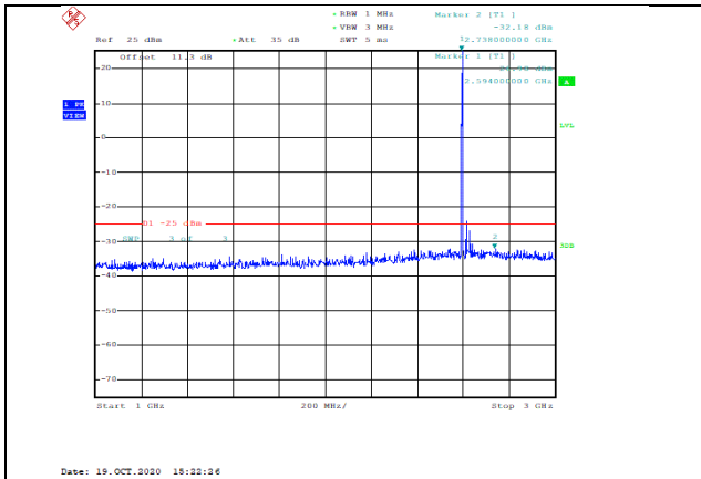
Band38-5MHz-16QAM-38000-1RB#0-Range2:1000~3000MHz--32.18-PASS
