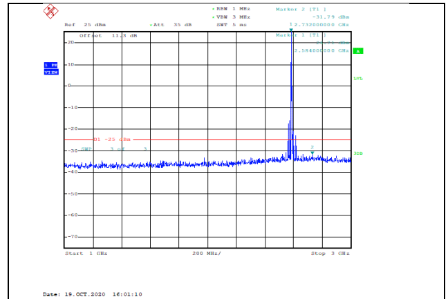
Band41-15MHz-QPSK-40590-1RB#0-Range2:1000~3000MHz--31.79-PASS
