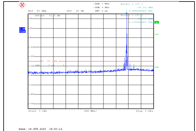
Band38-15MHz-16QAM-37825-1RB#0-Range2:1000~3000MHz--32.28-PASS
