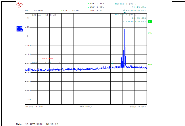
Band41-20MHz-QPSK-41140-1RB#0-Range2:1000~3000MHz--31.45-PASS
