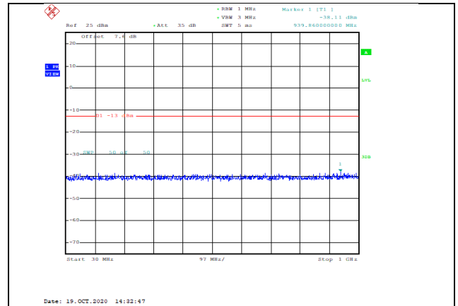
Band66-15MHz-16QAM-132597-1RB#0- Range1:30~1000MHz--38.11-PASS
