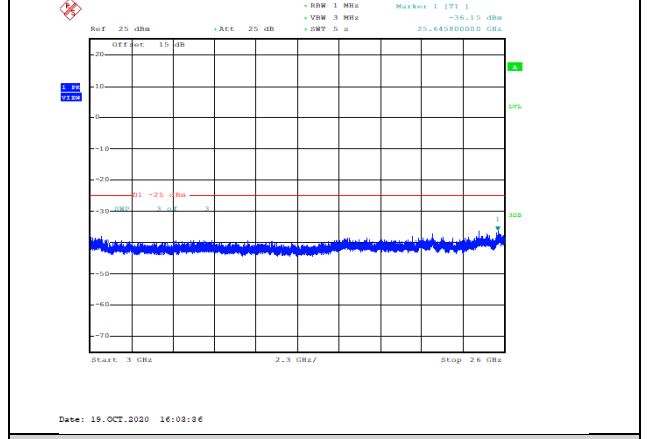
Band41-15MHz-16QAM-41165-1RB#0-Range3:3000~26000MHz--36.15-PASS
