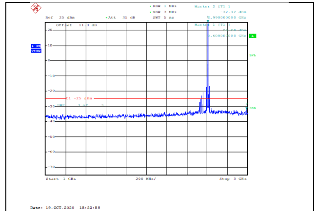
Band38-15MHz-16QAM-38175-1RB#0-Range2:1000~3000MHz--32.32-PASS
