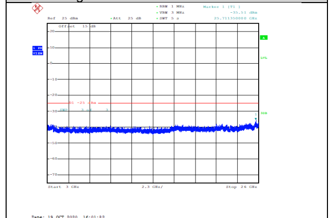
Band41-15MHz-QPSK-40590-1RB#0-Range3:3000~26000MHz--35.51-PASS
