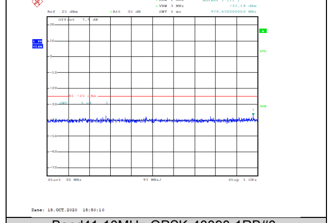
Band41-10MHz-QPSK-40090-1RB#0-Range1:30~1000MHz--37.18-PASS
