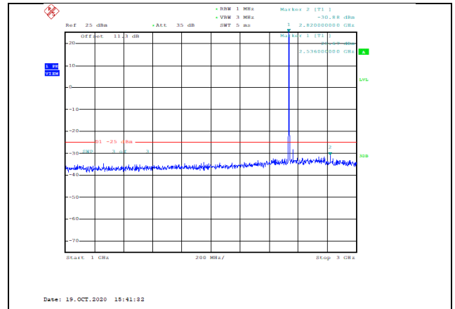
Band41-5MHz-16QAM-40065-1RB#0-Range2:1000~3000MHz--30.88-PASS
