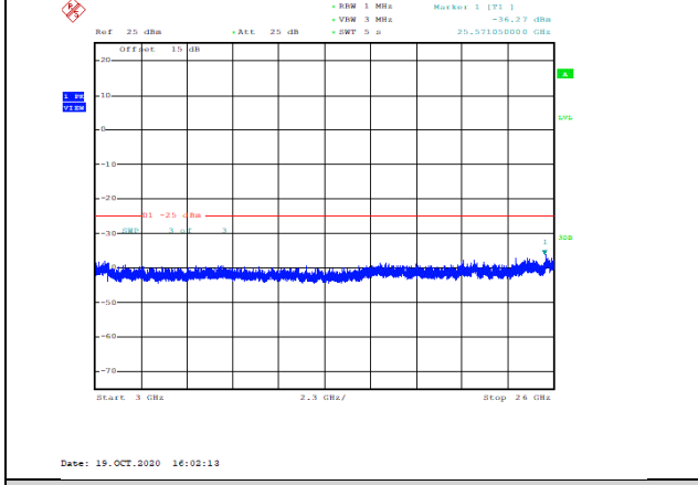
Band41-15MHz-16QAM-40590-1RB#0-Range3:3000~26000MHz--36.27-PASS
