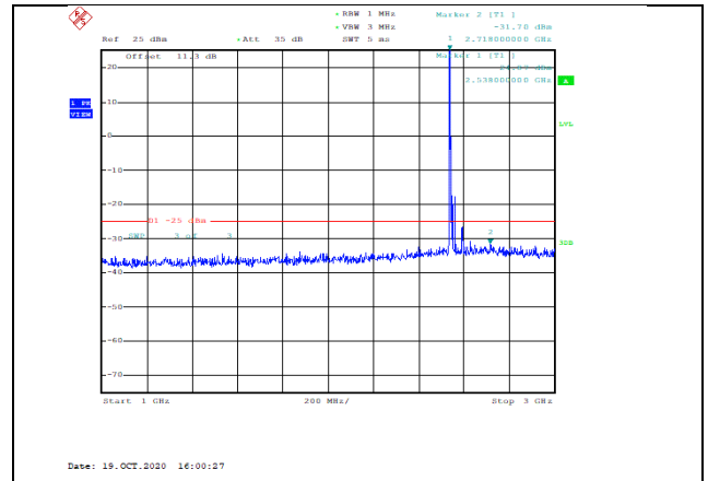
Band41-15MHz-16QAM-40115-1RB#0-Range2:1000~3000MHz--31.70-PASS
