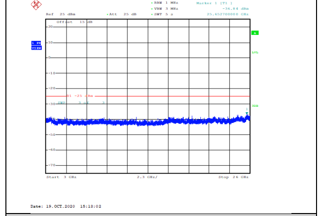
Band7-15MHz-QPSK-21100-1RB#0-Range3:3000~26000MHz--36.84-PASS
