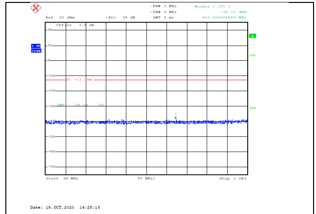
Band66-10MHz-QPSK-132622-1RB#0-Range1:30~1000MHz--38.55-PASS
