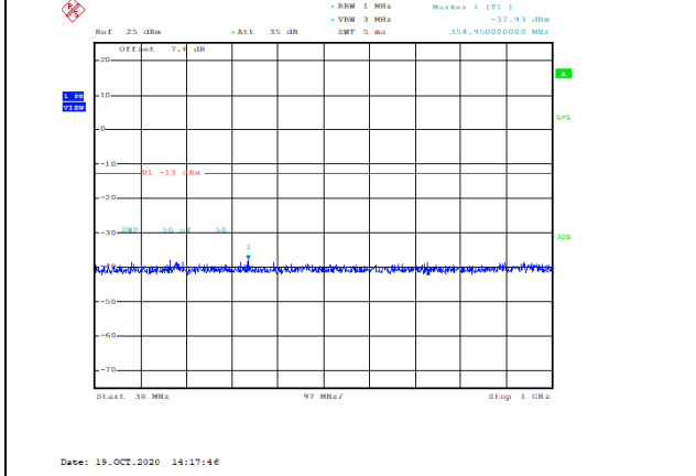
Band66-5MHz-16QAM-132322-1RB#0-Range1:30~1000MHz--37.93-PASS
