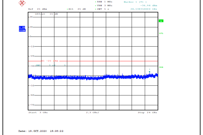
Band38-20MHz-QPSK-38000-1RB#0-Range3:3000~26000MHz--36.94-PASS
