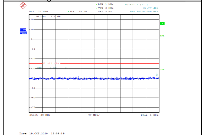
Band41-15MHz-QPSK-40115-1RB#0-Range1:30~1000MHz--37.77-PASS
