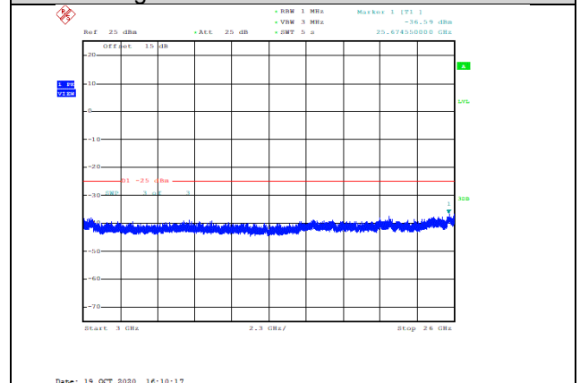
Band41-20MHz-16QAM-40140-1RB#0-Range3:3000~26000MHz--36.59-PASS
