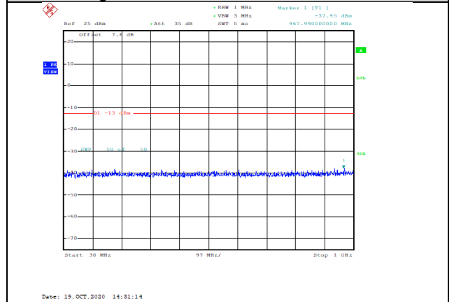
Band66-15MHz-QPSK-132047-1RB#0-Range1:30~1000MHz--37.95-PASS
