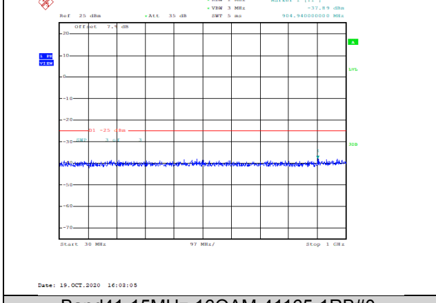
Band41-15MHz-16QAM-41165-1RB#0-Range1:30~1000MHz--37.89-PASS
