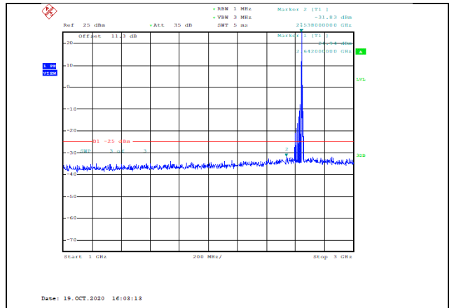
Band41-15MHz-16QAM-41165-1RB#0-Range2:1000~3000MHz--31.83-PASS
