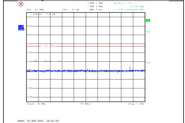
Band66-15MHz-16QAM-132047-1RB#0-Range1:30~1000MHz--37.66-PASS
