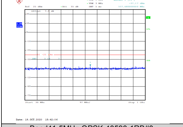
Band41-5MHz-QPSK-40590-1RB#0-Range1:30~1000MHz--37.17-PASS
