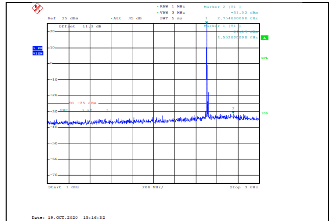
Band7-20MHz-16QAM-20850-1RB#0-Range2:1000~3000MHz--31.52-PASS
