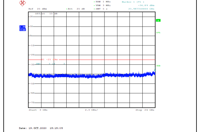
Band7-15MHz-16QAM-21375-1RB#0-Range3:3000~26000MHz--36.89-PASS
