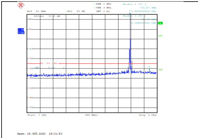
Band41-15MHz-16QAM-40590-1RB#0-Range2:1000~3000MHz--32.07-PASS
