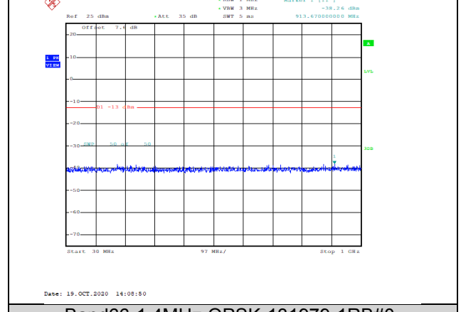
Band66-1.4MHz-QPSK-131979-1RB#0-Range1:30~1000MHz--38.26-PASS
