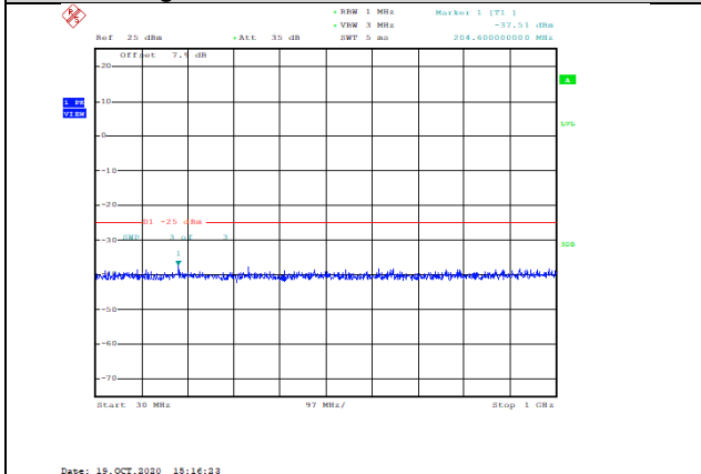
Band7-20MHz-16QAM-20850-1RB#0-Range1:30~1000MHz--37.51-PASS
