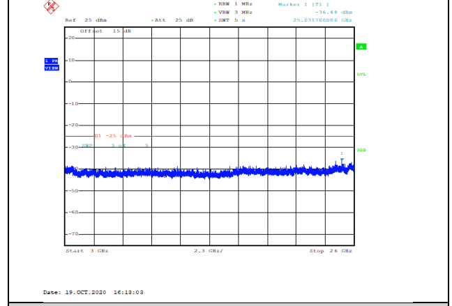
Band41-20MHz-16QAM-41140-1RB#0-Range3:3000~26000MHz--36.48-PASS
