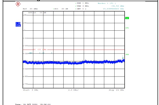
Band38-10MHz-16QAM-37800-1RB#0-Range3:3000~26000MHz--36.9-PASS
