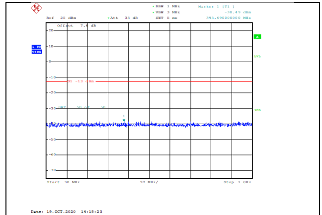
Band66-5MHz-16QAM-132647-1RB#0-Range1:30~1000MHz--38.49-PASS
