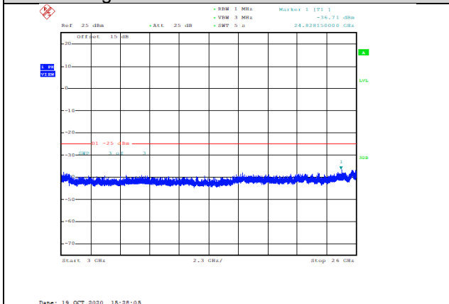
Band38-10MHz-QPSK-38200-1RB#0-Range3:3000~26000MHz--36.71-PASS
