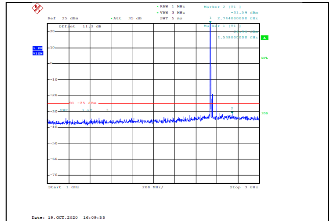
Band41-20MHz-16QAM-40140-1RB#0-Range2:1000~3000MHz--31.59-PASS
