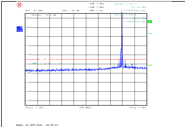
Band38-20MHz-16QAM-38000-1RB#0-Range2:1000~3000MHz--31.58-PASS
