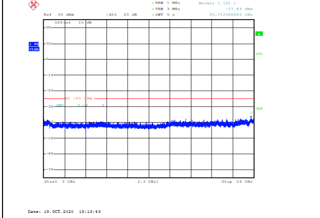
Band7-15MHz-16QAM-21100-1RB#0-Range3:3000~26000MHz--37.49-PASS
