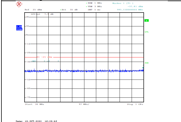
Band41-20MHz-16QAM-40140-1RB#0-Range1:30~1000MHz--37.41-PASS
