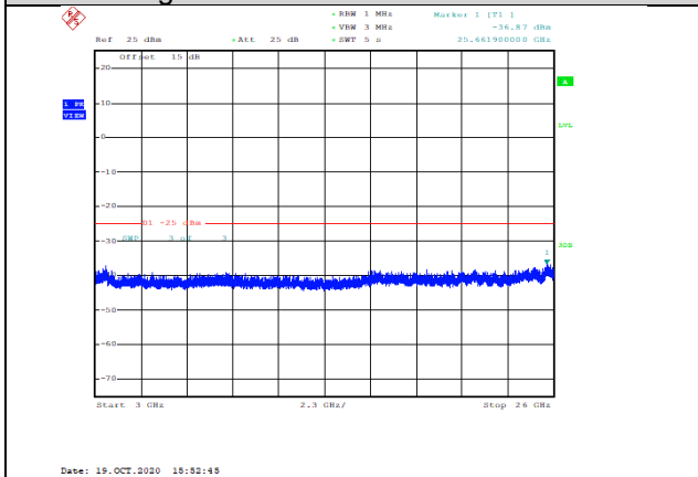
Band41-10MHz-16QAM-40590-1RB#0-Range3:3000~26000MHz--36.87-PASS
