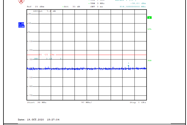
Band38-10MHz-QPSK-38200-1RB#0-Range1:30~1000MHz--38.01-PASS
