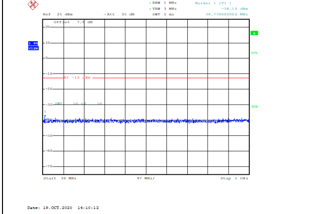
Band66-1.4MHz-16QAM-132322-1RB#0-Range1:30~1000MHz--38.1-PASS
