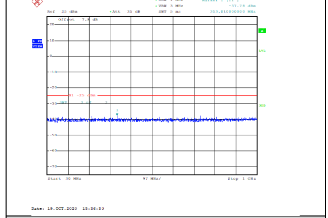
Band38-20MHz-QPSK-37850-1RB#0-Range1:30~1000MHz--37.78-PASS
