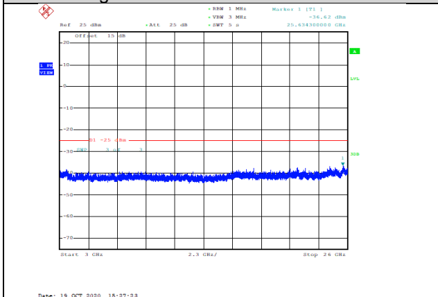
Band38-10MHz-16QAM-38000-1RB#0-Range3:3000~26000MHz--36.62-PASS
