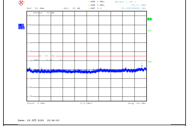
Band41-5MHz-16QAM-41215-1RB#0-Range3:3000~26000MHz--36.71-PASS
