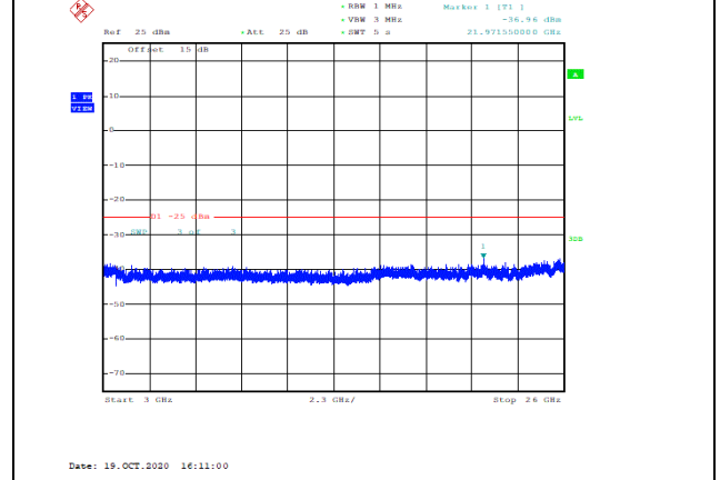
Band41-20MHz-QPSK-40590-1RB#0-Range3:3000~26000MHz--36.96-PASS
