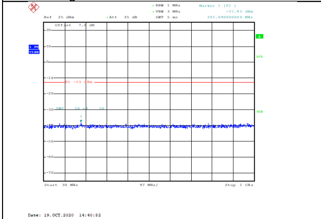
Band66-20MHz-16QAM-132322-1RB#0- Range1:30~1000MHz--37.85-PASS
