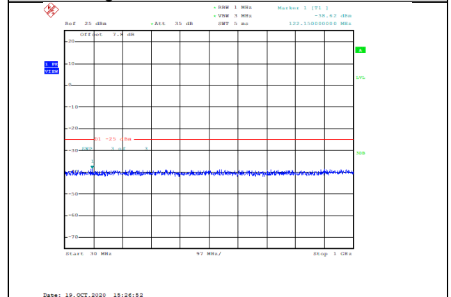
Band38-10MHz-16QAM-38000-1RB#0-Range1:30~1000MHz--38.62-PASS
