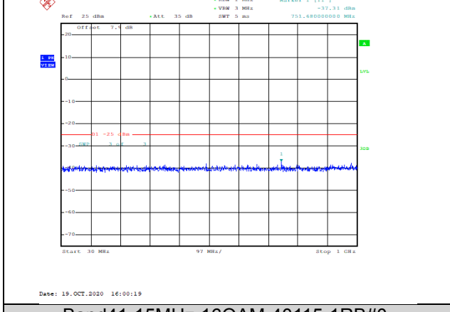
Band41-15MHz-16QAM-40115-1RB#0-Range1:30~1000MHz--37.31-PASS
