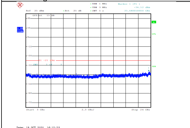
Band41-20MHz-QPSK-41140-1RB#0-Range3:3000~26000MHz--36.52-PASS
