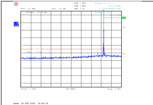
Band41-10MHz-QPSK-41190-1RB#0-Range2:1000~3000MHz--32.33-PASS
