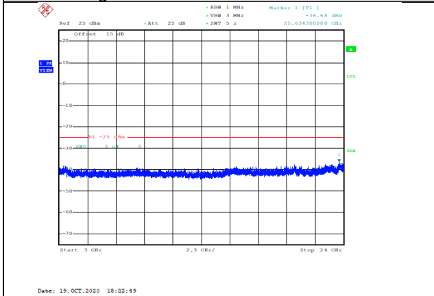
Band38-5MHz-16QAM-38000-1RB#0-Range3:3000~26000MHz--36.68-PASS
