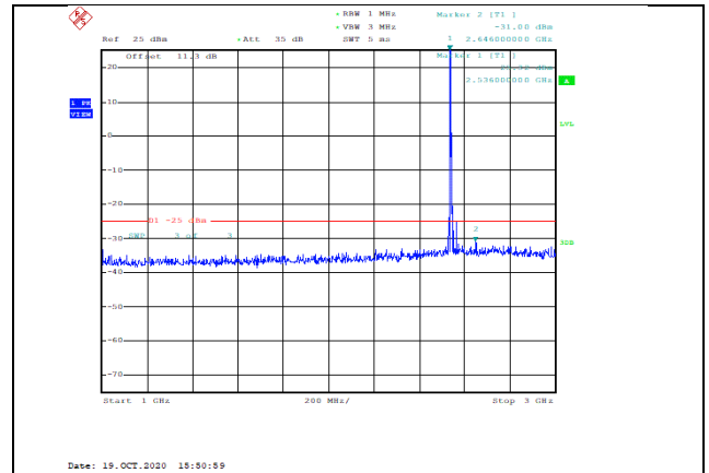
Band41-10MHz-16QAM-40090-1RB#0-Range2:1000~3000MHz--31.68-PASS
