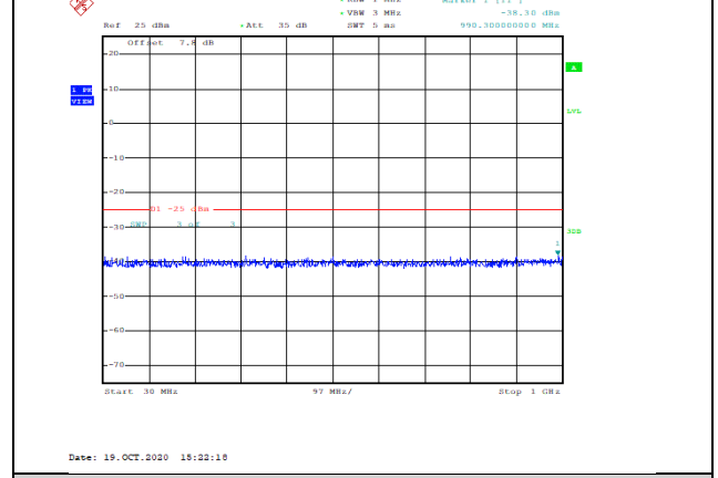
Band38-5MHz-16QAM-38000-1RB#0-Range1:30~1000MHz--38.3-PASS
