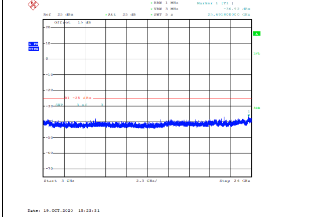
Band38-5MHz-QPSK-38225-1RB#0-Range3:3000~26000MHz--36.92-PASS
