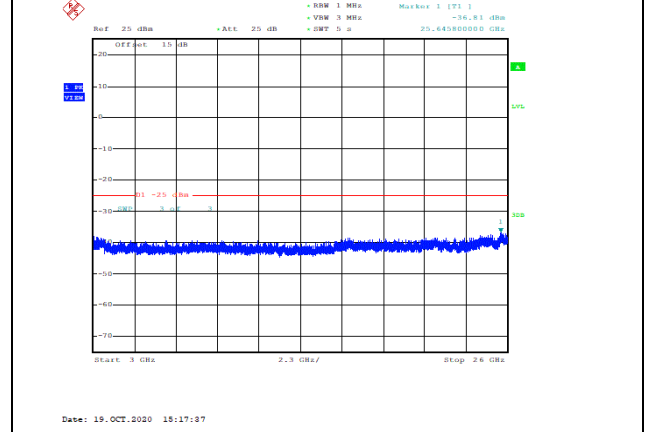
Band7-20MHz-QPSK-21100-1RB#0-Range3:3000~26000MHz--36.81-PASS
