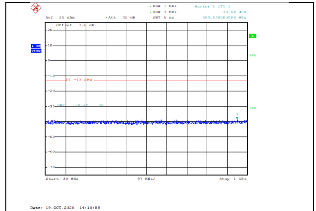
Band66-1.4MHz-QPSK-132665-1RB#0-Range1:30~1000MHz--38.6-PASS
