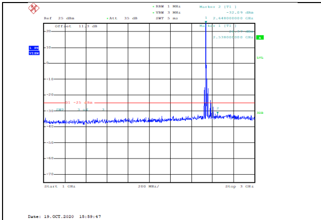
Band41-15MHz-QPSK-40115-1RB#0-Range2:1000~3000MHz--32.09-PASS
