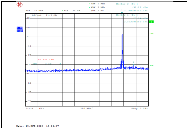
Band38-10MHz-QPSK-37800-1RB#0-Range2:1000~3000MHz--31.22-PASS
