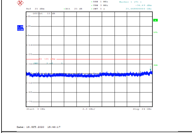
Band41-5MHz-16QAM-40590-1RB#0-Range3:3000~26000MHz--36.69-PASS
