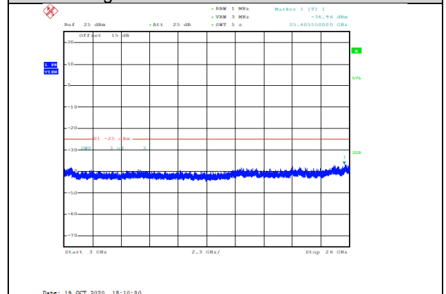
Band7-10MHz-16QAM-21400-1RB#0-Range3:3000~26000MHz--36.96-PASS
