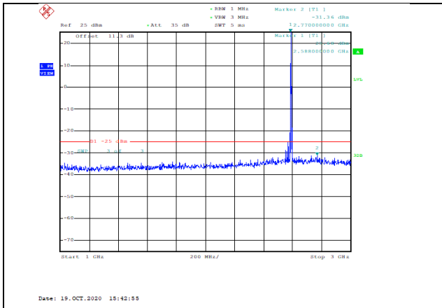
Band41-5MHz-16QAM-40590-1RB#0-Range2:1000~3000MHz--31.36-PASS
