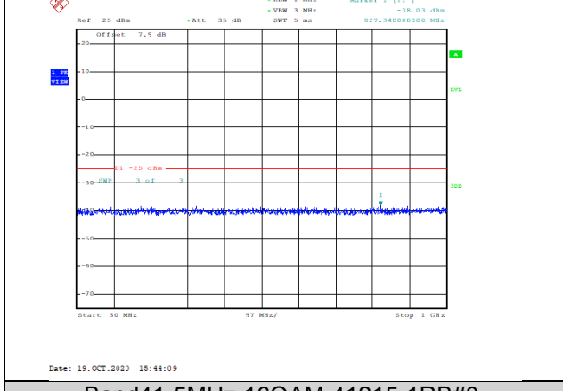
Band41-5MHz-16QAM-41215-1RB#0-Range1:30~1000MHz--38.03-PASS
