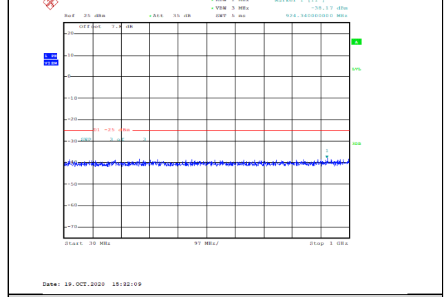
Band38-15MHz-QPSK-38175-1RB#0-Range1:30~1000MHz--38.17-PASS
