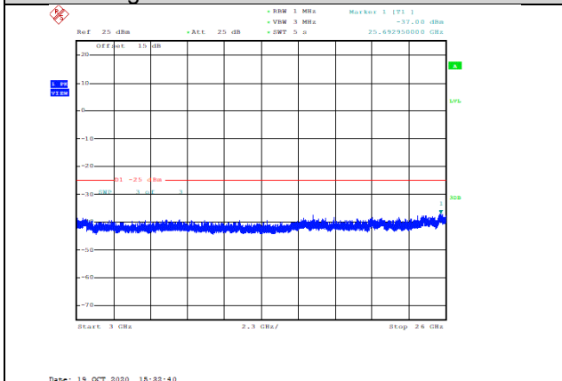
Band38-15MHz-QPSK-38175-1RB#0-Range3:3000~26000MHz--37-PASS
