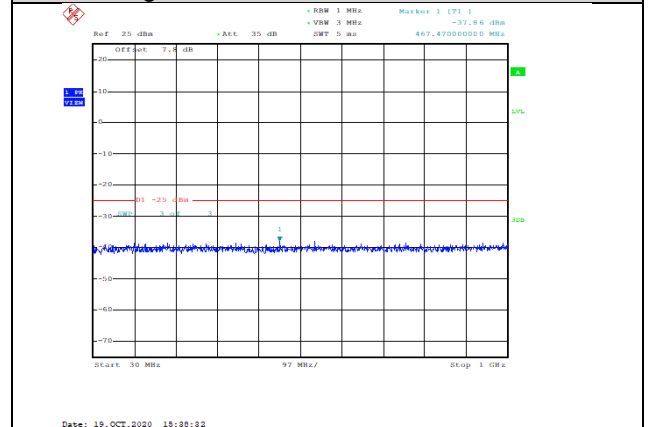
Band38-20MHz-16QAM-38000-1RB#0-Range1:30~1000MHz--37.86-PASS
