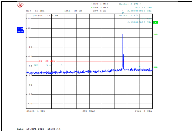
Band7-10MHz-16QAM-21100-1RB#0-Range2:1000~3000MHz--31.92-PASS
