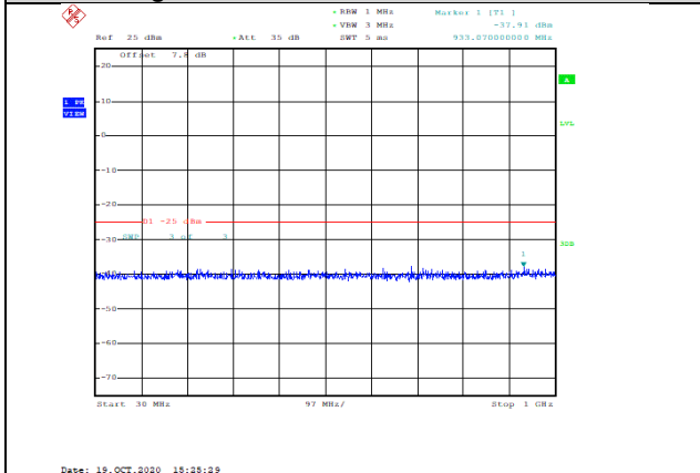
Band38-10MHz-16QAM-37800-1RB#0-Range1:30~1000MHz--37.91-PASS
