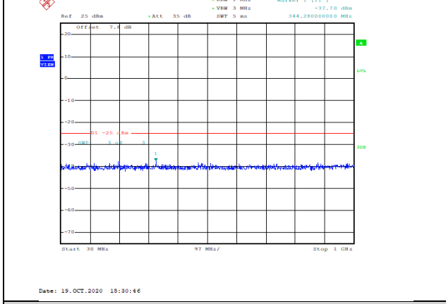
Band38-15MHz-QPSK-38000-1RB#0-Range1:30~1000MHz--37.7-PASS
