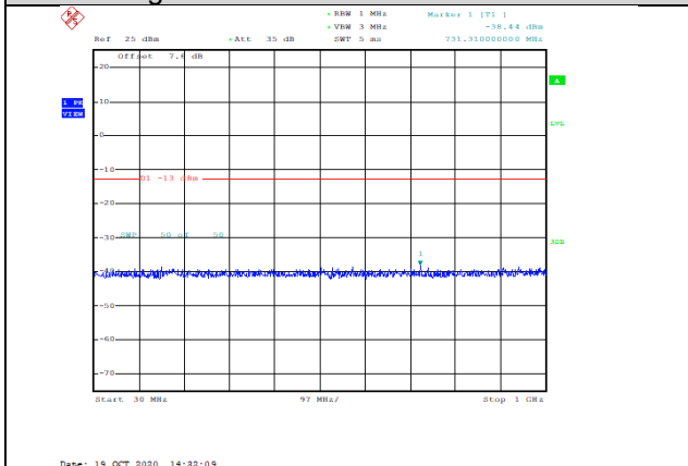
Band66-15MHz-16QAM-132322-1RB#0- Range1:30~1000MHz--38.44-PASS
