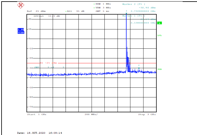
Band41-20MHz-QPSK-40140-1RB#0-Range2:1000~3000MHz--30.9-PASS
