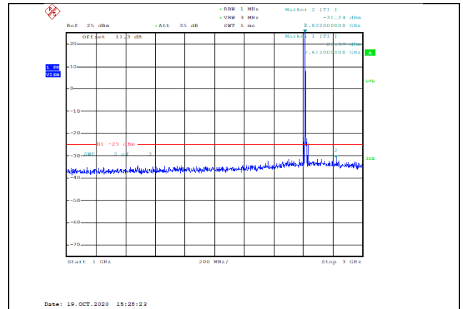
Band38-10MHz-16QAM-38200-1RB#0-Range2:1000~3000MHz--31.24-PASS
