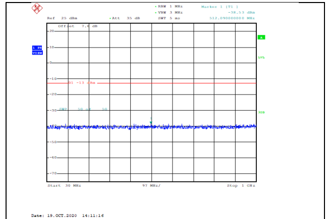
Band66-1.4MHz-16QAM-132665-1RB#0-Range1:30~1000MHz--38.53-PASS
