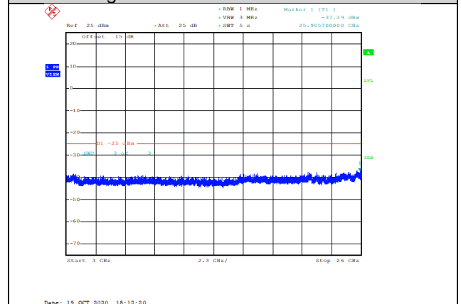
Band7-15MHz-16QAM-20825-1RB#0-Range3:3000~26000MHz--37.29-PASS
