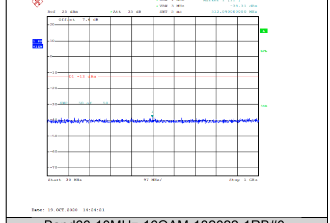
Band66-10MHz-16QAM-132022-1RB#0-Range1:30~1000MHz--38.31-PASS
