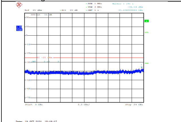
Band7-10MHz-16QAM-21100-1RB#0-Range3:3000~26000MHz--36.54-PASS
