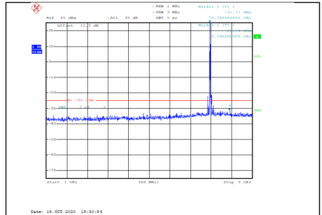
Band38-15MHz-QPSK-38000-1RB#0-Range2:1000~3000MHz--31.71-PASS
