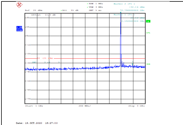
Band38-10MHz-16QAM-38000-1RB#0-Range2:1000~3000MHz--32.16-PASS
