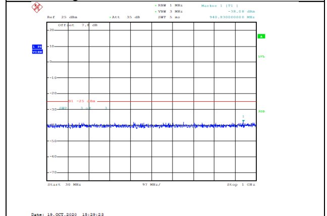
Band38-15MHz-QPSK-37825-1RB#0-Range1:30~1000MHz--38.08-PASS
