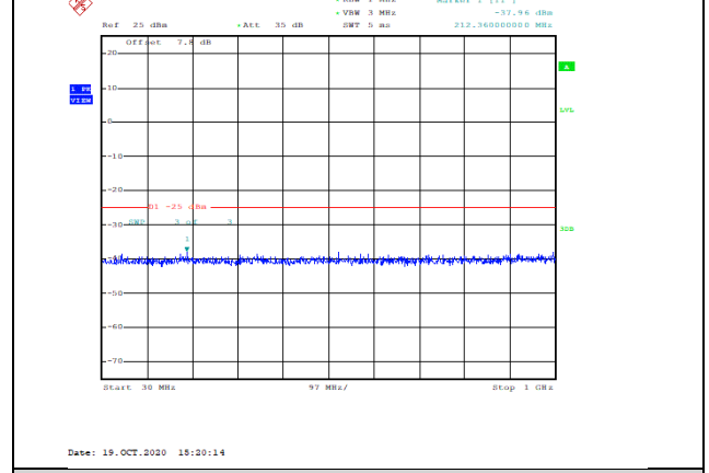
Band38-5MHz-QPSK-37775-1RB#0-Range1:30~1000MHz--37.96-PASS
