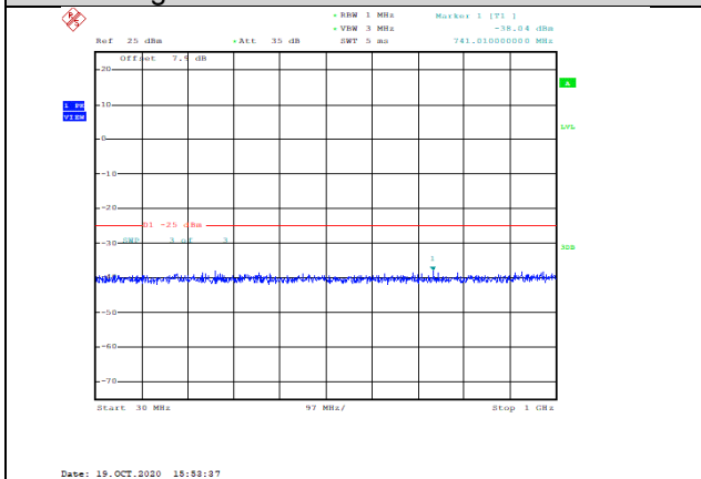
Band41-10MHz-16QAM-41190-1RB#0-Range1:30~1000MHz--38.04-PASS
