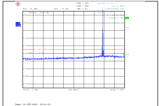
Band38-5MHz-16QAM-37775-1RB#0-Range2:1000~3000MHz--32.12-PASS
