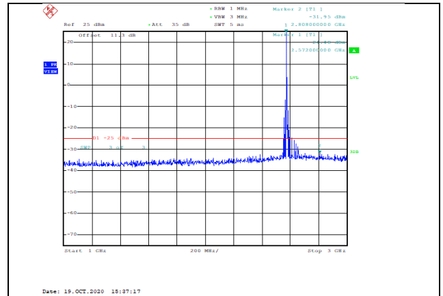
Band38-20MHz-16QAM-37850-1RB#0-Range2:1000~3000MHz--31.95-PASS
