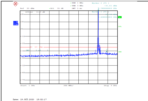
Band38-15MHz-QPSK-38175-1RB#0-Range2:1000~3000MHz--31.61-PASS
