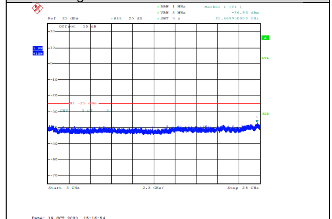
Band7-20MHz-16QAM-20850-1RB#0-Range3:3000~26000MHz--36.94-PASS
