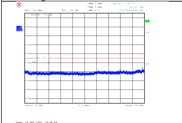
Band38-20MHz-QPSK-38150-1RB#0-Range3:3000~26000MHz--36.81-PASS
