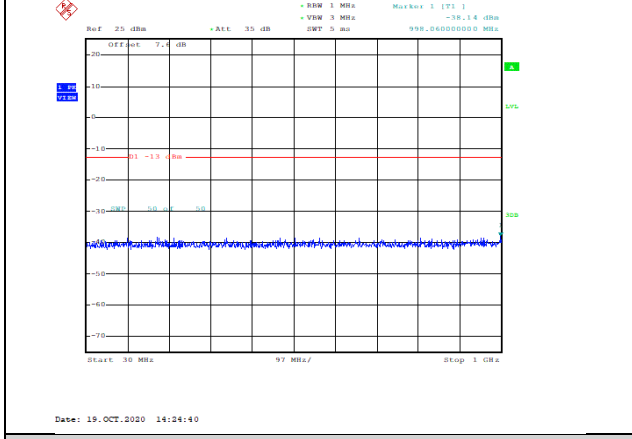
Band66-10MHz-QPSK-132322-1RB#0-Range1:30~1000MHz--38.14-PASS
