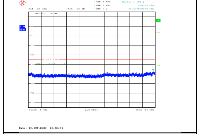
Band41-10MHz-QPSK-40590-1RB#0-Range3:3000~26000MHz--36.55-PASS
