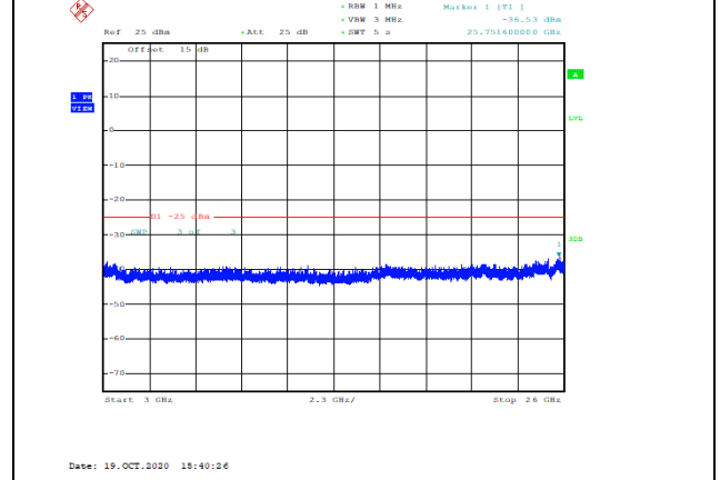
Band38-20MHz-16QAM-38150-1RB#0-Range3:3000~26000MHz--36.53-PASS
