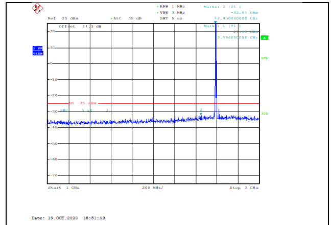
Band41-10MHz-QPSK-40590-1RB#0-Range2:1000~3000MHz--32.41-PASS
