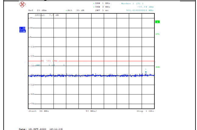
Band41-20MHz-16QAM-40590-1RB#0-Range1:30~1000MHz--37.34-PASS
