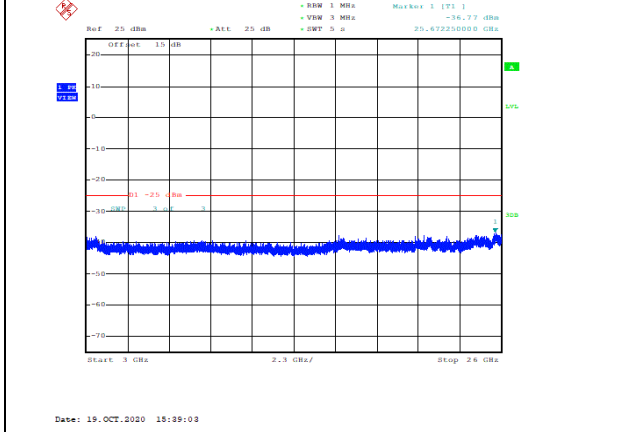
Band38-20MHz-16QAM-38000-1RB#0-Range3:3000~26000MHz--36.77-PASS
