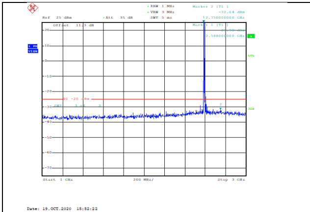
Band41-10MHz-16QAM-40590-1RB#0-Range2:1000~3000MHz--32.04-PASS
