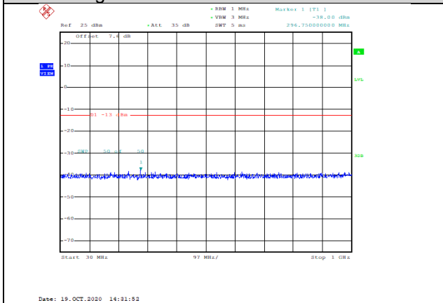
Band66-15MHz-QPSK-132322-1RB#0-Range1:30~1000MHz--38-PASS
