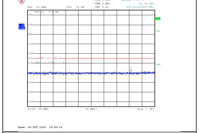
Band38-20MHz-QPSK-38150-1RB#0-Range1:30~1000MHz--38.39-PASS
