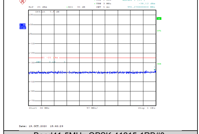
Band41-5MHz-QPSK-41215-1RB#0-Range1:30~1000MHz--38.12-PASS
