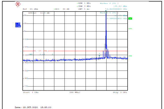
Band38-20MHz-QPSK-38000-1RB#0-Range2:1000~3000MHz--31.82-PASS
