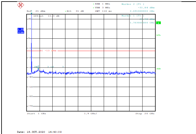
Band66-20MHz-16QAM-132072-1RB#0- Range2:1000~20000MHz--31.84-PASS
