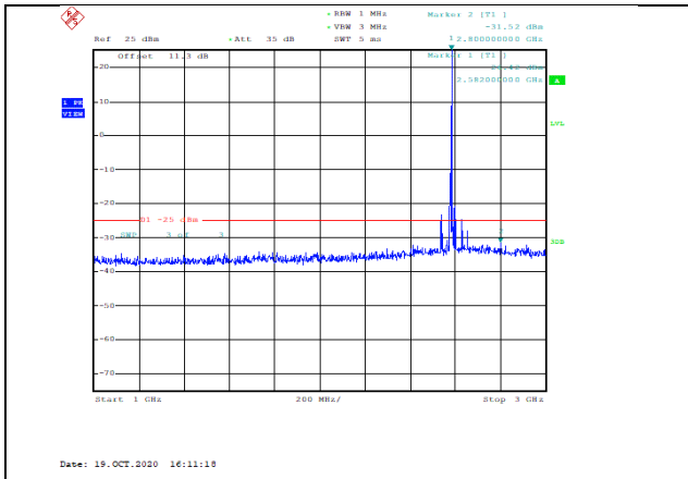
Band41-20MHz-16QAM-40590-1RB#0-Range2:1000~3000MHz--31.52-PASS
