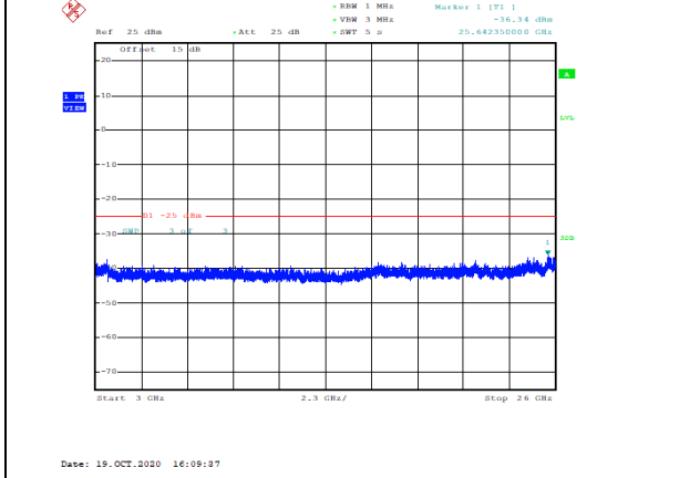
Band41-20MHz-QPSK-40140-1RB#0-Range3:3000~26000MHz--36.34-PASS
