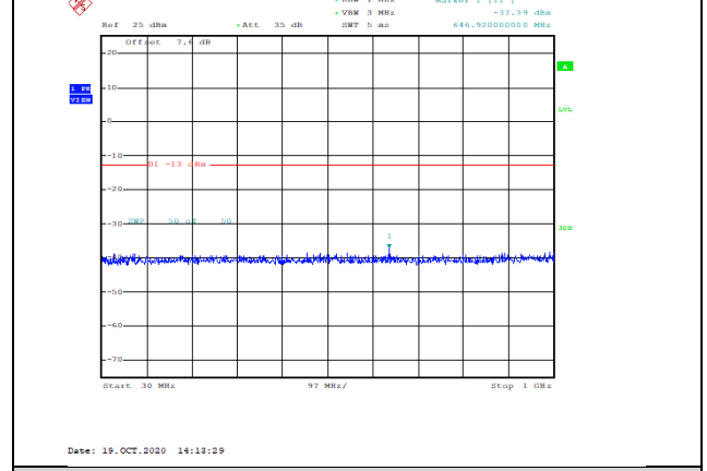
Band66-3MHz-16QAM-131987-1RB#0-Range1:30~1000MHz--37.39-PASS
