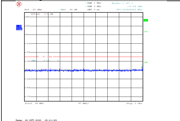
Band7-15MHz-16QAM-20825-1RB#0-Range1:30~1000MHz--37.48-PASS
