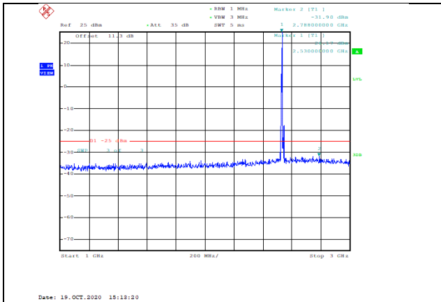
Band7-15MHz-16QAM-21100-1RB#0-Range2:1000~3000MHz--31.9-PASS
