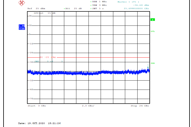
Band38-5MHz-16QAM-37775-1RB#0-Range3:3000~26000MHz--36.68-PASS
