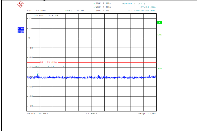
Band38-5MHz-QPSK-38000-1RB#0-Range1:30~1000MHz--37.84-PASS
