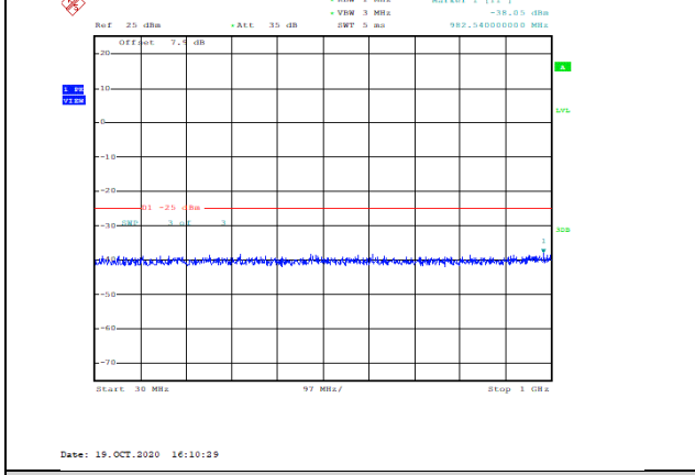
Band41-20MHz-QPSK-40590-1RB#0-Range1:30~1000MHz--38.05-PASS
