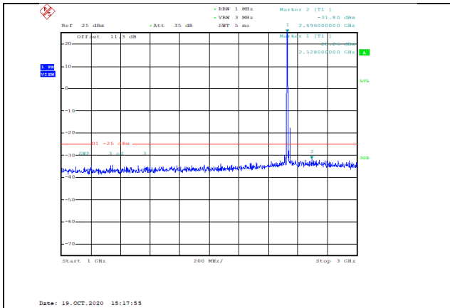
Band7-20MHz-16QAM-21100-1RB#0-Range2:1000~3000MHz--31.8-PASS
