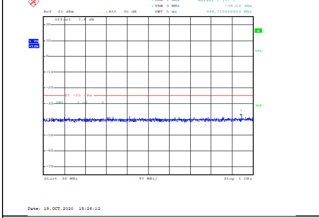
Band38-10MHz-QPSK-38000-1RB#0-Range1:30~1000MHz--38-PASS
