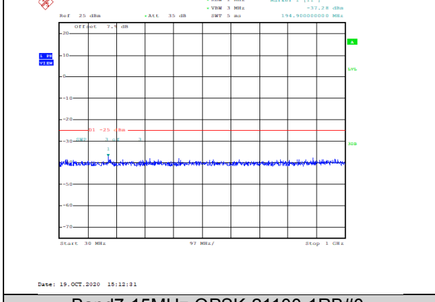
Band7-15MHz-QPSK-21100-1RB#0-Range1:30~1000MHz--37.28-PASS
