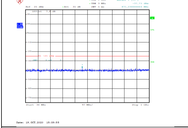
Band38-20MHz-16QAM-38150-1RB#0-Range1:30~1000MHz--37.75-PASS
