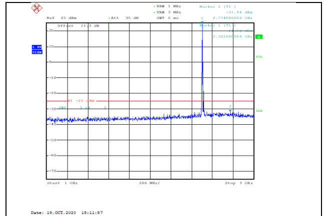
Band7-15MHz-16QAM-20825-1RB#0-Range2:1000~3000MHz--31.98-PASS
