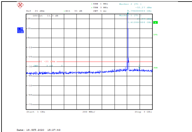
Band38-10MHz-QPSK-38200-1RB#0-Range2:1000~3000MHz--32.27-PASS
