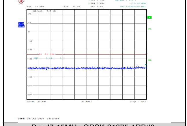
Band7-15MHz-QPSK-21375-1RB#0-Range1:30~1000MHz--37.56-PASS
