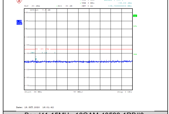
Band41-15MHz-16QAM-40590-1RB#0-Range1:30~1000MHz--38-PASS
