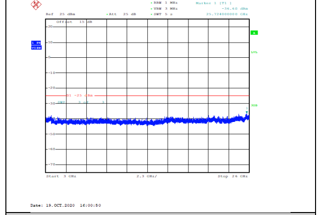
Band41-15MHz-16QAM-40115-1RB#0-Range3:3000~26000MHz--36.6-PASS
