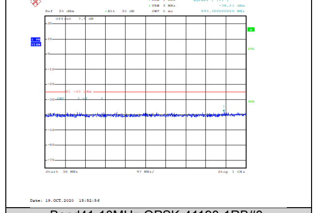
Band41-10MHz-QPSK-41190-1RB#0-Range1:30~1000MHz--38.21-PASS
