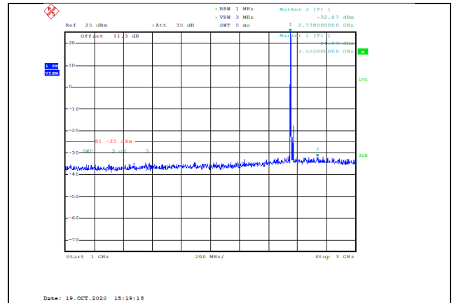
Band7-20MHz-16QAM-21350-1RB#0-Range2:1000~3000MHz--32.07-PASS
