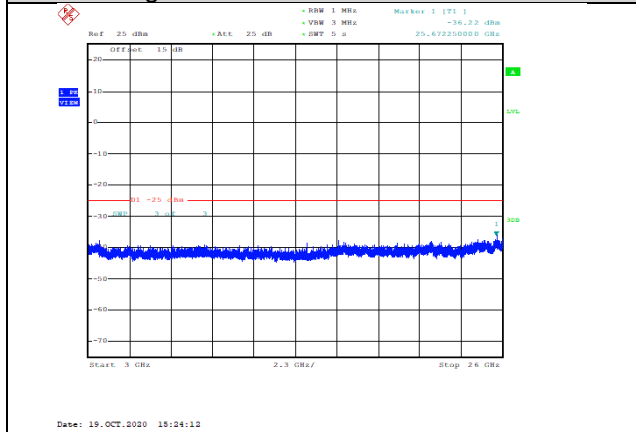
Band38-5MHz-16QAM-38225-1RB#0-Range3:3000~26000MHz--36.22-PASS
