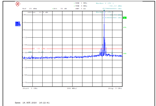
Band41-20MHz-16QAM-41140-1RB#0-Range2:1000~3000MHz--32.12-PASS
