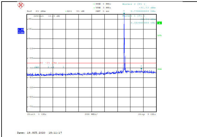
Band7-15MHz-QPSK-20825-1RB#0-Range2:1000~3000MHz--31.72-PASS
