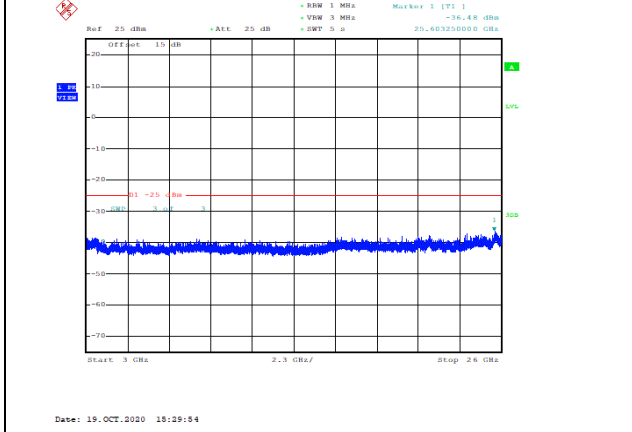
Band38-15MHz-QPSK-37825-1RB#0-Range3:3000~26000MHz--36.48-PASS
