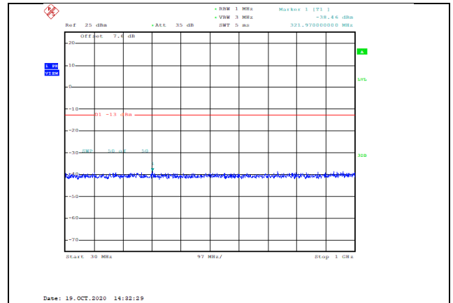
Band66-15MHz-QPSK-132597-1RB#0-Range1:30~1000MHz--38.46-PASS
