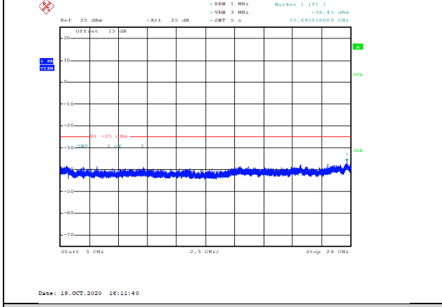
Band41-20MHz-16QAM-40590-1RB#0-Range3:3000~26000MHz--36.45-PASS
