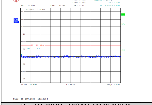
Band41-20MHz-16QAM-41140-1RB#0-Range1:30~1000MHz--38.35-PASS
