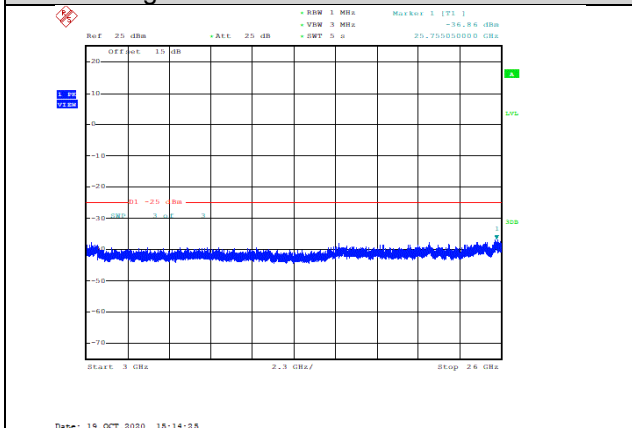
Band7-15MHz-QPSK-21375-1RB#0-Range3:3000~26000MHz--36.86-PASS
