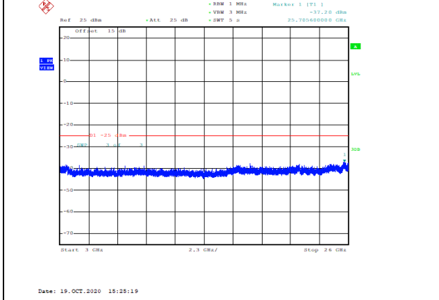
Band38-10MHz-QPSK-37800-1RB#0-Range3:3000~26000MHz--37.2-PASS
