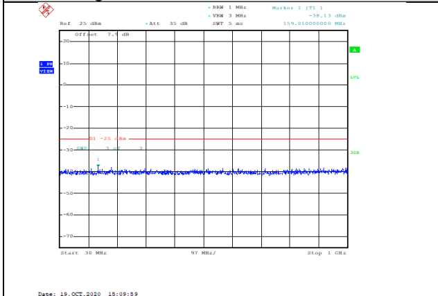
Band7-10MHz-16QAM-21400-1RB#0-Range1:30~1000MHz--38.13-PASS
