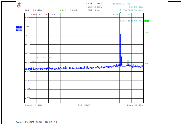
Band38-5MHz-QPSK-38225-1RB#0-Range2:1000~3000MHz--32.08-PASS
