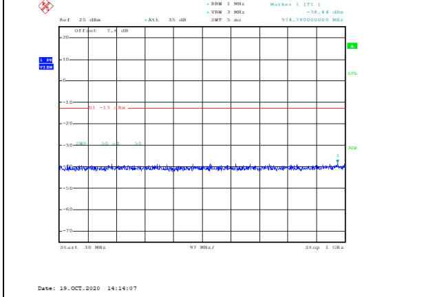
Band66-3MHz-16QAM-132322-1RB#0-Range1:30~1000MHz--38.44-PASS
