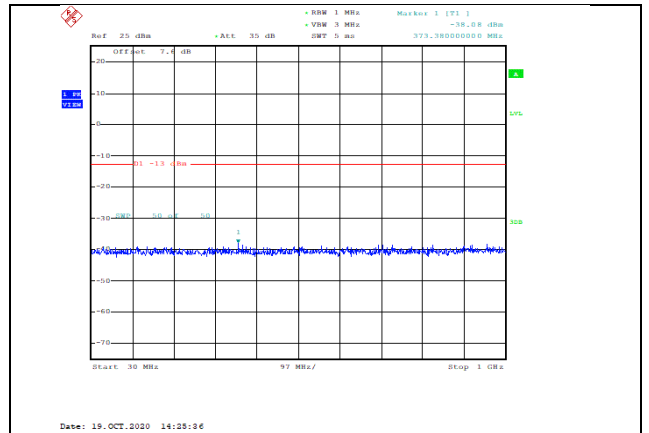
Band66-10MHz-16QAM-132622-1RB#0-Range1:30~1000MHz--38.08-PASS
