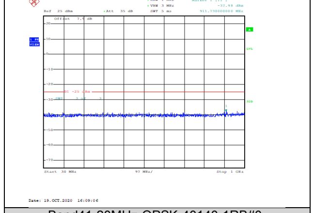
Band41-20MHz-QPSK-40140-1RB#0-Range1:30~1000MHz--37.98-PASS
