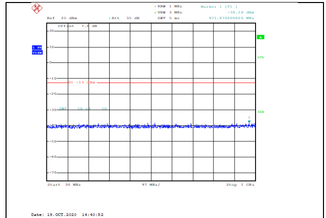
Band66-20MHz-QPSK-132572-1RB#0-Range1:30~1000MHz--38.28-PASS
