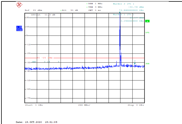
Band38-15MHz-16QAM-38000-1RB#0-Range2:1000~3000MHz--31.78-PASS
