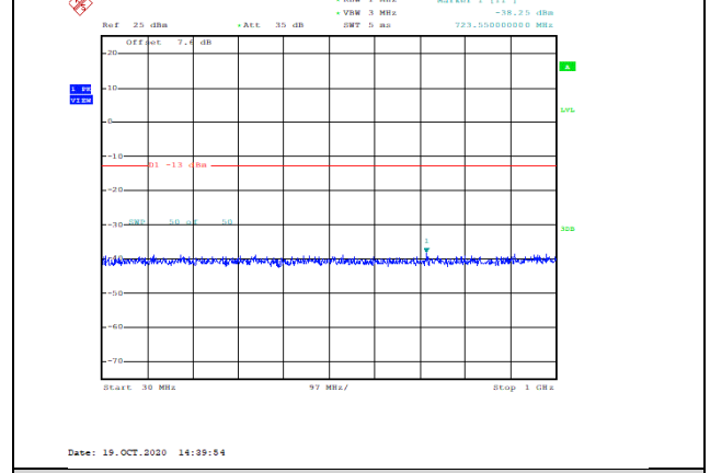
Band66-20MHz-16QAM-132072-1RB#0-Range1:30~1000MHz--38.25-PASS
