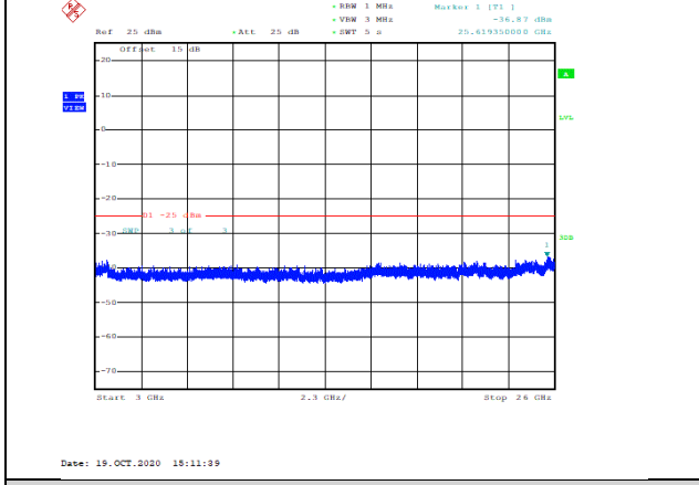
Band7-15MHz-QPSK-20825-1RB#0-Range3:3000~26000MHz--36.87-PASS
