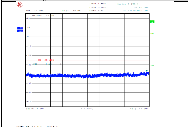
Band7-20MHz-QPSK-21350-1RB#0-Range3:3000~26000MHz--37.4-PASS
