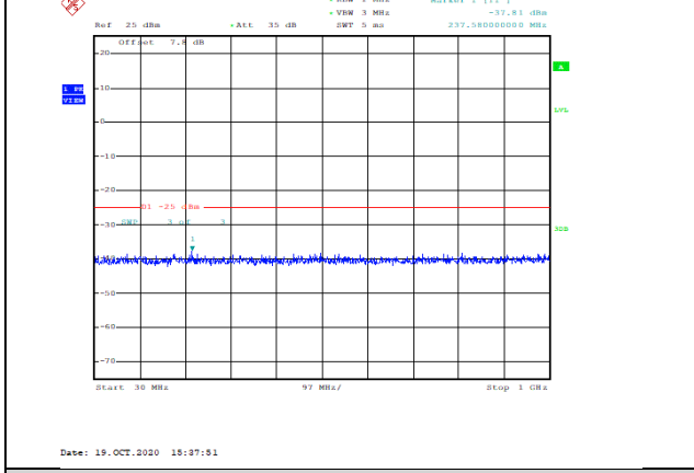
Band38-20MHz-QPSK-38000-1RB#0-Range1:30~1000MHz--37.81-PASS
