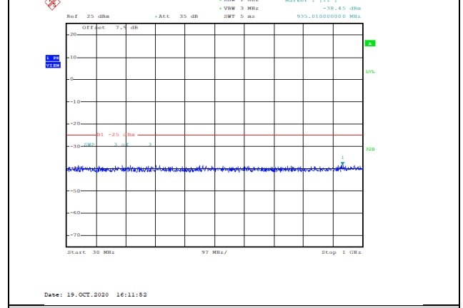
Band41-20MHz-QPSK-41140-1RB#0-Range1:30~1000MHz--38.45-PASS
