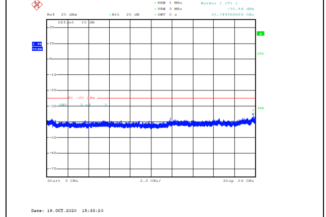
Band38-15MHz-16QAM-38175-1RB#0-Range3:3000~26000MHz--35.94-PASS
