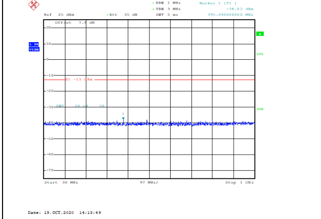
Band66-3MHz-QPSK-132322-1RB#0-Range1:30~1000MHz--38.02-PASS
