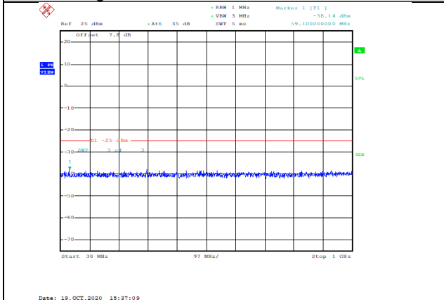
Band38-20MHz-16QAM-37850-1RB#0-Range1:30~1000MHz--38.14-PASS
