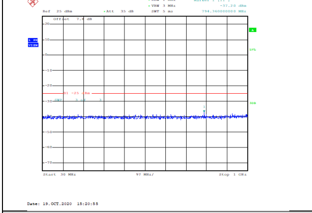
Band38-5MHz-16QAM-37775-1RB#0-Range1:30~1000MHz--37.2-PASS
