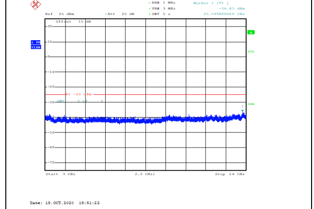
Band41-10MHz-16QAM-40090-1RB#0-Range3:3000~26000MHz--36.45-PASS
