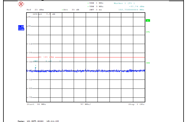
Band7-15MHz-QPSK-20825-1RB#0-Range1:30~1000MHz--37.76-PASS
