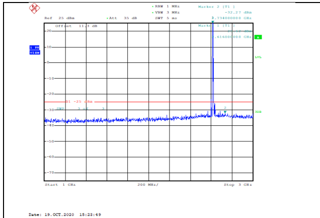
Band38-5MHz-16QAM-38225-1RB#0-Range2:1000~3000MHz--32.27-PASS
