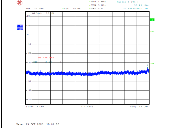
Band38-15MHz-16QAM-38000-1RB#0-Range3:3000~26000MHz--36.47-PASS
