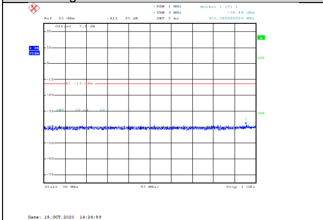
Band66-10MHz-16QAM-132322-1RB#0-Range1:30~1000MHz--38.48-PASS
