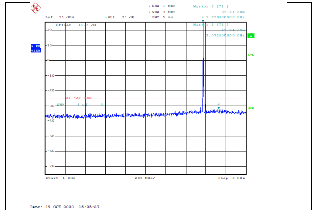
Band38-10MHz-16QAM-37800-1RB#0-Range2:1000~3000MHz--32.21-PASS
