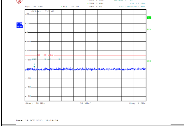
Band7-20MHz-16QAM-21350-1RB#0-Range1:30~1000MHz--38.29-PASS
