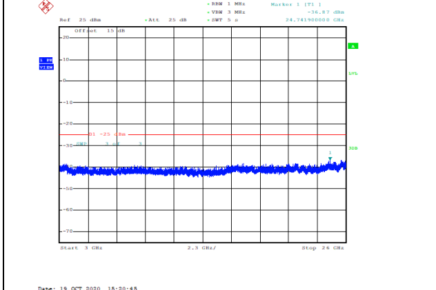
Band38-5MHz-QPSK-37775-1RB#0-Range3:3000~26000MHz--36.87-PASS
