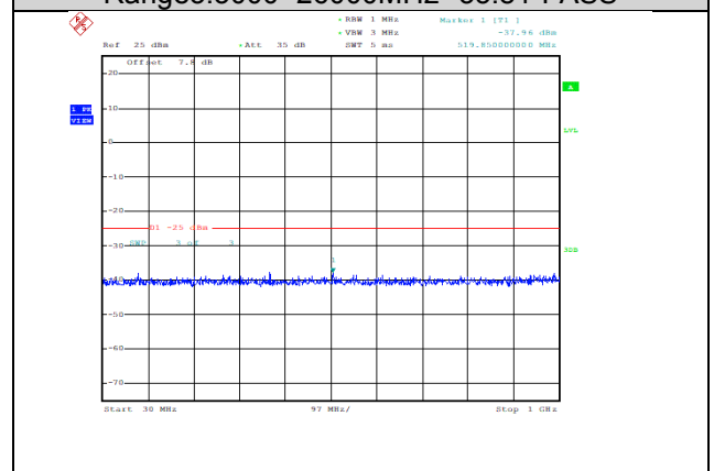
Band38-15MHz-16QAM-38000-1RB#0-Range1:30~1000MHz--37.96-PASS
