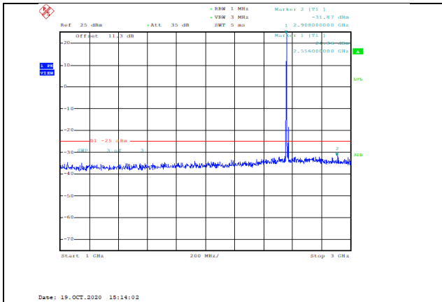
Band7-15MHz-QPSK-21375-1RB#0-Range2:1000~3000MHz--31.87-PASS
