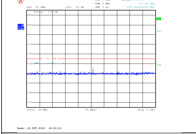
Band41-10MHz-16QAM-40090-1RB#0-Range1:30~1000MHz--37.68-PASS
