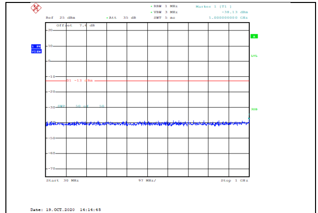
Band66-3MHz-16QAM-132657-1RB#0-Range1:30~1000MHz--38.13-PASS
