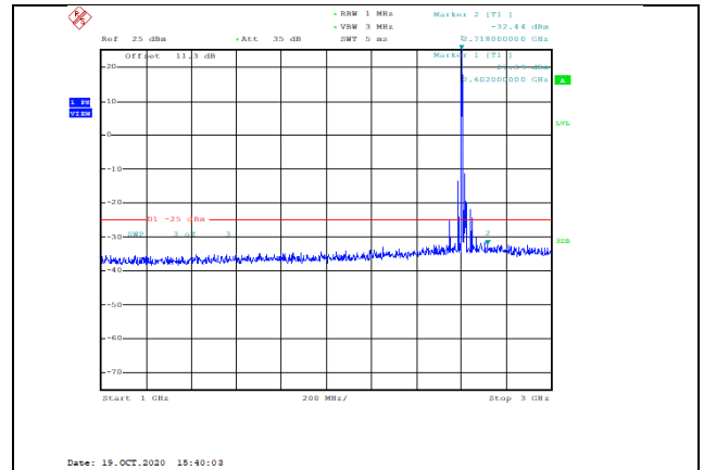
Band38-20MHz-16QAM-38150-1RB#0-Range2:1000~3000MHz--32.44-PASS
