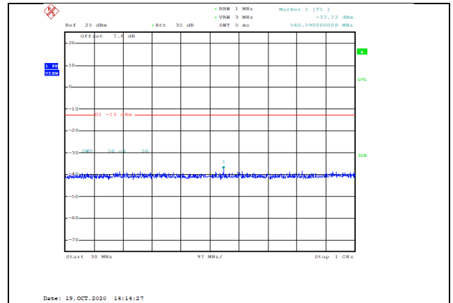
Band66-3MHz-QPSK-132657-1RB#0-Range1:30~1000MHz--37.72-PASS
