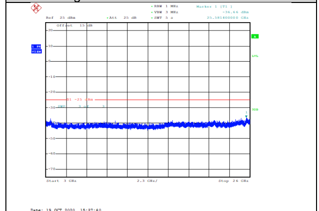
Band38-20MHz-16QAM-37850-1RB#0-Range3:3000~26000MHz--36.66-PASS
