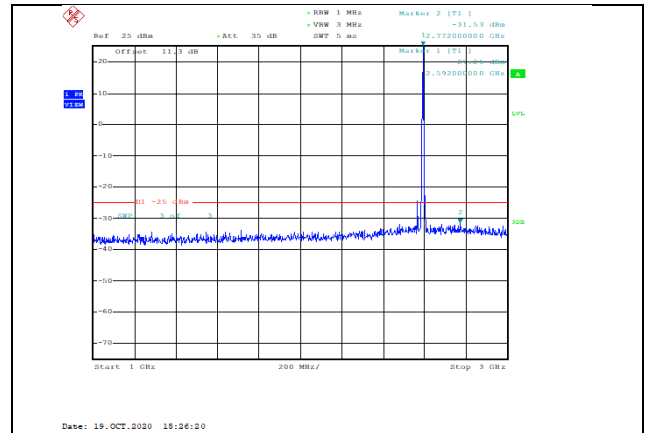
Band38-10MHz-QPSK-38000-1RB#0-Range2:1000~3000MHz--31.53-PASS
