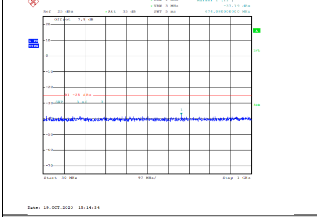
Band7-15MHz-16QAM-21375-1RB#0-Range1:30~1000MHz--37.79-PASS
