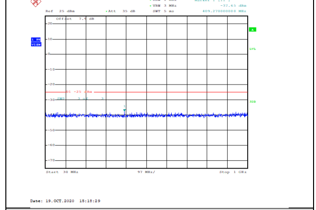
Band7-20MHz-QPSK-21350-1RB#0-Range1:30~1000MHz--37.65-PASS
