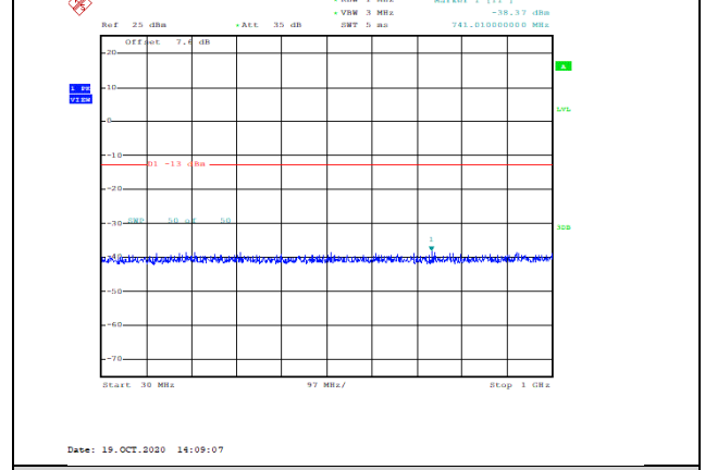
Band66-1.4MHz-16QAM-131979-1RB#0-Range1:30~1000MHz--38.37-PASS
