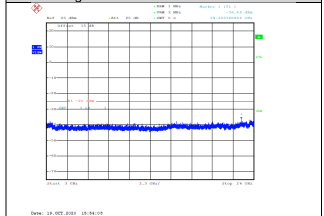
Band41-10MHz-16QAM-41190-1RB#0-Range3:3000~26000MHz--36.6-PASS
