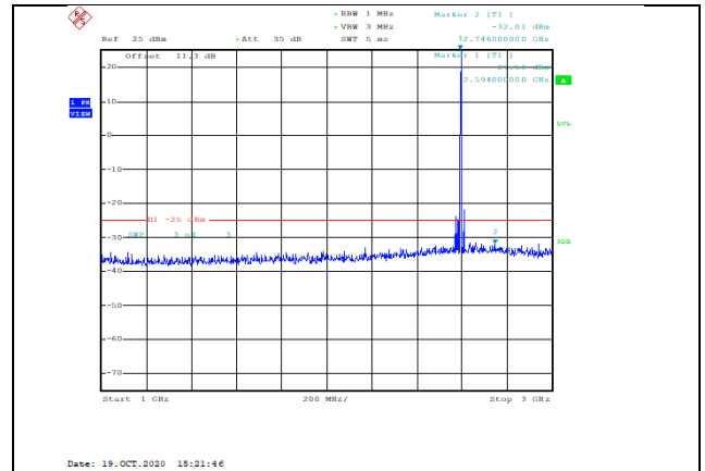
Band38-5MHz-QPSK-38000-1RB#0-Range2:1000~3000MHz--32.01-PASS
