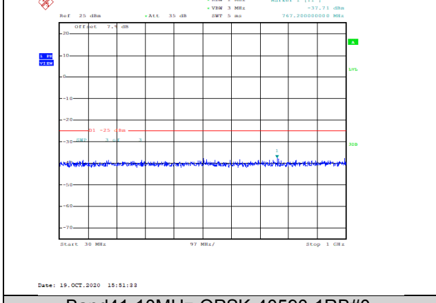
Band41-10MHz-QPSK-40590-1RB#0-Range1:30~1000MHz--37.71-PASS
