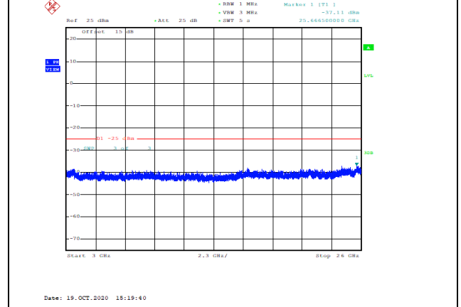
Band7-20MHz-16QAM-21350-1RB#0-Range3:3000~26000MHz--37.11-PASS
