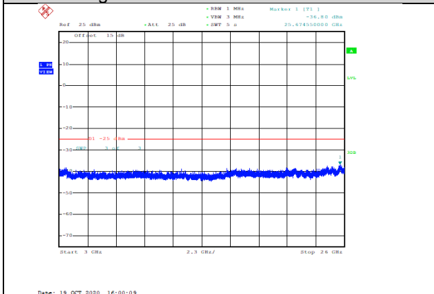
Band41-15MHz-QPSK-40115-1RB#0-Range3:3000~26000MHz--36.8-PASS
