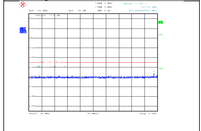
Band38-5MHz-QPSK-38225-1RB#0-Range1:30~1000MHz--37.93-PASS
