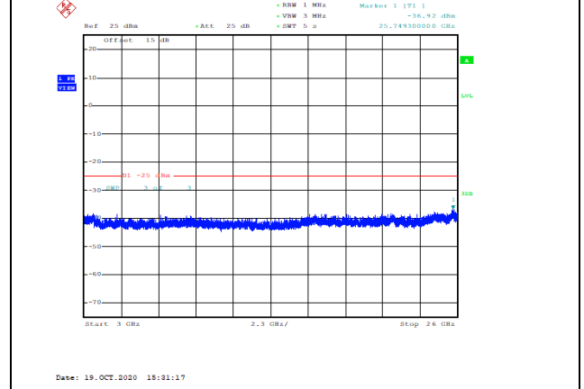
Band38-15MHz-QPSK-38000-1RB#0-Range3:3000~26000MHz--36.92-PASS
