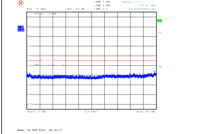
Band7-20MHz-16QAM-21100-1RB#0-Range3:3000~26000MHz--36.89-PASS
