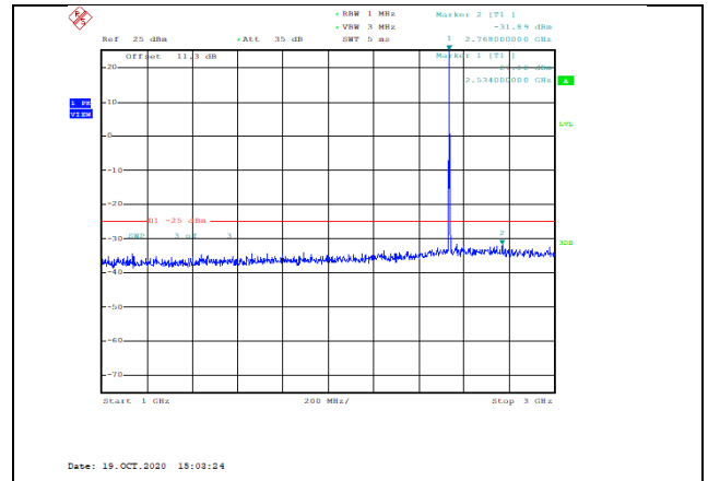
Band7-5MHz-QPSK-21100-1RB#0-Range2:1000~3000MHz--31.89-PASS
