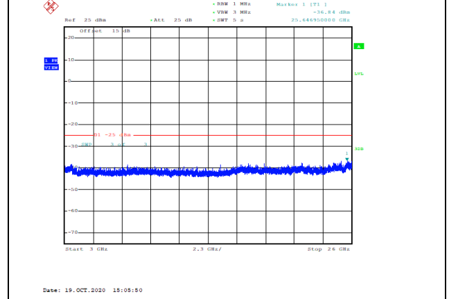
Band7-5MHz-16QAM-21425-1RB#0-Range3:3000~26000MHz--36.84-PASS
