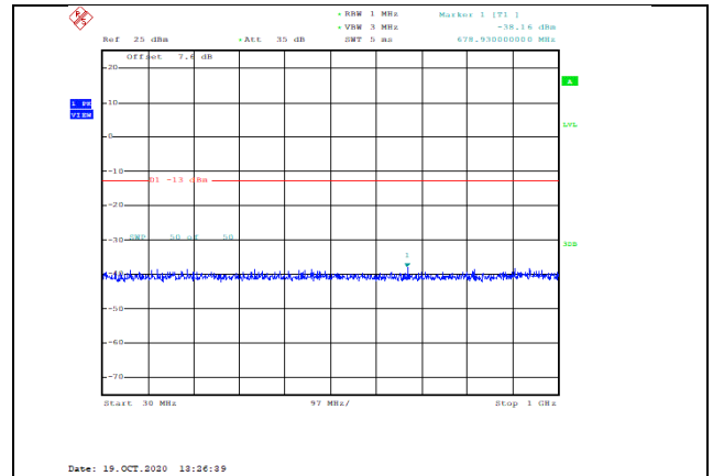
Band2-10MHz-16QAM-19150-1RB#0-Range1:30~1000MHz--38.16-PASS
