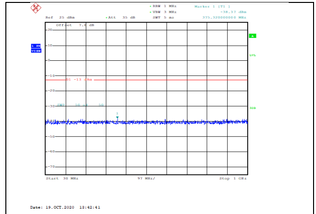
Band4-1.4MHz-QPSK-20393-1RB#0-Range1:30~1000MHz--38.37-PASS
