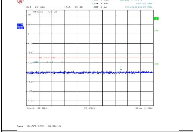
Band7-5MHz-16QAM-21425-1RB#0-Range1:30~1000MHz--38.06-PASS
