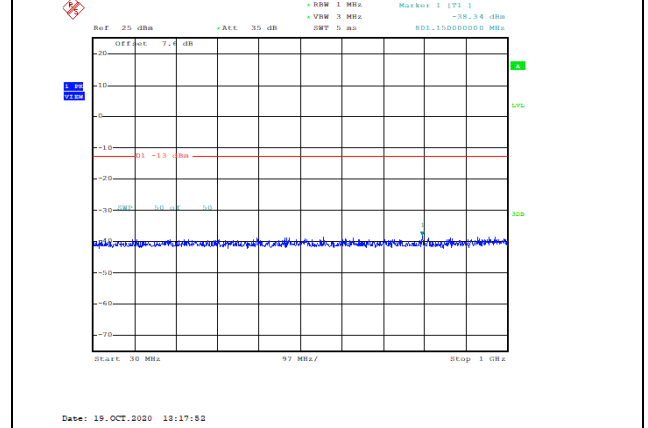
Band2-5MHz-QPSK-18625-1RB#0-Range1:30~1000MHz--38.34-PASS
