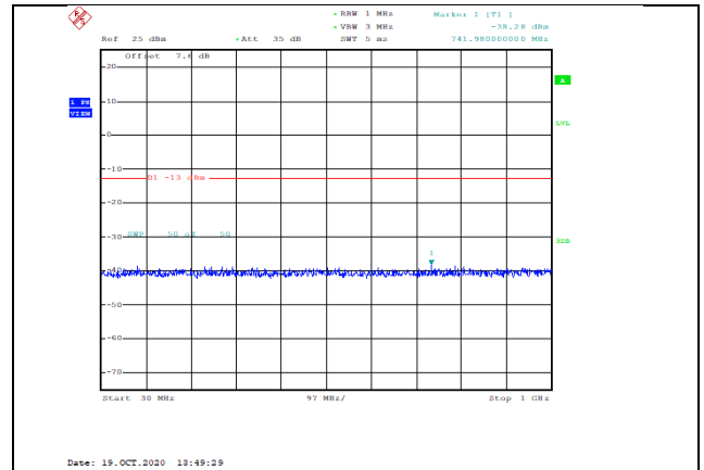
Band4-10MHz-QPSK-20350-1RB#0-Range1:30~1000MHz--38.28-PASS
