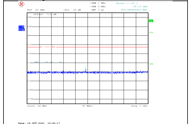
Band2-15MHz-QPSK-18675-1RB#0-Range1:30~1000MHz--38.56-PASS
