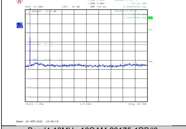
Band4-10MHz-16QAM-20175-1RB#0-Range2:1000~20000MHz--31.3-PASS
