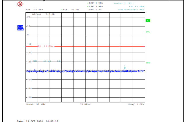
Band2-10MHz-QPSK-18650-1RB#0-Range1:30~1000MHz--37.87-PASS
