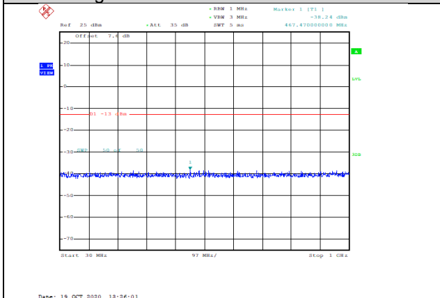
Band2-10MHz-16QAM-18900-1RB#0-Range1:30~1000MHz--38.24-PASS
