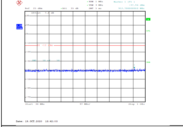
Band4-1.4MHz-QPSK-20175-1RB#0-Range1:30~1000MHz--37.96-PASS
