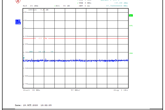
Band2-15MHz-16QAM-18675-1RB#0-Range1:30~1000MHz--37.88-PASS
