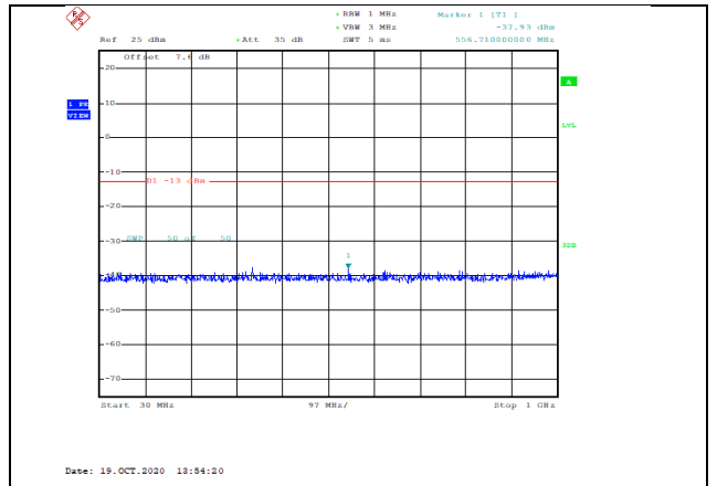
Band4-20MHz-QPSK-20300-1RB#0-Range1:30~1000MHz--37.93-PASS
