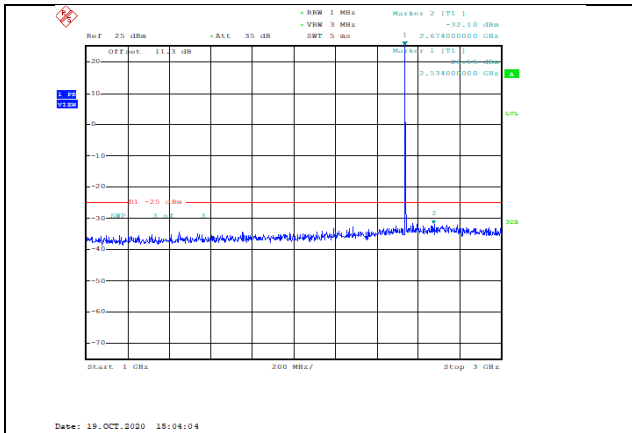
Band7-5MHz-16QAM-21100-1RB#0-Range2:1000~3000MHz--32.1-PASS
