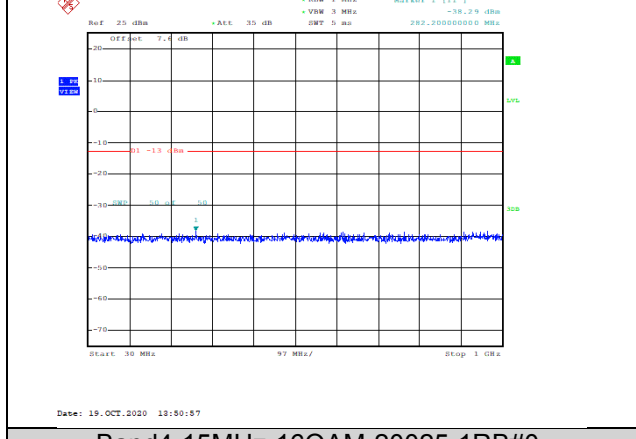
Band4-15MHz-16QAM-20025-1RB#0-Range1:30~1000MHz--38.29-PASS
