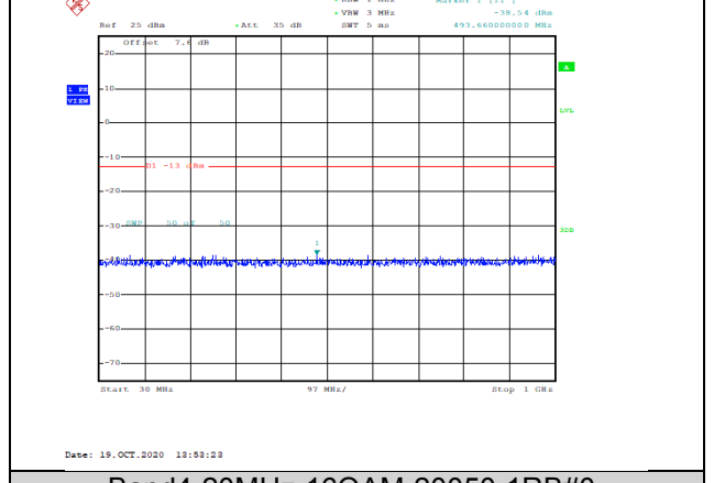
Band4-20MHz-16QAM-20050-1RB#0-Range1:30~1000MHz--38.54-PASS
