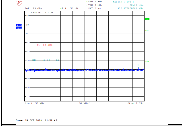
Band4-20MHz-QPSK-20175-1RB#0-Range1:30~1000MHz--38.38-PASS
