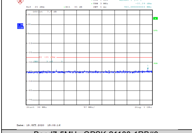
Band7-5MHz-QPSK-21100-1RB#0-Range1:30~1000MHz--37.39-PASS
