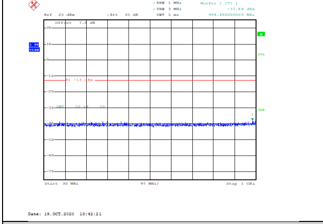
Band4-1.4MHz-16QAM-20175-1RB#0-Range1:30~1000MHz--37.88-PASS
