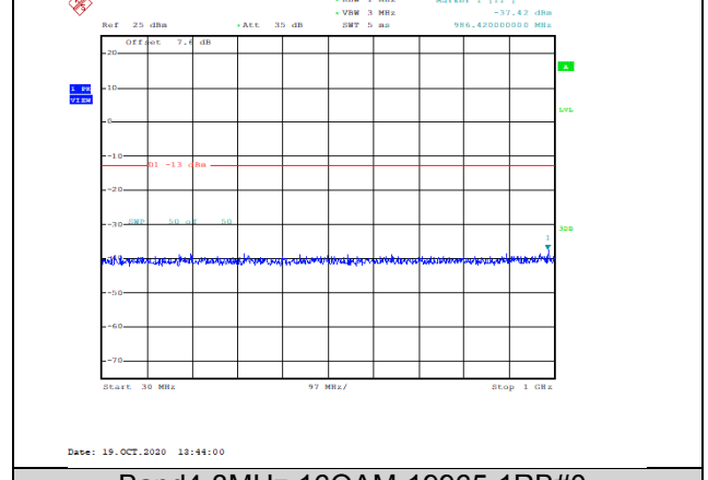
Band4-3MHz-16QAM-19965-1RB#0-Range1:30~1000MHz--37.42-PASS
