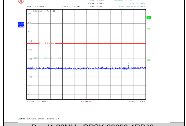
Band4-20MHz-QPSK-20050-1RB#0-Range1:30~1000MHz--38.52-PASS
