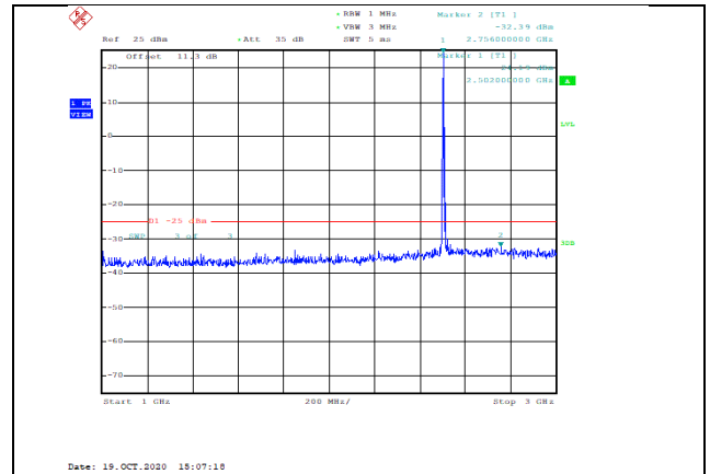
Band7-10MHz-16QAM-20800-1RB#0-Range2:1000~3000MHz--32.39-PASS
