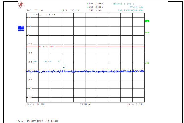
Band2-3MHz-16QAM-19185-1RB#0-Range1:30~1000MHz--37.59-PASS
