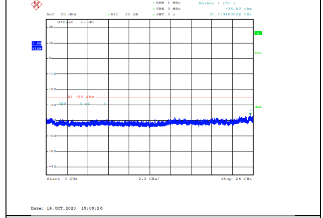
Band7-10MHz-QPSK-21100-1RB#0-Range3:3000~26000MHz--36.82-PASS
