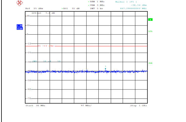
Band2-20MHz-16QAM-18900-1RB#0-Range1:30~1000MHz--38.36-PASS
