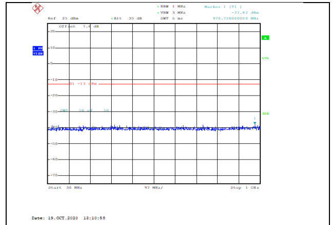
Band2-1.4MHz-16QAM-19193-1RB#0-Range1:30~1000MHz--37.82-PASS
