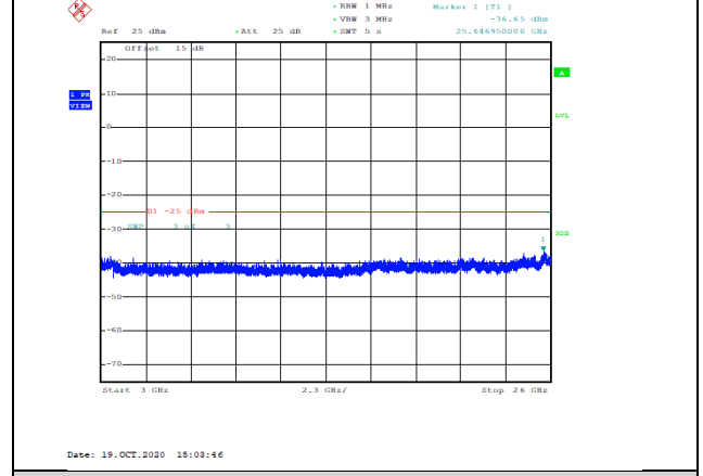
Band7-5MHz-QPSK-21100-1RB#0-Range3:3000~26000MHz--36.65-PASS
