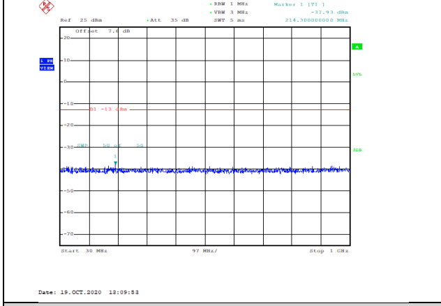
Band2-1.4MHz-16QAM-18900-1RB#0-Range1:30~1000MHz--37.93-PASS
