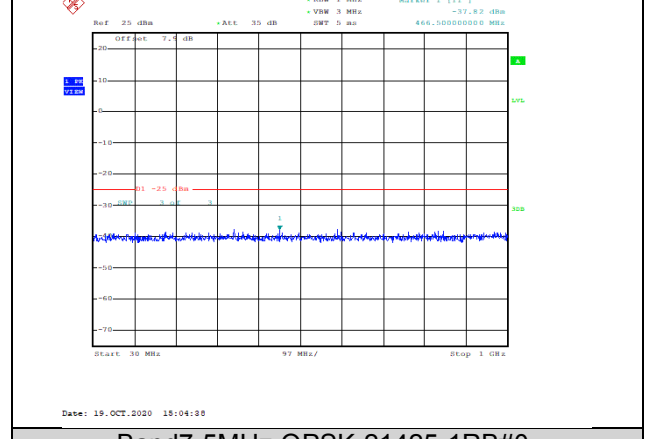
Band7-5MHz-QPSK-21425-1RB#0-Range1:30~1000MHz--37.82-PASS
