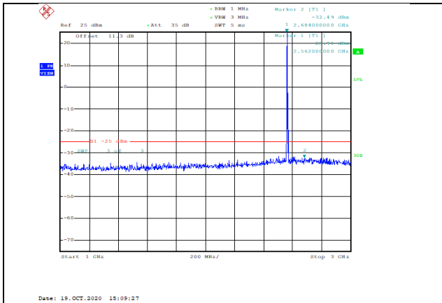
Band7-10MHz-QPSK-21400-1RB#0-Range2:1000~3000MHz--32.49-PASS
