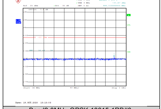
Band2-3MHz-QPSK-18615-1RB#0-Range1:30~1000MHz--37.47-PASS
