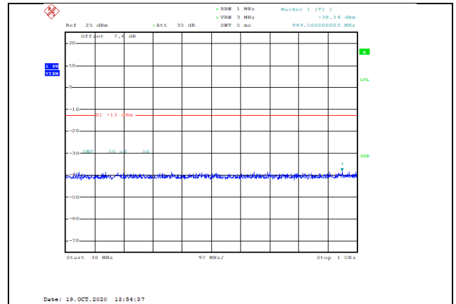
Band4-20MHz-16QAM-20300-1RB#0-Range1:30~1000MHz--38.34-PASS
