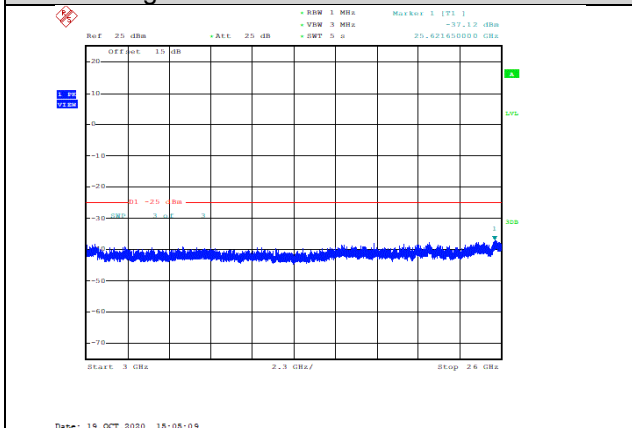
Band7-5MHz-QPSK-21425-1RB#0-Range3:3000~26000MHz--37.12-PASS
