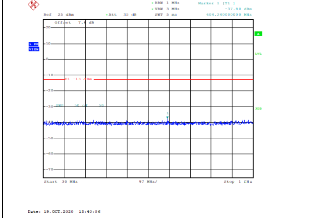
Band2-20MHz-QPSK-18900-1RB#0-Range1:30~1000MHz--37.8-PASS
