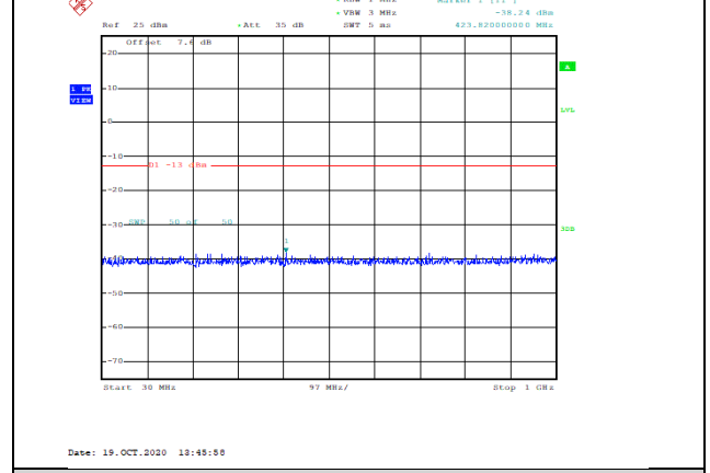
Band4-5MHz-QPSK-19975-1RB#0-Range1:30~1000MHz--38.24-PASS
