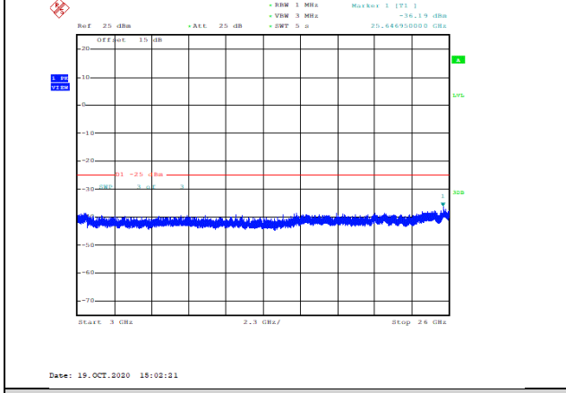
Band7-5MHz-QPSK-20775-1RB#0-Range3:3000~26000MHz--36.19-PASS
