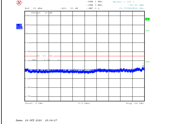
Band7-5MHz-16QAM-21100-1RB#0-Range3:3000~26000MHz--36.92-PASS
