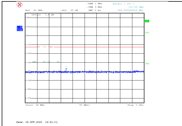
Band2-20MHz-16QAM-19100-1RB#0-Range1:30~1000MHz--37.99-PASS
