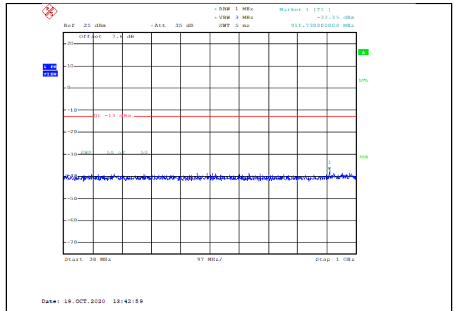
Band4-1.4MHz-16QAM-20393-1RB#0-Range1:30~1000MHz--37.35-PASS
