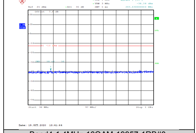
Band4-1.4MHz-16QAM-19957-1RB#0-Range1:30~1000MHz--38.38-PASS
