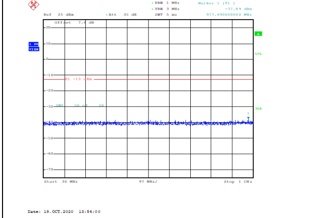
Band4-20MHz-16QAM-20175-1RB#0-Range1:30~1000MHz--37.89-PASS
