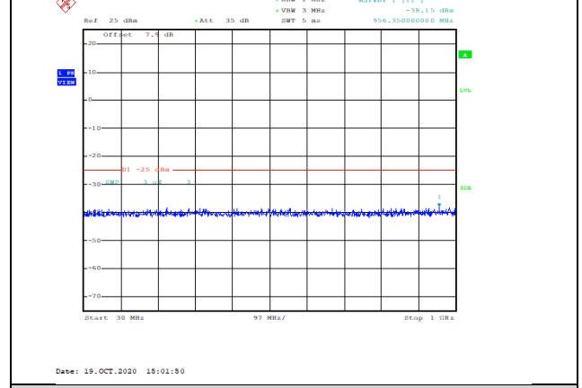
Band7-5MHz-QPSK-20775-1RB#0-Range1:30~1000MHz--38.15-PASS
