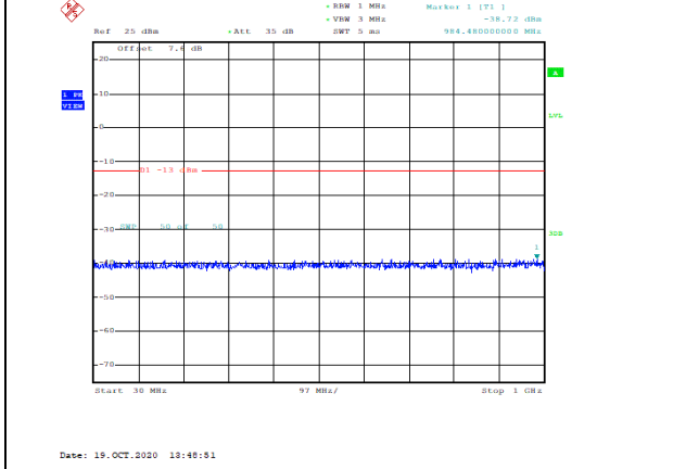
Band4-10MHz-QPSK-20175-1RB#0-Range1:30~1000MHz--38.72-PASS
