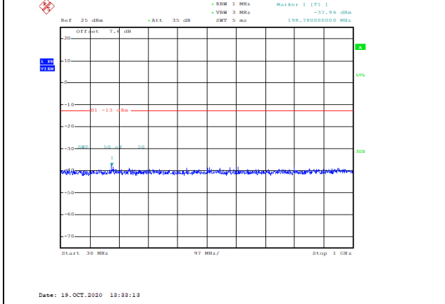
Band2-15MHz-16QAM-18900-1RB#0-Range1:30~1000MHz--37.96-PASS
