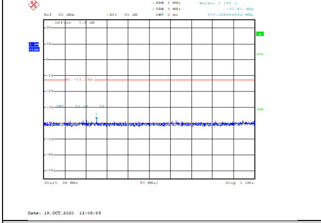
Band2-1.4MHz-QPSK-18900-1RB#0-Range1:30~1000MHz--37.81-PASS
