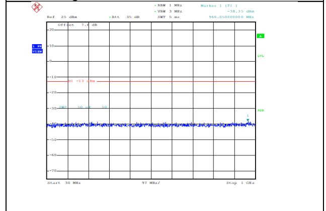
Band2-5MHz-16QAM-18625-1RB#0-Range1:30~1000MHz--38.35-PASS
