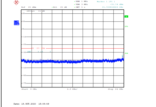
Band7-10MHz-QPSK-21400-1RB#0-Range3:3000~26000MHz--35.74-PASS
