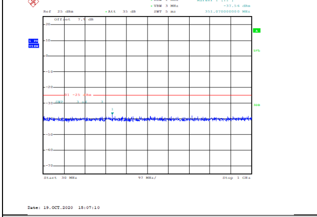
Band7-10MHz-16QAM-20800-1RB#0-Range1:30~1000MHz--37.56-PASS
