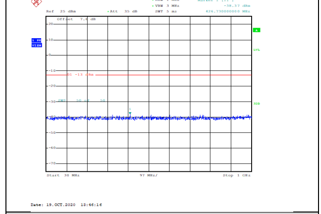
Band4-5MHz-16QAM-19975-1RB#0-Range1:30~1000MHz--38.37-PASS
