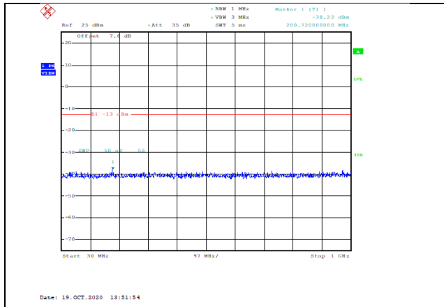
Band4-15MHz-QPSK-20325-1RB#0-Range1:30~1000MHz--38.22-PASS
