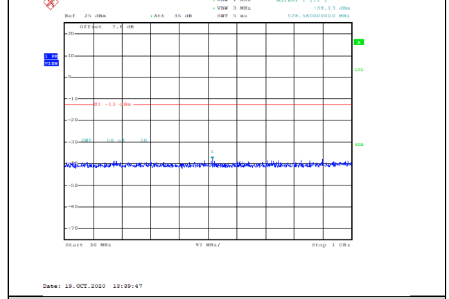
Band2-20MHz-16QAM-18700-1RB#0-Range1:30~1000MHz--38.13-PASS
