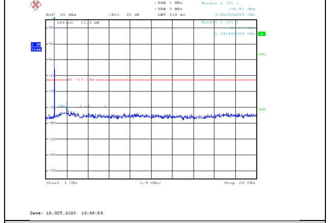
Band4-10MHz-16QAM-20350-1RB#0-Range2:1000~20000MHz--30.91-PASS
