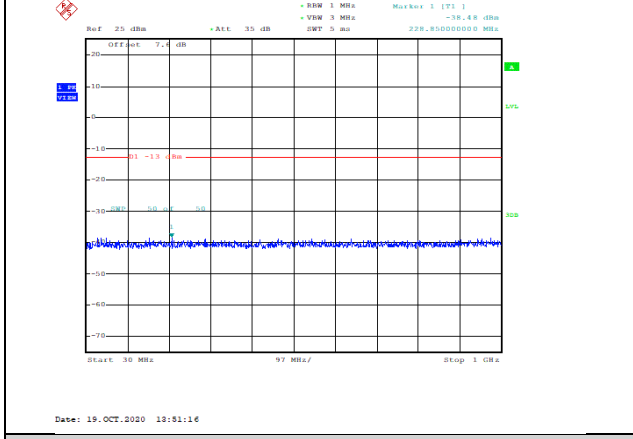
Band4-15MHz-QPSK-20175-1RB#0-Range1:30~1000MHz--38.48-PASS
