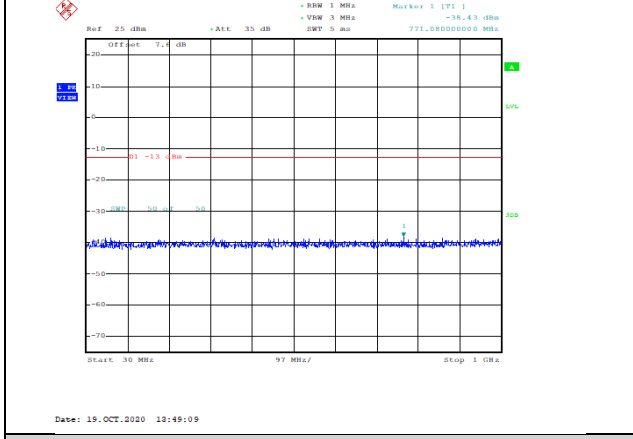
Band4-10MHz-16QAM-20175-1RB#0-Range1:30~1000MHz--38.43-PASS
