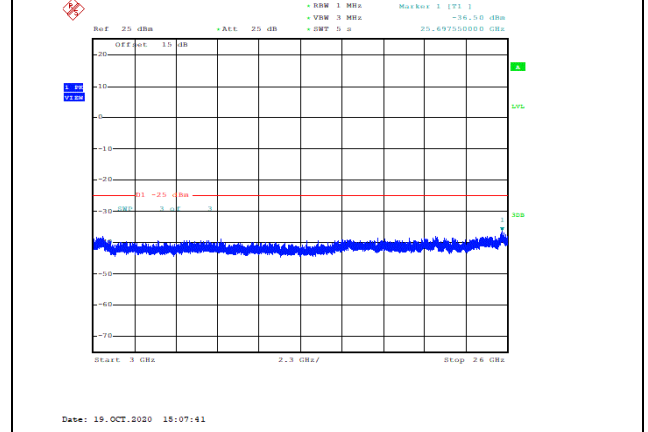
Band7-10MHz-16QAM-20800-1RB#0-Range3:3000~26000MHz--36.5-PASS
