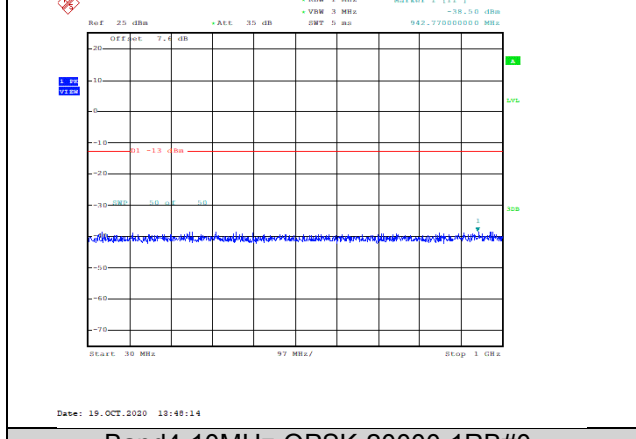
Band4-10MHz-QPSK-20000-1RB#0-Range1:30~1000MHz--38.5-PASS
