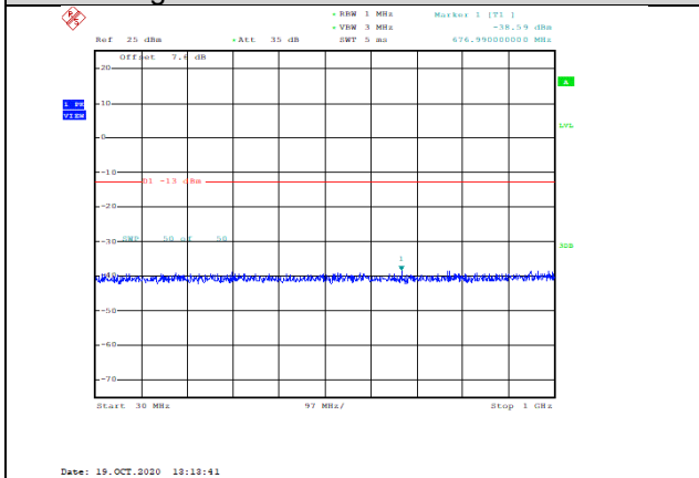
Band2-3MHz-QPSK-18900-1RB#0-Range1:30~1000MHz--38.59-PASS
