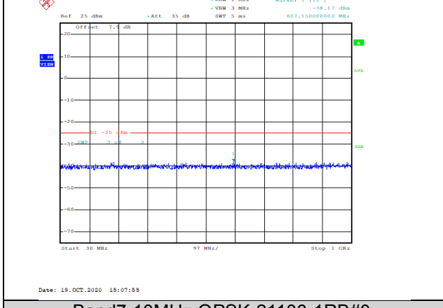
Band7-10MHz-QPSK-21100-1RB#0-Range1:30~1000MHz--38.17-PASS
