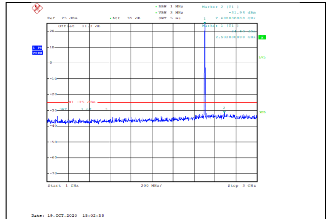
Band7-5MHz-16QAM-20775-1RB#0-Range2:1000~3000MHz--31.94-PASS
