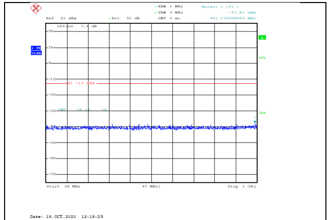
Band2-5MHz-16QAM-19175-1RB#0-Range1:30~1000MHz--37.81-PASS
