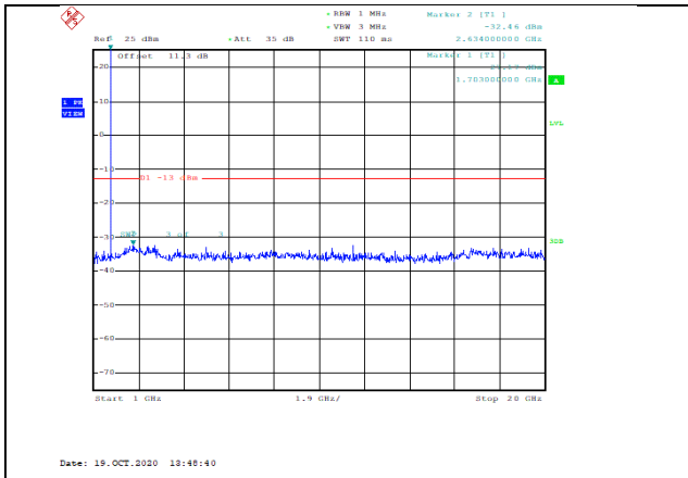
Band4-10MHz-16QAM-20000-1RB#0-Range2:1000~20000MHz--32.46-PASS
