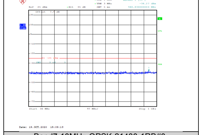
Band7-10MHz-QPSK-21400-1RB#0-Range1:30~1000MHz--38.27-PASS
