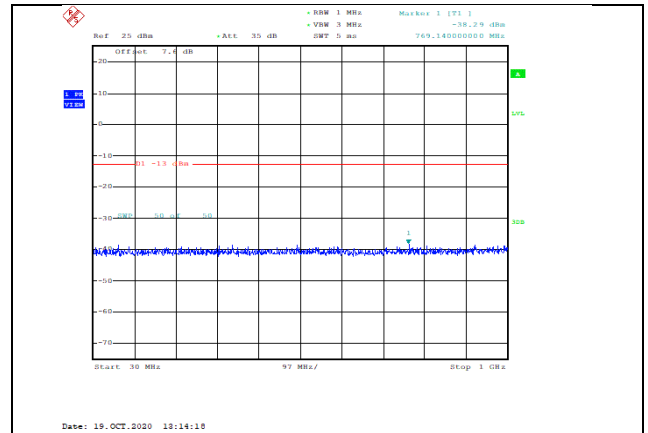
Band2-3MHz-QPSK-19185-1RB#0-Range1:30~1000MHz--38.29-PASS
