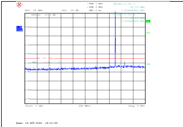
Band7-5MHz-QPSK-20775-1RB#0-Range2:1000~3000MHz--31.73-PASS
