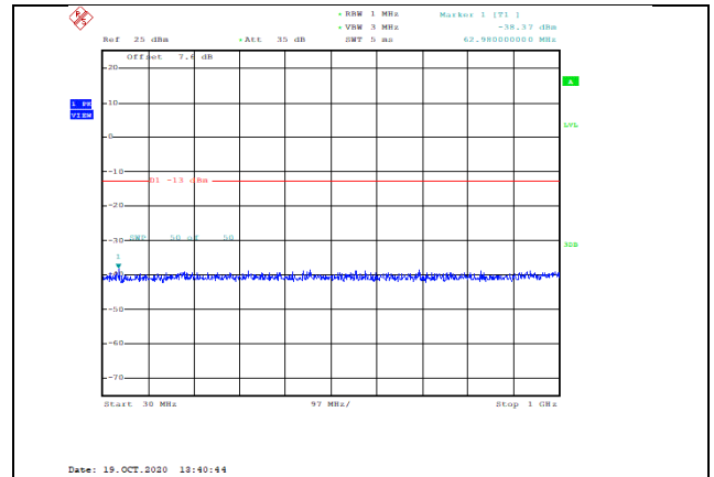
Band2-20MHz-QPSK-19100-1RB#0-Range1:30~1000MHz--38.37-PASS
