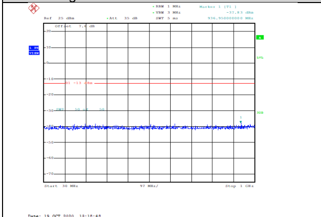
Band2-5MHz-16QAM-18900-1RB#0-Range1:30~1000MHz--37.83-PASS
