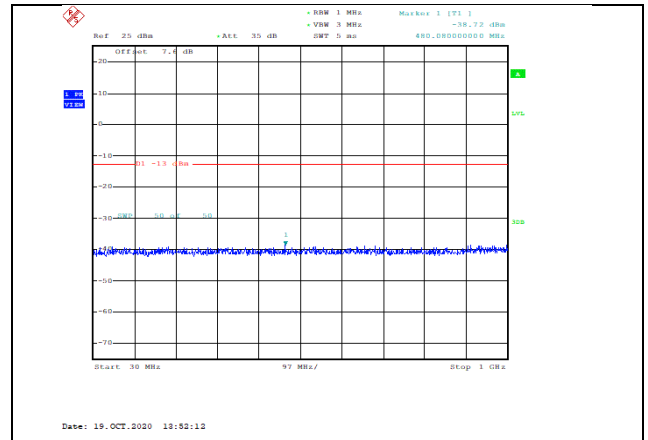
Band4-15MHz-16QAM-20325-1RB#0-Range1:30~1000MHz--38.72-PASS
