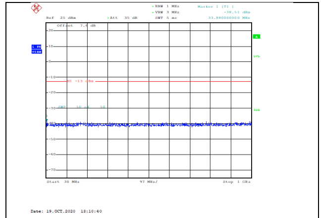
Band2-1.4MHz-QPSK-19193-1RB#0-Range1:30~1000MHz--38.51-PASS
