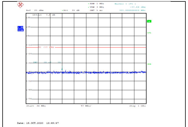
Band4-10MHz-16QAM-20350-1RB#0-Range1:30~1000MHz--37.88-PASS
