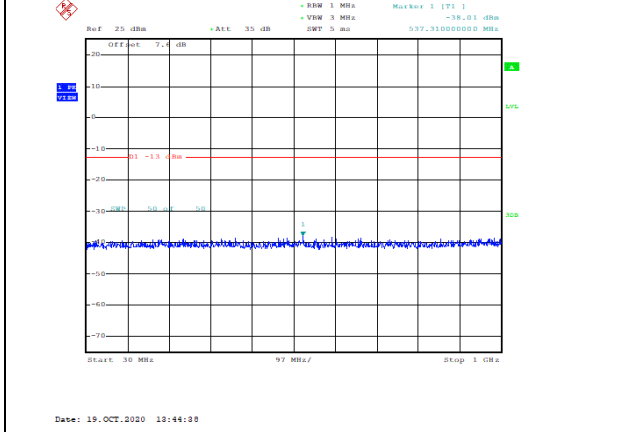
Band4-3MHz-16QAM-20175-1RB#0-Range1:30~1000MHz--38.01-PASS
