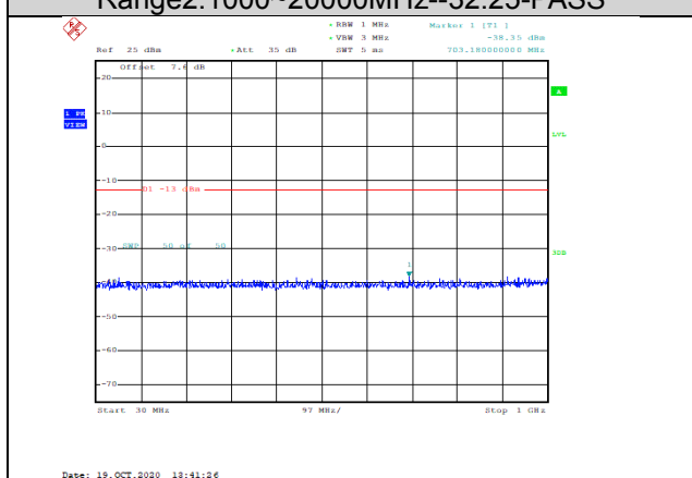
Band4-1.4MHz-QPSK-19957-1RB#0-Range1:30~1000MHz--38.35-PASS
