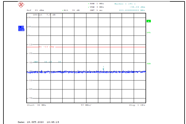
Band4-3MHz-16QAM-20385-1RB#0-Range1:30~1000MHz--38.28-PASS
