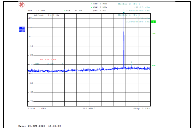
Band7-5MHz-16QAM-21425-1RB#0-Range2:1000~3000MHz--31.23-PASS
