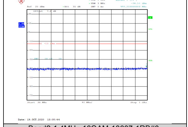
Band2-1.4MHz-16QAM-18607-1RB#0-Range1:30~1000MHz--38.51-PASS
