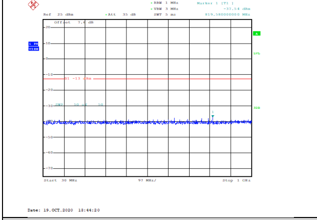
Band4-3MHz-QPSK-20175-1RB#0-Range1:30~1000MHz--37.54-PASS
