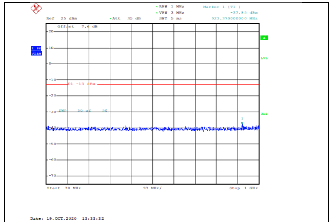
Band2-15MHz-QPSK-19125-1RB#0-Range1:30~1000MHz--37.85-PASS
