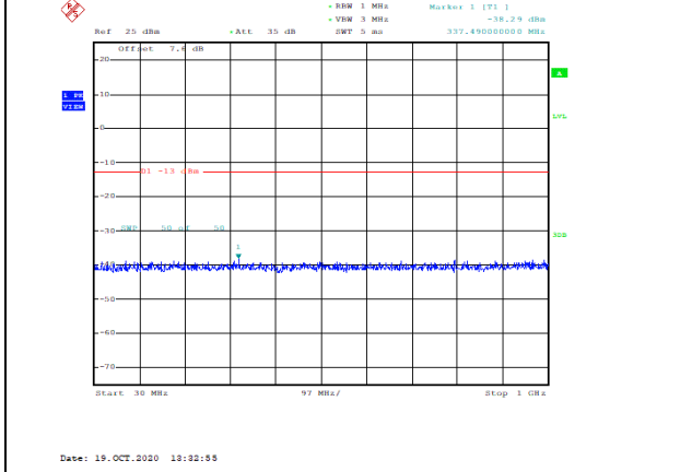
Band2-15MHz-QPSK-18900-1RB#0-Range1:30~1000MHz--38.29-PASS
