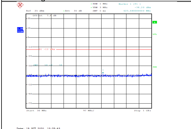
Band2-10MHz-QPSK-18900-1RB#0-Range1:30~1000MHz--38.2-PASS
