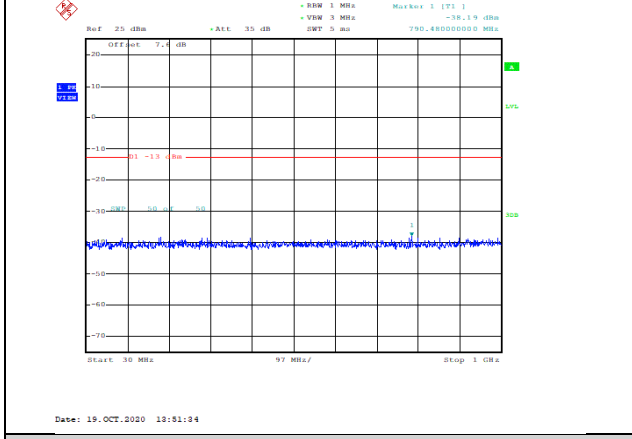
Band4-15MHz-16QAM-20175-1RB#0-Range1:30~1000MHz--38.19-PASS
