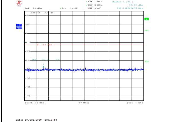
Band2-3MHz-16QAM-18900-1RB#0-Range1:30~1000MHz--38.08-PASS
