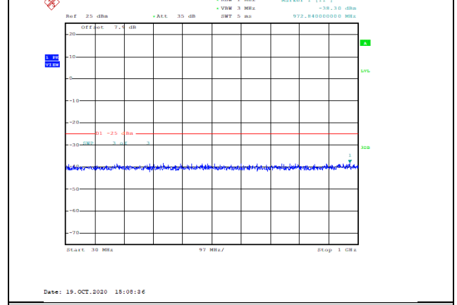
Band7-10MHz-16QAM-21100-1RB#0-Range1:30~1000MHz--38.3-PASS
