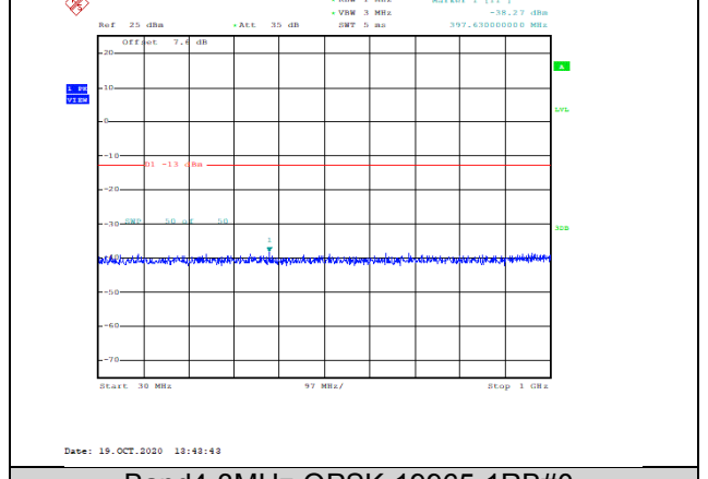
Band4-3MHz-QPSK-19965-1RB#0-Range1:30~1000MHz--38.27-PASS
