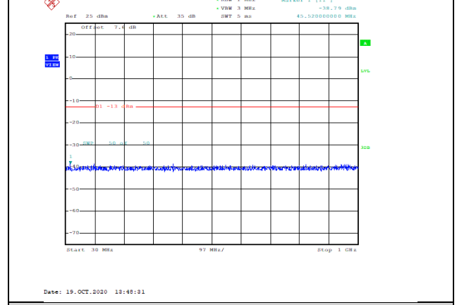
Band4-10MHz-16QAM-20000-1RB#0-Range1:30~1000MHz--38.79-PASS
