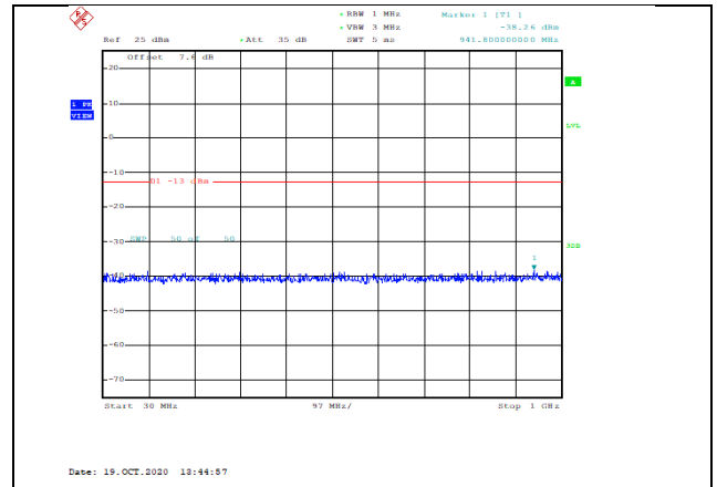
Band4-3MHz-QPSK-20385-1RB#0-Range1:30~1000MHz--38.26-PASS
