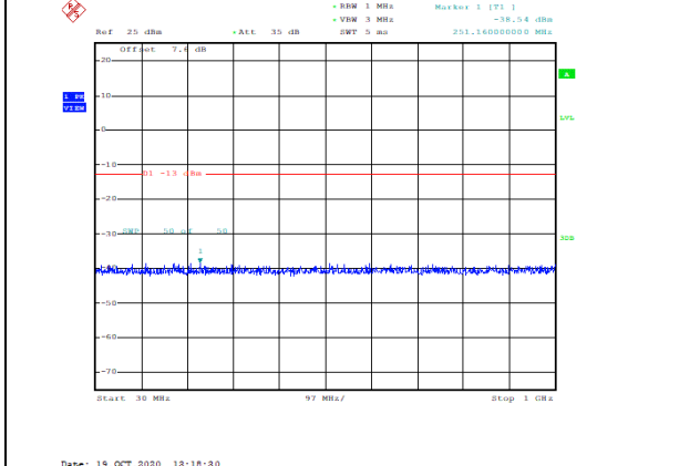
Band2-5MHz-QPSK-18900-1RB#0-Range1:30~1000MHz--38.54-PASS
