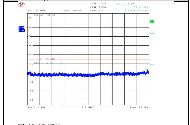
Band7-5MHz-16QAM-20775-1RB#0-Range3:3000~26000MHz--37.31-PASS
