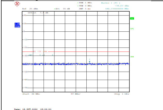
Band7-5MHz-16QAM-20775-1RB#0-Range1:30~1000MHz--38.03-PASS
