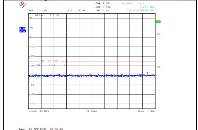
Band7-5MHz-16QAM-21100-1RB#0-Range1:30~1000MHz--37.95-PASS
