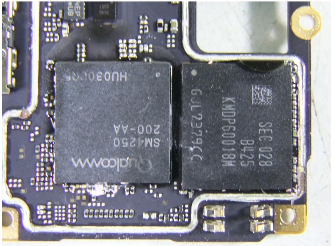
Photo 14 Inside of EUT
