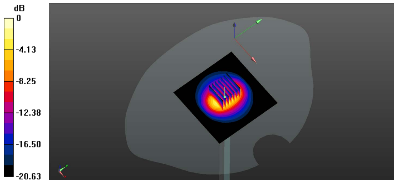
0 dB = 5.73 W/kg
