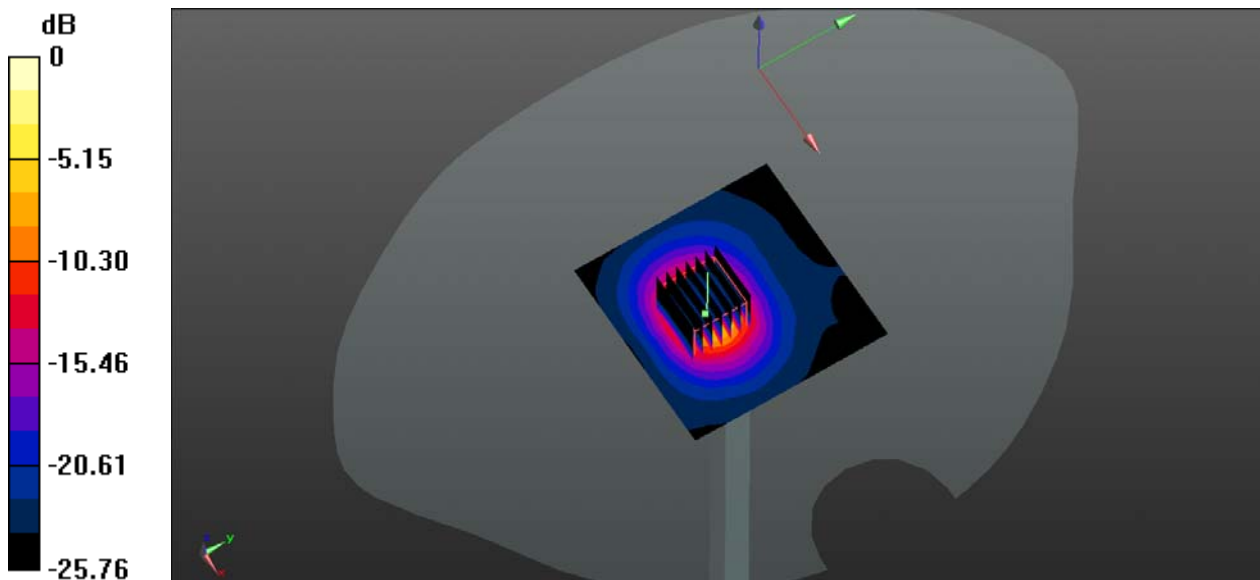
0 dB = 17.2 W/kg
