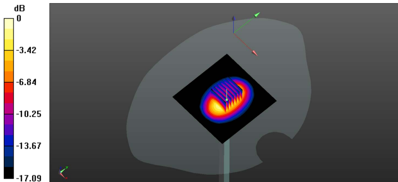
0 dB = 4.36 W/kg
