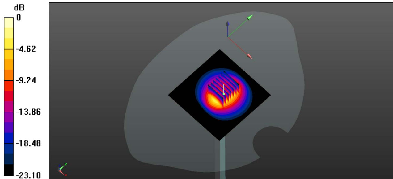
0 dB = 6.33 W/kg
